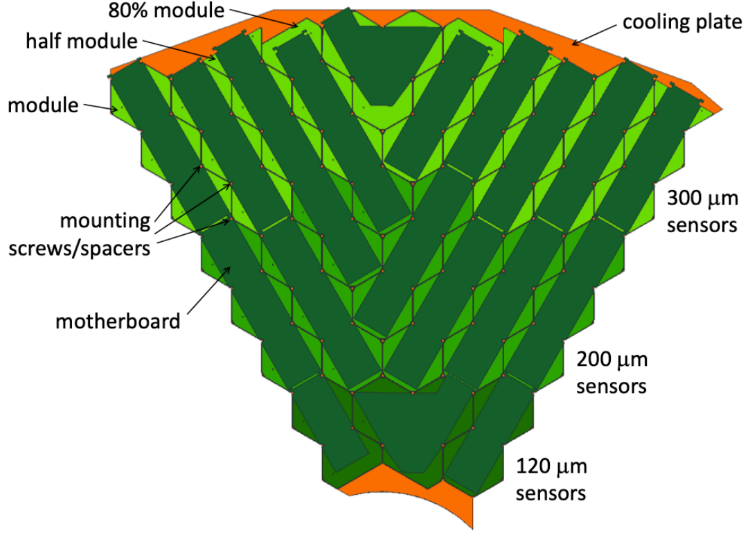
Figure 6.8. HGCal cassette structure.
