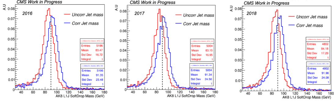
Figure 4.3. Distribution of the AK8 leading jet soft-drop mass before (red) and after (blue) correction. From left to right: signal sample (1 TeV VBF Gravtation) for 2016, 2017, and 2018.
