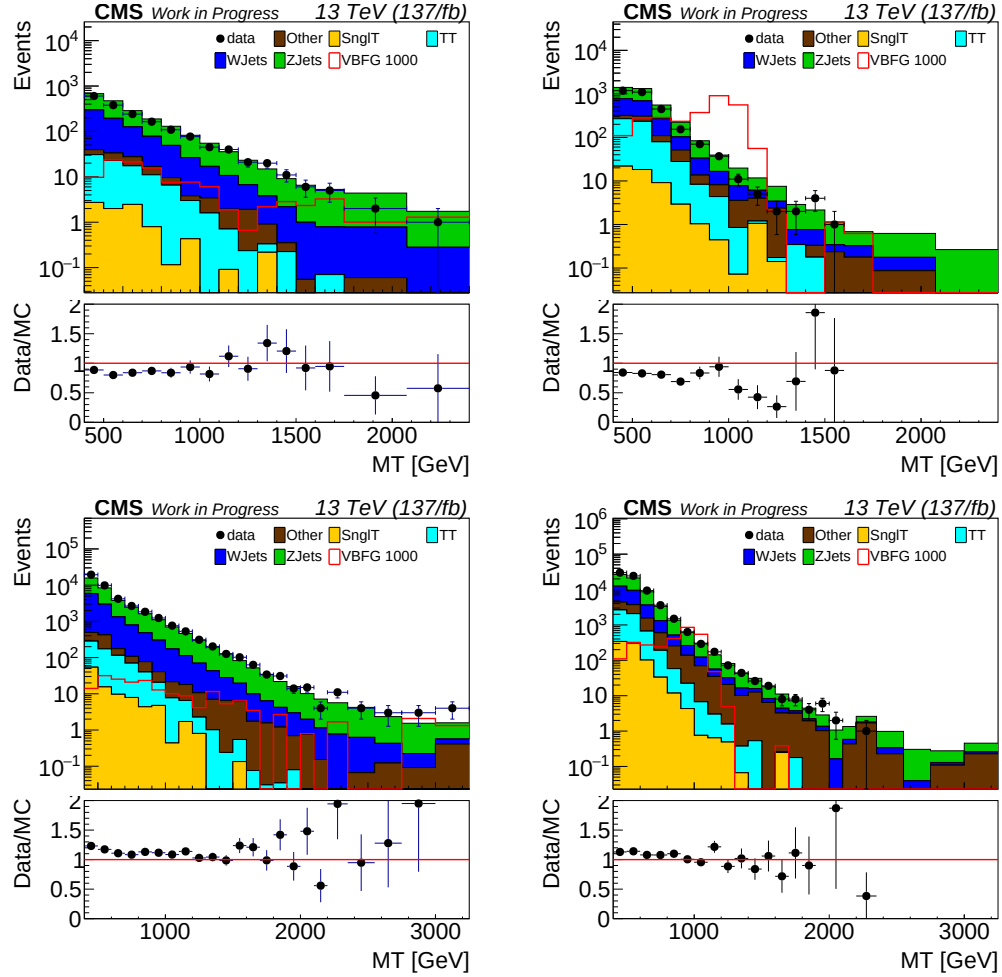
Figure 5.16. Distribution for the search variable m_T for VBF (top) and VBFfail (bottom) category. Last bin corresponds to the overflow bin. Left: High purity side band region, right: High purity signal region
