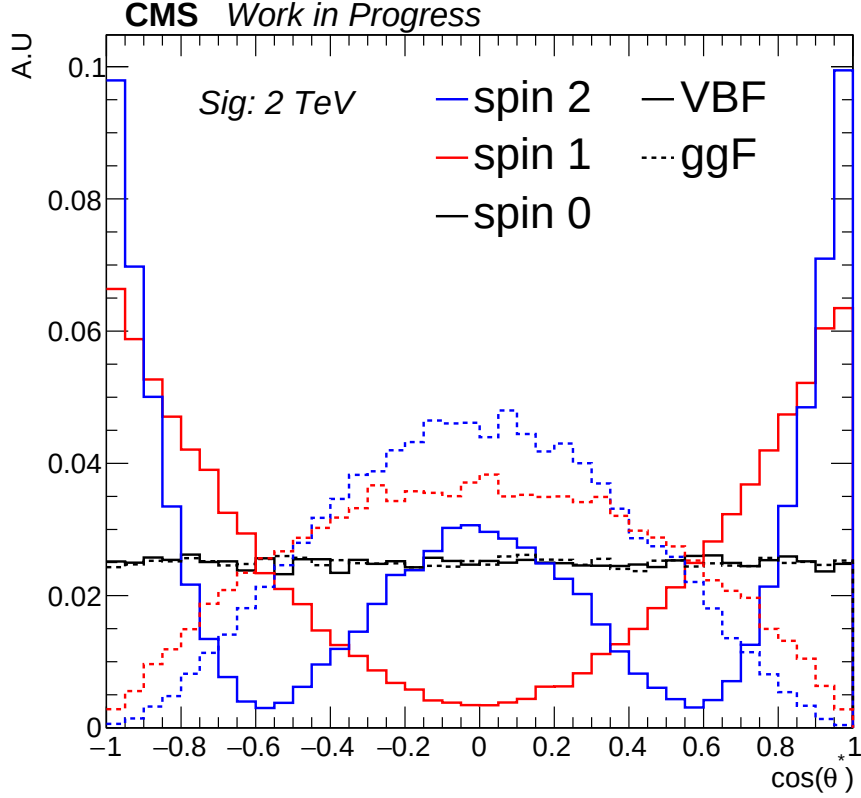
Figure 5.3. Distribution of the production polar angle for various VBF (solid line) and ggF-produced (dashed line) resonances decaying to WZ/ZZ bosons.
