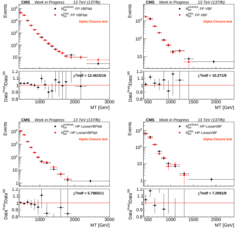
Figure 5.20. Alpha closure test after loosening few selections. From top to bottom: after loosening \tau_{21} cut, VBF cuts. Left: for events that failed the VBF selection, right: for events passing VBF selection
