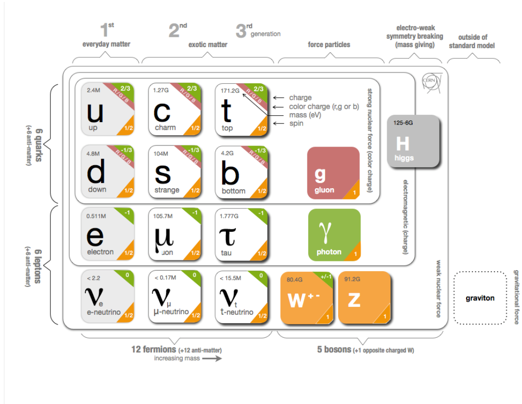
Figure 2.1. The Standard Model of the particle physics.
