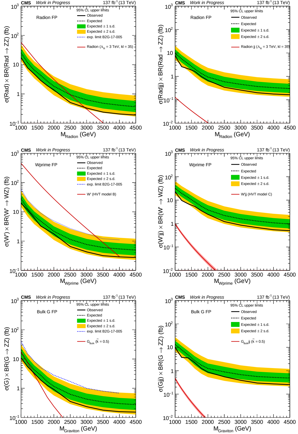
Figure 5.29. Expected 95% CL upper limit on \sigma \times BR(X \rightarrow WZ/ZZ) for spin 0, 1, and 2 (top to bottom) after combining the VBF-pass, VBF-fail, high, and low purity category using the ggF samples (left) and VBF samples (right).
