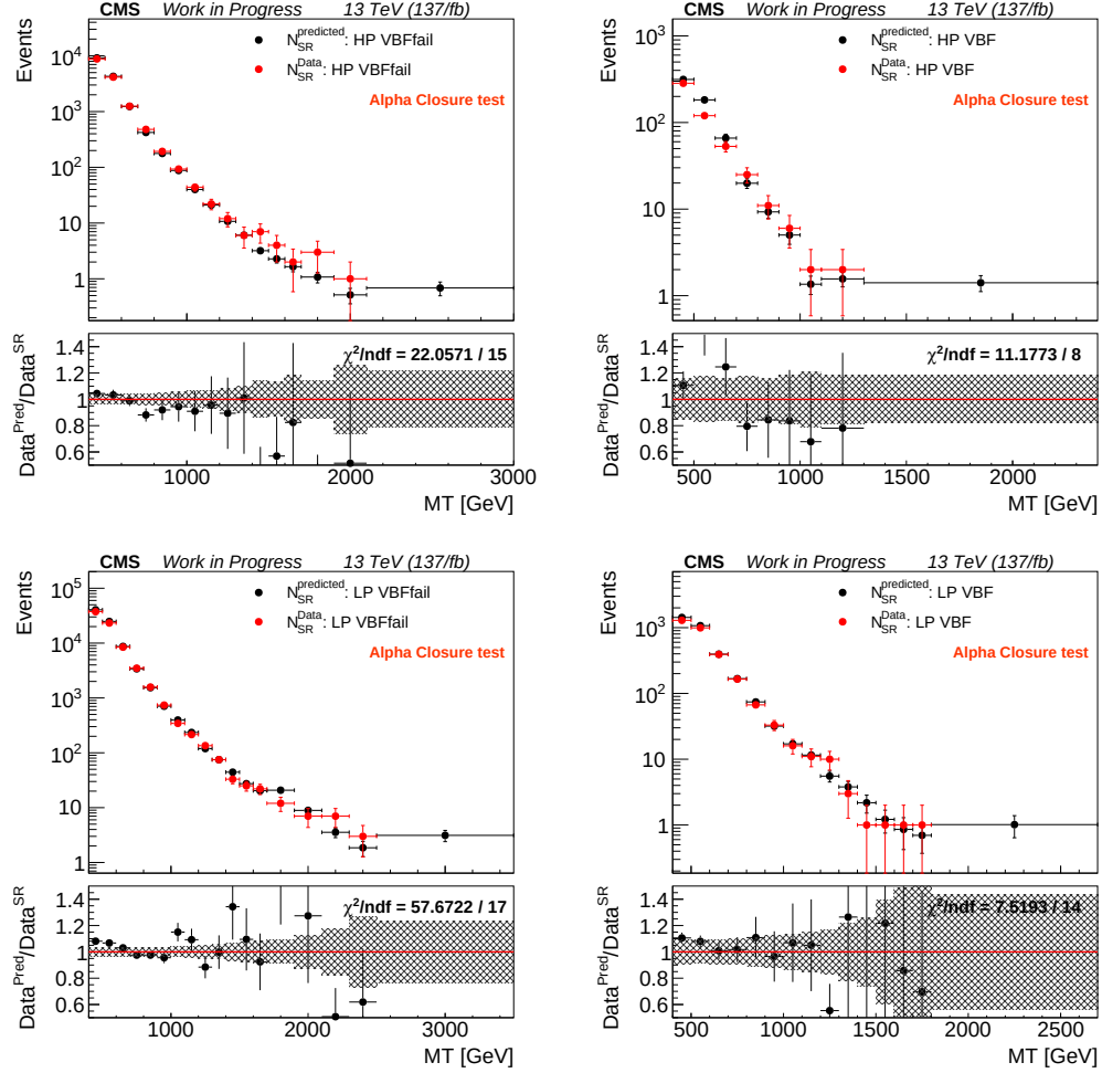
Figure 5.19. Distributions for predicted data in SR in high (top) and low (bottom) purity category. Black and red dots represent the predicted events in SR and the data in the SR (pseudo) respectively. Ratio of prediction in SR to data in SR is shown at the bottom which is \sim 1 . Left: For VBF-fail event, right: For VBF-pass event. The hashed region in the ratio panel corresponds to the total uncertainty on the prediction in the true signal region.
