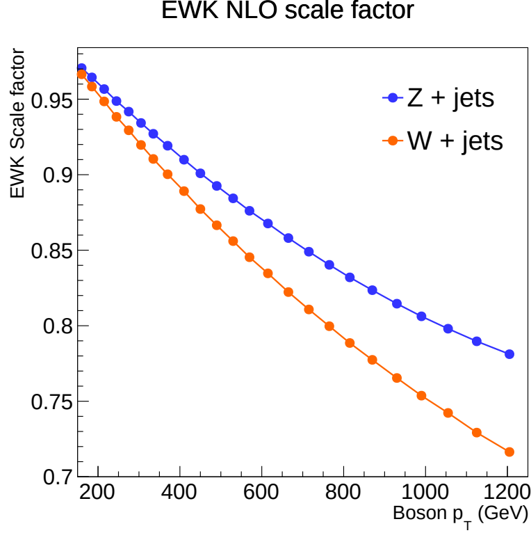
Figure 5.1. EWK NLO scale factors as a function of boson p_T .
