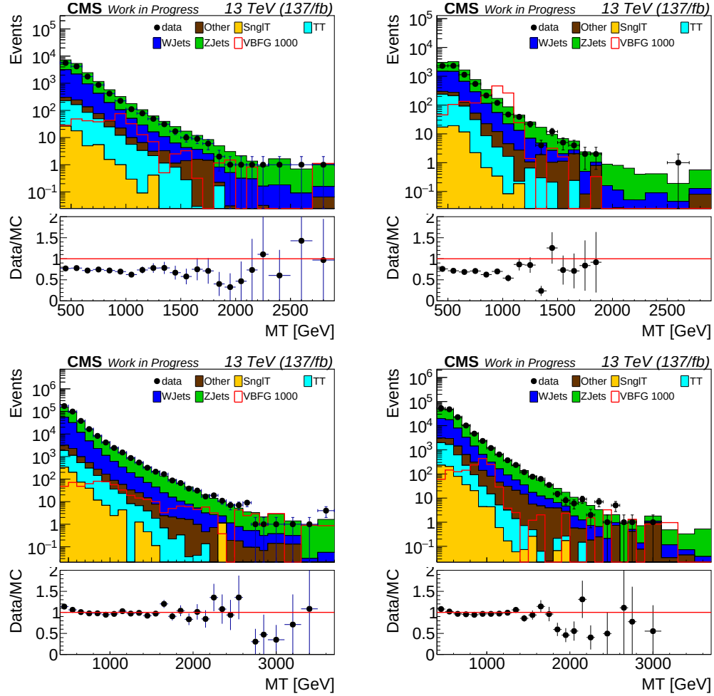
Figure 5.17. Distribution for the search variable m_T for VBF (top) and VBFfail (bottom) category. Last bin corresponds to the overflow bin. Left: Low purity side band region, right: Low purity signal region
