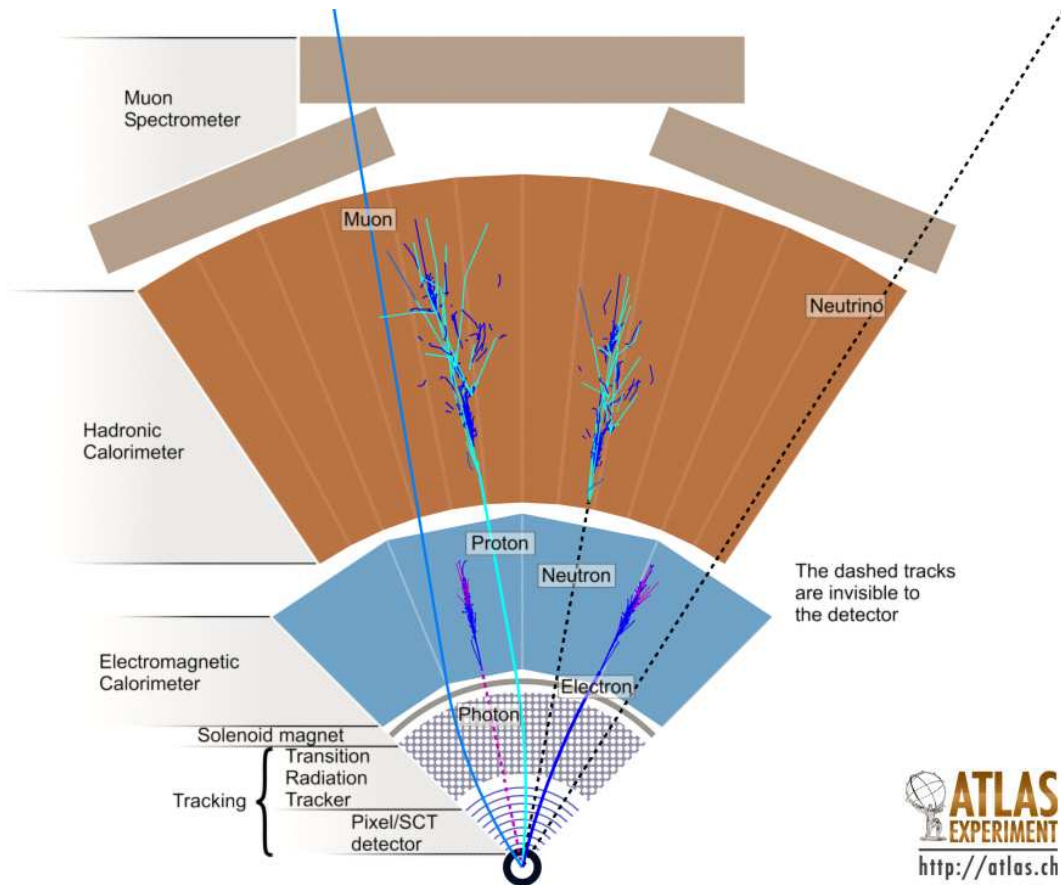
Figure 3.4: Schematic view of the specialized particle detectors of ATLAS and sketch of an event cross section. Not drawn: the toroid magnets between the hadronic calorimeter and the muon spectrometer; the radiation shields. [39]
