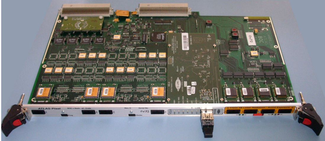
Figure 4.4: A Back Of Crate Card card in pixel assembly (Layer-2). [11]
