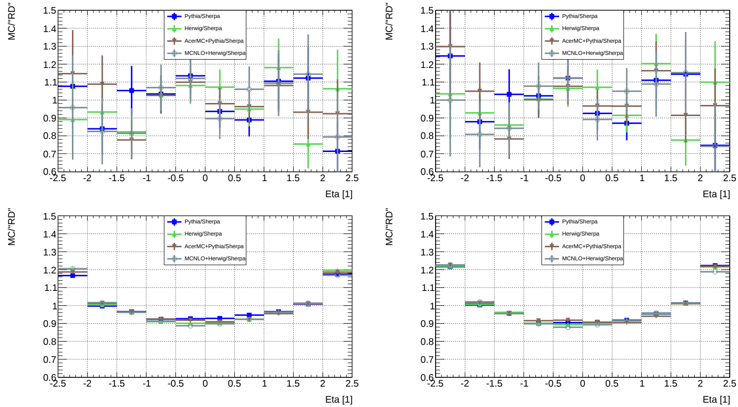
Figure B.5: Pseudrapidity of electrons in semileptonic t\bar{t} events for four common Monte Carlo generators relative to pseudo data (Shepra arbitrarily chosen). At the top: reconstructed events with cuts, at the bottom: generated events without cuts. At the left: before reweighting, at the right: after reweighting.
