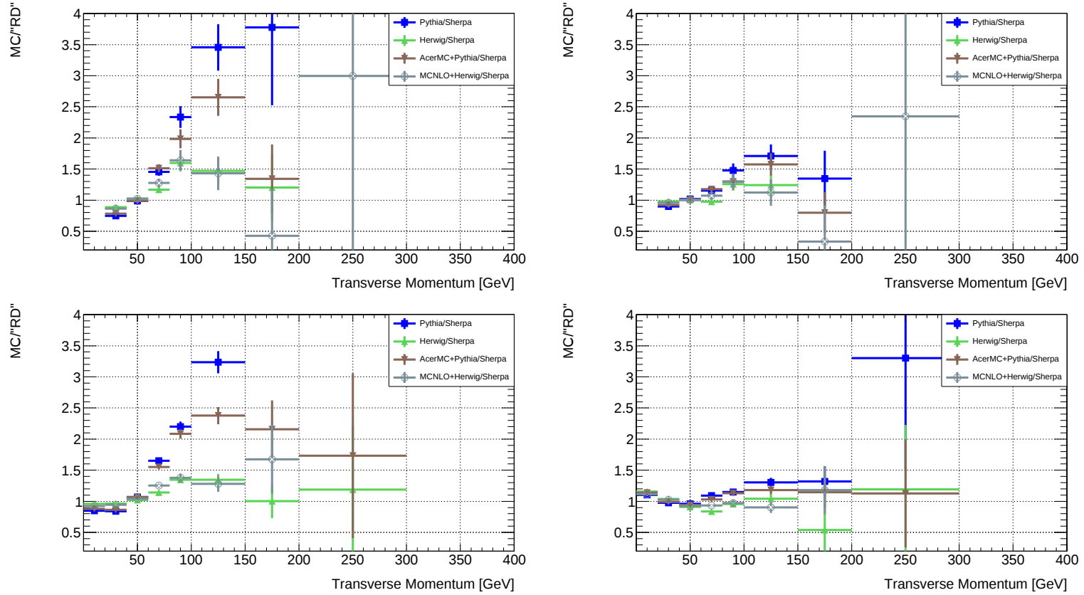
Figure B.14: Transverse momentum of the fourth leading jet in semileptonic t\bar{t} events for four common Monte Carlo generators relative to pseudo data (Sherpa arbitrarily chosen). At the top: reconstructed events with cuts, at the bottom: generated events without cuts. At the left: before reweighting, at the right: after reweighting.
