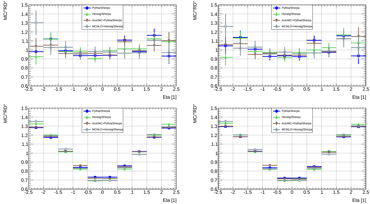
Figure B.7: Pseudorapidity of muons in semileptonic t\bar{t} events for four common Monte Carlo generators relative to pseudo data (Shepra arbitrarily chosen). At the top: reconstructed events with cuts, at the bottom: generated events without cuts. At the left: before reweighting, at the right: after reweighting.
