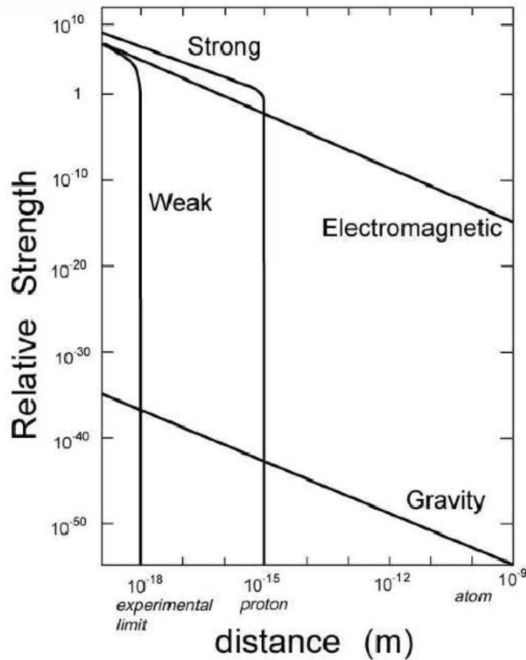
Figure 2.1: The relative strenghts of the four fundamental forces in dependence of the distance. The current experimental limit is noted as well. [3]
