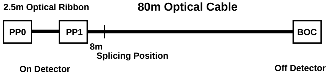
Figure 4.7: The ATLAS pixel optical connection between OBs and BOC cards.
