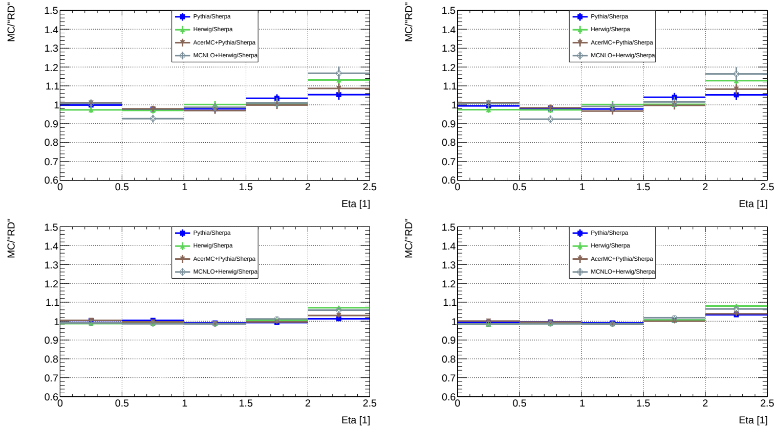
Figure B.9: Pseudorapidity of jets in semileptonic t\bar{t} events for four common Monte Carlo generators relative to pseudo data (Shepra arbitrarily chosen). At the top: reconstructed events with cuts, at the bottom: generated events without cuts. At the left: before reweighting, at the right: after reweighting.
