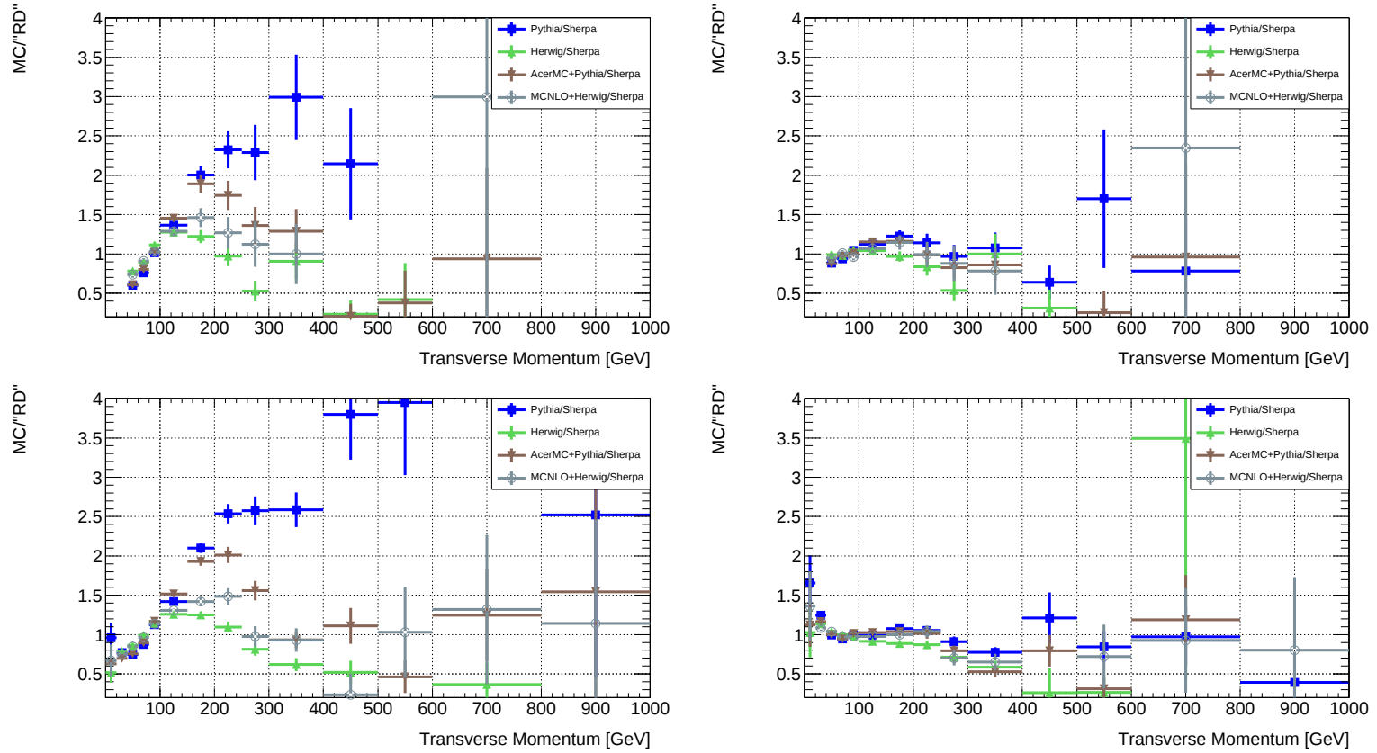
Figure B.12: Transverse momentum of the second leading jet in semileptonic t\bar{t} events for four common Monte Carlo generators relative to pseudo data (Sherpa arbitrarily chosen). At the top: reconstructed events with cuts, at the bottom: generated events without cuts. At the left: before reweighting, at the right: after reweighting.
