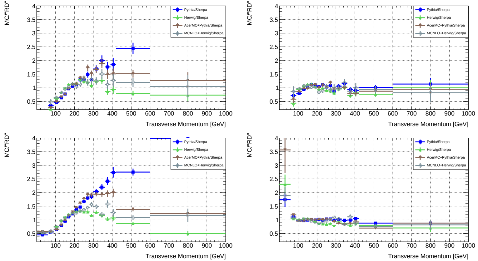
Figure B.2: Transverse momentum of the hadronically decaying top quark in semileptonic t\bar{t} events for four common Monte Carlo generators relative to pseudo data (Sherpa arbitrarily chosen). At the top: reconstructed events with cuts, at the bottom: generated events without cuts. At the left: before reweighting, at the right: after reweighting.
