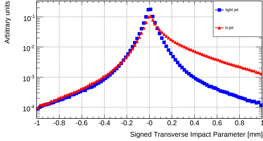
Figure 6.3: Signed transverse track impact parameter distribution for b - (red) and light (blue) jets in t\bar{t} events.
