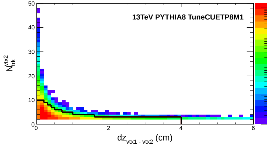
Figure 6.3 : the longitudinal displacement ( dz ) between additional primary vertices and the lead primary vertex versus the number of tracks ( N_{trk}^{vx2} ) associated with the additional primary vertex for the pythia8 MinBias sample.
