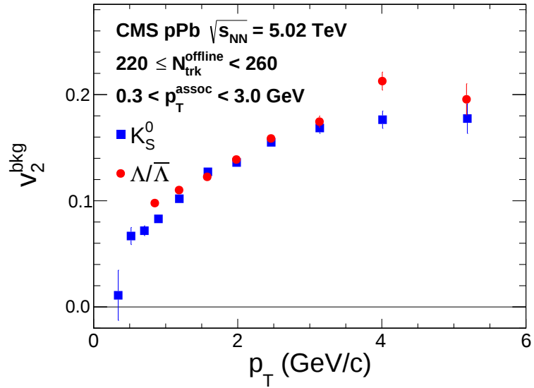
Figure 7.6 : v_2^{\text{bkg}} values for K_S^0 and \Lambda/\bar{\Lambda} as a function of p_T in 5 TeV pPb collisions for 220 \leq N_{\text{trk}}^{\text{offline}} < 260 .
