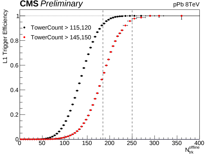
Figure 3.7 : Efficiency of L1 tower count triggers for 8 TeV pPb collisions. Vertical dash lines indicate the region of events used for analysis.
