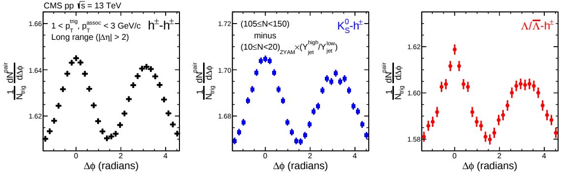
Figure 9.3 : The 1D \Delta\phi correlation functions for the long-range regions in the multiplicity range 105 \leq N_{\text{trk}}^{\text{offline}} < 150 of pp collisions at \sqrt{s} = 13 TeV, after subtracting scaled results from 10 \leq N_{\text{trk}}^{\text{offline}} < 20 with the ZYAM procedure applied. A selection of 1–3 GeV/c for both p_T^{\text{trig}} and p_T^{\text{assoc}} is used in all cases.
