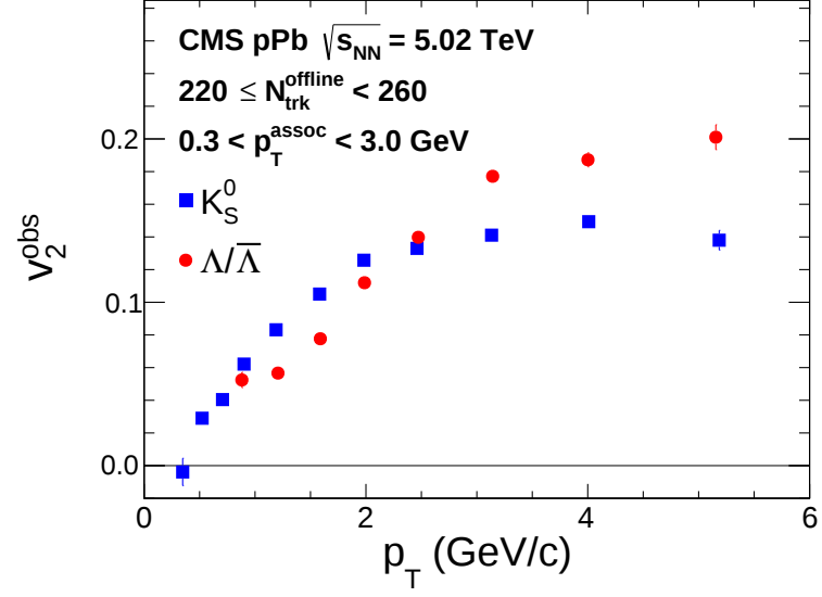
Figure 7.5 : v_2^{\text{obs}} values for K_S^0 and \Lambda/\bar{\Lambda} as a function of p_T in 5 TeV pPb collisions for 220 \leq N_{\text{trk}}^{\text{offline}} < 260 .
