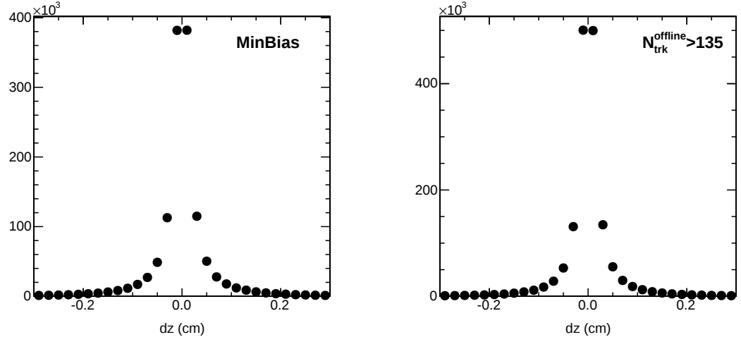
Figure 6.5 : Longitudinal displacement ( dz ) between the primary vertex and tracks selected by standard track selection described in Sec. 5.1.2 for 13 TeV pp data for MinBias events (left) and events with N_{\text{trk}}^{\text{offline}} > 135 triggered by HLT_PixelTracks_Multiplicity110 (right).
