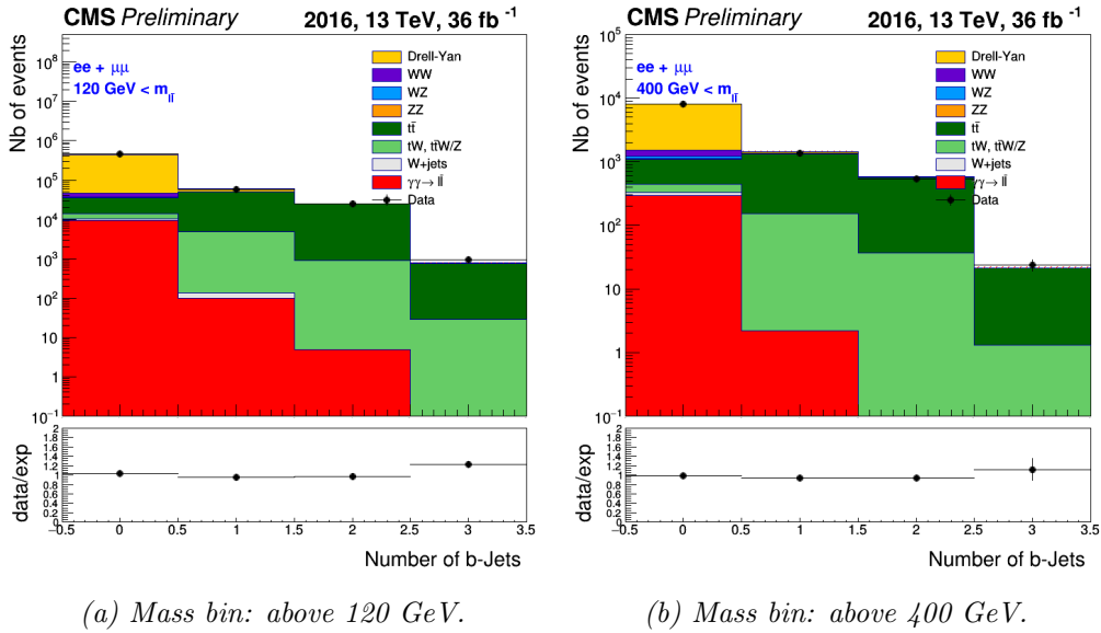
Figure 4.6 – Distributions of the number of b -jets for different mass bins (2016 data).
