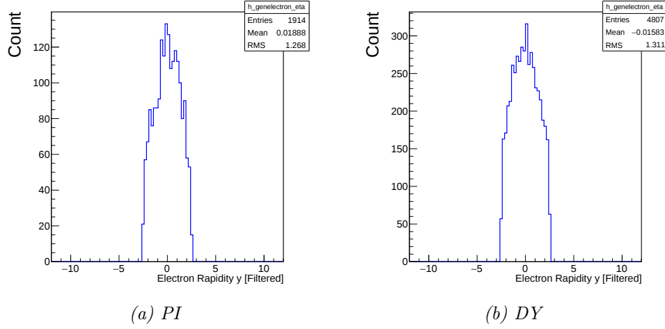
Figure C.2 – The electron \eta distributions, M_{\ell\bar{\ell}} > 60 GeV with acceptance cuts.
