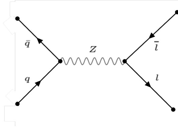
Figure A.3 – The frame to describe the Drell-Yan process.
