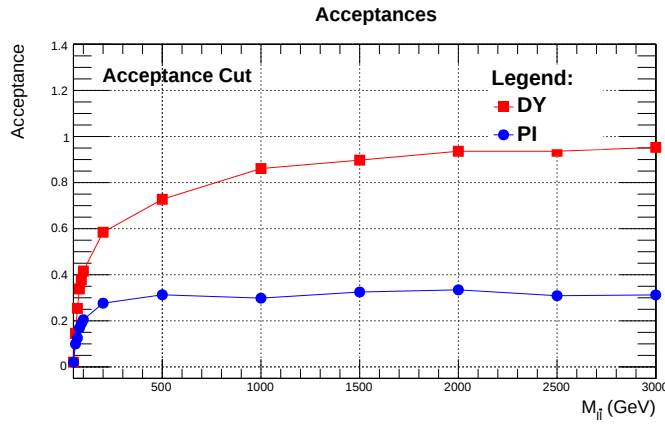
Figure 3.10 – The acceptance cut ratios for the DY (red) and PI (blue).
