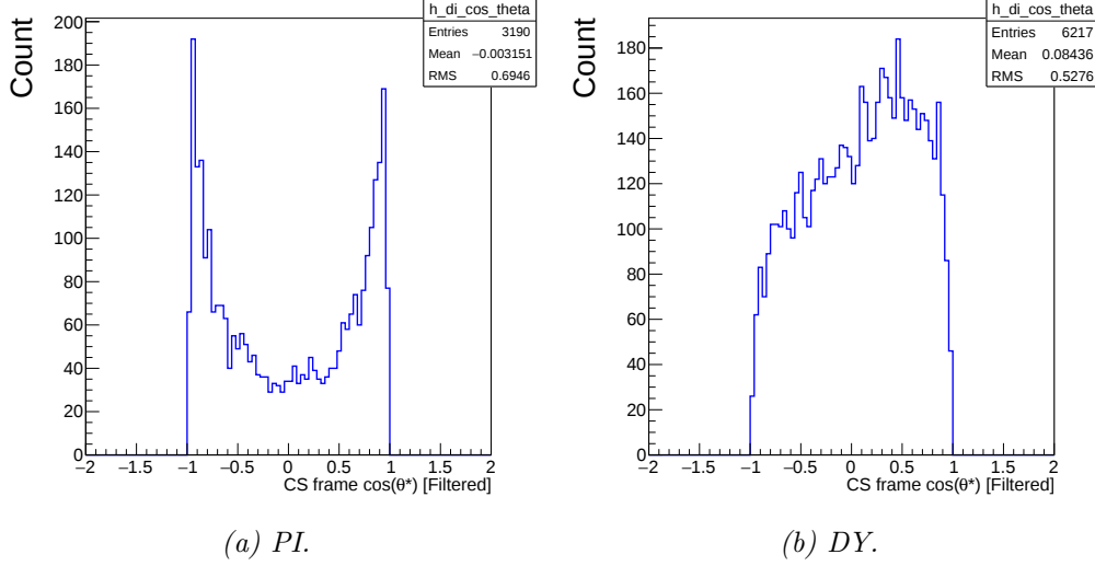
Figure 3.7 – The \cos\theta_{CS} distributions with M_{l\bar{l}} \in [200, 400] GeV and with acceptance cuts.
