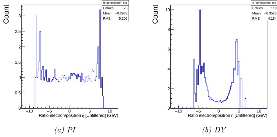
Figure C.5 – The ratio e^-/e^+ as a function of \eta , M_{l\bar{l}} \in [200, 400] GeV without acceptance cuts. The border of the distributions are impacted by low statistics.
