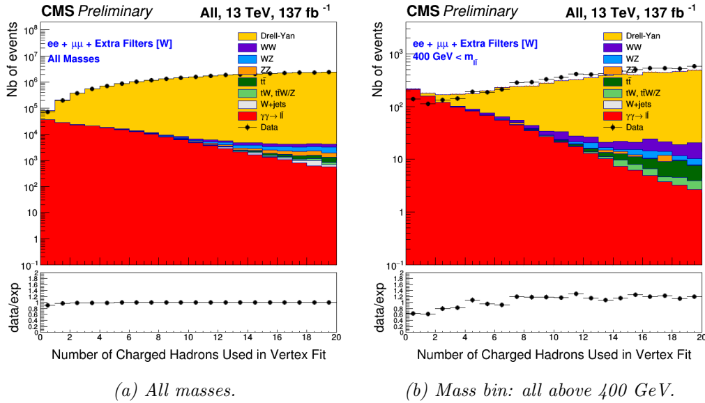
Figure 5.1 – The nCH -weighed filtered number of charged hadrons from the vertex fit distributions for two different mass bins (Run II data).
