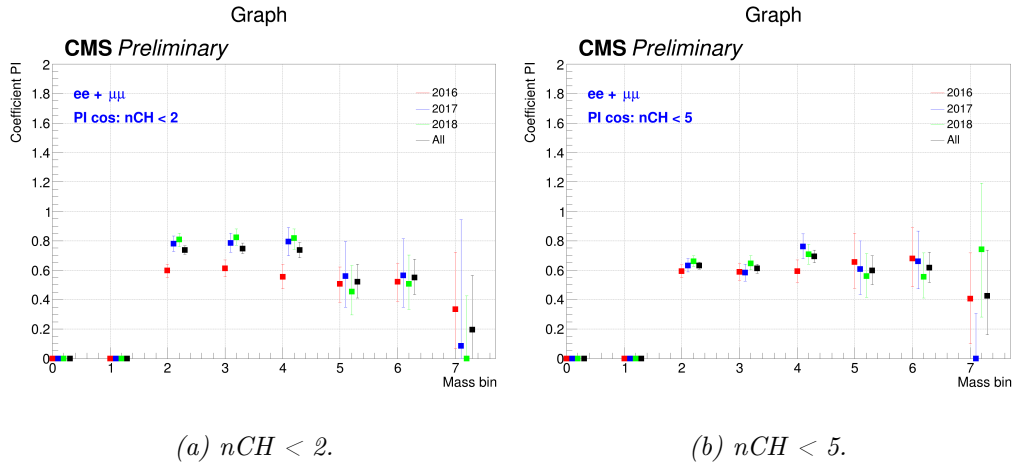
Figure 5.9 – The PI fitting weights for the \cos\theta_{CS} distributions for all mass bins (except 0 and 1), all years.
