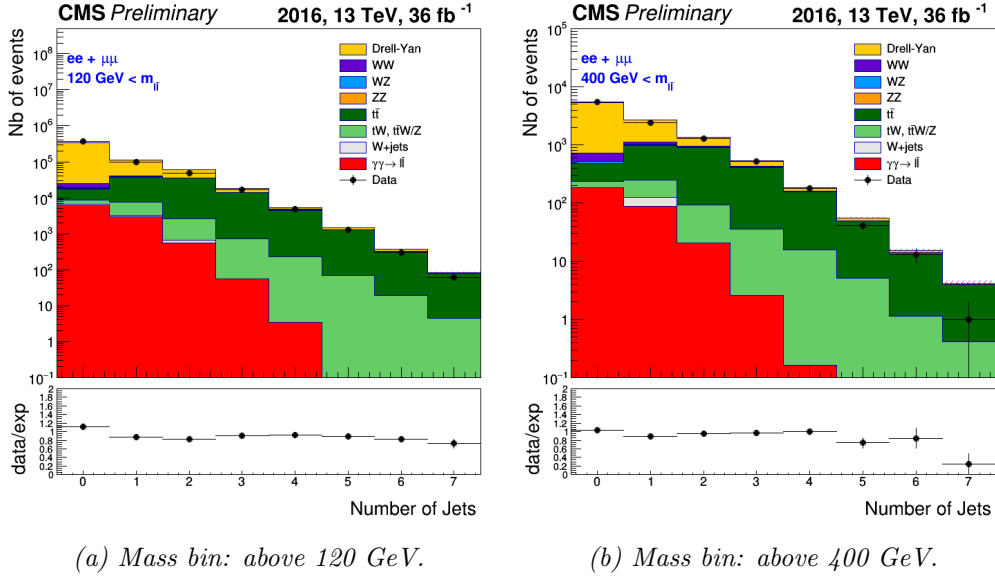
Figure 4.5 – Distributions of the number of jets for different mass bins (2016 data).
