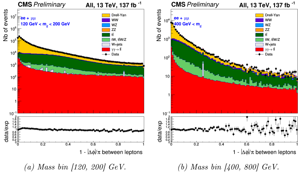
Figure D.2 – The acoplanarity distributions before filters (Run II data).
