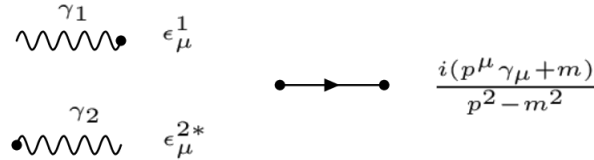
Figure A.4 – Additional Feynman rules for external photon and spinor propagator of mass m .
