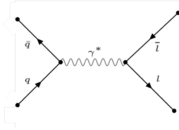
Figure A.2 – The frame to describe the Drell-Yan process.
