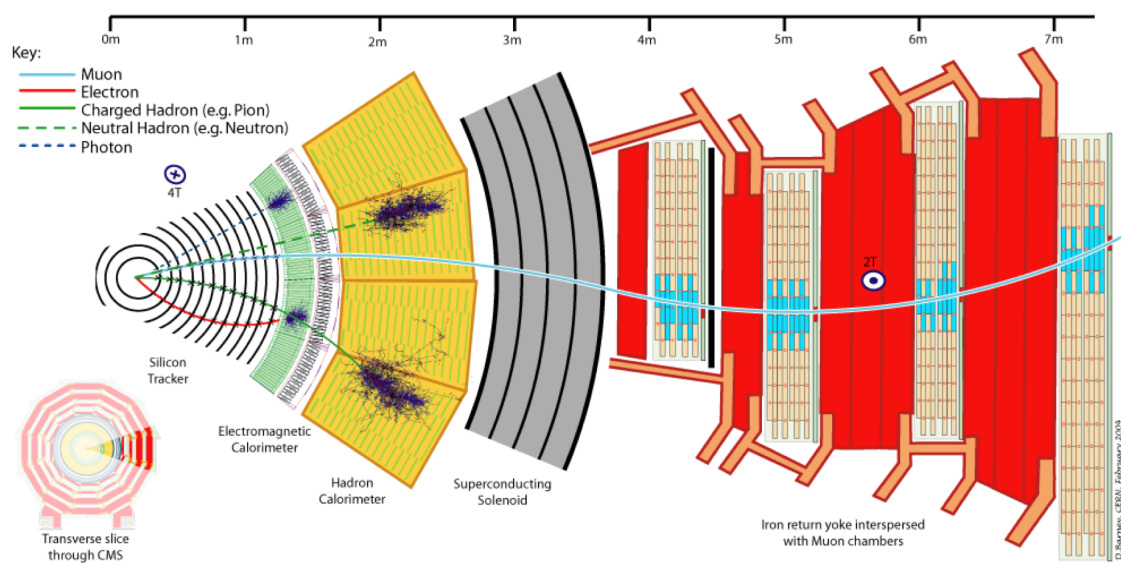
Figure 2.5 – A transverse slice of the CMS experiment with a schematic view of the path of various particles.
