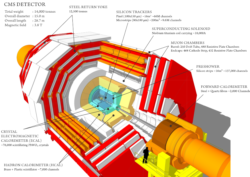
Figure 2.4 – A schematic view of the CMS detector and its various components.
