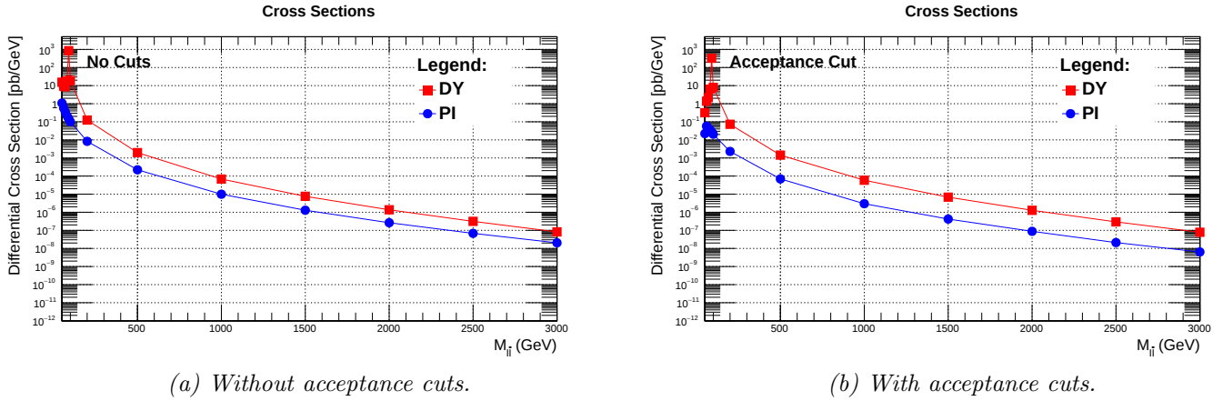
Figure 3.8 – The cross sections for the PI (blue) and DY (red) as a function of M_{l\bar{l}} .
