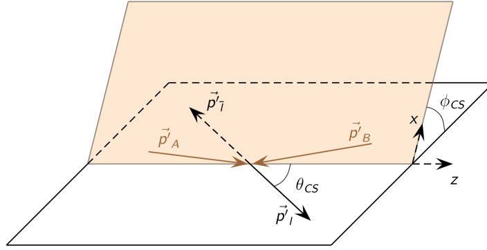
Figure 3.4 – The Collins-Soper frame. The protons momenta are in the orange plane and the leptons are emitted back-to-back in the white plane [15].
