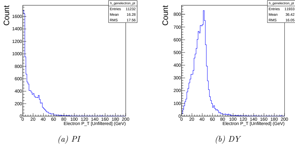
Figure C.11 – The electron p_T distributions, M_{l\bar{l}} > 60 GeV without acceptance cuts.
