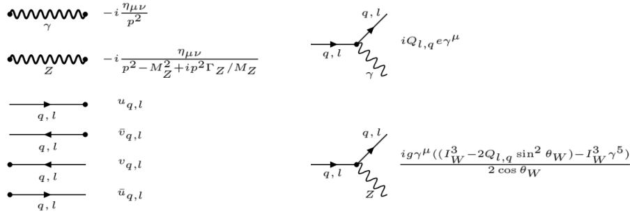
Figure A.1 – The Feynman rules for DY matrix element computation. M_Z and \Gamma_Z are respectively the Z boson mass and total decay width.
