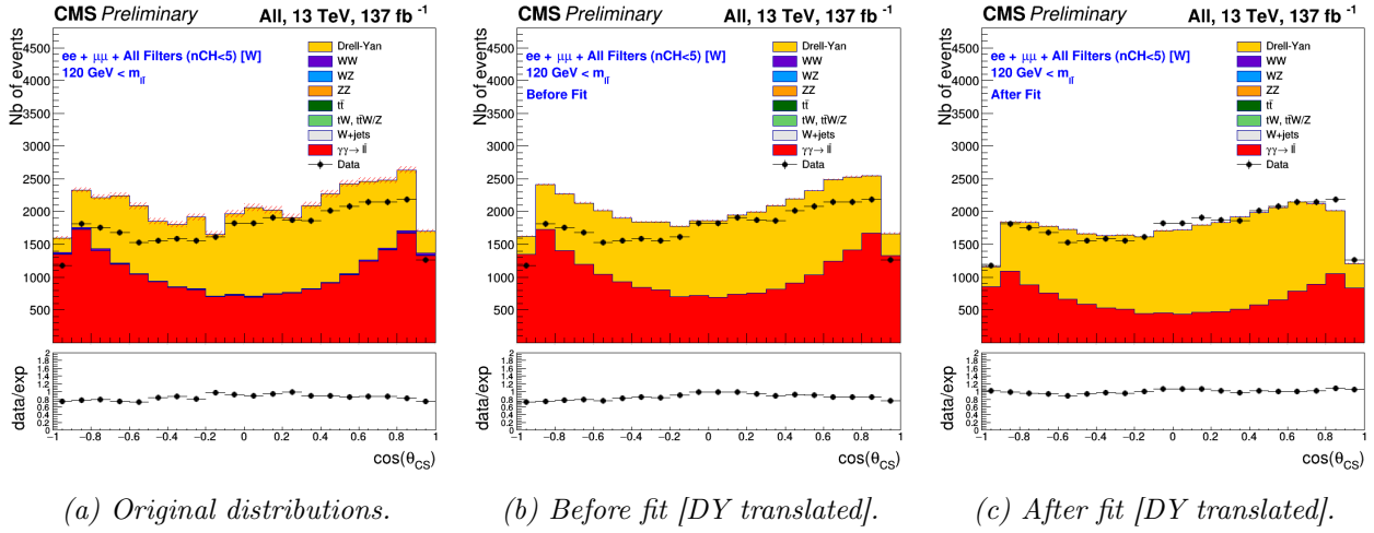
Figure 5.4 – The nCH -weighed \cos\theta_{CS} distributions in the above 120 GeV mass region with nCH < 5 (Run II data).
