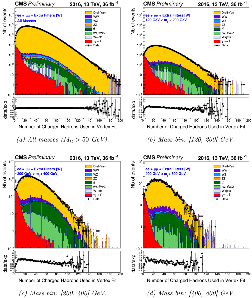
Figure 4.10 – The nCH -weighted filtered number of charged hadrons from the vertex fit distributions for different mass bins (2016 data).
