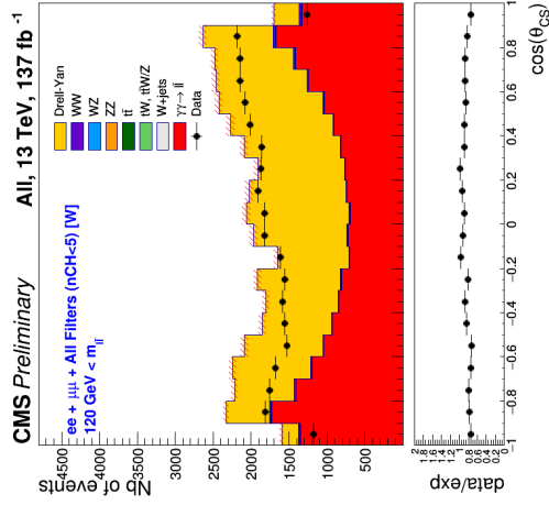
(c) Mass bin: all above 400 GeV.
