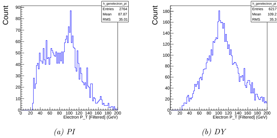
Figure C.14 – The electron p_T distributions, M_{l\bar{l}} \in [200, 400] GeV with acceptance cuts.
