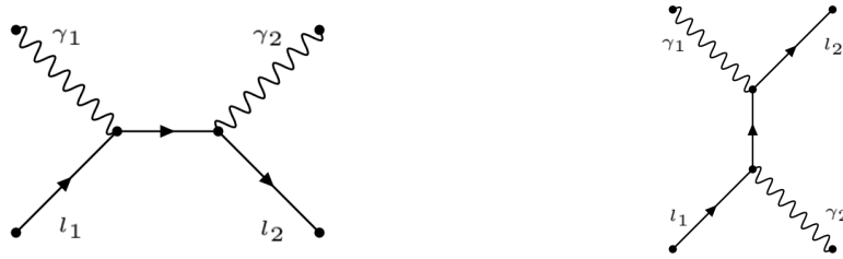
Figure 1.5 – The two tree level diagrams for Compton scattering.
