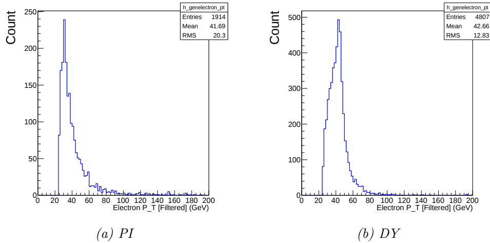
Figure C.12 – The electron p_T distributions, M_{l\bar{l}} > 60 GeV with acceptance cuts.
