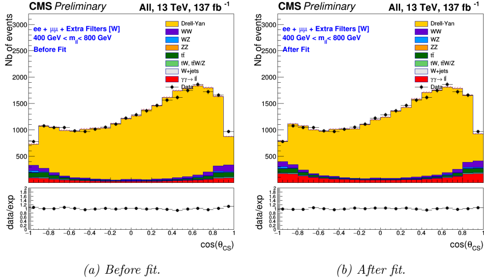
Figure 5.6 – The nCH -weighed \cos\theta_{CS} distributions in the [400, 800] GeV mass region (Run II data).
