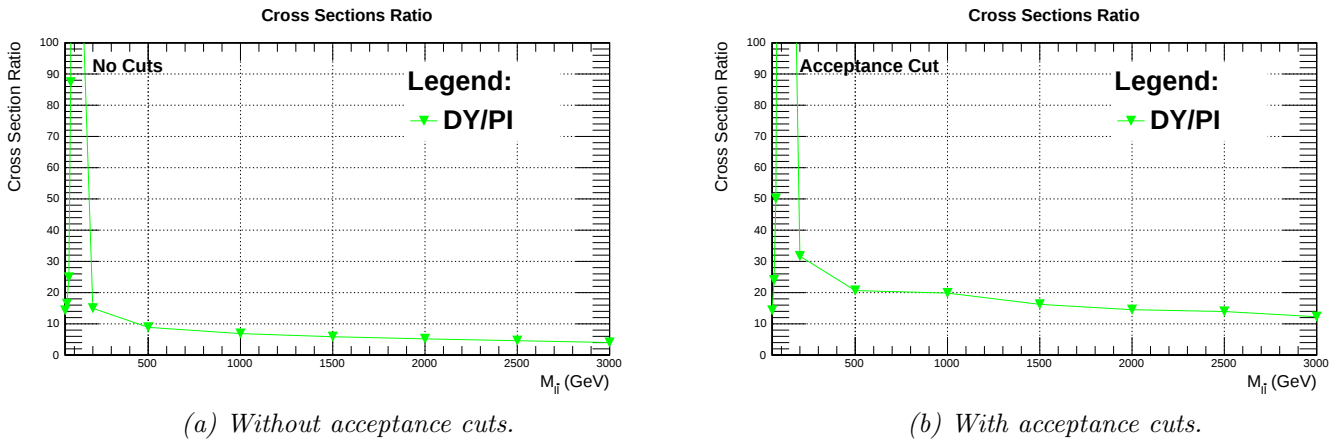
Figure 3.9 – The cross sections ratios DY/PI as a function of M_{l\bar{l}} .
