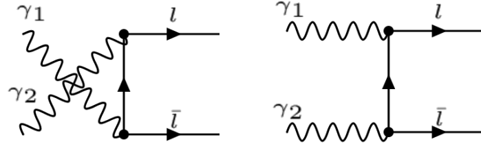
Figure 1.4 – The two tree level diagrams for the photon-induced lepton pair production.
