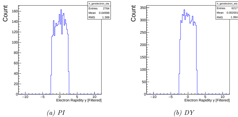
Figure C.4 – The electron \eta distributions, M_{\ell\bar{\ell}} \in [200, 400] GeV with acceptance cuts.
