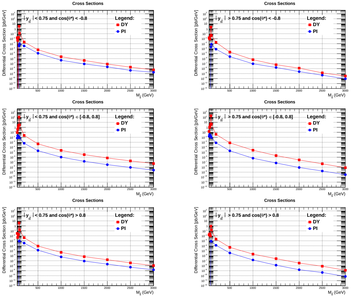
Figure C.17 – Cross sections of the DY (red) and the PI (blue) for the different sets of cuts.
