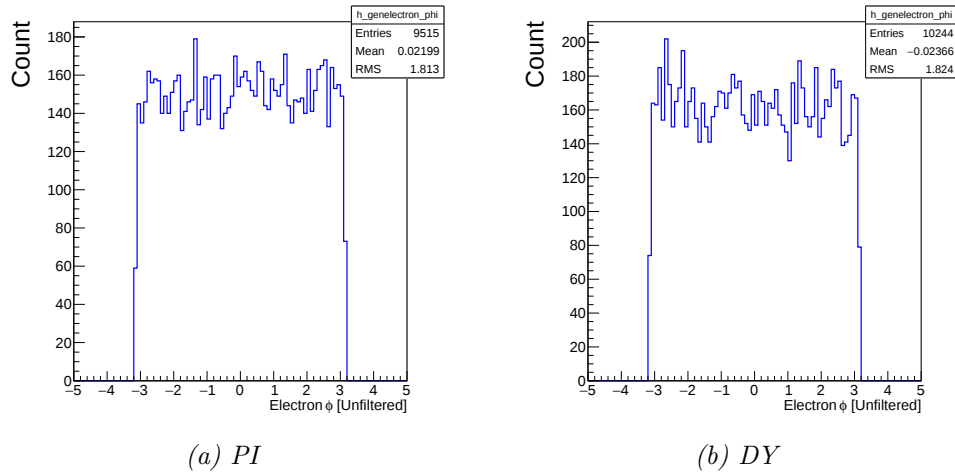
Figure C.9 – The electron \phi distributions, M_{l\bar{l}} \in [200, 400] GeV without acceptance cuts.
