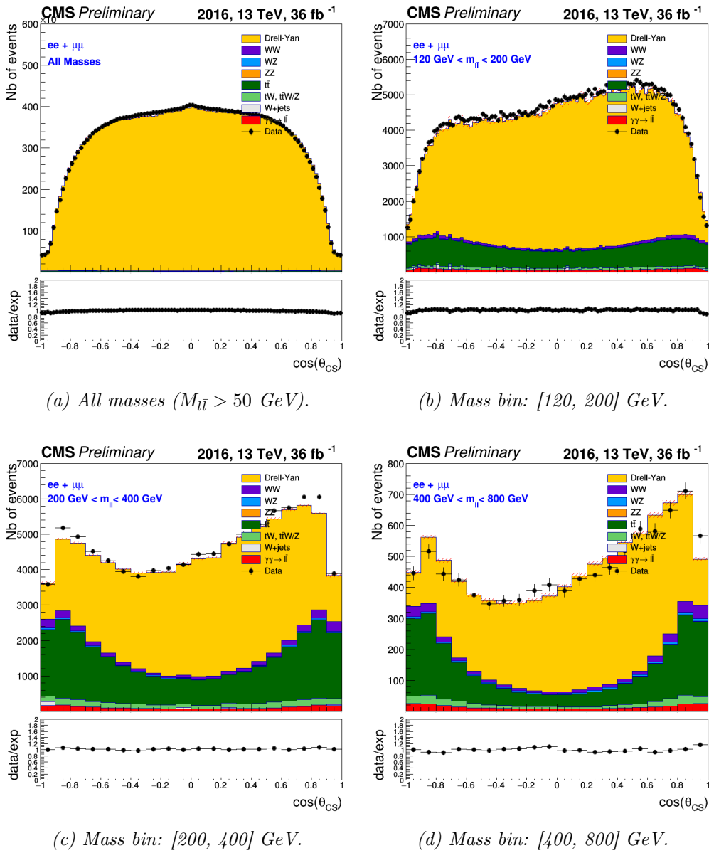
Figure 4.2 – The \cos\theta_{CS} distributions for ee/\mu\mu dilepton pair events (2016 data) for different mass bins.
