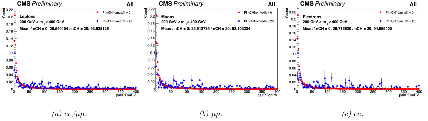
Figure 4.11 – The lepton pair p_T for nought (red) or twenty (blue) charged hadrons in vertex fit (Run II data) in the [200, 400] GeV mass bin.
