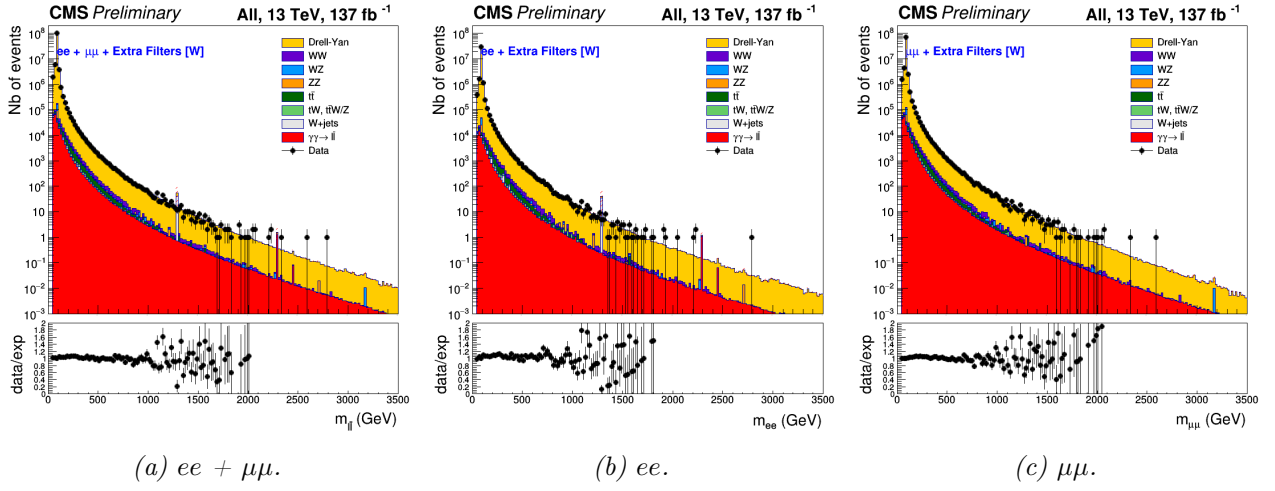
Figure 5.13 – The filtered invariant mass spectrum for all years combined and different lepton configurations.
