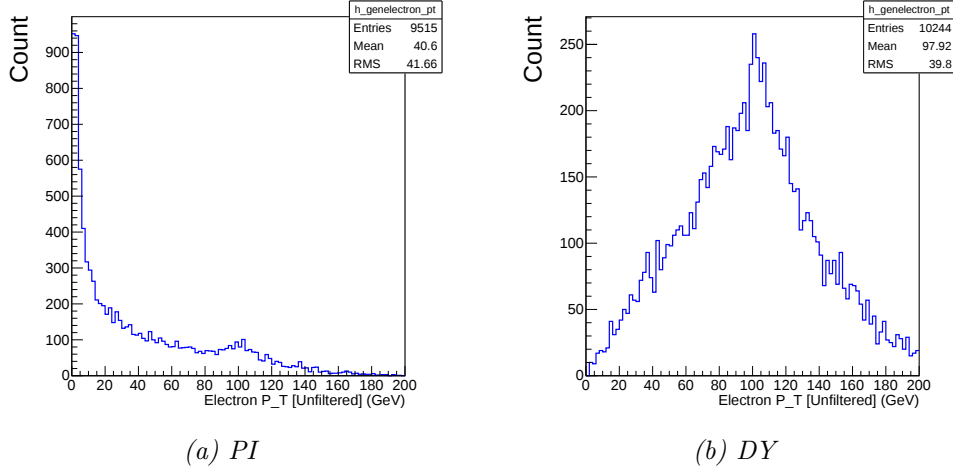
Figure C.13 – The electron p_T distributions, M_{l\bar{l}} \in [200, 400] GeV without acceptance cuts.
