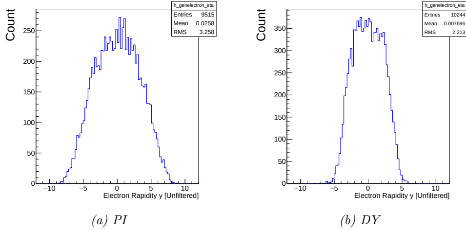
Figure C.3 – The electron \eta distributions, M_{\ell\bar{\ell}} \in [200, 400] GeV without acceptance cuts.
