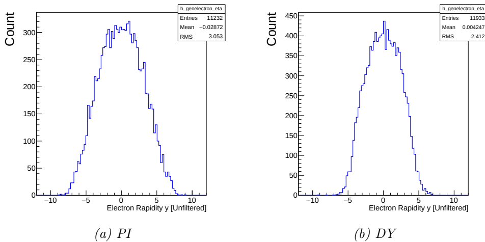
Figure C.1 – The electron \eta distributions, M_{l\bar{l}} > 60 GeV without acceptance cuts.
