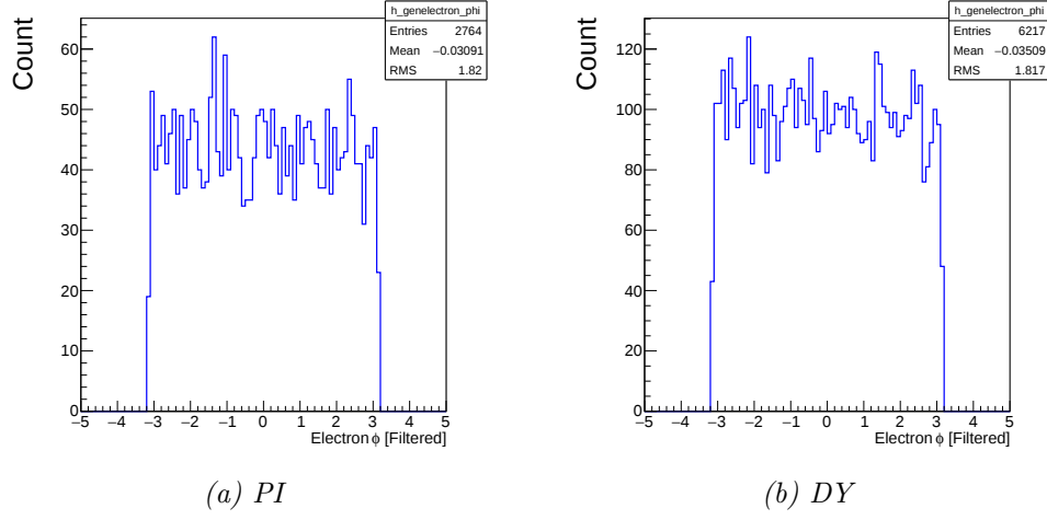
Figure C.10 – The electron \phi distributions, M_{l\bar{l}} \in [200, 400] GeV with acceptance cuts.
