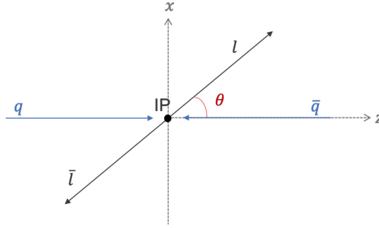
Figure 1.3 – The q\bar{q} centre of mass frame to describe the Drell-Yan process.
