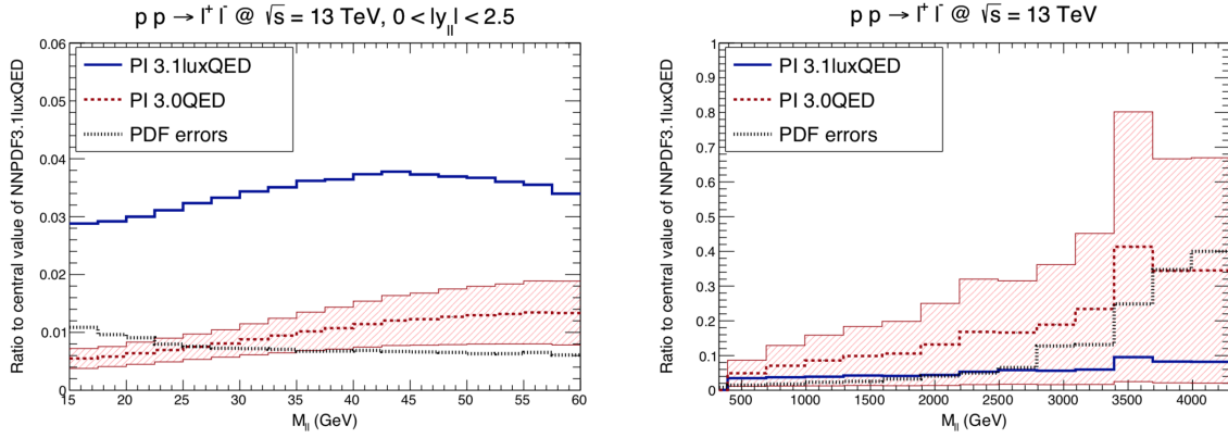
Figure 3.3 – Ratio of photon-initiated to DY neutral current lepton pair production as a function of the invariant mass of the pair M_{l\bar{l}} , for masses in the region [15, 60] GeV (left) and > 400 GeV (right). The NNPDF3.0QED uncertainty band is in red and the PDF errors give the uncertainties in NNPDF3.1luxQED [42].
