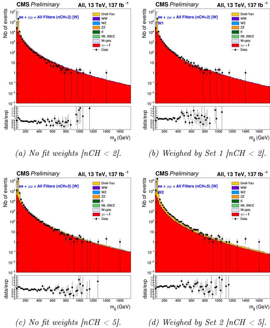
Figure 5.14 – The nCH-weighted filtered invariant mass spectrum with nCH cut (Run II data).
