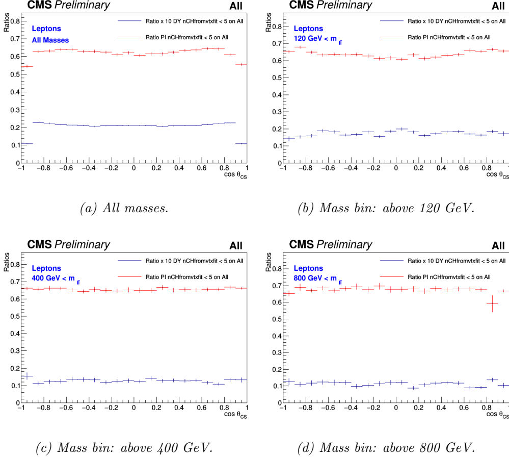
Figure 5.2 – The ratios nCH < 5 on no cut of \cos \theta_{CS} distributions for the DY (multiplied by 10) and PI at various mass bins (Run II data).
