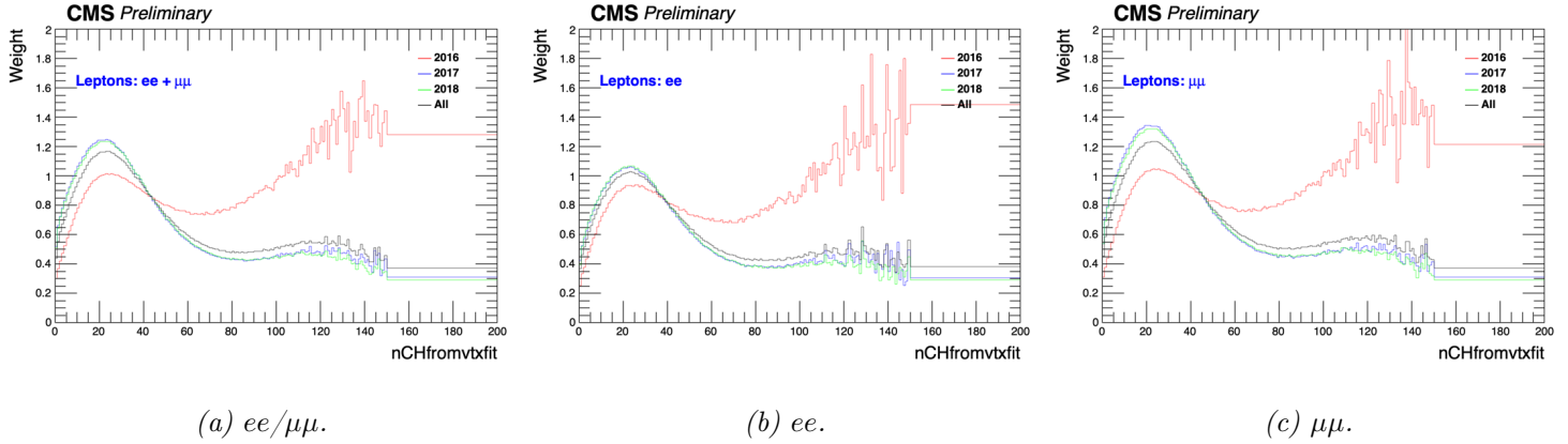
Figure 4.9 – The number of charged hadrons correction weights for all years and different lepton flavours.
