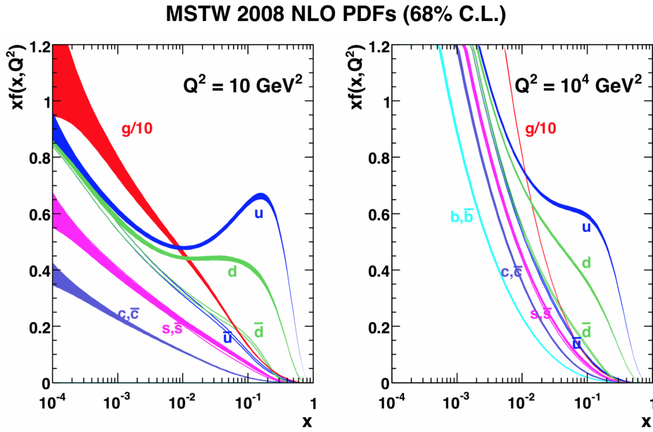
Figure 3.1 – The NLO PDF at the two different scales of Q^2 = 10 \text{ GeV}^2 and Q^2 = 10^4 \text{ GeV}^2 with 1\sigma uncertainty bands (68 % confidence level, CL) from [38].
