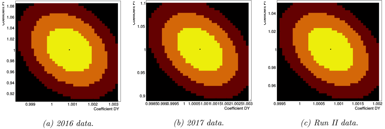
Figure 5.7 – The parameter fitted in the control region [70, 110] GeV of the nCH distributions for different years.
