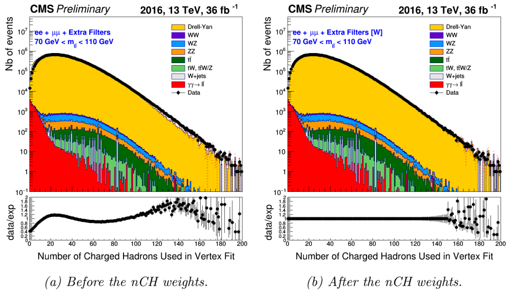
Figure 4.8 – The filtered number of charged hadrons from the vertex fit distribution for the [70, 110] GeV mass bin (2016 data).
