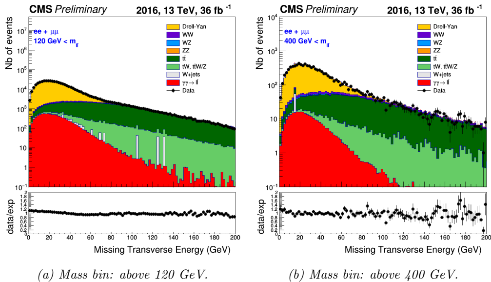
Figure 4.3 – The missing transverse energy distributions for different mass bins (2016 data).
