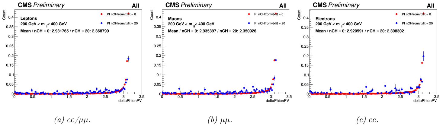
Figure 4.12 – The \Delta\phi between leptons for nought (red) or twenty (blue) charged hadrons in vertex fit (Run II data) in the [200, 400] GeV mass bin.
