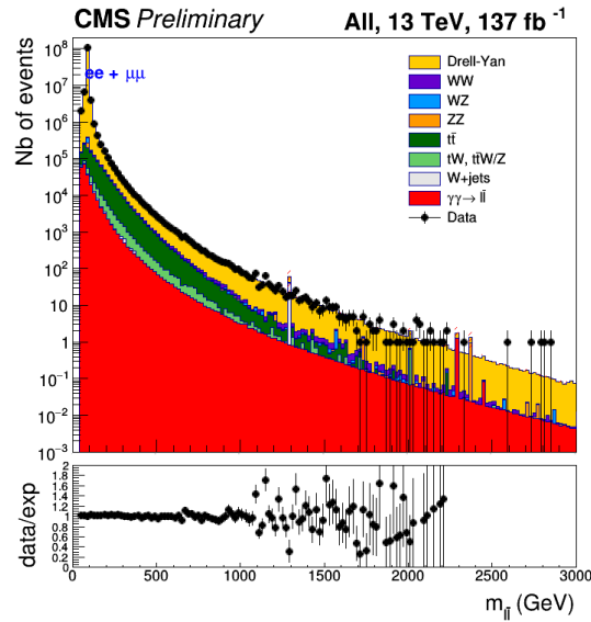
Figure 4.1 – The invariant mass spectrum of the ee/\mu\mu dilepton pairs for all years of Run II.
