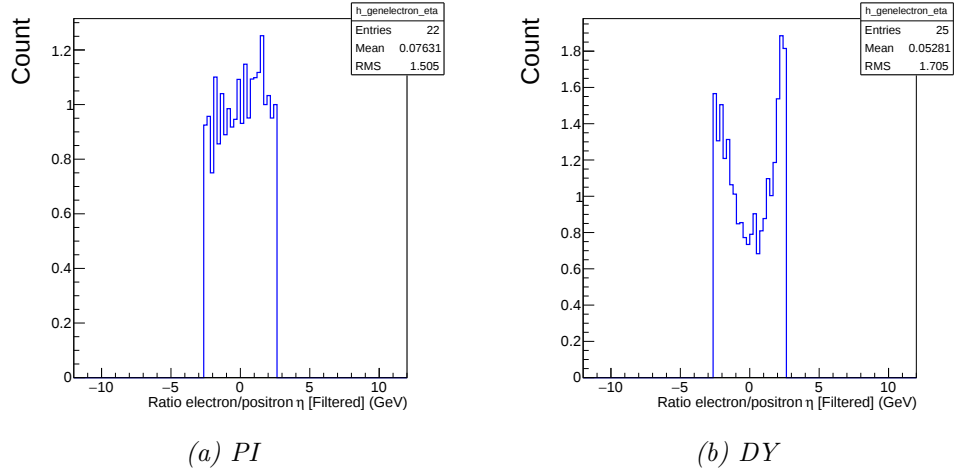
Figure C.6 – The ratio e^-/e^+ as a function of \eta , M_{l\bar{l}} \in [200, 400] GeV with acceptance cuts.
