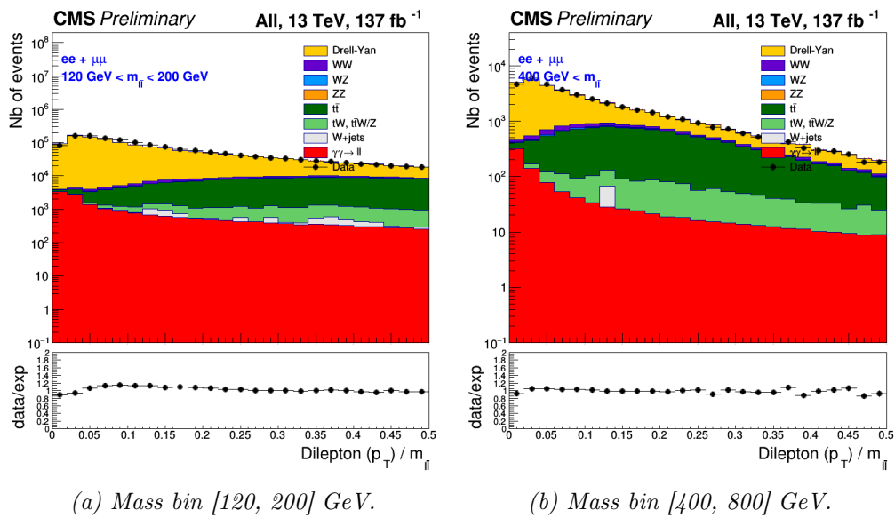
Figure D.1 – The lepton pair p_T on invariant mass distributions before filters (Run II data).
