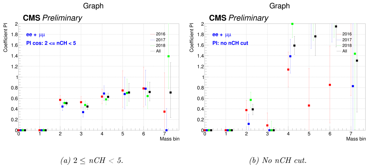
Figure D.5 – The PI fitting weights for the \cos \theta_{CS} distributions for all mass bins (except 0 and 1), Run II data of ee + \mu\mu events.
