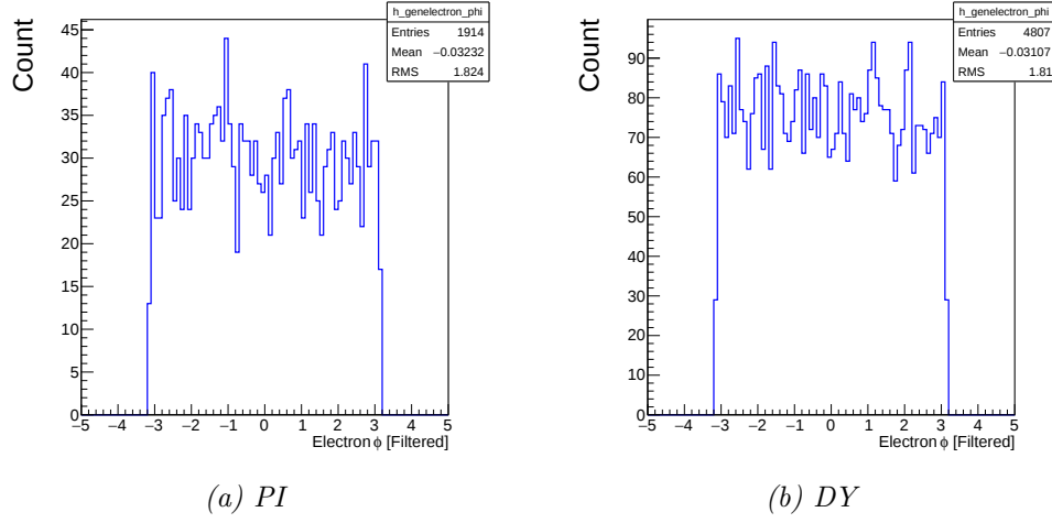
Figure C.8 – The electron \phi distributions, M_{l\bar{l}} > 60 GeV with acceptance cuts.
