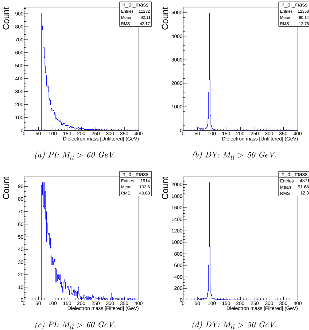
Figure 3.5 – Invariant mass of the dilepton pair at the generated level before (top) and after (bottom) acceptance cuts.
