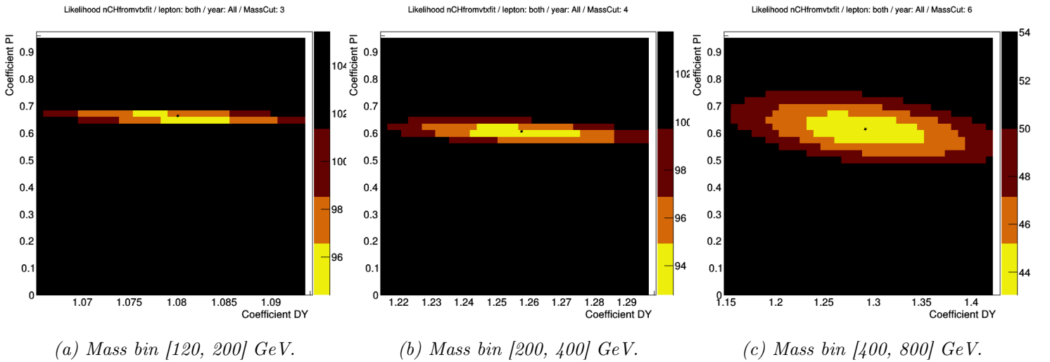
Figure D.8 – The parameters fitted in the different mass regions of the nCH distributions (Run II data).
