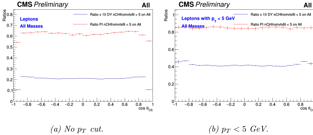
Figure 5.3 – The ratios n_{CH} < 5 on no cut (left) and idem with a lepton pair p_T < 5 GeV cut (right) of the \cos\theta_{CS} distribution for the DY (multiplied by 10) and PI at all masses (Run II data).
