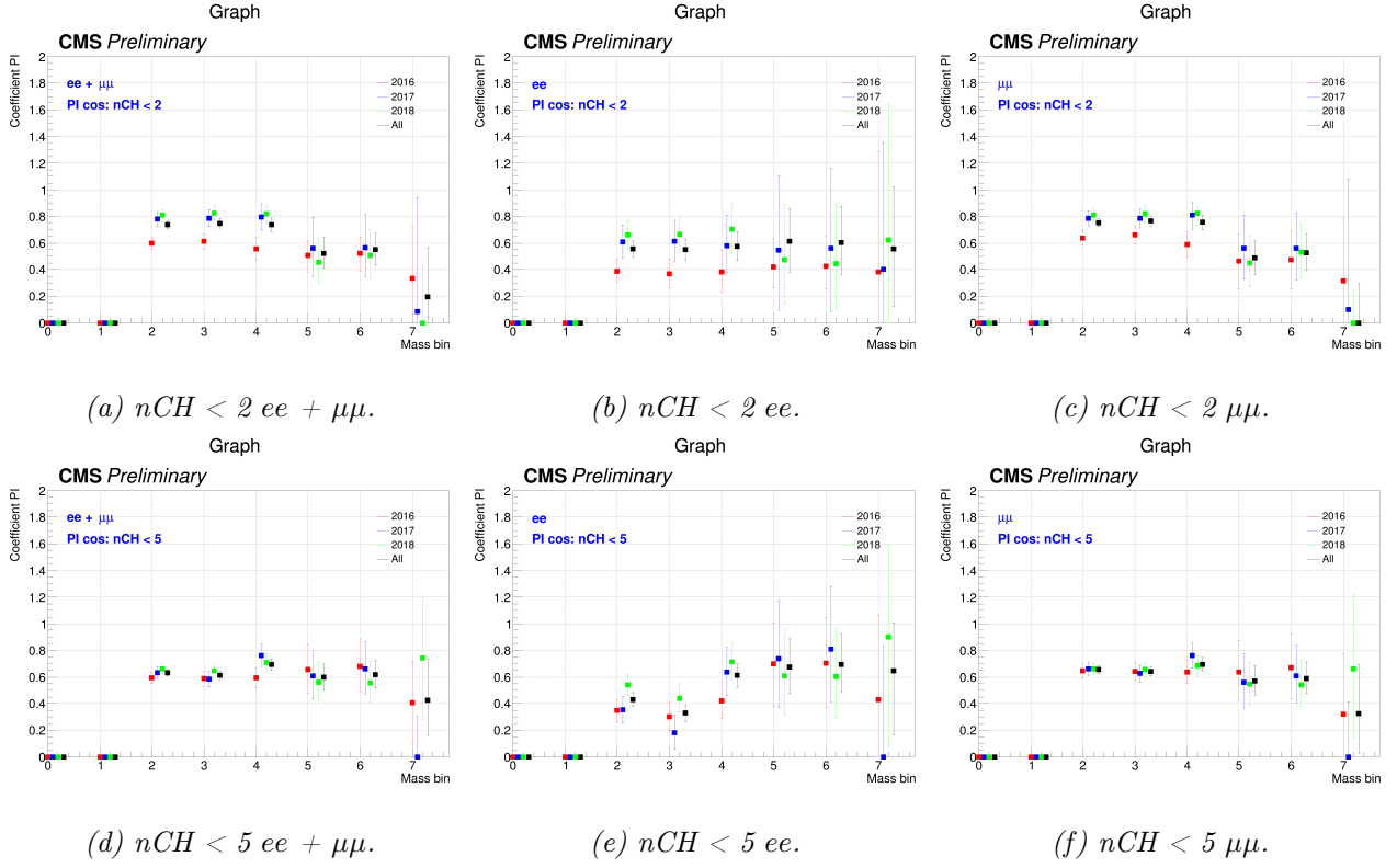
Figure D.7 – The PI fitting weights for the \cos\theta_{CS} distributions for all mass bins (except 0 and 1), all years and different lepton configurations.
