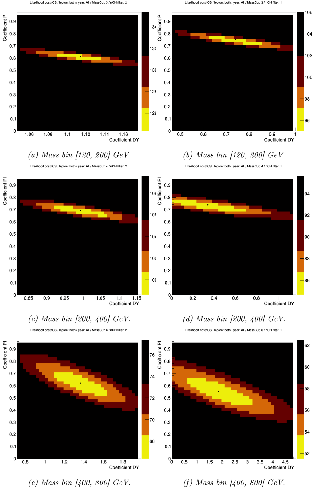
Figure D.6 – The parameters fitted in the different mass regions of the \cos\theta_{CS} distributions (Run II data) for nCH < 5 (left) and nCH < 2 (right).
