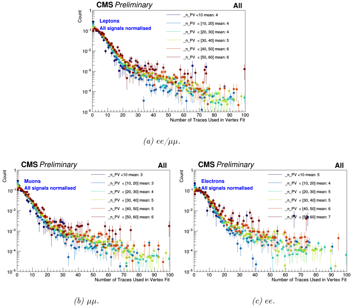
Figure 4.14 – The (normalised) nCH distributions of the PI for different bins of number of reconstructed vertices (Run II data) in the [200, 400] GeV mass bin.
