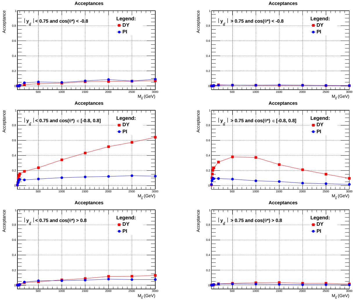
Figure 3.11 – Acceptance distributions as a function of the dilepton invariant mass M_{II} for the different sets of cuts.
