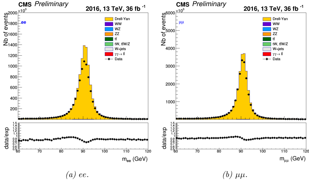
Figure 3.12 – The invariant mass spectra before normalisation scale factors (2016 data).
