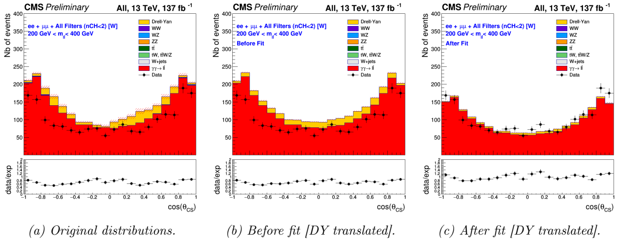
Figure 5.5 – The nCH -weighed \cos\theta_{CS} distributions in the [200, 400] GeV mass region with nCH < 2 (Run II data).
