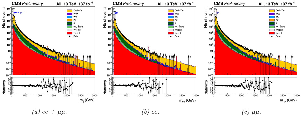
Figure 5.12 – The invariant mass spectrum for all years combined and different lepton configurations.
