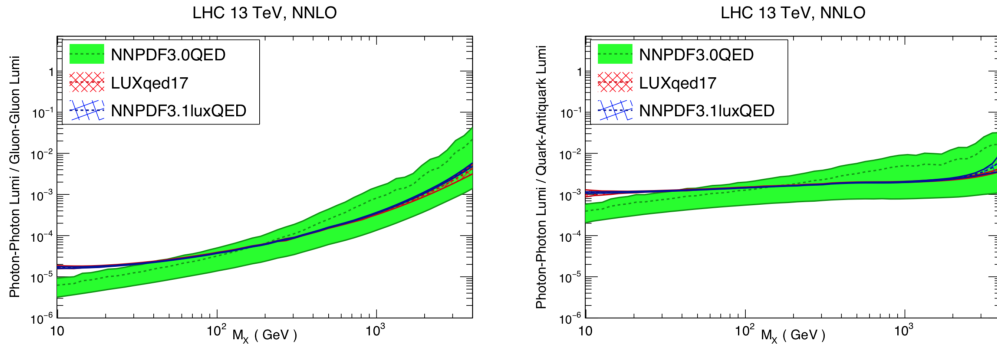
Figure 3.2 – The \mathcal{L}_{\gamma\gamma}/\mathcal{L}_{gg} (left) and \mathcal{L}_{\gamma\gamma}/\mathcal{L}_{q\bar{q}} (right) ratios for different PPDF [42].
