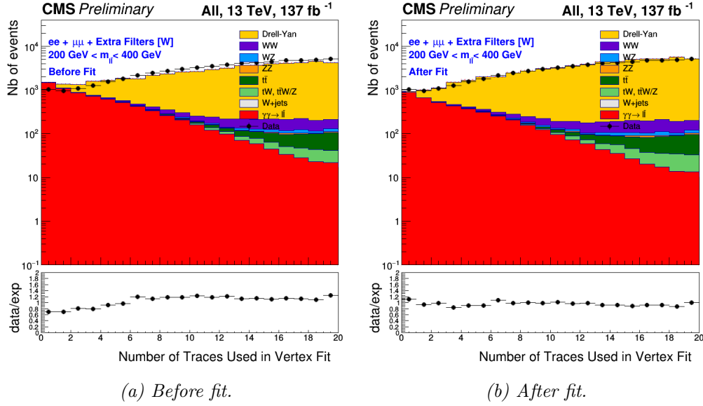
Figure 5.8 – The nCH -weighted nCH distributions in the [200, 400] GeV mass region (Run II data).
