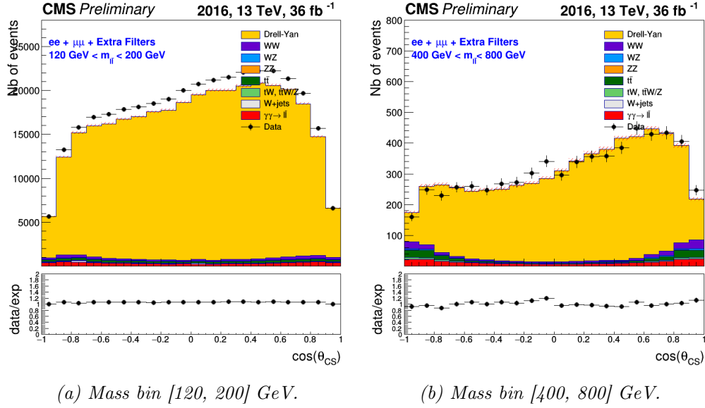
Figure 4.7 – The filtered \cos\theta_{CS} distributions for ee/\mu\mu dilepton pair events (2016 data) for different mass bins.
