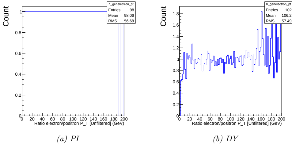
Figure C.15 – The ratio e^-/e^+ as a function of p_T , M_{l\bar{l}} \in [200, 400] GeV without acceptance cuts.
