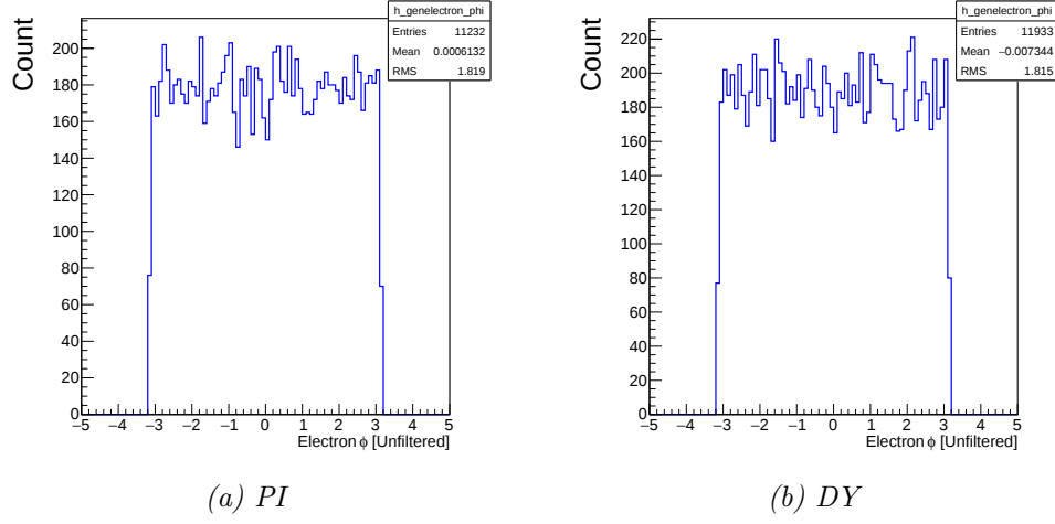
Figure C.7 – The electron \phi distributions, M_{l\bar{l}} > 60 GeV without acceptance cuts.
