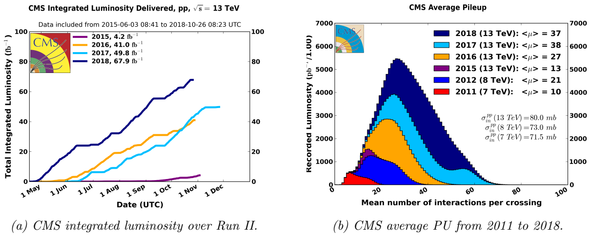
Figure 2.2 – CMS luminosity and pile-up. Extracted from the CMS public information page: https://twiki.cern.ch/twiki/bin/view/CMSPublic/LumiPublicResults .
