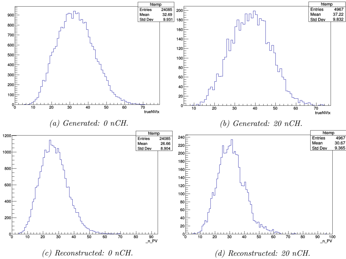
Figure 4.13 – The number of generated vertices (above, trueNVtx) and reconstructed ones (below, _n_PV) for nought (left) and twenty (right) charged hadrons in the PI simulation of the mass bin [200, 400] GeV.
