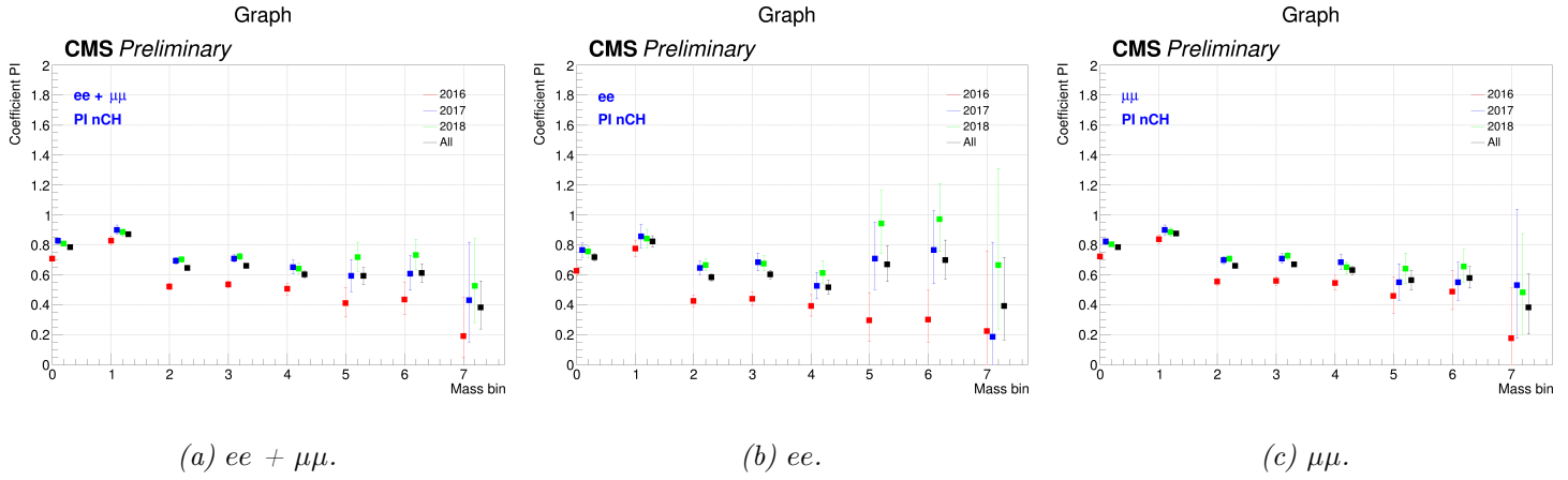
Figure 5.10 – The PI fitting weights for the nCH distributions for all years and different lepton configurations.
