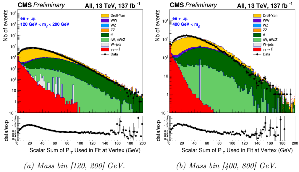
Figure D.3 – The p_T of charged hadron in the vertex fit distributions before filters (Run II data).
