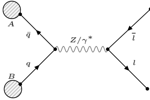
Figure 1.2 – The Drell-Yan process.
