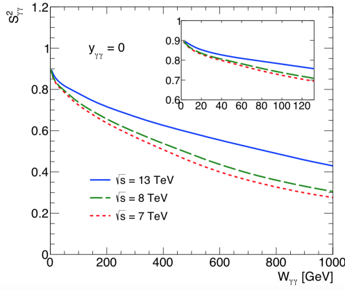
Figure 5.11 – The survival factor S_{\gamma\gamma} at zero rapidity as a function of the photon-photon centre of mass energy W_{\gamma\gamma} [46].
