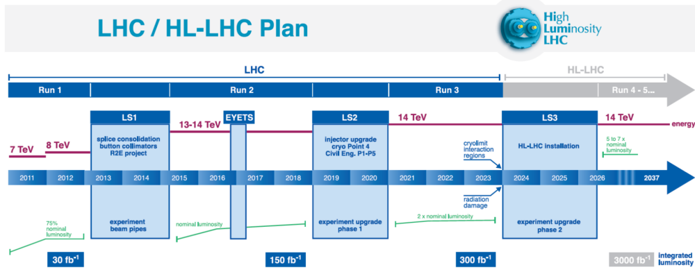
Figure 2.3 – Schedule of the LHC operation [32].
