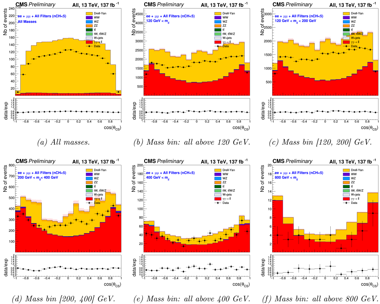
Figure D.4 – The unweighted ( nCH ) filtered \cos \theta_{CS} distributions for different mass bins (Run II data).
