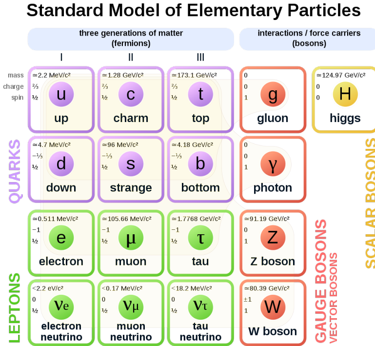
Figure 1.1 – Particles in the SM.
