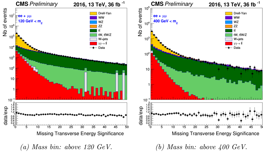
Figure 4.4 – The missing transverse energy significance distributions for different mass bins (2016 data).
