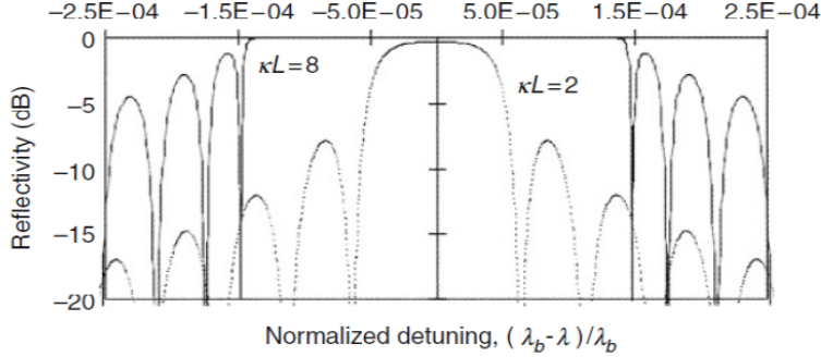
Figure 1.3: Reflectivity of two Bragg grating with coupling constants k_{ac}L = 2, 8 , as a function of the normalized detuning.
