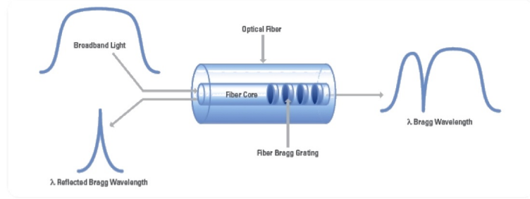
Figure 1.4: Schematics of the operative principle of a uniform fiber Bragg grating.
