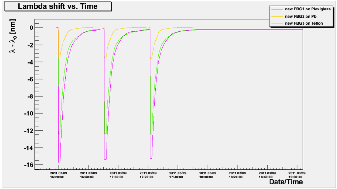
Figure 3.7: Bragg Wavelength response with respect of the time, during three cryogenic cycles.
