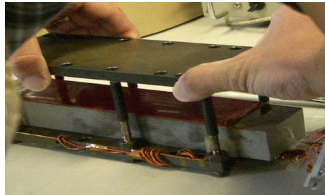
(d) Steel plates with screw-clamp.
