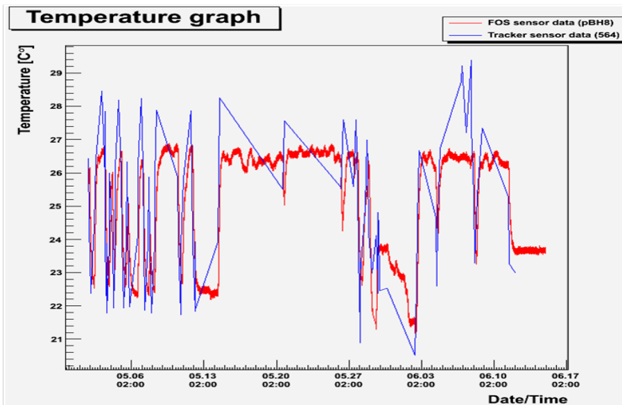
Figure 2.8: Performance comparison between FBG sensor (pBH8) and Tracker sensor. The picture shows a good agreement between the two sensing technology.
