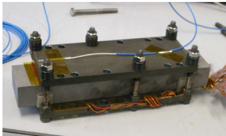
(e) Steel plates with screw-clamp screwed.
