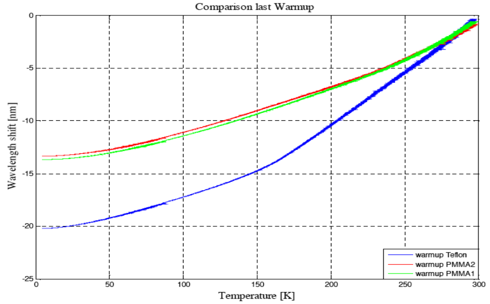
Figure 3.13: Sensitivity curve from experimental data for FBG bonded on PMMA and PTFE samples.
