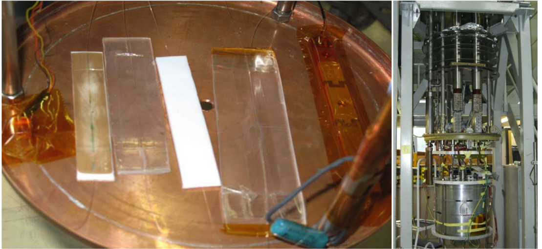
Figure 3.6: Experimental setup used in the Liquid Helium tests.
