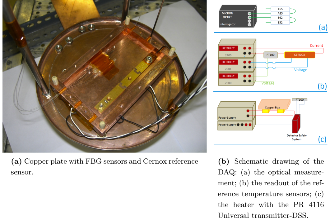
Figure 3.18: Experimental setup.
