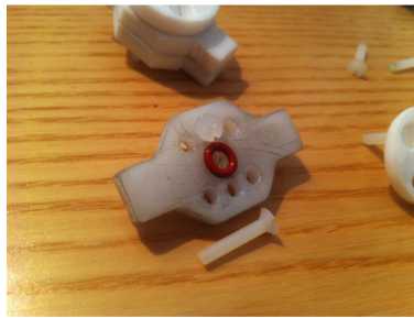
(b) Middle layer: silicon o-ring and nylon screws are fixed to it..
