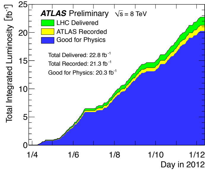
Fig. 2.2 Cumulative luminosity versus time delivered to (green), recorded by ATLAS (yellow), and certified to be good quality data (blue) during stable beams and for p - p collisions at 8 TeV centre-of-mass energy in 2012. Plot taken from [78].
