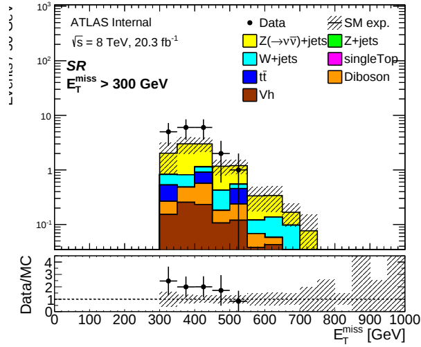
Fig. 8.4 E_T^{\text{miss}} distribution in the SR. The Z(\rightarrow \nu\bar{\nu}) +jets background events are estimated fully based on MC simulation. The hash band include both the statistical and systematic uncertainties.
