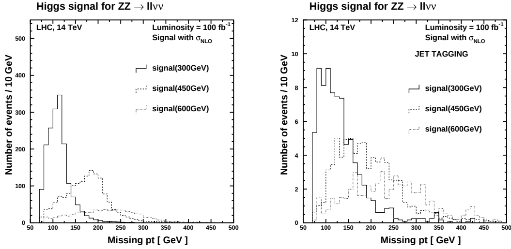
Figure 4.7: Missing p_t spectrum for a 300, 450 and 600 GeV Higgs without the backgrounds. (Left) without tagging (Right) with tagging. We can clearly see in all cases a peak in the distribution.
