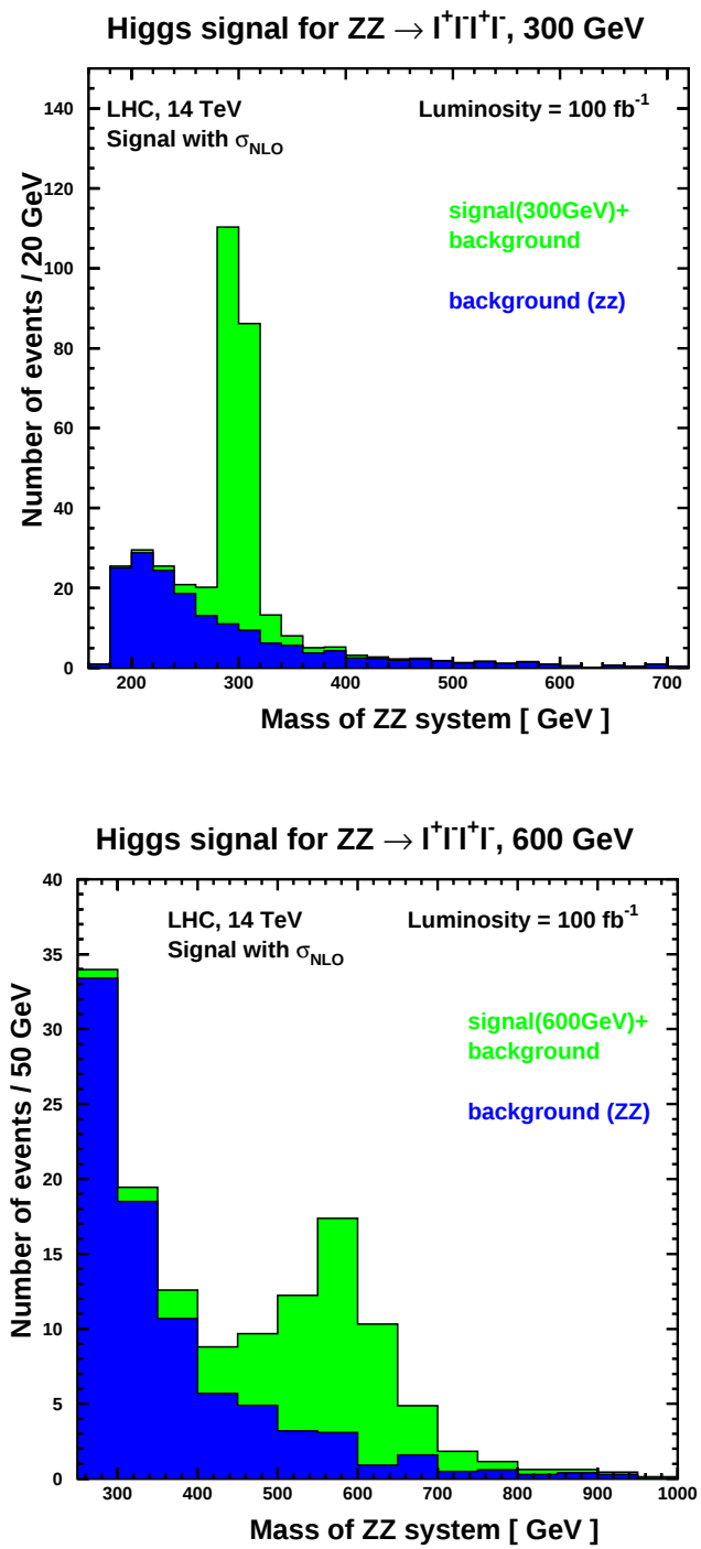
Figure 4.6: Mass spectrum for a 300 (Up) and 600 (Down) GeV Higgs for a luminosity of 100 \text{ fb}^{-1} , without jet tagging.
