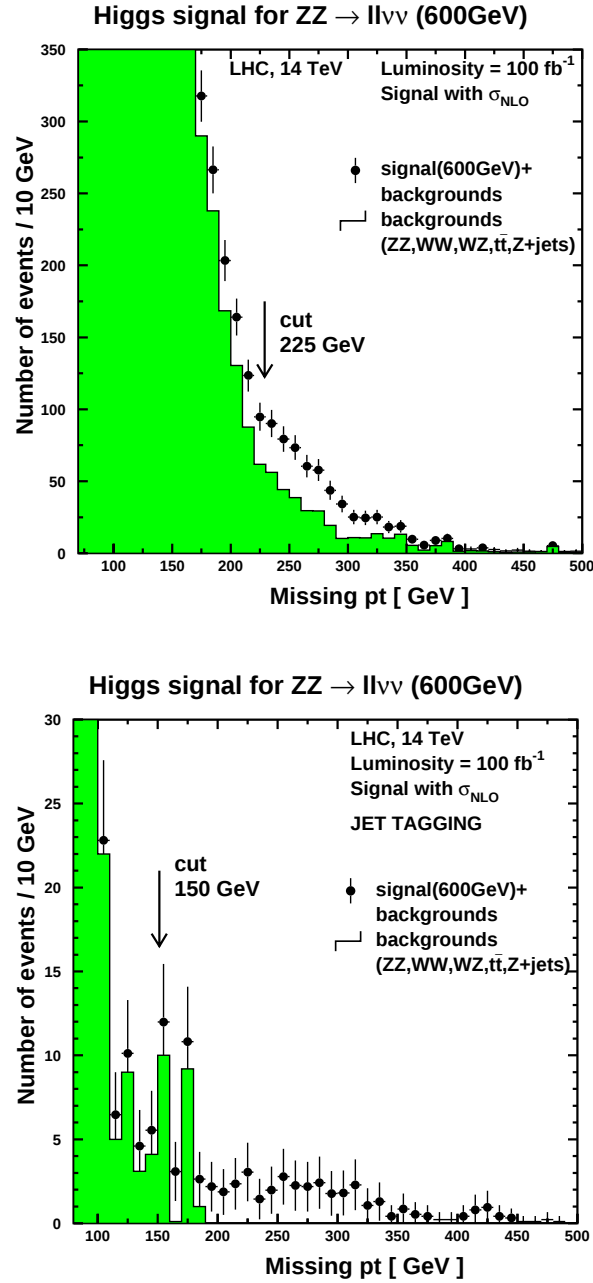
Figure 4.10: Missing p_t spectrum for a 600 GeV Higgs signal with the back-grounds. (Up) without tagging (Down) with tagging.
