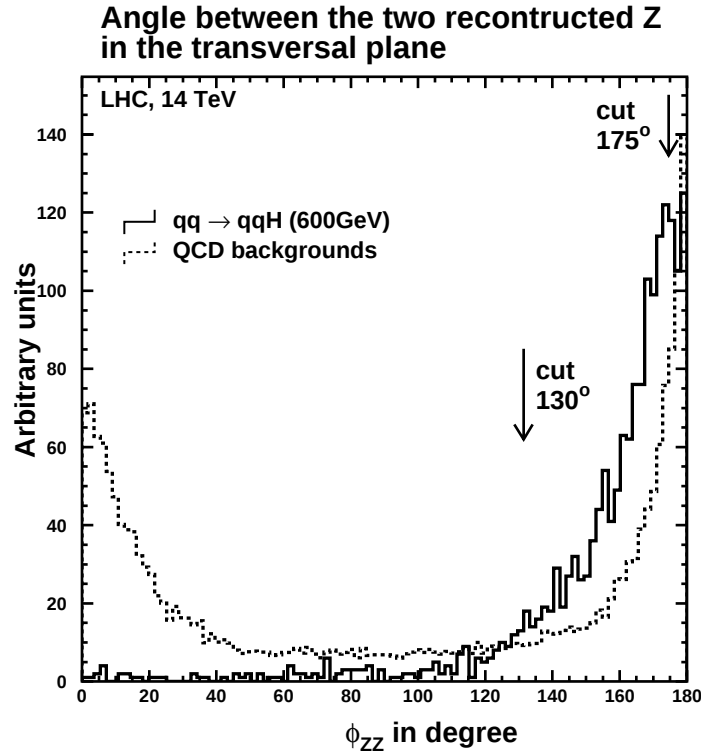
Figure 4.21: Angle between the two reconstructed Z, for the signal and the QCD background. The two histograms are not made for the same luminosity in order to compare the shapes. To have a number of events corresponding to the same luminosity for the signal and the background, the number of background events should be multiplied by 2 \cdot 10^6 .
