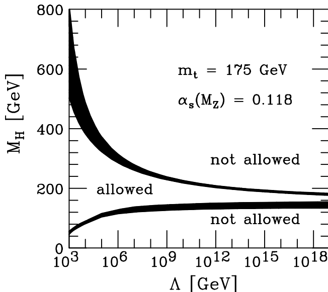
Figure 1: The area between black curves shows the allowed Higgs mass range assuming the validity of the Standard Model up to an energy scale of \Lambda , [3].
