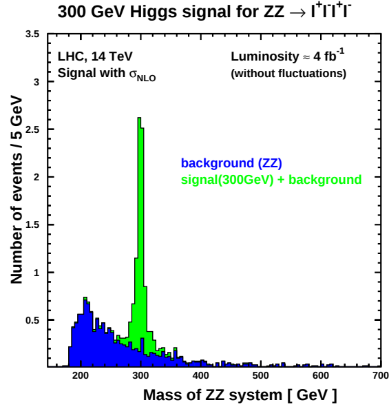
Figure 4.4: Higgs mass peak for a Higgs mass of 300 GeV, when no jet tagging is done. The signal and background were generated in a way to reduce as much as possible the statistical fluctuations.
