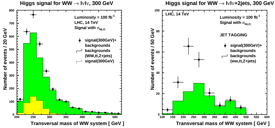
Figure 4.12: Transverse mass of the WW system for a 300 GeV Higgs, before tagging (Left) and after tagging (Right).
