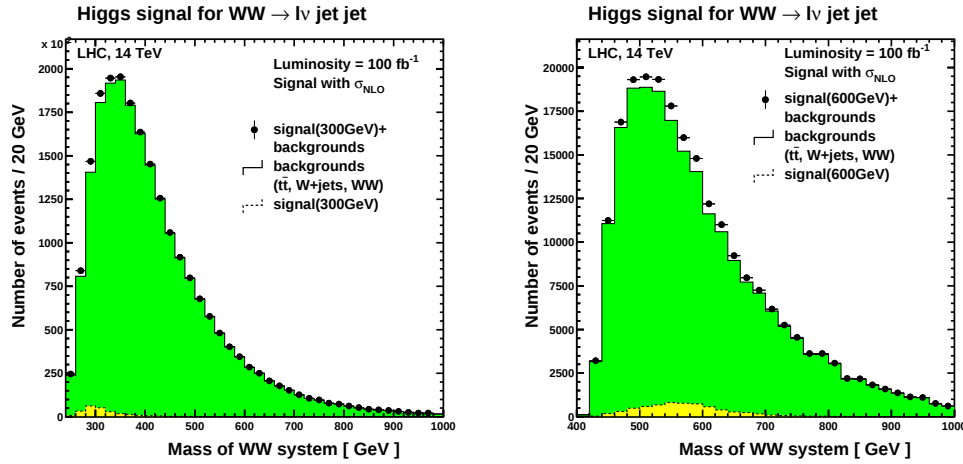
Figure 4.14: Mass spectrum of a 300 (Left) and a 600 GeV Higgs (Right) in the H \rightarrow WW \rightarrow \ell\nu q\bar{q} channel, when no jet tagging is applied.
