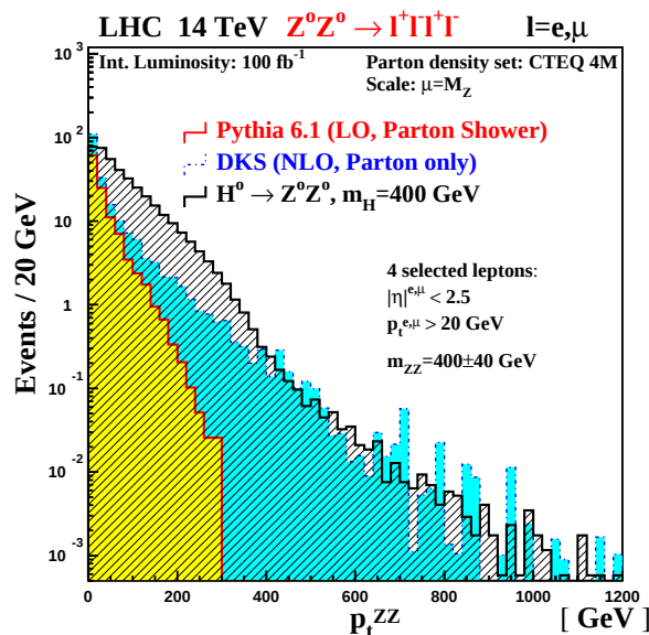
Figure 4.1: Transverse momentum of the ZZ system in the four leptons channel for signal and background (LO and NLO) [19].
