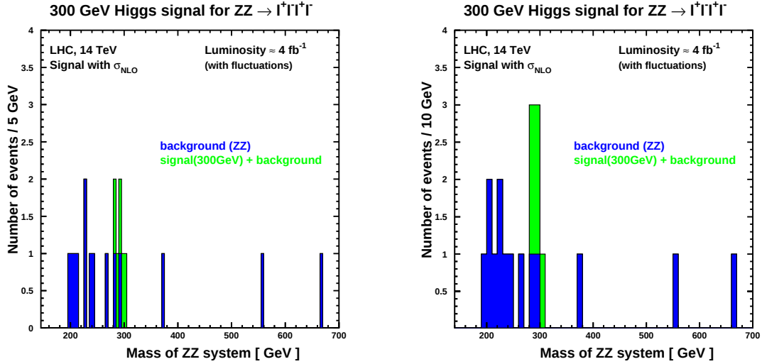
Figure 4.5: Higgs mass peak for a Higgs mass of 300 GeV, for a 'real' experiment and two different binnings, the 5 GeV bins are optimized according to our high luminosity plot while the 10 GeV bins are more for the small statistic samples.
