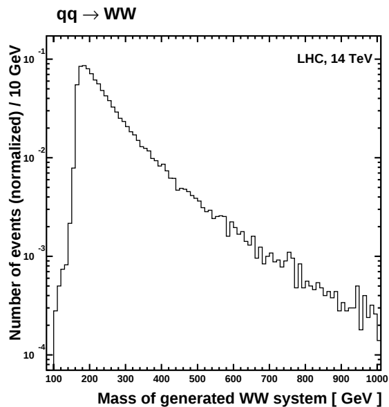
Figure 4.3: Mass spectrum of the generated WW system, produced through qq \rightarrow WW .
