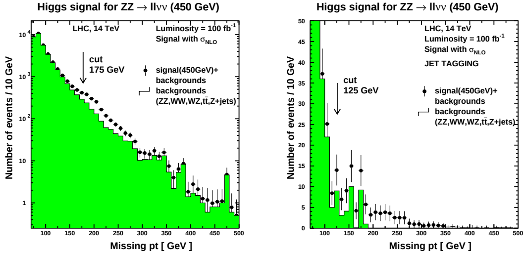
Figure 4.9: Missing p_t spectrum for a 450 GeV Higgs signal with the backgrounds. (Left) without tagging (Right) with tagging.
