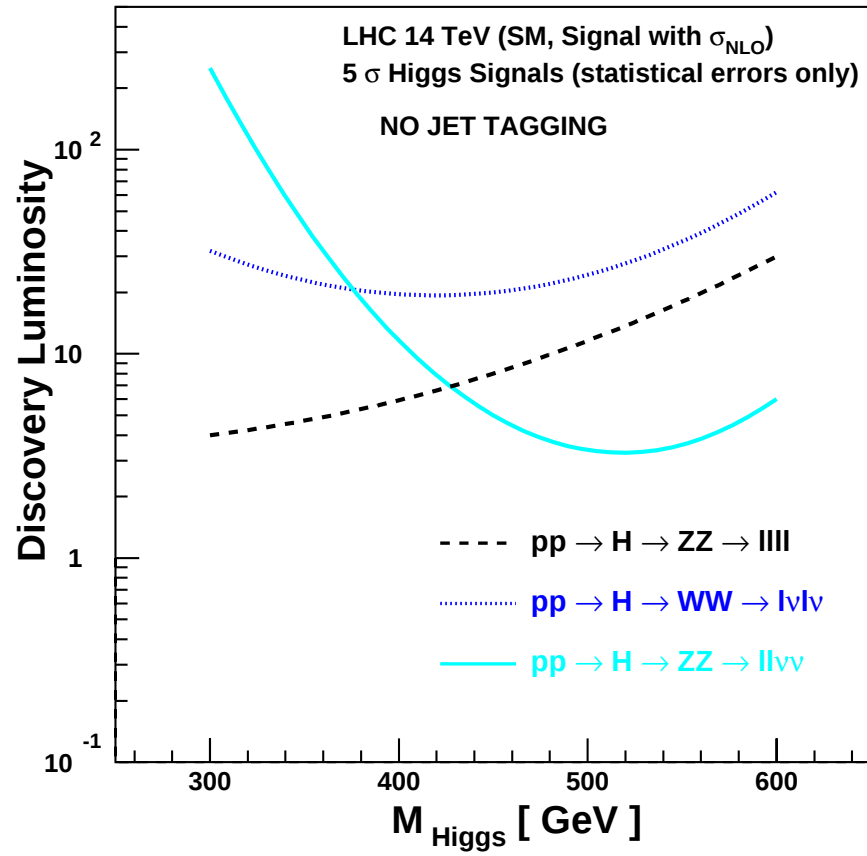
Figure 5.1: Expected luminosity for a 5\sigma standard deviation, for the 3 channels that give the most significant contribution when no jet tagging is made. Note that in the H \rightarrow WW \rightarrow \ell\nu\ell\nu channel, the signal to background ratio is low (about 0.15). For the signal, NLO cross sections are used.
