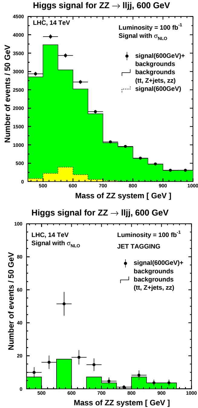
Figure 4.20: Mass spectrum of the reconstructed ZZ system for a 600 GeV Higgs. (Up) without jet tagging (Down) with jet tagging.
