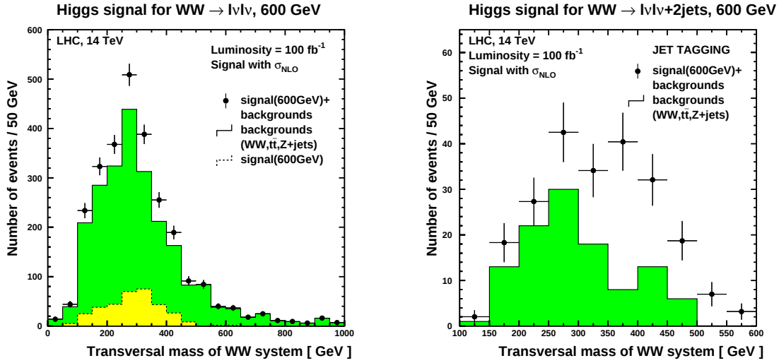
Figure 4.13: Transverse mass of the WW system for a 600 GeV Higgs. (Left) before tagging (Right) after tagging.
