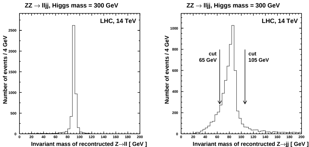
Figure 3.1: Reconstructed Z 's in the channel gg \rightarrow H \rightarrow ZZ \rightarrow \ell\ell jj for a 300 GeV Higgs after minimal cuts (e.g. asking two isolated leptons and more than two jets). (Left) Z \rightarrow \ell\ell (Right) Z \rightarrow jj .
