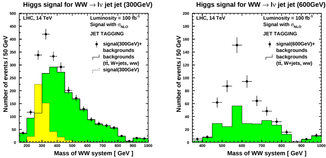
Figure 4.16: Mass spectrum of a 300 (Left) and a 600 GeV Higgs (Right) in the H \rightarrow WW \rightarrow \ell\nu jj channel, with forward jet tagging.
