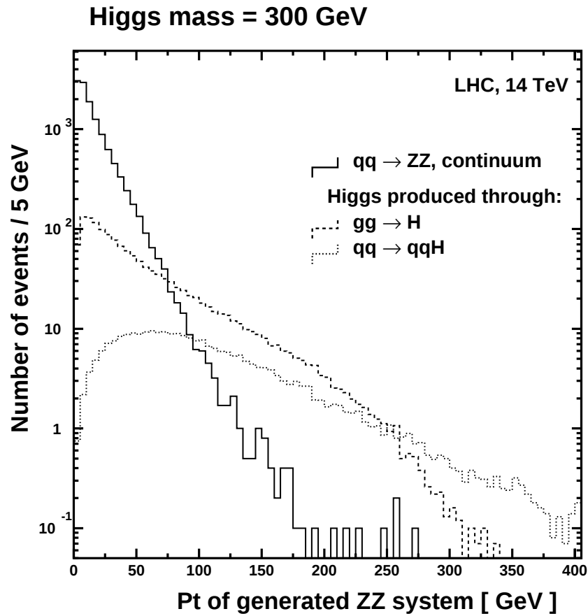
Figure 3.3: Generated transverse momentum for a 300 GeV Higgs for the two signal processes (with K-factors) and for the ZZ continuum.
