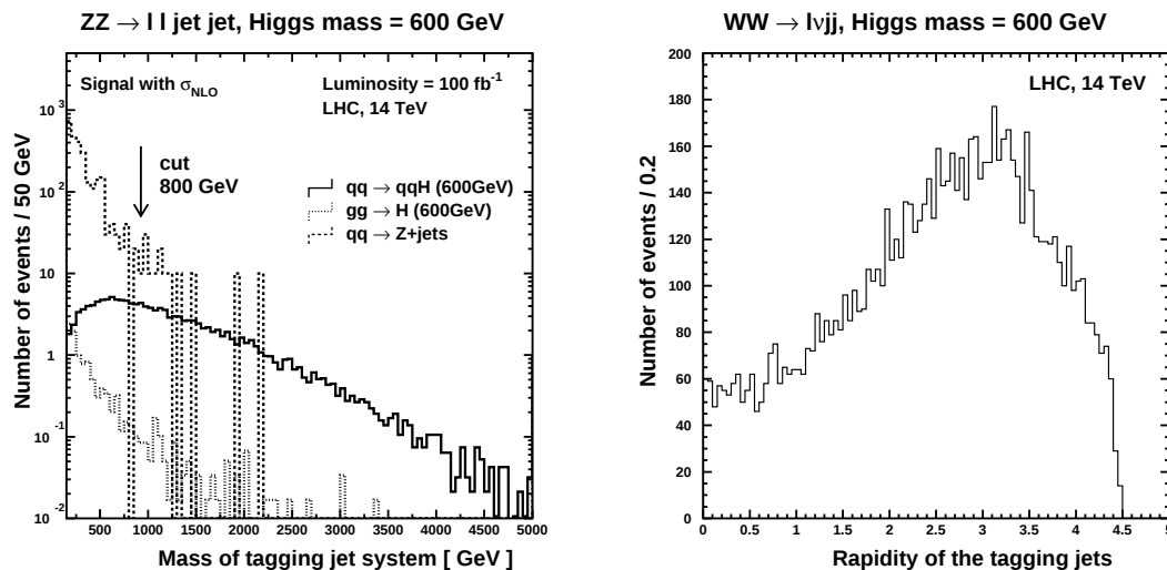
Figure 3.5: Characteristics of the tagging jets system: (Left) Mass of the tagging jet system for different processes in the channel qq \rightarrow qqH \rightarrow ZZ \rightarrow \ell\ell jj (Right) Rapidity of the tagging jets for the channel qq \rightarrow qqH \rightarrow WW \rightarrow \ell\nu jj .
