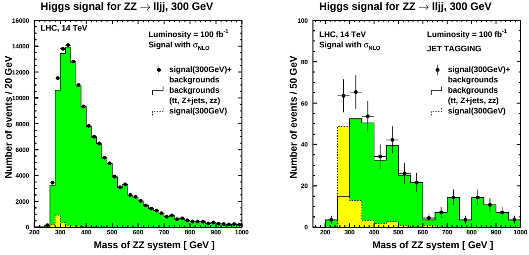
Figure 4.18: Mass spectrum of the reconstructed ZZ system for a 300 GeV Higgs. (Left) without jet tagging (Right) with jet tagging.
