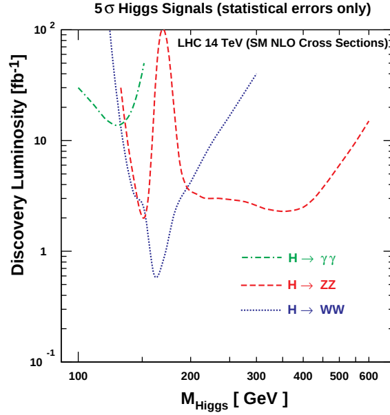
Figure 2.3: Discovery luminosity as a function of the Higgs mass as given in Ref. [9].
