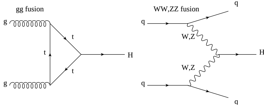
Figure 2.1: Feynman diagrams for two production mechanisms of Higgs. (Left) gluon fusion (Right) weak boson fusion.
