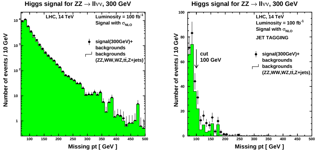
Figure 4.8: Missing p_t spectrum for a 300 GeV Higgs signal with the backgrounds. (Left) without tagging (Right) with tagging.
