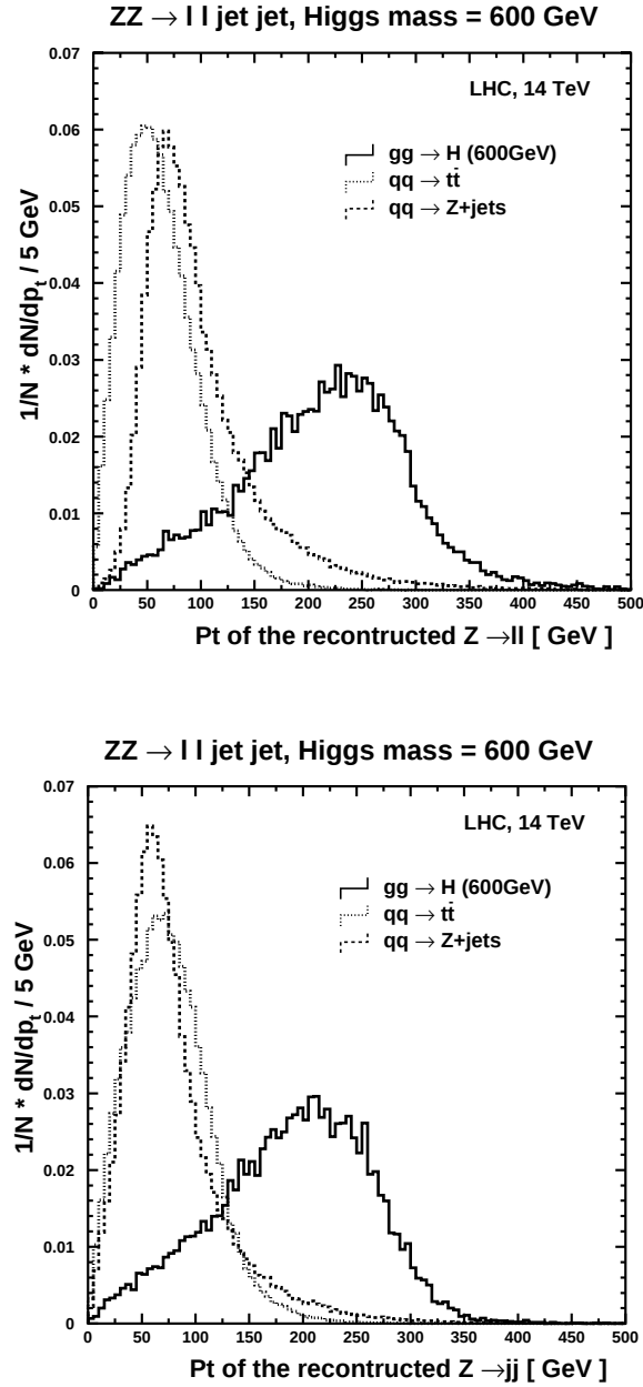
Figure 3.4: p_t spectra of the reconstructed Z for a 600 GeV Higgs and for different backgrounds in the H \rightarrow ZZ \rightarrow \ell\ell jj channel, before the selection cuts and normalized to the total number of events. (Up) p_t spectrum for the reconstructed Z decaying leptonically (Down) p_t spectrum for the reconstructed Z decaying hadronically.
