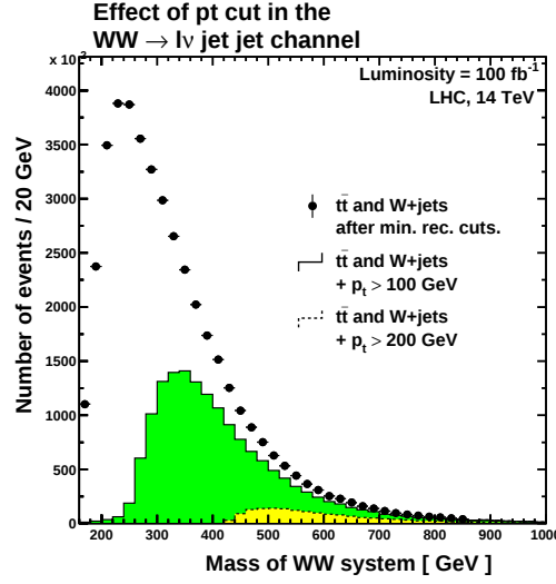
Figure 4.15: Effect of the cuts on the reconstructed WW mass spectrum. It is shown for W + jets and t\bar{t} backgrounds, with a number of events corresponding to a luminosity of 100fb^{-1} . A first plot is done with the events that survived the minimal reconstruction cuts. As p_t cuts of 100 and 200 GeV were done to isolate a 300 and 600 GeV Higgs respectively, we show how the WW mass spectrum for background looks like after these two cuts.
