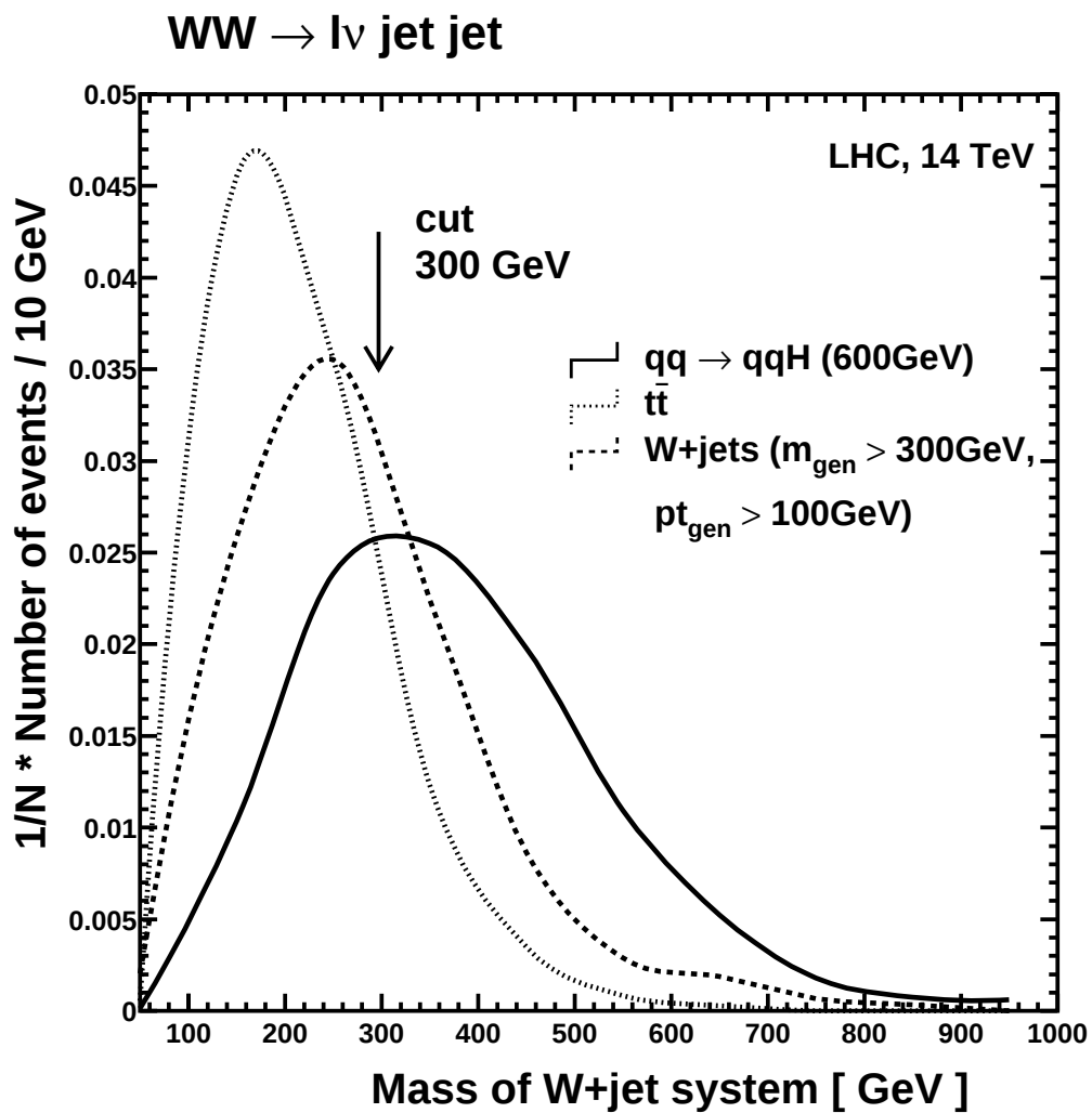
Figure 3.6: Distribution of the m_{W_{jet}} candidates for the signal, the top-antitop and W + \text{jets} backgrounds. The curves are normalized to 1.
