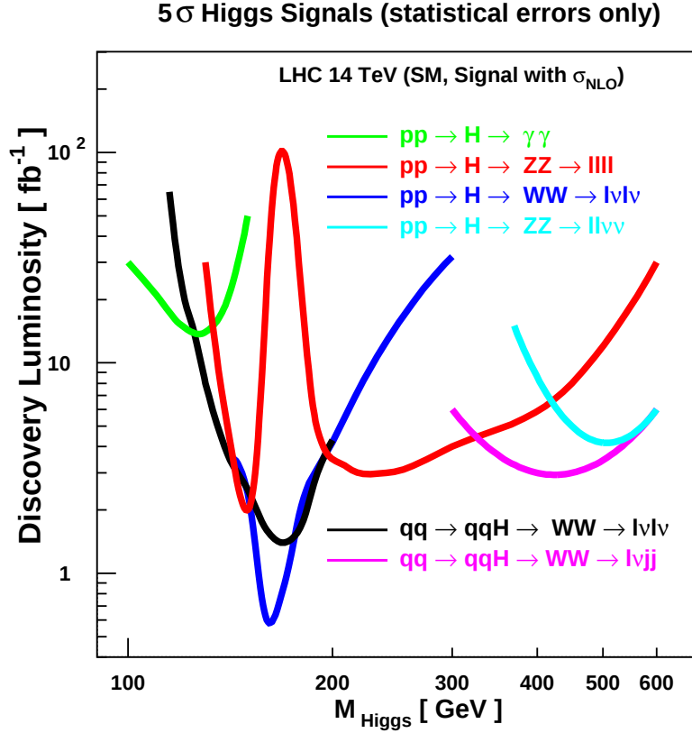
Figure 5.3: Expected luminosity for a 5 \sigma standard deviation, as presented in the CMS meeting of 9th March 2001. For the signal, NLO cross sections are used.
