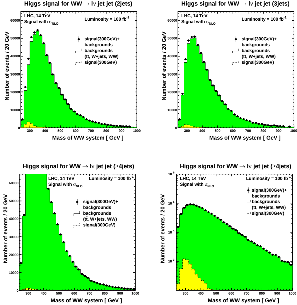
Figure 4.17: Mass spectrum of a 300 GeV Higgs in the H \rightarrow WW \rightarrow \ell\nu jj channel, for different number of jets in event. (Up left) exactly 2 jets (Up right) exactly 3 jets (Down left) more than 3 jets. (Left) with the same scale used than for the other plots (Right) with a logarithmic scale. As soon as there are more than 3 jets in events, the t\bar{t} background begins to be important and overwhelm a possible signal. Furthermore the number of signal events produced through gluon fusion is strongly reduced as soon as the number of required jets is higher than 2.
