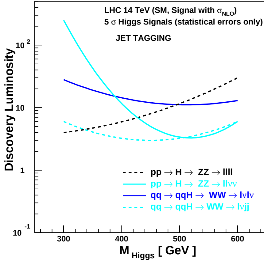
Figure 5.2: Expected luminosity for a 5\sigma standard deviation, for the channels that can give an interesting contribution. The channels where the jet tagging technique is used are taken here into account. For the signal, NLO cross sections are used.
