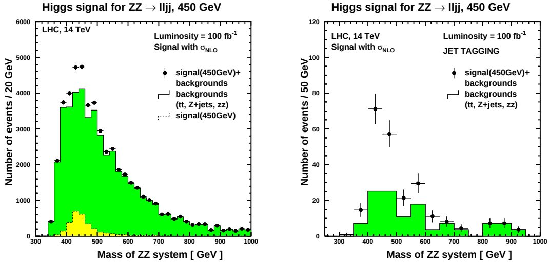
Figure 4.19: Mass spectrum of the reconstructed ZZ system for a 450 GeV Higgs. (Left) without jet tagging (Right) with jet tagging.
