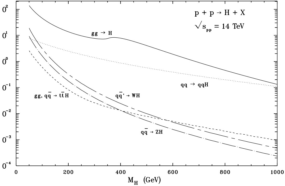
Figure 2.2: Cross sections of different production mechanisms of Higgs as a function of the Higgs mass, given at the next to leading order, Ref. [8].
