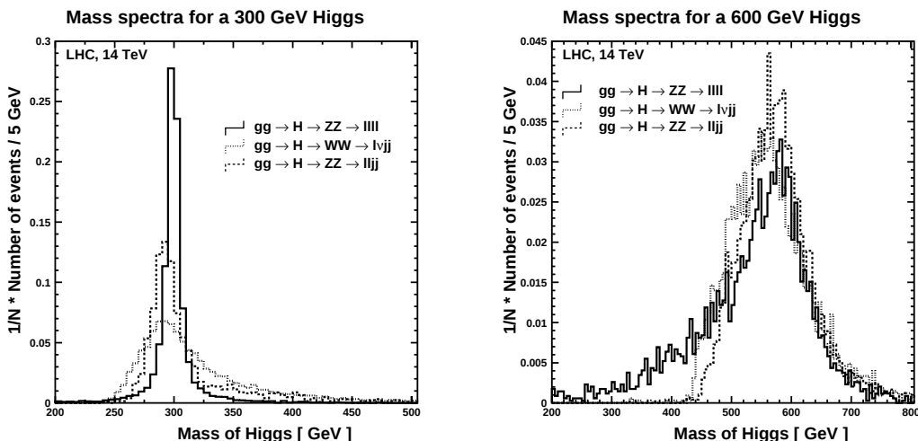
Figure 3.2: Comparison between the mass resolution the reconstructed Higgs mass spectrum for different signatures. The plots are made after the reconstruction cuts. The Higgs is produced through the gluon fusion. (Left) for a 300 GeV Higgs (Right) for a 600 GeV Higgs.
