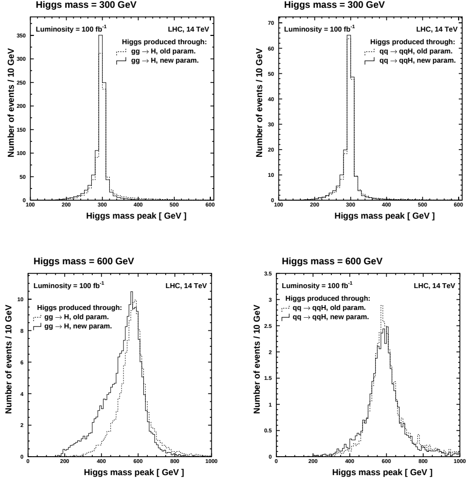
Figure 4.2: Difference between the generated Higgs mass peak obtained with the old and the new parameterization. Upper plots correspond to a 300 GeV Higgs and lower plots to a 600 GeV Higgs. The Higgs events on the left plots were produced through gluon fusion and on the right plots through weak boson fusion. The plots are made on the generator level, without any selection cuts and NLO cross sections are used.
