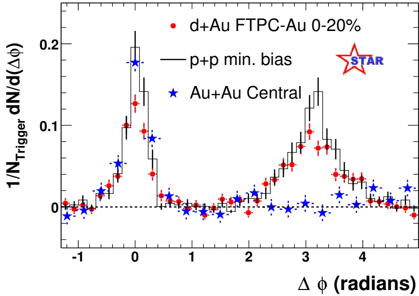
Figure 1.9: Di-hadron azimuthal co-relation for pp, d-Au and Au-Au collisions at \sqrt{s_{NN}} = 200 GeV in STAR experiment [25].
