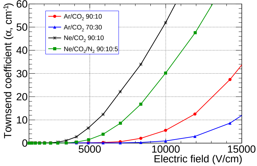
Figure 6.4: Townsend coefficients in different Argon and Neon-based gas mixtures as a function of the electric field is calculated using Magboltz software [97]. The avalanche shifted by 1 kV/cm upward with the admixture of N 2 . The avalanche of Argon is sustainable away.
