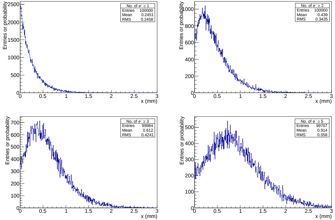
Figure 4.49: Simulation of primary electron clusters distribution in a 3 mm thick Ar/CO 2 70:30. The figures are corresponding to the position distribution of the clusters with total electrons 1, 2, 3 and 5.
