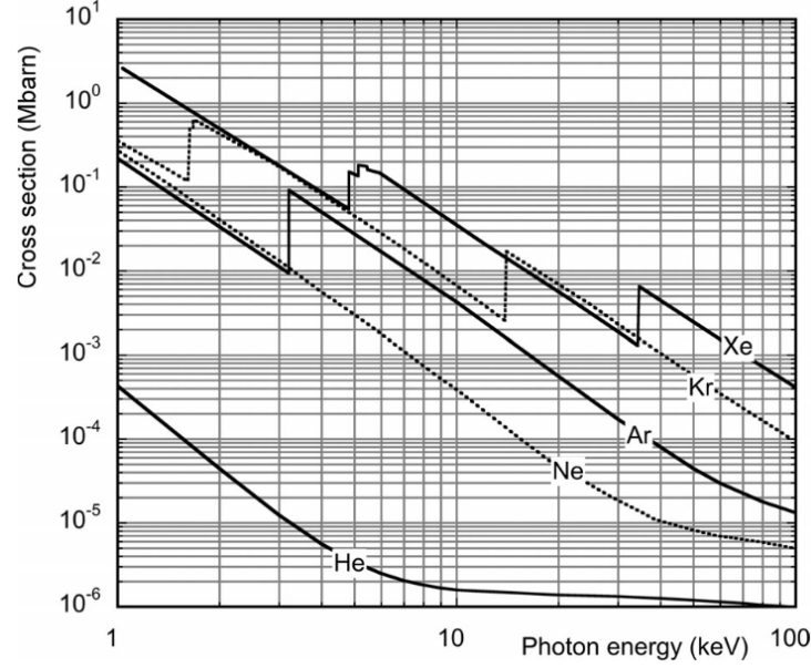
Figure 4.9: Photon total cross-section for noble gases.
