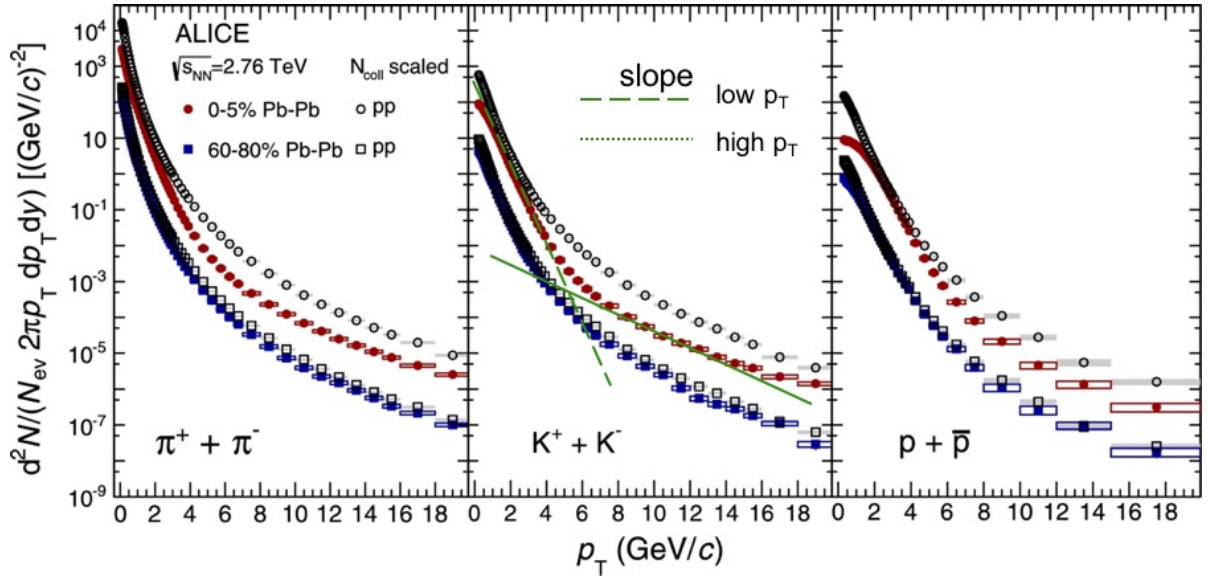
Figure 7.8: Transverse momentum distribution for the charged particles: \pi^+ + \pi^- , K^+ + K^- , p + \bar{p} . Two different slopes can be realized for the low and high p_T particles. The figure is adopted from [153].
