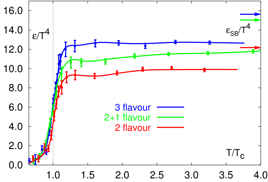
Figure 1.3: Lattice QCD prediction, the temperature dependence of energy density of QCD medium. Sudden change in the energy density below and above the critical temperature ( T_c ): an evidence of phase change [16].
