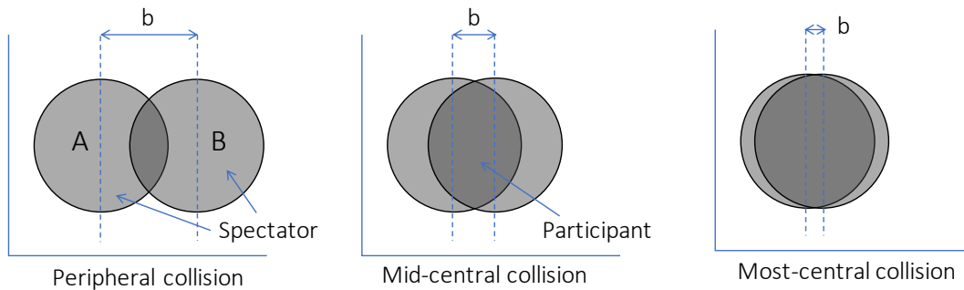
Figure 7.1: Projection of the collision of two nuclei in x, y -plane for different impact parameters.
