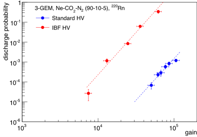
Figure 6.7: Discharge probability of a triple GEM detector measured for different HV settings. Dashed lines corresponding to power law function fits [88].
