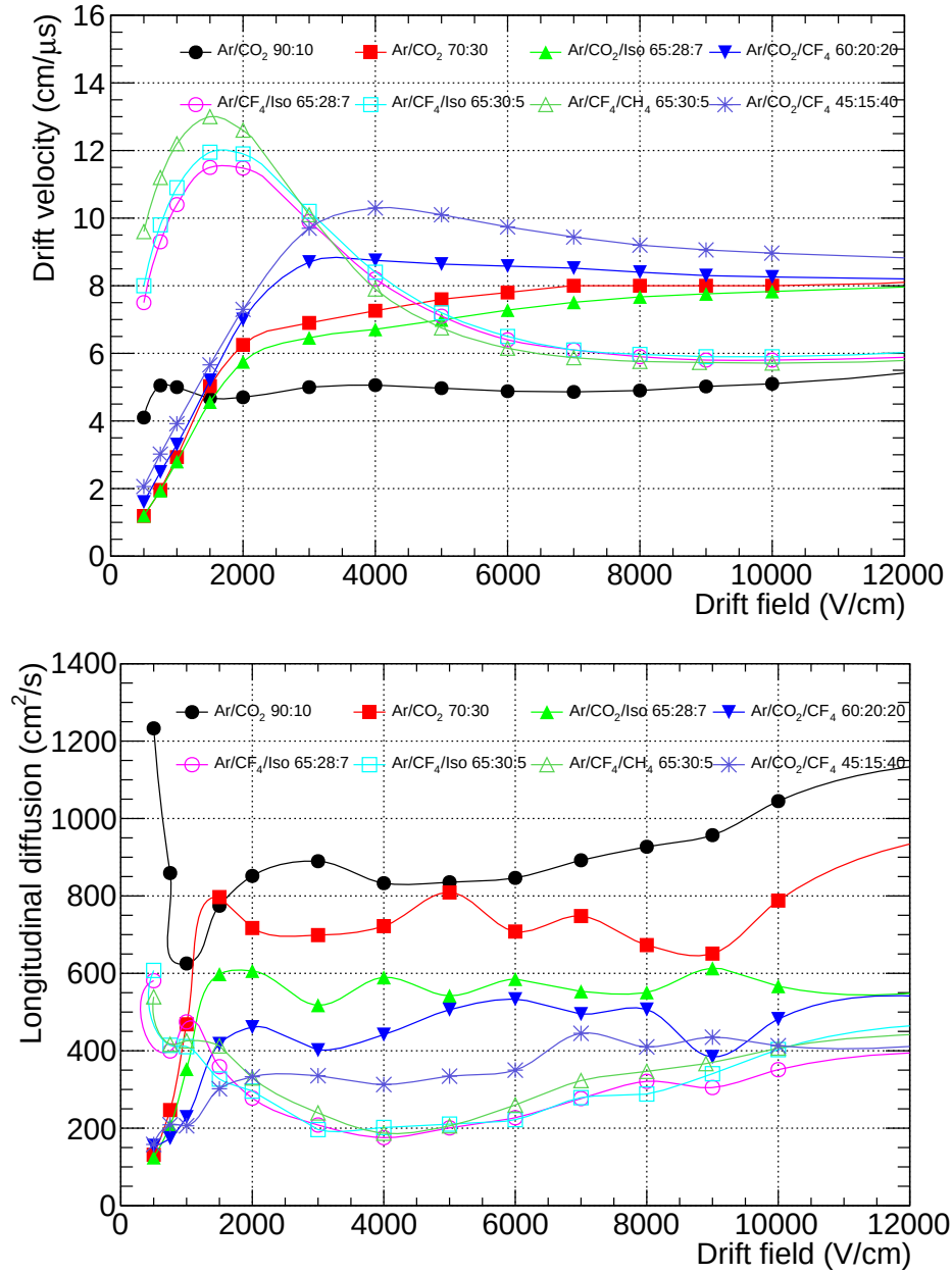
Figure 4.47: Variation of the electron drift velocity (top panel) and longitudinal diffusion (bottom panel) with electric field for different Argon based gas mixtures.
