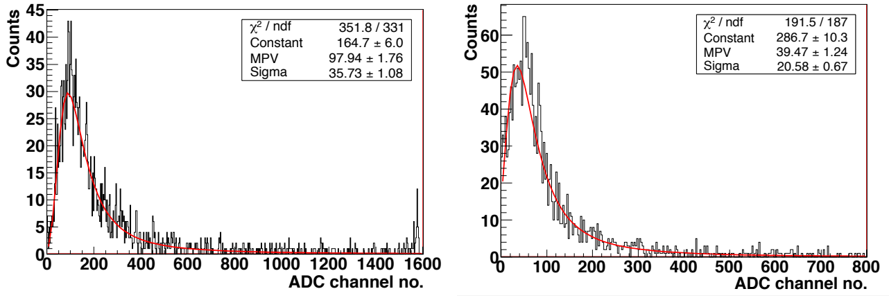
Figure 5.6: Cosmic muon spectrum of the MWPC-1 detector using MANAS electronics operated at 1850 V. The spectrum from anode in left panel and spectrum from pad in right panel.
