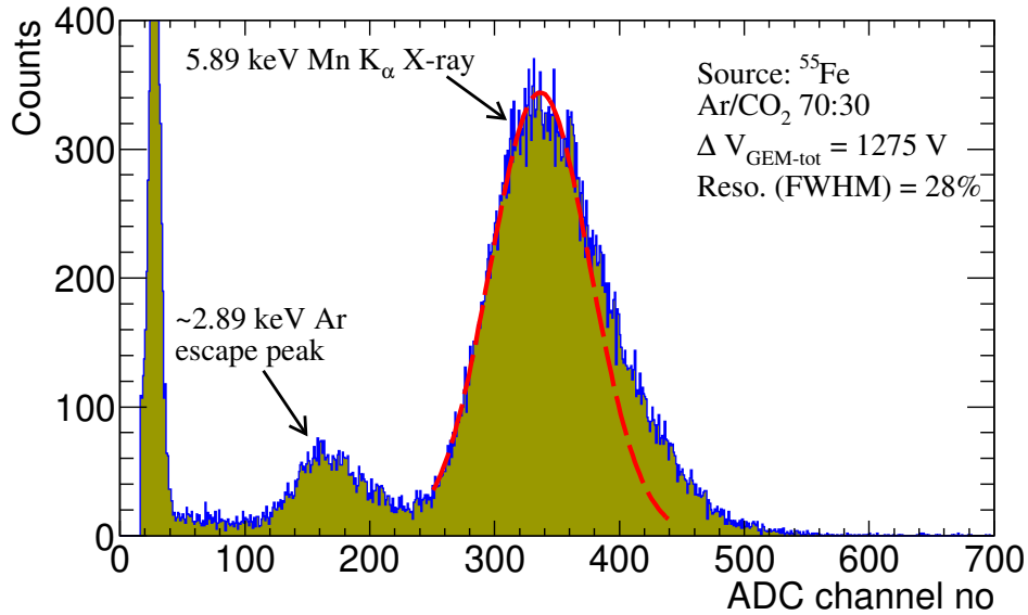
Figure 4.31: The energy spectrum of the quadruple GEM detector using the ^{55}\text{Fe} X-ray source. The peak at 2.89 keV corresponds to the Ar escape peak. The main photo peak corresponds to the X-ray of energy 5.89 keV.
