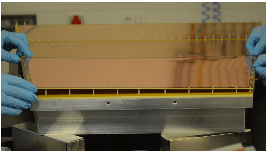
Figure 6.17: Stack of the GEM foils. Frame holes are aligned with the screw pillar.
