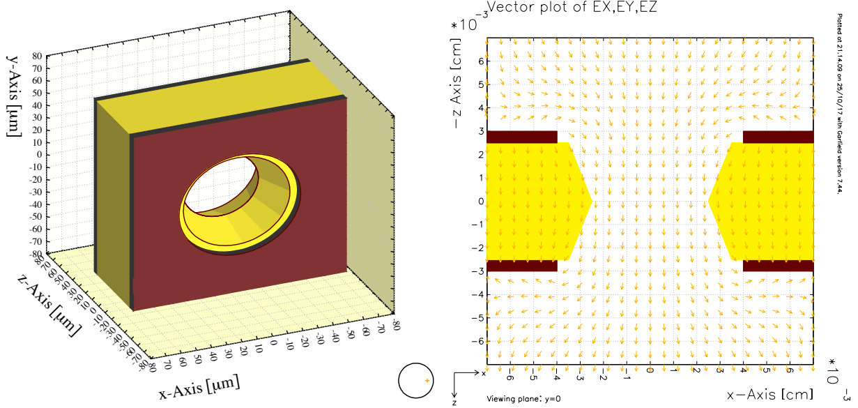
Figure 3.11: 3D view of a GEM hole in left panel. Electric field lines through the GEM holes in the right panel.
