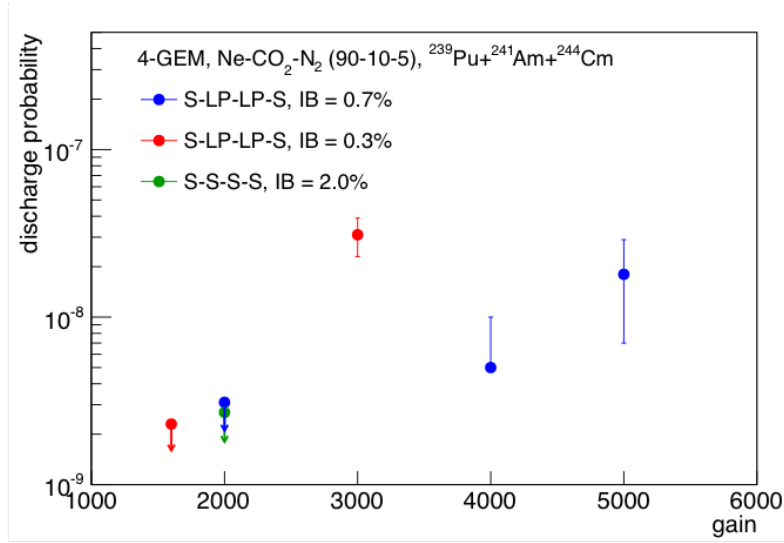
Figure 6.8: Discharge probability of a quadruple GEM detector measured for different gain. Corresponding values of ion backflow are indicated. Upper limits for discharge probability as indicated with arrows [88].
