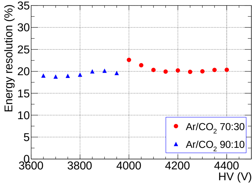
Figure 4.18: Energy resolution of the triple GEM detector as a function of HV for both Ar/CO 2 90:10 and 70:30 gas mixtures. Statistical errors are small and within the symbol size.
