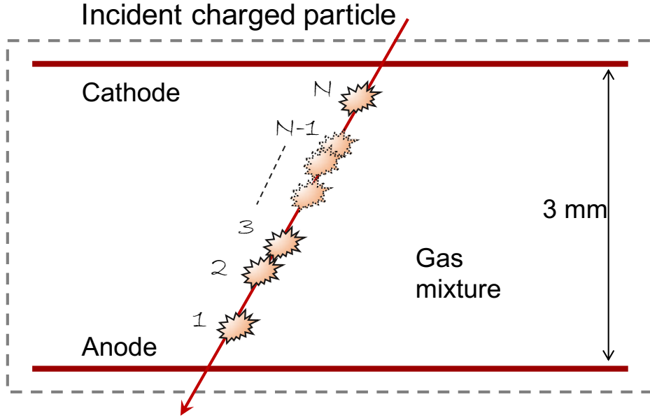
Figure 4.48: Schematic geometry of the time resolution simulation.
