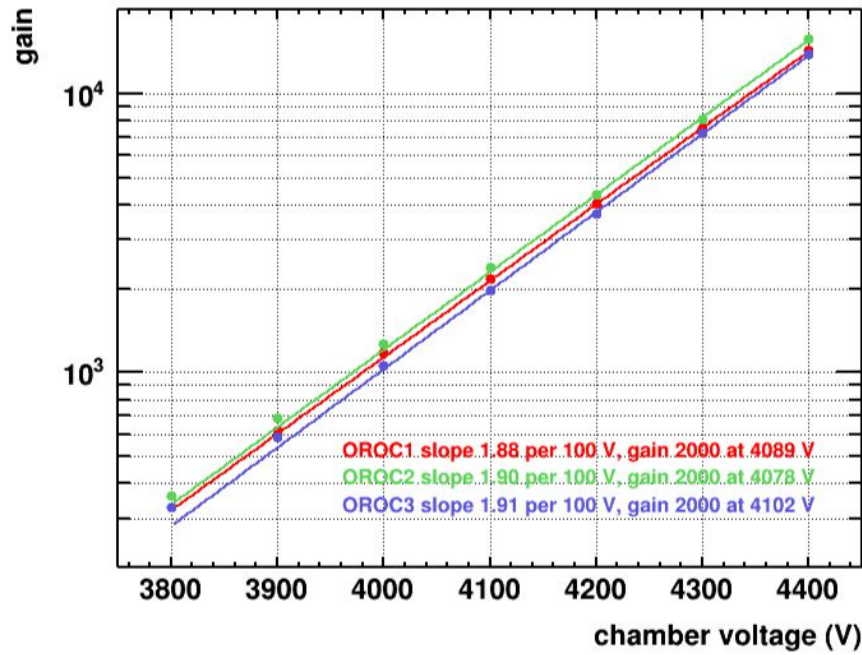
Figure 6.22: Effective gain variation as a function of applied voltage of the OROC. The voltage and the current associated with a gain of 2000 can calculate from the tangent of the fitting function.
