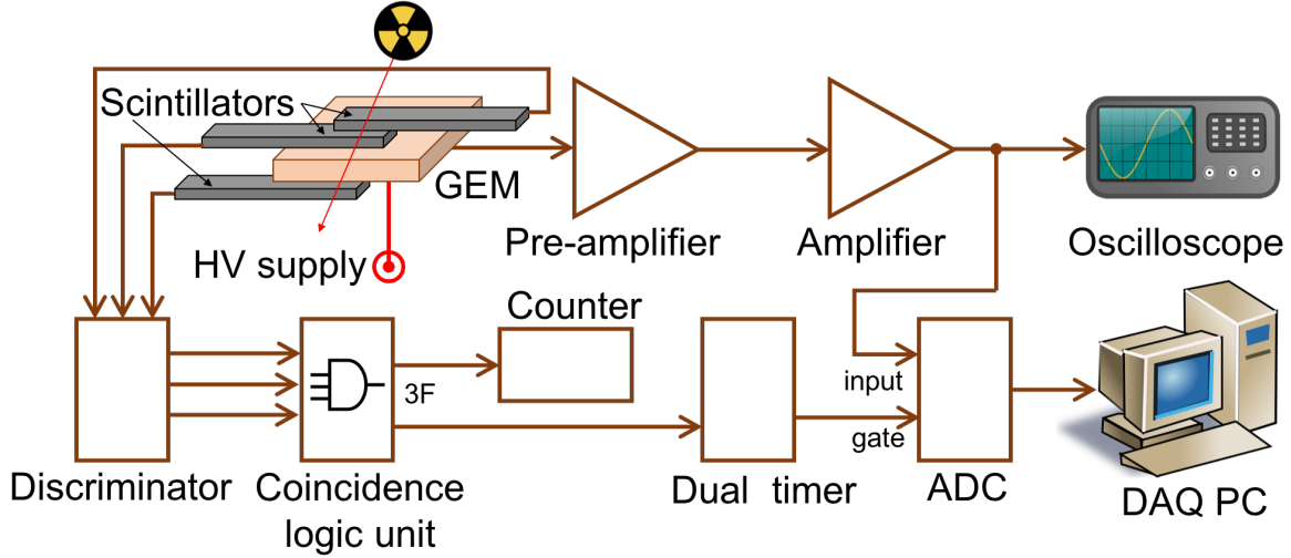
Figure 4.12: Electronics setup for the efficiency measurement of the triple GEM detector.
