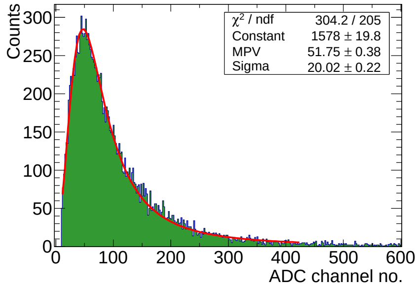
Figure 4.11: ^{106}\text{Ru-Rh} \beta^- -spectrum of the triple GEM detector at 4400 V. The spectrum with Ar/CO 2 70:30 gas.
