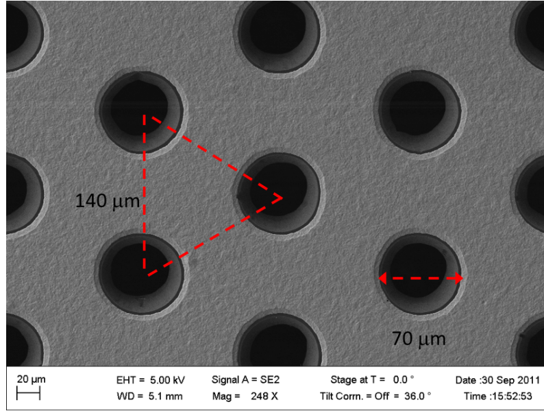
Figure 3.9: Electron microscope photograph of standard GEM foil on right.
