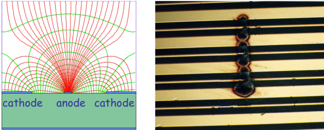
Figure 3.3: Schematic design of MSGCs in left panel and breakdown of strips due to discharges of MSGC in right panel.
