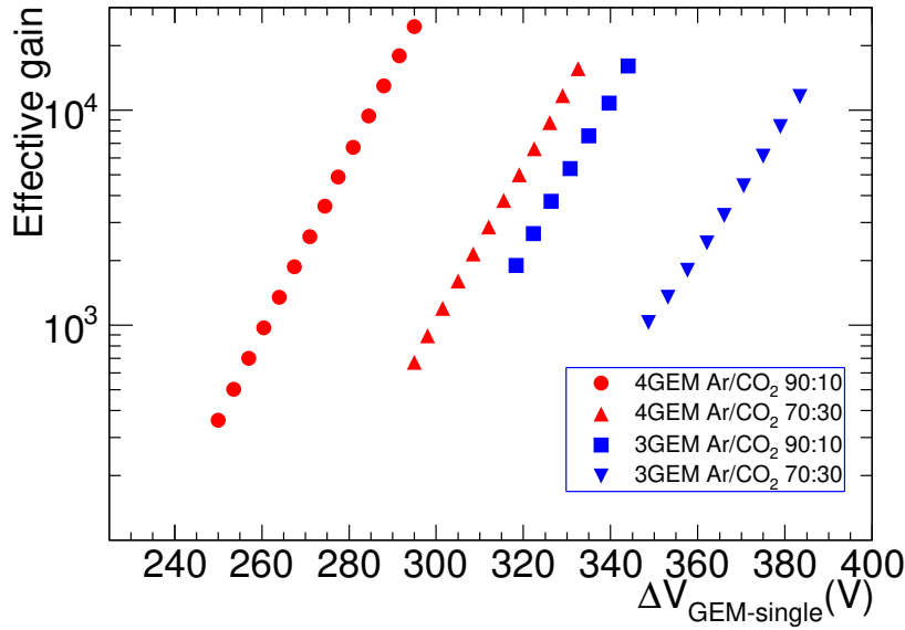
Figure 4.35: Effective gain as a function of \Delta V_{GEM-single} with different Ar/CO 2 gas mixtures for the quadruple GEM and triple GEM detectors. Statistical errors are small and within the symbol size.
