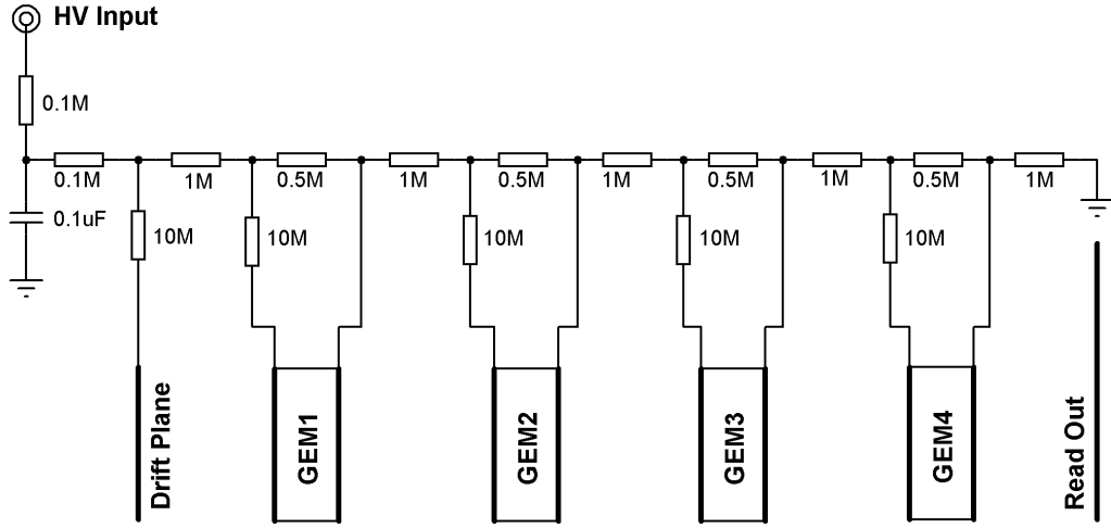
Figure 4.30: The voltage divider resistor chain used for standard field configuration of the quadruple GEM detector. The resistors' value in unit of M\Omega .
