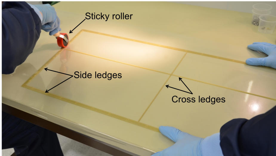
Figure 6.14: Gluing of the GEM frame.
