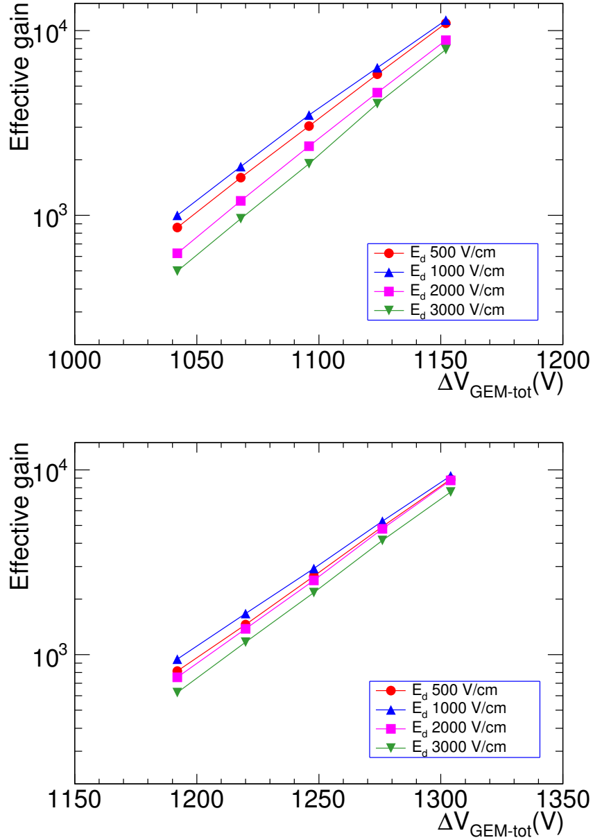
Figure 4.44: Gain variation as a function \Delta V_{GEM-tot} with different drift field ( E_d ) sets. (Top) Ar/CO 2 90:10 and (bottom) 70:30 gas mixtures. Statistical errors are small and within the symbol size.
