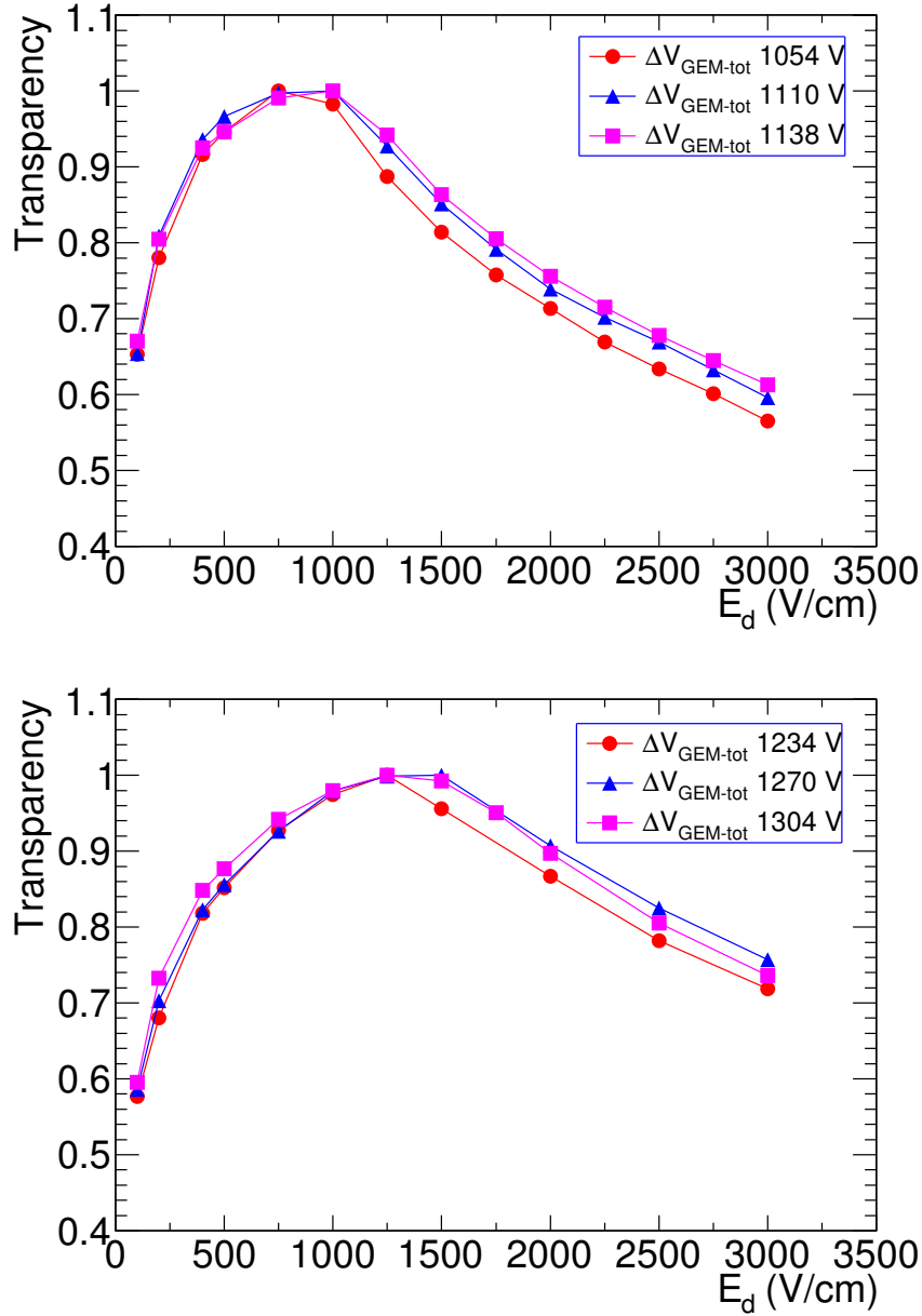
Figure 4.43: Electron transparency as a function of drift field ( E_d ). (Top) Ar/CO 2 90:10 and (bottom) 70:30 gas mixtures with different \Delta V_{\text{GEM-tot}} sets. Statistical errors are small and within the symbol size.
