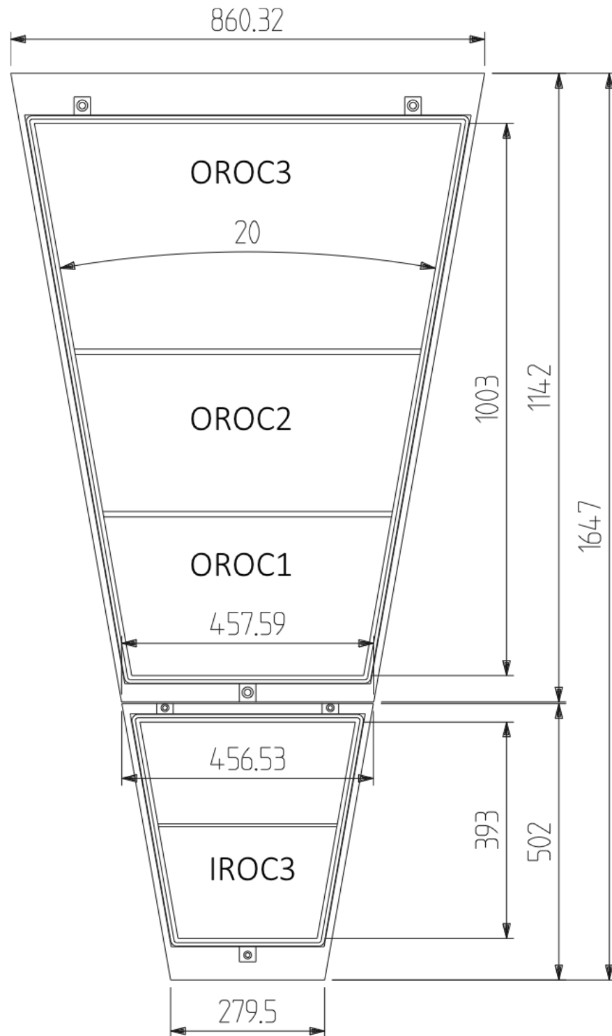
Figure 6.10: Design of TPC readout chamber. The dimension (mm) of the IROC and OROC are labeled. Each readout chamber cover 20^\circ . The figure is adopted from [30].
