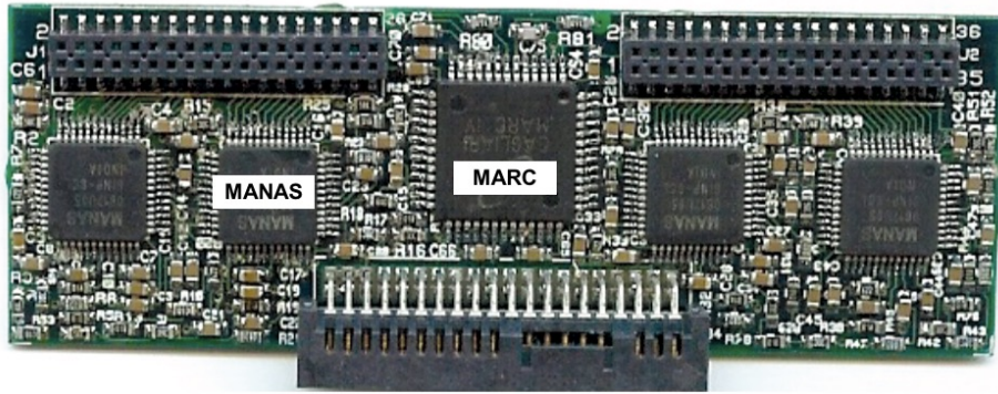
Figure 5.3: Photograph of a FEE board with MANAS and MARC chips.
