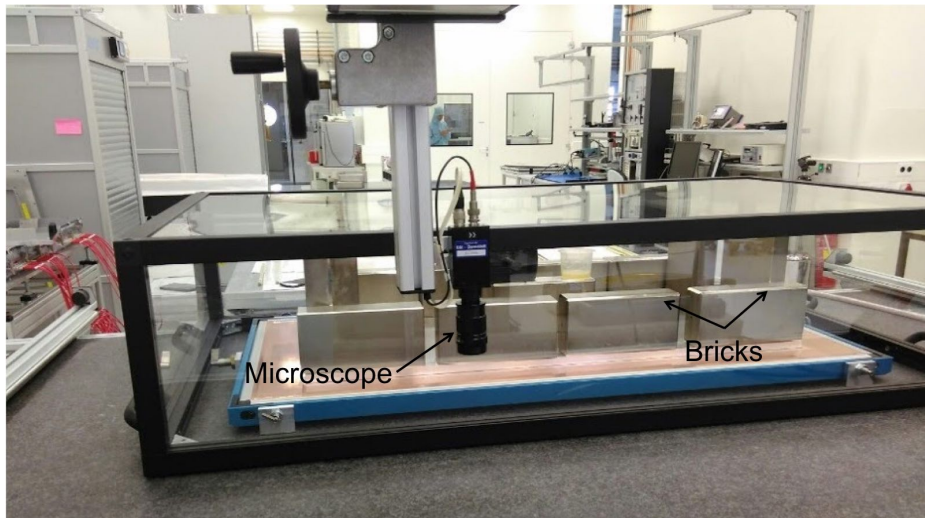
Figure 6.15: Gluing of the GEM foil. The foil is covered using a perspex box for keeping inside dry.
