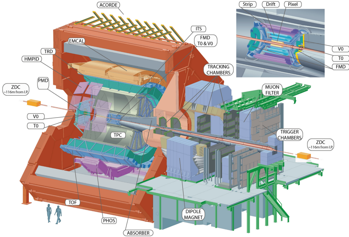
Figure 2.1: ALICE experiment labeled with all the detectors [41].
