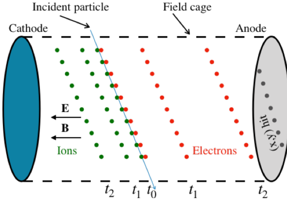
Figure 6.1: Schematic of the TPC detector. The red and green bullets are corresponding to the electrons and ions. Positions of the electrons at different time t_2 > t_1 > t_0 .
