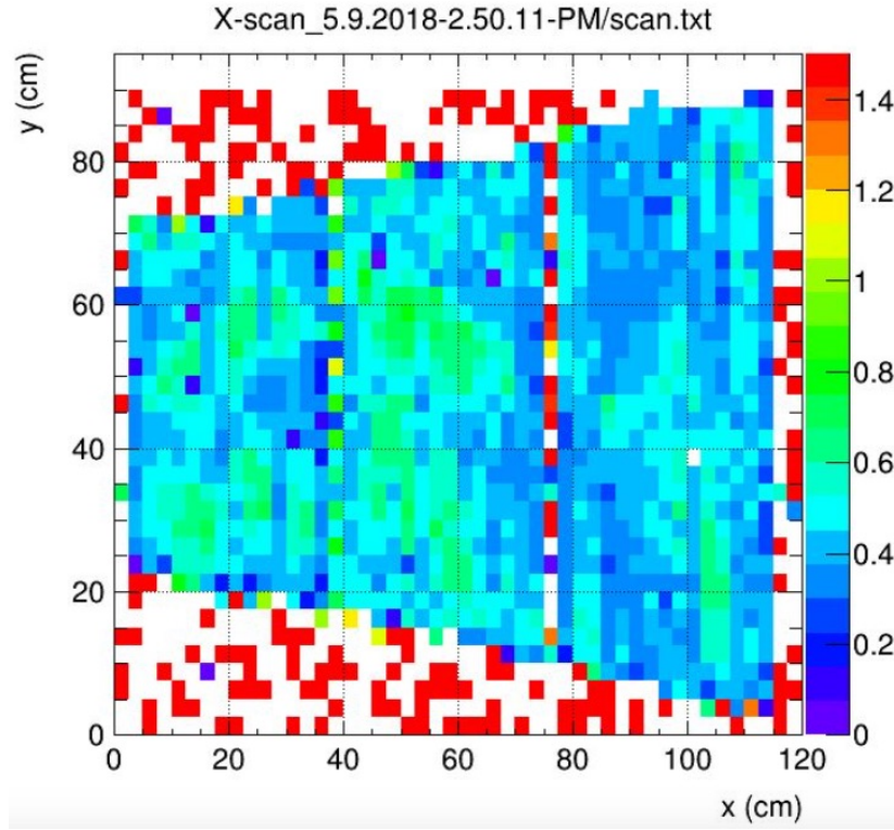
Figure 6.20: 2D distribution of ion backflow of a sample OROC.
