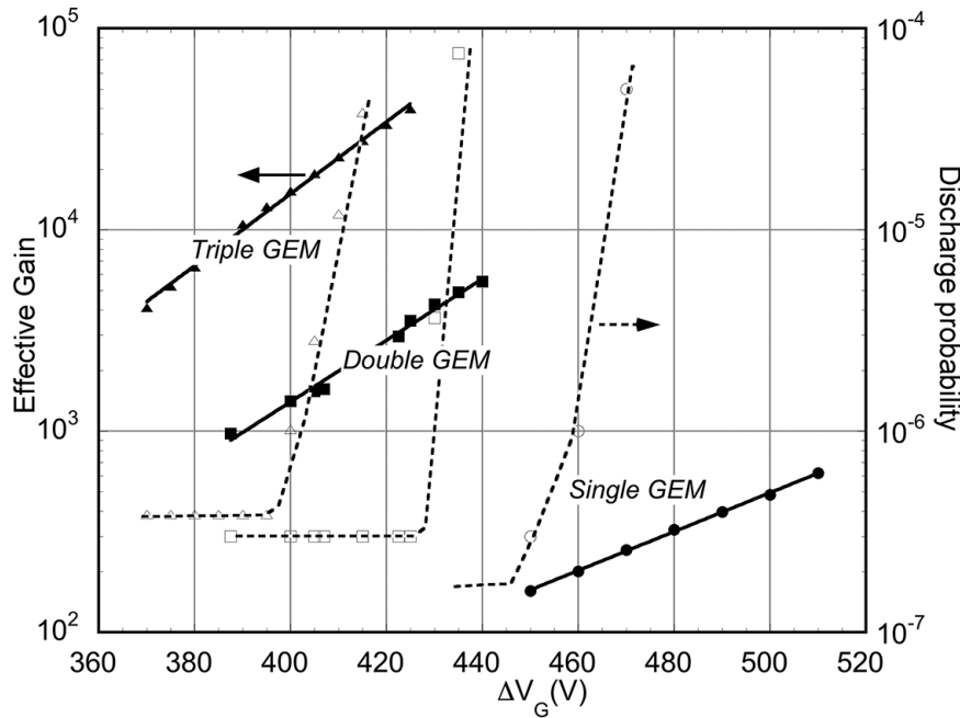
Figure 4.36: Gain and discharge probability variation with GEM voltages for a single, double and triple GEM detectors using \alpha -particle in Ar/CO 2 70:30 gas mixture [90].
