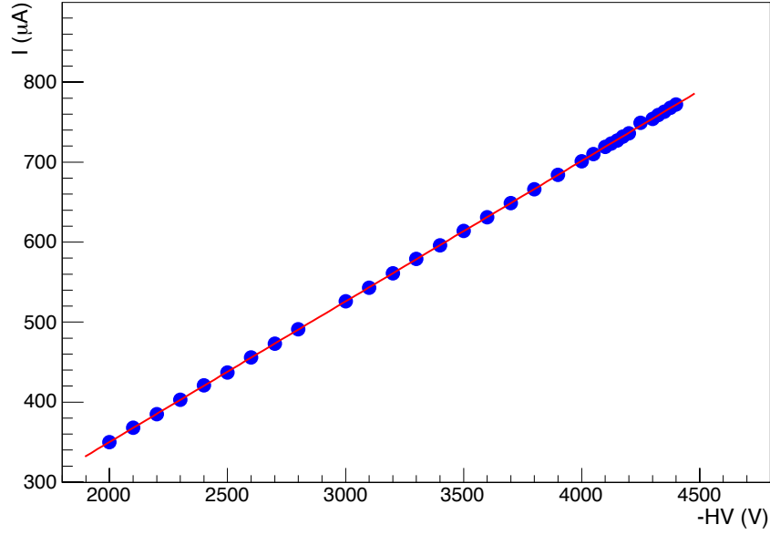
Figure 4.4: Ohmic characteristic of the voltage divider resistor chain. Current vs. voltage measurement.
