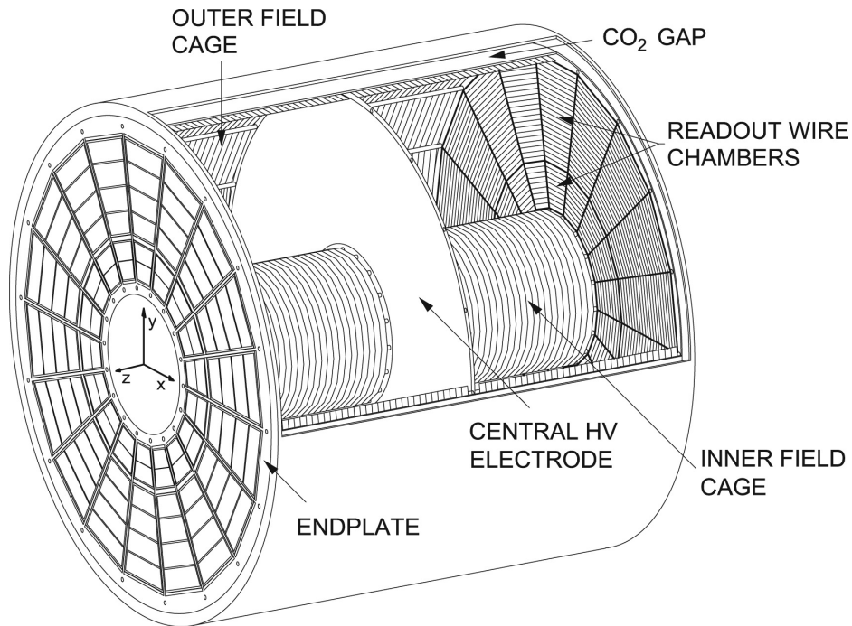
Figure 6.2: Schematic 3D design of the ALICE TPC detector. The high voltage electrode is located at the center of the drift volume. The endplates with 36 ( 18 \times 2 ) readout chambers on each end are shown. The figure is adopted from [118].
