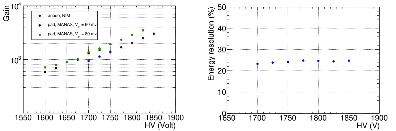
Figure 5.8: Measurement of gain using NIM and MANAS electronics in left panel and energy resolution (FWHM) of ^{55}\text{Fe} energy spectrum as a function of HV in right panel for the MWPC-1 detector. The measurements with Ar/CO 2 70:30 gas.
