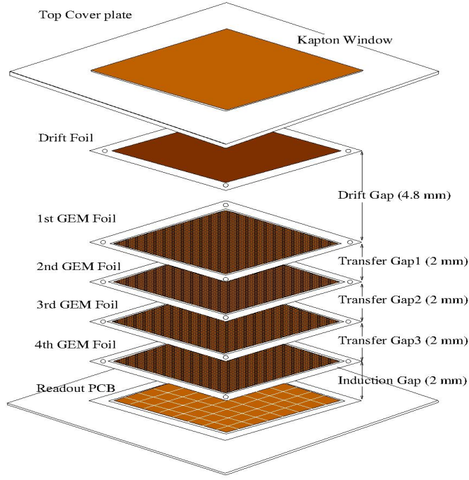
Figure 4.29: Schematic design of the quadruple GEM detector. Different components and the gas gaps are as labeled in the figure.
