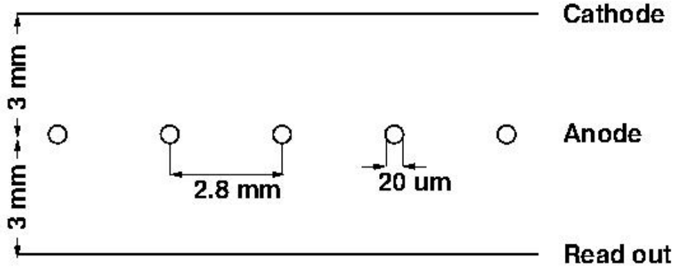
Figure 5.1: Schematic design of the MWPC detector.
