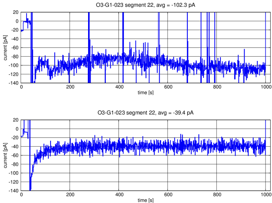
Figure 6.13: Sample plot, short-term leakage current measurement of individual GEM segment. The current plot on the top panel shows spurious current measurement. After recleaning the segment by air blow and tested with 550 V across it, current becomes normal as in the lower panel.
