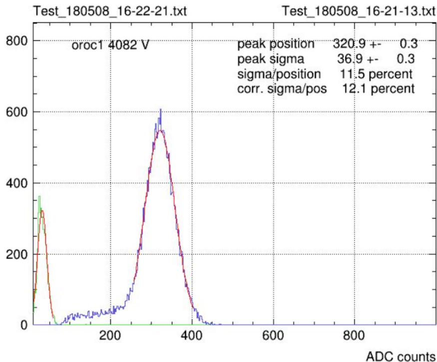
Figure 6.23: ^{55}\text{Fe} X-ray energy spectrum of the OROC in \text{Ne}/\text{CO}_2/\text{N}_2 (90:10:5) gas.
