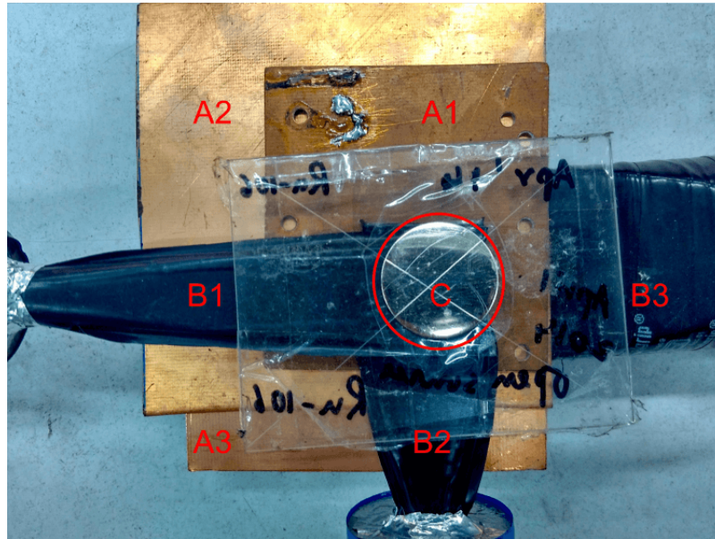
Figure 4.14: Photograph of the \beta^- penetration test using ^{106}\text{Ru-Rh} source. A1, A2, A3 are both side copper laminated FR4 sheets, B1 and B2 are two small scintillators on top. B3 is big scintillator at bottom.
