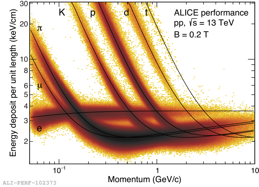
Figure 6.3: Particle identification performances of the ALICE TPC. Specific energy deposition dE/dx as a function of particle momentum [119].
