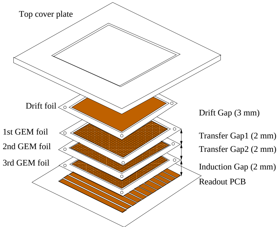
Figure 4.1: Schematic design of the triple GEM detector.
