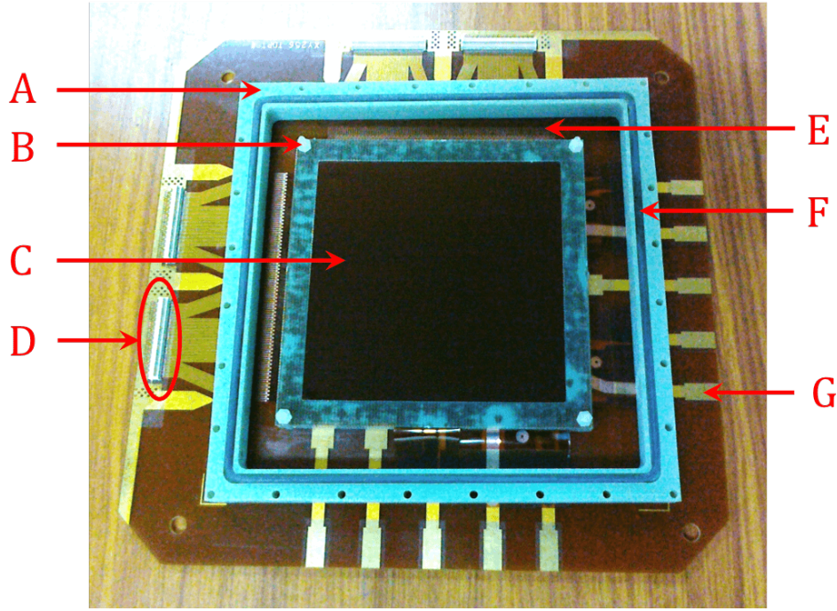
Figure 4.2: Components of the GEM detector: A - Edge frame, B - Nylon screw, C - GEM foil, D - Readout connector, E - readout strips, F - Gas tightness O-ring, G - HV strips for the GEM voltage supply.
