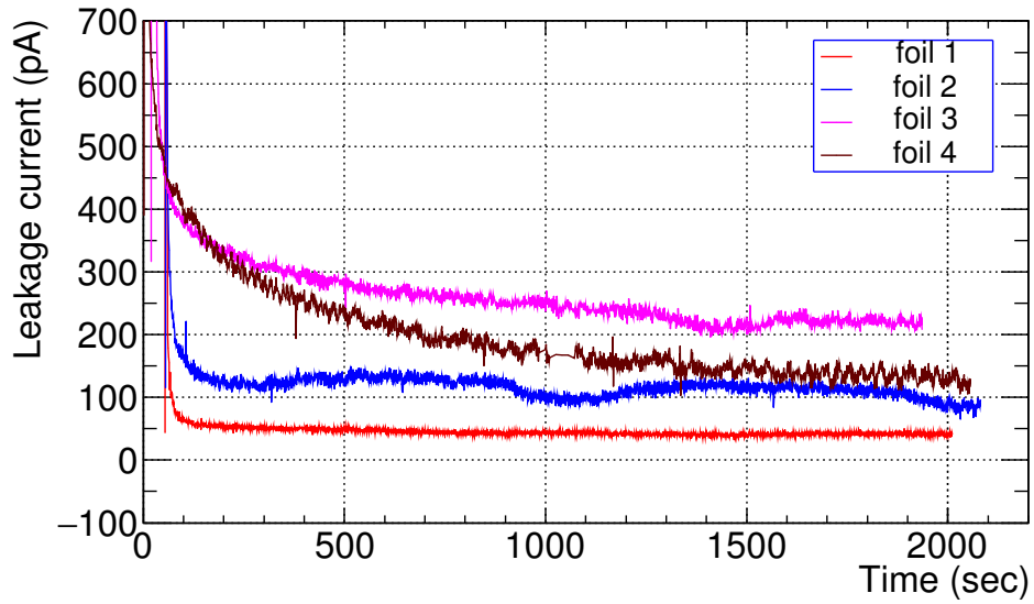
Figure 4.28: Leakage current measurement of the GEM foils.
