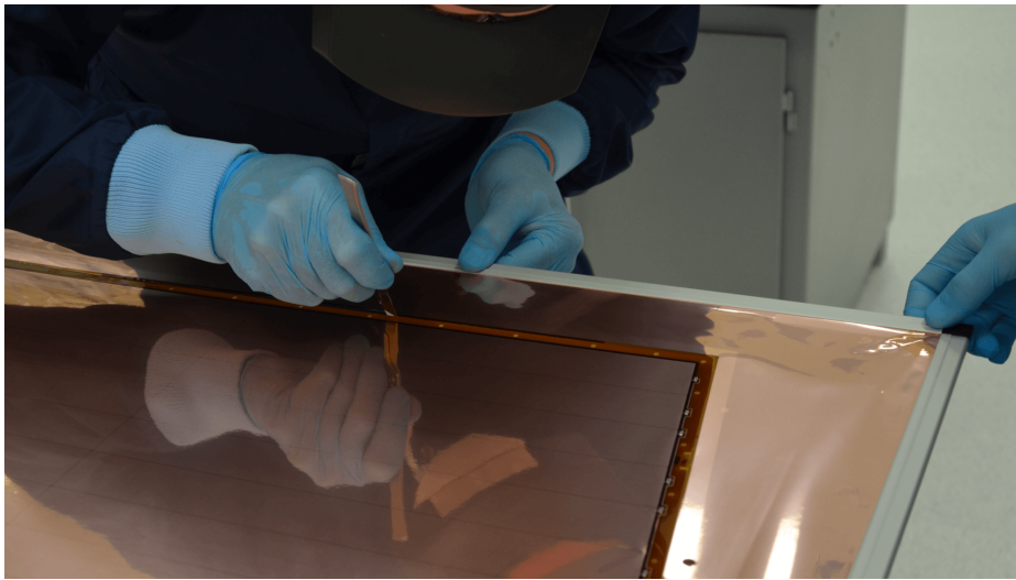
Figure 6.16: Cutout of the active area of a GEM foil.
