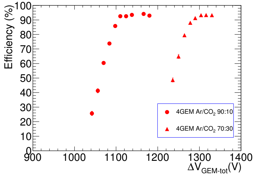
Figure 4.34: Efficiency of the quadruple GEM detector as a function of \Delta V_{GEM-tot} is presented for both the Ar/CO 2 gas mixtures. Statistical errors are small and within the symbol size.
