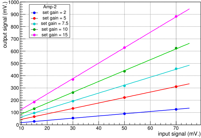
Figure 4.6: Gain calibration plot of the spectroscopic amplifier (ORTEC 572A).
