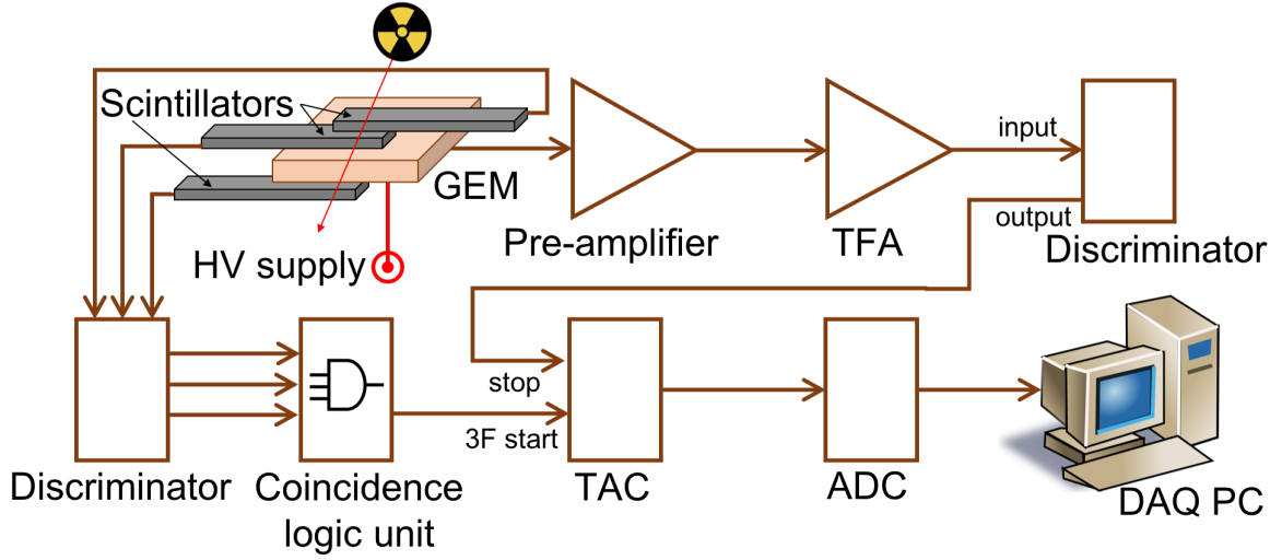
Figure 4.19: Schematic of the detector setup for the time resolution measurement.
