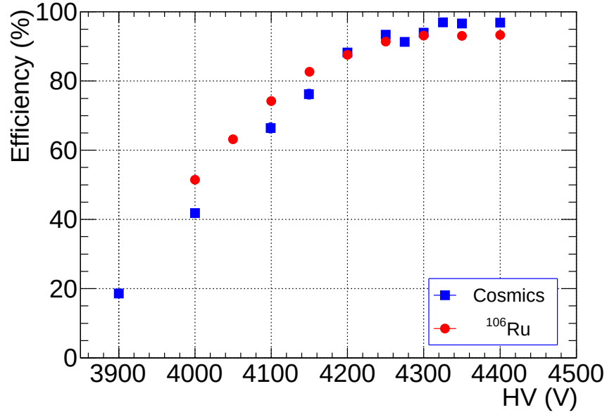
Figure 4.15: Efficiency measurement of the triple GEM detector as a function of applied HV. The efficiency is obtained by using cosmic muon and ^{106}\text{Ru} -Rh source with Ar/ \text{CO}_2 70:30 gas. Statistical errors are small and within the symbol size.
