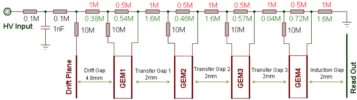
Figure 4.38: Voltage divider resistor chain. Values (in M\Omega ) in red upper are for standard and in green lower are for IBF settings. Resistors of drift and transfer gap-3 are changed with 1 and 0.34, respectively for Ar/ CO_2 70:30 in IBF setting.
