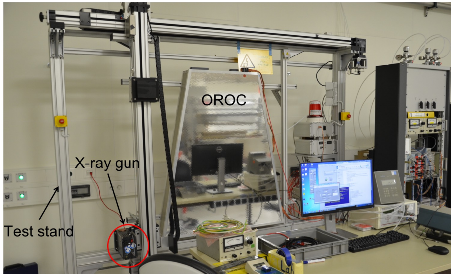
Figure 6.18: X-ray test station of the OROC.
