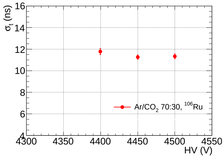
Figure 4.21: Time resolution of the triple GEM detector as a function of applied HV. Statistical errors are small and within the symbol size.
