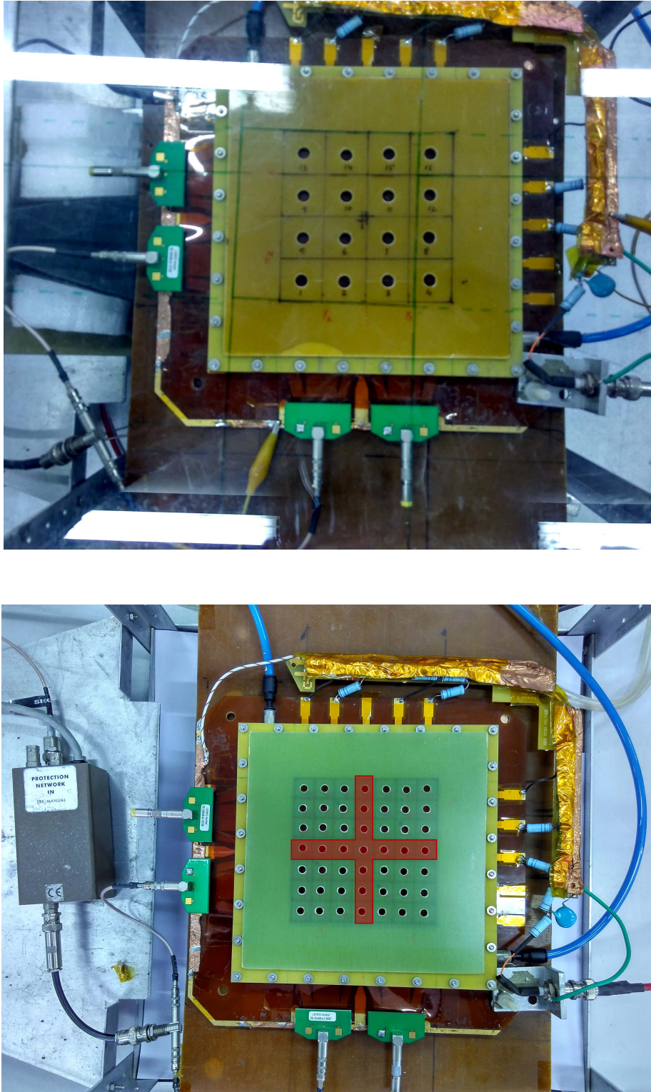
Figure 4.22: Photograph of the detector setup for uniformity measurement of the triple GEM detector. The upper panel is for 4 \times 4 hole matrices and the lower panel is for 7 \times 7 hole matrices.
