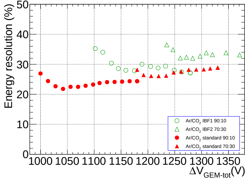
Figure 4.40: Energy resolution as a function of total GEM voltage ( \Delta V_{GEM-tot} ) with different field setting of the quadruple GEM detector. Results with IBF field setting is in open bullets and standard setting is in solid bullets. Statistical errors are small and within the symbol size.
