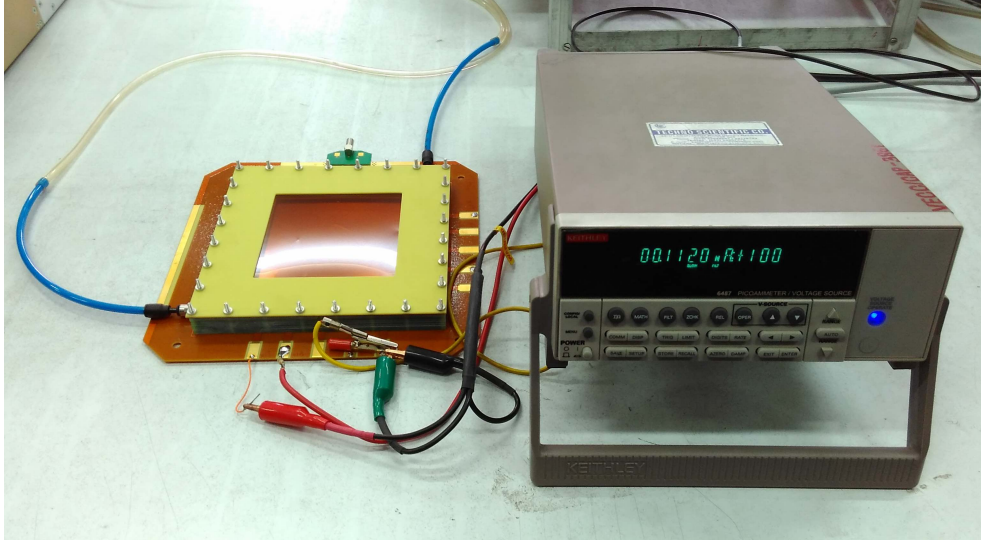
Figure 4.27: Photograph of the leakage current measurement setup of the GEM foils.
