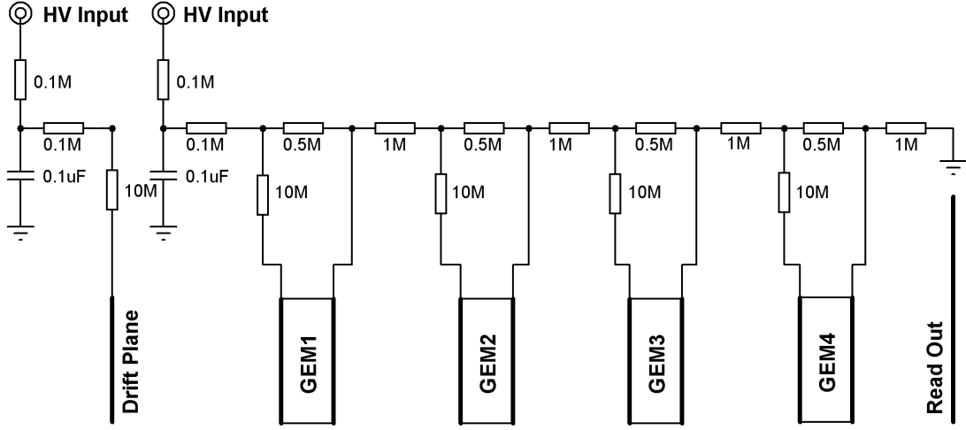
Figure 4.42: Voltage divider resistor chain for independent drift field ( E_d ) configuration.
