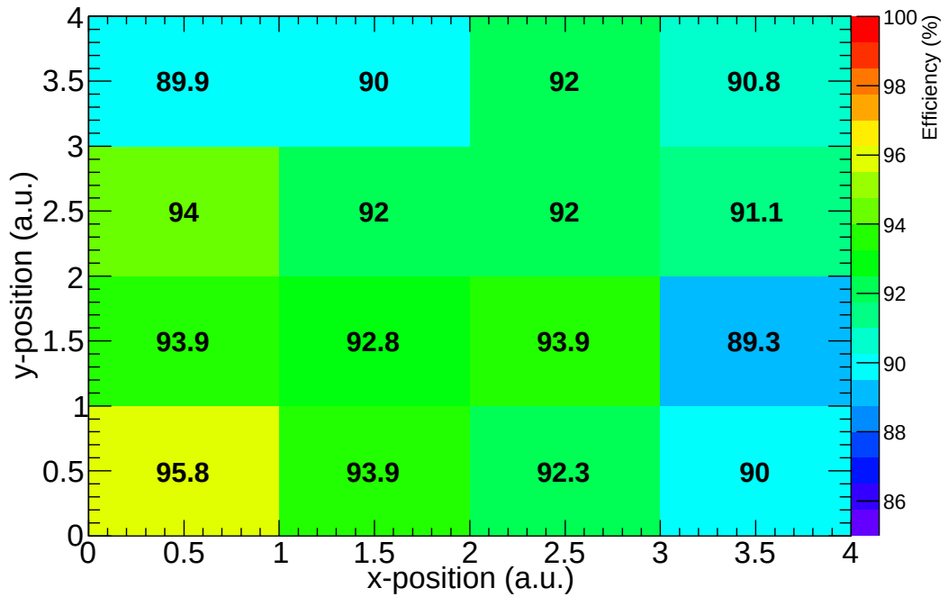
Figure 4.26: 2D mapping of the efficiency measurement of the triple GEM detector for the 16 zones at an applied voltage of 4400 V for 4 \times 4 matrices.
