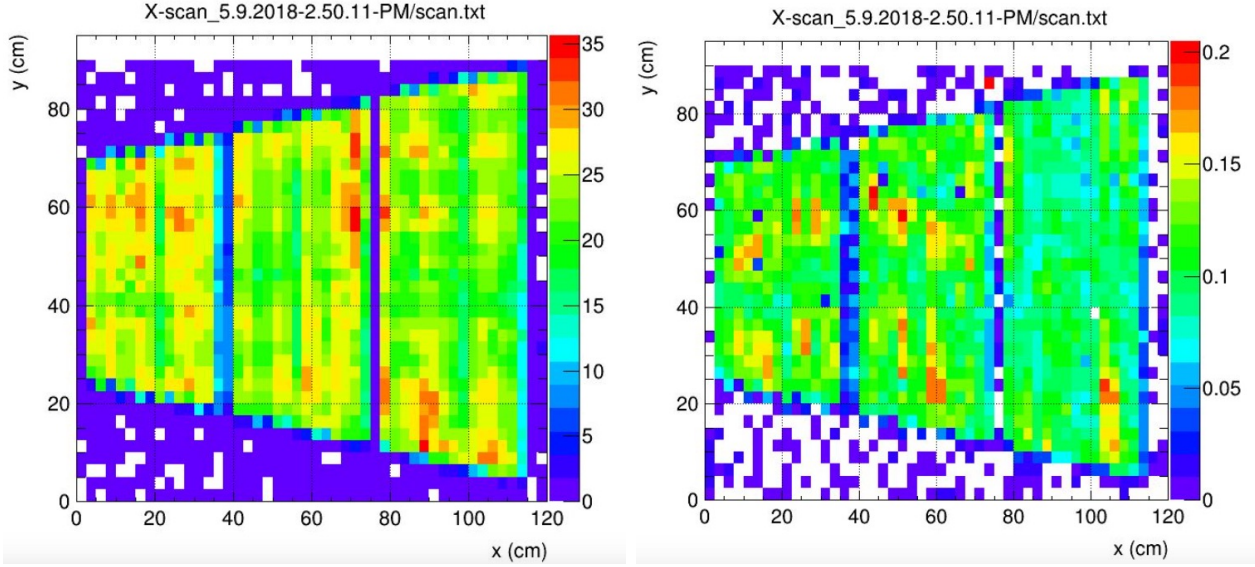
Figure 6.19: x, y -scan of the gain of an OROC using an X-ray gun. Readout pad current in the left panel and cathode current in the right panel.
