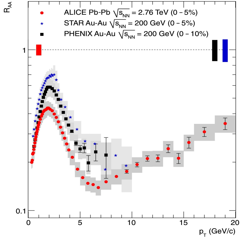
Figure 1.8: Nuclear modification factor R_{AA} as a function of p_T . Data from central Pb-Pb collisions at LHC and Au-Au collision at RHIC are compared. Figure is adopted from [24]
