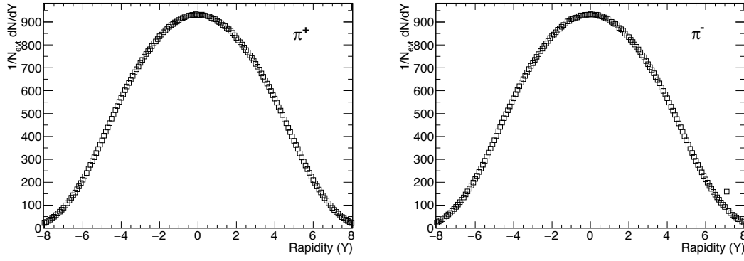
Figure 7.6: Rapidity density distribution of \pi^+ and \pi^- for 0 – 5% central Pb-Pb collision at \sqrt{s_{\text{NN}}} = 5.5 TeV. Results are from AMPT model calculation.
