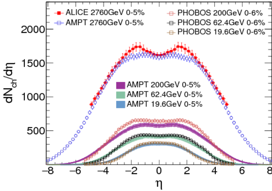
Figure 7.3: Beam energy dependency of charged particle pseudorapidity distributions. Results of most central collision from PHOBOS [137] and ALICE [138, 139] are shown along with calculations from AMPT model [136].
