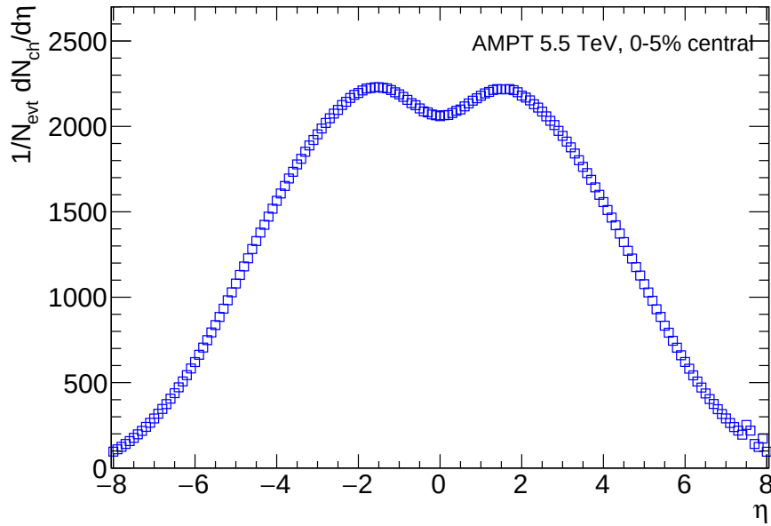
Figure 7.4: Charged particle pseudorapidity distributions. Result for Pb-Pb 0-5% central collisions of \sqrt{s_{NN}} = 5.5 TeV calculated using AMPT model, string melting mode.
