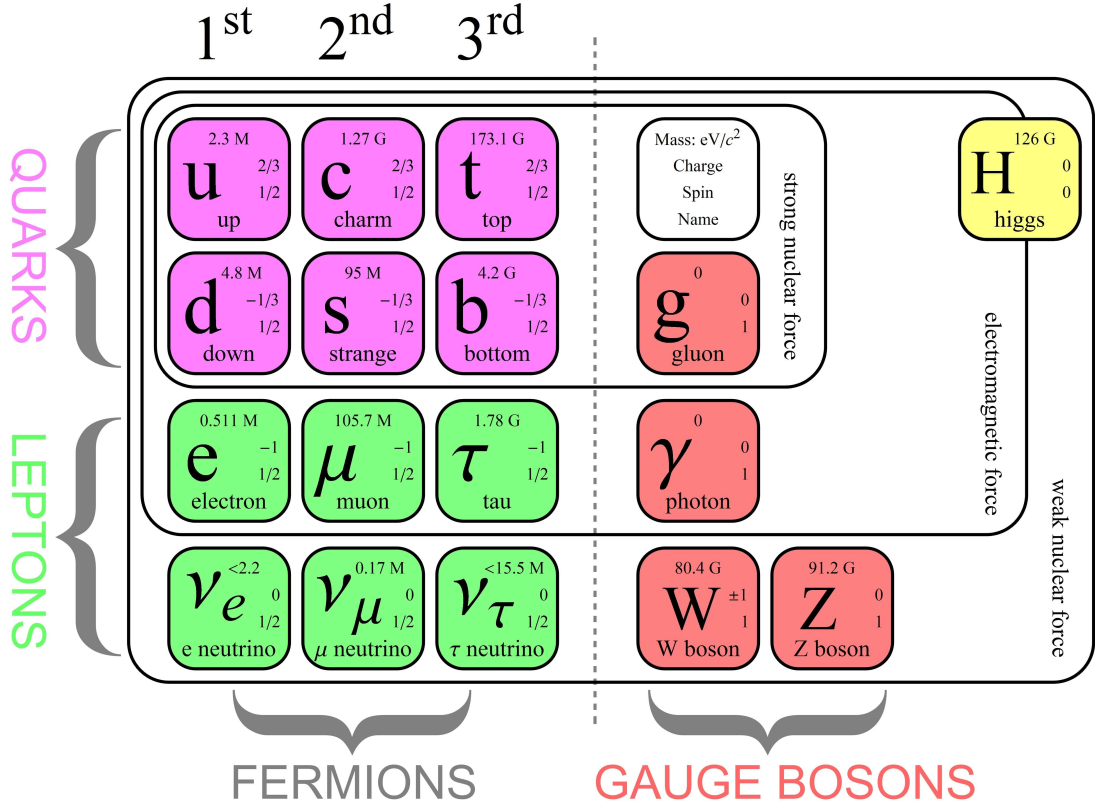
Figure 1.1: Standard model of particle physics: fundamental particles and mediators of the fundamental forces.
