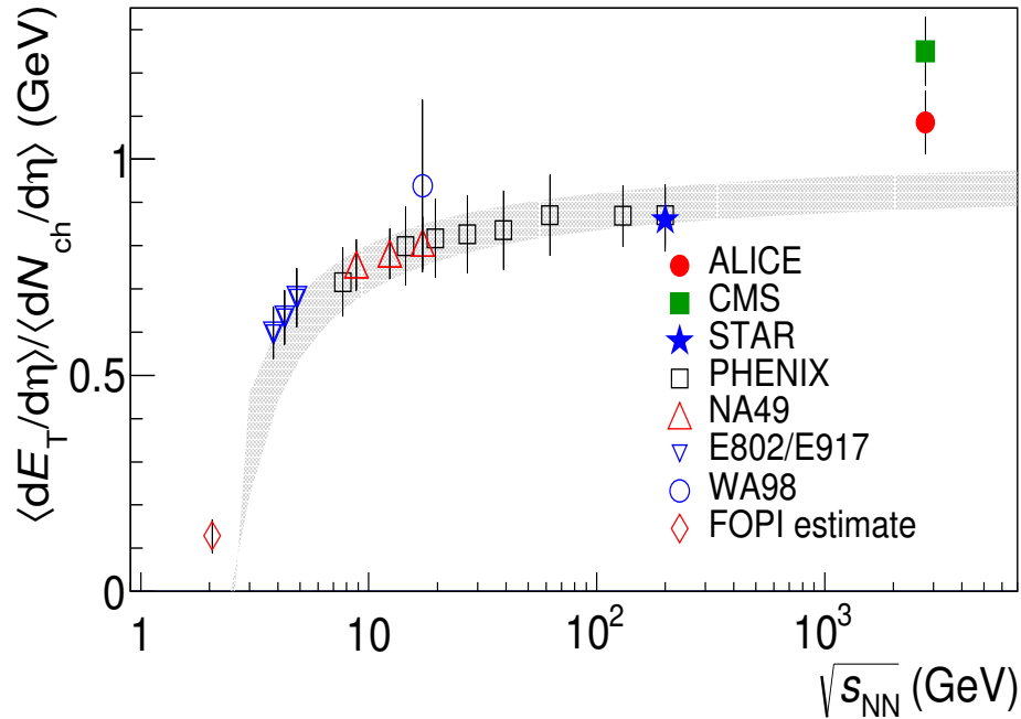
Figure 1.7: Energy dependence of the ratio of the mean transverse energy density over the mean charged particle density. Data from different experimental facilities. Figure is adopted from [23].
