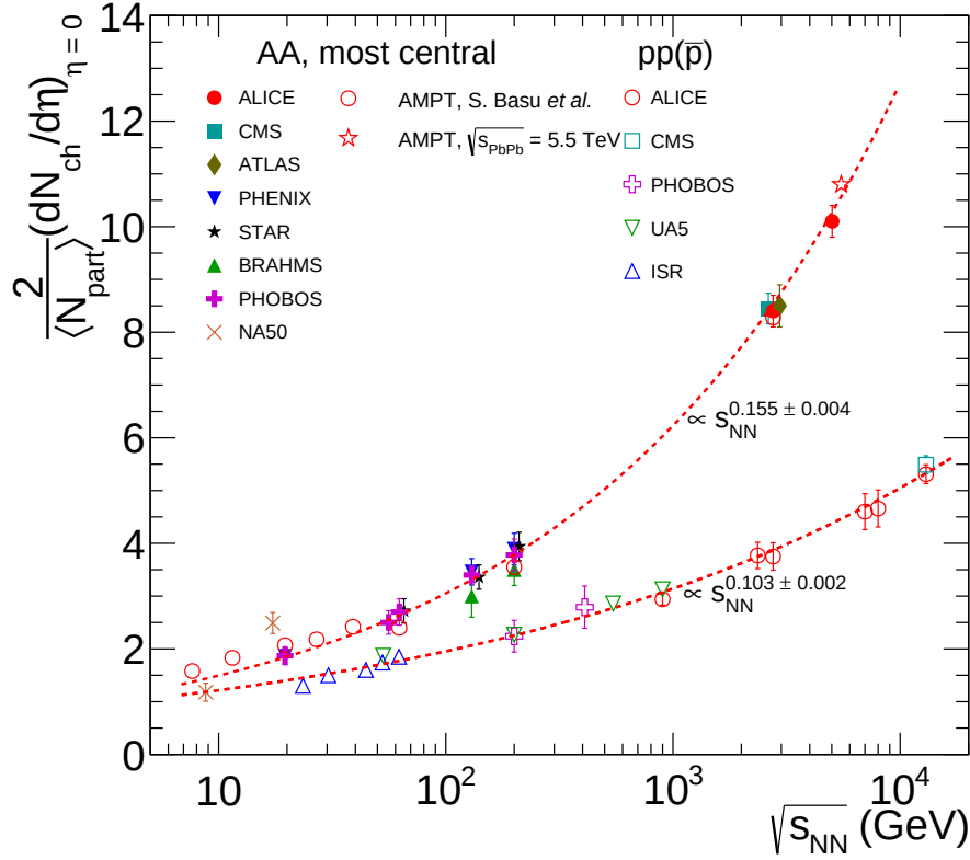
Figure 7.7: Variation of (2/\langle N_{part} \rangle)dN_{ch}/d\eta for most central collision in A-A as a function of \sqrt{s_{NN}} . Experimental data for central Pb-Pb [140–142, 147] and Au-Au [137, 143–146], and pp( \bar{p} ) [137, 148–152]. collisions. AMPT calculation from [136].
