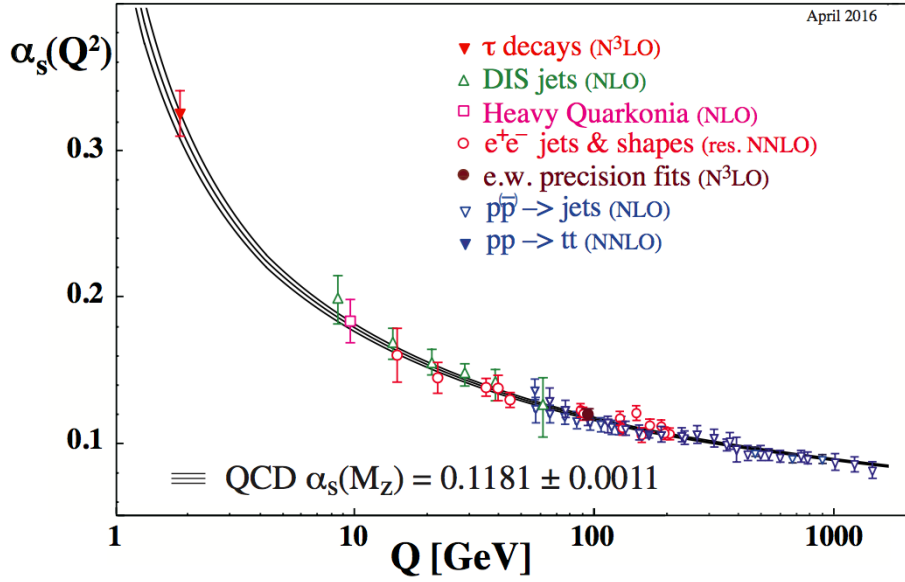
Figure 1.2: Coupling constant as a function of energy scale from different experimental results. The figure is adopted from [11].
