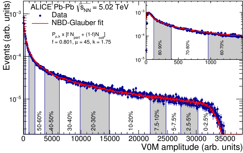
Figure 7.2: Collision centrality determination from the multiplicity measurement in ALICE. The distribution of the sum of the amplitudes in the ALICE V0 detector. The inset shows a zoom of the most peripheral region. The vertical lines separate the centrality classes. Figure is adopted from [134].
