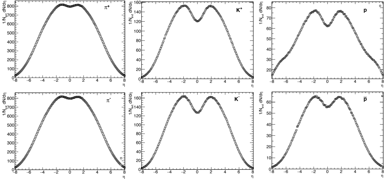
Figure 7.5: Pseudorapidity density distribution of \pi^\pm , K^\pm , p , \bar{p} for 0 – 5% central Pb-Pb collision at \sqrt{s_{\text{NN}}} = 5.5 TeV. Results are from AMPT model calculation.
