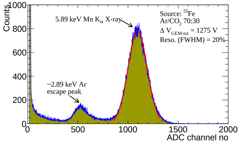
Figure 4.8: The obtained energy spectrum of the ^{55}\text{Fe} X-ray source of the triple GEM detector. The peak at \sim 2.89 \text{ keV} correspond to the Ar escape peak. The main photopeak correspond to the K_\alpha X-ray of energy 5.89 \text{ keV} .
