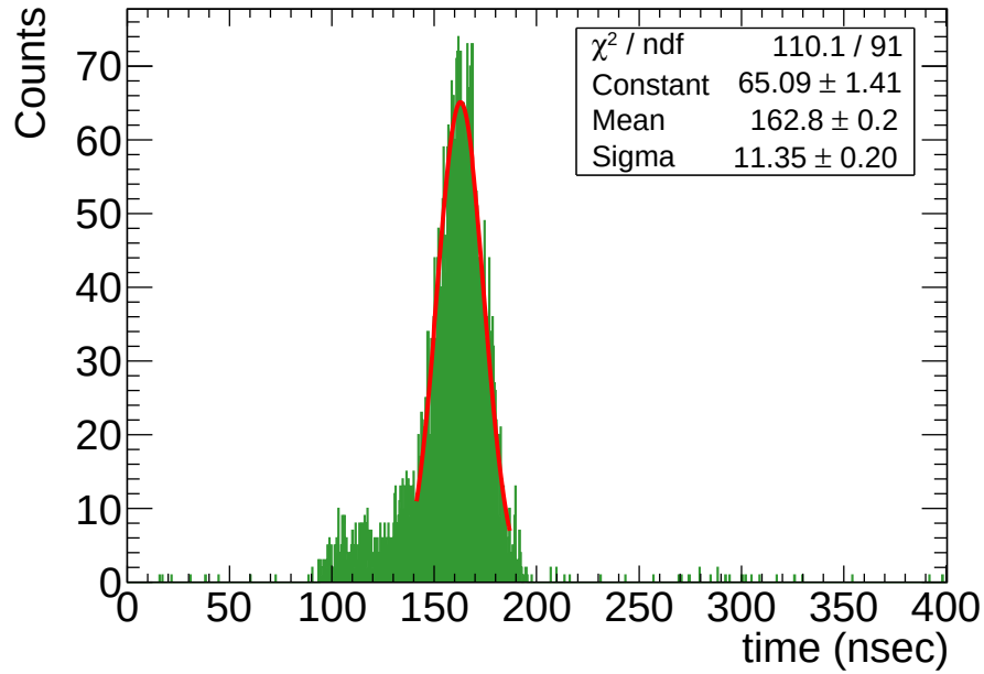
Figure 4.20: Time spectrum of the triple GEM detector at 4450 V in Ar/CO 2 70:30 gas.
