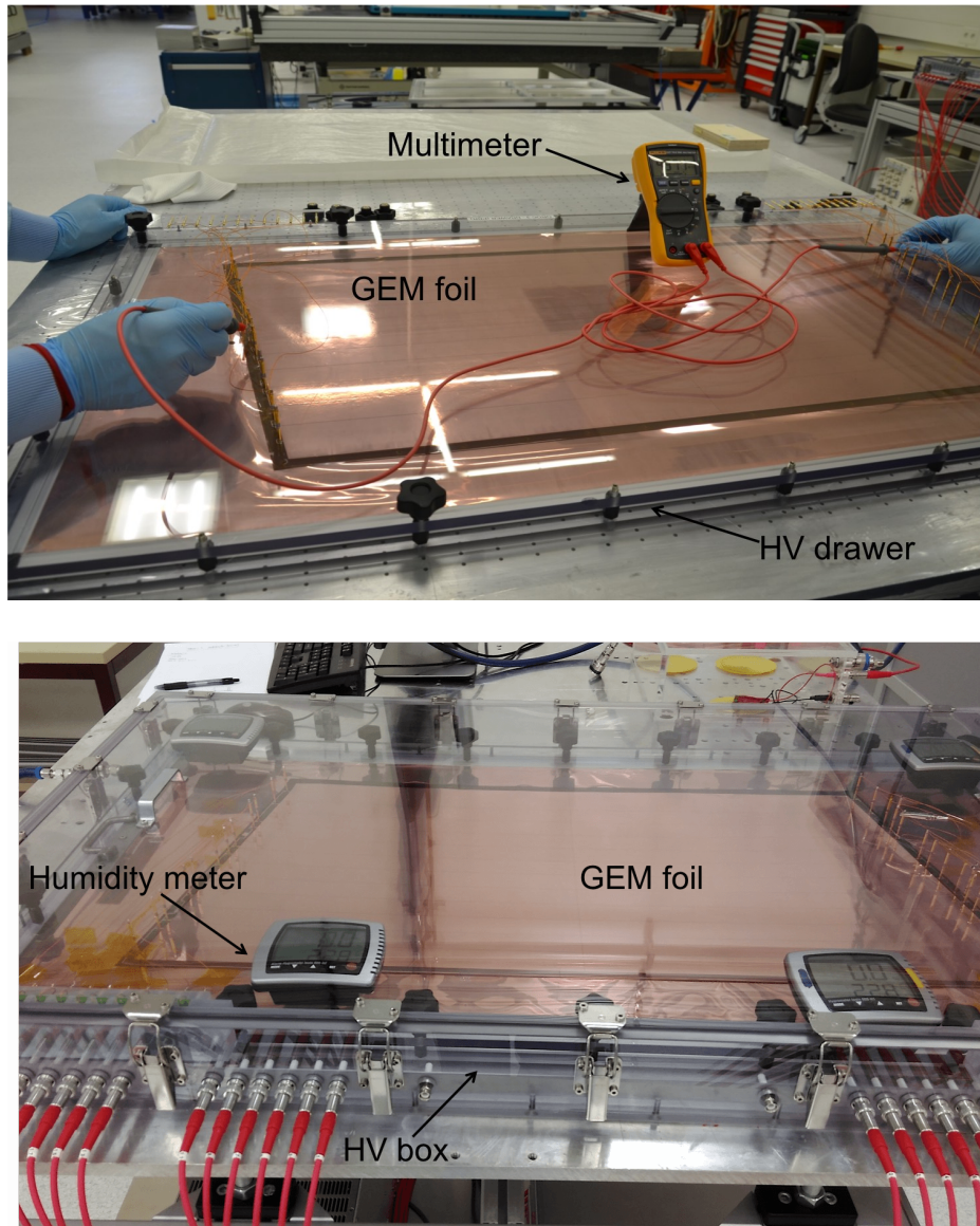
Figure 6.11: The resistance measurement of a GEM foil inside the HV drawer in top panel. Leakage current measurement of the GEM foil in HV box in bottom panel. Different components are labeled. N_2 gas flowed for dryness within the HV box.
