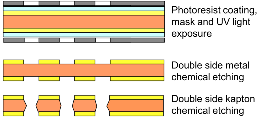
Figure 3.7: GEM foil fabrication steps using double-mask photolithographic technology.
