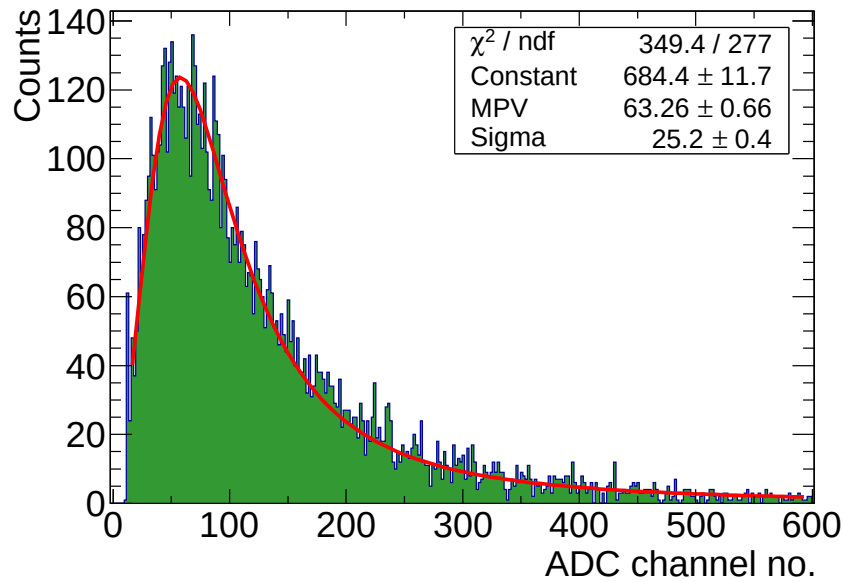
Figure 4.10: Cosmic muon spectrum of the triple GEM detector at 4400 V. The spectrum with Ar/CO 2 70:30 gas.
