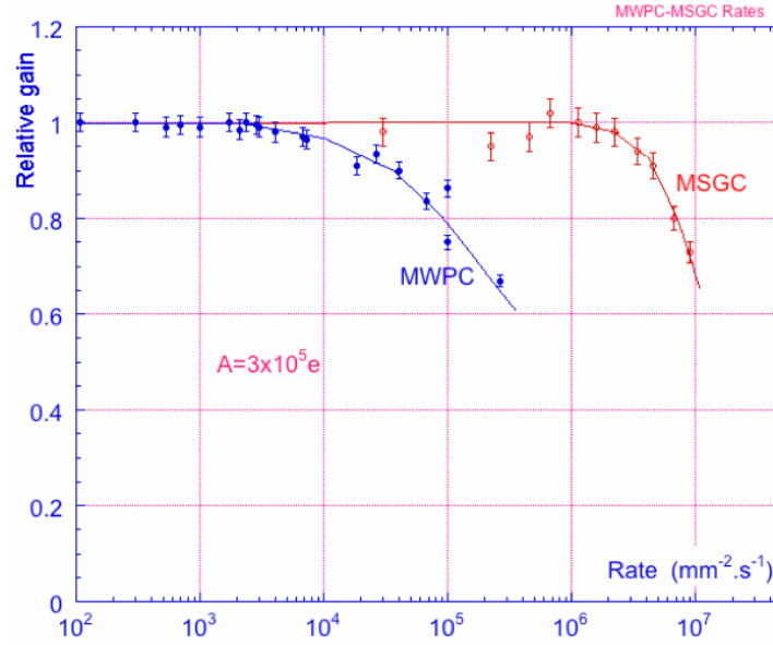
Figure 3.4: Gain as a function of particle rate for both the MWPC and the MSGC.
