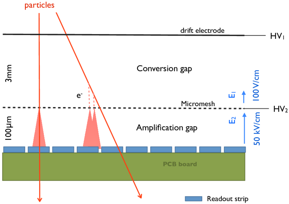
Figure 3.5: Schematic design with operating principle of Micromegas detector.
