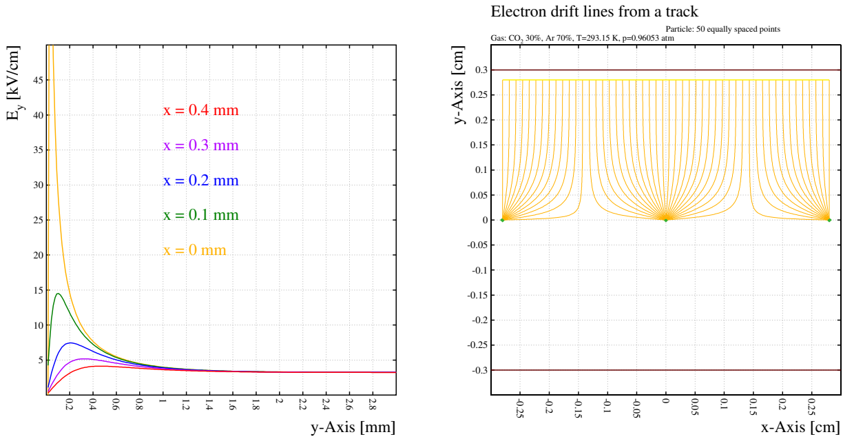
Figure 5.2: Variation of the electric field in space in left panel. Drift line following by the electrons are shown in right panel.
