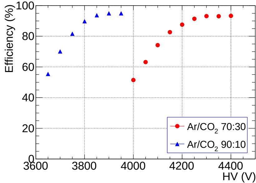
Figure 4.16: Efficiency measurement of the triple GEM detector as a function of applied HV. The efficiency is obtained by using ^{106}\text{Ru} -Rh source with Ar/ \text{CO}_2 90:10 and 70:30 gas. Statistical errors are small and within the symbol size.
