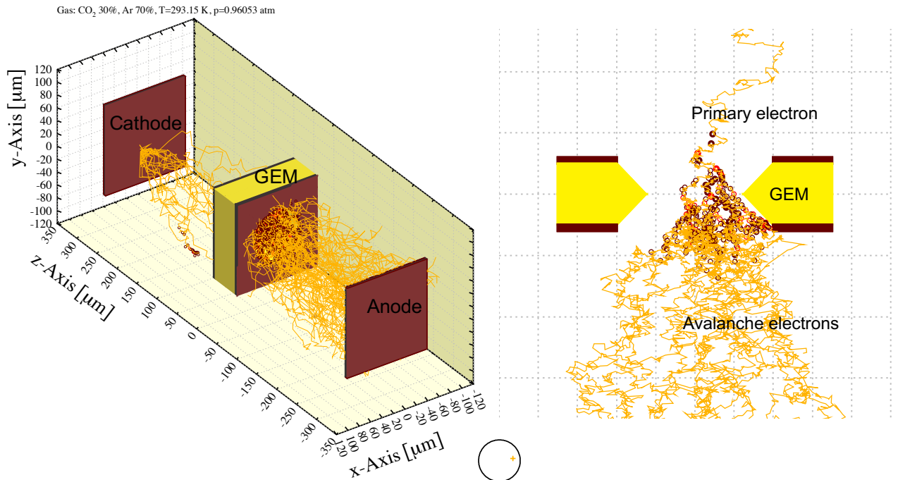
Figure 3.12: Simulation of electron avalanche within the GEM hole using Garfield.
