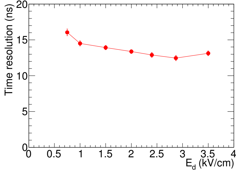
Figure 4.46: Time resolution as a function of drift field of the quadruple GEM detector. Applied gas is Ar/CO 2 70:30. Statistical errors are small and within the symbol size.
