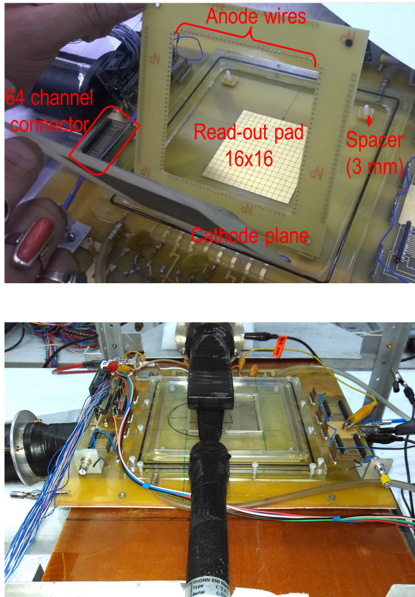
Figure 5.4: Components of the MWPC detector are labeled in upper panel. Laboratory setup picture of the MWPC in lower panel.
