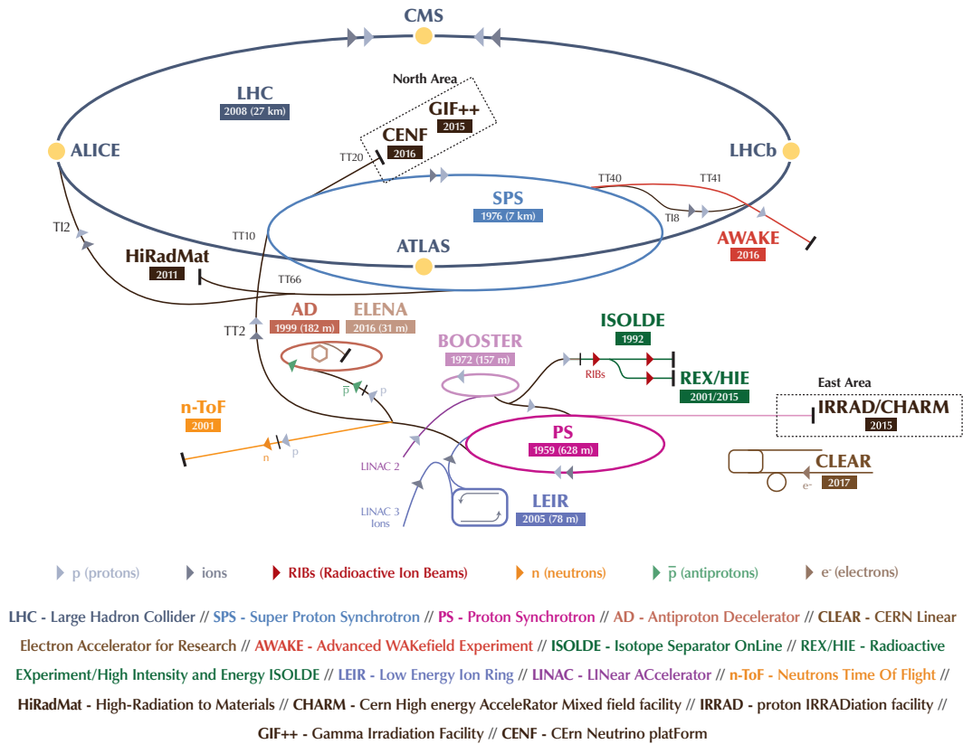
Figure 1.5: Schematic view of CERN accelerator complex and its four experiments. Figure is adopted from [20].
