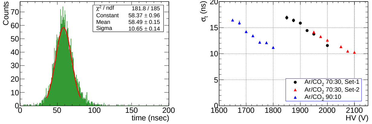
Figure 5.12: Time spectrum of MWPC-2 at 2075 V for Ar/CO 2 70:30 gas in left panel. Time resolution variation as a function of applied HV for Ar/CO 2 90:10 and 70:30 gas mixtures in the right panel.
