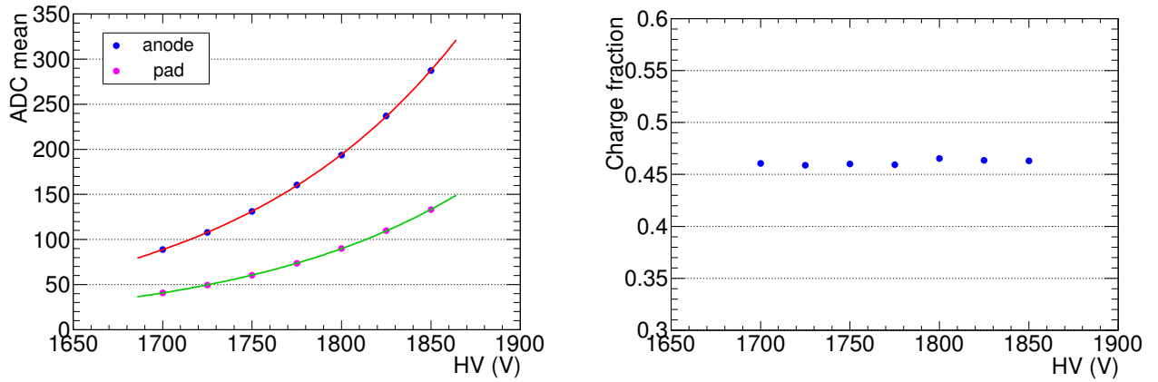
Figure 5.7: The variation of the ADC mean of the ^{55}\text{Fe} photopeak as a function of HV using NIM electronics in left panel and fraction of the avalanche charge induced in pad plane as a function of HV in right panel for MWPC-1 detector.
