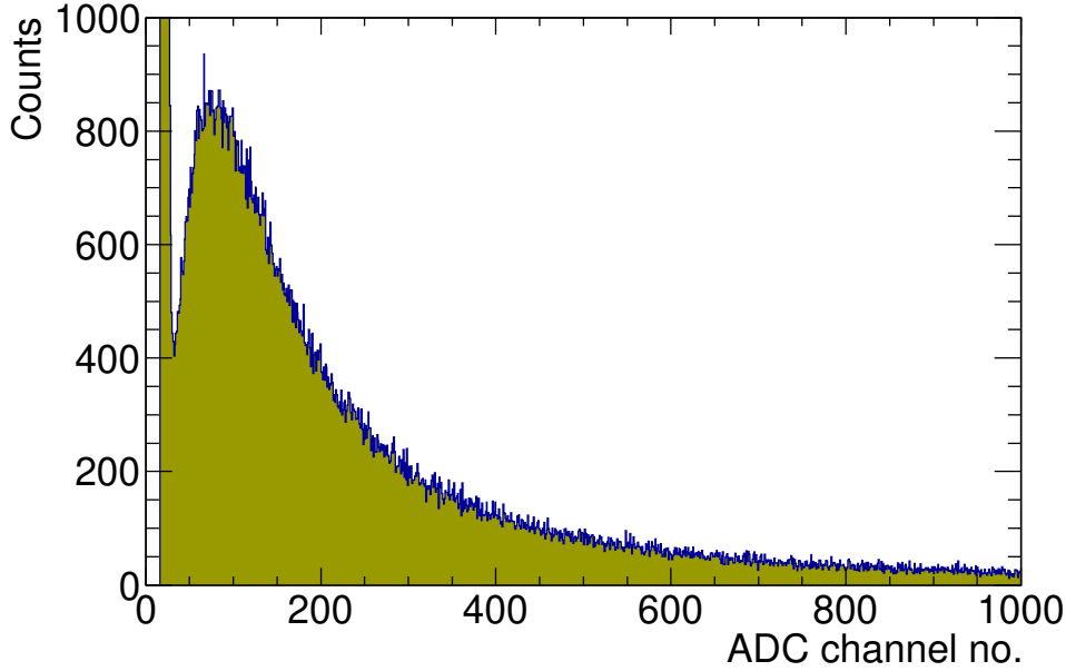
Figure 4.32: The energy spectrum of the quadruple GEM detector using ^{106}\text{Ru-Rh} \beta^- -source at \Delta V_{GEM-tot} = 1316 V with Ar/CO 2 70:30 gas.
