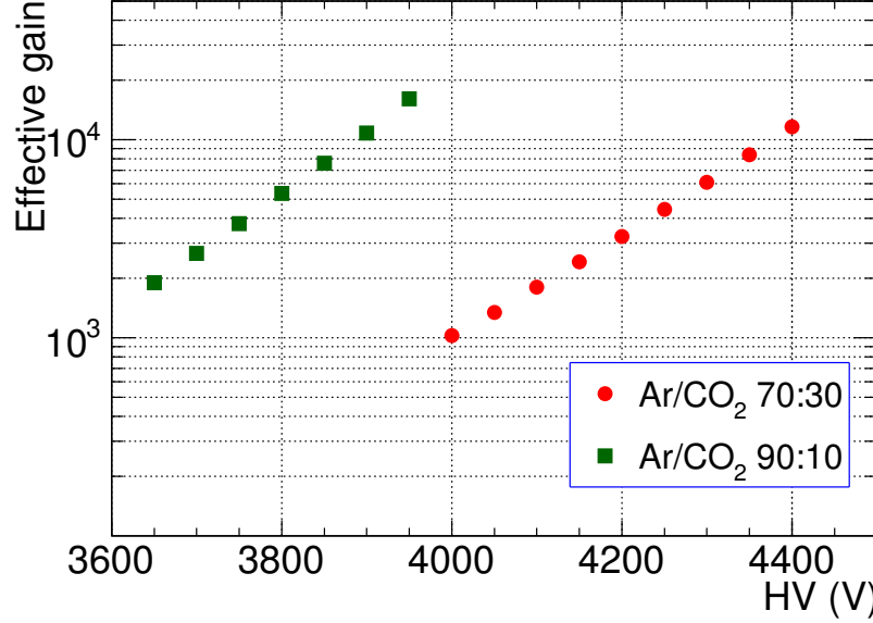
Figure 4.17: Effective gain of the triple GEM detector as a function of HV for both Ar/CO 2 90:10 and 70:30 gas mixtures. Statistical errors are small and within the symbol size.
