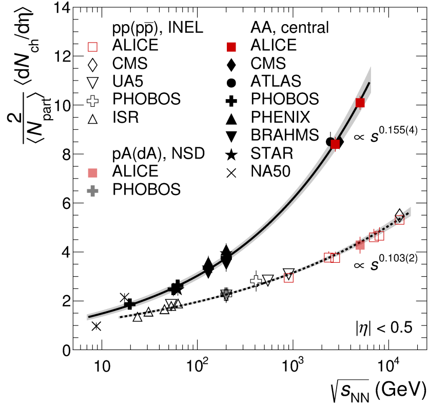
Figure 1.6: Charged particle pseudorapidity density variation with collision energy \sqrt{s_{NN}} for pp(pp), p-A(d-A) and A-A collision systems. Figure is adopted from [21].
