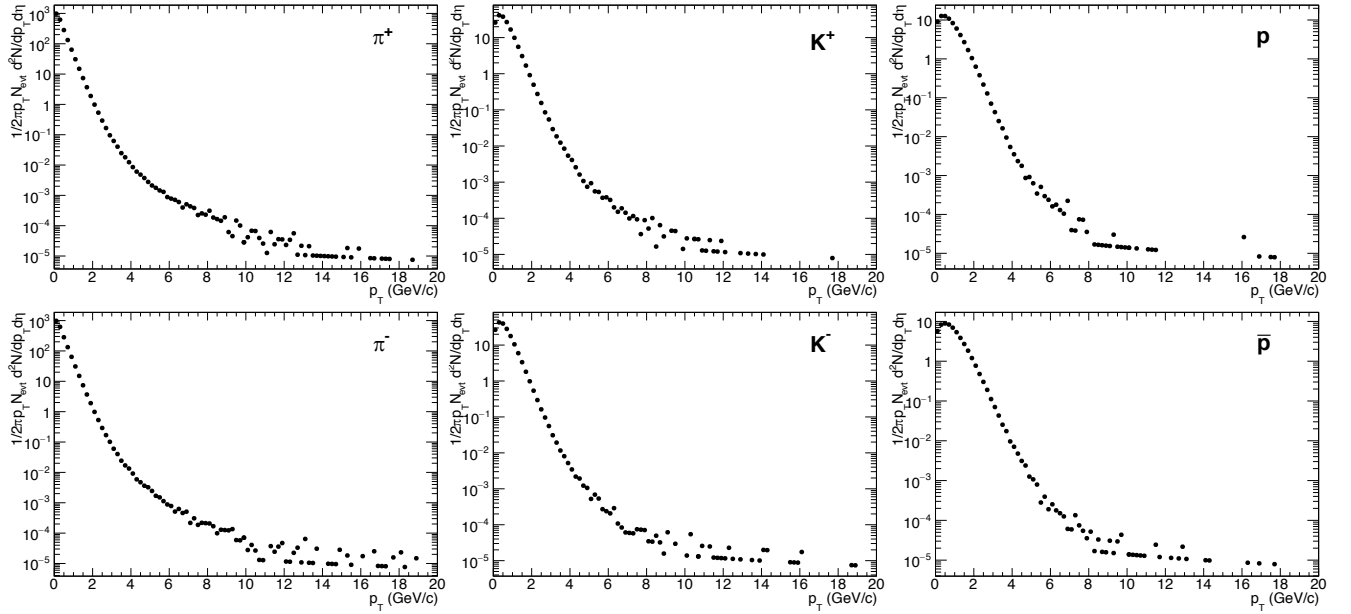
Figure 7.9: Transverse momentum spectrum of \pi^\pm , K^\pm , p , \bar{p} at mid-rapidity ( \langle\eta\rangle < 0.5 ) in most central (0 – 5%) Pb-Pb collision at \sqrt{s_{NN}} = 5.5 TeV using AMPT model.
