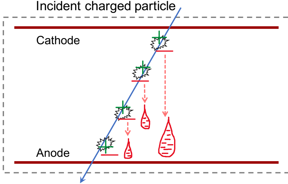
Figure 3.2: Working mechanism of a simple parallel plate gas detector.
