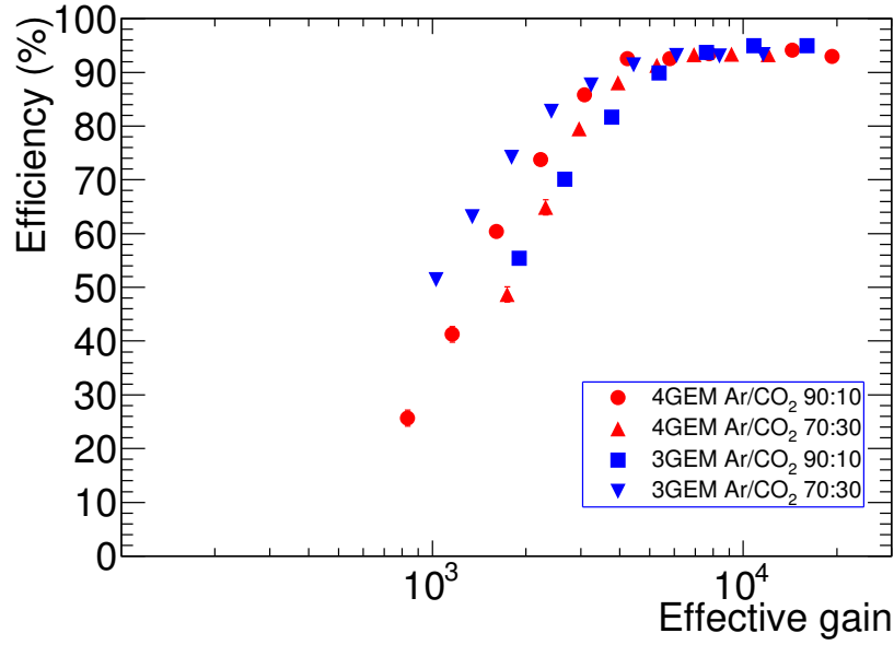
Figure 4.41: Variation of the efficiency as a function of effective gain with different Ar/CO 2 gas mixtures for both the triple GEM and the quadruple GEM detectors. Statistical errors are small and within the symbol size.
