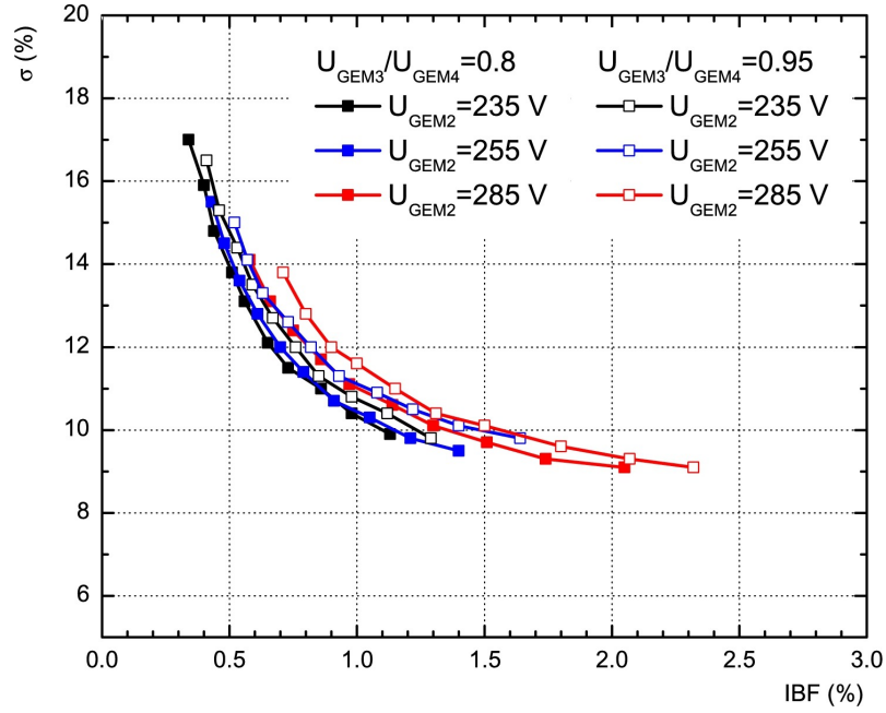
Figure 6.5: Correlation between ion backflow and energy resolution in a quadruple S-LP-LP-S GEM configuration in Ne/CO 2 /N 2 90:10:5 for various settings of \Delta U_{GEM2} . The voltage on GEM1 increases for a given setting between 225 and 315 V from left to right. The voltages on GEM3 and GEM4 are adjusted to maintain the gain of 2000 while keeping their ratio fixed. The transfer and induction fields are 4, 2, 0.1 and 4 kV/cm, respectively [30].
