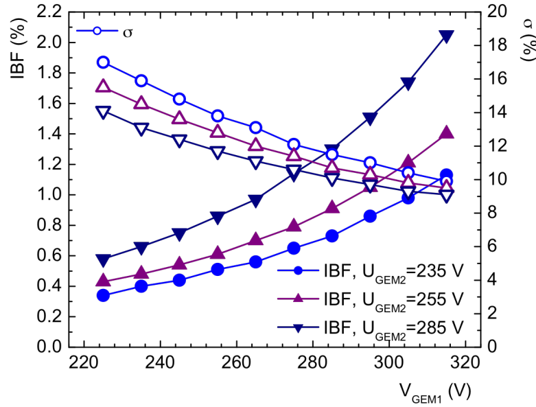
Figure 6.6: Ion backflow and energy resolution as a function of \Delta U_{GEM1} , for various settings of \Delta U_{GEM2} . The transfer and induction fields are 4, 2, 0.1 and 4 kV/cm, respectively, and the voltages on GEM3 and GEM4 are such that their ratio is 0.8 and the gain is 2000 [30].
