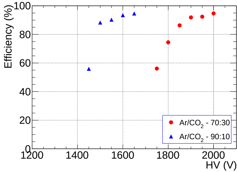
Figure 5.9: Efficiency as a function of HV of the MWPC-2 detector. The measurement performed using Ar/CO 2 70:30 and 90:10 gas mixtures.
