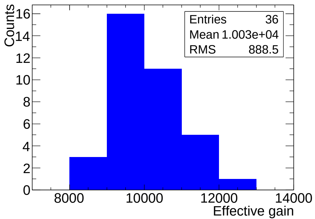
Figure 4.23: Distribution of the effective gain for 36 zones of the triple GEM detector at an applied voltage of 4400 V for 7 \times 7 matrices.
