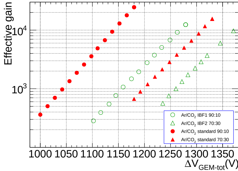
Figure 4.39: Effective gain as a function of total GEM voltage ( \Delta V_{GEM-tot} ) with different field settings of the quadruple GEM detector. Results with IBF field setting are in open bullets and standard setting are in solid bullets. Statistical errors are small and within the symbol size.
