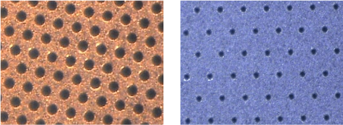
Figure 3.10: Photograph using optical microscope: standard pitch GEM foil in left panel and large pitch GEM foil in right panel with pitch 140\ \mu\text{m} and 280\ \mu\text{m} , respectively. Note the length scales are different.
