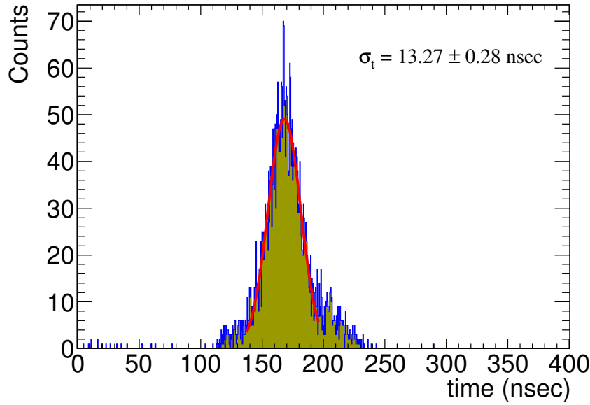
Figure 4.45: Time spectrum of the quadruple GEM detector with Ar/CO 2 70:30 gas mixture.
