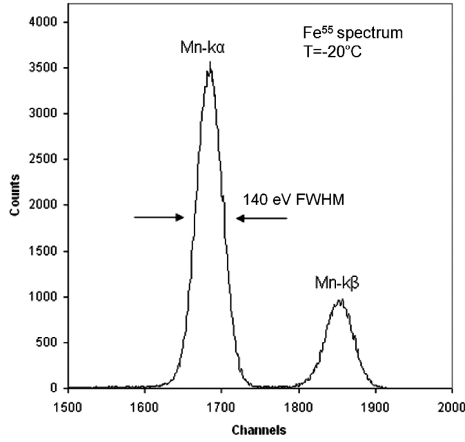
Figure 4.7: The energy spectrum of ^{55}\text{Fe} X-ray source of a Silicon detector. Both K_\alpha and K_\beta peaks are clearly separated [63].
