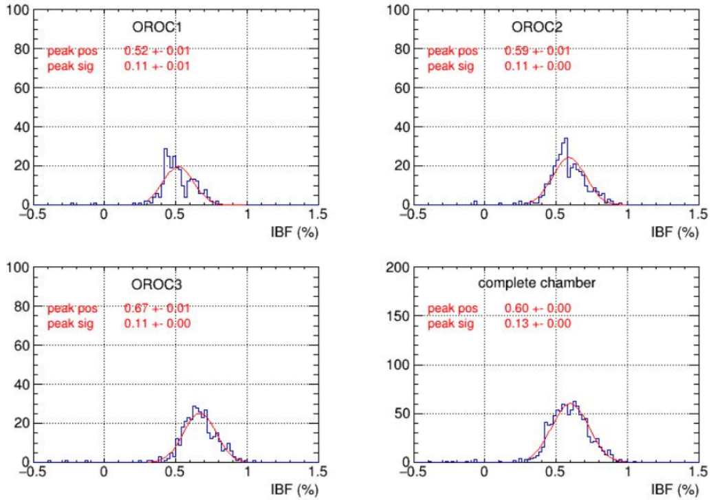
Figure 6.21: Ion backflow distribution of the OROC segments. The ion backflow is < 1\% .
