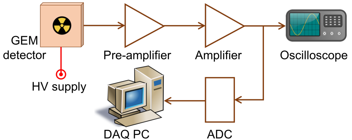
Figure 4.5: Electronics setup for the energy spectrum study of different radiations.
