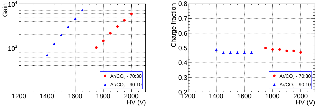
Figure 5.10: The gain as a function of HV for Ar/CO 2 90:10 and 70:30 gas mixtures in left panel and the fraction of the avalanche charge induced in the pad as a function of HV in right panel for the MWPC-2 detector.
