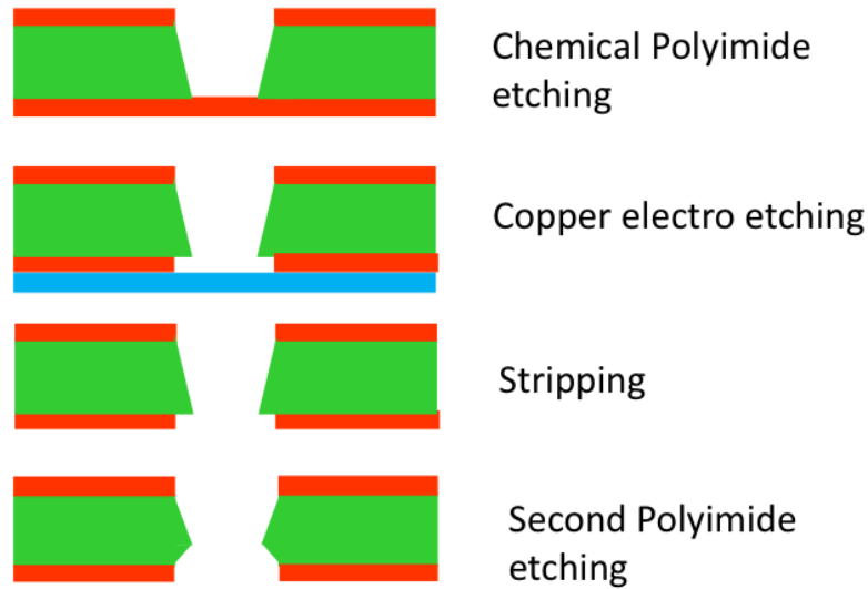
Figure 3.8: GEM foil fabrication steps using single-mask photolithographic technology.
