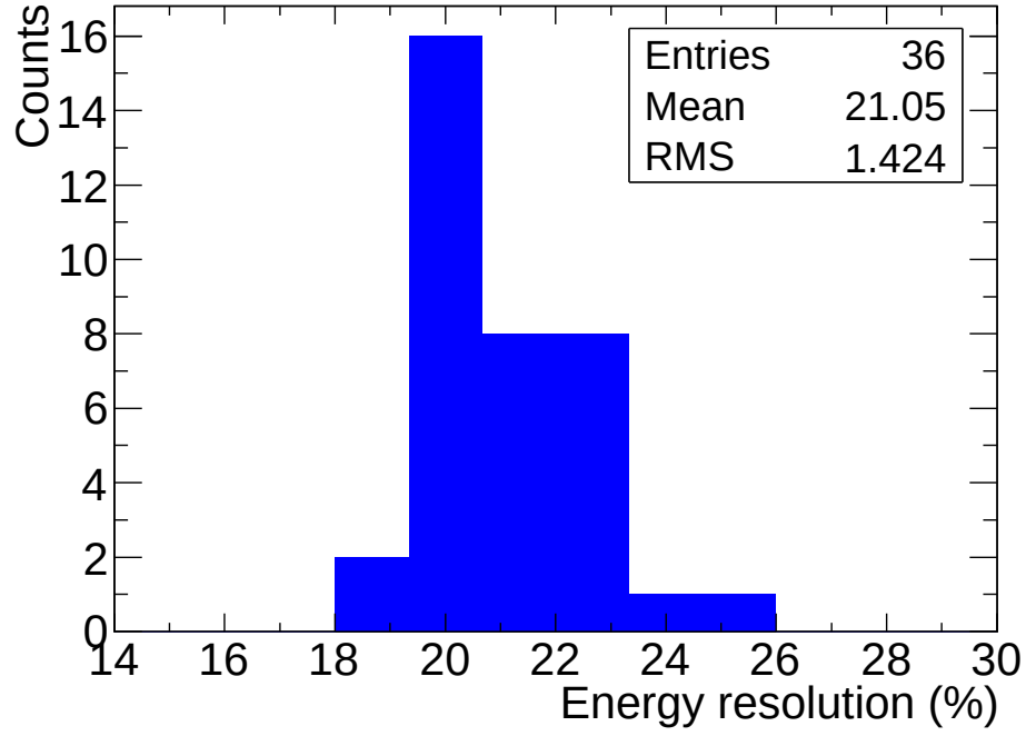
Figure 4.25: Distribution of energy resolution for the 36 zones of the GEM detector at an applied voltage of 4400 V for 7 \times 7 matrices.
