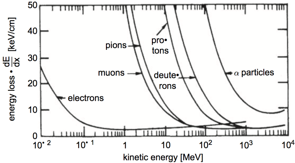
Figure 3.1: Specific energy loss of different charged particles in air [51].
