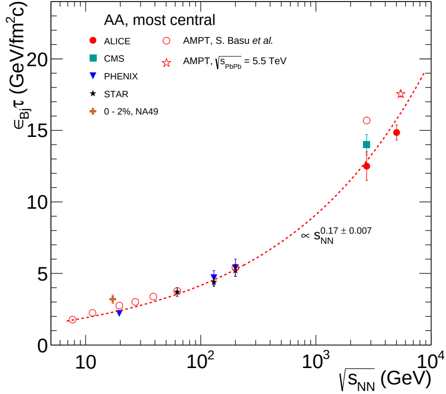
Figure 7.10: Variation of the Bjorken energy density \epsilon_{\text{Bj}}\tau for most central A-A collisions as a function of \sqrt{s_{\text{NN}}} . Experimental data for central Pb-Pb [23, 154, 159, 160] and Au-Au [146, 155–158]. AMPT calculation from [136].
