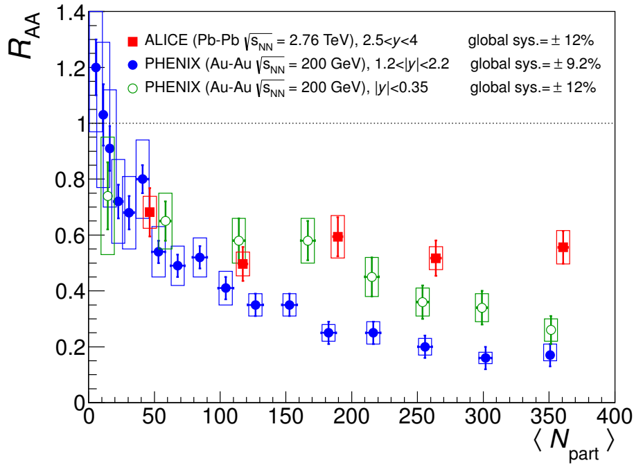
Figure 1.10: Nuclear modification factor R_{AA} of J/\Psi for Pb-Pb collisions measured in ALICE at \sqrt{s_{NN}} = 2.76 TeV [26]. The results of PHENIX experiment are taken for comparison [27].
