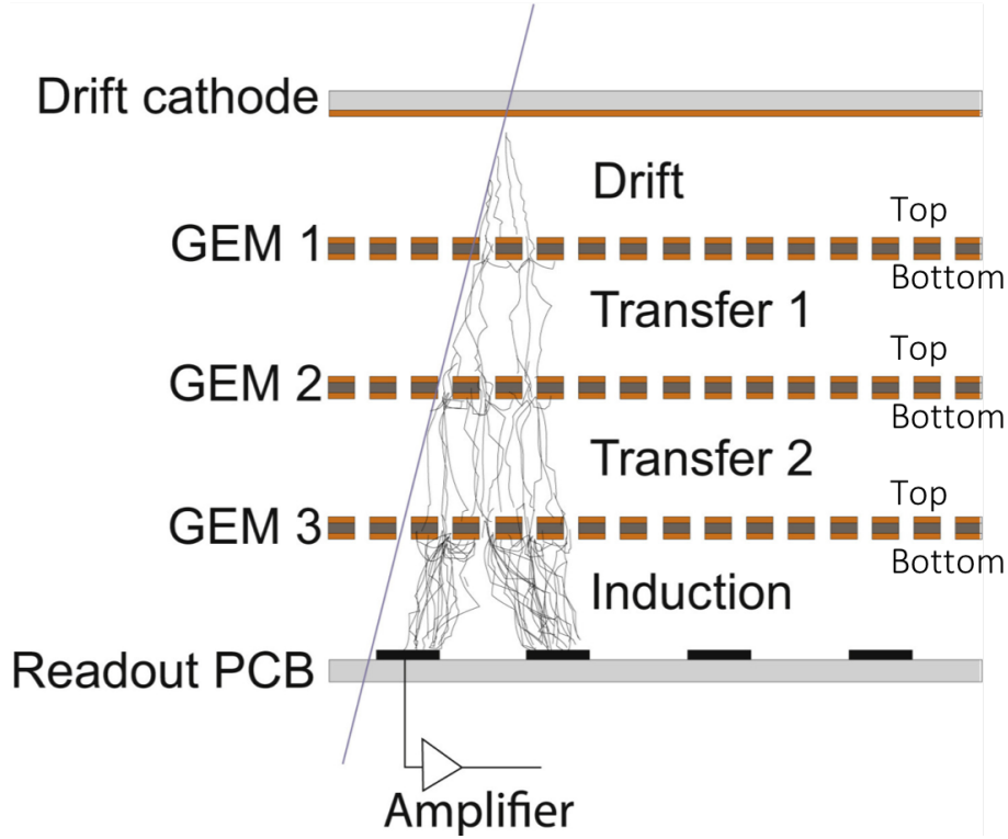
Figure 3.13: Multi-stage avalanche formations and charge collection in a triple GEM detector.
