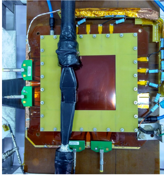
Figure 4.13: Photograph of the efficiency measurement setup of the triple GEM detector.
