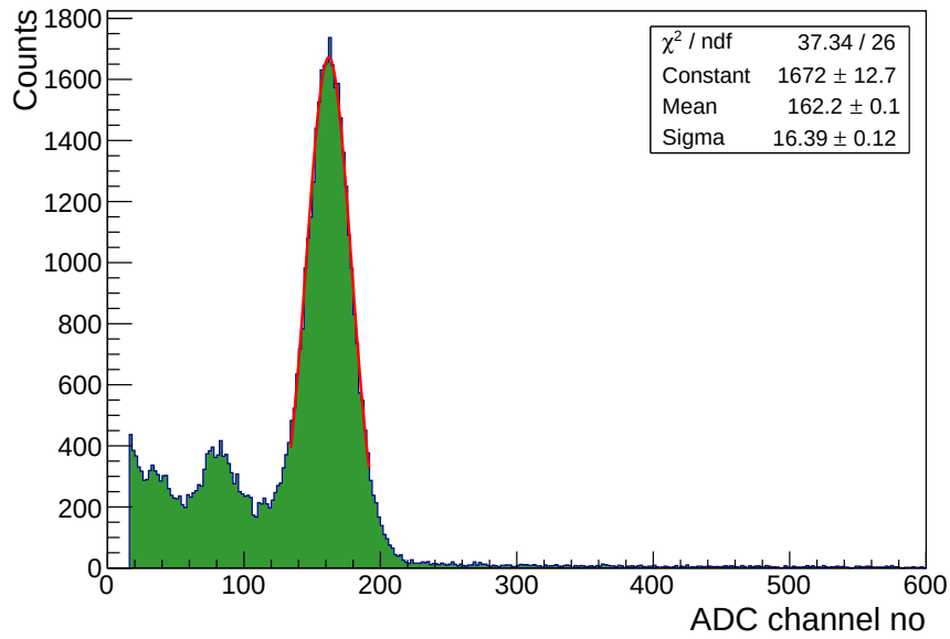
Figure 5.5: Energy spectrum of 55 Fe X-ray source of the MWPC-1 detector operated at 1800 V. The spectrum from anode signals using NIM electronics.
