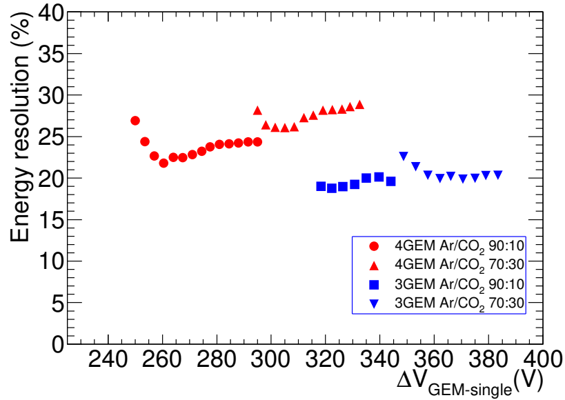
Figure 4.37: Energy resolution as a function of \Delta V_{\text{GEM-single}} with different Ar/CO 2 gas mixtures. Statistical errors are small and within the symbol size.
