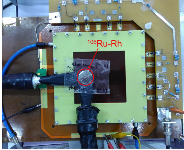
Figure 4.33: Photograph of the efficiency measurement setup of the quadruple GEM detector.
