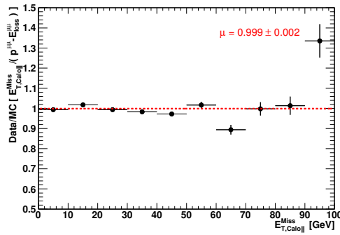
Figure 4.22: The Data/MC ratio of parallel component of E_{T,\text{Calo}}^{\text{Miss}} to the direction of Z to the transverse momentum of the di-muon system corrected for the muon energy deposition in the calorimeter.
