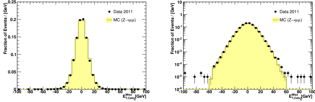
Figure 4.21: Perpendicular component of E_{T,\text{Calo}}^{\text{Miss}} to the direction of Z . The filled histogram is the reweighted Z \rightarrow \mu\mu MC and the circles represent data for the full luminosity. Linear scale is given on left, and log scale on right.
