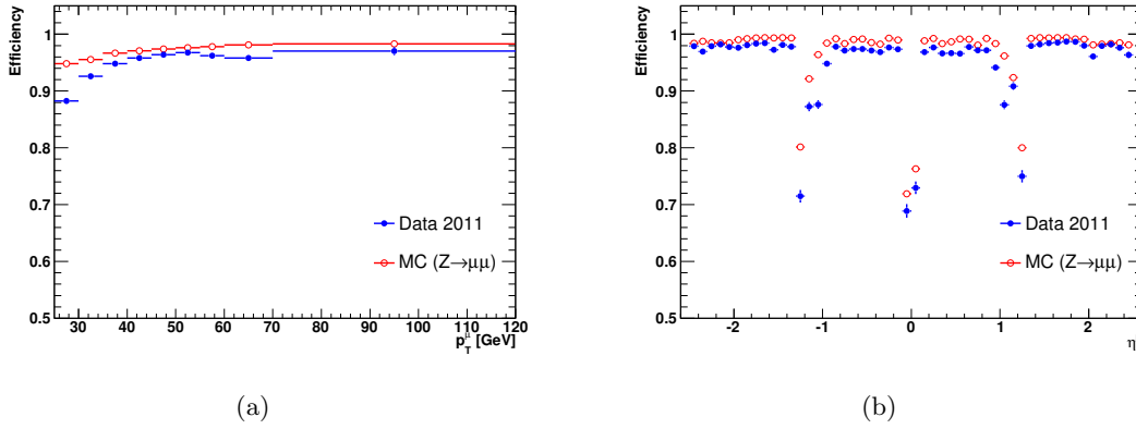
Figure 4.10: Combined muon reconstruction efficiency as a function of muon p_T and \eta .
