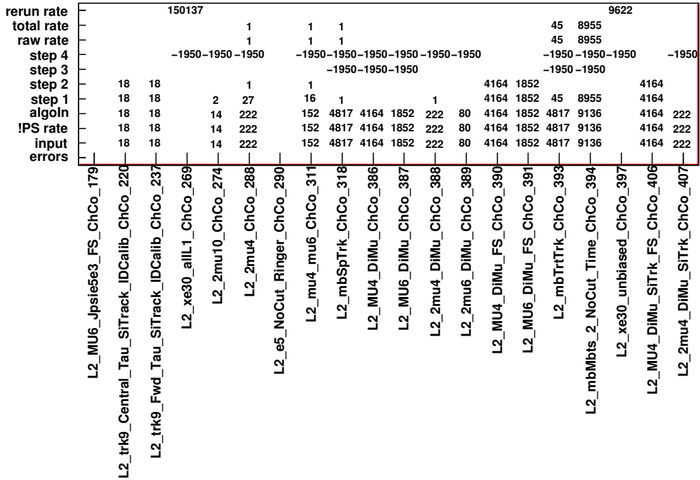
Figure 3.1: An example Signature Acceptance histogram. The x -axis holds a subset of L2 trigger chains and the y -axis holds the different counts.
