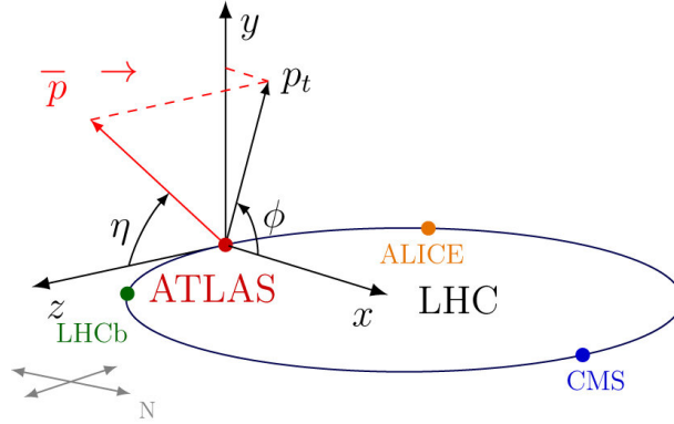
Figure 3.5: The ATLAS coordinate system [77].
