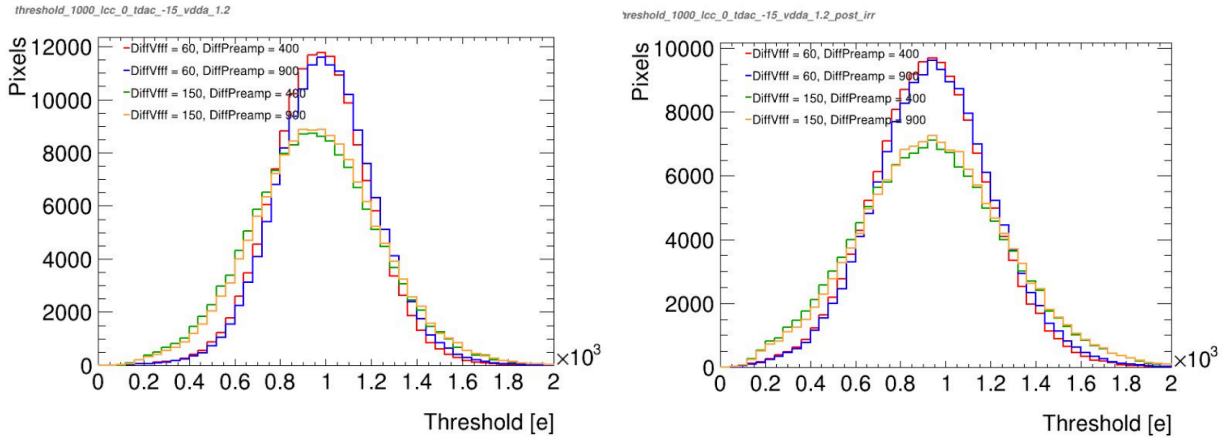
Figure 5.25: The threshold distribution before (left) and after (right) irradiation. The chip threshold was tuned to 1000 e before irradiation with DiffVtff, DiffPreamp, LCC, TDAC, and VDDA fixed at specific settings.
