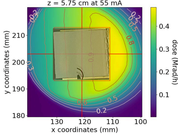
Figure 5.20: The X-ray beam spot for irradiating the ITkPixV1 chip. A 2 \times 2 cm square is drawn around the beam center with the ITkPixV1 chip overlaid. The chip bottom with the wire bonds connected to the single chip card is placed at the maximum dose rate regions.
