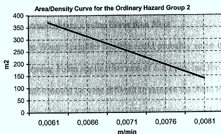
Figure 43. Area/density curve for the ordinary hazard group 2.
