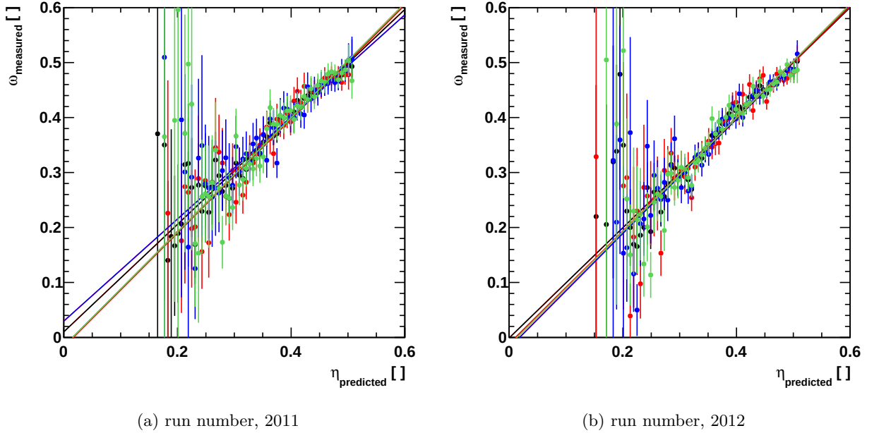
Figure 3.41.: Calibration systematics for (left 2011 data, right 2012 data) splitting the sample according to the run number, representing the time the data was taken (red: \text{run\#} < 9.5 \times 10^4 , blue: \text{run\#} \in [9.5 \times 10^4, 1.01 \times 10^5] , green: \text{run\#} > 1.01 \times 10^5 ), red: \text{run\#} < 1.19 \times 10^5 , blue: \text{run\#} \in [1.19 \times 10^5, 1.29 \times 10^5] , green: \text{run\#} > 1.29 \times 10^5 , respectively for 2012 data. The calibration of the whole sample is shown in black.
