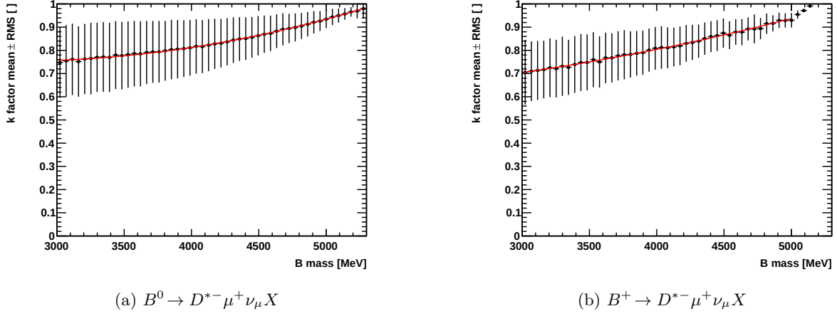
Figure 4.19.: Mean k factor in bins of the visible B mass for tagged events in B^0 \rightarrow D^{*-} \mu^+ \nu_\mu X mode 2012 MC. Left: signal component, right: B^+ \rightarrow D^{*-} \mu^+ \nu_\mu X background component. The plotted k factor mean error is given as RMS of each k factor histogram per bin.
