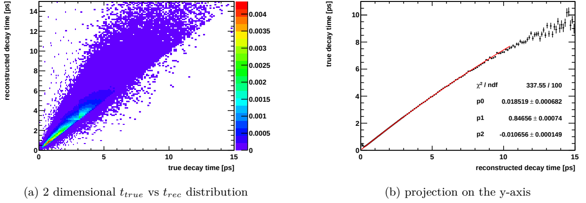
Figure 4.26.: MC true versus reconstructed decay time of tagged events in B^0 \rightarrow D^{*-} \mu^+ \nu_\mu X mode 2012 MC. Left: the 2 dimensional distribution, right: projected on the y-axis. The dependence of the reconstructed decay time on the true decay time is fitted by a second order polynomial.
