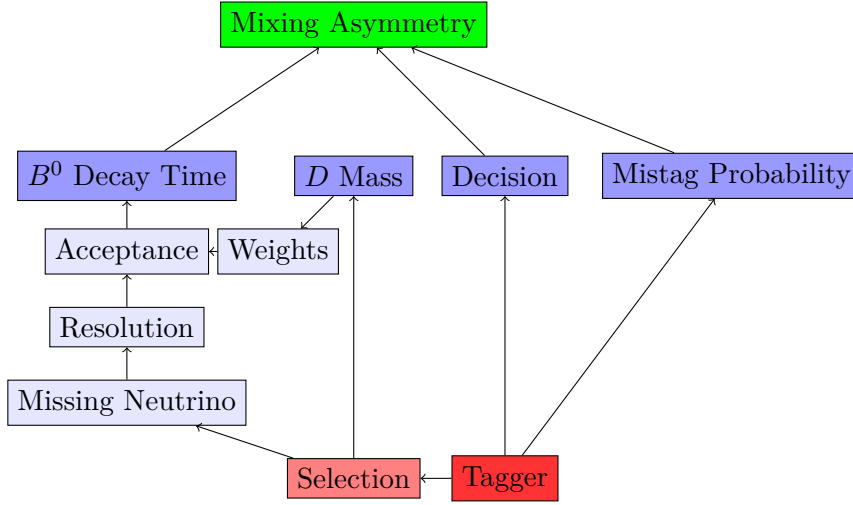
Figure 4.5.: Flow chart to illustrate the measurement of the oscillation frequency \Delta m_d extracted from the mixing asymmetry (from bottom to top). The tagging efficiency and selection requirements define the data set. The missing momentum of the neutrino and the decay time resolution and acceptance shape the B^0 decay time distribution. The D mass resonance is used to statistically remove hadronic background via weights. The tagging decision and mistag probability construct the mixing asymmetry out of the decay time distribution.
