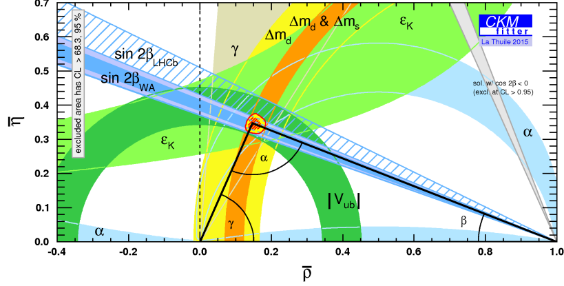
Figure 1.2.: Unitarity triangle, see equation 1.6, in the \bar{\rho}-\bar{\eta} plane. Including the new LHCb \sin 2\beta measurement (blue dashed band), presented at the La Thuile 2015 conference [19], into the World Average of \sin 2\beta (blue band) leaves not much space for NP to break the triangle condition. Taken from [20]
