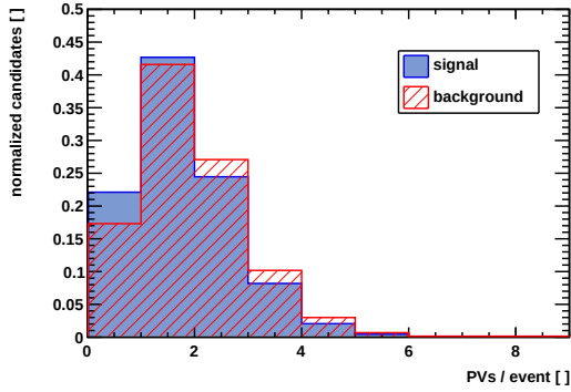
(e) \#PVs/event
