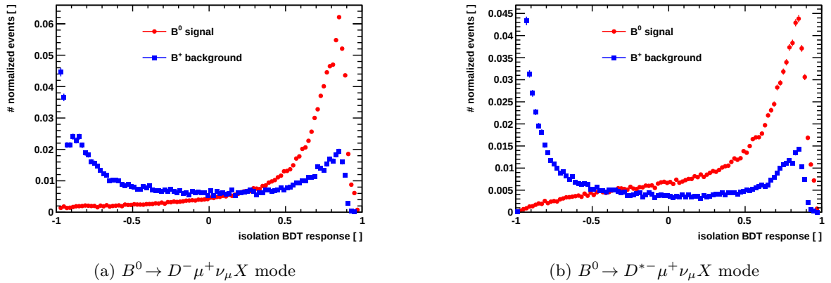
Figure 4.11.: Isolation BDT response in B^0 signal MC and B^+ background MC in the B^0 \rightarrow D^-\mu^+\nu_\mu X mode (left) and B^0 \rightarrow D^{*-}\mu^+\nu_\mu X mode (right).
