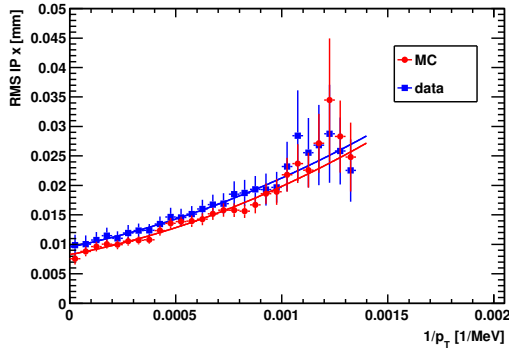
(c) 3 PVs
