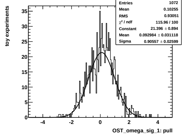
(b) Category 1
