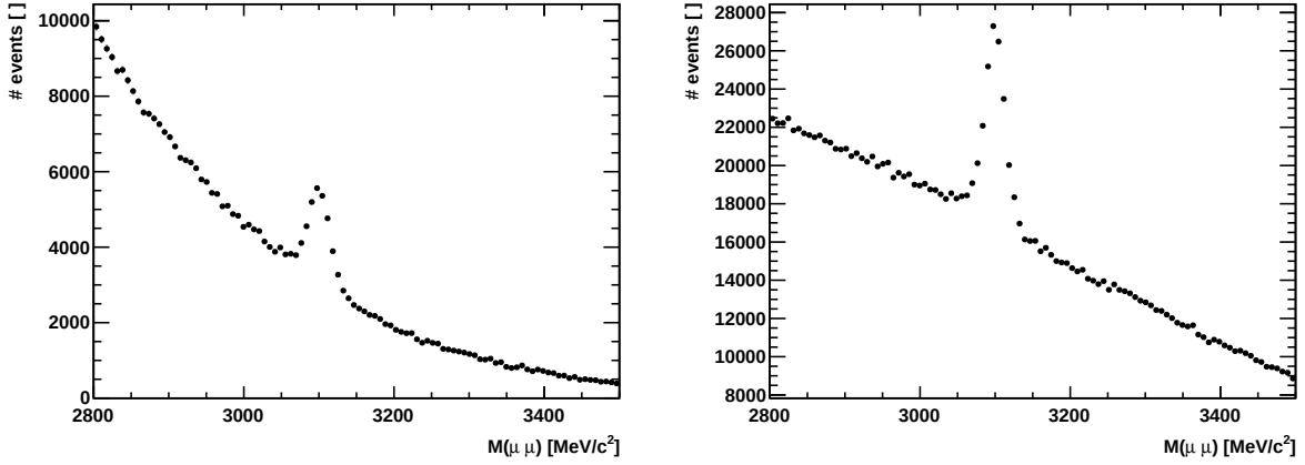
Figure 4.10.: \mu\mu invariant mass distributions in the B^0 \rightarrow D^- \mu^+ \nu_\mu X (left) and the B^0 \rightarrow D^{*-} \mu^+ \nu_\mu X mode (right) on 2012 data, computed under the muon mass hypothesis for the highest momentum pion. In both distributions a clear peak at the J/\psi mass, m_{J/\psi} = 3096.916 \pm 0.011 \text{ MeV} [18], is visible.
