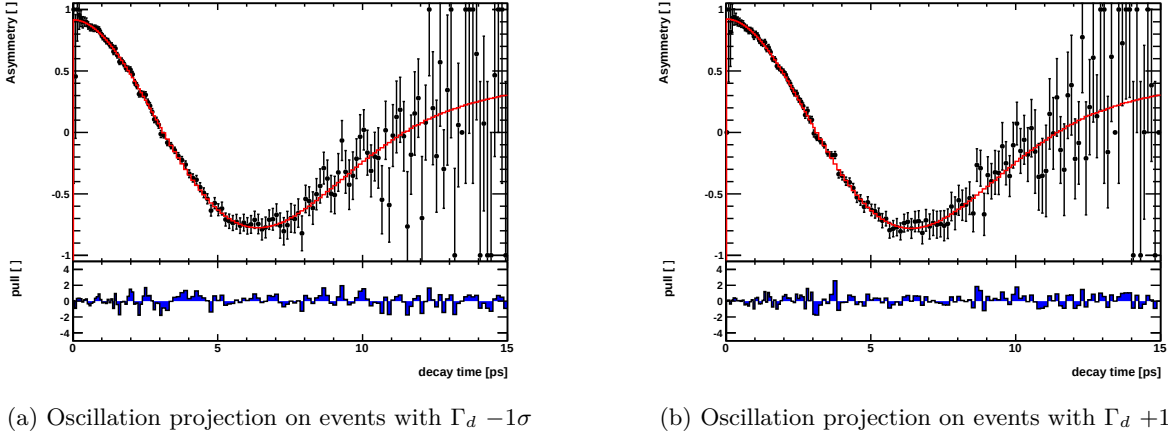
Figure 4.35.: Mixing asymmetry fit projections of the \Delta m_d fit to 2012 MC events in the B^0 \rightarrow D^{*-} \mu^+ \nu_\mu X mode using cheated tagging. Left: \Gamma_d is lowered by 1\sigma , right: \Gamma_d is increased by 1\sigma by changing the sample composition.
