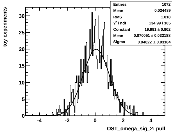
(c) Category 2
