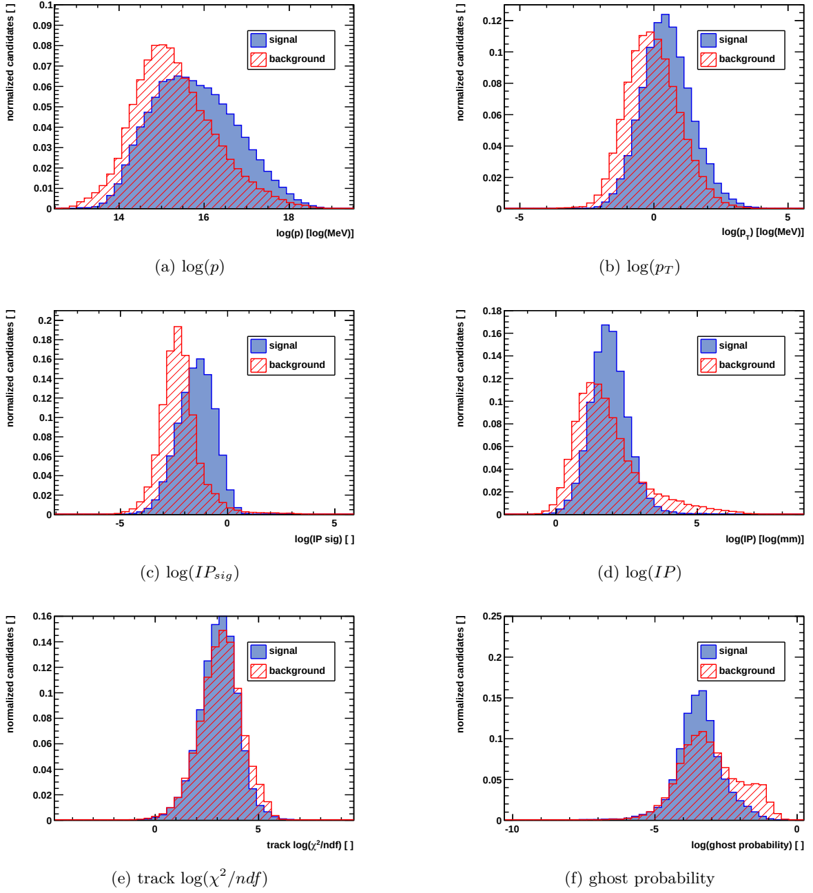
Figure 3.17.: ANN1 input variables separately drawn for signal, which are OS kaons (blue) and background particles, which are all other particles in the event (red): \log(p) , \log(p_T) , \log(IP_{sig}) , \log(IP) , \text{track } \log(\chi^2/ndf) , \log(\text{ghost probability}) . The linear decorrelation transformation is applied.
