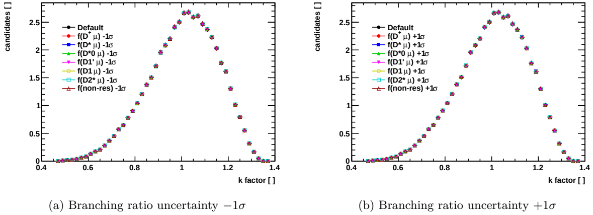
Figure 4.43.: Comparison of k factor distributions in the B^0 \rightarrow D^- \mu^+ \nu_\mu X mode after applying weights corresponding to a variation of (a) -1\sigma and (b) +1\sigma of the semileptonic branching ratio uncertainties.
