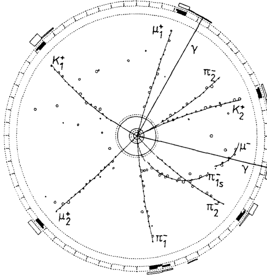
Figure 4.1.: Fully reconstructed \Upsilon(4S) \rightarrow B^0B^0 event in the ARGUS detector, part of the discovery of B^0-\bar{B}^0 mixing. One B^0 decays into B_1^0 \rightarrow D_1^{*-} \mu_1^+ \nu_1 , with D_1^{*-} \rightarrow \pi_{1s}^- \bar{D}^0 and \bar{D}^0 \rightarrow K_1^+ \pi_1^- . The other B^0 decays into B_2^0 \rightarrow D_2^{*-} \mu_2^+ \nu_2 , with D_2^{*-} \rightarrow \pi^0 D^- , where \pi^0 \rightarrow \gamma\gamma and D^- \rightarrow K_2^+ \pi_2^- \pi_2^- . Taken from [23]
