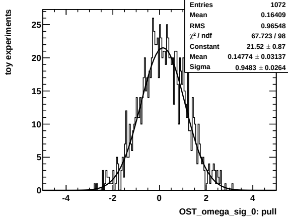
(a) Category 0
