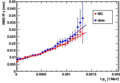
(a) 1 PV
