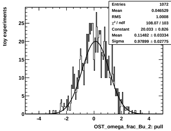
(c) Category 2
