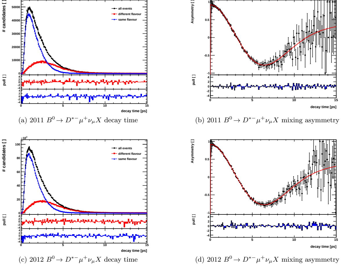
Figure 4.31.: Fit projections of the \Delta m_d fit to 2011 (upper row) and 2012 (lower row) B^0 \rightarrow D^{*-} \mu^+ \nu_\mu X signal MC with cheated tagging.
