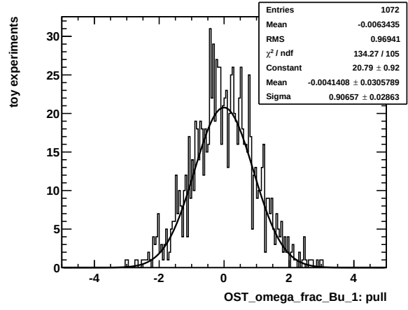
(b) Category 1
