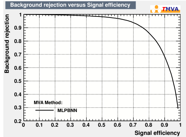
Figure 3.21.: Background rejection against signal efficiency of ANN1.
