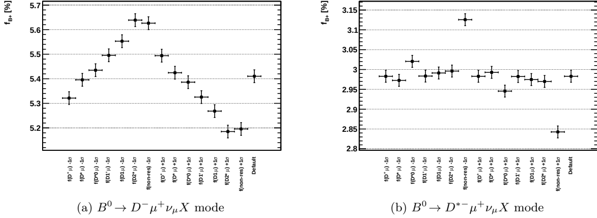
Figure 4.38.: Fitted B^+ fractions ( f_{B^+} ) in B^0 \rightarrow D^- \mu^+ \nu_\mu X mode (a) and B^0 \rightarrow D^{*-} \mu^+ \nu_\mu X mode (b), where the signal B^0 MC isolation BDT distribution template is weighted according to the semileptonic branching ratio uncertainties.
