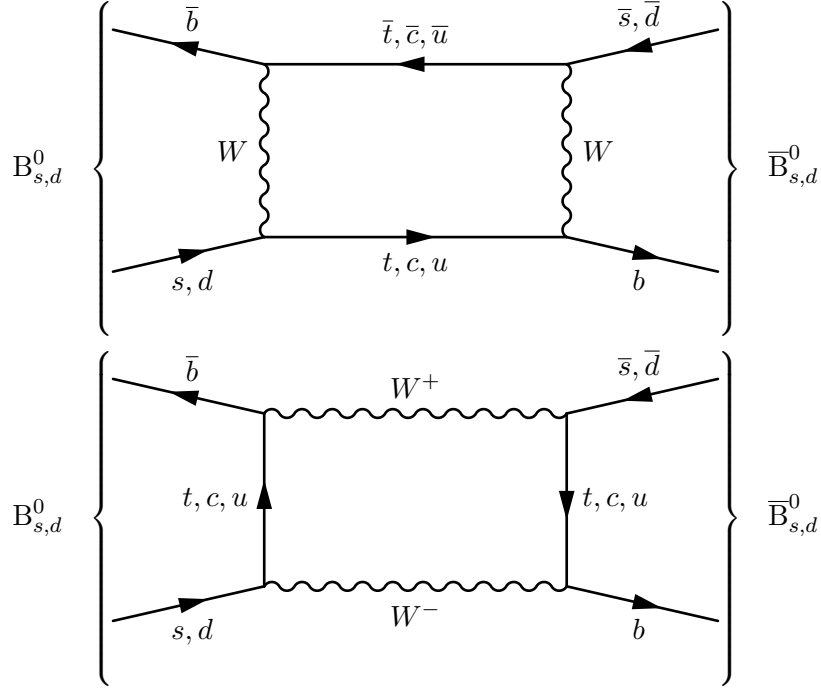
Figure 1.3.: Feynman diagrams of the leading order contributions to B^0-\bar{B}^0 mixing. B_q^0 oscillate into \bar{B}_q^0 mesons via an internal loop of up-type quarks and W^\pm bosons.
