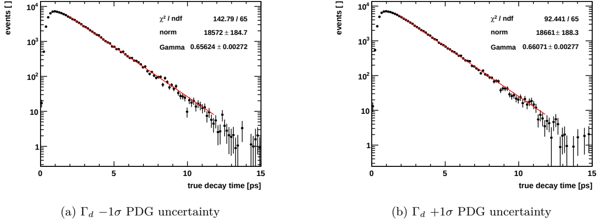
Figure 4.34.: True decay time distribution of 2012 MC events in the B^0 \rightarrow D^{*-}\mu^+\nu_\mu X mode. Left: the sample is enriched with long-lived events by randomly rejecting short-lived events, the mean B^0 decay width is 1\sigma of the PDG uncertainty smaller, right: the other way around.
