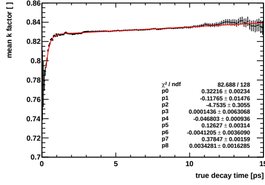
Figure 4.24.: Fitted mean k factor distribution in MC true decay time bins of tagged events in B^0 \rightarrow D^{*-}\mu^+\nu_\mu X 2012 MC. The distribution is fitted by an empirical function given in equation 4.40. The uncertainty per bin in y direction is given by the uncertainty on the mean value of the k factor histogram.
