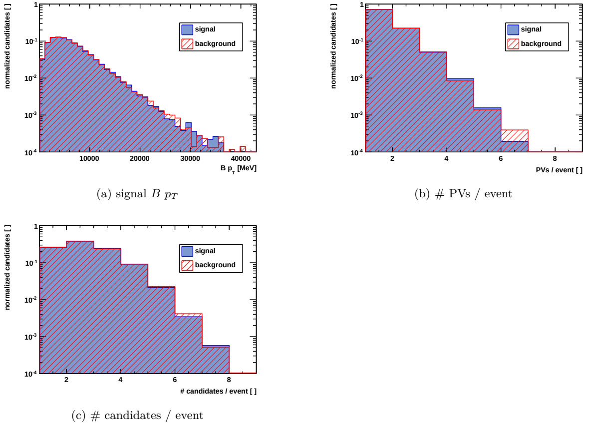
Figure 3.25.: ANN2 input variables separately drawn for signal (blue), which are arbitrarily chosen to be B^+ decays, and background (red), which are B^- decays: p_T of the signal B , # of PVs per event and # tagging candidates per event. The latter is evaluated after the cut on the ANN1 response is applied.
