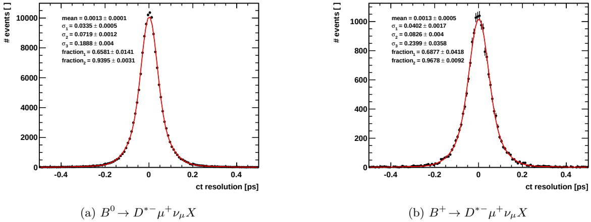
Figure 4.28.: Decay time resolution for tagged events in B^0 \rightarrow D^{*-}\mu^+\nu_\mu X mode 2012 MC (left) and for B^+ \rightarrow D^{*-}\mu^+\nu_\mu X 2012 MC (right). The effect of the reconstructed flight distance on the decay time resolution is evaluated. It is fitted by a triple Gaussian.
