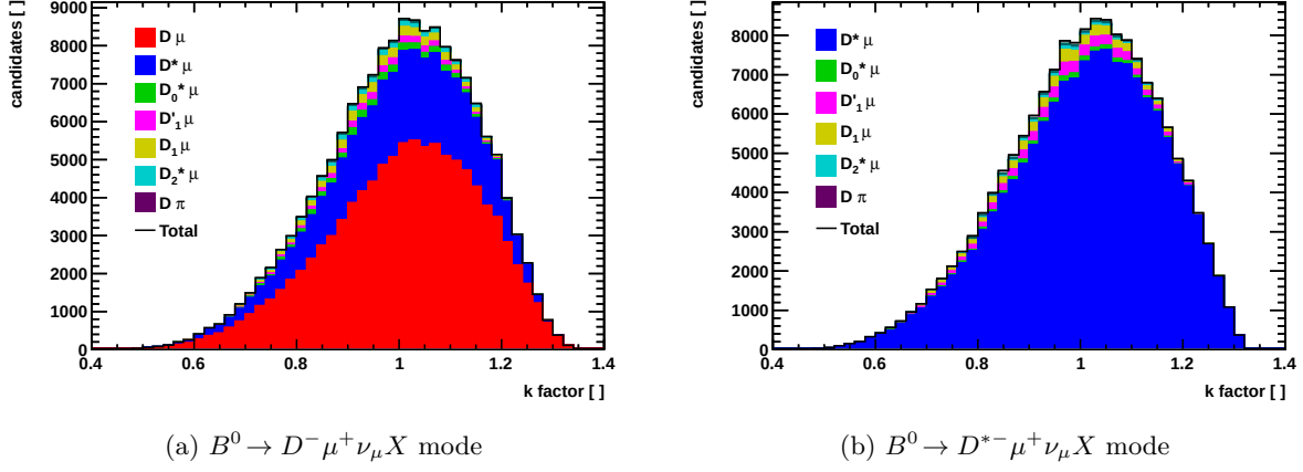
Figure 4.42.: Sample composition of B^0 \rightarrow D^- \mu^+ \nu_\mu X (a) and B^0 \rightarrow D^{*-} \mu^+ \nu_\mu X (b) displayed in stacked k factor histograms. The corresponding fraction numbers are given in table 4.21 and table 4.22.
