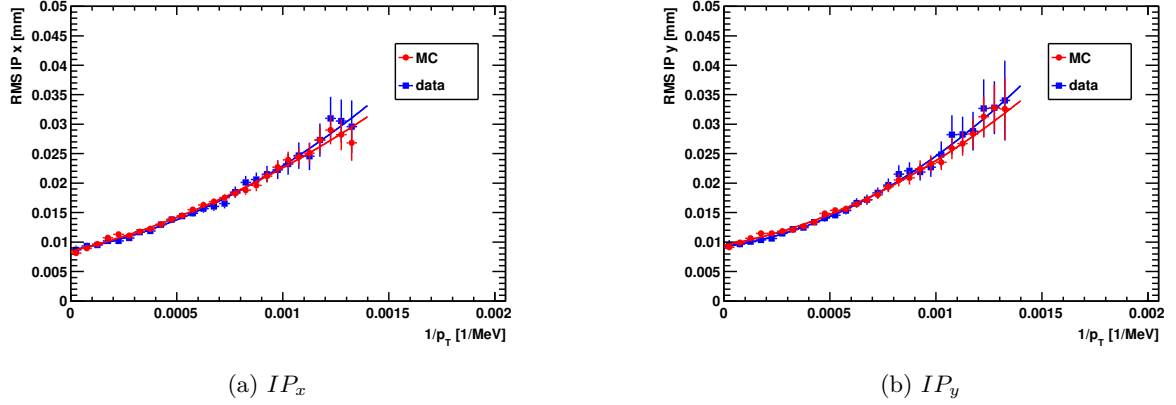
Figure 3.11.: Smeared impact parameter resolution distributions (a) in x direction and (b) in y direction.
