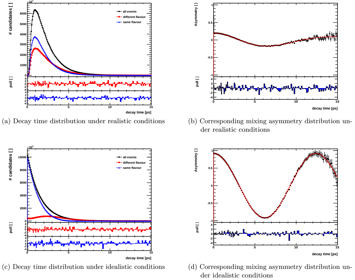
Figure 4.6.: Illustration of the damping factors on the mixing asymmetry using 1.6 \times 10^7 simulated B^0 decays, generated under realistic conditions (upper plots) and under idealistic conditions (lower plots). Left: the B^0 decay time distributions for all events (black) and split up according to mixed (red, different production and decay flavour) and unmixed (blue, same production and decay flavour) events. The corresponding mixing asymmetry distributions are shown (right). Idealistic conditions contain 4% mistag probability, therefore, \mathcal{A}|_{t=0} = 0.92 .
