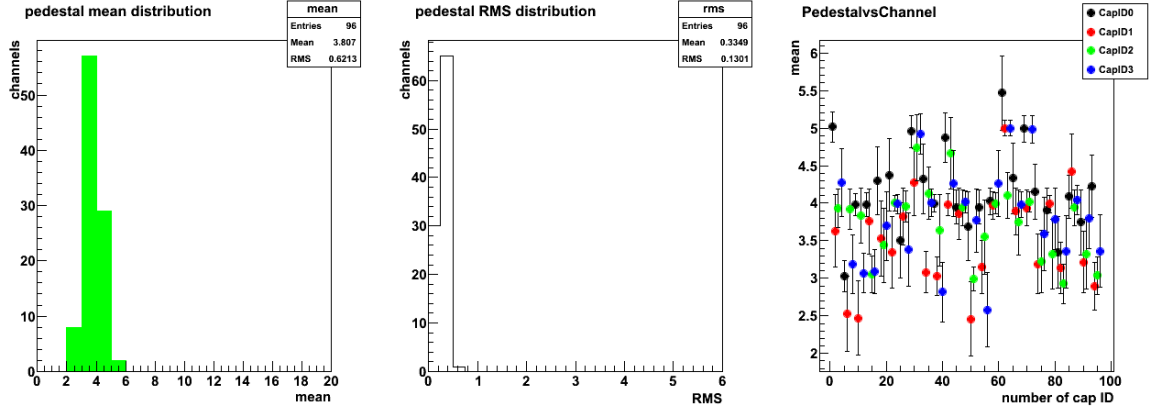
Figure 7.5. Result of a successful pedestal test. Histogram to the left shows the pedestal ADC value distribution of all QIE10 chips over all Cap IDs on a QIE card. This value should be between 2 and 6. Histogram to the right shows the raw data of this distribution.
