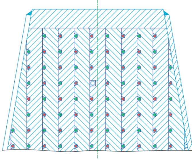
Figure 5.4. Fiber configuration of a tower (#13). (Red: Short fibers, Green: Long fibers, White: Radioactive source wire) [8]
