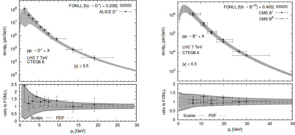
Figure 2.7 – FONLL predictions for the p_T -differential production cross section of D^+ (left) and B^+ (right) mesons, evaluated in the central rapidity interval |y| < 0.5 . Gray shaded bands represents the overall theoretical uncertainties due to the choice of the factorization and renormalization scales, the PDFs and the quark masses. Predictions are compared to LHC data from ALICE [82] and CMS [83], [84]. Figures are taken from [80].
