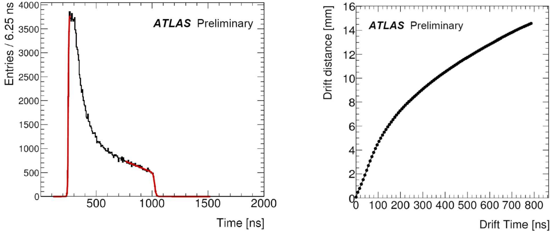
Figure 2.11. A typical MDT drift time spectrum (left) and space-time (r-t) relationship for MDT chambers (right).
