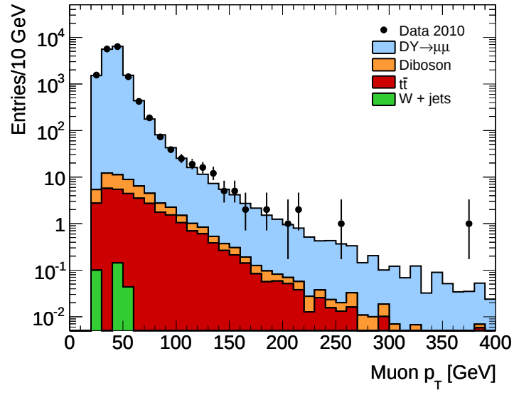
Figure 6.11. Muon momentum of both muons per event after all selection. Here, DY includes both Z \rightarrow \mu\mu and Z \rightarrow \tau\tau processes.
