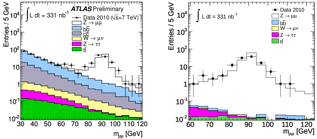
Figure 4.2. Dimuon invariant mass distribution after preselection (left) and after all selection (right).
