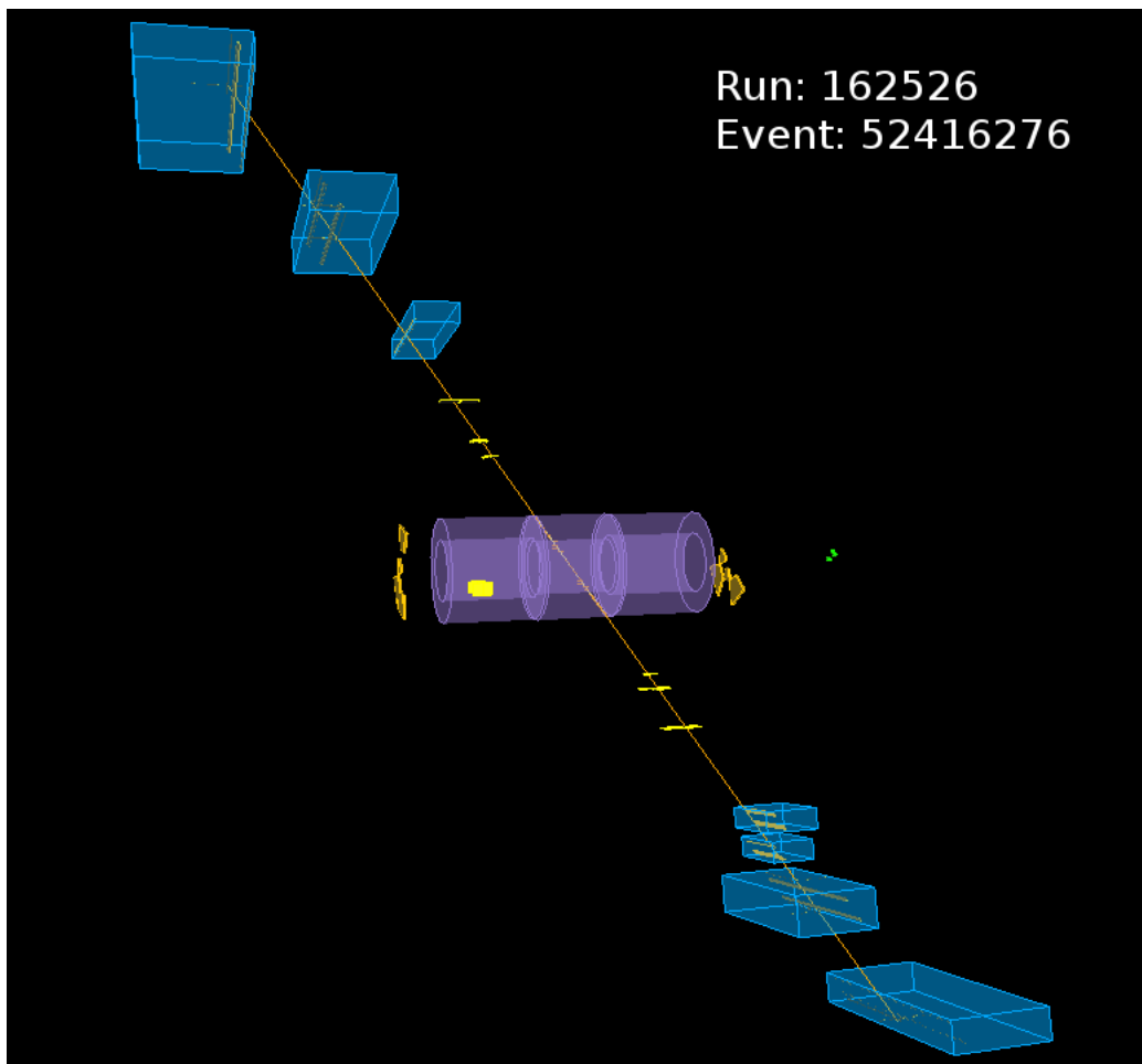
Figure 3.9. Cosmic muon event triggered in ATLAS, passing close to the interaction point in a non-collision event. The first muon in the upper hemisphere has \eta = -0.63 , p_T = 177.9 GeV, and the second muon in the lower hemisphere has \eta = 0.63 , p_T = 176.1 GeV. The combined invariant mass of the two muons is 425.7 GeV.
