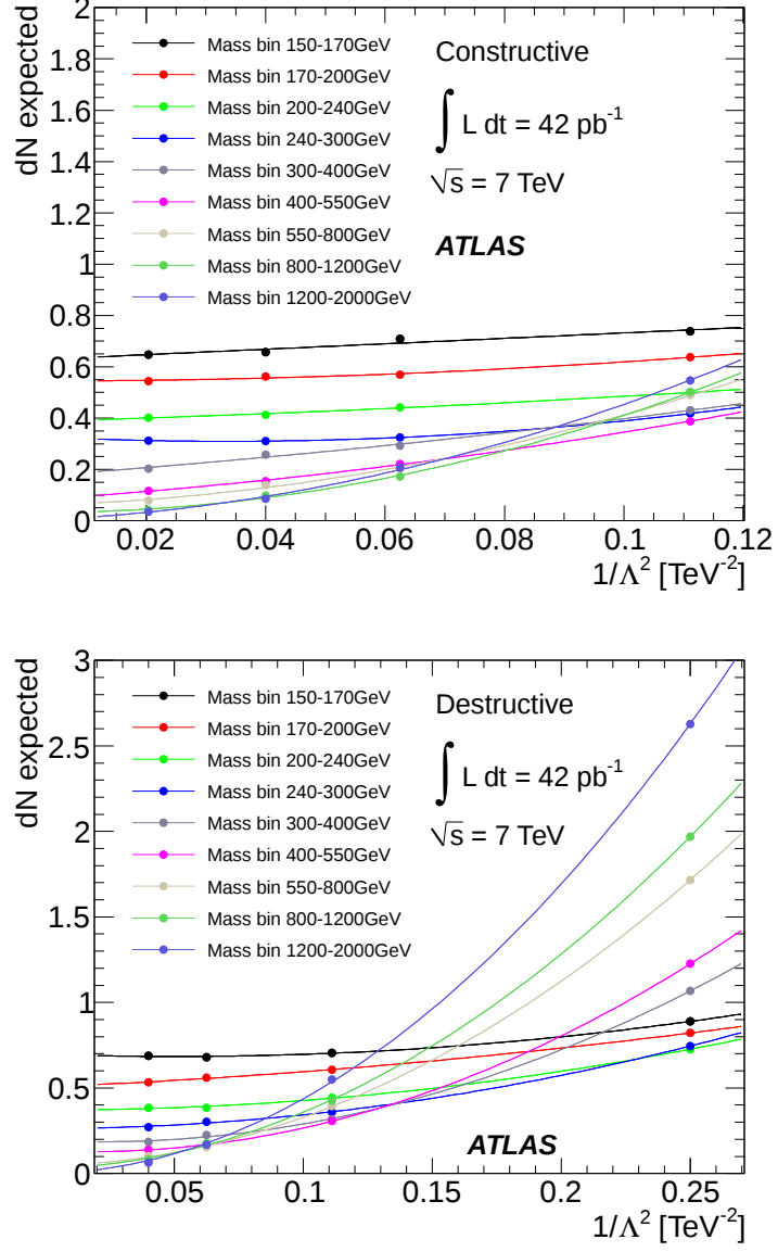
Figure 8.2. Values of dN_{\Lambda}^k in each mass bin for the constructive (top) and destructive (bottom) interference models shown as points corresponding to the benchmark signal samples. The second-order polynomial fits to dN_{\Lambda}^k as a function of 1/\Lambda^2 in each mass bin are also shown.
