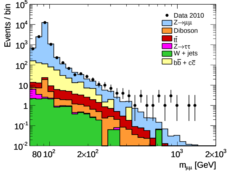
Figure 6.2. Invariant mass of two combined muons after event preselection.
