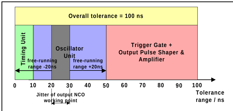
Figure 21: Time tolerance distribution
