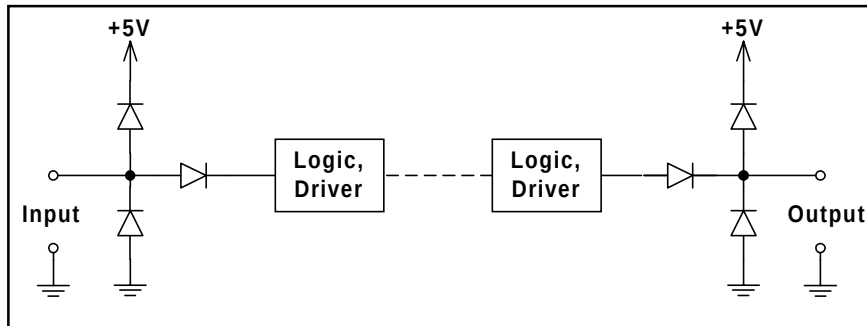
Figure 31: Input/Output-Protection circuits
