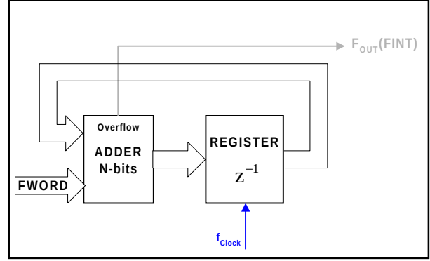
Figure 11: Phase Accumulator
