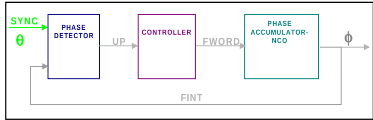
Figure 9: RFM-Phase-Locked-Loop
