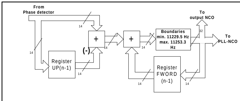
Figure 10: Controller realisation
