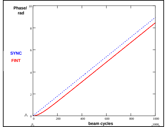
Figure 15: PLL frequency offset response
