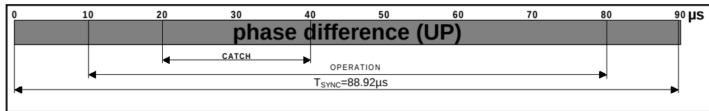
Figure 17: RFM operating ranges
