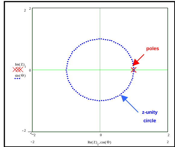
Figure 18: poles in the z-plane
