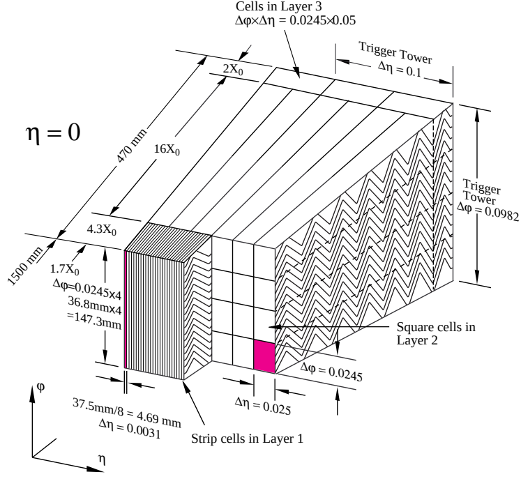
Figure 4.5: A sketch of the accordion and cell struction of the EM calorimeter [8].
