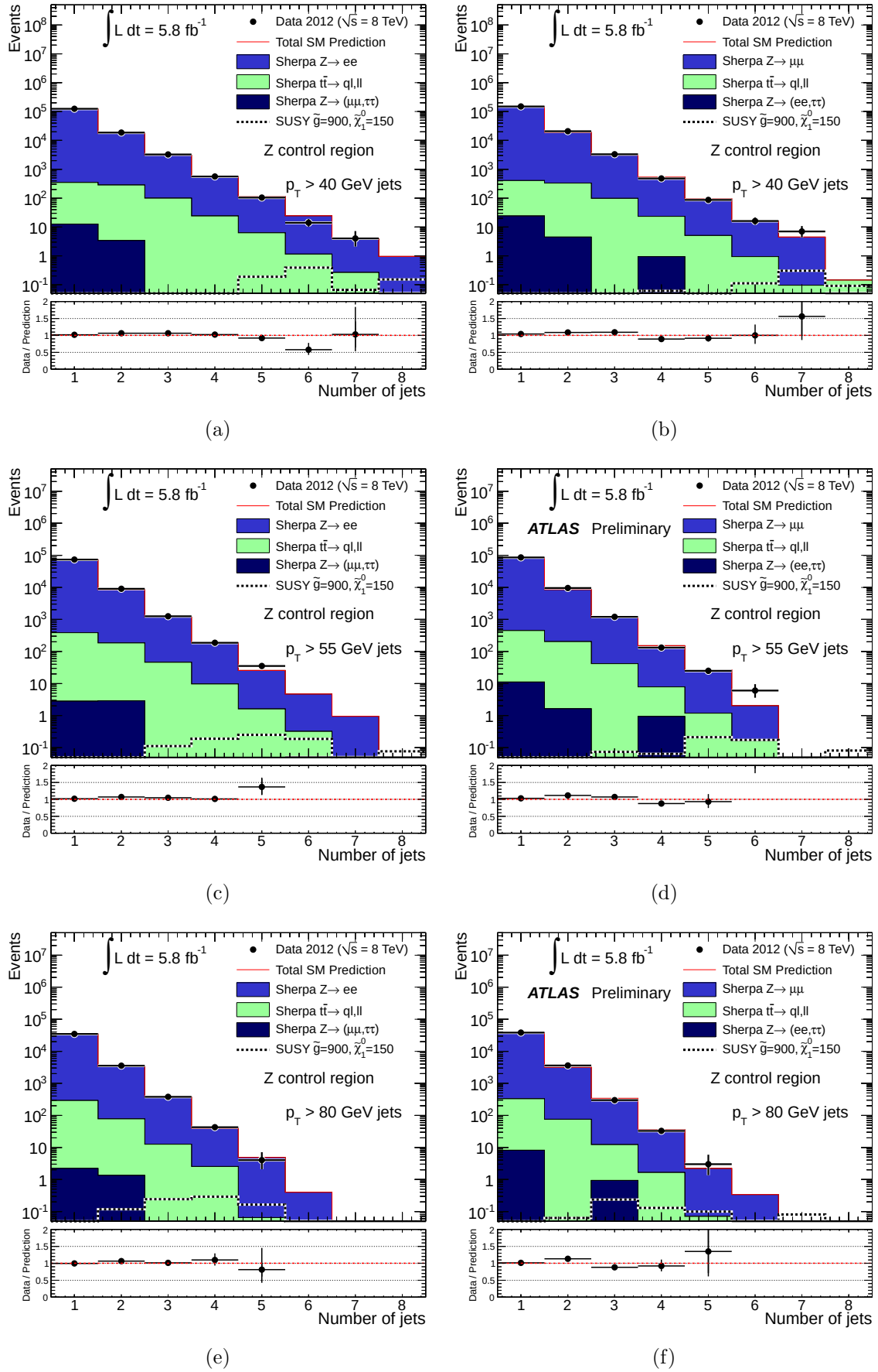
Figure 7.10: The jet multiplicity distribution for the control regions for Z +jets. (a) and (b) show the jet multiplicity distribution for p_T > 40 GeV jets for the electron and muon selections respectively. (c) and (d) show the distribution for p_T > 55 GeV jets while (e) and (f) are for p_T > 80 GeV jets.
