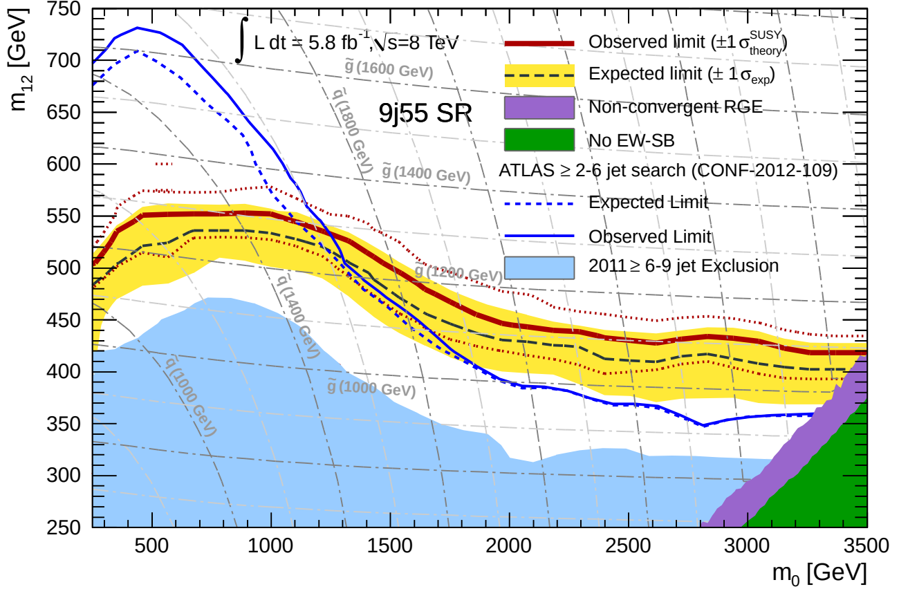
Figure 7.13: The limit in the MSUGRA/CMSSM plane with the same colour scheme as Figure 7.12. The blue shaded area shows the points excluded by the ATLAS multi-jets and missing transverse momentum analysis using 4.7 \text{ fb}^{-1} of 7 TeV data recorded in 2011 [3]. The blue solid and dashed lines give the observed and expected limit from a search requiring \geq 2 - 6 jets using the same dataset as the search presented here [88].
