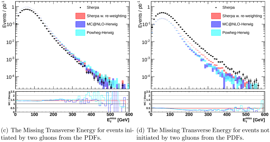
Figure 7.7: Truth level motivation for the t\bar{t} re-weighting. (a) and (b) show the E_T^{\text{miss}} and leading lepton p_T , for di-leptonic (electron or muon) t\bar{t} events. The PowHeg and MC@NLO (both showered with HERWIG ) simulations are seen to be softer than the SHERPA Monte-Carlo. (c) and (d) show the E_T^{\text{miss}} distribution for events initiated by two gluons and others respectively. It is clear that the agreement between the LO multi-leg Monte-Carlo can be improved by re-weighting in this variable. This is seen in (a) and (b) where the re-weighted Sherpa distribution is also shown. All of the error bands are purely statistical.
