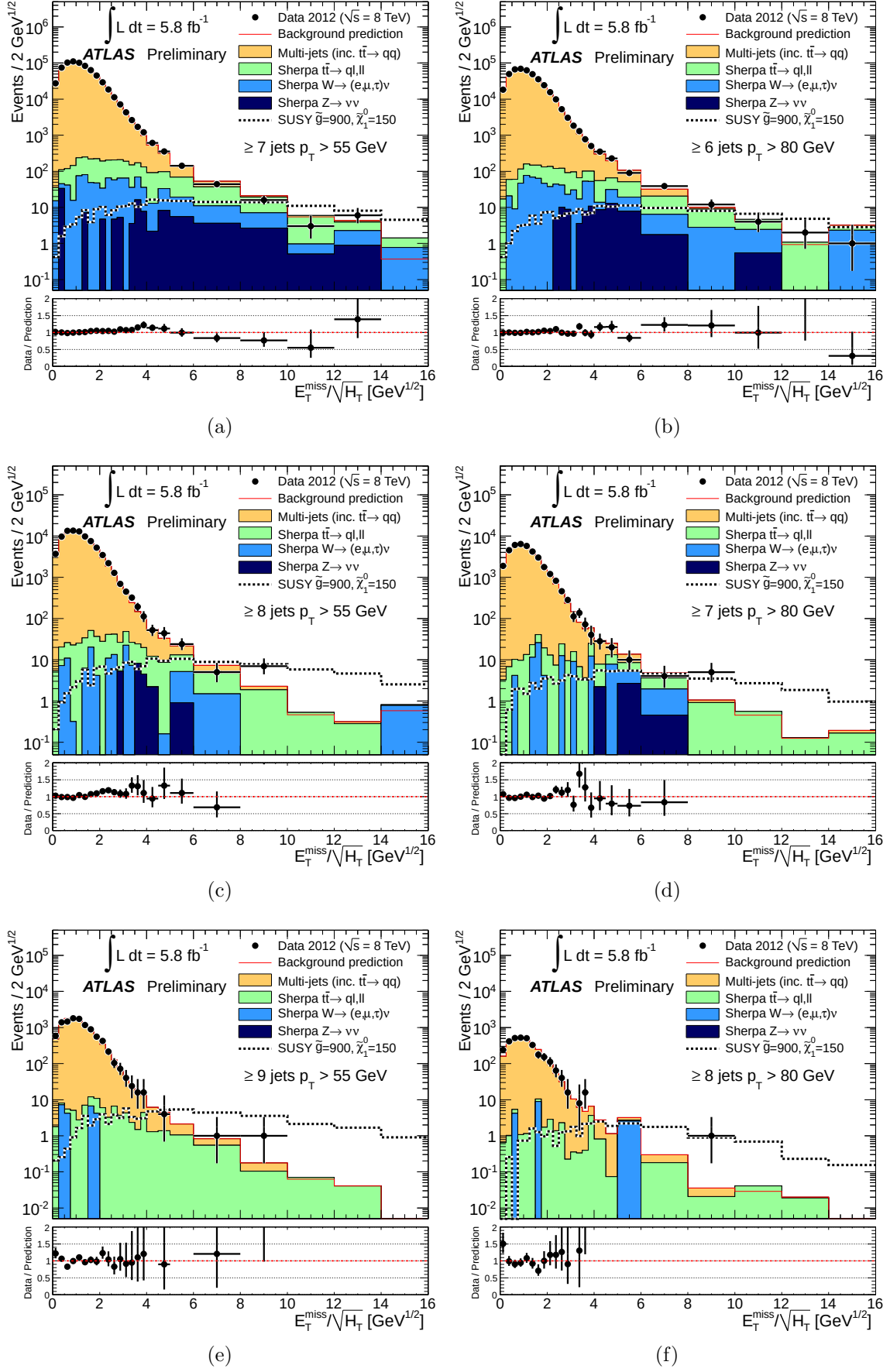
Figure 7.11: The E_T^{\text{miss}} / \sqrt{H_T} distributions for the six signal regions before the final cut of E_T^{\text{miss}} / \sqrt{H_T} > 4 GeV 1/2 .
