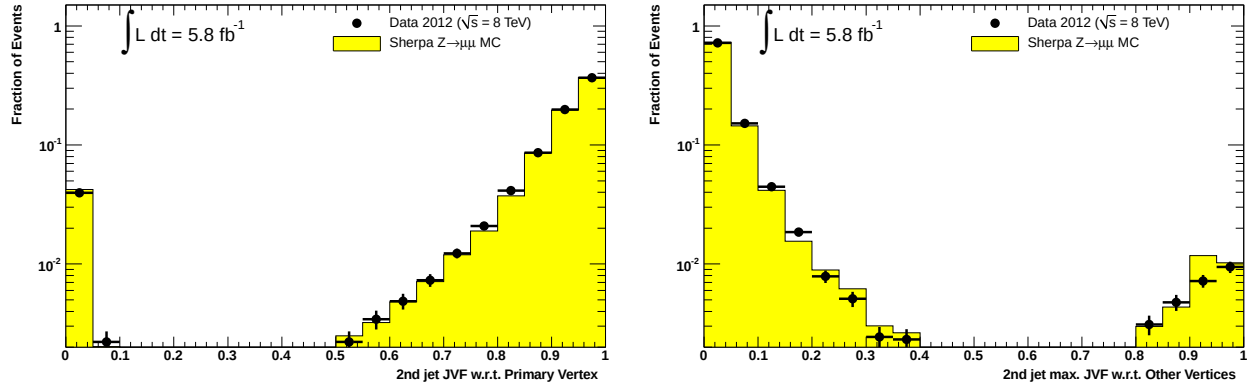
(a) The fraction of the momenta of tracks pointing at the sub-leading jet which originate from the 1st primary interaction vertex. (b) The maximum fraction of the momenta of tracks from a vertex other than the leading primary vertex pointing at the sub-leading jet.
