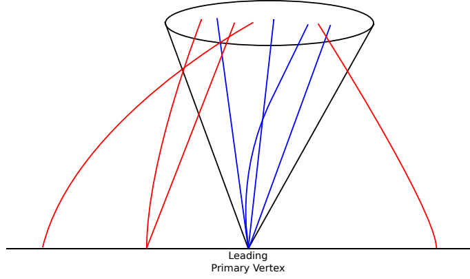
Figure 7.2: A pictorial illustration of the quantity used to evaluate the effect of pile-up. The ratio is taken of the sum of the transverse momenta of tracks from the leading primary vertex associated with the jet (blue) to the sum of the transverse momenta of all tracks associated with the jet (red and blue). ( Not to scale. )
