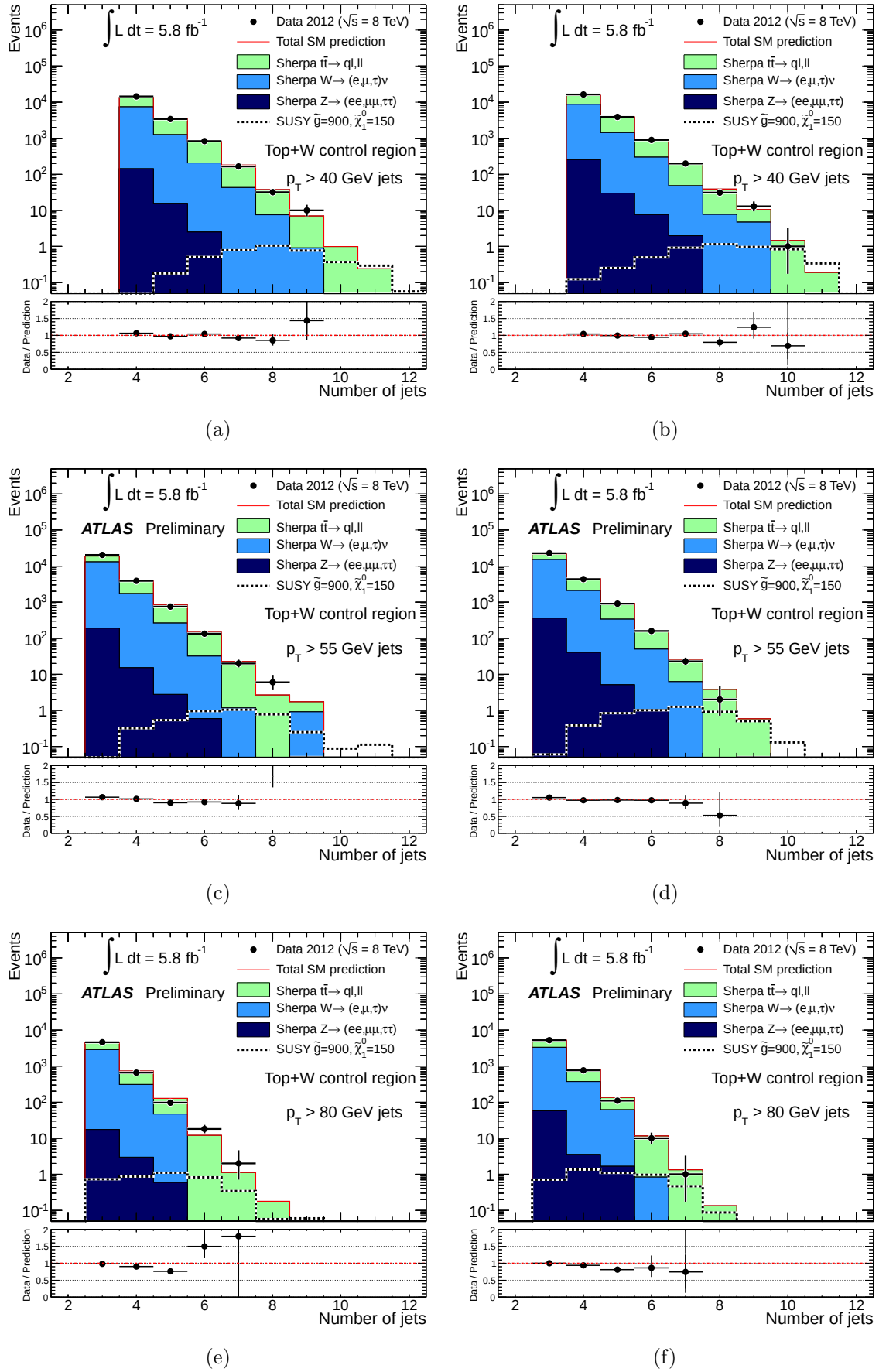
Figure 7.8: The jet multiplicity distribution for the control regions for t\bar{t} and W +jets. (a) and (b) show the jet multiplicity distribution for p_T > 40 GeV jets for the electron and muon selections respectively. (c) and (d) show the distribution for p_T > 55 GeV jets while (e) and (f) are for p_T > 80 GeV jets.
