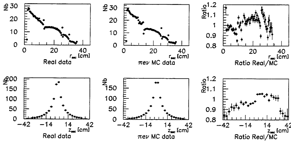
Figure 6.10: r_{sec} and z_{sec} distributions of the secondary vertex.
