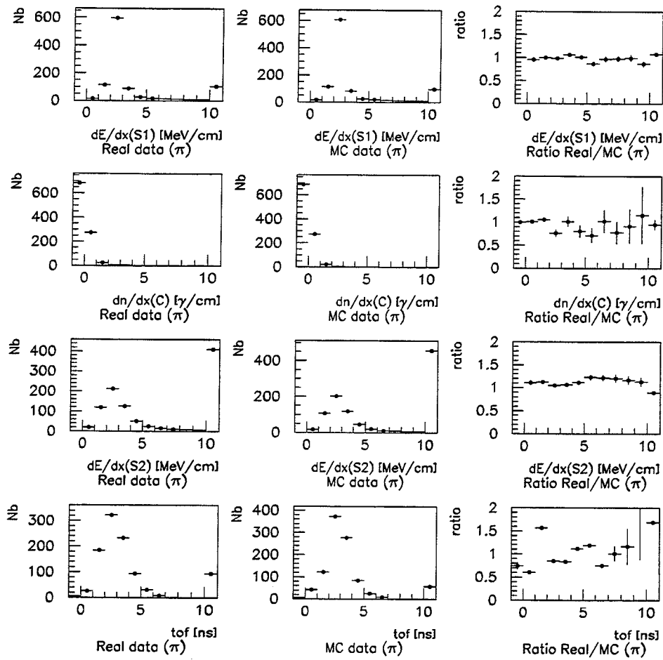
Figure 5.5: Corrected PID response to the pions . The four rows correspond to the d1dx , dndx , d2dx and tof . In each row, the real and simulation data distributions, as well as their ratio are presented. This ratio is expected to be constant if the variable is correctly described by the simulation. It should be noted that the number of events in the distributions is arbitrary.
