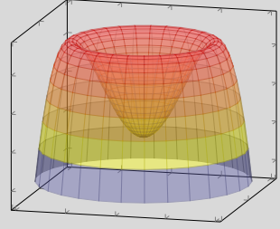
(b) \mu^2 > 0, \lambda > 0 .
