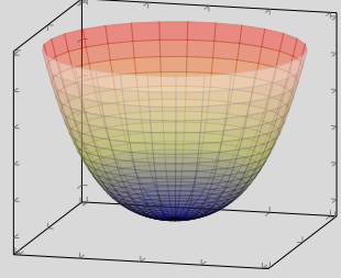
(a) \mu^2 < 0, \lambda < 0 .
