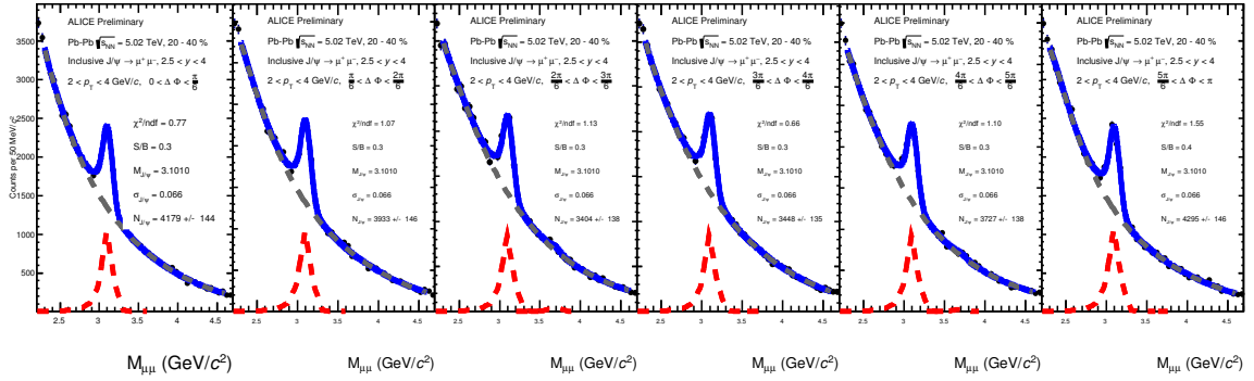
Figure 5.7 – Example of J/\psi invariant mass distributions for 2 < p_T < 4 GeV/c and 2.5 < y < 4 in the 20–40 % centrality range for 6 \Delta\phi bins
