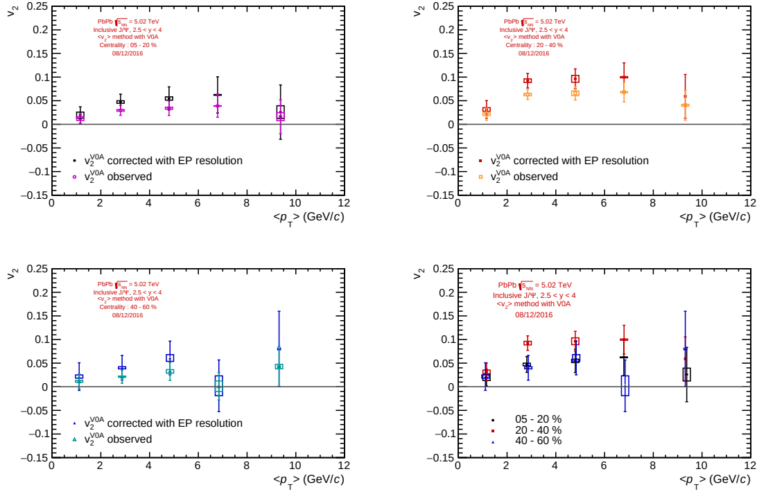
Figure 5.12 – Inclusive J/\psi v_2 as a function of p_T in the rapidity range 2.5 < y < 4 in 3 centrality classes using the mean v_2 method and the VOA as event plane detector. Boxes represent the systematic uncertainty from the signal extraction.
