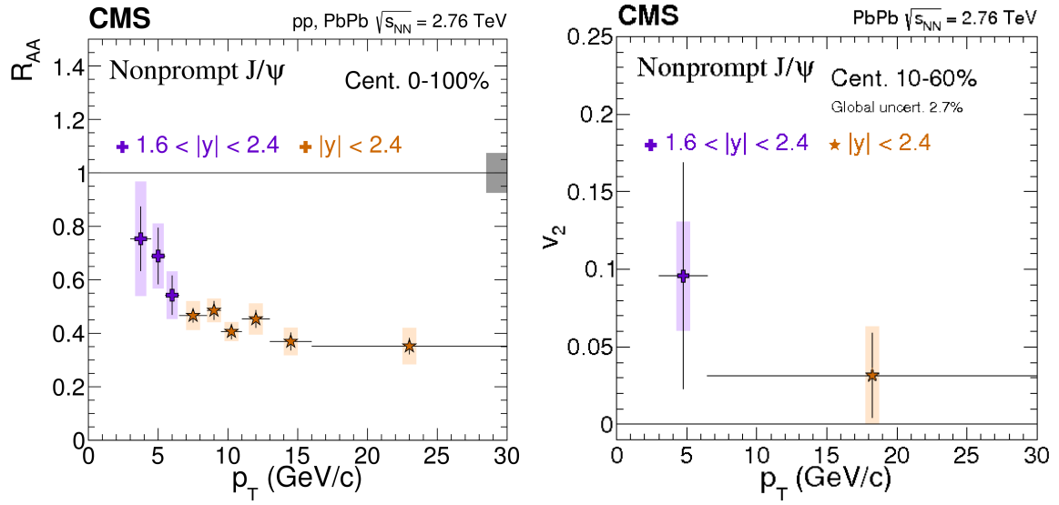
Figure 4.17 – p_T dependence of non-prompt J/ \psi R_{AA} (Left) and \nu_2 (Right) measured with the CMS detector [K + 17]
