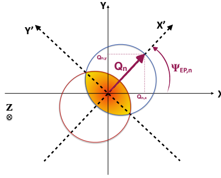
Figure 5.1 – Illustration of the event plane frame
