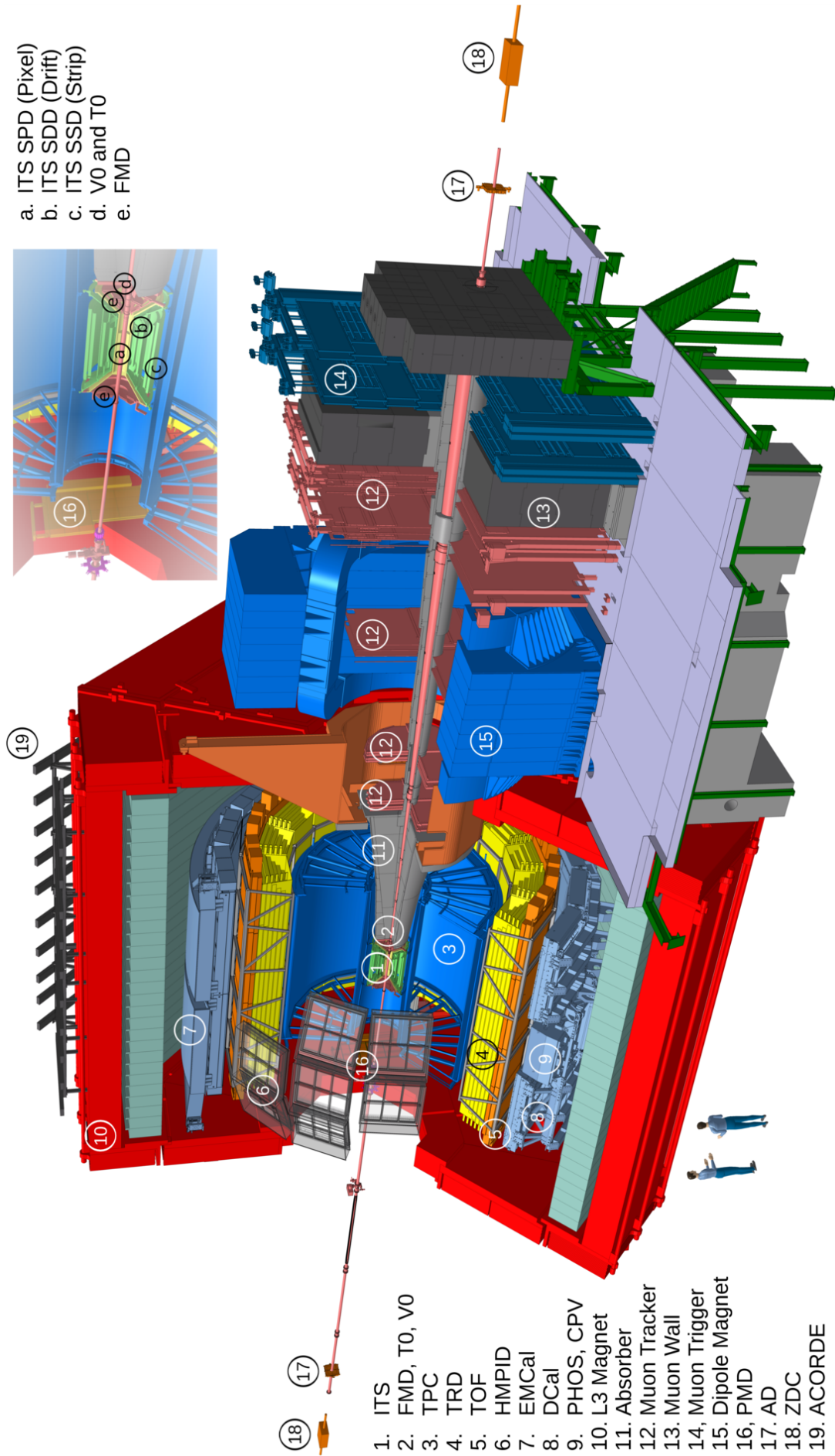
Figure 2.5 – The ALICE apparatus and its subdetectors
