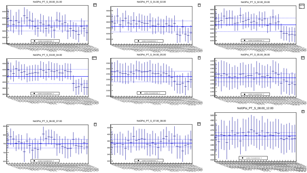
Figure B.11 – In-plane signal extraction tests for the 20-40% centrality class
