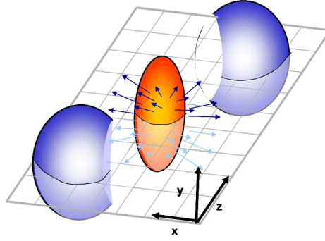
Figure 3.1 – Illustration of the reaction plane
