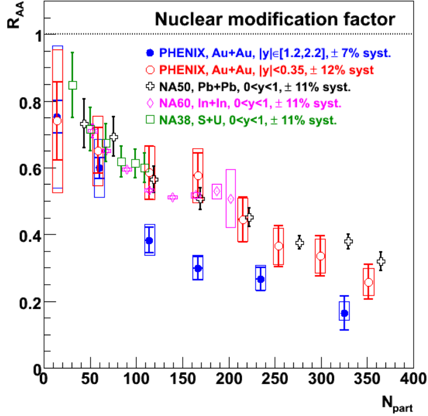
Figure 4.5 – Comparison of J/\psi nuclear modification factors as a function of the number of participants at RHIC and SPS for various collision systems [dC13]
