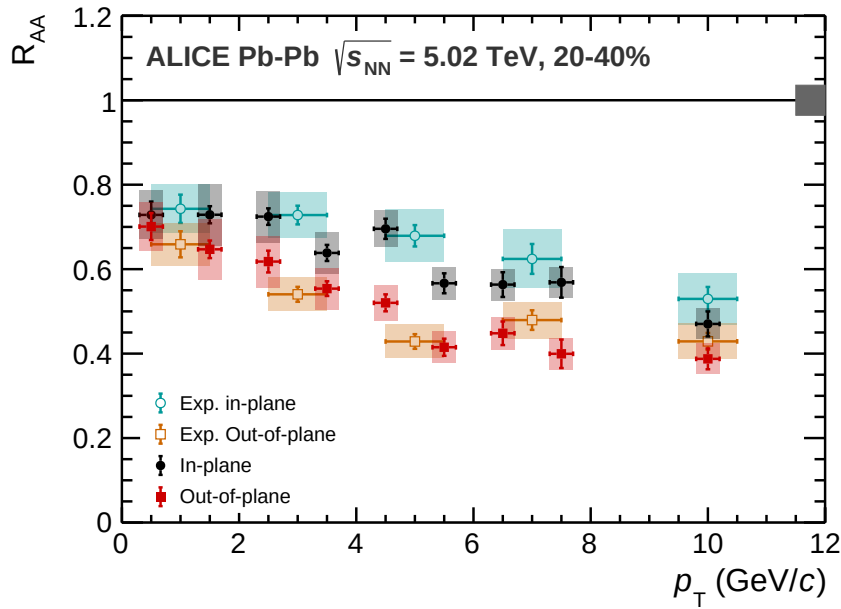
Figure 5.34 – Comparison of nuclear modification factor values from the in- and out-of-plane binning analysis to the computed values from integrated R_{AA} and v_2 results for the 20–40% centrality class
