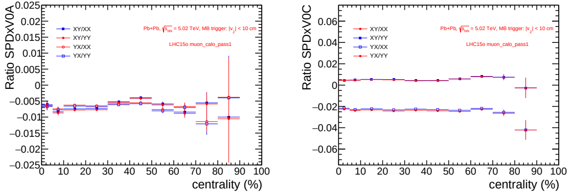
Figure 5.18 – (Left) Ratio of \langle Q_{2,x}^{SPD} Q_{2,y}^{V0A} \rangle and \langle Q_{2,y}^{SPD} Q_{2,x}^{V0A} \rangle by \langle Q_{2,x}^{SPD} Q_{2,y}^{V0A} \rangle and \langle Q_{2,y}^{SPD} Q_{2,x}^{V0A} \rangle , (Right) Ratio of \langle Q_{2,x}^{SPD} Q_{2,y}^{V0C} \rangle and \langle Q_{2,y}^{SPD} Q_{2,x}^{V0C} \rangle by \langle Q_{2,x}^{SPD} Q_{2,y}^{V0C} \rangle and \langle Q_{2,y}^{SPD} Q_{2,x}^{V0C} \rangle as a function of centrality
