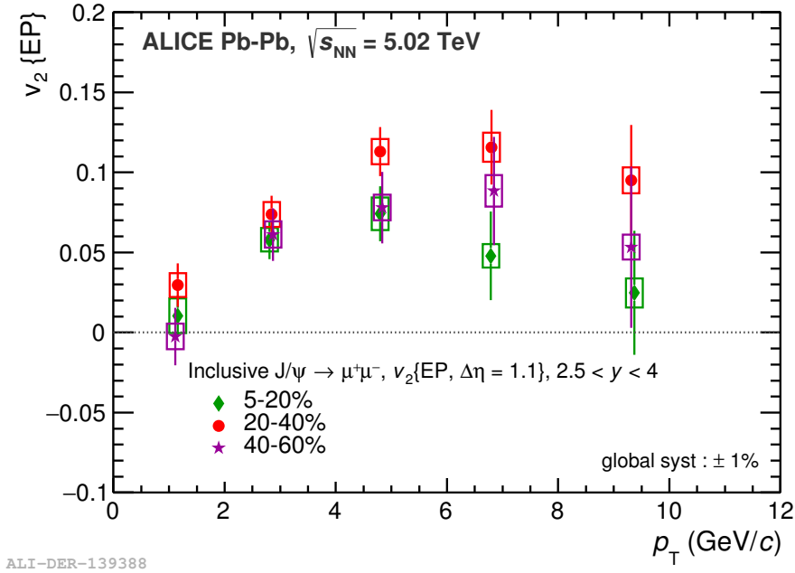
Figure 6.1 – J/\psi v_2 in Pb–Pb collisions at \sqrt{s_{NN}} = 5.02 TeV at forward rapidity for three centrality classes. Numerical values can be found in Tab. 5.5 and Tab. 5.4
