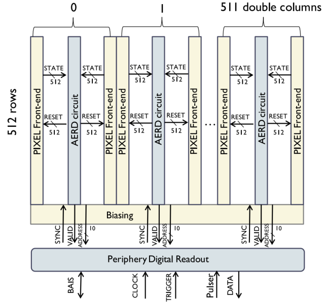
Figure 2.11 – Structure of the ALICE Pixel Detector (ALPIDE) AERD circuit, figure taken from [Y + 15]
