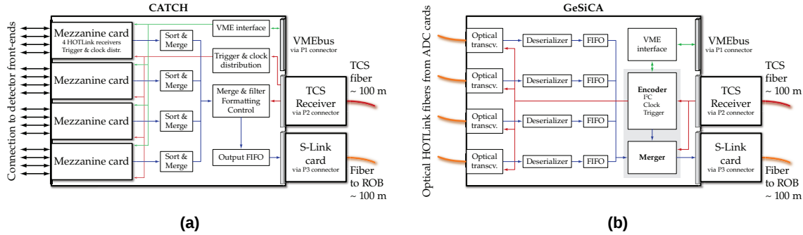
Figure 3.2: (a) Schematic of the CATCH module. (b) the same view of the GeSiCA. (from [Fis00] and [Gru01a], respectively)
