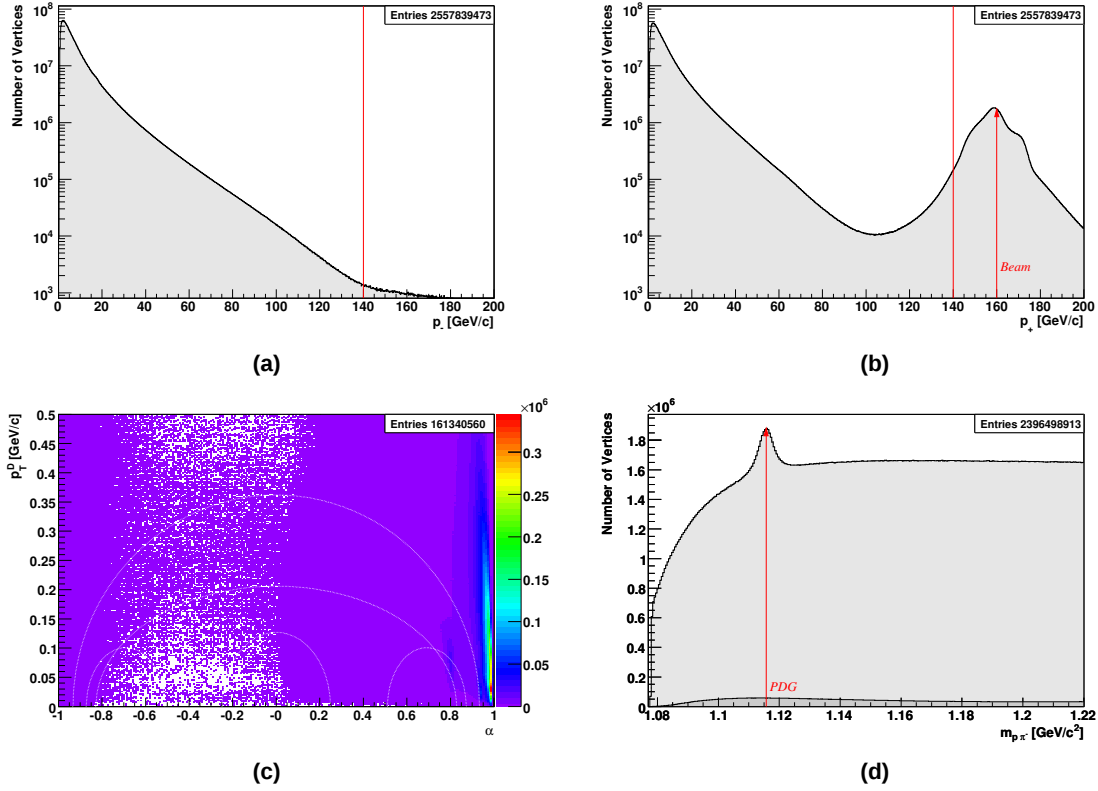
Figure 7.8: Suppression of halo muons: (a) Distribution of the momentum of the negative V^0 daughter particle. (b) shows the same for the positive particle. A peak around the beam momentum, indicated by the arrow, is clearly visible. The vertical line marks the cut on the momentum. (c) Armenteros plot of the sample, that was cut away. (d) m_{p\pi^-} invariant mass distribution after the cut. The darker area shows the sample, that was cut away.
