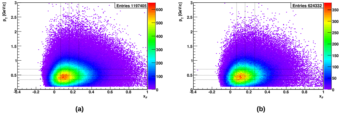
Figure 8.31: (a) Correlation of p_T and x_F for the \Lambda . The 4 \times 4 bins are indicated by lines. (b) shows the same for the \bar{\Lambda} . The two distributions are very similar, so that in both cases the same binning was applied.
