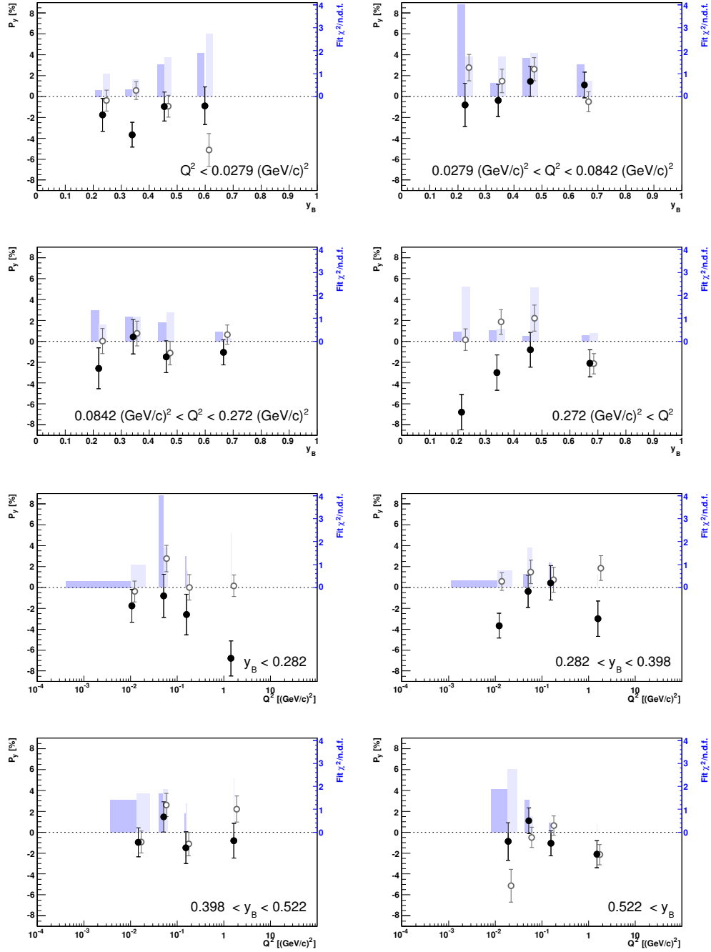
Figure 8.40: \bar{\Lambda} polarization as a function of Q^2 and y : The same conventions as in fig. 8.39 are used.
