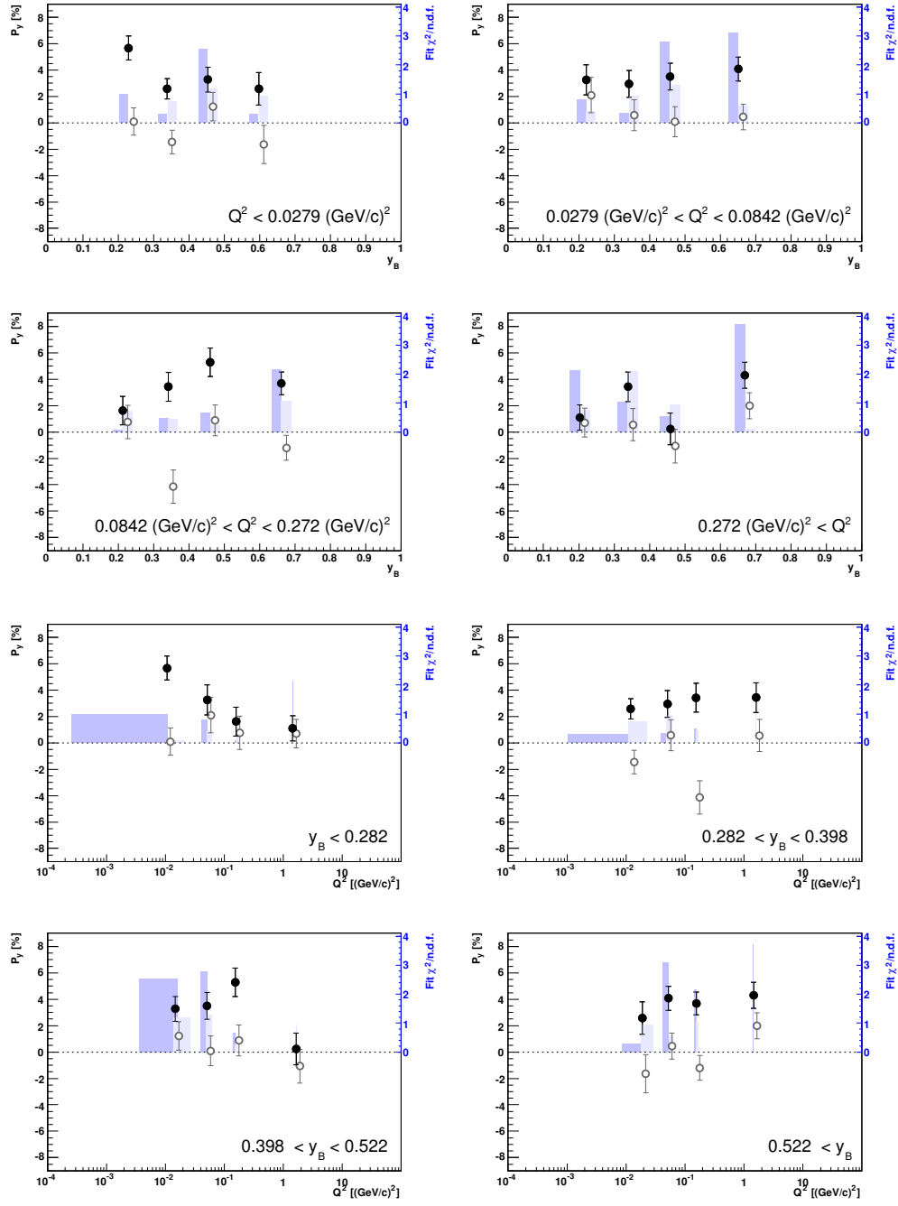
Figure 8.39: \Lambda polarization as a function of Q^2 and y : The upper four plots depict the y dependence of the \Lambda polarization (full circles) and that of the K^0 background (open circles, right shifted for better visibility) for the four bins in Q^2 . The lower four graphs show the same 16 data points, but this time the Q^2 dependence for the four y bins. The bars display the \chi^2/\text{n.d.f.} values of the respective R(\cos\theta_y) fits for the \Lambda (dark bars) and for the K^0 background (light bars).
