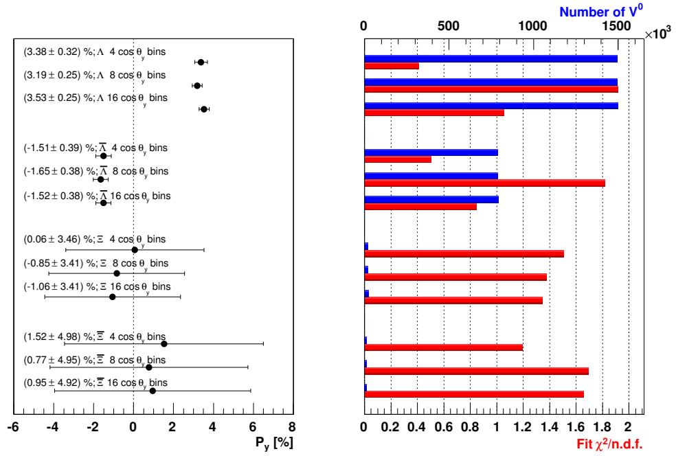
Figure 8.13: Dependence of \Lambda , \bar{\Lambda} , \Xi^- , and \Xi^+ polarizations on binning in \cos \theta_y : In each case the polarization is calculated using four, eight, and sixteen bins for the angular distributions R(\cos \theta_y) . The values show that the binning has no systematic effect on the polarization. The graph on the right displays for each point the total number of hyperons and the \chi^2/\text{n.d.f.} of the R(\cos \theta_y) fit.
