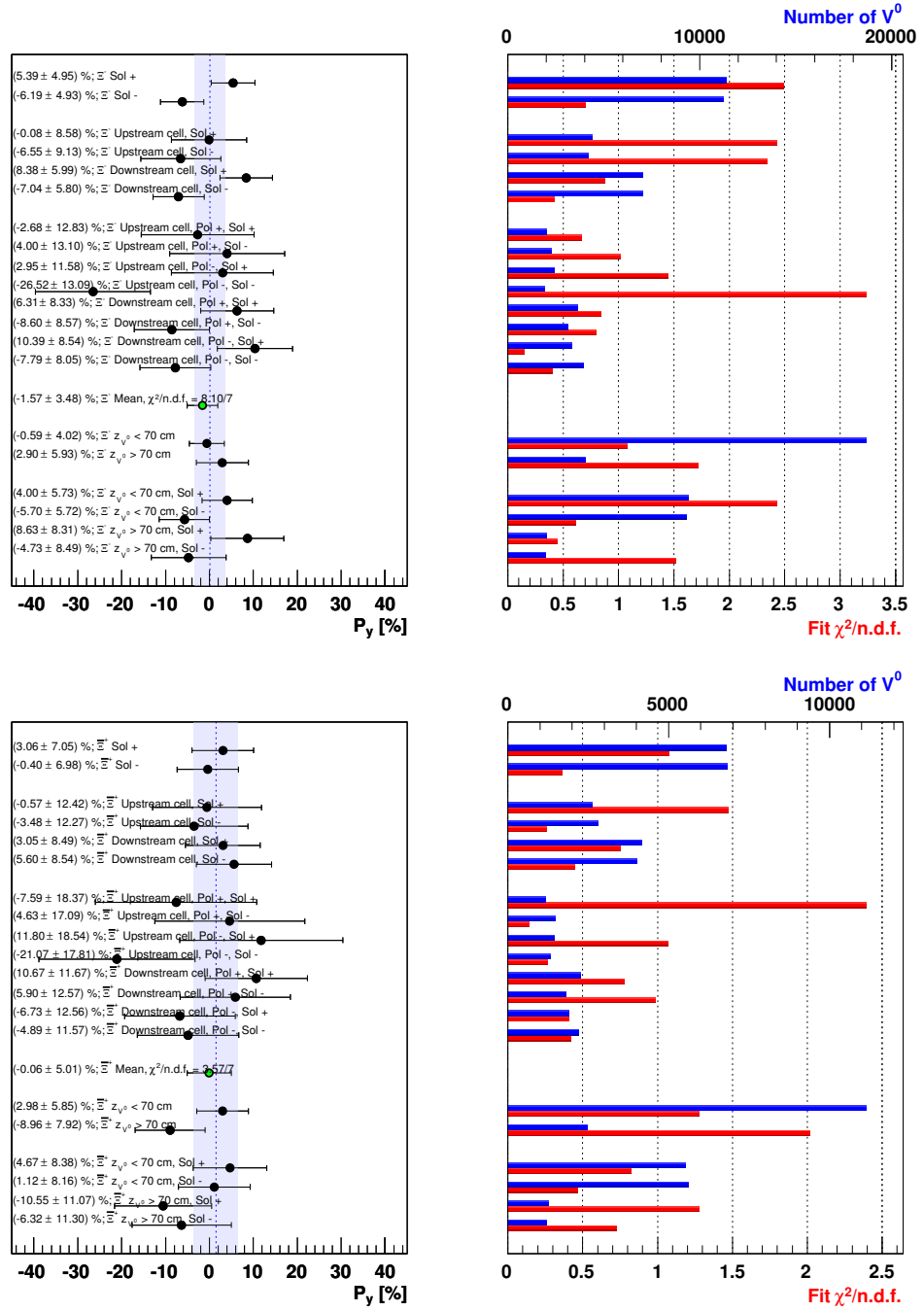
Figure 8.24: Influence of the target solenoid on the \Xi^- and \Xi^+ polarizations: The upper graph shows the \Xi^- polarization the lower one the results for the \Xi^+ . The definition of the bins is the same as in fig. 8.22.
