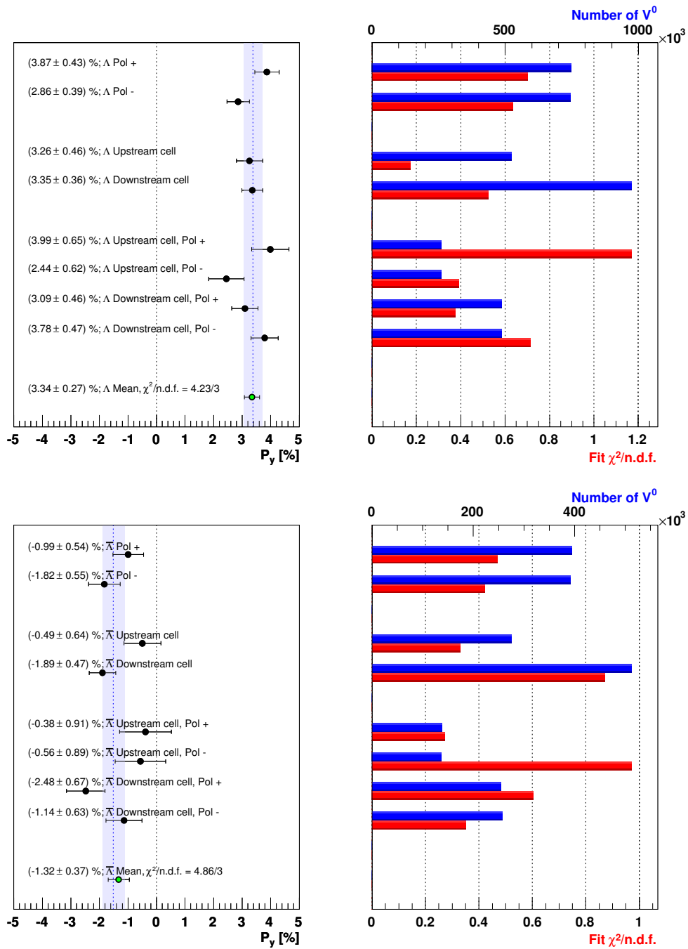
Figure 8.18: Dependence of the \Lambda and \bar{\Lambda} polarizations on the target polarization: The plot on the top shows the results for the \Lambda , the lower one for the \bar{\Lambda} . In each case the upper two points represent the hyperon polarization for the two possible configurations of the target cell polarizations (cf. subsection 2.2.3), where the sign refers to the state of the upstream cell. Within the statistical errors the polarizations agree with the respective overall polarization, that is indicated by the band. The next two points show, that the polarization does not depend on the target cell in which the hyperon was produced. Similarly the weighted means of the four disjoint subsamples for the two target cells and their polarization indicate no systematic influence of the polarization of the target material. The graphs on the right display for each point the total number of hyperons and the \chi^2/n.d.f. of the R(\cos \theta_y) fit.
