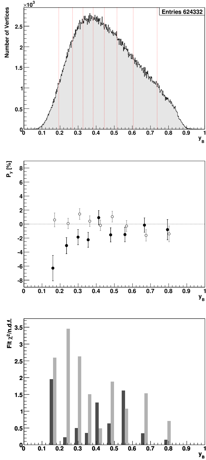
Figure 8.37: Dependence of the \bar{\Lambda} polarization on y : The conventions are the same as in fig. 8.36.
