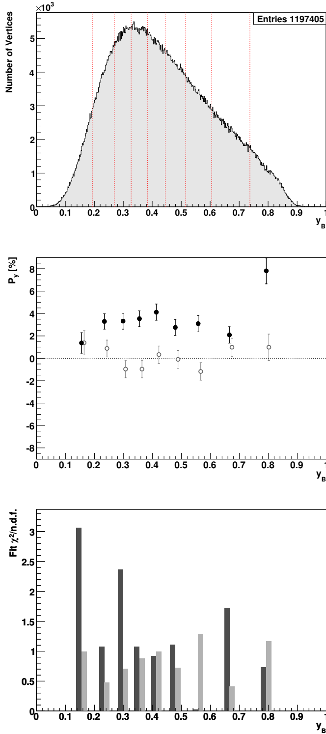
Figure 8.36: Dependence of the \Lambda polarization on the relative energy transfer y of the virtual photon: The upper plot depicts the background corrected y distribution. The definition of the bins is illustrated by vertical lines. The graph in the middle shows both the polarization values for the \Lambda (filled circles) and those of the K^0 background (open circles, right shifted for better visibility) at the average y values of the respective bins. The lower plot displays the \chi^2/n.d.f. values of the R(\cos \theta_y) fits for the \Lambda (dark bars) and for the K^0 background (light bars).
