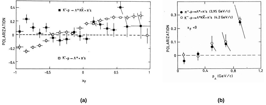
Figure 8.44: (a) \Lambda polarization in a 4.2 GeV/c K^- beam measured over the full x_F range: Depending on whether the s quark in the \Lambda stems from the beam ( K^-p \rightarrow \Lambda + (\pi)_n ) or from the sea ( K^-p \rightarrow \Lambda K \bar{K} + (\pi)_n ), the polarization exhibits a different behavior in the target fragmentation region. (from [Gan78]) (b) p_T dependence of the \Lambda polarization in the target fragmentation region: If the s quark of the \Lambda stems from the sea the polarization is independent of the beam particle. (from [Ade84])
