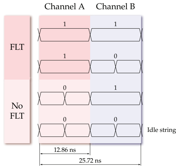
Figure 5.2: The four possible symbols, that can be transmitted during one TCS clock cycle using two-channel time division multiplexing with a biphase mark encoding. (from [Tay98])
