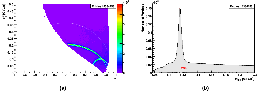
Figure 7.17: \Lambda sample after selection: (a) Armenteros plot and (b) m_{p\pi^-} invariant mass distribution of the final \Lambda sample after excluding events, that were exclusively triggered by the outer or the middle trigger hodoscopes. The darker area in (b) shows the sample, that was cut away.
