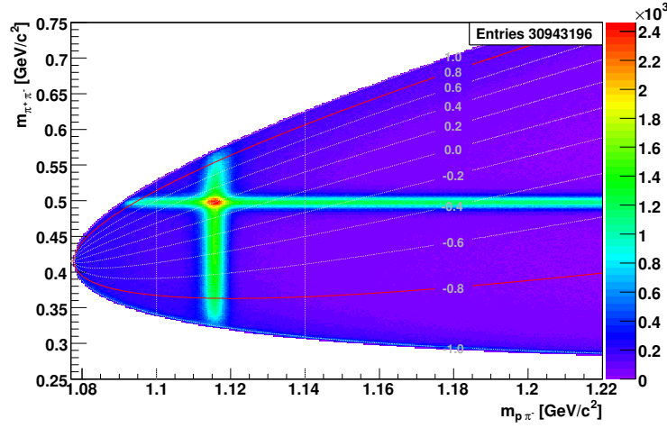
Figure 7.35: Iso- \cos \theta_z lines in the (m_{p\pi^-}, m_{\pi^+\pi^-}) invariant mass histogram without cut on \cos \theta_z . The kinematical boundary is described by the lines \cos \theta_z = \pm 1 . The red curves show the effective boundary of the histogram, defined by the cut |\cos \theta_z| < 0.8 . The vertical lines indicate the position of the slices shown in fig. 7.37
