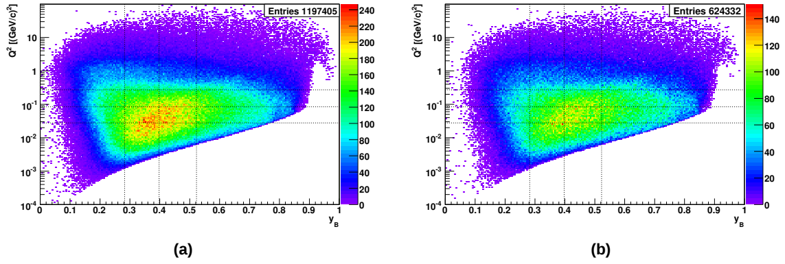
Figure 8.38: (a) Correlation of Q^2 and y for the \Lambda . The 4 \times 4 bins are indicated by lines. (b) shows the same for the \bar{\Lambda} . The two distributions are very similar, so that in both cases the same binning was used.
