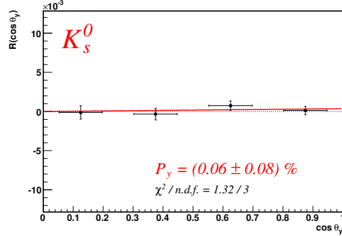
Figure 8.3: Angular distribution R(\cos \theta_y) and polarization for the overall K^0 sample: The polarization is small and compatible with zero. The straight line hypothesis has a probability of 72.4 %.
