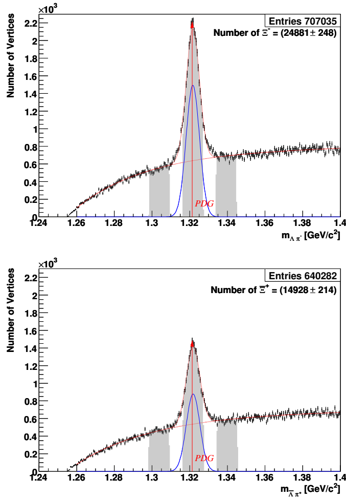
Figure 7.30: Final \Xi^- and \Xi^+ samples after event selection: The upper plot shows the m_{\Lambda\pi^-} , the lower one the m_{\Lambda\pi^+} distribution of the final \Xi sample, where the \Lambda ( \bar{\Lambda} ) mass was fixed to its nominal value. The 24,900 \Xi^- s have a mean mass of 1321.7 \text{ MeV}/c^2 , which corresponds to a deviation of \Delta m = 400 \text{ keV}/c^2 with respect to the PDG value. The width of the \Xi^- peak is 3.54 \text{ MeV}/c^2 . The mass of the 14,900 \Xi^+ s is measured to 1321.8 \text{ MeV}/c^2 ( \Delta m = 500 \text{ keV}/c^2 ) with a mass resolution of 3.61 \text{ MeV}/c^2 . The fitting procedure is described in subsection 7.4.2. In both plots the shaded bands indicate the peak- and side-band regions used for the background subtraction.
