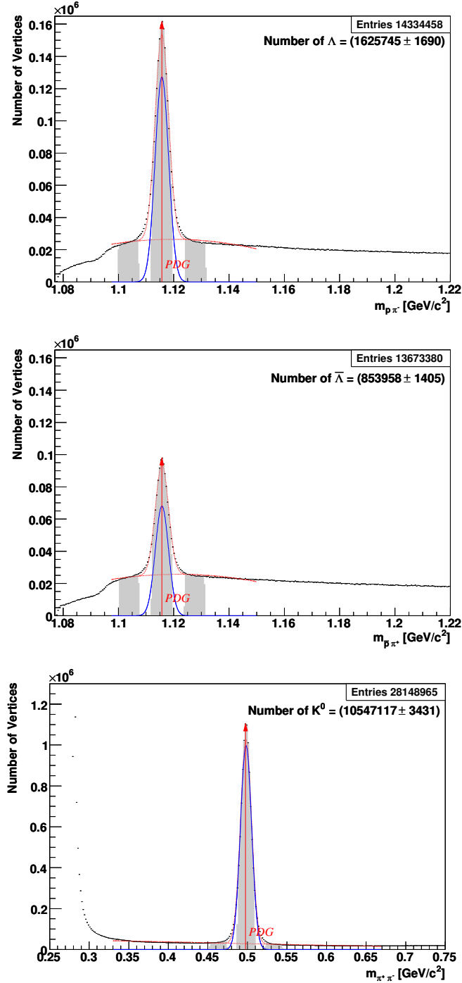
Figure 7.18: Final \Lambda and \bar{\Lambda} samples after event selection: The upper two plots show the m_{p\pi^-} and the m_{\bar{p}\pi^+} invariant mass distributions, respectively. The 1,626,000 \Lambda s in the peak have a mean mass of 1115.72 \text{ MeV}/c^2 , which corresponds to a deviation of \Delta m = 40 \text{ keV}/c^2 with respect to the PDG value. The width of the \Lambda peak is \sigma_\Lambda = 2.43 \text{ MeV}/c^2 . The mass of the 854,000 \bar{\Lambda} s is measured to 1115.74 \text{ MeV}/c^2 ( \Delta m = 60 \text{ keV}/c^2 ) with a resolution of \sigma_{\bar{\Lambda}} = 2.38 \text{ MeV}/c^2 . The lower plots depicts the m_{\pi^+\pi^-} invariant mass distribution. The 10,547,000 K^0 s are reconstructed with a mass of 498.24 \text{ MeV}/c^2 ( \Delta m = 590 \text{ keV}/c^2 ) and a width of \sigma_{K^0} = 7.02 \text{ MeV}/c^2 . The fitting procedure is described in subsection 7.4.1. In all three plots the shaded bands indicate the peak- and side-band regions used for the background subtraction.
