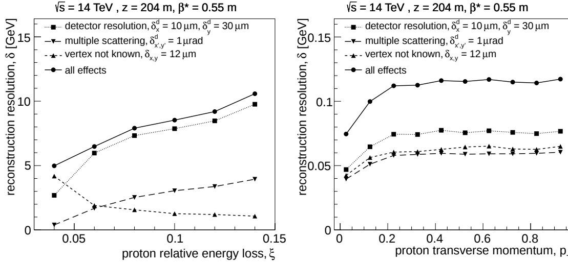
Figure 3.15.: The resolution of the reconstructed proton relative energy loss (left) and transverse momentum (right). The experimental effects taken into account are: the AFP detector spatial resolution, the lack of information about the vertex coordinates, and multiple scattering. Taken from [29].
