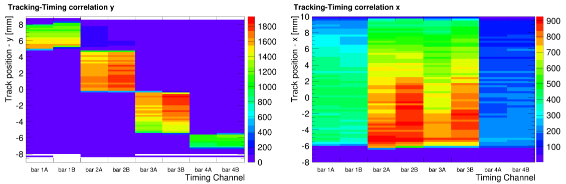
Figure 3.40.: Correlation between timing channel and reconstructed track position along y (left) and x (right) at V_{MCP-PMT}=1,800 V.
