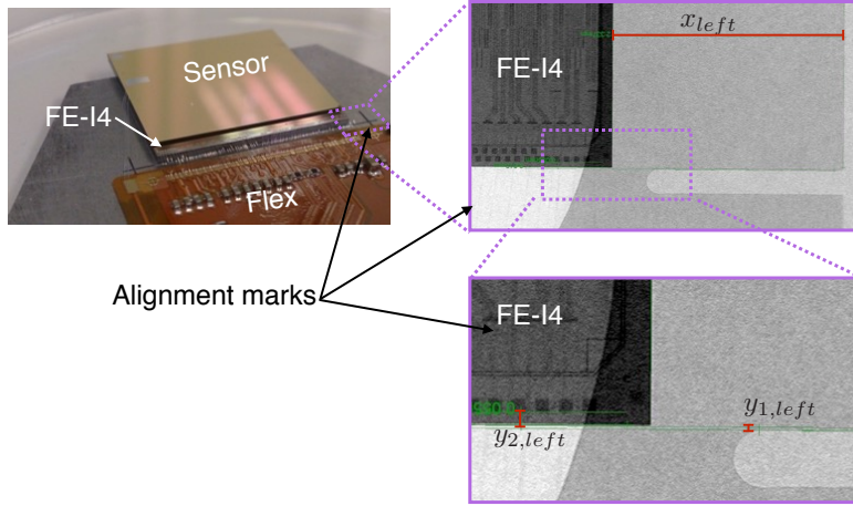
Figure 4.6.: X-ray picture of an assembly module showing the positions measured for the alignment determination.
