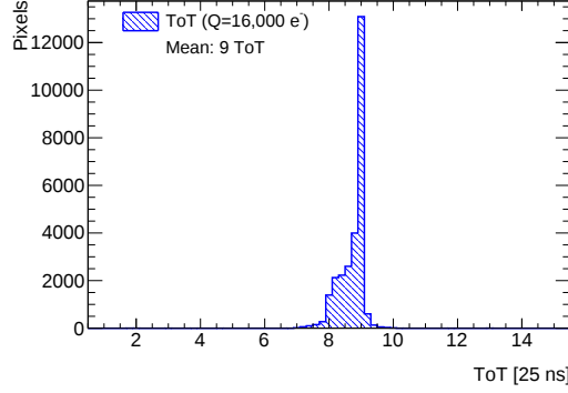
Figure 3.22.: Results from a ToT scan after calibration, using an injected charge of 16000 electrons.
