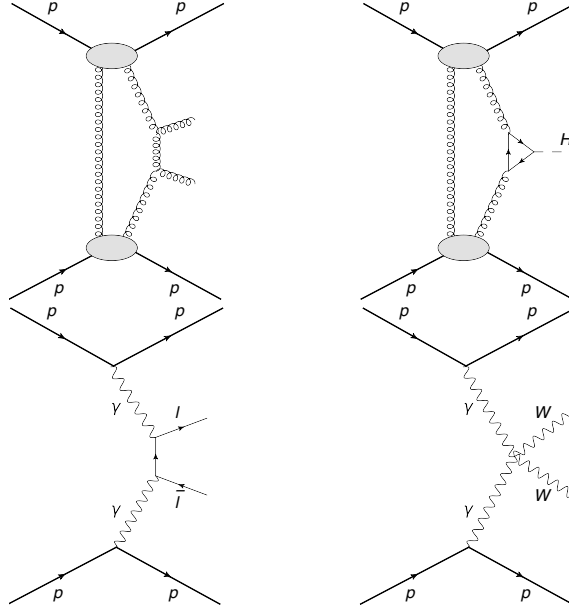
Figure 1.9.: Feynman diagrams of central exclusive production processes (top) with a dijets (left) and a Higgs boson (right) in the final state. Below are Feynman diagrams of \gamma\gamma productions with two leptons and intact protons (left), and two gauge bosons ( W , Z or \gamma ) and two protons in the final state (right).
