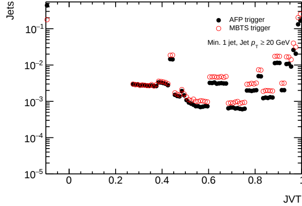
Figure 5.6.: Jet-Vertex-Tagger distribution for AFP triggered data (black) and Minimum Bias triggered data (red), with p_T \geq 20 GeV in events with exactly one primary vertex. The value JVT = -0.1 is assigned to jets with no associated tracks.
