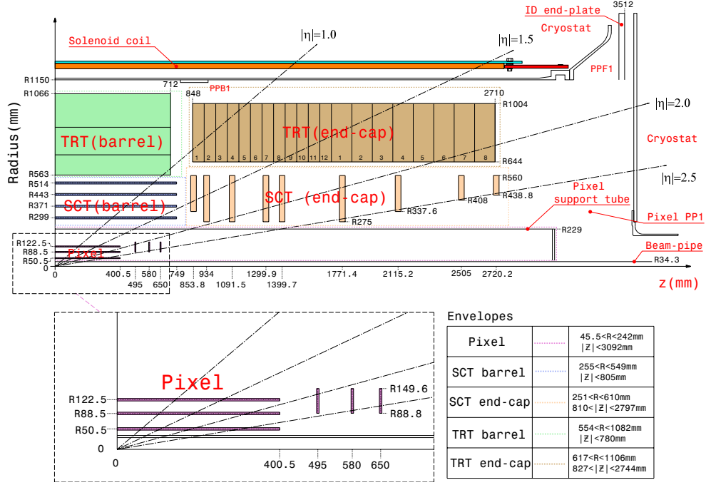
Figure 2.4: Schematic view of the quarter-section of the ATLAS inner detector [42]. The Insertable B-layer is not shown but fits inside the pixel detector.
