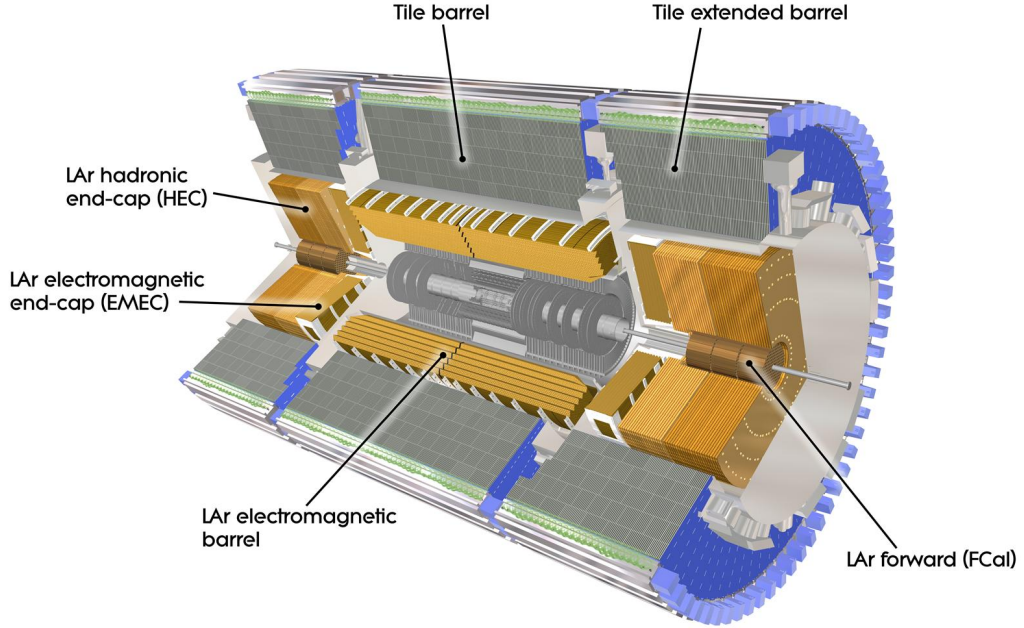
Figure 2.5: The structure of the ATLAS calorimeter [42].
