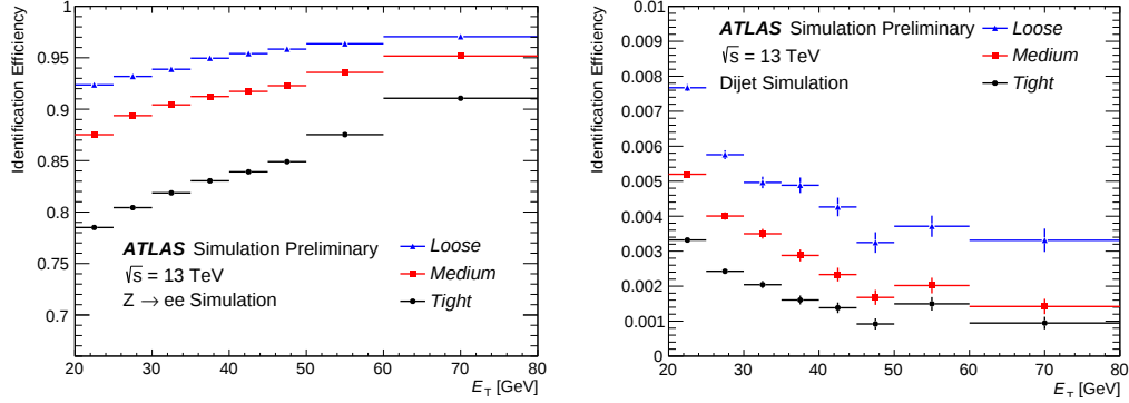
Figure 3.1: (left) Electron and (right) background identification efficiencies for the three working points as a function on the transverse energy [49].
