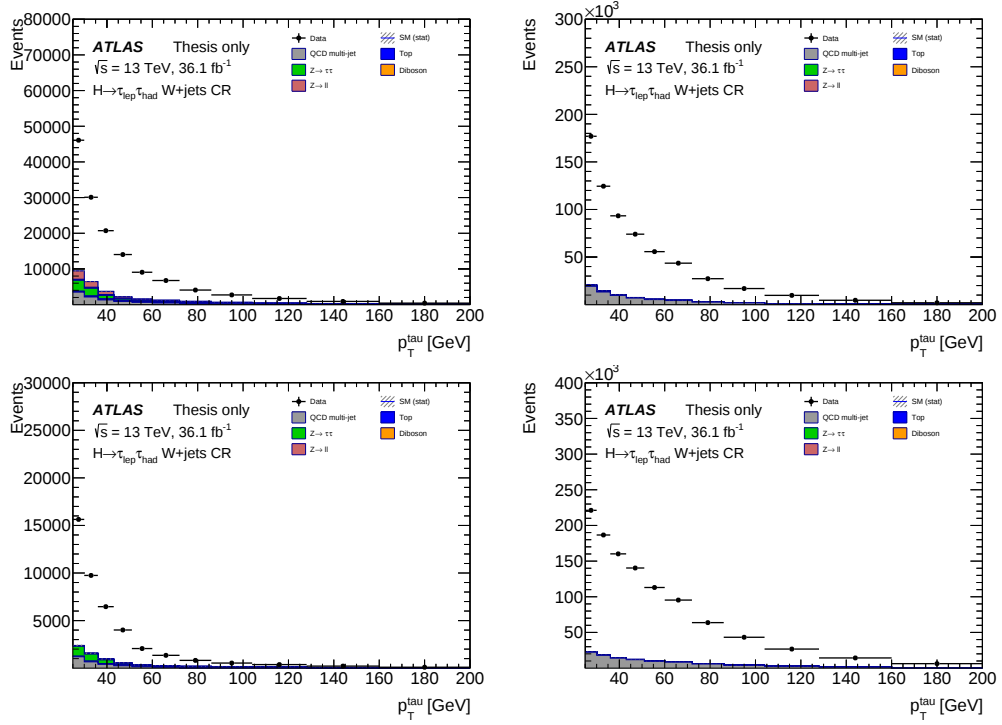
Figure 4.5: \tau_{\text{had}} transverse momentum distributions in combined electron and muon channels in W+\text{jets} Control Region. Shown are events with (top) 1-prong and (bottom) 3-prong \tau_{\text{had}} candidates (left) passing and (right) failing the tau identification criterion. The difference between the data and background is taken as the W+\text{jets} contribution.
