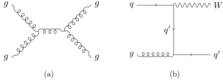
Figure 4.2: Leading order Feynman diagrams for (a) QCD multi-jet and (b) W+jets processes.
