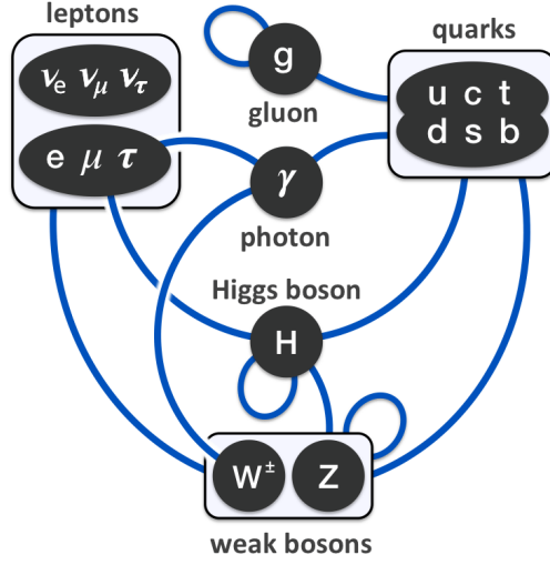
Figure 1.2: Interactions between particle in the SM [5].
