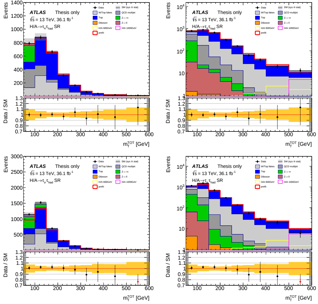
Figure 4.20: Post-fit distributions of the total transverse mass in the b -tag category of the (top) electron and (bottom) muon channels displayed in (left) linear and (right) logarithmic scales. The ratio of the data and the expected background events is shown in the lower panel of each subplot. Statistical and systematic uncertainties are included in the error band.
