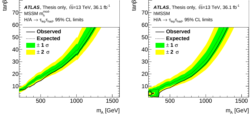
Figure 4.23: 95% confidence level exclusion limits in the m_A - \tan\beta parameter space of the MSSM. The expected and observed limits are shown for the (left) m_h^{\text{mod-}} and (right) hMSSM benchmark scenarios.
