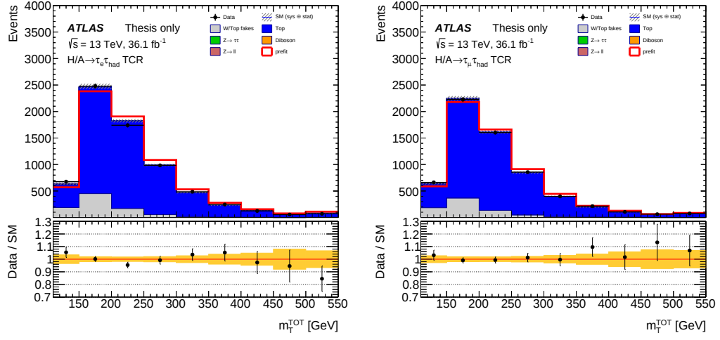
Figure 4.21: Post-fit distributions of the total transverse mass in the Top control region of the (left) electron and (right) muon channels. The ratio of the data and the expected background events is shown in the lower panel of each subplot. Statistical and systematic uncertainties are included in the error band.
