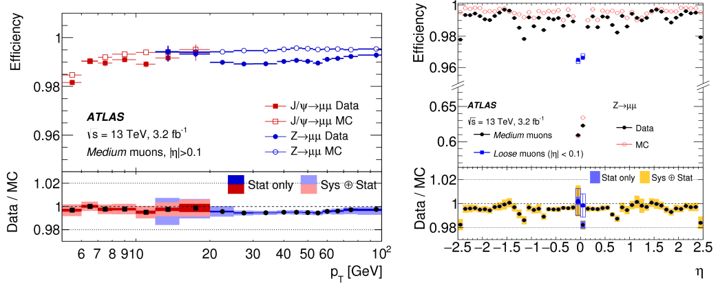
Figure 3.2: Muon reconstruction and identification efficiency for the “medium” working point as a function of the (left) muon p_T and (right) muon \eta [51].
