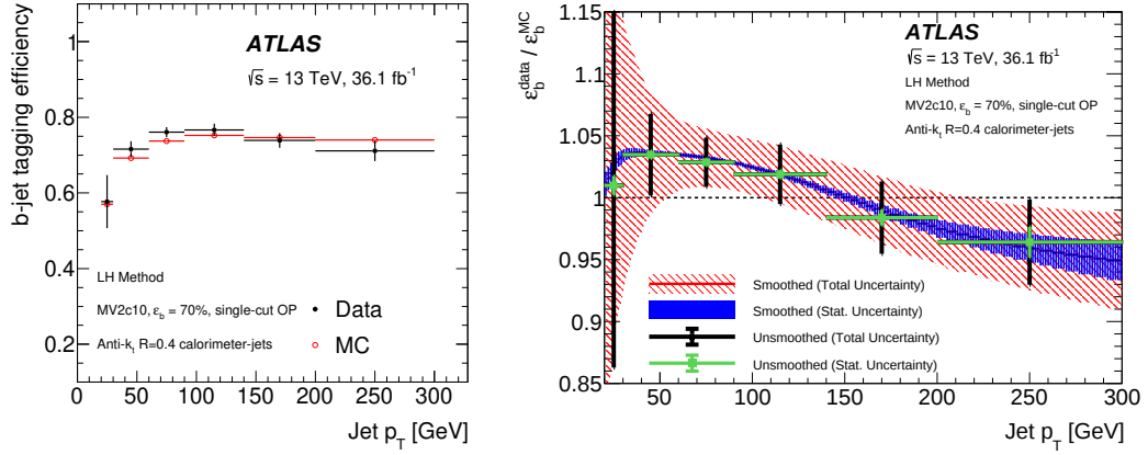
Figure 3.3: (left) The b -tagging efficiency of the 70% working point measured in data and simulation and (right) data-to-simulation scale factors [58].
