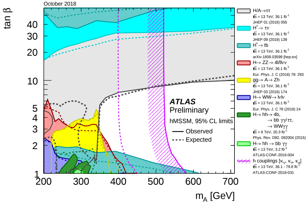
Figure 1.6: Summary plot of ATLAS searches for additional Higgs bosons interpreted in the hMSSM parameter space [32].
