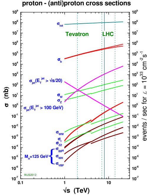
Figure 1.4: Cross sections of various processes in proton-(anti)proton collisions as a function of the center-of-mass energy [21]. The graph breaks appear due to the differences between proton-anti-proton (applicable at the Tevatron) and proton-proton (applicable at the LHC) collisions.
