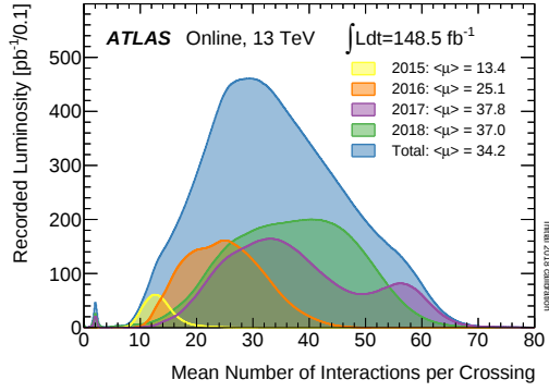
Figure 2.9: Distributions of the average number of interactions per bunch crossing in ATLAS during Run 2 [48].
