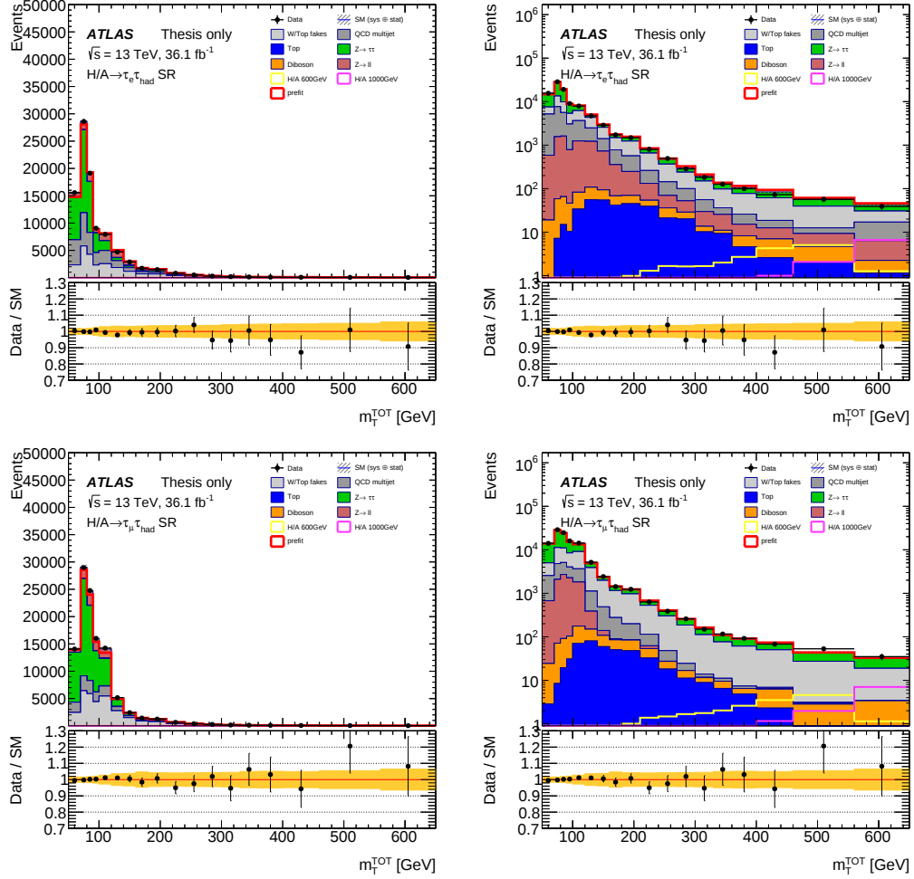
Figure 4.19: Post-fit distributions of the total transverse mass in the b -veto category of the (top) electron and (bottom) muon channels displayed in (left) linear and (right) logarithmic scales. The ratio of the data and the expected background events is shown in the lower panel of each subplot. Statistical and systematic uncertainties are included in the error band.
