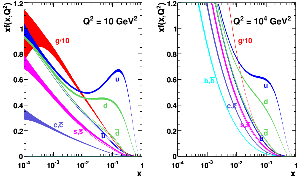
Figure 1.3: Parton distribution functions from the MSTW group [20]. The plots show the distributions for valence quarks, sea-quarks, and gluons, and the evolution of distributions from the interaction scale of (left) Q^2 = 10 \text{ GeV}^2 to (right) Q^2 = 10^4 \text{ GeV}^2 .
