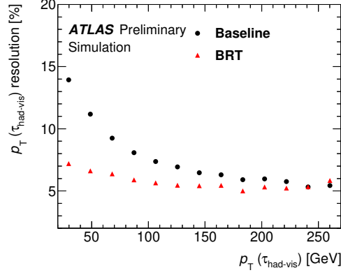
Figure 3.5: Tau energy resolution with the baseline and with the BRT calibrations applied [62].
