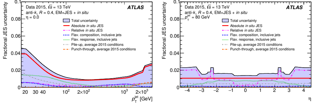
Figure 4.25: The jet energy scale uncertainty as a function of the (left) jet p_T and (right) jet \eta [56].
