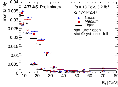
Figure 4.24: Electron reconstruction and identification uncertainties as a function of the electron E_T [49]. Uncertainties for electrons with p_T > 30 GeV and “medium” identification are below 0.5%.
