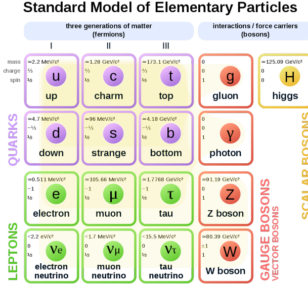
Figure 1.1: Particles of the Standard Model arranged by spin, mass, generation and electric charge [5].
