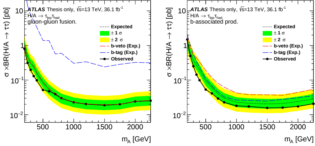
Figure 4.22: Higgs boson production cross-section times branching fraction to a pair of tau leptons 95% confidence level upper limits. The expected and observed limits are shown for the (left) gluon-gluon fusion and (right) b -associated production modes. The signal sensitivity in the b -veto and b -tag categories are indicated by the expected exclusion limits derived separately in those categories.
