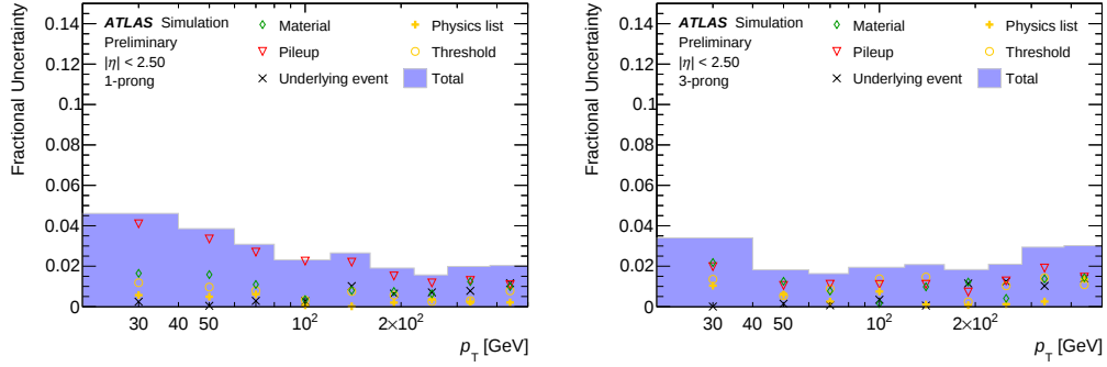
Figure 4.26: Systematic uncertainties of the reconstruction of hadronically decaying tau leptons as a function of the tau p_T for (left) 1-prong taus and (right) 3-prong taus [60].
