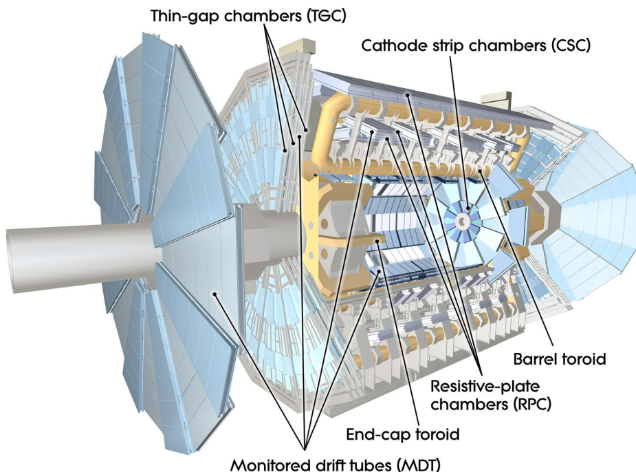
Figure 2.6: The ATLAS muon spectrometer and its components, located outside the ATLAS calorimeter [42].
