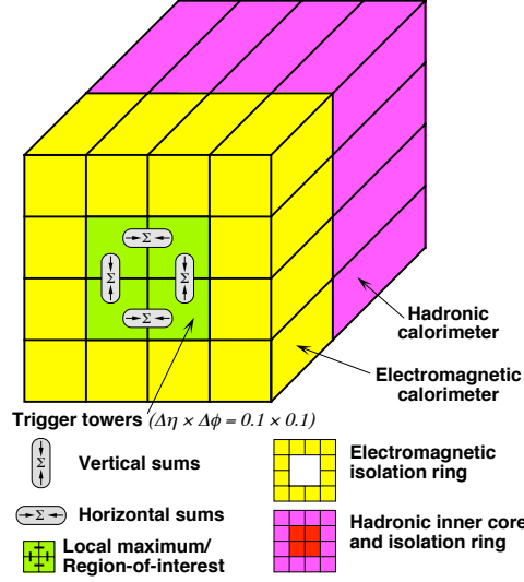
Figure 2.7: Schematic view of the trigger towers used as input to the L1Calo trigger algorithms [44].
