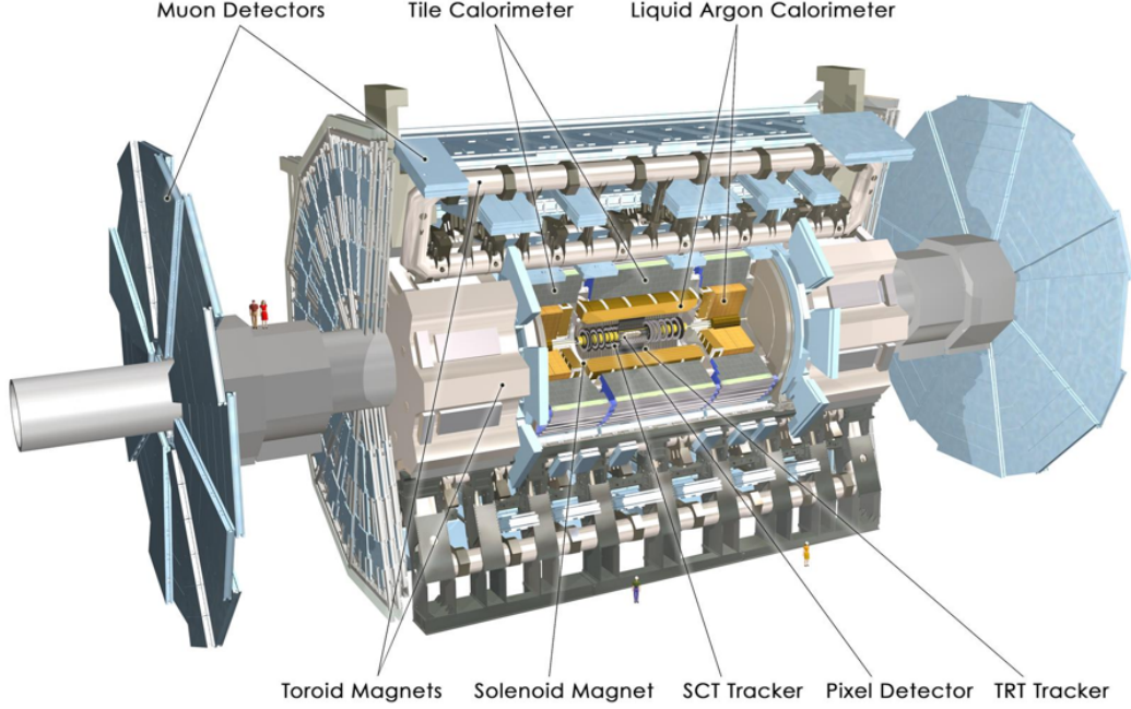
Figure 2.2: ATLAS detector in its entirety. The pixel detector, SCT tracker and TRT tracker make the inner detector which is surrounded by the solenoid magnet. Muon detectors and toroid magnets make the muon spectrometer. The entire calorimeter comprise tile and liquid argon calorimeters [43].
