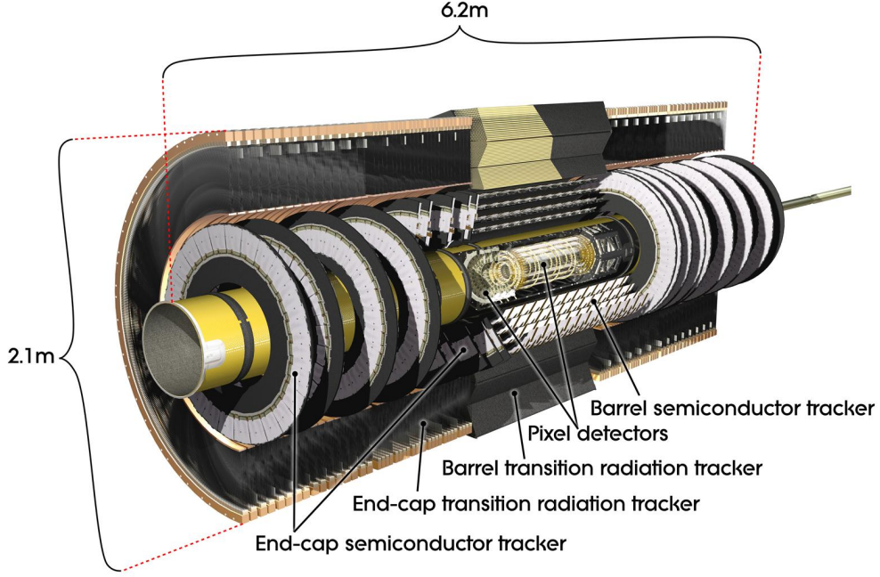
Figure 2.3: Cut-away view of the ATLAS inner detector [42].
