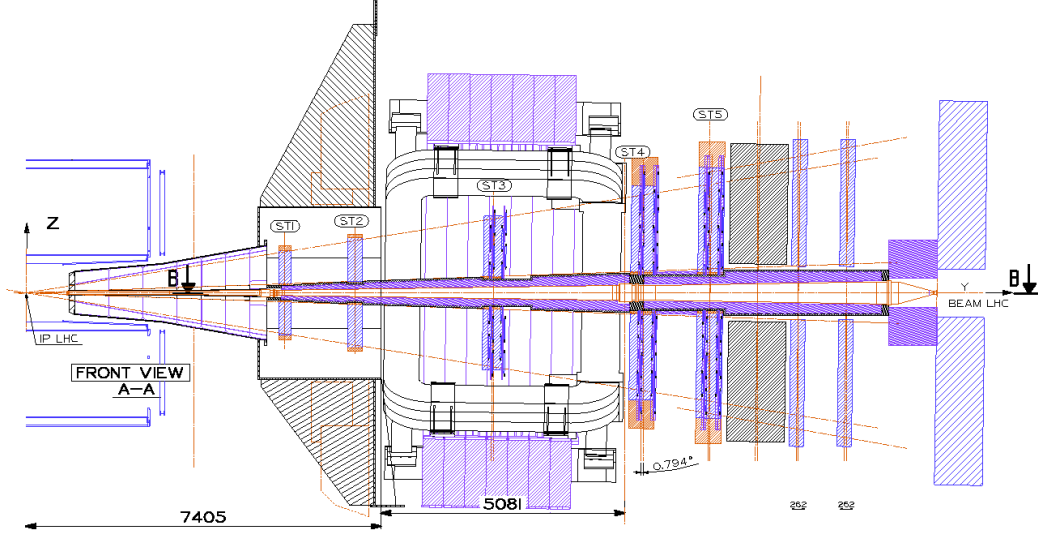
Fig. 2.3 The layout of the muon spectrometer [73].
