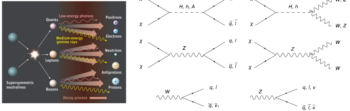
Figure 2.8.: Self-annihilation products of two neutralinos. The annihilation products can be ordinary matter due to the positive R-parity product. Left: Illustration (Credit: Sky & Telescope / Gregg Dinderman). Right: Example Feynman diagrams of neutralino annihilation via supersymmetric scalar Higgs ( h, H ) or pseudoscalar Higgs ( A ) and Z boson into quarks and leptons and bosons. The W and Z bosons on their part decay again into quarks or leptons, as do the heavy fermions, which leads in the end to final products like protons, antiprotons, electrons, positrons, neutrinos and photons.
