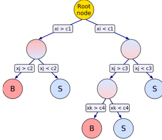
Figure 6.9.: Scheme of a decision tree for signal and background identification. The layout of the branches of the BDT is set up in the training of the BDT, as are the cut values c1, c2, c3, c4 . The x_{i,j,k} represent the input variables. [153]
