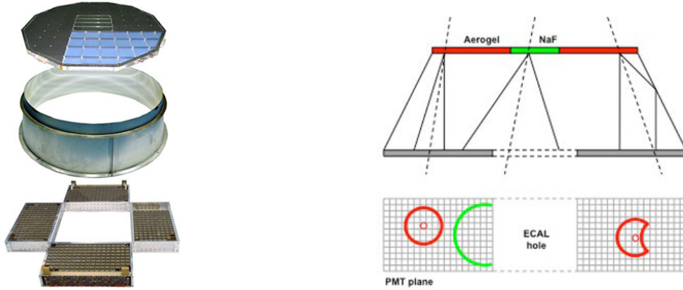
Figure 3.9.: The AMS-02 RICH. On the left the constituents of the RICH before assembly are shown. The top part is the radiator layer, with a change in structure in the middle, where the radiator material changes from aerogel to NaF. Beneath the radiator the conical mirror is shown, which reflects the photons that are emitted with a too large angle to reach the detection layer. At the bottom a preassembly of the PMT layer with the whole for the ECAL is shown. On the right is a demonstration of possible signals in the detector. [121]
