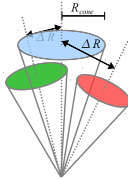
Figure 5.1.: Illustration of the cone radius R_{\text{cone}} for the central object (e.g. jet) and the \Delta R , used for matching, between the central and each of the other two objects (e.g. trigger and MC truth jet).
