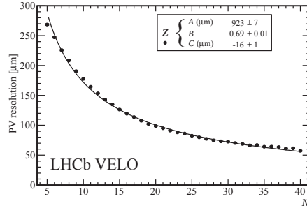
Figure 2.7: Resolution on the reconstructed position of vertices as a function of the number of tracks in the vertex. Figure reproduced from [34].
