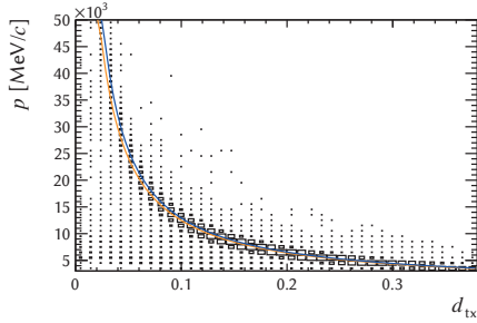
(b) 2D scatter-plot of the momentum of a muon versus its deflection by the magnet. The lines show the parameterisation used in 2011 and 2012 in blue and the one obtained from the fit shown in fig. 3.3c in orange.
