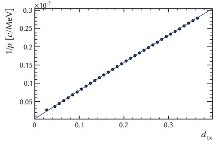
(c) Central values of the peaks fitted to the distribution of the number of muons as a function of 1/p in bins of d_{tx} . A fit of a straight line is shown as the blue line.
