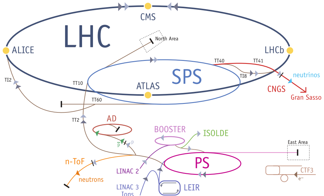
Figure 1.1: CERN accelerator complex, source: Haffner/CERN [Haf 13].
