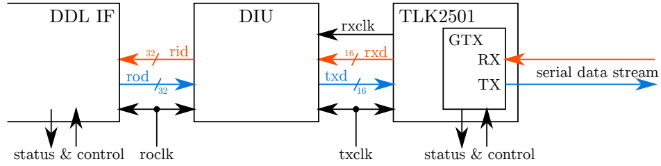
Figure 3.5: DIU integration into the HLT C-RORC firmware.
