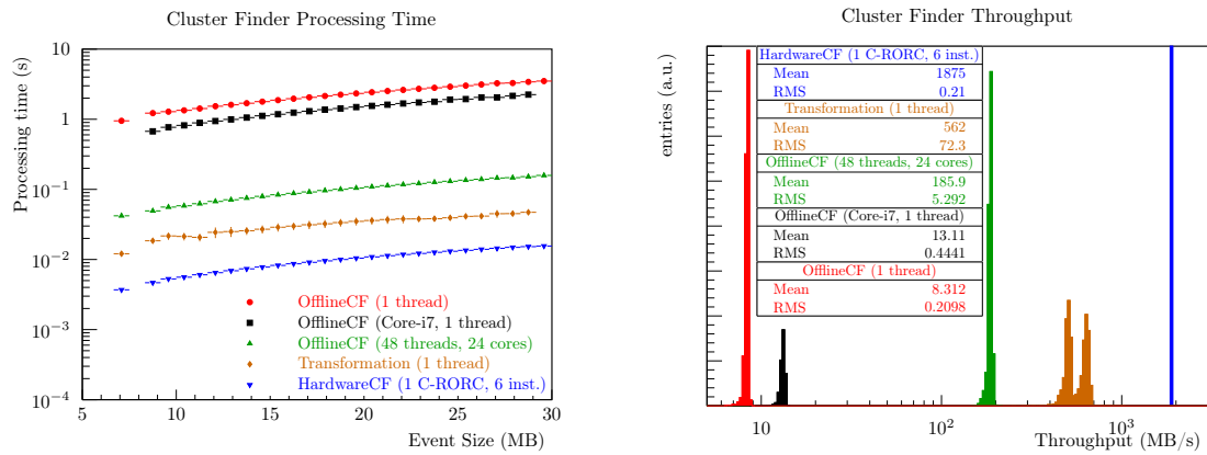
Figure 4.19: Comparison of the computing performance of the hardware cluster finder with different setups of the Offline cluster finder. The same measurements are shown in different ways. Left: Processing time in relation to the event size. Right: Throughput distribution.
