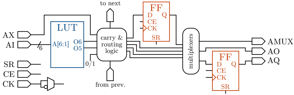
Figure 1.3: Illustration of an FPGA logic block with a 6-input look-up table (LUT) and two flip-flops (FF), similar to the internals of XILINX Virtex-6 Configurable Logic Blocks [Xil 12].
