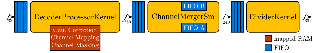
Figure 5.6: Cluster finder partitioning into dataflow kernels.
