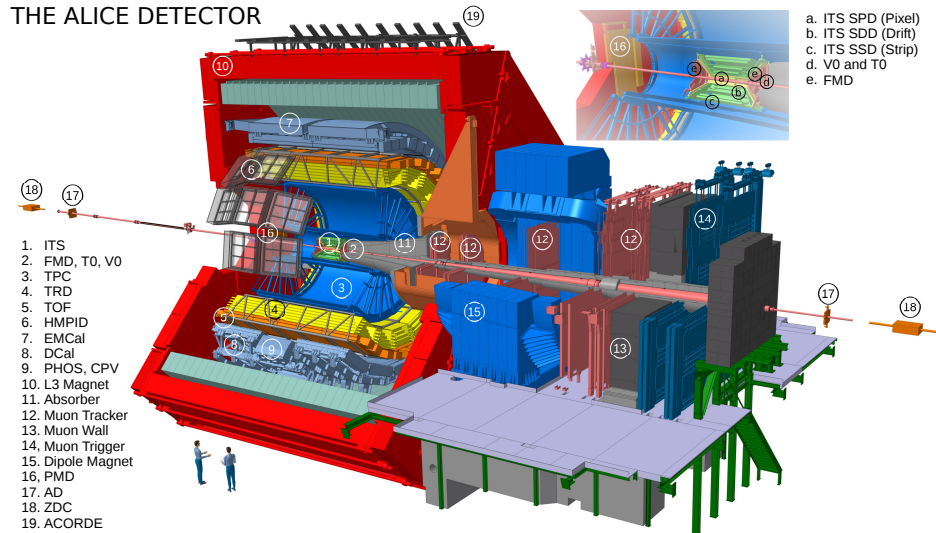
Figure 1.5: ALICE schematics. Source: A. Tauro/CERN [Tau 17].
