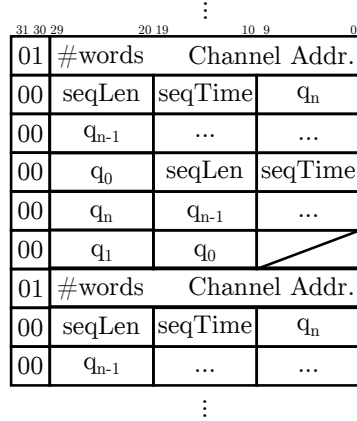
Figure 4.3: Cluster finder input data format. The figure shows a sample temporal sequence of 32 bit data words received via DDL with the TPC specific encoding of bit fields.
