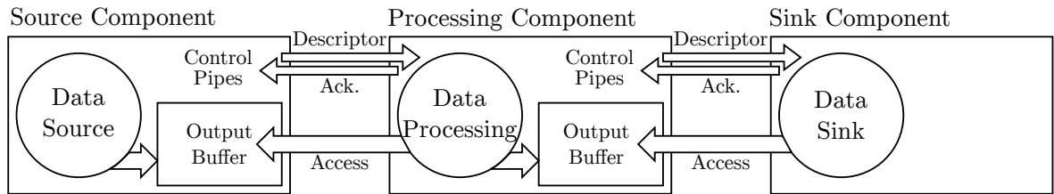
Figure 1.14: Publisher-subscriber model.
