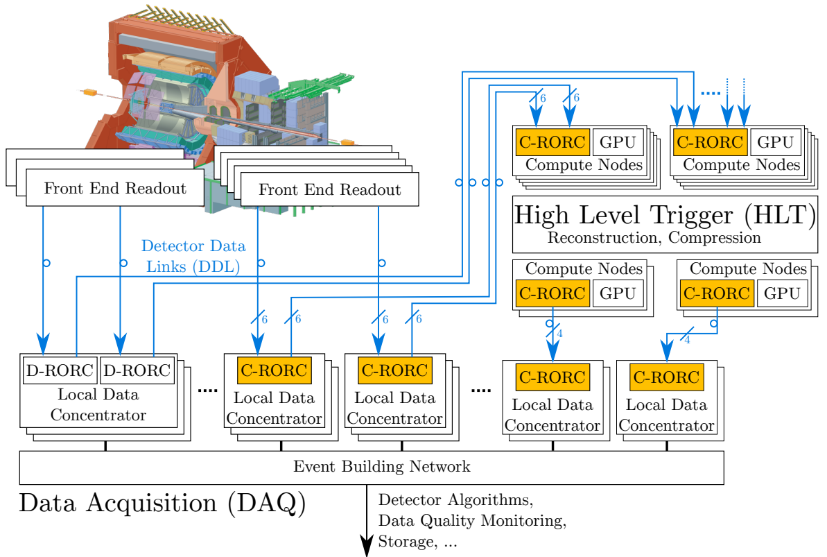
Figure 3.1: ALICE online readout architecture in LHC RUN 2.
