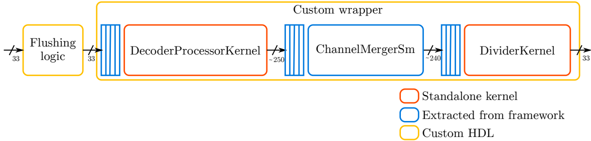
Figure 5.13: Building blocks of the cluster finder implementation using dataflow standalone kernels and framework generated parts.
