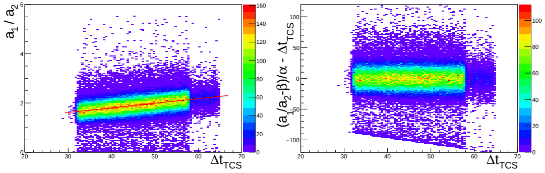
Figure 3.13: Distribution of \frac{a_1}{a_2} with \Delta t_{TCS} (left) and \frac{a_1/a_2 - \beta}{\alpha} (right) for an APV of MP01V1 (strips) for the run 253851 of 2014
