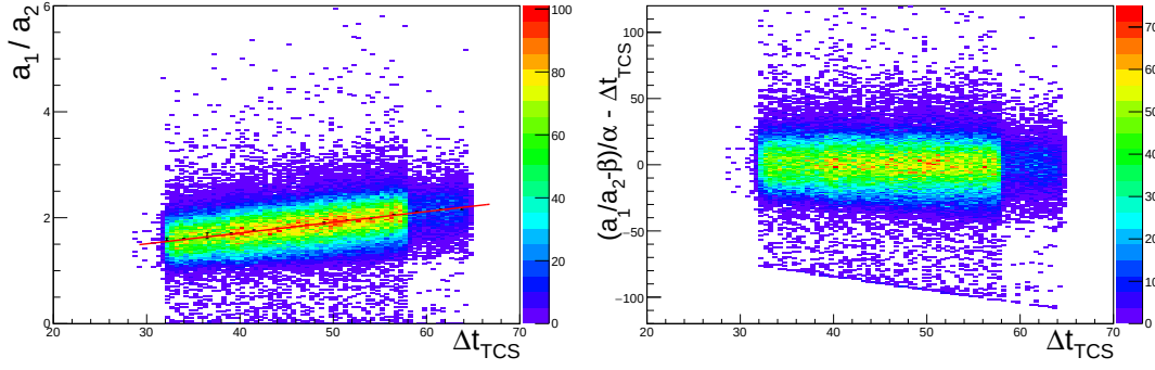
Figure 3.12: Distribution of \frac{a_1}{a_2} with \Delta t_{TCS} (left) and \frac{a_1/a_2 - \beta}{\alpha} (right) for an APV of MP01MV (pixel) for the run 253851 of 2014
