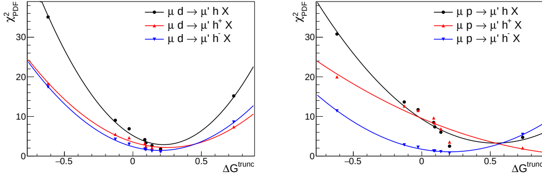
Figure 5.14: Illustration of \chi^2 minimisation to extract \Delta G_{data}^{trunc} based on DSS14 FFs set
