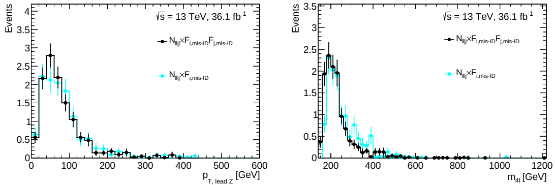
FIGURE 7.12: Data driven background shape as a function of m_{4l} and p_{T, \text{lead } Z} of the Z boson candidate with higher transverse momentum. The real lepton contribution is not subtracted.
