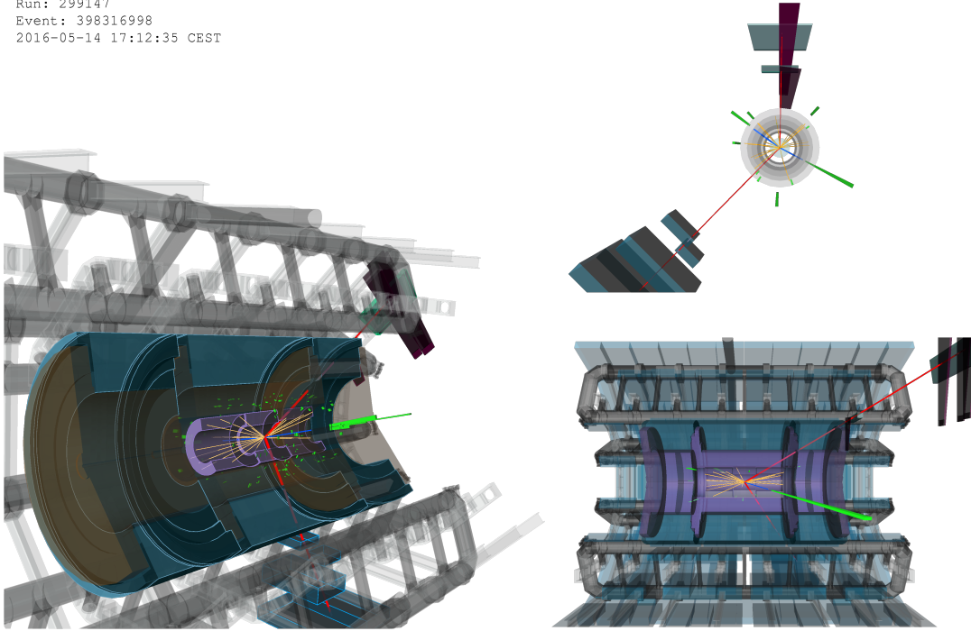
FIGURE C.1: Event display of an event recorded in 2016. The top right panel shows the r - \phi plane and the bottom right panel the z - \eta plane. The energy depositions of the electrons in the calorimeter are visualized in green. The tracks of the electrons are shown in blue and the one of the muons in red. Inner detector tracks with a transverse momentum larger than 2.5 GeV are shown in yellow. The four lepton system has an invariant mass of 209 GeV, a transverse momentum of 31 GeV, and a rapidity of 0.8. The first Z boson candidate is reconstructed from two oppositely charged electrons ( p_T = 67 GeV, \eta = 1.23 and p_T = 12 GeV, \eta = -1.03 ), has a mass of 96 GeV and a transverse momentum of 55 GeV. The other candidate has a mass of 91 GeV, a transverse momentum of 40 GeV and is reconstructed from two oppositely charged muons ( p_T = 36 GeV, \eta = 1.29 and p_T = 56 GeV, \eta = 0.45 ).
