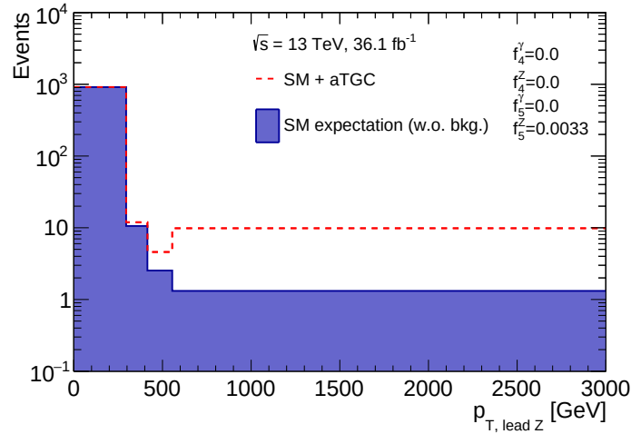
FIGURE 9.4: Comparison of the Standard Model p_{T, \text{lead } Z} distribution with a distribution allowing for aTGCs after binning optimization for highest sensitivity to aTGC effects. The Standard Model expectation is build without background due to its small size. The aTGC configuration is shown as label. The distribution is normalized to the integrated luminosity of 36.1 \text{ fb}^{-1} .
