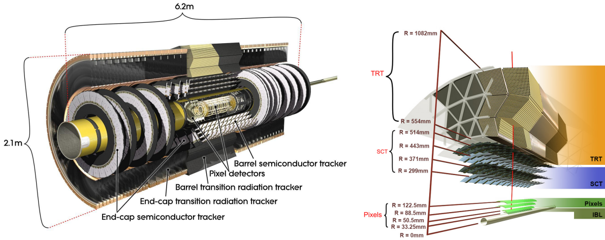
FIGURE 3.3: The left part of the figure, taken from [80], shows a cut-away view of the ATLAS inner detector. The right side, taken from [87], shows the schematic view of the components in the r - \phi plane.
