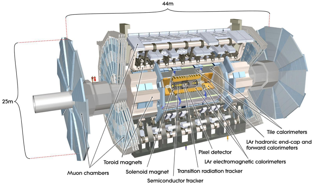
FIGURE 3.2: Cut-away view of the ATLAS experiment. The different components are marked in different colors. It is about 25 m high and 44 m long and weighs 7000 t. The figure is taken from [80].
