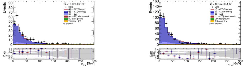
FIGURE 7.30: Comparison between data and expectation as function of the four lepton transverse momentum for the 4e channel (left side) and the 2e2μ channel (right side) using 10 GeV bins. The contributions of the individual parts are stacked on each other. In addition to the q\bar{q} induced prediction from POWHEG also the total prediction using SHERPA is shown. The bottom panels show the ratio between data and expectations, in blue for q\bar{q} induced process using POWHEG and in red using SHERPA. The relative systematic uncertainty is shown as gray band.
