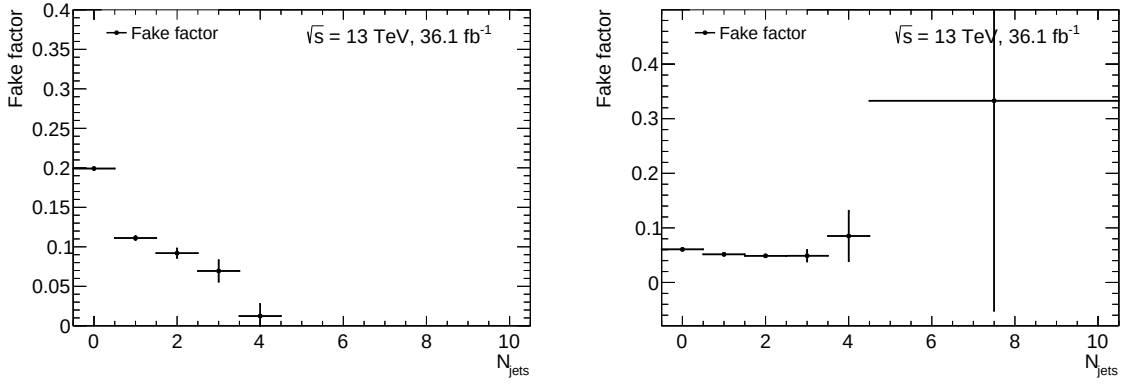
FIGURE 7.9: Fake factor as a function of N_{jets} . The left side shows the distribution for the case when the additional object is reconstructed as a muon and the right side when it is reconstructed as an electron.
