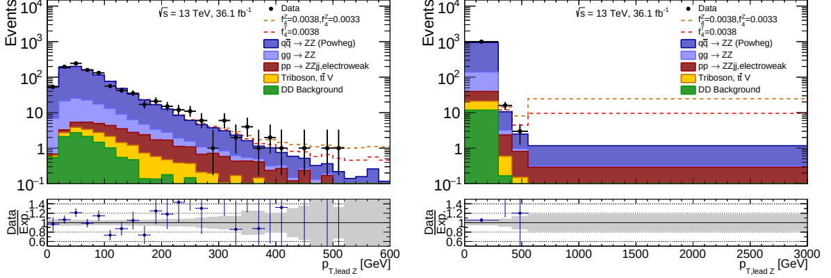
FIGURE 9.5: Data and SM prediction as function of p_{T,lead Z} . Also shown are the signal+SM expectations with f_4^\gamma=0.0038 and f_4^\gamma=0.0038 , f_4^Z=0.0033 . The left hand side shows a fine binning and the right side the optimized binning. The grey band reflects the total systematic uncertainty.
