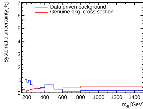
FIGURE 7.23: Relative systematic uncertainties from background related sources as function of the four lepton mass.
