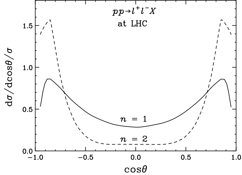
Figure 5.6: Normalized angular distributions for n = 1 (solid) and n = 2 (dashed) string resonances in the DY channel pp \rightarrow \ell^+ \ell^- X with appropriate cuts of Eq. (5.22).
