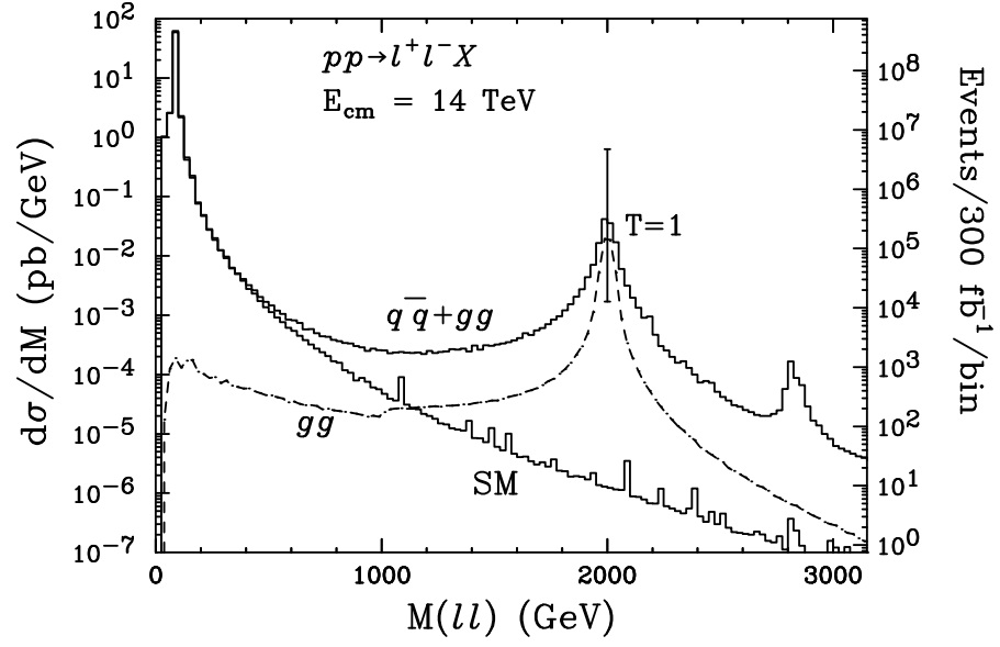
Figure 5.2: Invariant mass distributions for DY dilepton production at the LHC, for the continuum SM expectation and the SR contributions with M_S = 2 \text{ TeV} and T = 1 : q\bar{q} + gg (top curve) and gg only (dashed). The vertical bar at the n = 1 SR peak indicates the enhancement for T = 4 .
