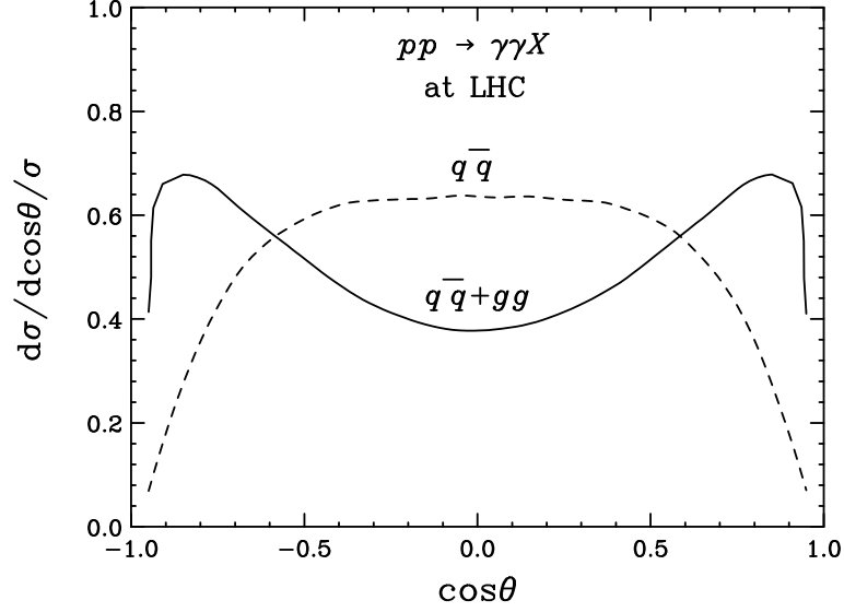
Figure 5.7: Normalized angular distributions for n = 1 string resonance in the diphoton channel pp \rightarrow \gamma\gamma X with appropriate cuts of Eq. (5.22). The solid curve represents the total contribution of q\bar{q} + gg and the dashed curve is for q\bar{q} only.
