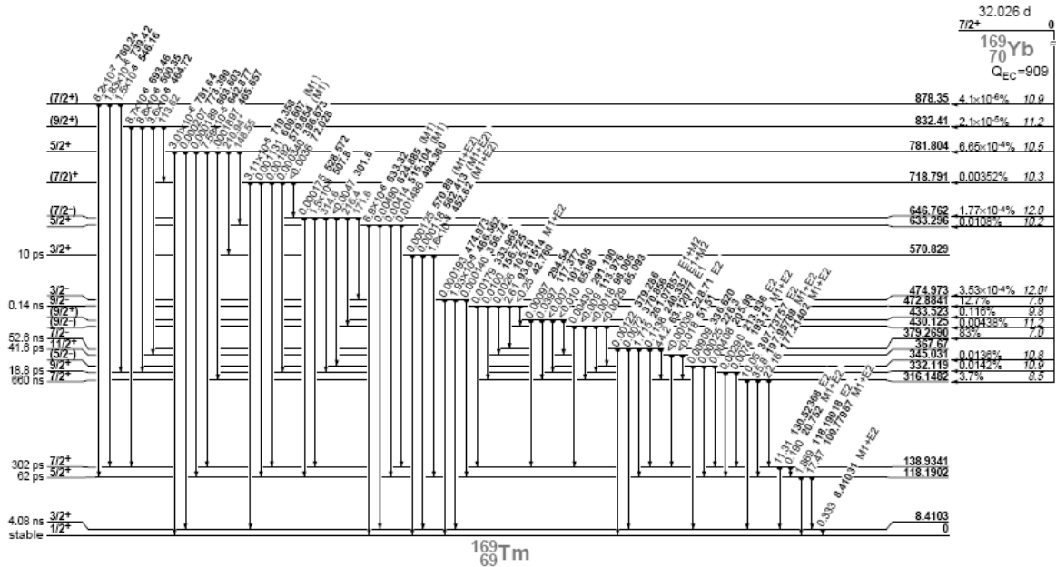
Figure A.8 – ^{169}\text{Yb} decay to ^{169}\text{Tm} by Electronic Capture. The conversion electrons emitted in this decay were used in the EC experiments presented in section 4.3.2.1.
