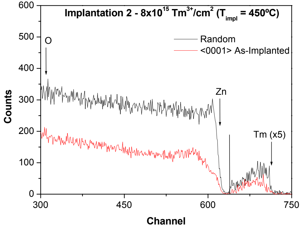
Figure 4.43 – Random and <0001>-aligned RBS spectra for a ZnO single-crystal implanted with 8 \times 10^{15} at/cm 2 of Tm 3+ ions. The Tm signal was once again multiplied by 5.
