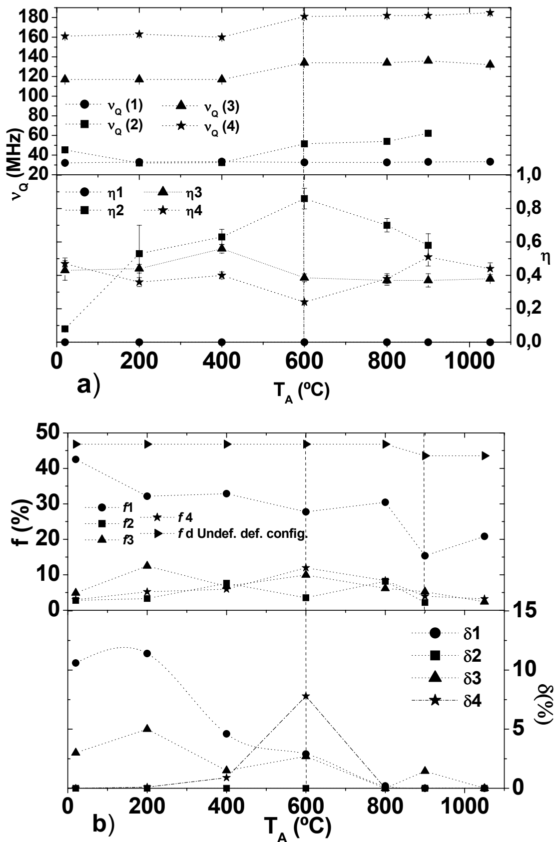
Figure 4.12 – Annealing temperature dependence of a) \nu_Q and \eta and b) of the ^{111}\text{Ag} fractions f and attenuation \delta . Above 900°C, the quoted fractions were equally normalized to account for 23% of ^{111}\text{Ag} out-diffusion, except for f_5 , as from this fraction only 7% out-diffused.
