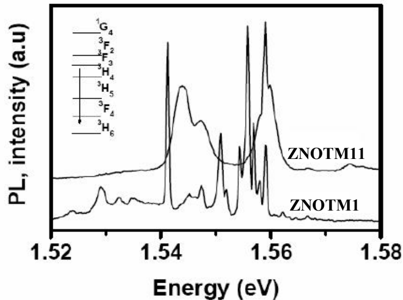
Figure 4.48 – 13K Tm-related PL spectra observed for samples implanted at (a) RT (ZNOTM1) and (b) 450°C (ZNOTM11), with 5 \times 10^{15} \text{ Tm}^{3+}/\text{cm}^2 . Both samples were air annealed at 800°C.
