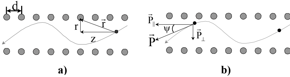
Figure 2.10 – a) A particle travels in between two rows of atoms with periodicity d , being channeled through small scattering angle collisions. In b) the particle motion is decomposed in a longitudinal term and a transverse term.
