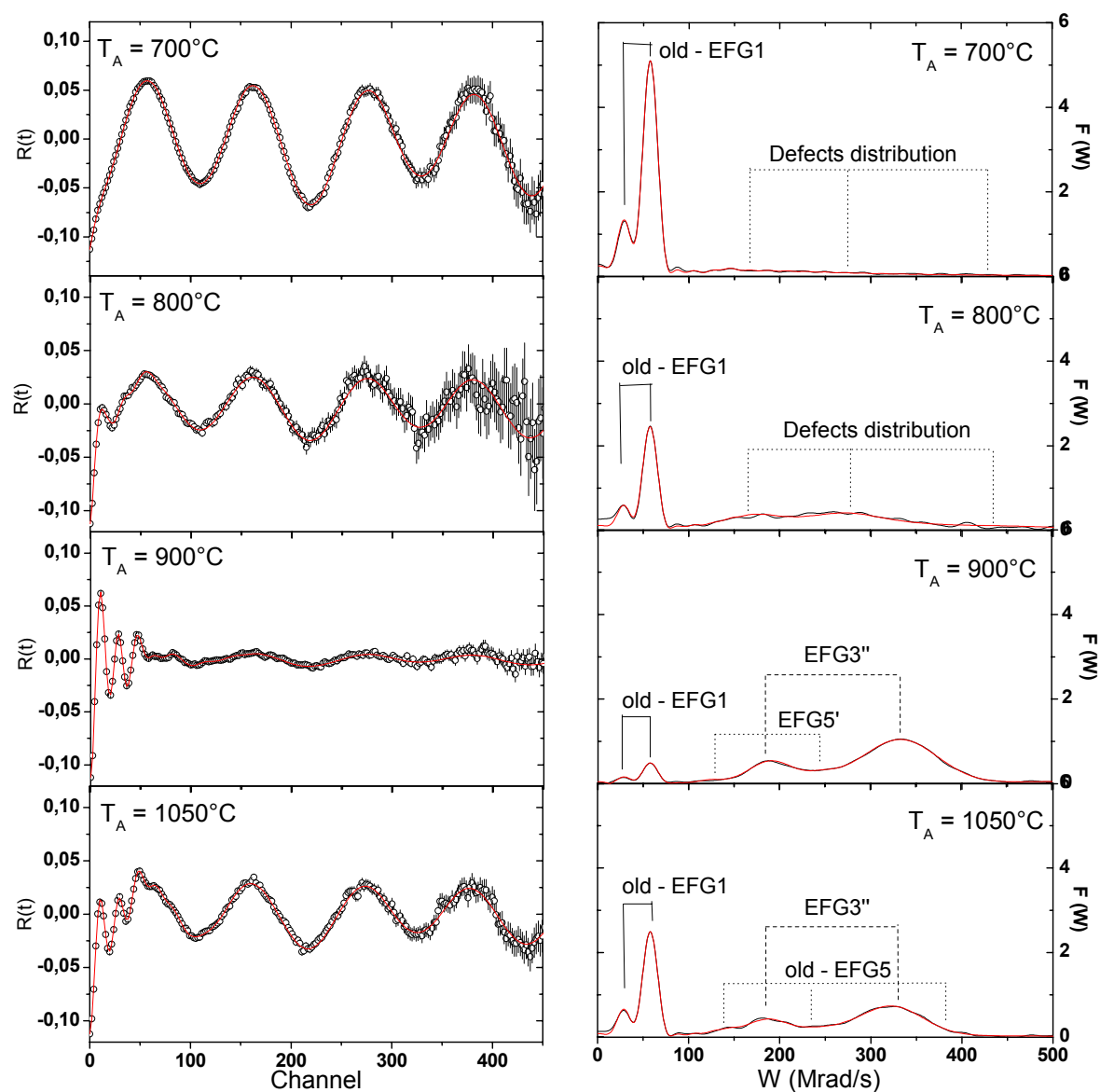
Figure 4.20 – ^{111}\text{In} R(t) and FFT functions obtained for sample E-C5 (Crystal 2 - co-implanted with 1 \times 10^{14} at/cm 2 of stable As) for the (A) as-implanted state and after the 200°C, 400°C, 600°C, (B) 700°C, 800°C, 900°C and 1050°C 30 min vacuum annealing steps. The red solid line represents the functions that best fitted the experimental data. All measurements were carried out at room temperature.
