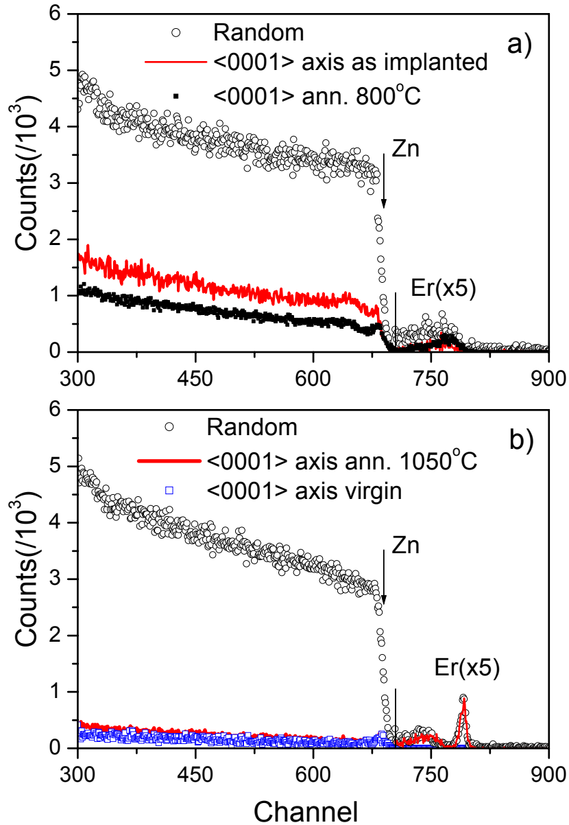
Figure 4.29 – Random and <0001>-aligned RBS spectra of a ZnO single-crystal implanted with 5 \times 10^{15} \text{Er}^+/\text{cm}^2 (sample ZNOER1) for a) the as-implanted state and after a 800°C 30 min air annealing. Figure b) represents the spectra following the 1050°C annealing, from which the lattice recovery and Er surface segregation are evident. In both graphs the Er profile was 5x magnified.
