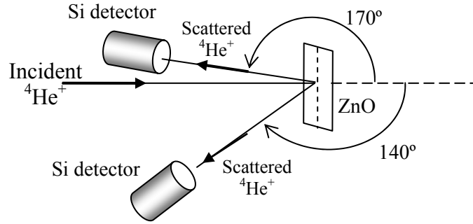
Figure 2.5 – Geometrical arrangement used in the RBS experiments (IBM geometry) where two surface barrier silicon detectors are placed at 140° and 170° with respect to the incident beam direction. The ZnO samples were mounted in a computer controlled two-axis goniometer that allowed the sample orientation relatively to the incident beam.
