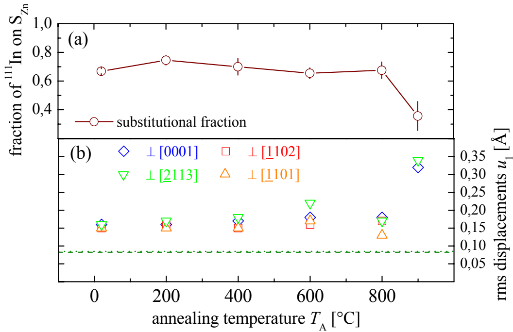
Figure 4.24 – ^{111}\text{In} lattice site location results for sample E-C6 from Crystal 2 (co-implanted with 1 \times 10^{14} at/ \text{cm}^2 of stable As). (a) Fraction of ^{111}\text{In} atoms at S_{\text{Zn}} sites and (b) their rms displacements u_1 perpendicular to the four symmetry crystalline directions as a function of 10 min vacuum annealing steps. The dash and dotted lines represent the thermal vibration amplitudes of the Zn and O atoms, respectively.
