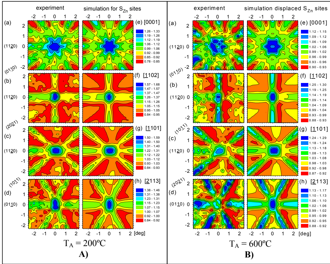
Figure 4.7 – \beta^- emission channeling patterns from ^{67}\text{Cu} implanted on a ZnO single-crystal around the four symmetry directions [0001], [1102], [1101] and [2113] (patterns (a) - (d)), following the A) 200°C and the B) 600°C 10 min vacuum annealing steps. The corresponding theoretical patterns that best fitted the experimental ones are also presented (patterns (e) - (h)).
