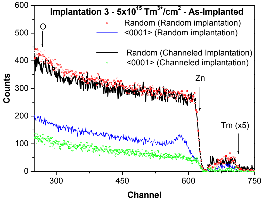
Figure 4.44 – RBS spectra for random and <0001>-aligned implantations of two ZnO single-crystals implanted with 5 \times 10^{15} at/cm 2 of Tm 3+ ions. The Tm signal was multiplied by 5.
