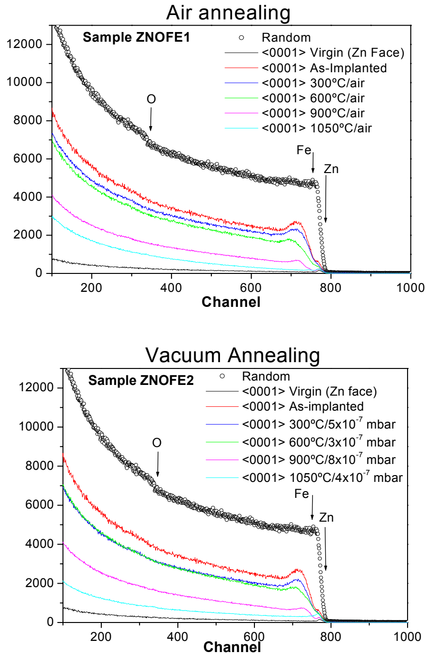
Figure 4.1 – Random and \langle 0001 \rangle -aligned RBS spectra of a ZnO single-crystal implanted with 1 \times 10^{16} \text{ }^{57}\text{Fe}/\text{cm}^2 for the as-implanted state and following 30 min annealing steps at 300°C, 600°C, 900°C and 1050°C in air (Sample ZNOFE1) or in vacuum (sample ZNOFE2).
