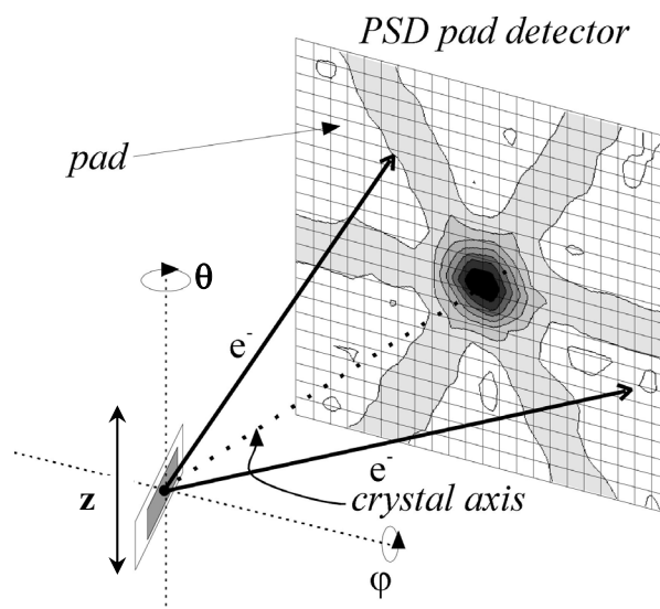
Figure 2.11 – Representation of the degrees of freedom of the emission channeling goniometer. A typical 2D – pattern acquired with a position sensitive (PSD) detector is also depicted.
