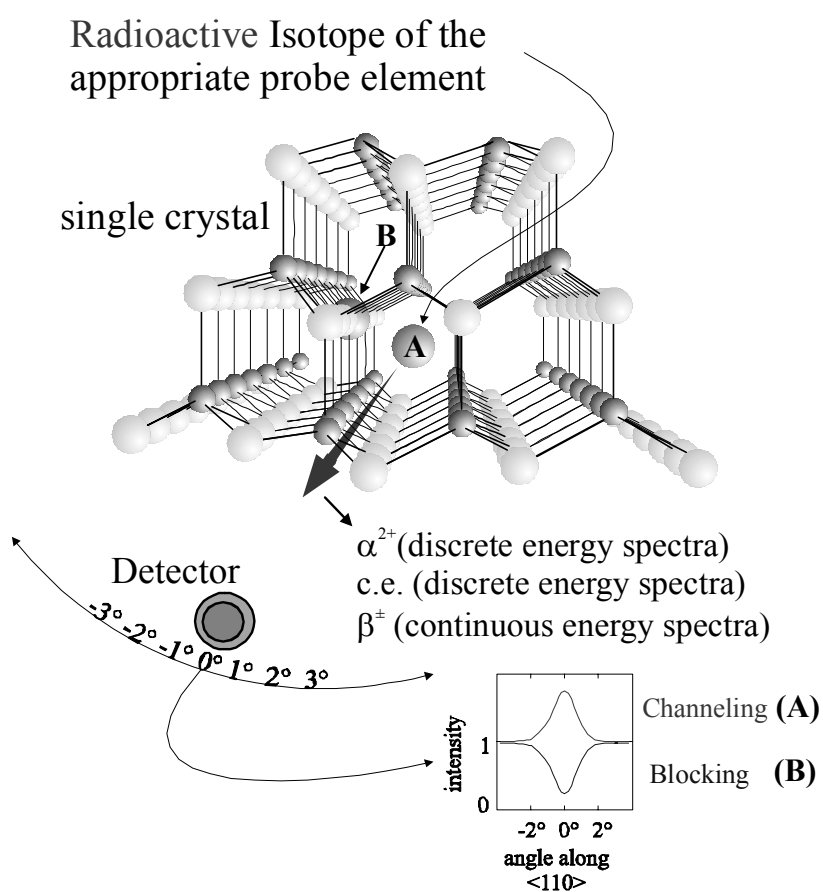
Figure 2.9 – Emission Channeling basic principle. After implantation, the radioactive probe isotope sits in a preferred lattice site of the single-crystal. The particles emitted in the radioactive decay are then guided by the lattice potentials in their way out of the crystal. By means of a particle detector, the angular distribution of the emitted particles is measured around a given crystallographic direction. Depending on where the probe sits and on the particles nature different effects are observed: Channeling (probe at position A) or Blocking (probe at position B).
