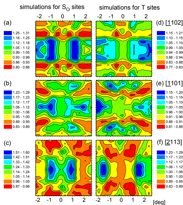
Figure 4.14 – Theoretical emission channelling patterns for 100% of emitter atoms located at substitutional S_O sites (patterns (a)-(c)) and 100% on tetrahedral T sites (patterns (d)-(f)). Notice that no patterns are depicted for [0001] because these sites cannot be distinguished along this direction (they are identical to the patterns for S_{Zn} ).
