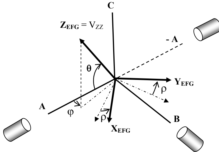
Figure 2.18 – Definition of the EFG system axis ( X_{\text{EFG}} , Y_{\text{EFG}} , Z_{\text{EFG}} ) relatively to the lab system (A, B, C) through angles theta ( \theta ), phi ( \phi ) and rho ( \rho ). Here, a three-detector setup is represented since these angle definitions are used in the data fitting software NNFIT (section 2.4.3), which is based in setups with this configuration. Refer to the text for a detailed explanation of the angles.
