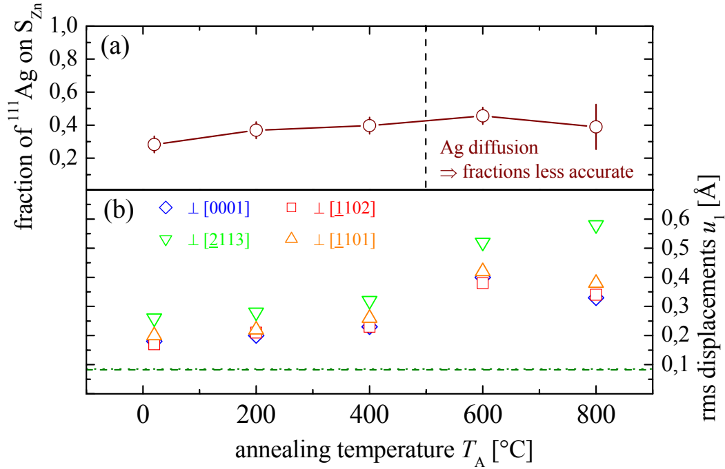
Figure 4.10 – (a) Fraction of ^{111}\text{Ag} atoms at S_{\text{Zn}} sites and (b) their rms displacements u_{\perp} perpendicular to the four symmetry crystal directions as a function of 10 min vacuum annealing steps. The dashed and dotted lines represent the room temperature Zn and O vibration amplitudes, respectively.
