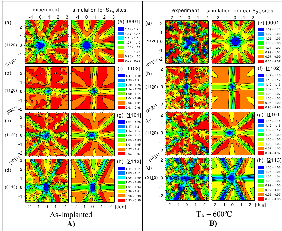
Figure 4.9 – Angular distributions of the \beta -particles emitted from ^{111}\text{Ag} in ZnO around the four symmetry directions [0001], [1102], [1101] and [2113] (patterns (a) - (d)), for the A) as-implanted state and B) following the a 600^\circ\text{C} 10 min vacuum annealing. The corresponding theoretical patterns that best fitted the experimental ones are also presented (patterns (e) - (h)).
