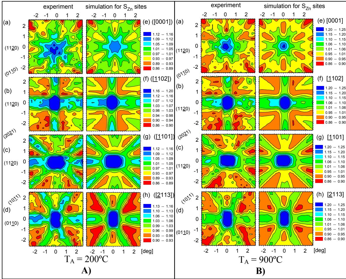
Figure 4.3 – \beta^- emission channeling patterns from ^{45}\text{Ca} implanted on a ZnO single-crystal around the four symmetry directions [0001] , [1102] , [1101] and [2113] (patterns (a) - (d)), following the A) 200°C and the B) 900°C 10 min vacuum annealing steps. The corresponding theoretical patterns that best fitted the experimental ones are also presented (patterns (e) - (h)).
