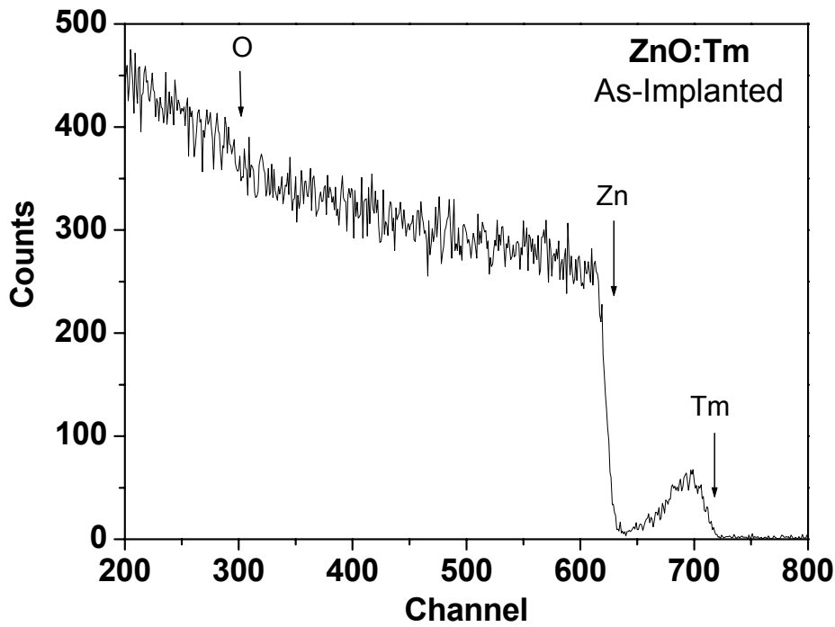
Figure 2.7 – Random RBS spectrum for a ZnO single-crystal implanted with 5 \times 10^{16} \text{ at/cm}^2 of Tm ions. The Tm signal is easily distinguished since it has a higher mass than Zn and O.
