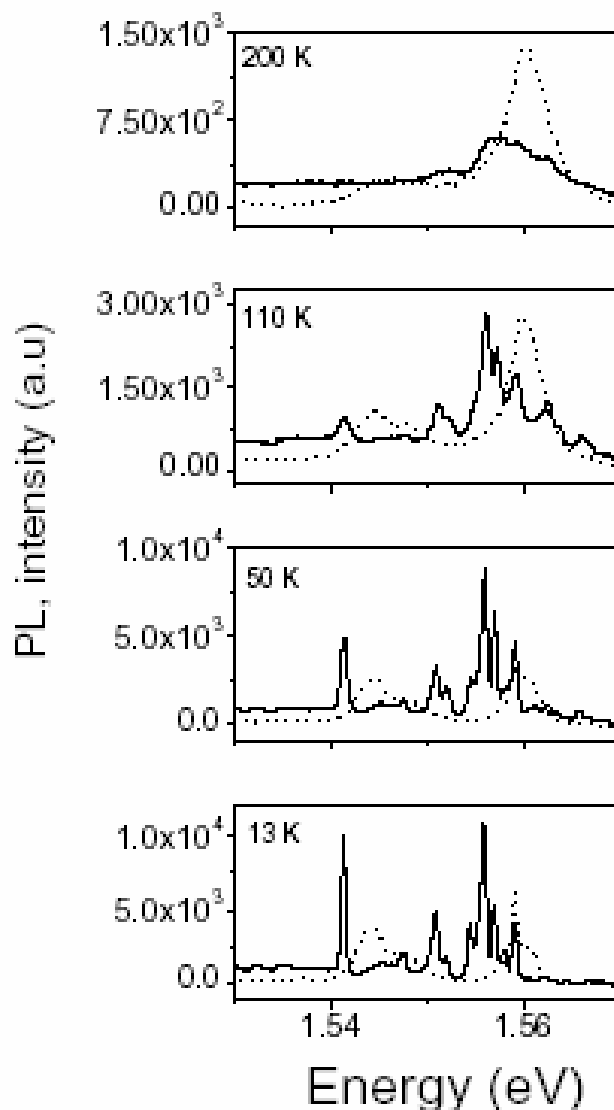
Figure 4.50 – Temperature dependence of PL spectra for samples ZNOTM1 (full line) and ZNOTM11 (dashed line) implanted at RT and 450°C, respectively, with 5 \times 10^{15} \text{ Tm}^{3+}/\text{cm}^2 and annealed at 800°C/air/30 min. [49].
