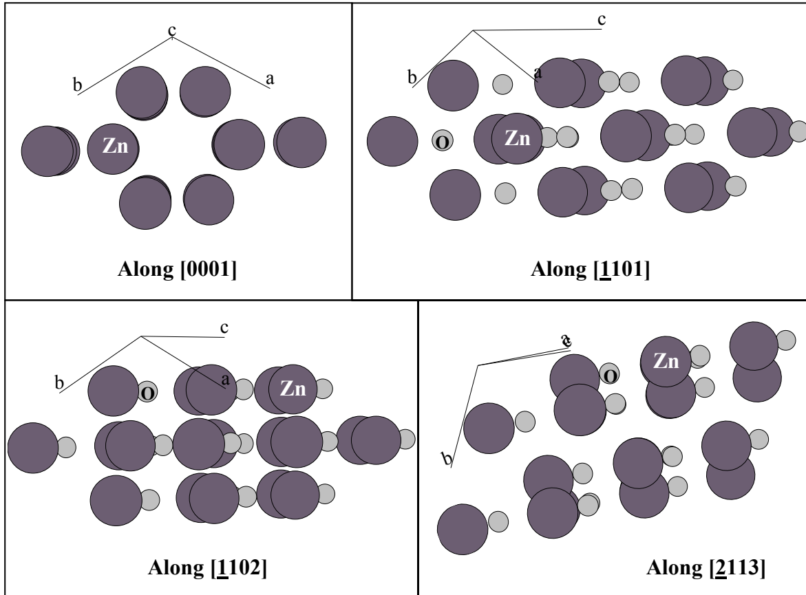
Figure 1.2 – Projections along the main symmetry crystallographic directions of ZnO ( [0001] , [1102] , [1101] and [2113] ). These directions were used in the experiments presented in Chapter 4, particularly for the Emission Channelling technique.
