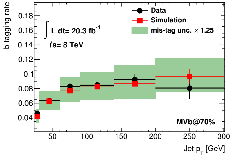
Figure 8.13: The b -tagging rates for the MVb algorithm corresponding to an operating point of an overall efficiency of 70% displayed as a function of the transverse momentum of the jets that are associated to the hadronic W -boson decays in fully reconstructed t\bar{t} single lepton candidate events. In order to be considered, the events are required to have both the b -jet candidates on the hadronic and the leptonic side of the event b -tagged using the MV1 algorithm. The b -tagging rates are shown for the predictions by the simulation (as red lines) and the measurements in data (as black dots). In addition, the mis-tagging uncertainties for c -jets corresponding to the MV1 algorithm (as measured by the D^* method) and increased by 25% are presented (as a green filled area).
