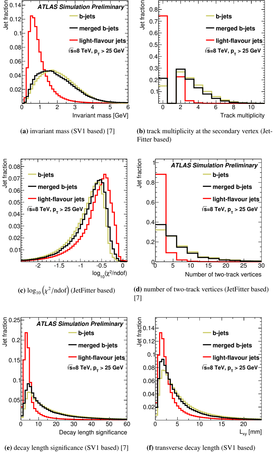
Figure 6.9: Distributions of the invariant mass (a), the track multiplicity at the secondary vertex (b), the \log_{10}(\chi^2/\text{n dof}) (c), the number of two-track vertices (d), the decay length significance (e) and the transverse decay length (f) are presented for the inclusive b - (yellow), merged b - (black) and light-flavour jets (red). Each distribution is individually normalised to unit area. The considered jets stem from simulated t\bar{t} decays that are generated with \sqrt{s} = 8 TeV and have p_T > 25 GeV and |\eta| < 2.5 .
