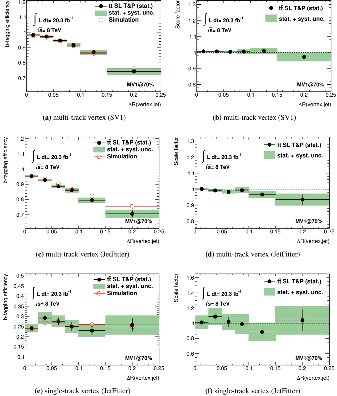
Figure 8.18: Results of the b -tagging efficiency measurements for the MV1 algorithm corresponding to an operating point of 70% efficiency as a function of the angular separation between the vertex direction and the jet axis \Delta R(\text{vertex}, \text{jet}) . The measurement is performed separately for jets having a vertex reconstructed with the iterative vertex finder (a-b) and the JetFitter algorithm (c-f), where the vertex candidates based on the JetFitter are subdivided into single- and mutitrack-vertices. The b -tagging efficiencies (left column) are shown for the predictions by the simulation (as a red line) and the measurements in data by the tag and probe (T&P) method (as black dots). The total uncertainties of these measurements are displayed as well (by the green filled area). The uncertainties on the predicted tagging efficiencies are based only on the Monte Carlo statistics. The corresponding data-to-simulation scale factors are presented in addition (right column). As these measurements take only jets into account that have an appropriate type of secondary vertex reconstructed, the definition of the presented b -tagging efficiencies is not inclusive as in the measurements corresponding to the jet p_T , \eta or \Delta R^{\min} .
