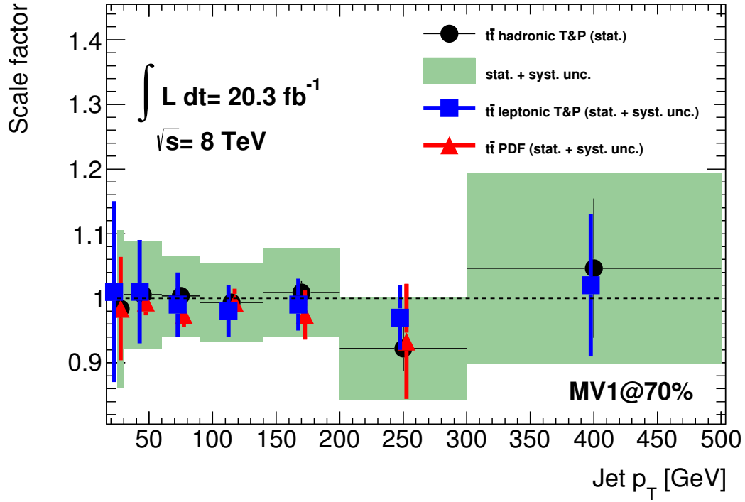
Figure 8.19: Data-to-simulation scale factors for the MV1 algorithm evaluated at an operating point that matches an overall b -tagging efficiency of 70%. The results of the tag and probe method (T&P) applied to t\bar{t} candidate decays into a final state of a single lepton (SL), at least four jets and missing transverse momentum are compared to the scale factors that are obtained with the combinatorial likelihood (PDF) method applied to t\bar{t} dilepton events containing exactly two or three jets (presented as red triangles). The results of the tag and probe method (T&P) are displayed for the case that the b -jet candidates on the hadronic side of the selected events are used as the probe jets (shown as black dots) and also for the case that the b -jet candidates on the leptonic side are used (blue squares).
