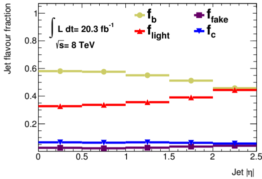
(b) Flavour fractions as a function of the jet |\eta|
