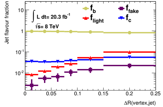
(c) multi-track vertices based on SV1
