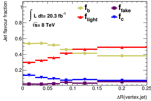
(a) single-track vertices based on JetFitter
