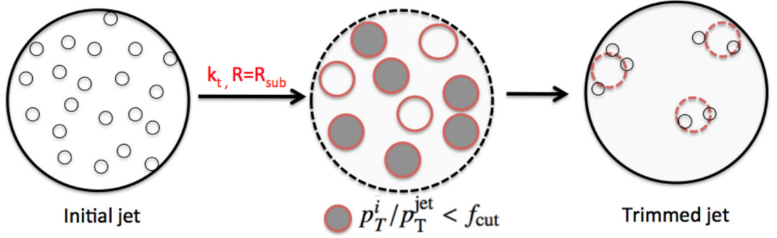
Figure 3.10: Schematic view of the jet trimming procedure [91] in case of the use of subjets. The trimming algorithm takes a jet as input and re-clusters its components into k_T subjets. In the last step all subjets are discarded that have p_T^{\text{subjet}}/p_T^{\text{jet}} < f_{\text{cut}} .
