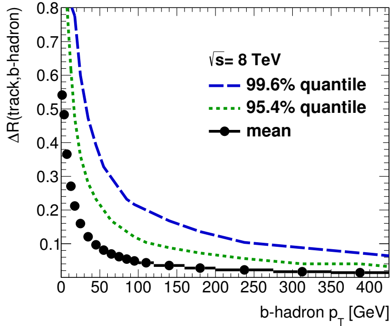
Figure 7.1: Average angular separation between a b -hadron and the tracks corresponding to its decay products \langle \Delta R(\text{track}, b - \text{hadron}) \rangle presented as a function of the b -hadron p_T (as black markers). In addition, the two quantiles corresponding to 95.4% (green dashed line) and 99.6% (blue dashed line) of all tracks matched to the studied b -hadrons are shown as well. The simulated b -hadron decays stem from a sample of SM t\bar{t} decays, which is produced with the POWHEG and PYTHIA generators.
