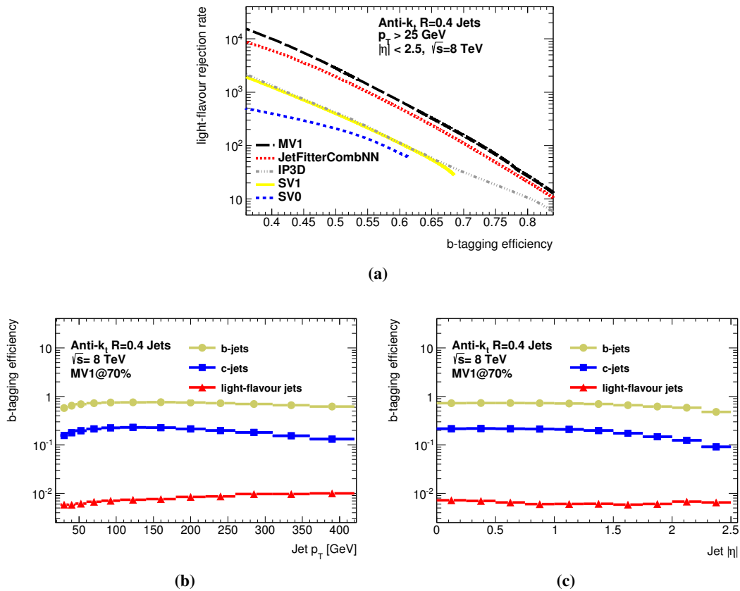
Figure 4.4: The light-flavour rejection rate as a function of the b -tagging efficiency for different b -taggers available at ATLAS (a). The jets are extracted from a t\bar{t} sample that is simulated using the POWHEG and PYTHIA generators. As it can be seen, the MV1 tagger shows the best rejection power for light-flavour jets. Its tagging efficiencies for b -, c - and light-flavour jets are presented as well as a function of the jet p_T (b) and |\eta| (c) for a representative working point corresponding to an overall b -tagging efficiency of 70%.
