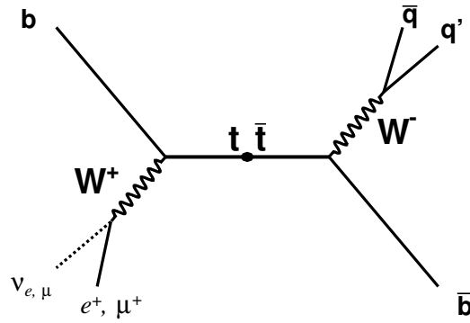
Figure 5.1: Schematic view of a single lepton t\bar{t} decay at parton level (i.e. a decay into a final state with one charged lepton, one neutrino, two b -quarks and two additional quarks from the hadronic decay of a W -boson).
