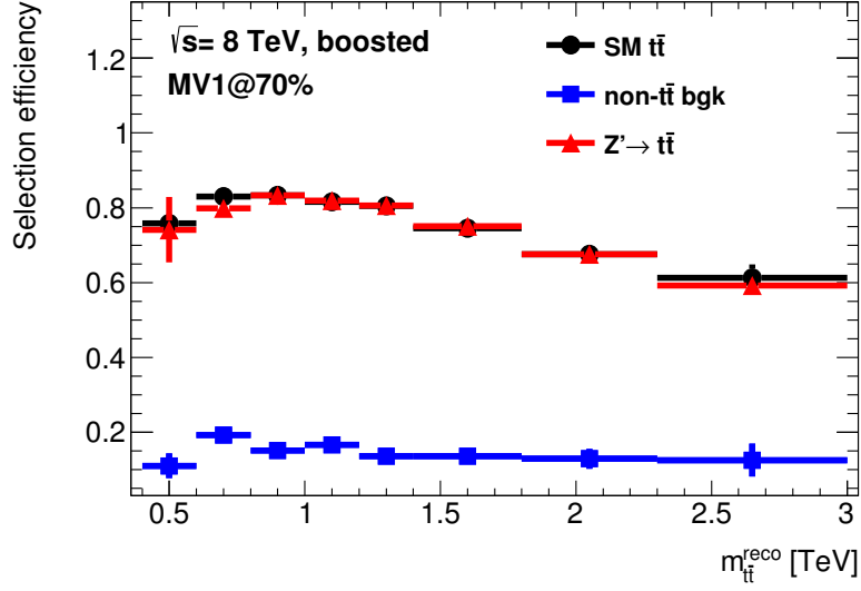
(a) Selection efficiencies based on MV1
