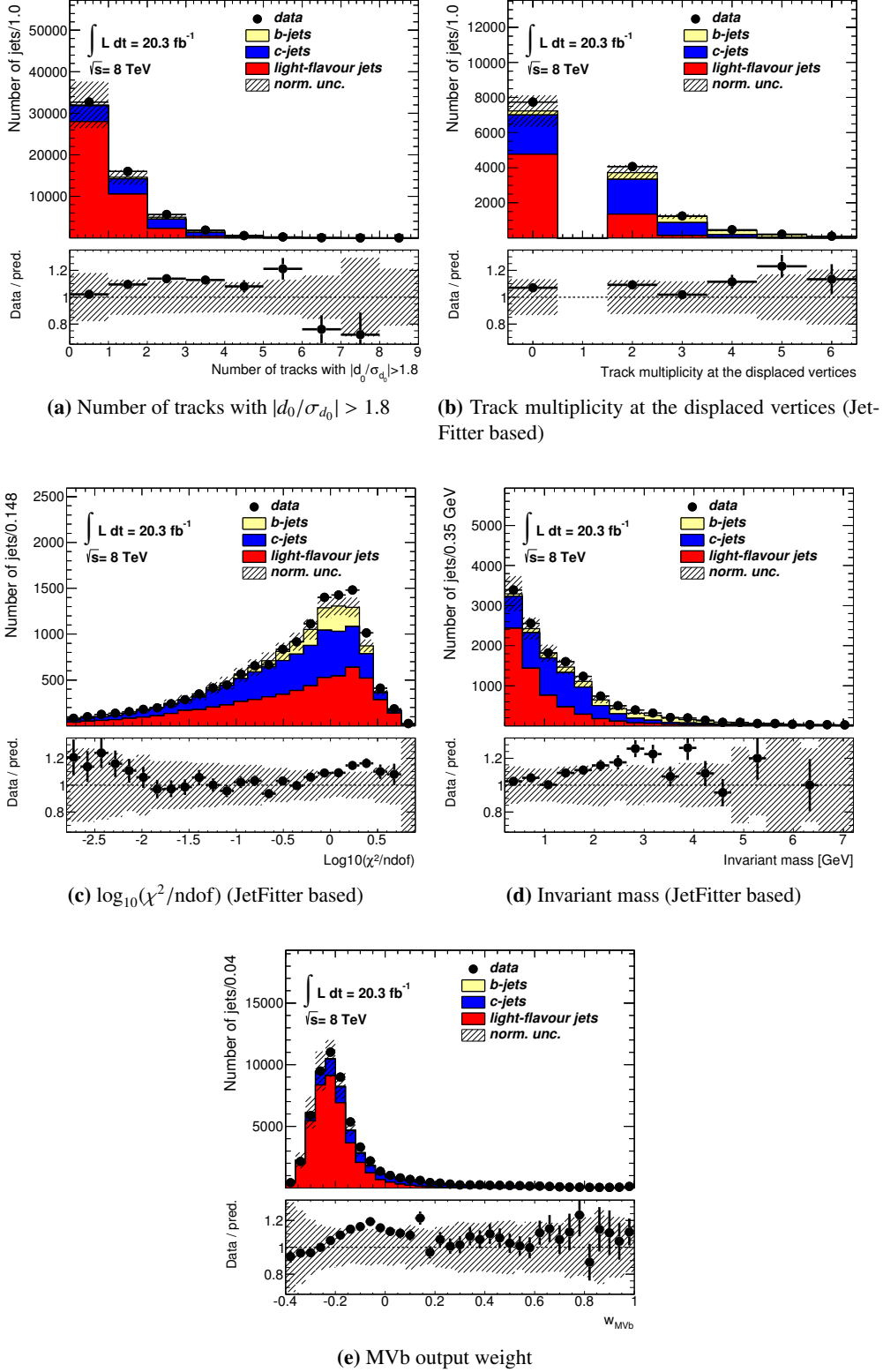
Figure 8.7: Distribution of several input quantities of the MVb and MVbCharm tagger (a-d) as well as the MVb output weight (e) for jets contained in the charm and light-flavour jet control region. The predictions by the simulation are subdivided into the three different jet flavour types. The simulated Monte Carlo samples are normalised according to their predicted cross-sections to an integrated luminosity of 20.3 \text{ fb}^{-1} . In addition, ratios of the data and the simulation are shown at the bottom of each plot.
