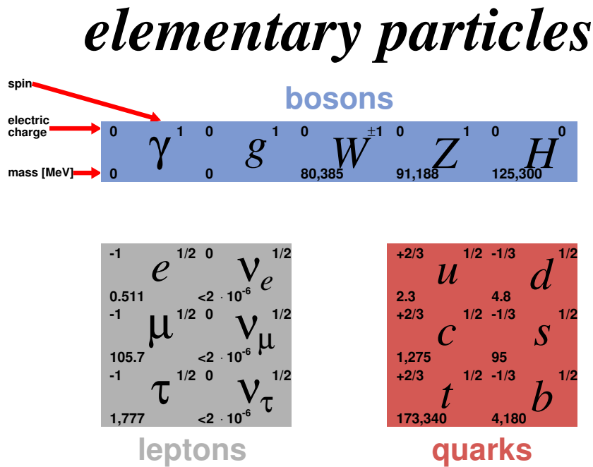
Figure 2.1: Elementary particles described by the SM displayed together with a subset of their properties including the spin, the electric charge (in units of the elementary charge) and the mass (in MeV) [12].
