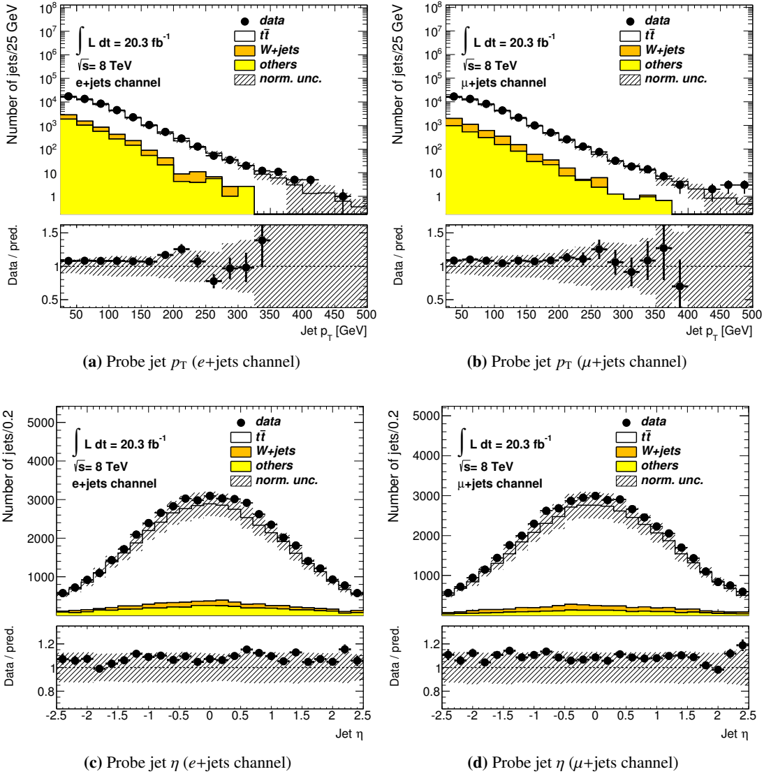
Figure 8.4: Distribution of the transverse momentum (a-b) and the pseudorapidities (c-d) of the selected probe jets displayed separately for the electron plus jets (left column) and muon plus jets (right column) channel. The simulated Monte Carlo samples are normalised according to their predicted cross-sections to an integrated luminosity of 20.3 \text{ fb}^{-1} . Data-to-simulation ratios are shown at the bottom of each plot.
