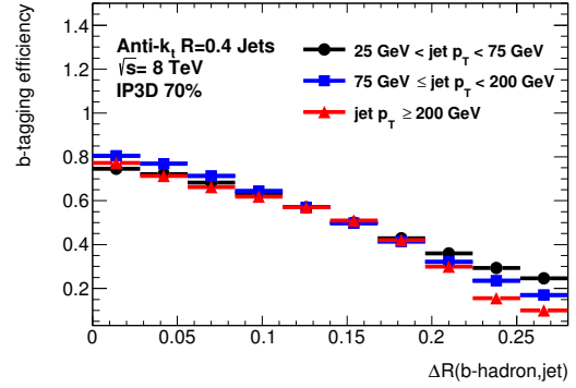
(c) Impact parameter based tagger (IP3D)
