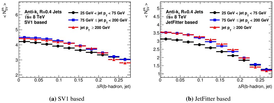
Figure 6.5: Average number of tracks associated to the secondary vertex candidates as a function of the angular separation between the jet axis and the b -hadron flight direction for vertices reconstructed with the iterative vertex finder using the SV1 setup (a) and the JetFitter algorithm (b). These properties are investigated for selected b -jets that are obtained from SM t\bar{t} decays, which are simulated using the POWHEG and PYTHIA generators. Jets are classified into three different p_T regions and studied separately.
