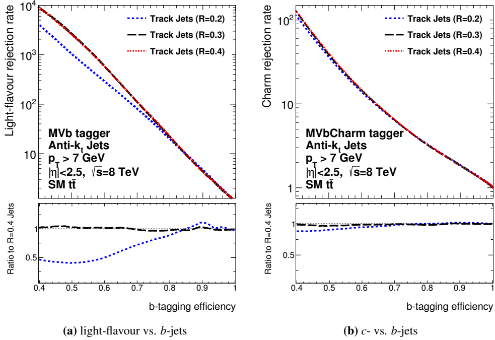
Figure 7.5: Light-flavour (a) and charm (b) rejection rates as a function of the b -tagging efficiency corresponding to the MVb (a) and MVbCharm (b) algorithms for the three different track jet collections. All considered track based jets stem from a sample of simulated SM t\bar{t} events that are generated using POWHEG and PYTHIA. The performance curves corresponding to the R = 0.2 track based jets are displayed as a blue line, while the R = 0.3 and R = 0.4 track based jets are represented by a black and a red line, respectively.
