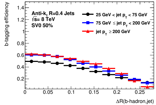
(e) Secondary vertex based tagger (SV0)
