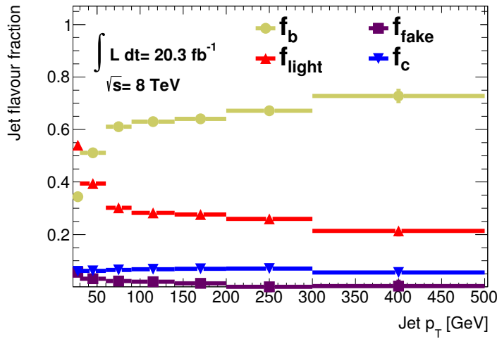
(a) Flavour fractions as a function of the jet p_T
