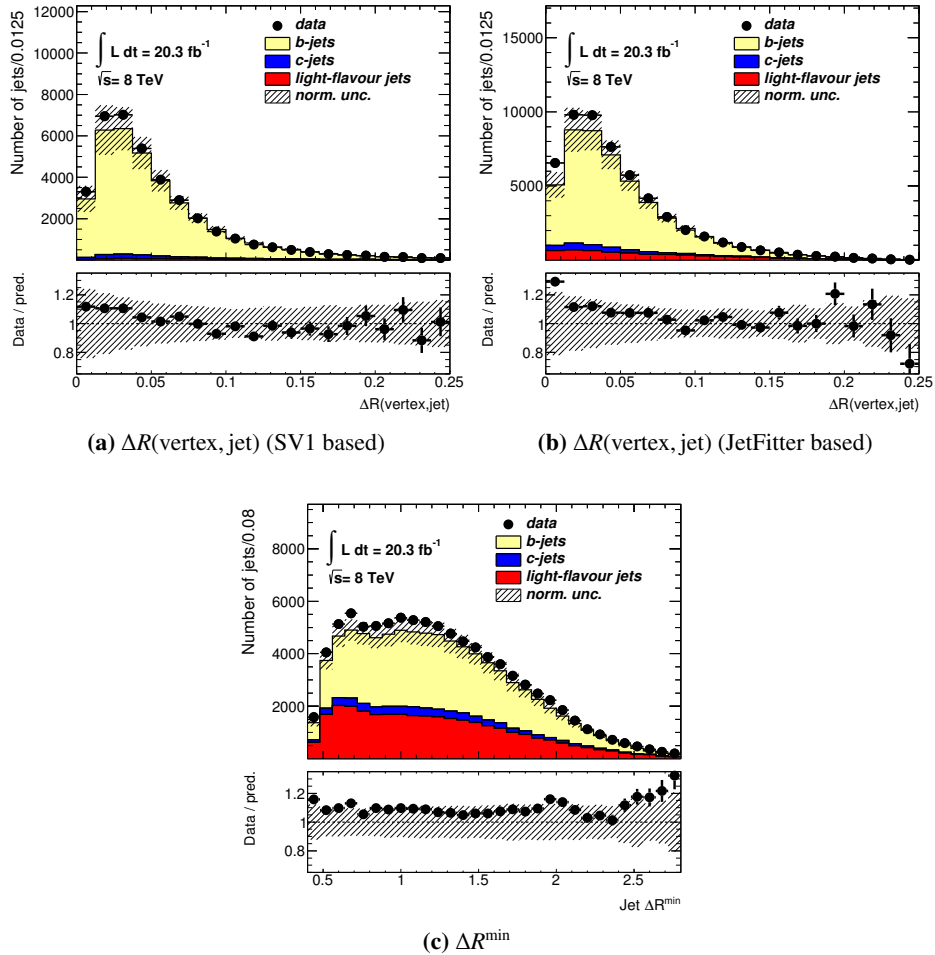
Figure 8.5: Distribution of the \Delta R(\text{vertex}, \text{jet}) for secondary vertex candidates contained in the selected probe jets (a-b) as well as their \Delta R^{\min} (c). The predictions from the simulation are subdivided into the three different jet flavour types. The simulated samples are normalised according to their predicted cross-sections to an integrated luminosity of 20.3 \text{ fb}^{-1} . Ratios of the data and the simulation are shown as well at the bottom of each plot.
