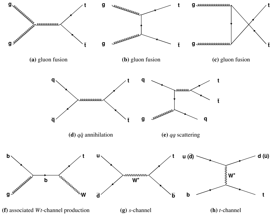
Figure 2.3: Examples for Feynman diagrams of the leading order top-quark pair production due to gluon-fusion (a-c) and quark-antiquark-annihilation (d). In addition, examples for the next-to-leading order production of top-quark pairs via qg scattering (e) and the s -, t - and Wt -channel production of single top-quarks are presented as well.
