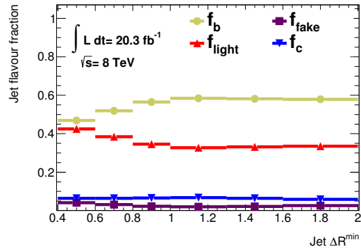
(c) Flavour fractions as a function of the \Delta R^{\min}
