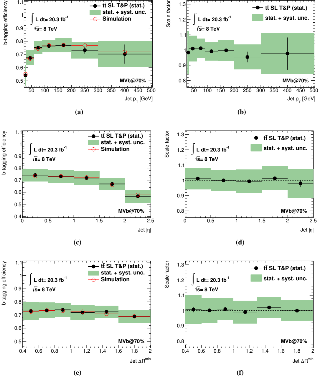
Figure 8.14: The b -tagging efficiencies for the MVb algorithm corresponding to an operating point of an overall efficiency of 70% as a function of the transverse momentum (a), the absolute pseudorapidity (c) and the \Delta R^{\min} (e) of the jets contained in the sample of t\bar{t} single lepton (SL) candidate events. The b -tagging efficiencies are shown for the predictions by the simulation (as a red line) and the measurements in data by the tag and probe (T&P) method (as black dots). The total uncertainties of these measurements are displayed as well (by the green filled area). The uncertainties on the predicted tagging efficiencies are based only on the the Monte Carlo statistics. The corresponding data-to-simulation scale factors are presented in addition also as a function of the jet p_T (b), |\eta| (d) and \Delta R^{\min} (f).
