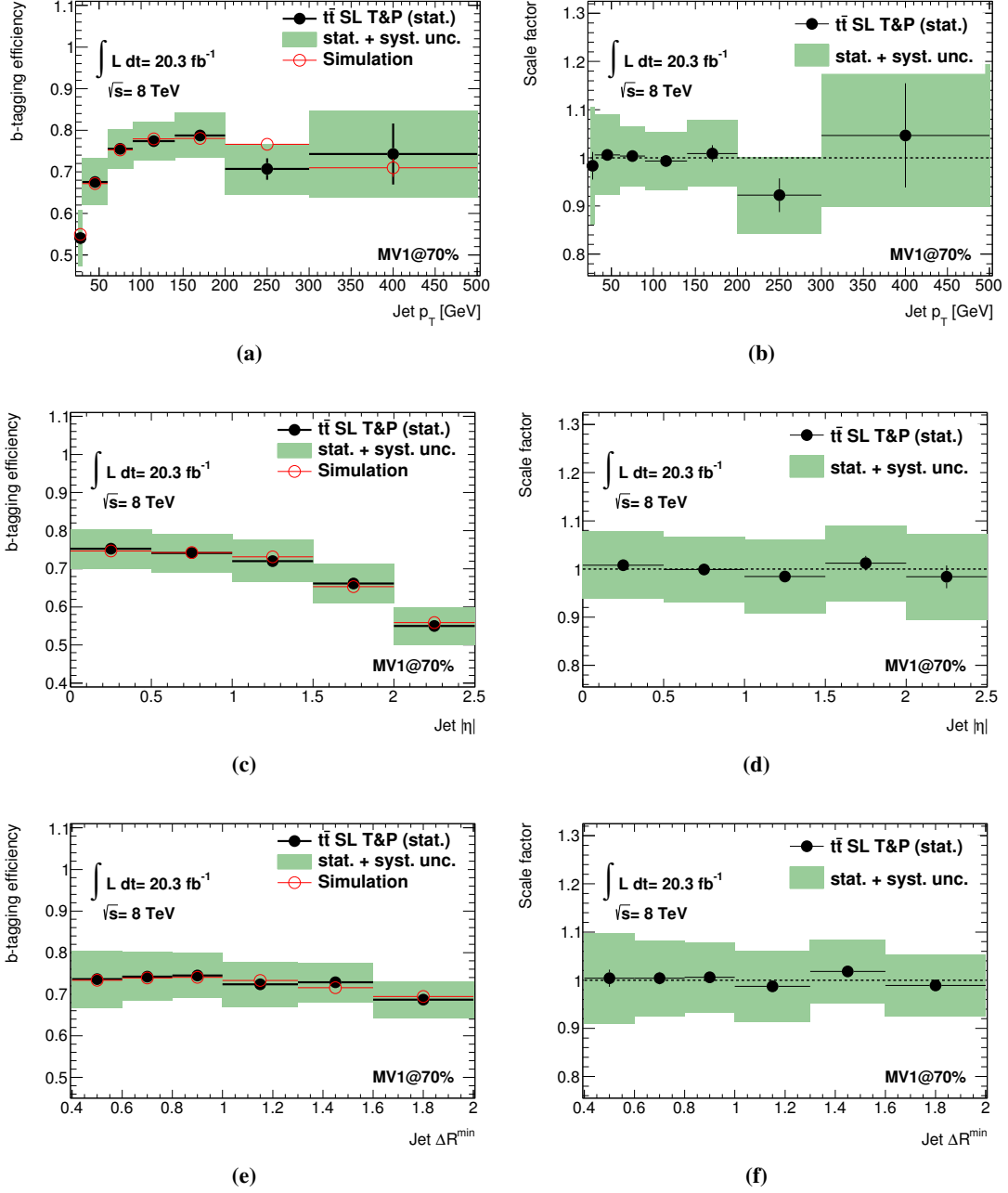
Figure 8.17: The b -tagging efficiencies for the MV1 algorithm corresponding to an operating point of an overall efficiency of 70% as a function of the transverse momentum (a), the absolute pseudorapidity (c) and the \Delta R^{\min} (e) of the jets contained in the sample of t\bar{t} single lepton (SL) candidate events. The b -tagging efficiencies are shown for the predictions by the simulation (as a red line) and the measurements in data by the tag and probe (T&P) method (as black dots). The total uncertainties of these measurements are displayed as well (by the green filled area). The uncertainties on the predicted tagging efficiencies are based only on the Monte Carlo statistics. The corresponding data-to-simulation scale factors are presented in addition also as a function of the jet p_T (b), |\eta| (d) and \Delta R^{\min} (f).
