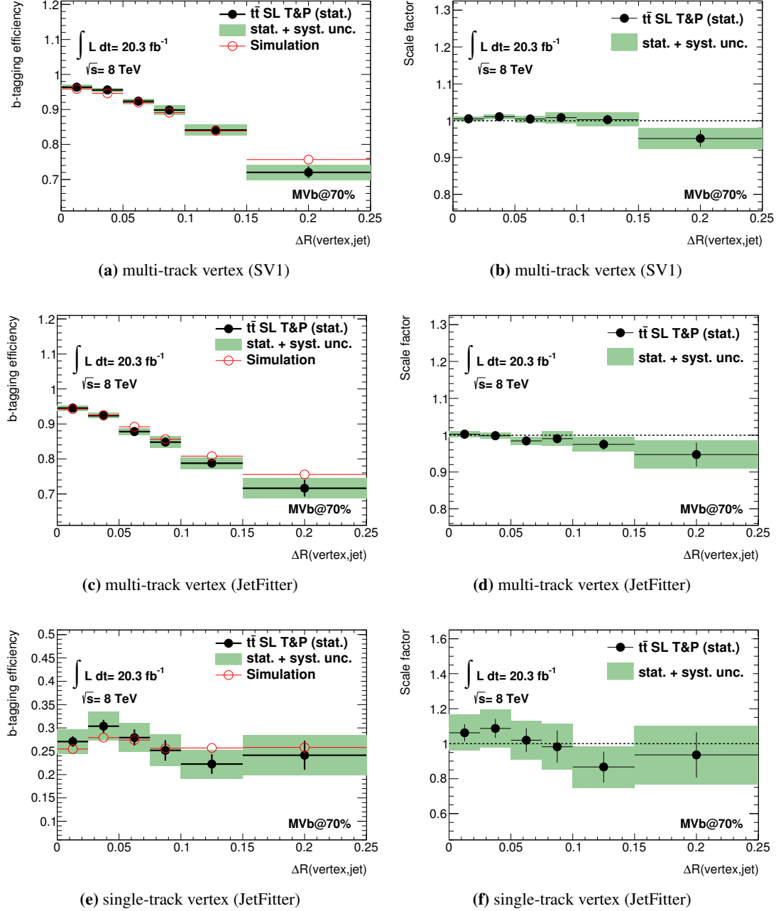
Figure 8.15: Results of the b -tagging efficiency measurements for the MVb algorithm corresponding to an operating point of 70% efficiency as a function of the angular separation between the vertex direction and the jet axis \Delta R(\text{vertex}, \text{jet}) . The measurements are performed separately for jets having a vertex reconstructed with the iterative vertex finder (a-b) and the JetFitter algorithm (c-f), where the vertex candidates based on the JetFitter are subdivided into single- and multitrack-vertices. The b -tagging efficiencies (left column) are shown for the predictions by the simulation (as a red line) and the measurements in data by the tag and probe (T&P) method (as black dots). The total uncertainties of these measurements are displayed as well (by the green filled area). The uncertainties on the predicted tagging efficiencies are based only on the Monte Carlo statistics. The corresponding data-to-simulation scale factors are presented in addition (right column). As these measurements take only jets into account that have an appropriate type of secondary vertex reconstructed, the definition of the presented b -tagging efficiencies is not inclusive as in the measurements corresponding to the jet p_T , \eta or \Delta R^{\min} .
