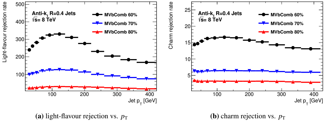
Figure 6.22: Rejection rates for light-flavour (a) and charm (b) jets corresponding to three different operating points of the MVbComb algorithm as a function of the jet p_T . The considered jets are obtained from a sample of SM t\bar{t} decays that are simulated using the POWHEG and PYTHIA generators.
