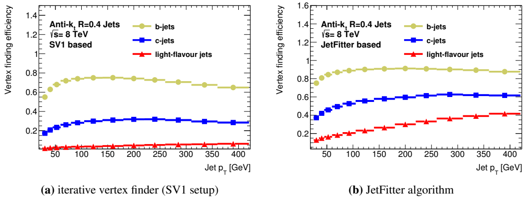
Figure 4.3: Efficiencies to reconstruct a secondary vertex provided by the iterative vertex finder (a) and the JetFitter algorithm (b) as a function of the jet p_T presented separately for b -, c - and light-flavour jets. These jets are obtained from a t\bar{t} sample that is simulated using the POWHEG and PYTHIA generators.
