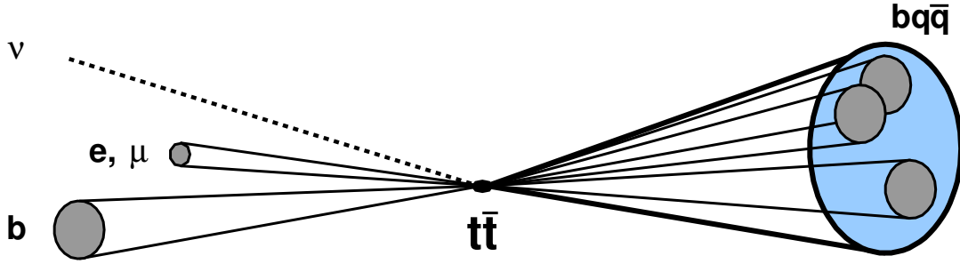
Figure 5.2: Schematic view of the decays of a boosted top and antitop-quark into a final state containing leptons and jets. The decay products on both the leptonic and hadronic side of the event are strongly collimated and their signatures might overlap in the calorimeter system. As the standard narrow-cone jet algorithms might fail to resolve the hadronic side of the event, the t \rightarrow bW \rightarrow bq\bar{q} decay is reconstructed as one single large-radius jet in order to recover sensitivity.
