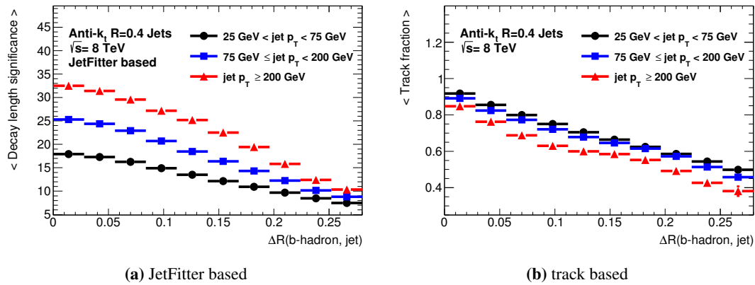
Figure 6.6: Average decay length significance (a) for vertices reconstructed with the JetFitter algorithm as well as the average fraction of b -hadron tracks inside a flavour labelled b -jet that have a positive impact parameter sign. Both jet properties are shown as a function of the angular separation between the b -hadron flight direction at generator level and the axis direction of the associated jet. The track fractions are determined using only those jets which contain at least four tracks associated to the decay products of the b -hadron (using information at the generator level). Both studies are based on selected b -jets that are obtained from SM t\bar{t} decays, which are simulated using the POWHEG and PYTHIA generators. Jets are classified into three different p_T regions and studied separately.
