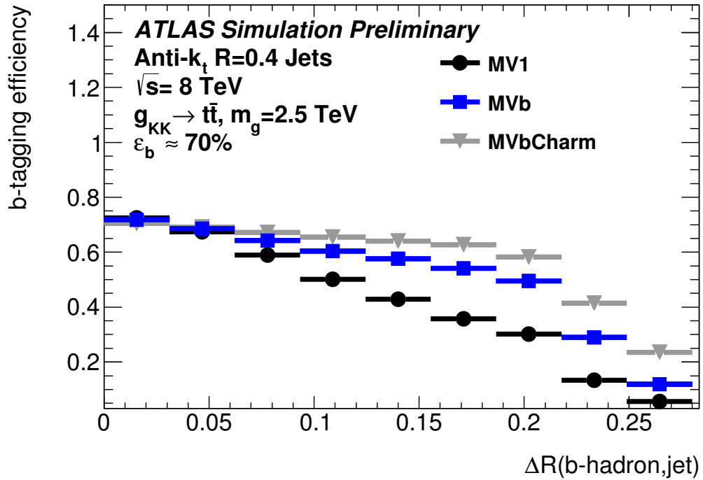
(b) b -tagging efficiencies vs. \Delta R(b\text{-hadron}, \text{jet})
