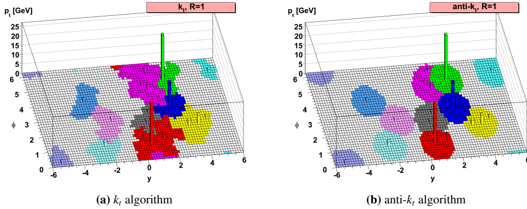
Figure 3.8: Shape comparison of the active jet areas for two different jet clustering algorithms. All particles within the active area of a particular jet will be clustered into this jet [88].
