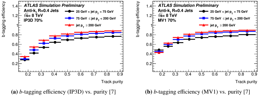
Figure 6.7: b -tagging efficiencies of the IP3D (a) and MV1 (b) algorithms as a function of the track purity of the studied jets. The results are shown separately for three different jet p_T ranges and correspond to an operating point that has an overall efficiency of 70%. To ensure that a low track purity is related to a contamination with tracks from light-flavour decays, rather than to the missing of tracks from the b -hadron decay, only those jets that contain at least three tracks associated to the decay products of the b -hadron are considered. The jets used for this study are obtained from a sample of SM t\bar{t} decays, which are simulated using the POWHEG and PYTHIA generators.
