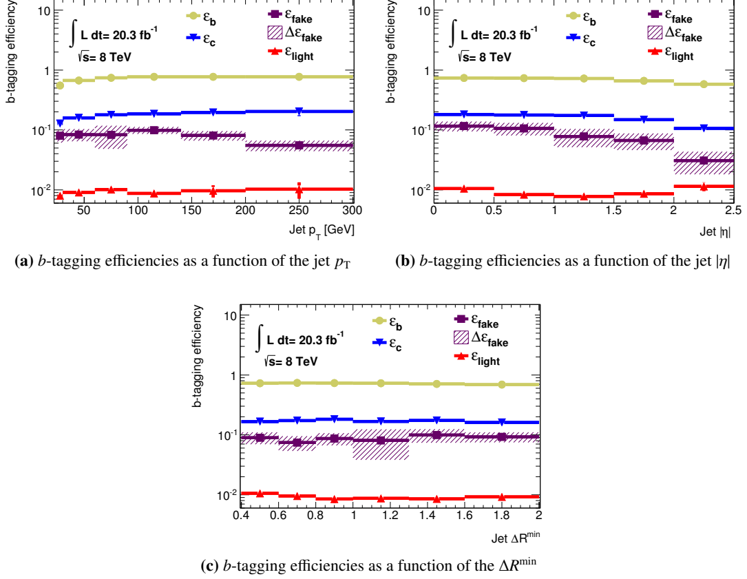
Figure 8.12: b -tagging efficiency for b -, c - and light-flavour jets (extracted from the simulation) as well as for jets stemming from the non-prompt and fake lepton background (obtained from a control region in data) corresponding to the MVb algorithm at an operating point that provides an overall efficiency of 70%. The systematic uncertainties assigned to \epsilon_{\text{fake}} (shaded areas) correspond to the envelope of the different results obtained from the various control regions. Both the efficiencies of the various jet flavours and the uncertainties on \epsilon_{\text{fake}} are shown as a function of the probe jet p_T (a), \eta (b) and \Delta R^{\min} (c).
