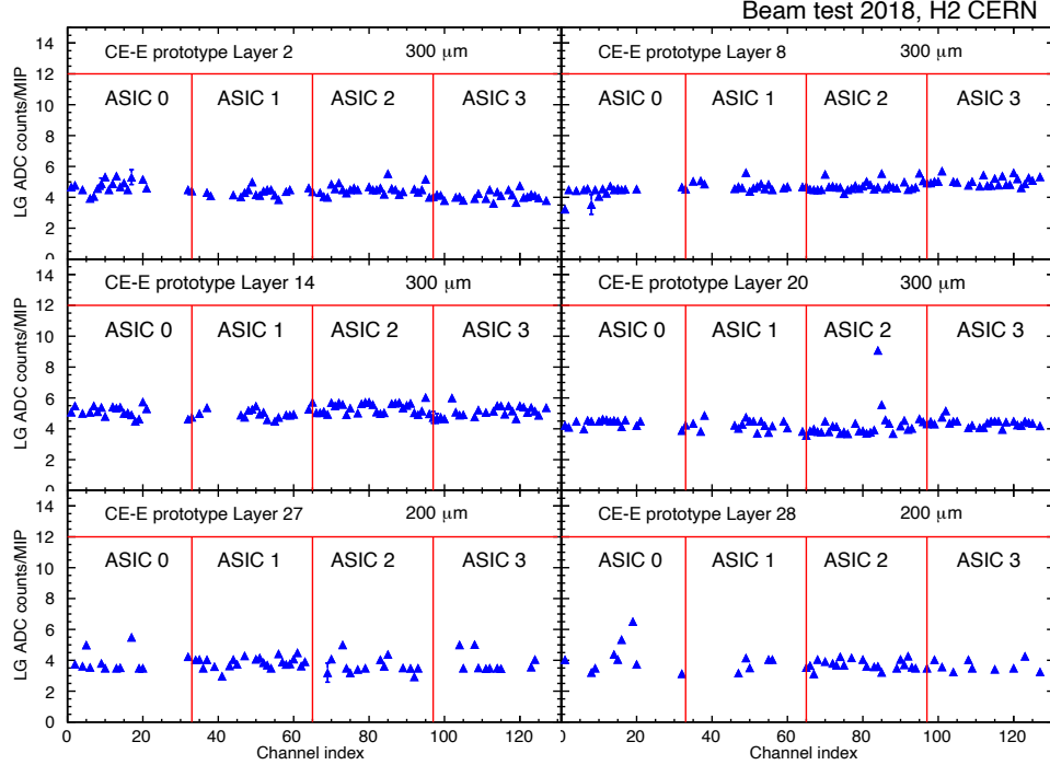
FIGURE 6.39: Summary plot for LG ADC counts per MIP for LG channels for a few CE-E layers. Bottom two plots corresponds to 200 \mu\text{m} thick silicon cells.
