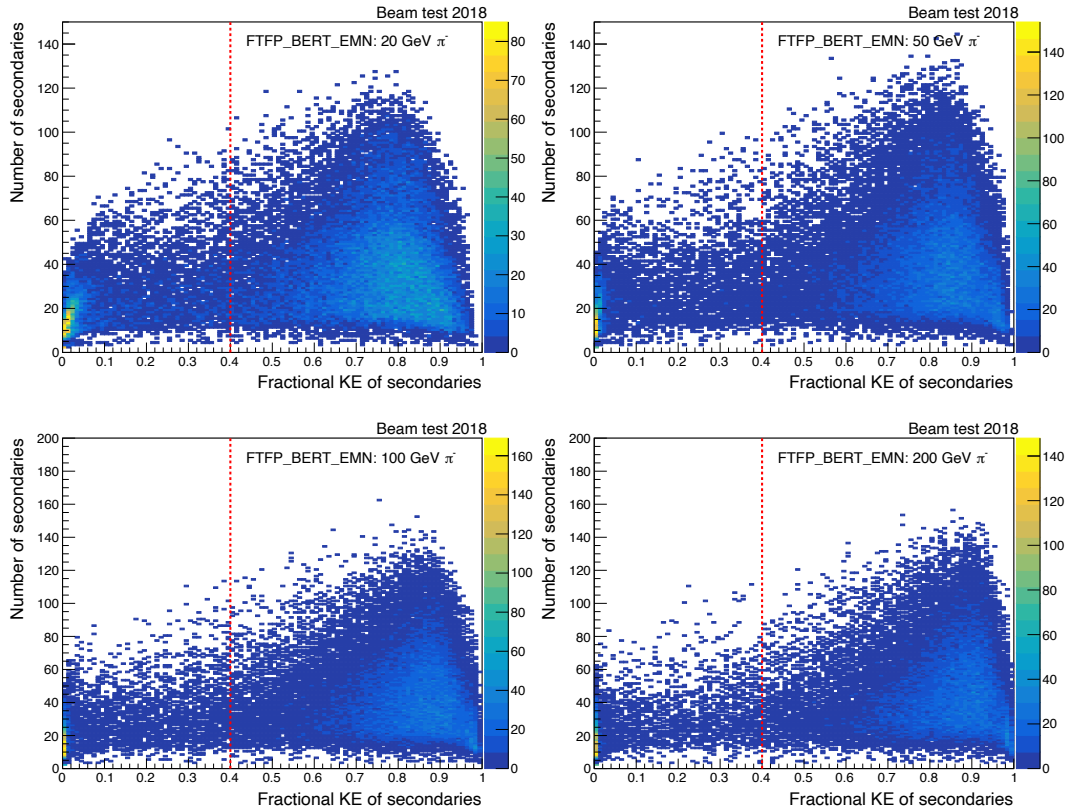
FIGURE 7.14: The correlation between fractional kinetic energy carried by secondary particles versus number of secondary particles produced at the first hadronic interaction for different \pi^- beam. The population at the left bottom corner of the plot corresponds to interactions where the number of secondary particles produced are small and the fractional energy carried by the incident \pi^- is large. A cut at 0.4 as indicated by vertical dotted red line is applied to reject such events for optimization purpose.
