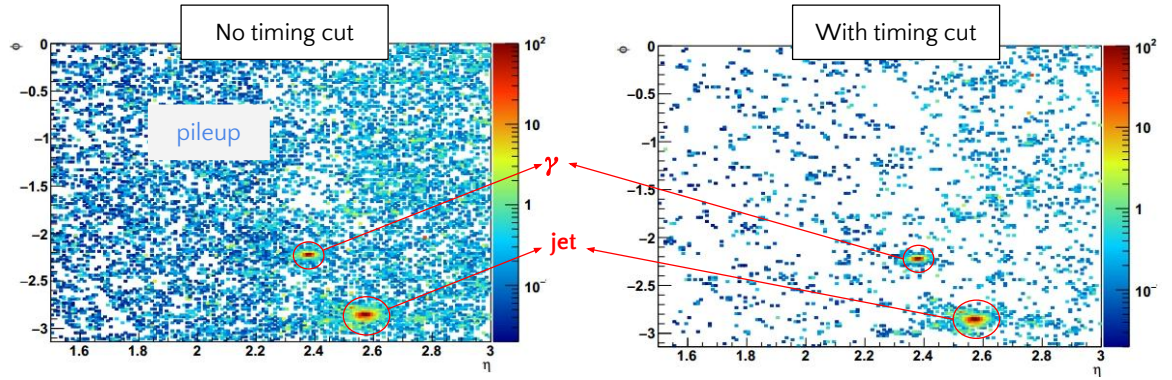
FIGURE 4.16: VBF ( H \rightarrow \gamma\gamma ) event with one \gamma and VBF jet in the same quadrant (shown in red circles). The image is projected onto the front face of HG-CAL. The left figure corresponds to without requiring any timing cut and the right figure corresponds to after applying a time window cut of |\Delta t| < 90 ps on cells with charge q > 12 fC [23].
