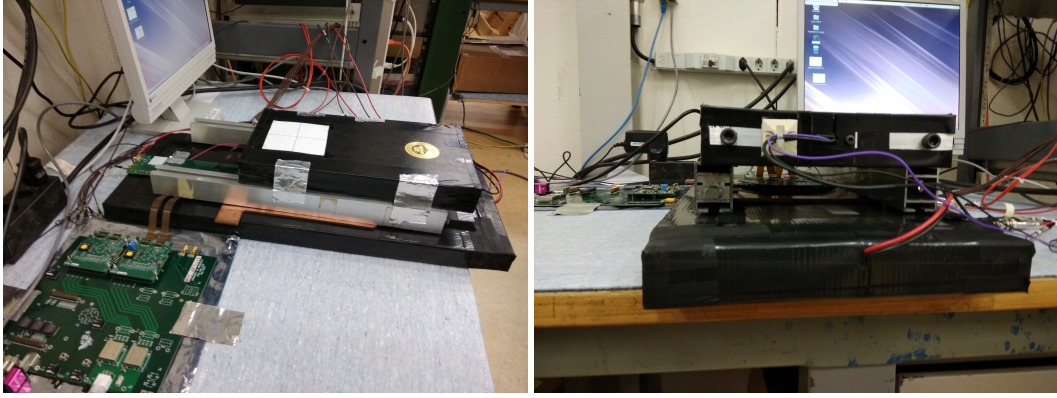
FIGURE 5.12: Two images show the cosmic muon setup from two angles. Sensor module is placed in between two scintillator tiles (right).
