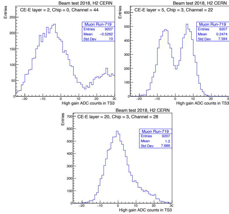
FIGURE 6.43: HG ADC distribution for two channels in the neighbourhood of \mu HDMI connection. These channels showed abnormal behaviour noise behaviour therefore were masked (not used) for further data analysis.
