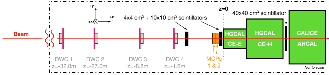
FIGURE 6.12: The image shows an schematic view of all the detectors deployed in the beamline upstream of HGCAL + AHCAL prototype experimental setup.
