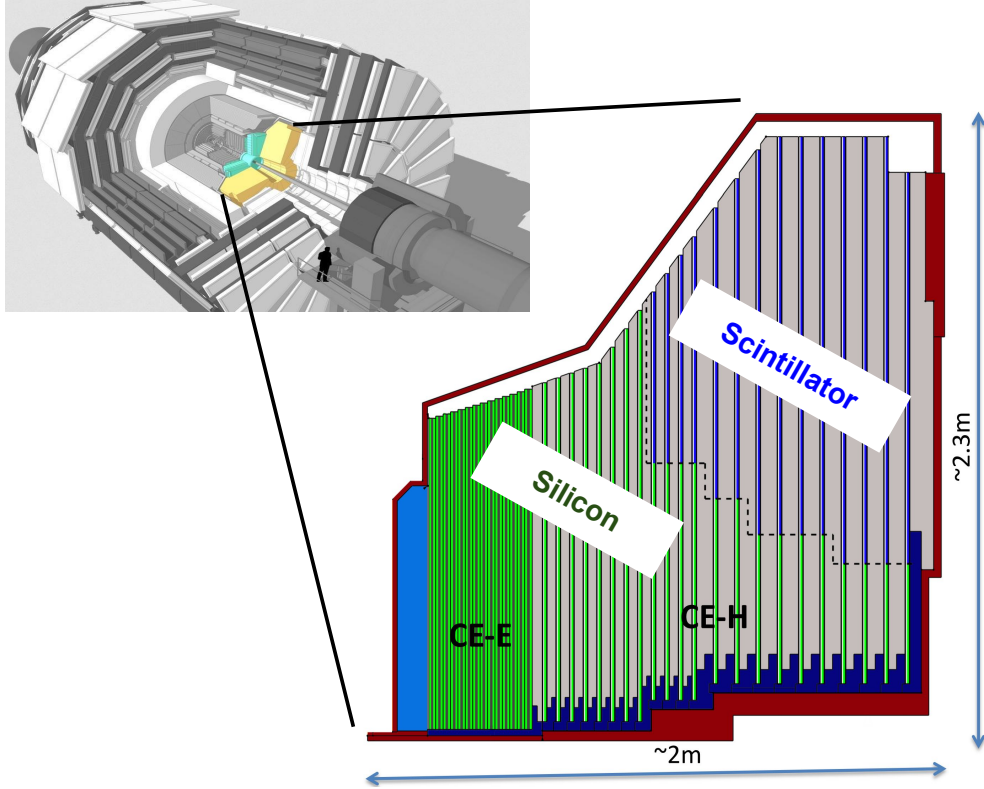
FIGURE 4.6: The longitudinal cross-sectional view of proposed HGCal calorimeter.
