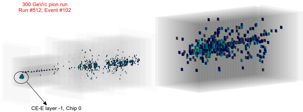
FIGURE 7.1: Event display of a 300 GeV/c pion event. Pion initiates a shower in CE-H prototype compartment which continues to develop in AHCAL section. Chip 0 of the first layer of CE-E shows full occupancy. This behaviour was observed in other runs as well therefore this whole chip is masked at the analysis level.
