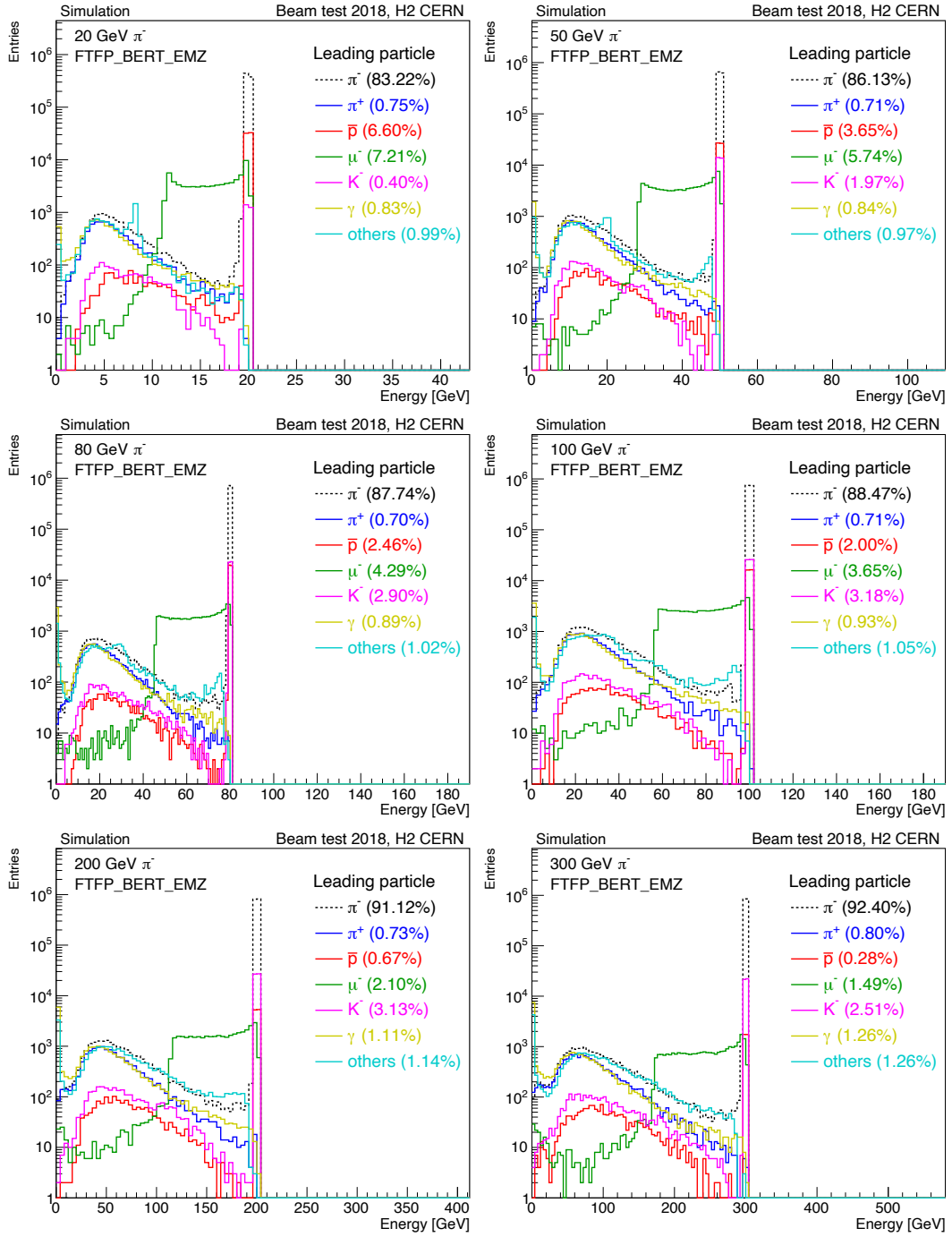
FIGURE 7.2: Energy distribution of leading particle and their event fractions (as indicated in the legends) reaching HGCal surface for different pion beam energy. The fraction and energy distributions are obtained from full beamline simulation. The beam purity is more than 80% or 90% depending on beam energy.
