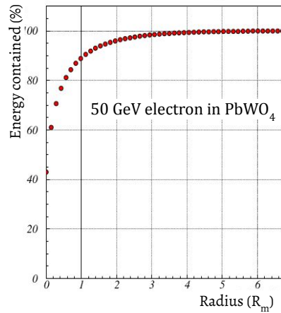
FIGURE 2.12: Transverse shower development for 50 GeV electron in PbWO_4 . The x-axis is the radius or distance from the shower axis in terms of Molière radius, of an infinite cylinder, and y-axis is the fractional energy contained in the the cylinder of radius R . By definition, 90% energy is contained at 1 R_m as indicated by the vertical black line.
