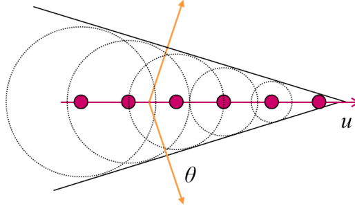
FIGURE 2.19: Cerenkov radiation generated by a charged particle passing through the dielectric medium with a velocity u which is greater than velocity of light in the same medium. The Cerenkov photons radiate at an angle \theta from particle trajectory.
