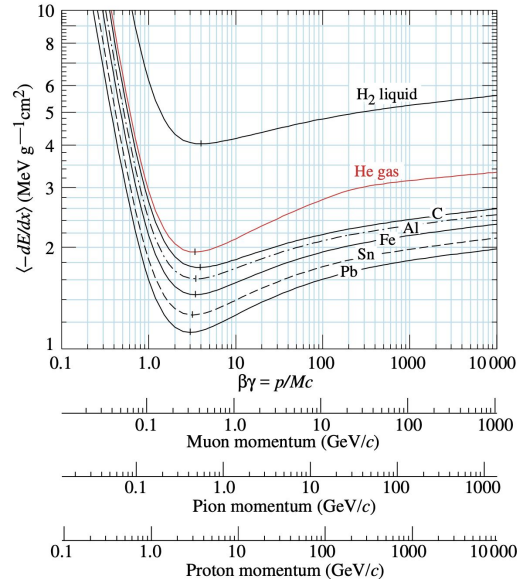
FIGURE 2.3: Mean energy loss of charged particle as a function of \beta\gamma in different materials. The x-axis scale is also shown as a function of momentum for different charged particles [36].
