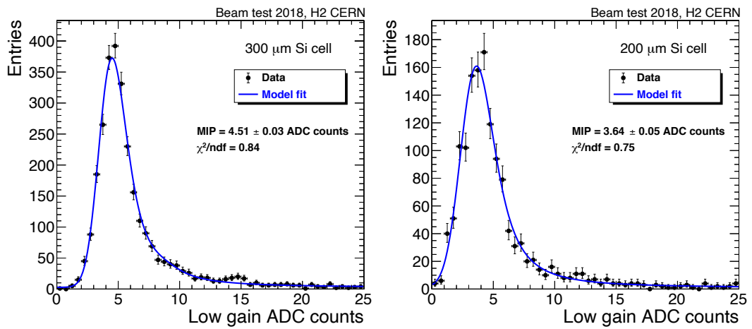
FIGURE 6.38: Figure shows LG ADC distributions fitted with landau convoluted with Gaussian distribution for 300 \mu\text{m} (left) and 200 \mu\text{m} (right) thick silicon cell.
