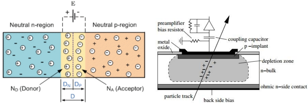
FIGURE 2.20: Schematics of a typical p-n junction diode (left) and a transverse view of ionizing particle traversing through silicon sensor (right) [45].
