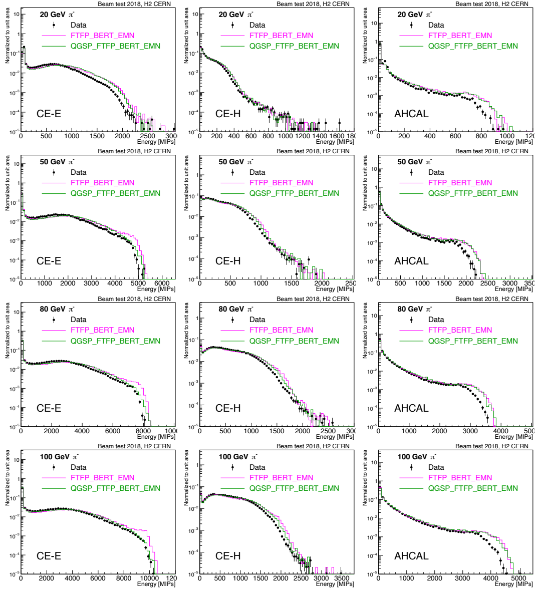
FIGURE 7.6: Energy comparison between data and simulation in CE-E (left column), CE-H (middle column) and AHCAL (right column) for 20, 50, 80 and 100 GeV pions. The black dots correspond to data points and magenta and green line corresponds to simulation with FTFP.BERT.EMN and QGSP.FTFP.BERT.EMN physics list, respectively.
