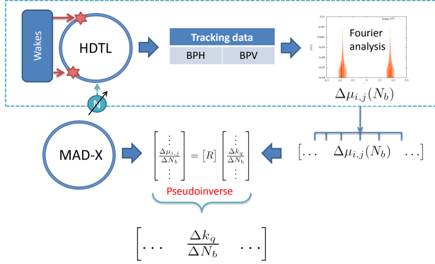
Figure 4.7: Recostruction algorithm.
