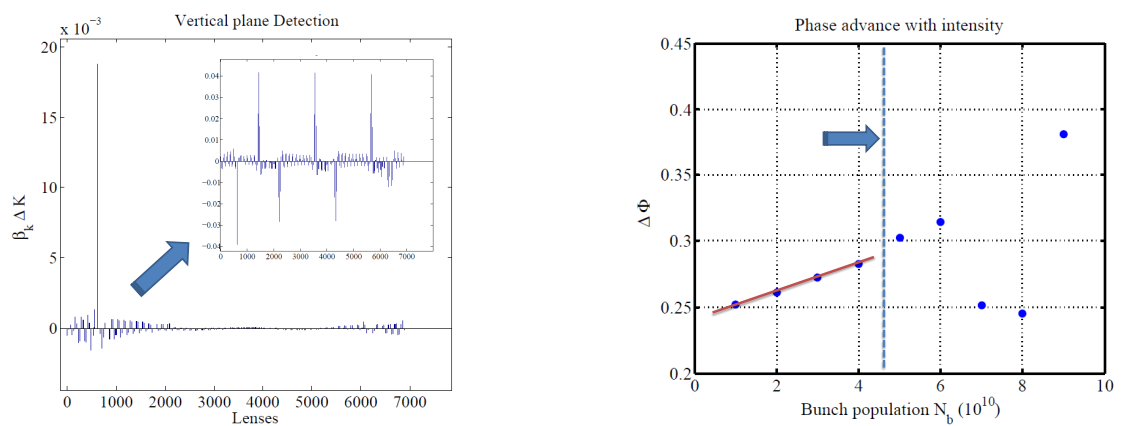
Figure 5.14: Single MKPx100 reconstruction. \Delta K refers to thin lens error slope with intensity. Problems in tune shift, beam stability, and reconstruction, can arise.
