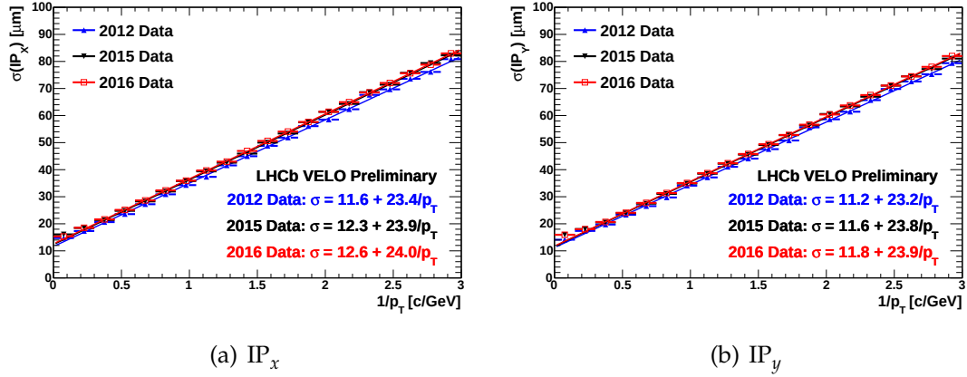
Figure 3.6: IP resolutions of the components as a function of the inverse of the transverse momentum. The resolution quoted in the text refers to the total IP = \sqrt{\text{IP}_x^2 + \text{IP}_y^2} , where the \text{IP}_z component is neglected due to the LHCb forward geometry [83].
