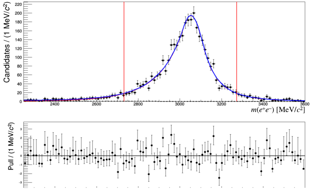
Figure B.22: Fit to the e^+e^- mass for bin 3, bremsstrahlung added, \text{PIDE} > 0 .
