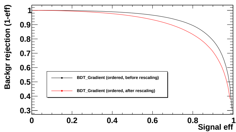
Figure A.7: Comparison of the BDT performance before and after MC scaling.
