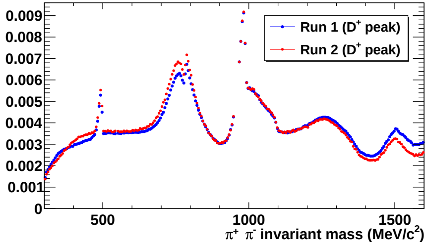
Figure 4.30: Distributions of \pi^+ \pi^- mass for Run 1 and Run 2, for the D^+ peak region.
