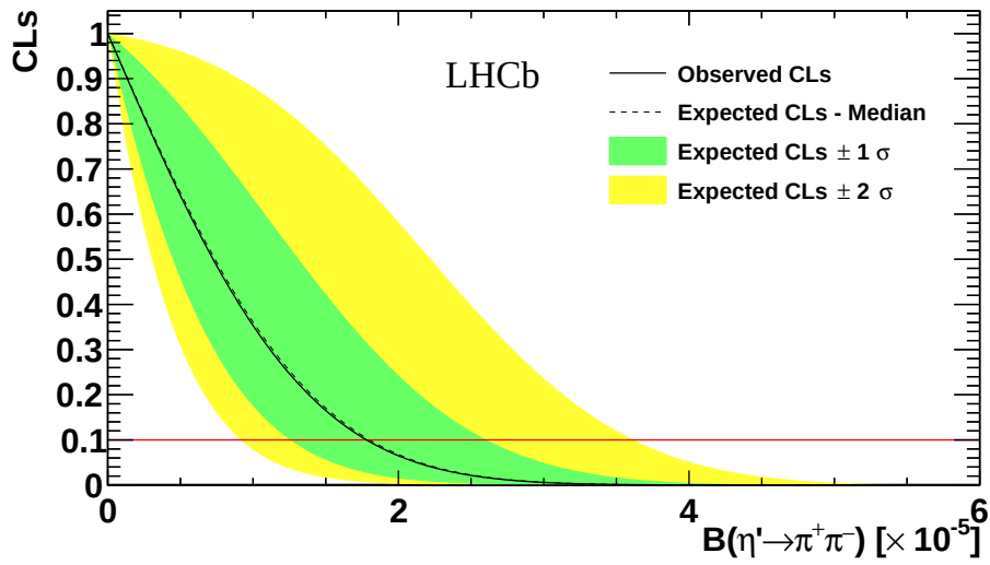
Figure 4.53: CL_s distribution for B(\eta' \rightarrow \pi^+ \pi^-)
