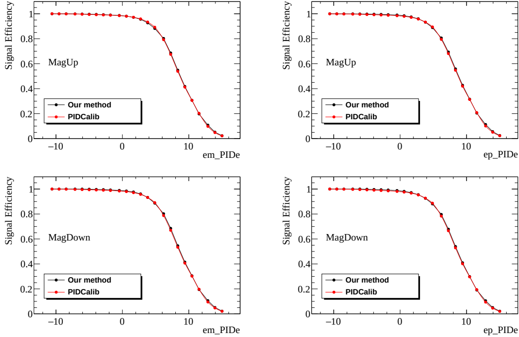
Figure 5.17: Comparison between the tag-and-probe method (“Our method”) and the standard method (“PIDCalib”) to calculate electron PID efficiencies, for both magnet polarities and both values of charge of the probe. No bremsstrahlung photons are added.
