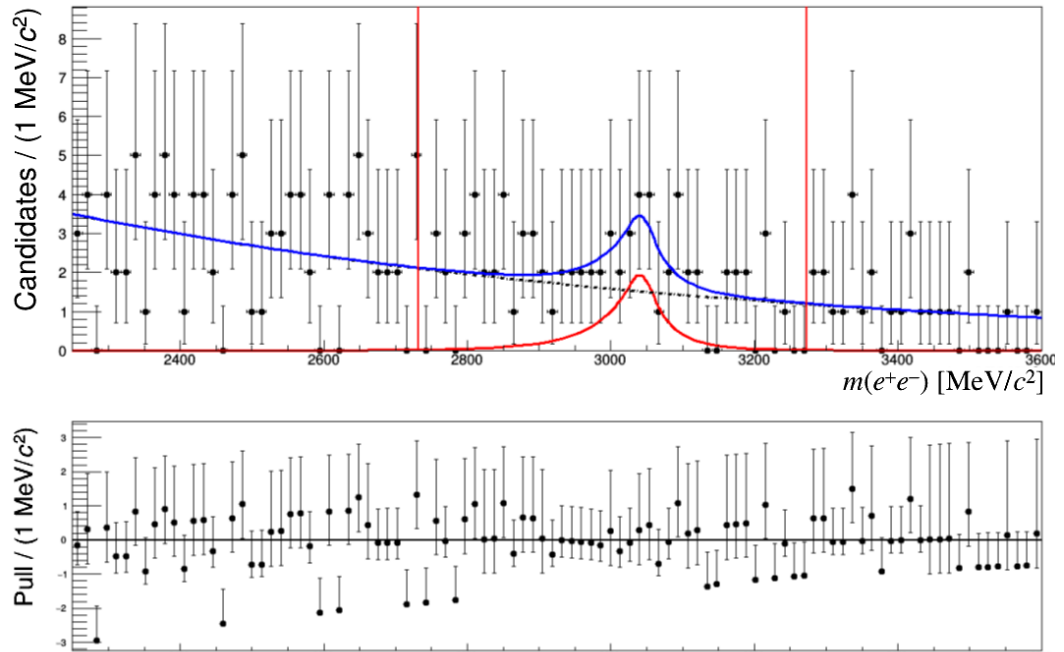
Figure B.23: Fit to the e^+e^- mass for bin 3, bremsstrahlung added, \text{PIDE} < 0 .
