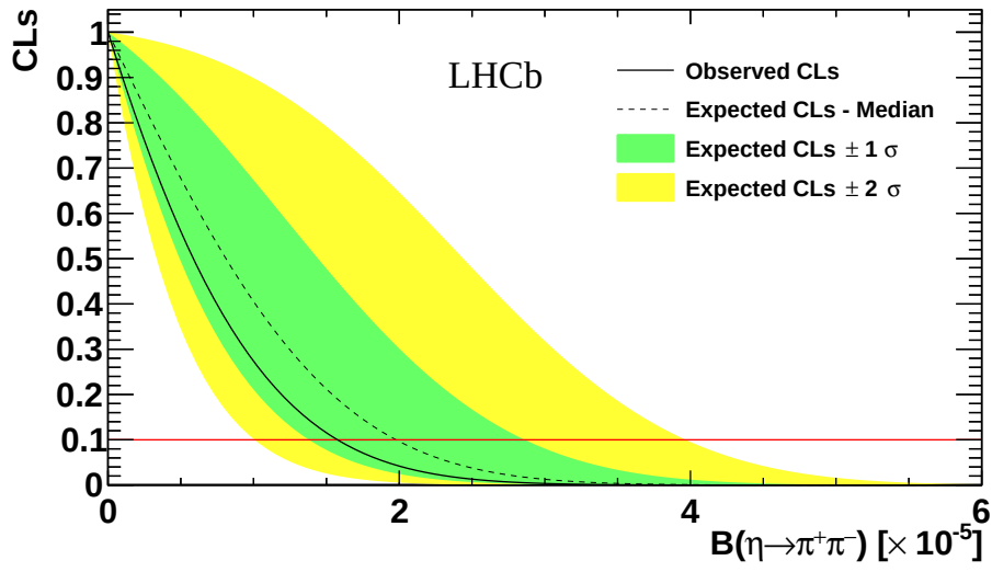
Figure 4.52: CL_s distribution for B(\eta \rightarrow \pi^+ \pi^-)
