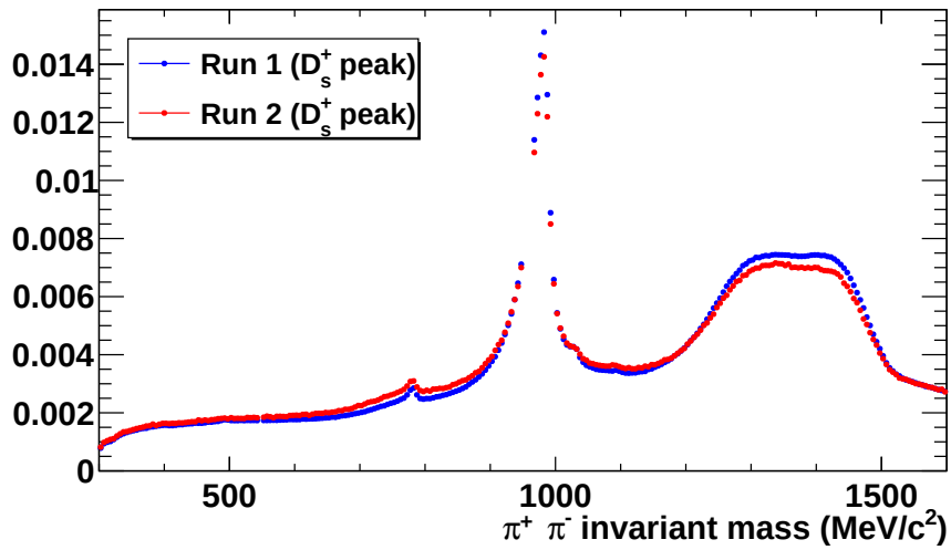
Figure 4.31: Distributions of \pi^+ \pi^- mass for Run 1 and Run 2, for the D_s^+ peak region.
