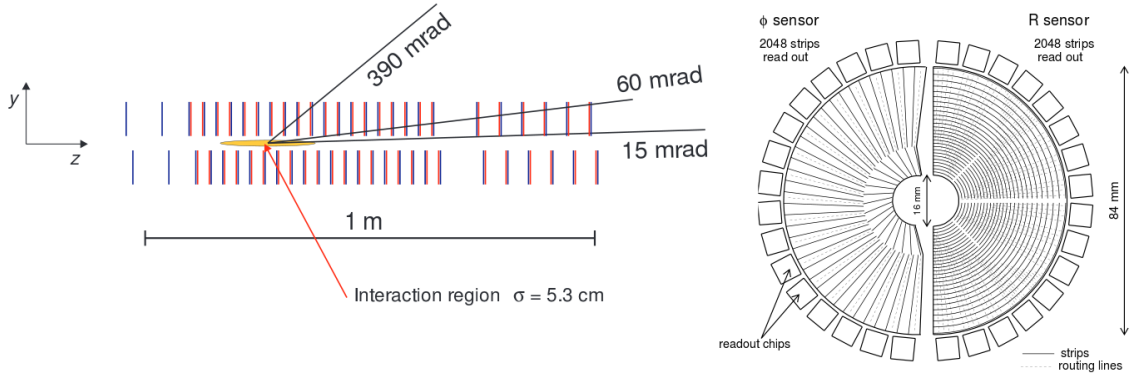
Figure 3.4: VELO system configuration and VELO sensors [81].
