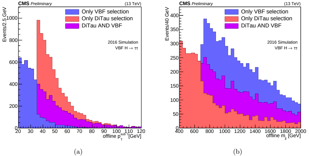
Figure 3.7 – Additional events from the L1 VBF seed (with at least one jet with E_T > 110 GeV and at least two jets with E_T > 35 GeV and m_{jj} > 620 GeV) with respect to the double- \tau_h seed (at least 2 isolated taus with E_T > 32 GeV and |\eta| < 2.1 ) as a function of the p_T of the offline subleading tau (a) and of the invariant mass of the offline jets with highest m_{jj} (b). The events in each of the categories “Only VBF selection” and “Only di-tau selection” are events that fired only one of the triggers and pass only the offline selection corresponding to that trigger. The events in the category “di-tau AND VBF” fire both triggers and pass both offline selections [95].
