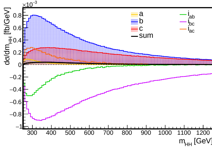
Figure 1.13 – Differential cross section corresponding to each of the VBF production diagrams, represented in Fig. 1.8, and their interference, as a function of the invariant mass of the Higgs pair.
