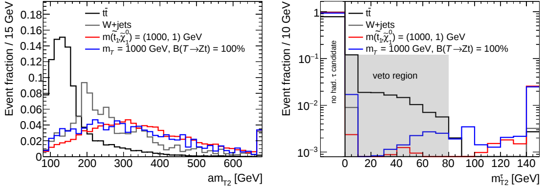
Figure 8.4: Comparison of the distributions of am_{T2} (left) and m_{T2}^{\tau} (right) for the dominant background processes t\bar{t} and W +jets, and for two signal models, after the preselection and m_T > 120 GeV. Due to the m_T requirement, the t\bar{t} process is dominated by dileptonic decay modes. The left-most column of the right plot shows the fraction of events without a hadronic \tau candidate.
