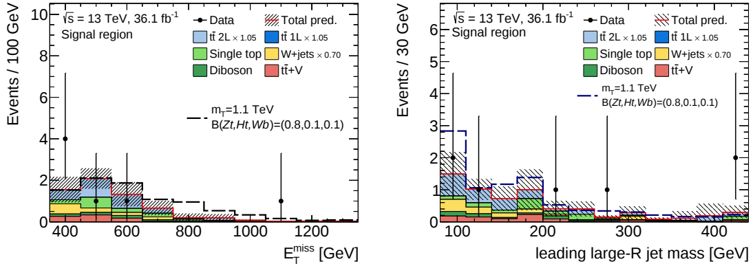
Figure 9.32: Comparison of data and prediction in the E_T^{\text{miss}} distribution (left) and the mass of the leading large- R jet (right) in the SR. The error bands include statistical and systematic uncertainties. The expected shape for a signal with m_T = 1.1 TeV and \mathcal{B}(T \rightarrow Zt) = 80\% is overlaid on the SM prediction.
