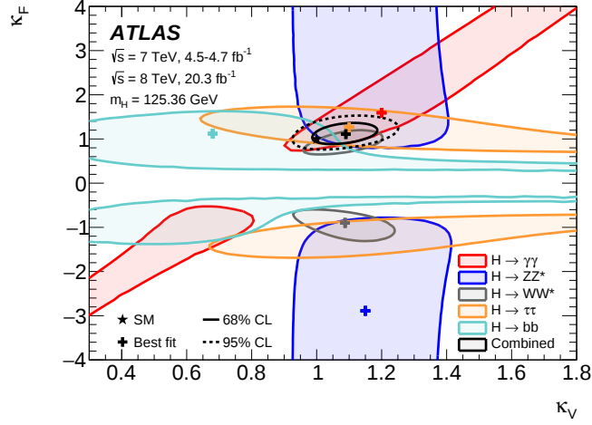
Figure 1.5: Results of the two-dimensional fit to the Higgs boson coupling-strength scale factors \kappa_F for fermions and \kappa_V for vector bosons [20].
