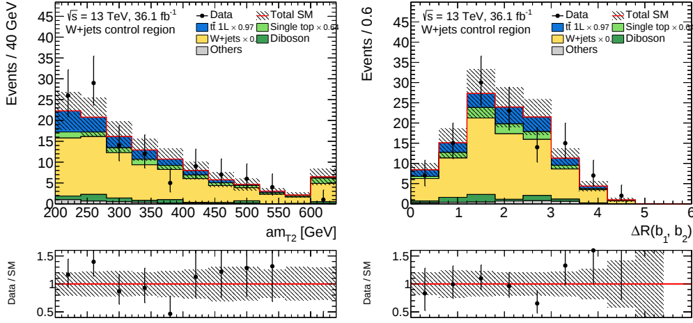
Figure C.9: Distribution of the am_{T2} and the \Delta R(b, b) in the WCR. The background normalisation factors are applied as indicated in the legend. The lower panels show the ratio of the data to the prediction. The error bands include statistical and systematic uncertainties.
