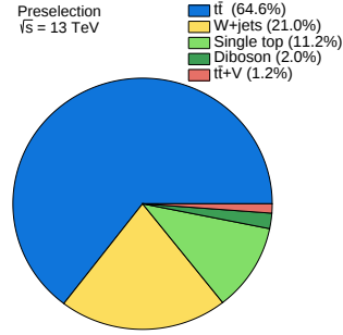
Figure 8.1: Relative contribution of the SM processes after the preselection.
