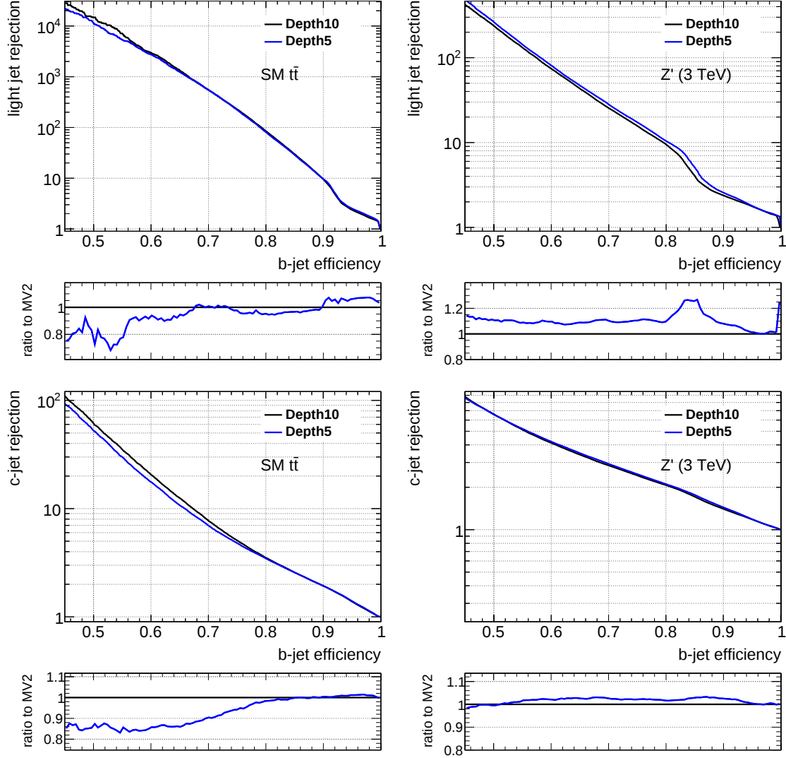
Figure A.4: Light flavour jet rejection (top) and c -jet rejection (bottom) as a function of the b -tagging efficiency for multiple training options based on MV2 and additional variables, evaluated on an inclusive t\bar{t} sample (left) and on Z' \rightarrow t\bar{t} events (right). The black line shows the training with depth=10, nTrees=400 and the blue line shows the results for the training with depth=5, nTrees=500.
