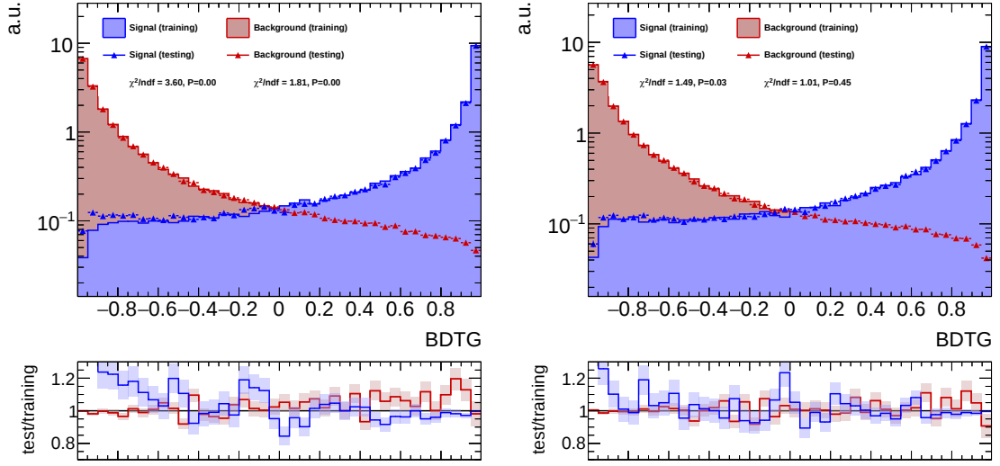
Figure A.3: Comparison of the BDT result for the training and the test samples, for two different sets of BDT settings. The left figure shows the training with depth=10 , nTrees=400 and the right figure shows the training with depth=5 , nTrees=500 . The reduced \chi^2 and the \chi^2 -probability are given below the legends.
