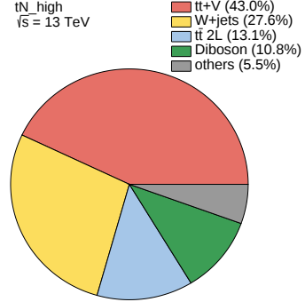
Figure 10.12: Breakdown of the individual SM contributions in the signal region.
