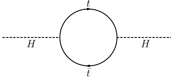
Figure 1.6: Example of a one-loop correction to the Higgs mass.
