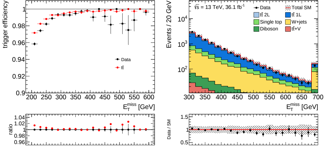
Figure 8.6: Comparison of the trigger efficiency for data and t\bar{t} simulation (left), and comparison of data and simulation in the E_T^{\text{miss}} distribution after preselection (right). The lower panels show the ratio of the data to the prediction. The error bands include statistical and systematic uncertainties.
