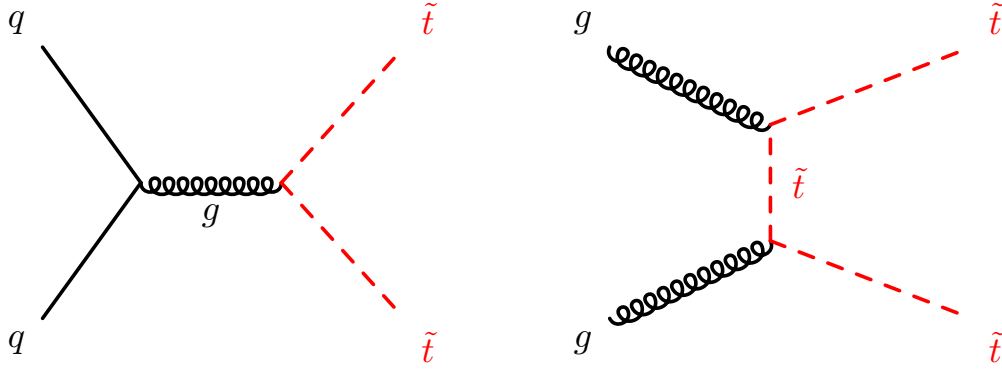
Figure 3.3: Example diagrams for the pair production of top squarks from quark–anti-quark annihilation and gluon fusion.
