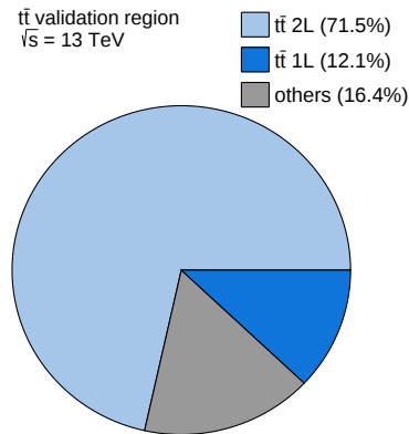
Figure 9.20: Breakdown of the individual SM contributions in the TVR.
