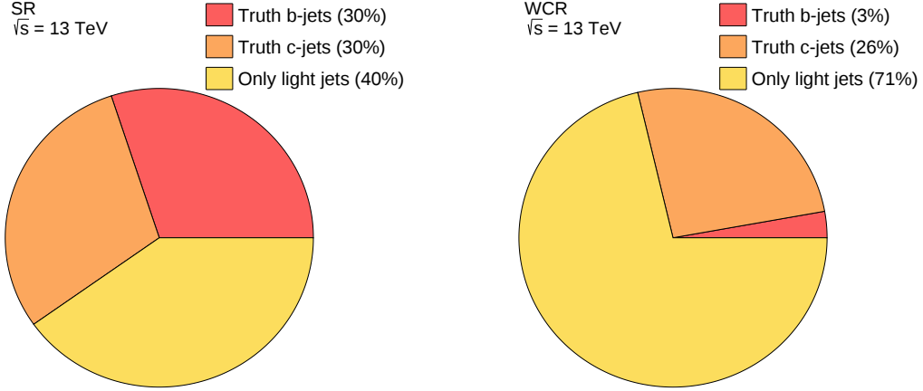
Figure 9.19: Breakdown of the flavour components of the W +jets process in the SR (left) and the W +jets control region (right). Events are classified as containing truth b -jets, when one or more of the reconstructed jets originates from a MC truth B hadron. Events with truth c -jets are classified accordingly, if they are not already classified as containing a truth b -jet. Events not falling in either category are marked as “only light jets”.
