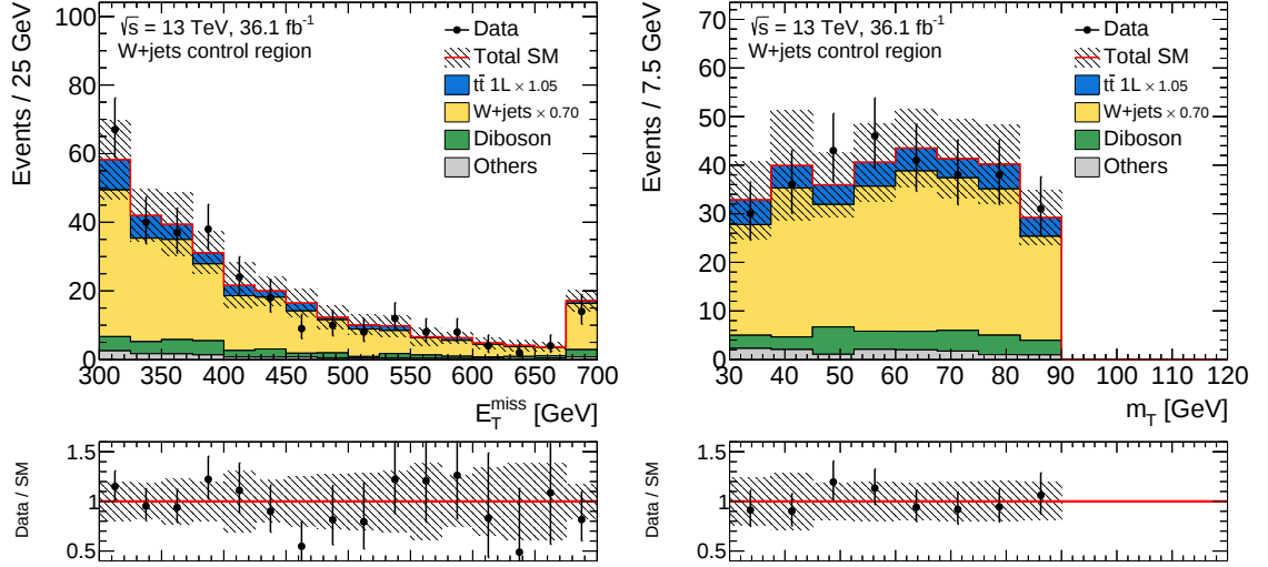
Figure 9.17: Distribution of E_T^{\text{miss}} and m_T in the W +jets control region. The t\bar{t} and W +jets normalisation factors are applied as indicated in the legend and the last bin contains overflow events. The lower panels show the ratio of the data to the prediction. The error bands include statistical and systematic uncertainties.
