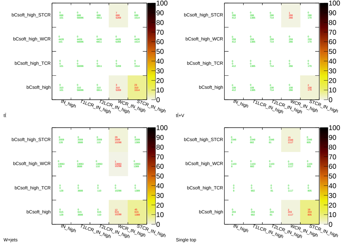
Figure C.22: Number of simulated events selected by both a bCsoft_high and tN_high associated region for the t\bar{t} (top left), t\bar{t} + V (top right), W +jets (bottom left) and single top (bottom right) backgrounds after the overlap veto. The numbers in each bin give the number of overlapping events and the number of events selected by the region indicated on the vertical axis and the horizontal axis, respectively, from top to bottom. The colour scale indicates the fraction of overlapping events.
