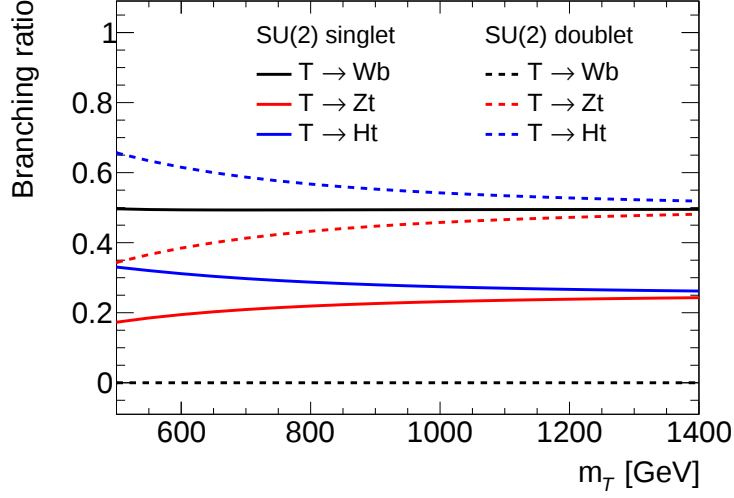
Figure 2.4: Branching ratios of the vector-like top quark decay for a SU(2)_L singlet and for the SU(2)_L doublet model, in case that V_{Tb} \ll V_{tB} [38, 39].
