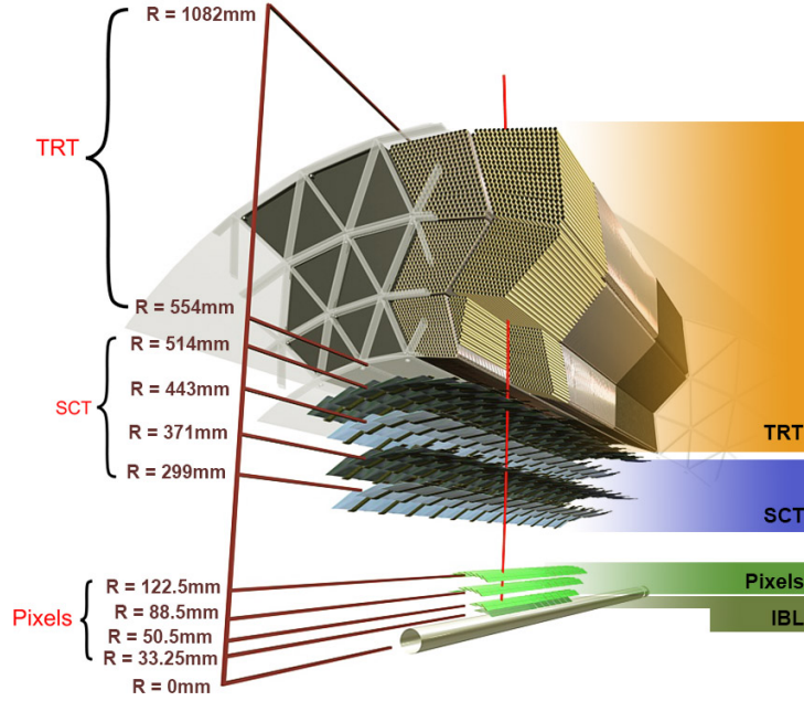
Figure 6.2: Schematic view of the barrel part of the inner detector [93].
