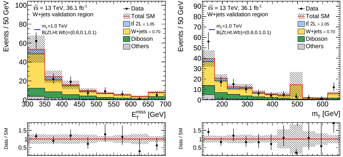
Figure 9.24: Distribution of E_T^{\text{miss}} and m_T in the W +jets validation region. The t\bar{t} and W +jets normalisation factors are applied as indicated in the legend and the last bin contains overflow events. The lower panels show the ratio of the data to the prediction. The error bands include statistical and systematic uncertainties.
