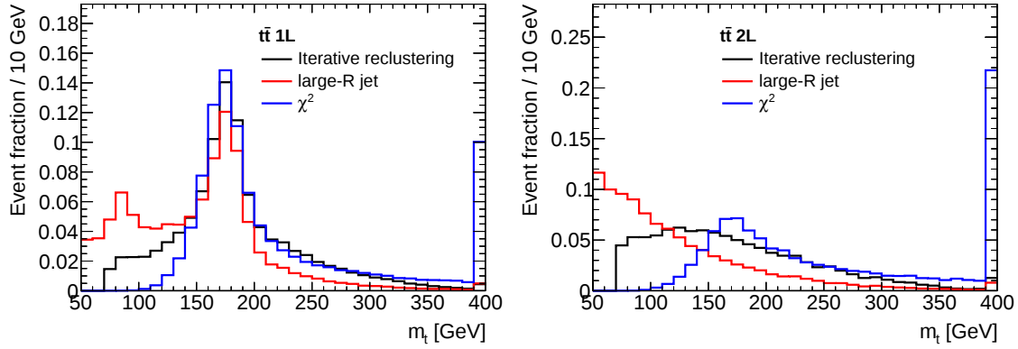
Figure 10.5: Distribution of the mass of reconstructed hadronic top candidates for semi-leptonic t\bar{t} events (left) and dileptonic t\bar{t} events (right), where the candidate always is a fake, in comparison for different reconstruction techniques. Events are required to fulfil the preselection requirements.
