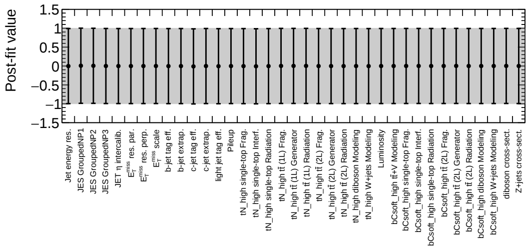
Figure 10.35: Fit values and errors of the Gaussian nuisance parameters in the combined background only fit to bCsoft_high and tN_high. The expected result is 0 with an uncertainty of \pm 1 .
