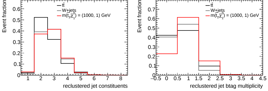
Figure 10.10: Comparison of constituent jet multiplicity (left) and constituent b -jet multiplicity (right) in the hadronic top candidate for the dominant background processes t\bar{t} and W +jets, and for a signal process after the preselection and m_T > 120 GeV.
