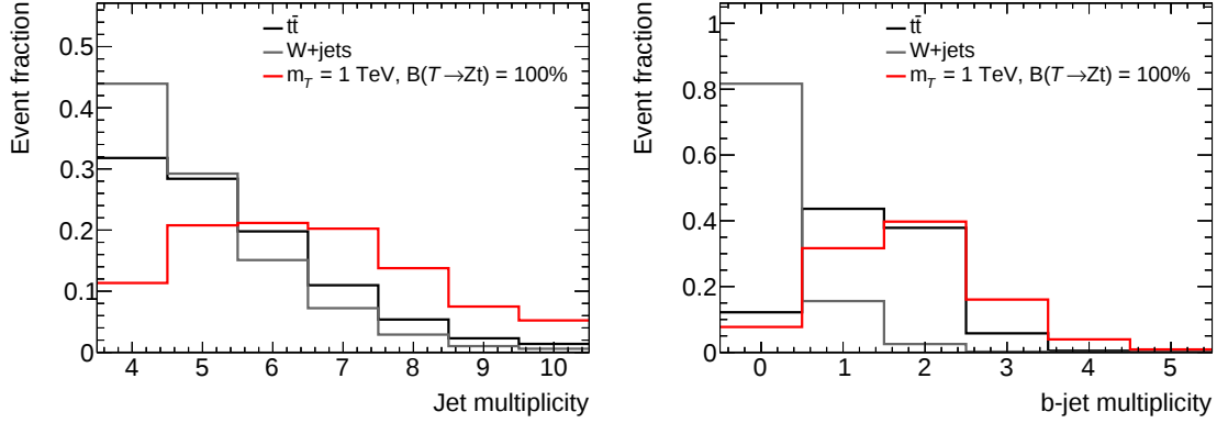
Figure 9.3: Comparison of the jet multiplicity (left) and b -jet multiplicity (right) for the dominant background processes t\bar{t} and W +jets, and for a signal process after the preselection. No requirement on the b -jet multiplicity is set for the right plot.
