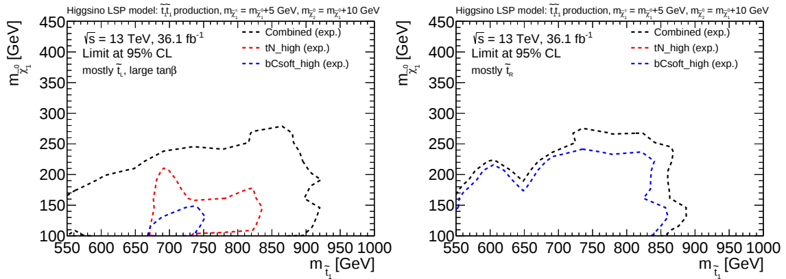
Figure 10.36: Expected 95% CL exclusion contour for the higgsino LSP signal with \tilde{t}_1 \sim \tilde{t}_L and large \tan\beta (left) and \tilde{t}_1 \sim \tilde{t}_R (right) in the m_{\tilde{t}_1} versus m_{\tilde{\chi}_1^0} plane for the individual tN_high and bCsoft_high regions and for the combination.
