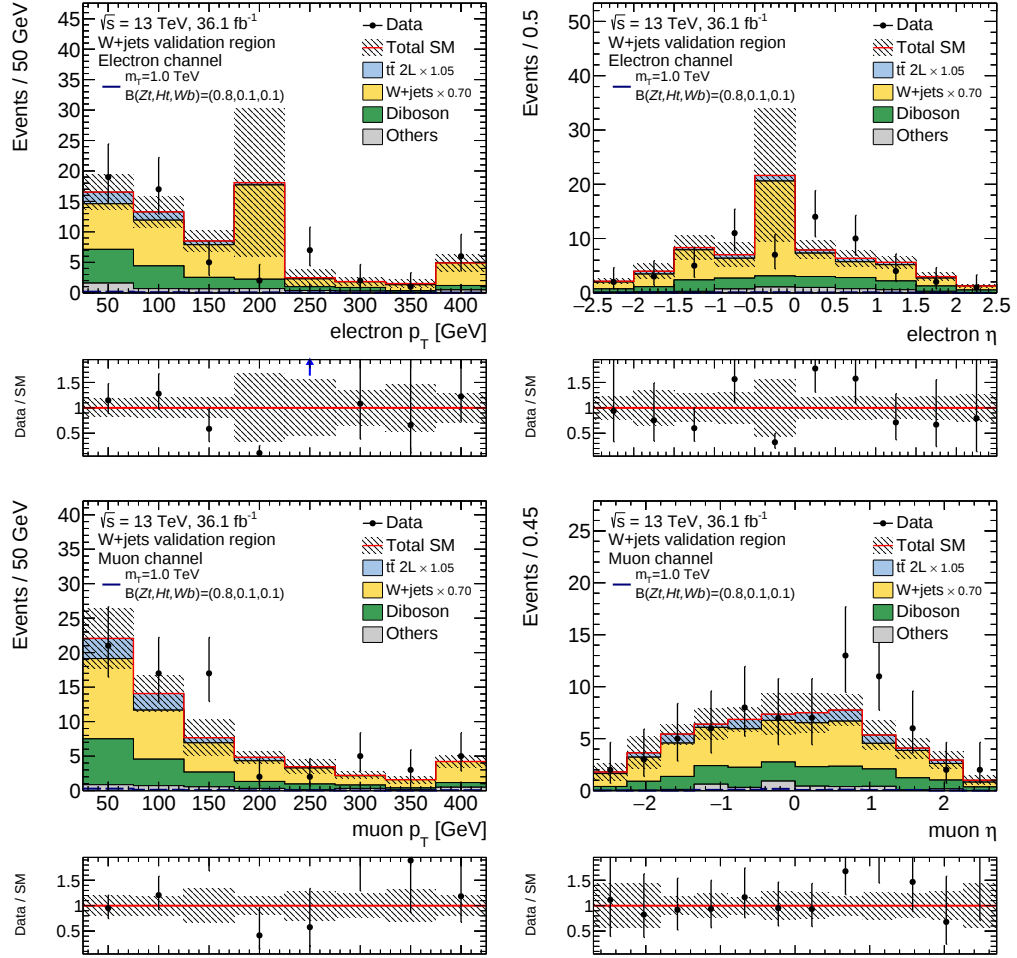
Figure B.18: Distribution of the p_T and the pseudo-rapidity of the signal electron (top) and muon (bottom) in the WVR. The t\bar{t} and W +jets normalisation factors are applied as indicated in the legend. The lower panels show the ratio of the data to the prediction. The error bands include statistical and systematic uncertainties.
