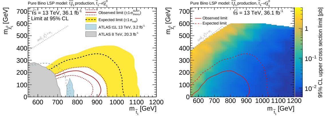
Figure 10.32: Expected and observed 95% CL excluded region (left) and upper cross-section limit (right) in the plane of m_{\tilde{t}_1} versus m_{\tilde{\chi}_1^0} for direct top squark pair production assuming a \tilde{t}_1 \rightarrow t\tilde{\chi}_1^0 decay with 100% branching ratio. The excluded regions from previous publications [2, 61] are shown with grey and blue shaded areas.
