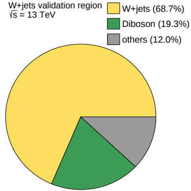
Figure 9.23: Breakdown of the individual SM contributions in the WVR.
