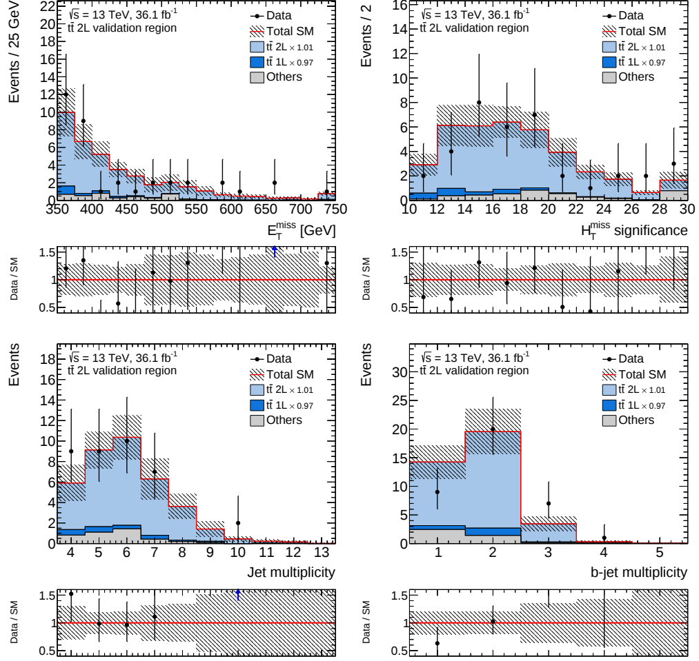
Figure C.13: Distribution of the E_T^{\text{miss}} and the H_{T,\text{sig}}^{\text{miss}} (top) and the jet and b -jet multiplicity (bottom) in the T2LVR. The background normalisation factors are applied as indicated in the legend. The lower panels show the ratio of the data to the prediction. The error bands include statistical and systematic uncertainties.
