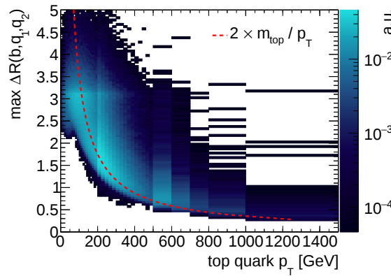
Figure 10.2: Distribution of the maximal separation of the top quark decay products versus the top quark p_T . The red dotted line shows the approximation R(p_T) = 2 \times m/p_T .
