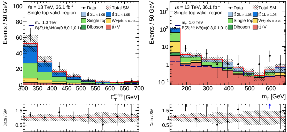
Figure 9.30: Distribution of E_T^{\text{miss}} and m_T in the single top validation region. The t\bar{t} and W +jets normalisation factors are applied as indicated in the legend and the last bin contains overflow events. The lower panels show the ratio of the data to the prediction. The error bands include statistical and systematic uncertainties.
