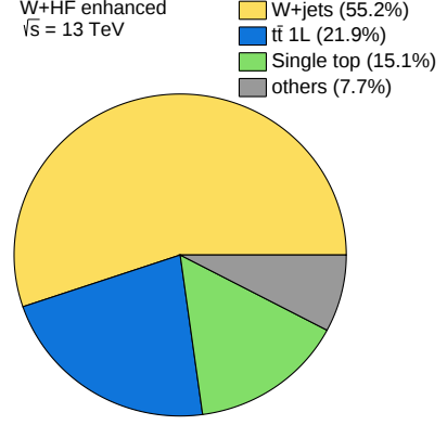
Figure 9.26: Breakdown of the individual SM contributions in the W +HF enhanced selection.
