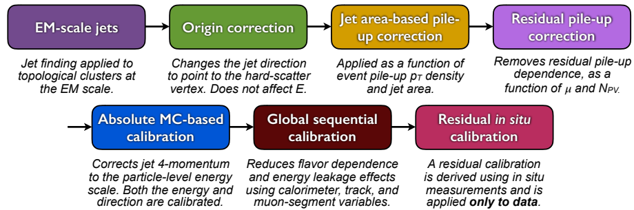
Figure 7.1: Overview of the ATLAS jet calibration scheme [112].
