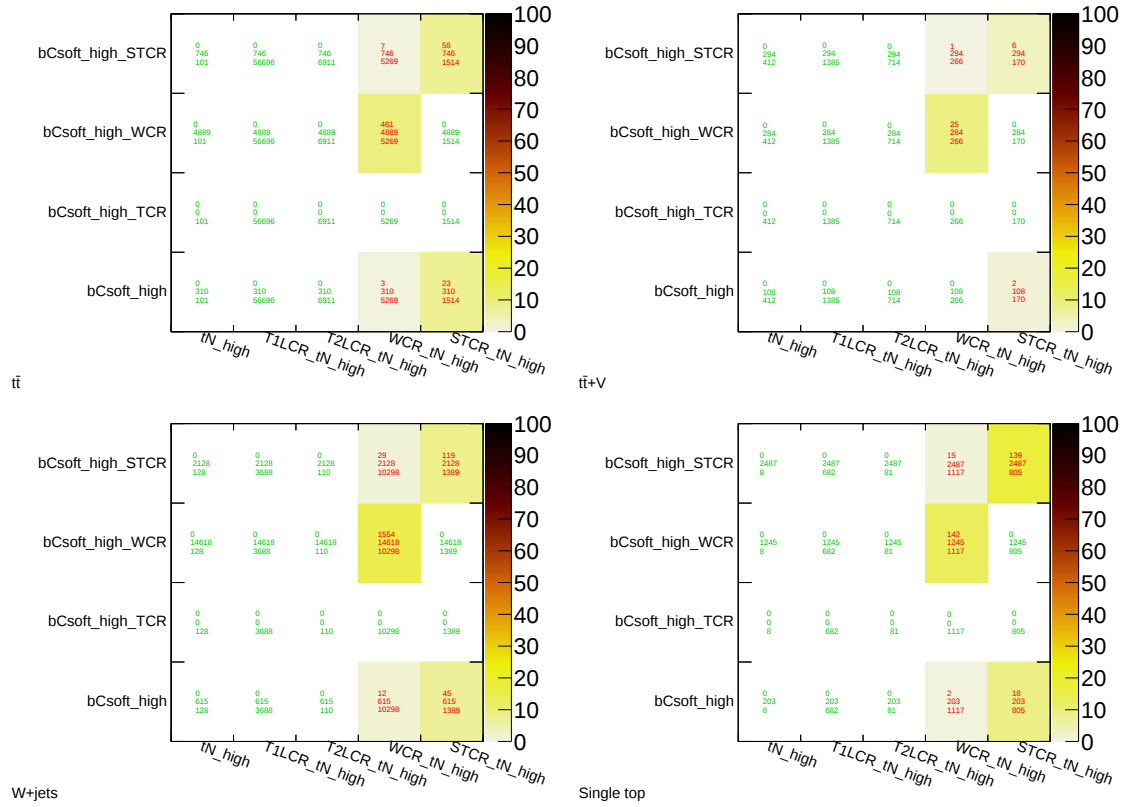
Figure 10.34: Number of simulated events selected by both a bCsoft_high and tN_high associated region for the t\bar{t} (top left), t\bar{t} + V (top right), W +jets (bottom left) and single top (bottom right) backgrounds. The numbers in each bin give the number of overlapping events and the number of events selected by the region indicated on the vertical axis and the horizontal axis, respectively, from top to bottom. The colour scale indicates the fraction of overlapping events in a bin.
