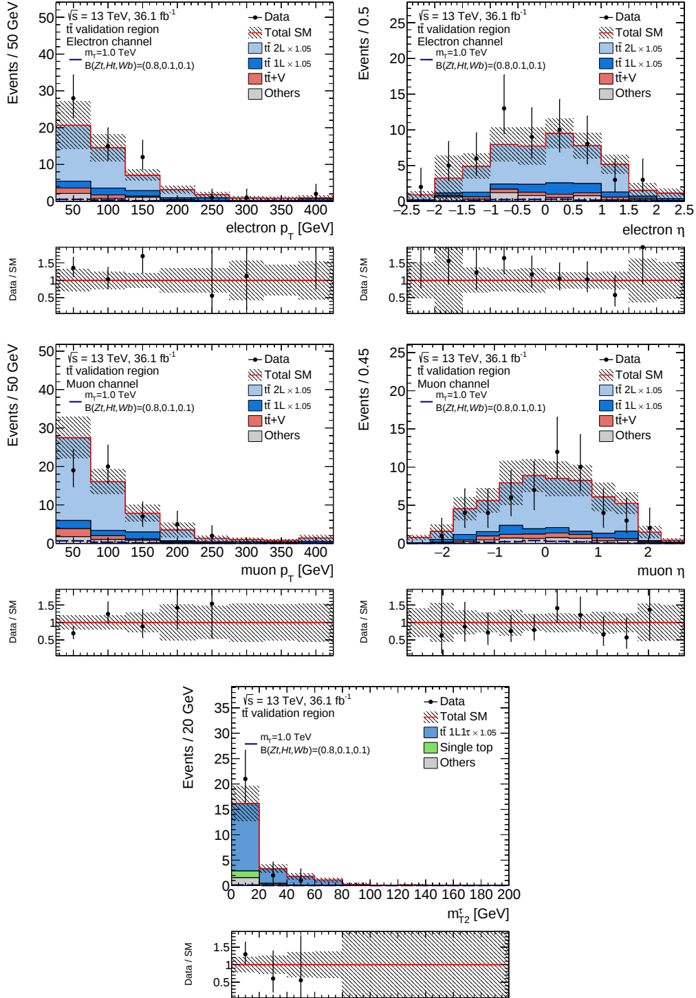
Figure B.15: Distribution of the p_T and the pseudo-rapidity of the signal electron (top) and muon (middle) and the m_{T2}^\tau distribution (bottom, without the m_{T2}^\tau requirement) in the TVR. The t\bar{t} and W +jets normalisation factors are applied as indicated in the legend. The lower panels show the ratio of the data to the prediction. The error bands include statistical and systematic uncertainties.
