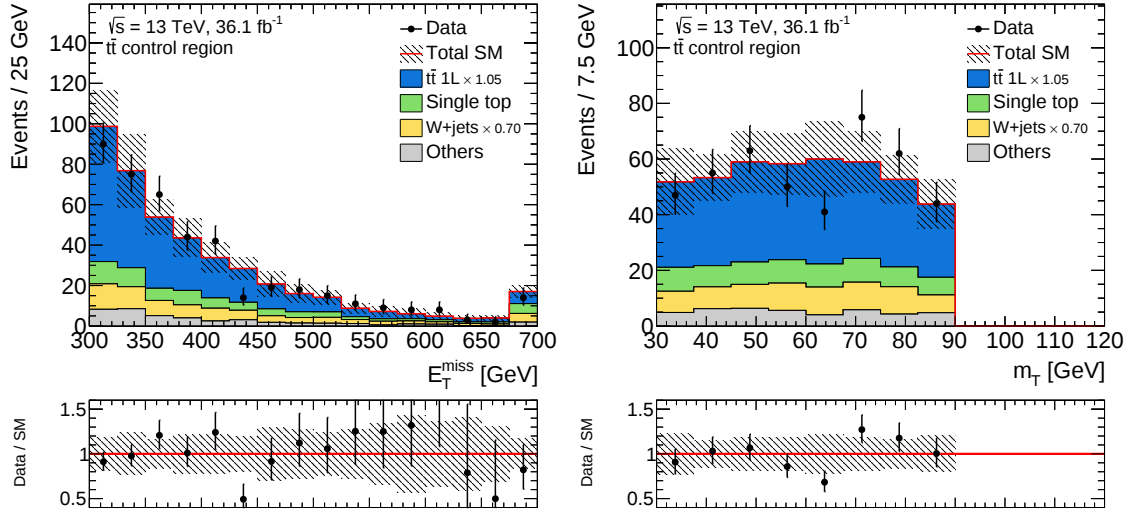
Figure 9.14: Distribution of E_T^{\text{miss}} (left) and m_T (right) in the t\bar{t} control region. The t\bar{t} and W +jets normalisation factors are applied as indicated in the legend and the last bin contains overflow events. The lower panels show the ratio of the data to the prediction. The error bands include statistical and systematic uncertainties.
