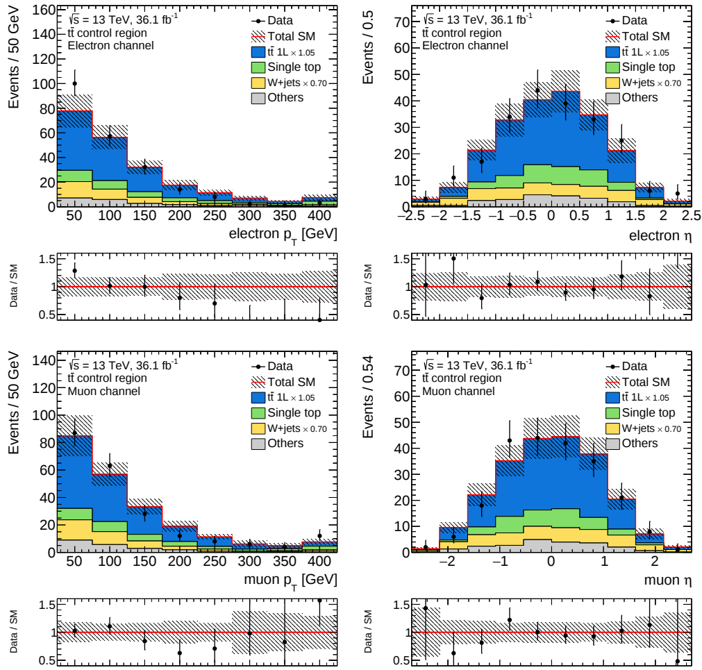
Figure B.9: Distribution of the p_T and the pseudo-rapidity of the signal electron (top) and muon (bottom) in the TCR. The t\bar{t} and W +jets normalisation factors are applied as indicated in the legend. The lower panels show the ratio of the data to the prediction. The error bands include statistical and systematic uncertainties.
