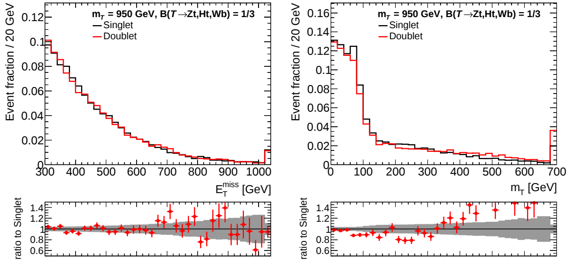
Figure 9.6: Comparison of the E_T^{\text{miss}} and the m_T distribution for a vector-like top quark signal with a mass of m_T = 950 GeV and equal branching ratios into all three decay modes for couplings according to the singlet and the doublet models after the preselection.
