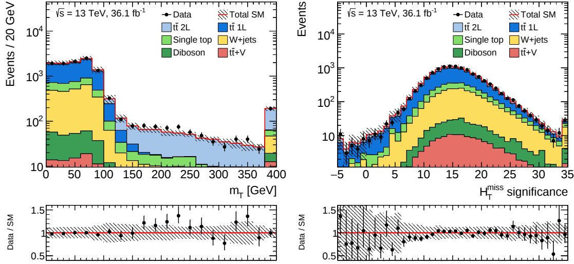
Figure 8.8: Comparison of data and simulation in the m_T and H_{T,\text{sig}}^{\text{miss}} distributions after the preselection. The lower panels show the ratio of the data to the prediction. The error bands include statistical and systematic uncertainties.
