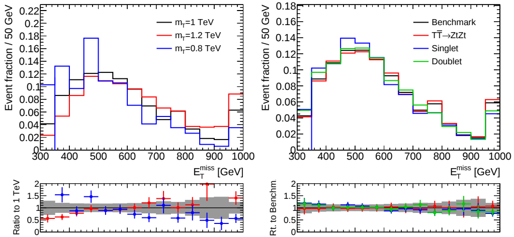
Figure B.4: Comparison of the E_T^{\text{miss}} distribution for different signal masses for \mathcal{B}(T \rightarrow Zt) = 100\% (left) and for different decay modes for m_T = 1 TeV (right) in the signal region. The cut on the displayed variable is not applied, but indicated with a blue vertical line.
