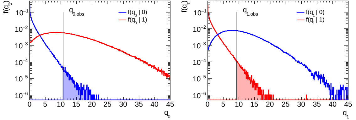
Figure 8.9: Distributions of the q_0 (left) and q_1 (right) test statistics under the background-only hypothesis (blue) and the signal-and-background hypothesis (red). The observed values of the test statistics are taken from the median of f(q_0|1) (left) and f(q_1|0) (right) and the filled areas give the p_0 and p_1 , respectively.
