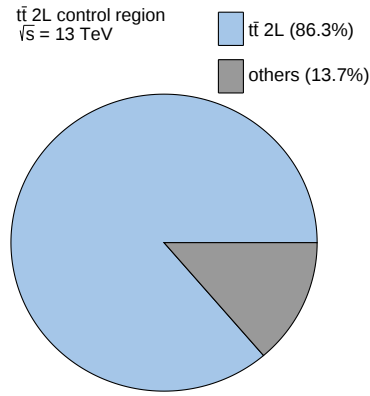
Figure 10.16: Breakdown of the individual SM contributions in the T2LCR.
