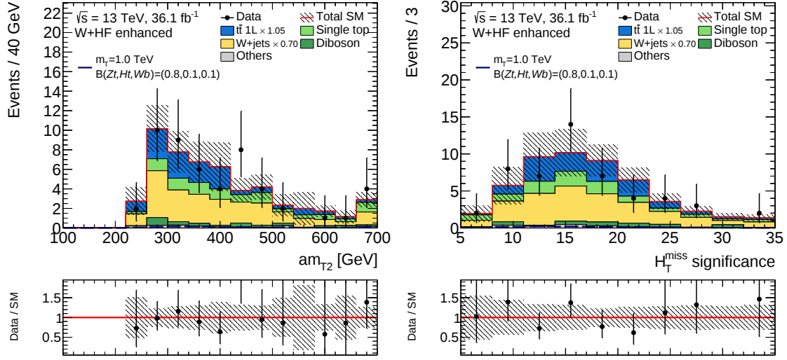
Figure 9.28: Distribution of the am_{T2} and the H_{T,\text{sig}}^{\text{miss}} in the W +HF enhanced region. The t\bar{t} and W +jets normalisation factors are applied as indicated in the legend and the last bin contains overflow events. The lower panels show the ratio of the data to the prediction. The error bands include statistical and systematic uncertainties.
