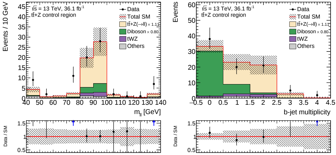
Figure 10.25: Distribution of the m_{\ell\ell} (left) and the b -jet multiplicity in the t\bar{t} + Z(\rightarrow \ell\ell) control region, without the requirement on the displayed variable. The t\bar{t} + V and diboson normalisation factors are applied as indicated in the legend. The lower panels show the ratio of the data to the prediction. The errors bands include statistical and systematic uncertainties.
