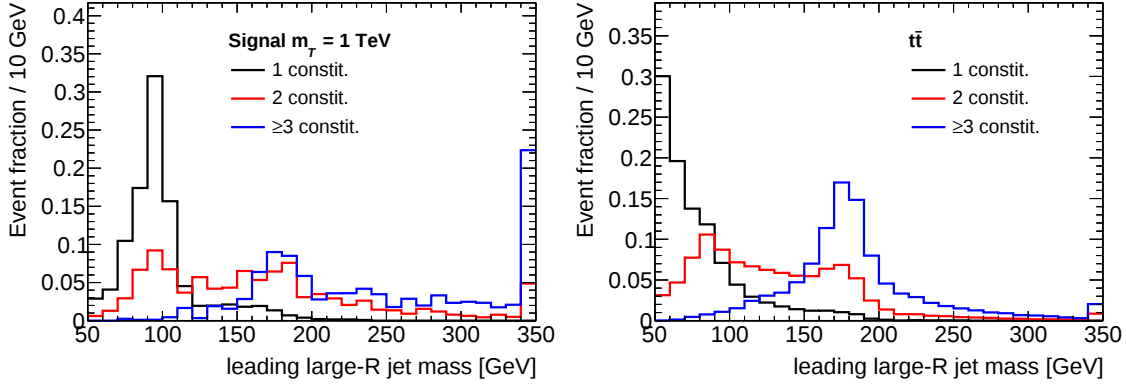
Figure 9.1: Mass of the leading large- R jet for different number of constituent jets for a benchmark signal (left) and for t\bar{t} events (right).
