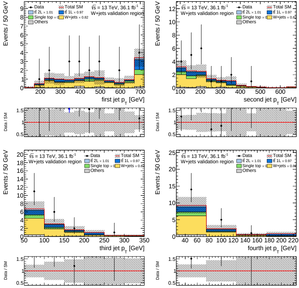
Figure C.20: Distribution of the jet p_T in the WVR. The background normalisation factors are applied as indicated in the legend. The lower panels show the ratio of the data to the prediction. The error bands include statistical and systematic uncertainties.
