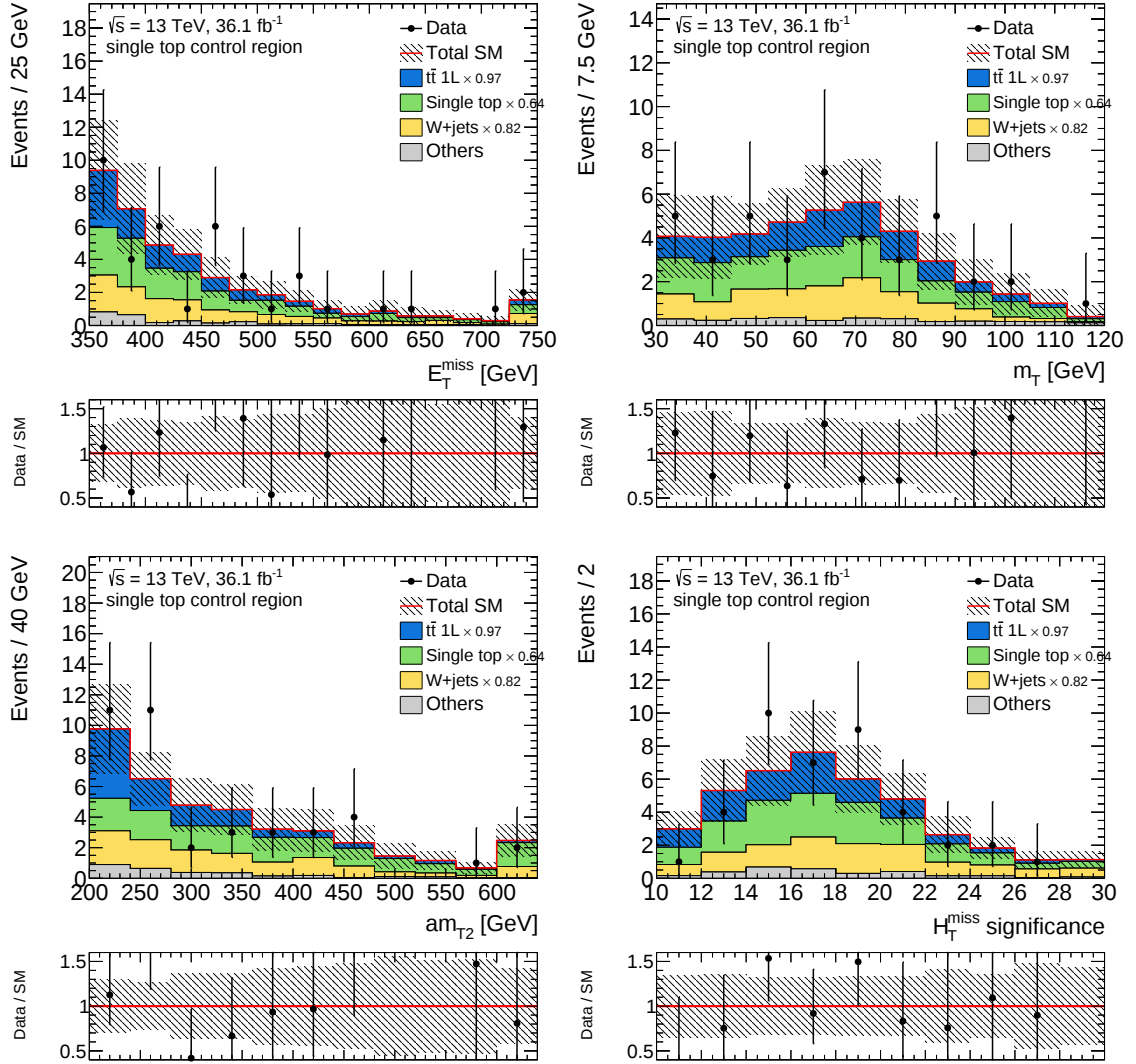
Figure 10.24: Distribution of E_T^{\text{miss}} (top left), m_T (top right), am_{T2} (bottom left) and H_T^{\text{miss}} (bottom right) in the single top control region. The background normalisation factors are applied as indicated in the legend and the last bin contains overflow events. The lower panels show the ratio of the data to the prediction. The error bands include statistical and systematic uncertainties.
