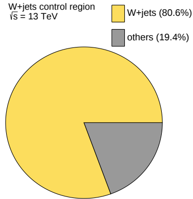
Figure 9.16: Breakdown of the individual SM contributions in the WCR.
