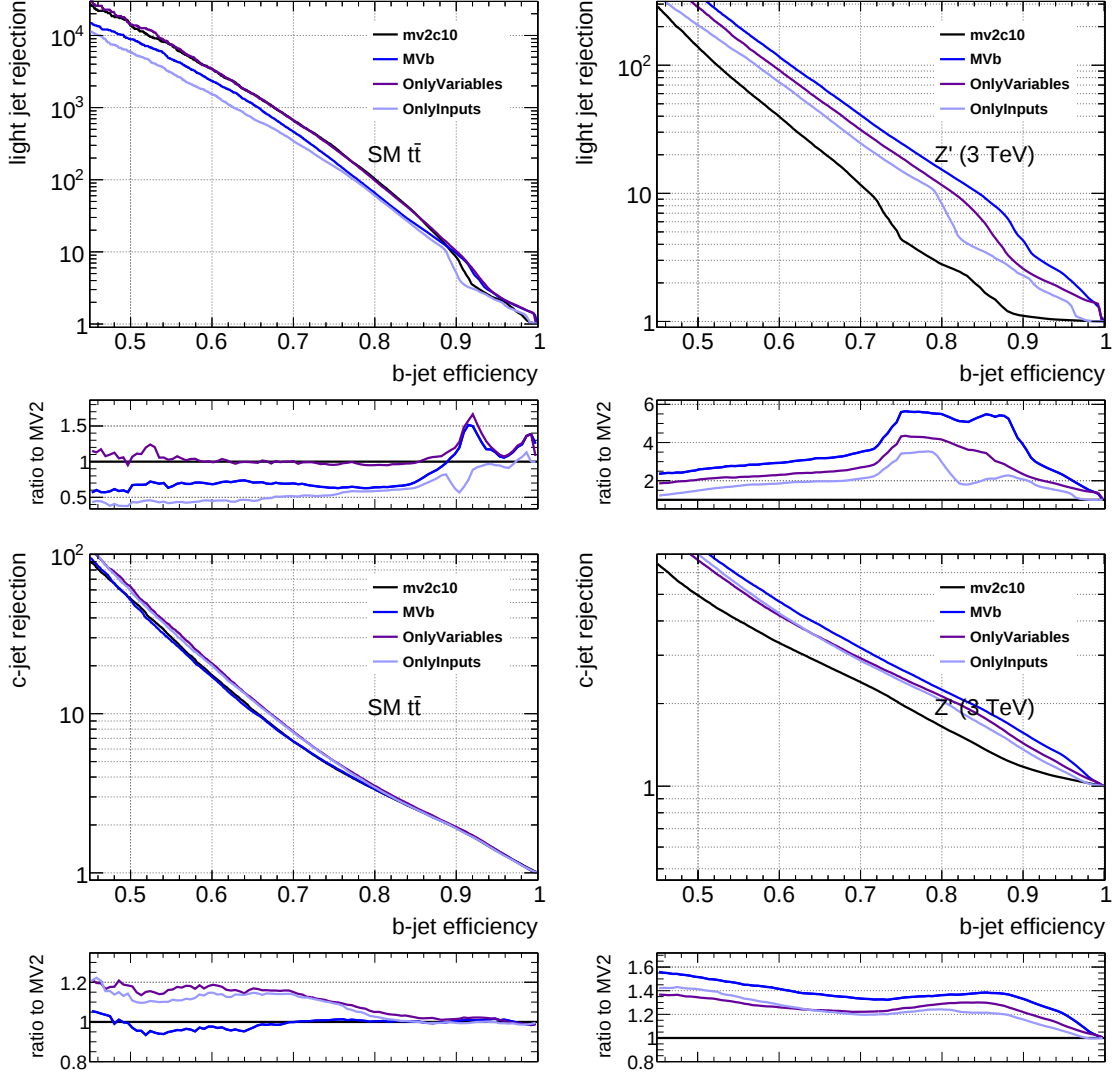
Figure A.6: Light flavour jet rejection (top) and c -jet rejection (bottom) as a function of the b -tagging efficiency for multiple training options based on MV2 and additional variables, evaluated on an inclusive t\bar{t} sample (left) and on Z' \rightarrow t\bar{t} events (right). The black line shows the MV2 tagger as the reference, the purple line the performance for MV2 with additional variables and the light blue line the performance for MV2 trained on the dense environment inputs. The blue line shows the performance of the full MVb training.
