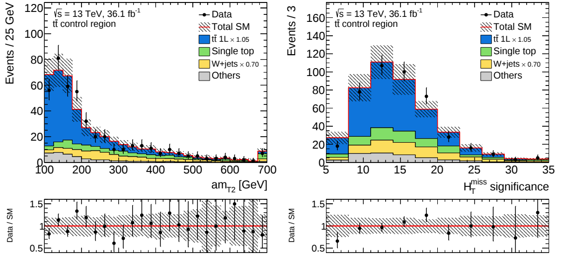
Figure 9.15: Distribution of am_{T2} (left) and H_T^{\text{miss, sig}} (right) in the t\bar{t} control region. The t\bar{t} and W +jets normalisation factors are applied as indicated in the legend and the last bin contains overflow events. The lower panels show the ratio of the data to the prediction. The error bands include statistical and systematic uncertainties.
