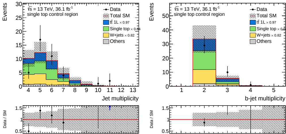
Figure C.10: Distribution of the jet and the b -jet multiplicity in the STCR. The background normalisation factors are applied as indicated in the legend. The lower panels show the ratio of the data to the prediction. The error bands include statistical and systematic uncertainties.
