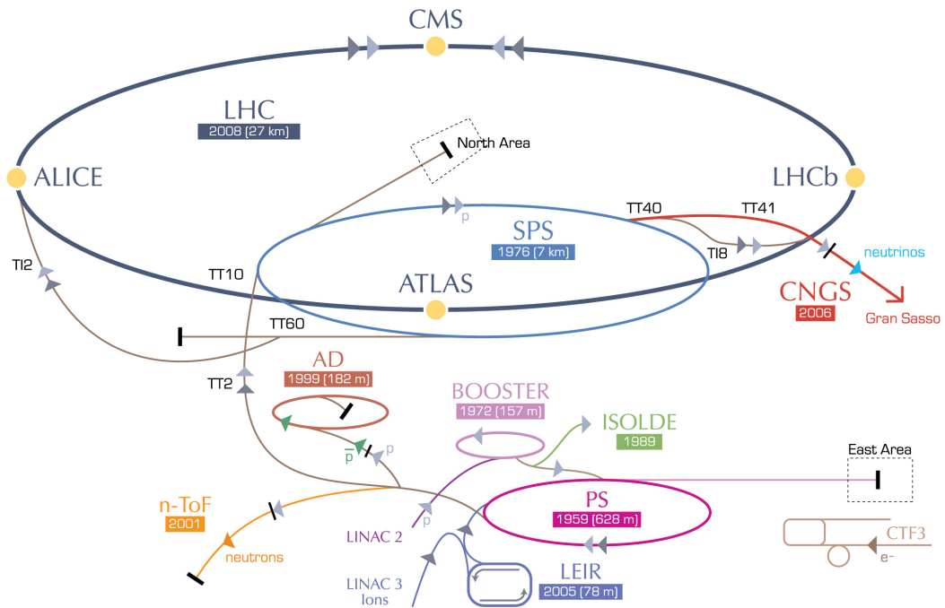
Figure 5.1: Schematic view of the CERN accelerator complex [86].
