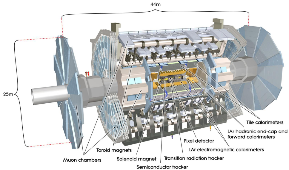
Figure 6.1: Overview of the ATLAS detector, with the different sub-detectors and the magnet systems [90].
