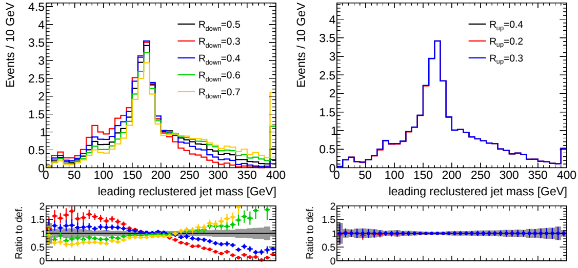
Figure 10.7: Distribution of the mass of the leading top candidate for different parameters in the algorithm, varying R_{\text{down}} (left) and R_{\text{up}} (right). Only one parameter is varied at a time, with the first setting in the list being the default value.
