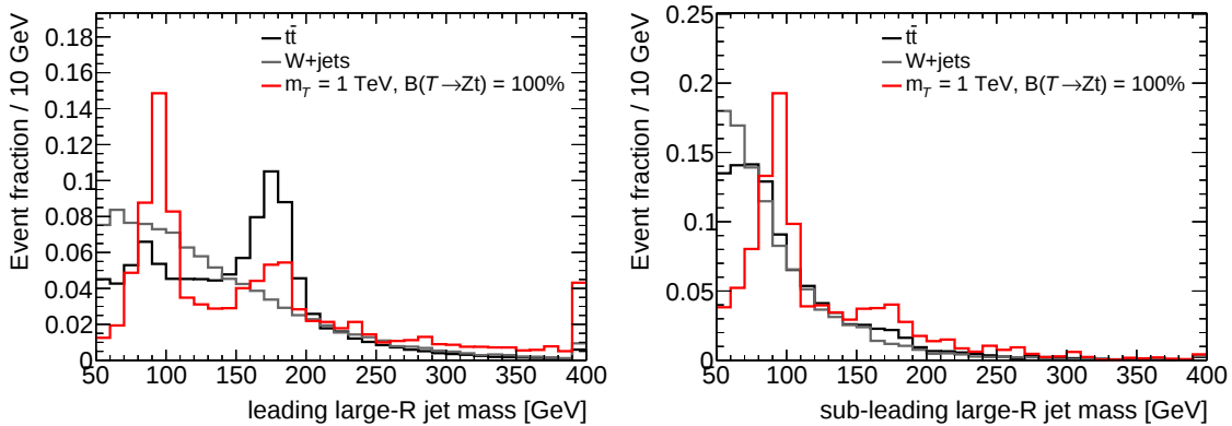
Figure 9.2: Comparison of the mass of the leading (left) and the sub-leading large- R jet (right) for the dominant background processes t\bar{t} and W +jets, and for a signal process after the preselection.
