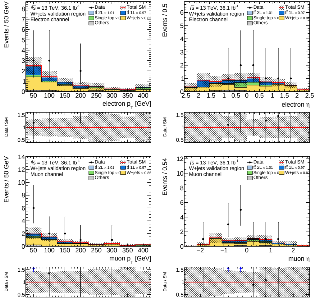
Figure C.21: Distribution of the electron (top) and muon (bottom) p_T and \eta in the WVR. The background normalisation factors are applied as indicated in the legend. The lower panels show the ratio of the data to the prediction. The error bands include statistical and systematic uncertainties.
