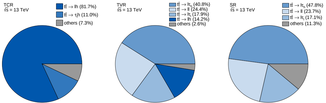
Figure 9.22: Breakdown of the t\bar{t} decay mode into hadrons, h , electrons or muons, l , hadronically decaying \tau leptons, \tau_h or leptonically decaying \tau leptons, \tau_l , in the TCR (left), TVR (middle) and SR (right).
