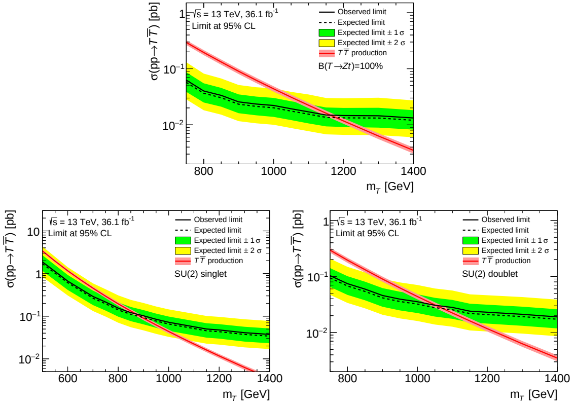
Figure 9.33: Observed and expected 95% CL upper limit on the cross-section times branching ratio for VLT pair production as a function of the T mass for \mathcal{B}(T \rightarrow Zt) = 100\% (top) and for branching ratios according to the singlet model (bottom left) and the doublet model (bottom right). Contributions from the X or B quark in the (X^{5/3}, T) or (T, B) doublet models are neglected, leading to conservative limits. The thickness of the theory curve represents the theoretical uncertainty from PDFs, scale and the strong coupling constant \alpha_s .
