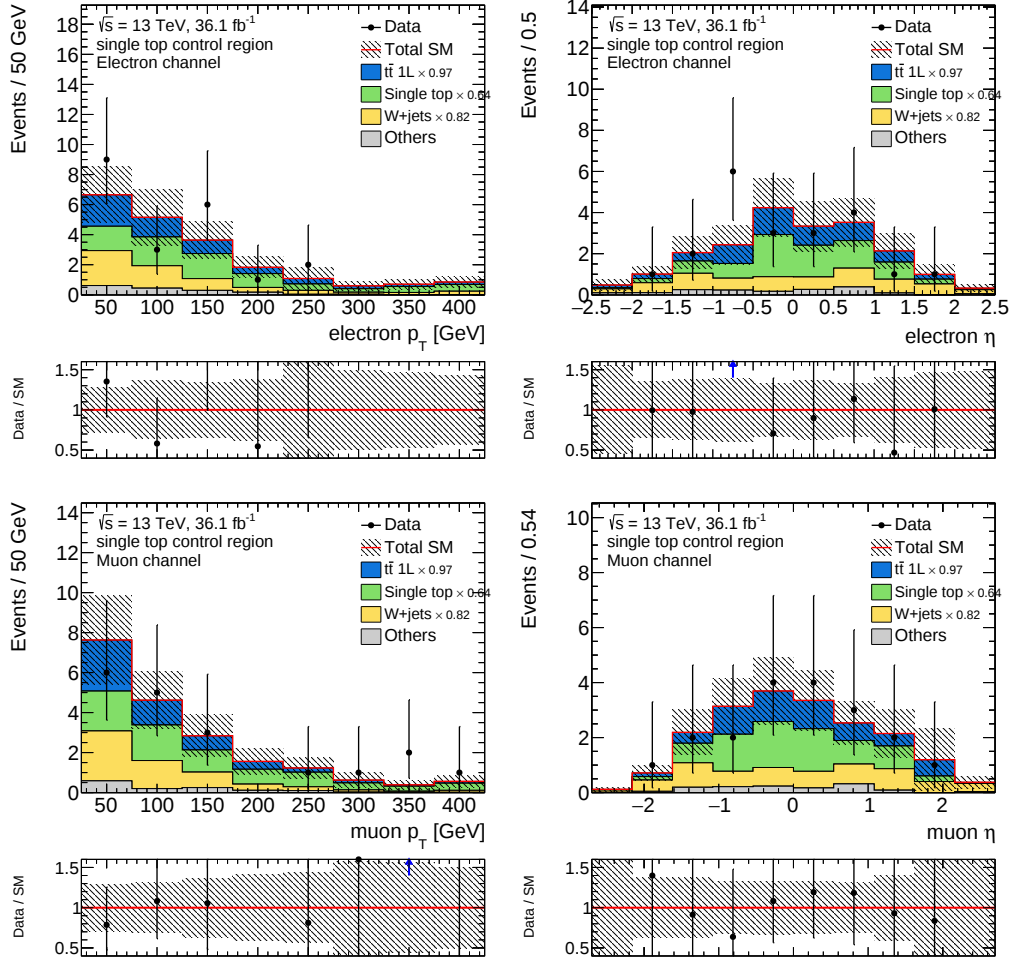
Figure C.12: Distribution of the electron (top) and muon (bottom) p_T and \eta in the STCR. The background normalisation factors are applied as indicated in the legend. The lower panels show the ratio of the data to the prediction. The error bands include statistical and systematic uncertainties.
