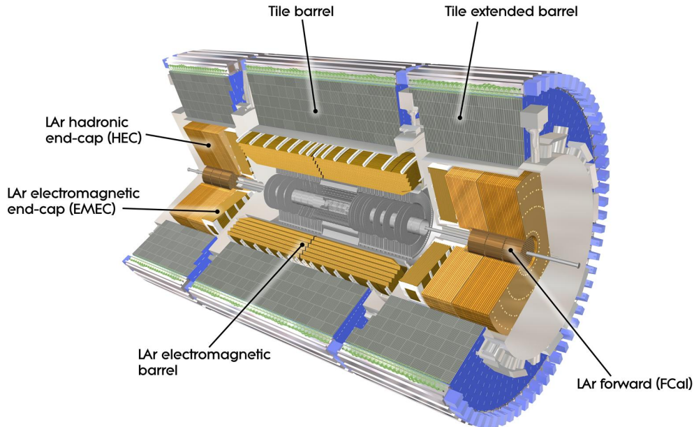
Figure 6.3: Schematic view of the ATLAS calorimeters [95].
