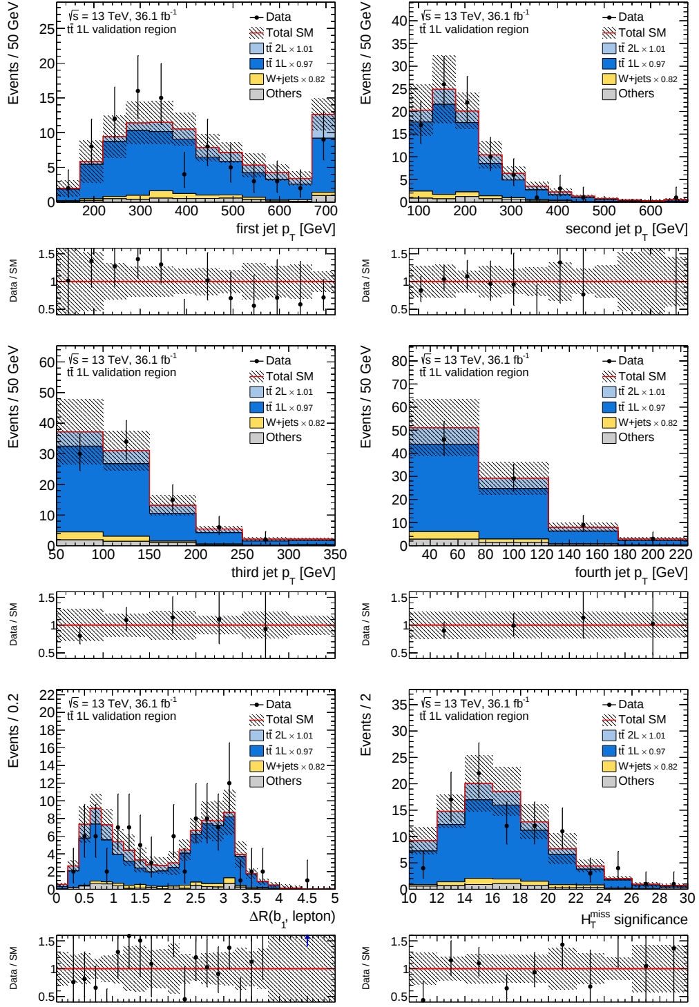
Figure C.17: Distribution of the jet p_T (top, middle) and the \Delta R(b, \ell) and the H_T^{\text{miss}} (bottom) in the T1LVR. The background normalisation factors are applied as indicated in the legend. The lower panels show the ratio of the data to the prediction. The error bands include statistical and systematic uncertainties.
