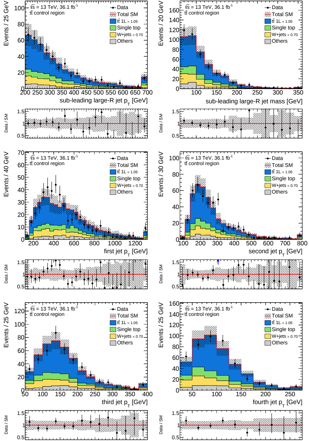
Figure B.8: Distribution of the p_T and the mass of the sub-leading large- R jet (top), the p_T of the leading and sub-leading jet (middle) and the p_T of the third and fourth leading jet (bottom) in the TCR. The t\bar{t} and W+jets normalisation factors are applied as indicated in the legend. The lower panels show the ratio of the data to the prediction. The error bands include statistical and systematic uncertainties.
