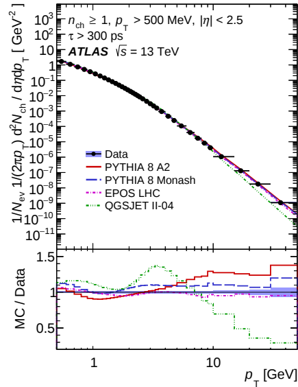
Figure 4.3: Charged-particle multiplicity as a function of the p_T in minimum bias events [1].
