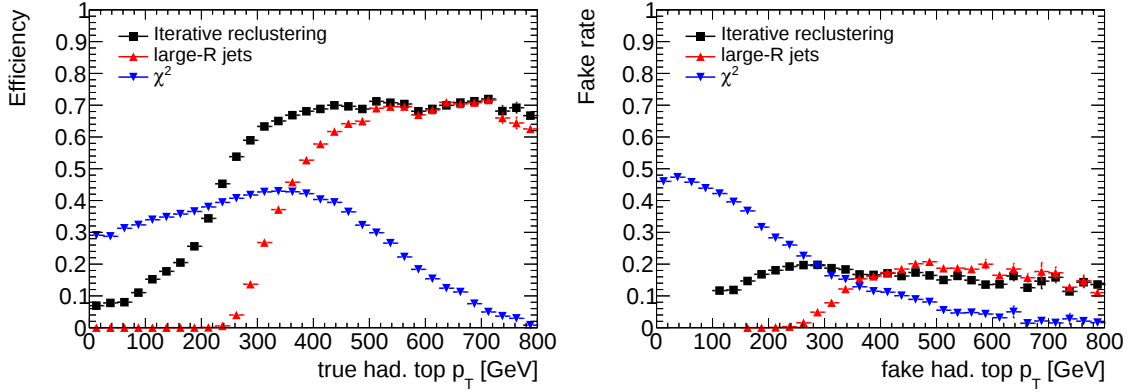
Figure 10.6: Efficiency of reconstructing exactly the hadronic top decay as a function of the hadronic top p_T (left) and the fake rate as a function of the reconstructed top p_T (right) for the recursive reclustering algorithm, for R = 1.0 large- R jets and for the \chi^2 minimisation.
