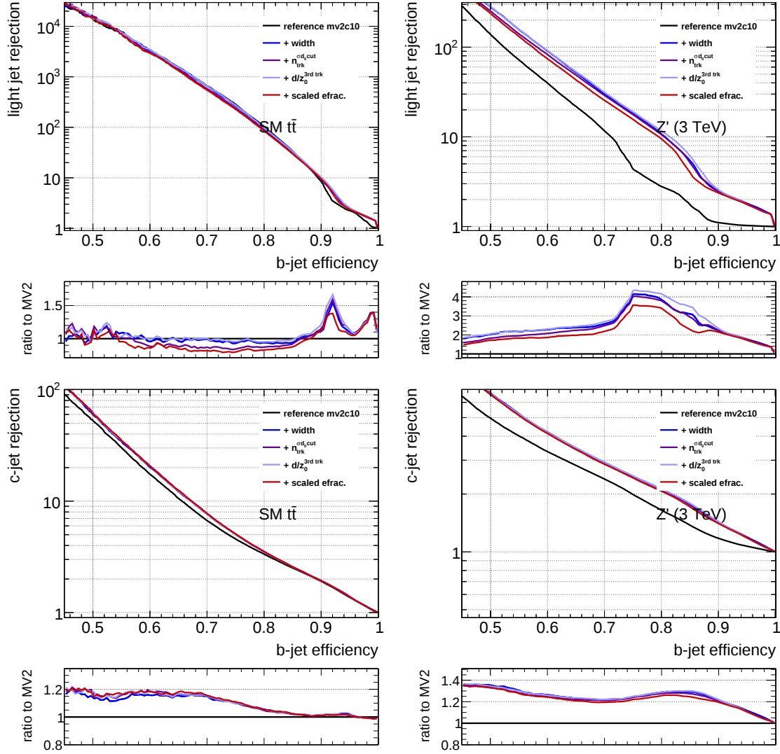
Figure A.2: Light flavour jet rejection (top) and c -jet rejection (bottom) as a function of the b -tagging efficiency for multiple training options based on MV2 and additional variables, evaluated on an inclusive t\bar{t} sample (left) and on Z' \rightarrow t\bar{t} events (right). The black line shows the reference MV2 training, the coloured lines show the results for subsequently adding additional variables.
