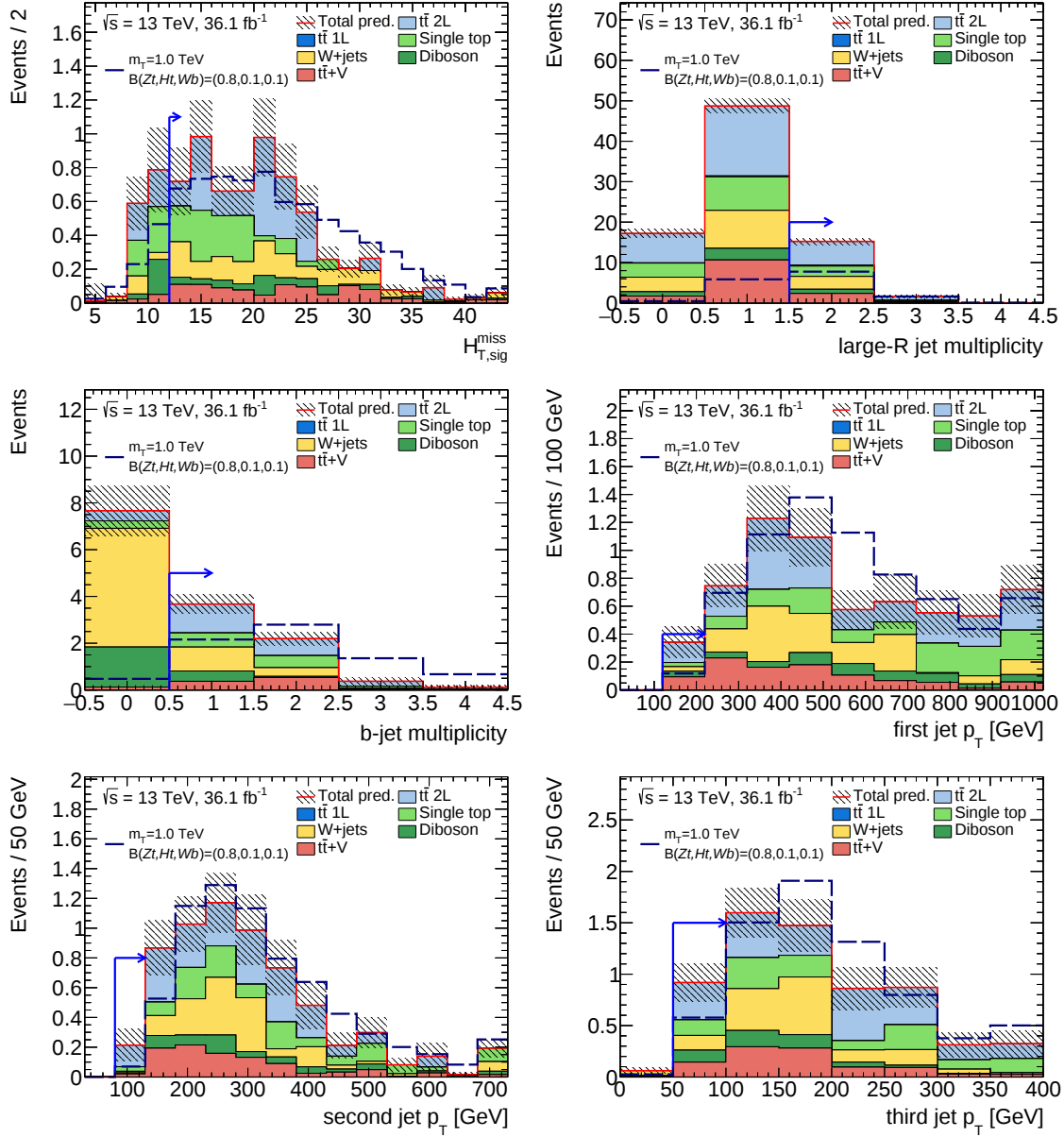
Figure 9.12: The H_{T,\text{sig}}^{\text{miss}} distribution, the large- R jet and b -jet multiplicities, as well as the p_T of the leading three jets in the signal region. The requirement on the displayed distribution, as indicated by the vertical line, is not applied. All large- R jets fulfilling the reconstruction requirements of p_{T,\text{jet}} > 150 \text{ GeV} and m_{\text{Jet}} > 50 \text{ GeV} are counted in the large- R jet multiplicity.
