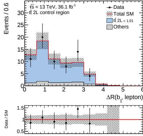
Figure C.3: Distribution of the \Delta R(b, \ell) in the T2LCR. The background normalisation factors are applied as indicated in the legend. The lower panels show the ratio of the data to the prediction. The error bands include statistical and systematic uncertainties.
