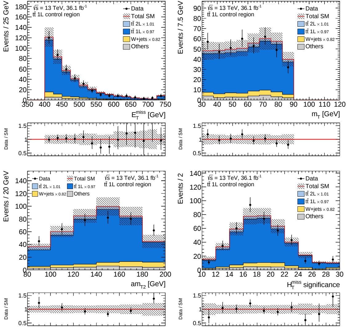
Figure 10.19: Distribution of E_T^{\text{miss}} (top left), m_T (top right), am_{T2} (bottom left) and H_{T,\text{sig}}^{\text{miss}} (bottom right) in the semi-leptonic t\bar{t} control region. The background normalisation factors are applied as indicated in the legend and the last bin contains overflow events. The lower panels show the ratio of the data to the prediction. The error bands include statistical and systematic uncertainties.
