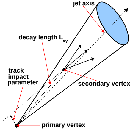
Figure 7.2: Sketch of the b -hadron decay in a jet, with the most important variables indicated [117].
