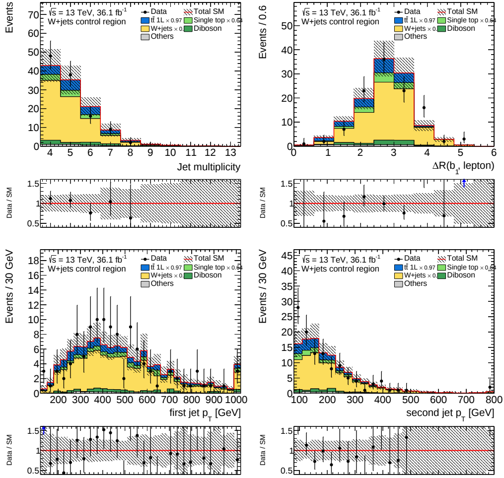
Figure C.7: Distribution of the jet multiplicity and the \Delta R(b, \ell) (top) and the first and second jet p_T (bottom) in the WCR. The background normalisation factors are applied as indicated in the legend. The lower panels show the ratio of the data to the prediction. The error bands include statistical and systematic uncertainties.
