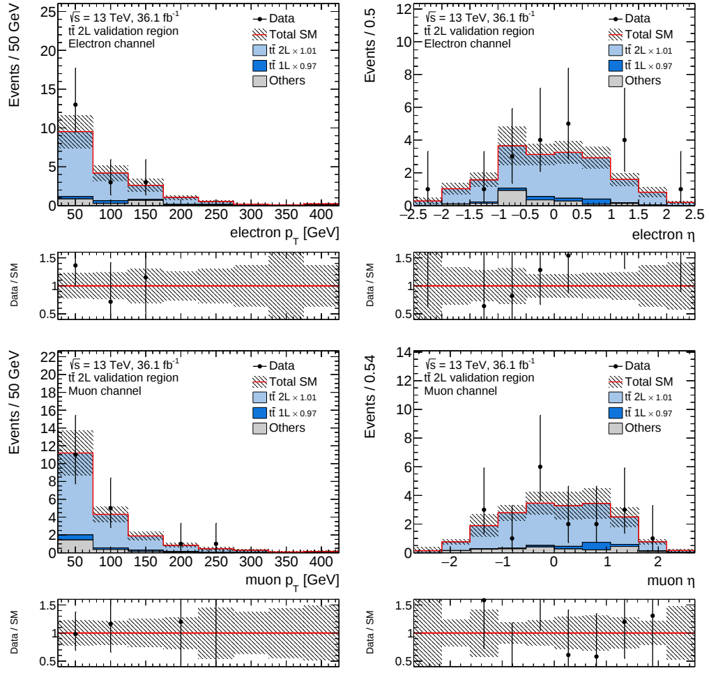
Figure C.15: Distribution of the electron (top) and muon (bottom) p_T and \eta in the T2LVR. The background normalisation factors are applied as indicated in the legend. The lower panels show the ratio of the data to the prediction. The error bands include statistical and systematic uncertainties.
