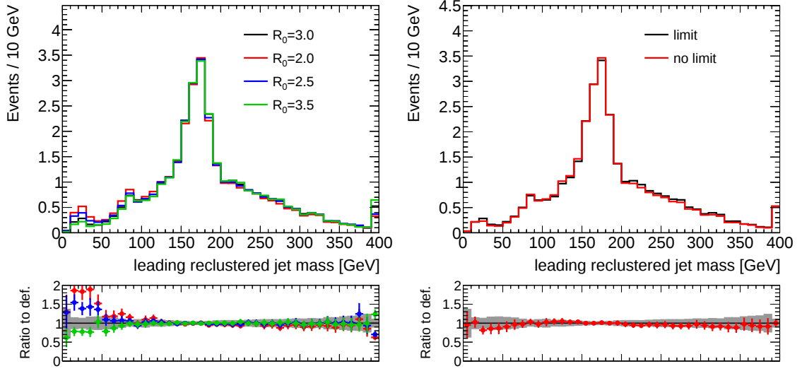
Figure 10.8: Distribution of the mass of the leading top candidate for different parameters in the algorithm, varying R_0 (left) or the limit on the minimal size of the new radius (right). Only one parameter is varied at a time, with the first setting in the list being the default value.
