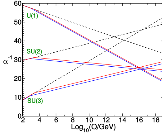
Figure 3.1: Evolution of the inverse coupling constants with energy in the SM (dashed lines) and in the MSSM (solid lines) for two common particle masses of 750 GeV (blue) and 2.5 TeV (red) [54].
