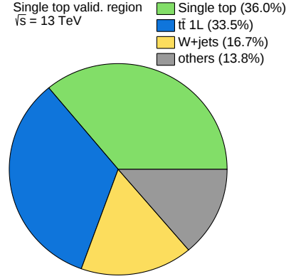
Figure 9.29: Breakdown of the individual SM contributions in the STVR.
