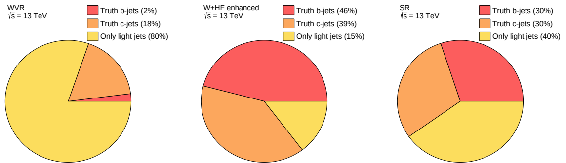
Figure 9.25: Breakdown of the flavour components of the W +jets process in the WVR (left), the cross-check selection (middle) and the SR (right).
