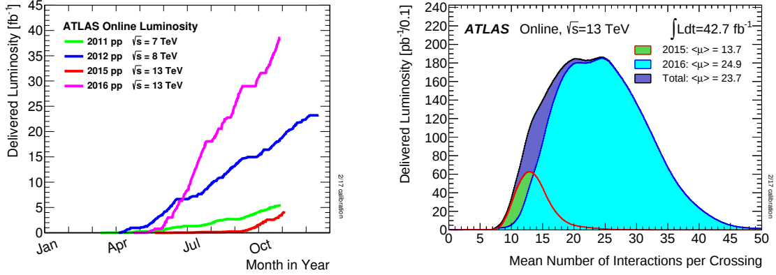
Figure 5.2: Integrated luminosity delivered to ATLAS versus the day (left) and the luminosity weighted distribution of the mean number of interactions per bunch crossing for 2015 and 2016 (right) [88, 89].
