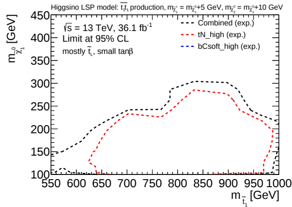
Figure C.23: Expected 95% CL exclusion contour for the higgsino LSP signal with \tilde{t}_1 \sim \tilde{t}_L and small \tan\beta in the m_{\tilde{t}_1} versus m_{\tilde{\chi}_1^0} plane for the individual tN_high and bCsoft_high regions and for the combination.
