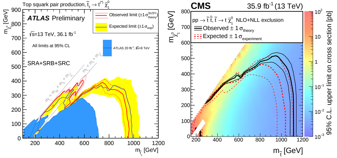
Figure 10.33: Expected and observed 95% CL excluded region in the plane of m_{\tilde{t}_1} versus m_{\tilde{\chi}_1^0} for direct top squark pair production assuming a \tilde{t}_1 \rightarrow t \tilde{\chi}_1^0 decay with 100% branching ratio for the ATLAS direct stop search in the fully hadronic channel [163] (left) and the CMS search in the 1 lepton channel [164] (right).
