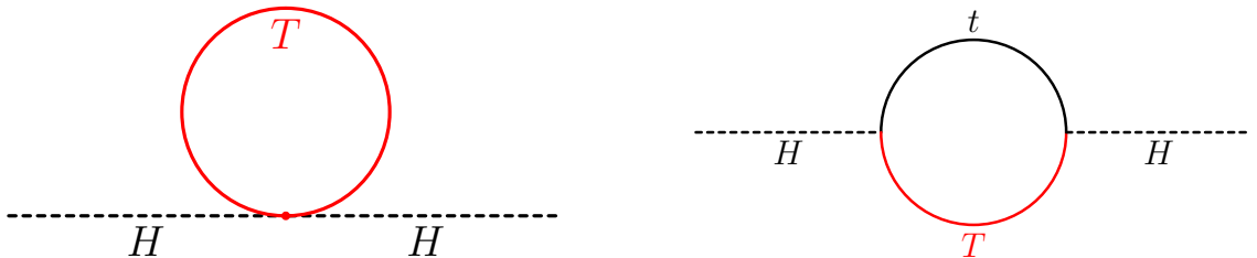
Figure 2.1: Radiative corrections to the Higgs mass involving a vector-like T quark.
