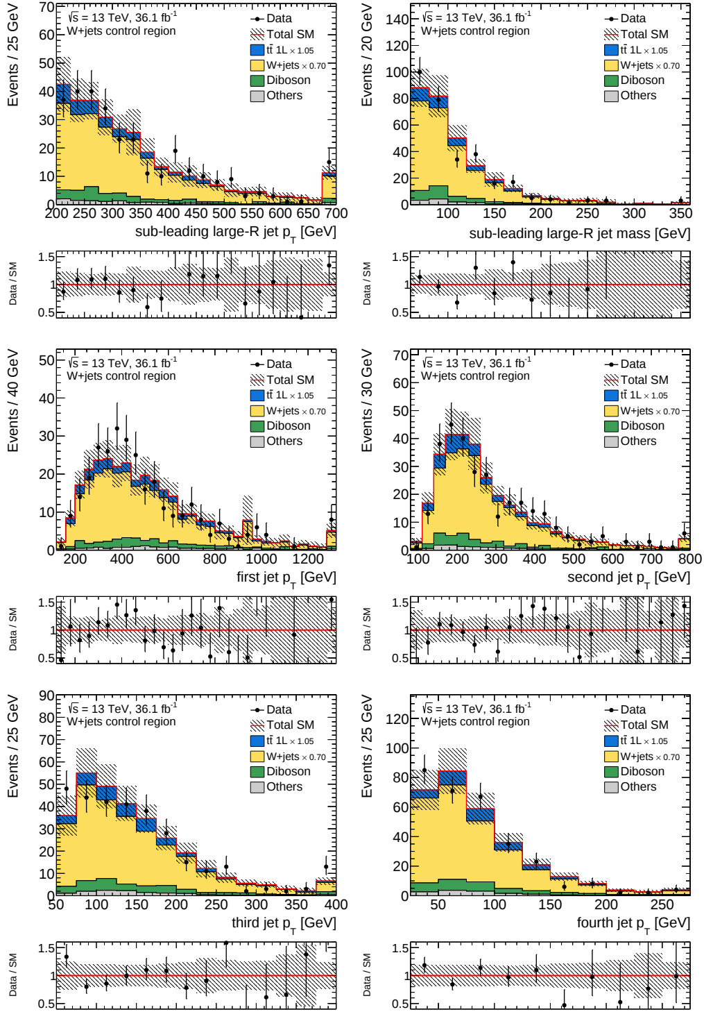
Figure B.11: Distribution of the p_T and the mass of the sub-leading large- R jet (top), the p_T of the leading and sub-leading jet (middle) and the p_T of the third and fourth leading jet (bottom) in the WCR. The t\bar{t} and W+jets normalisation factors are applied as indicated in the legend. The lower panels show the ratio of the data to the prediction. The error bands include statistical and systematic uncertainties.
