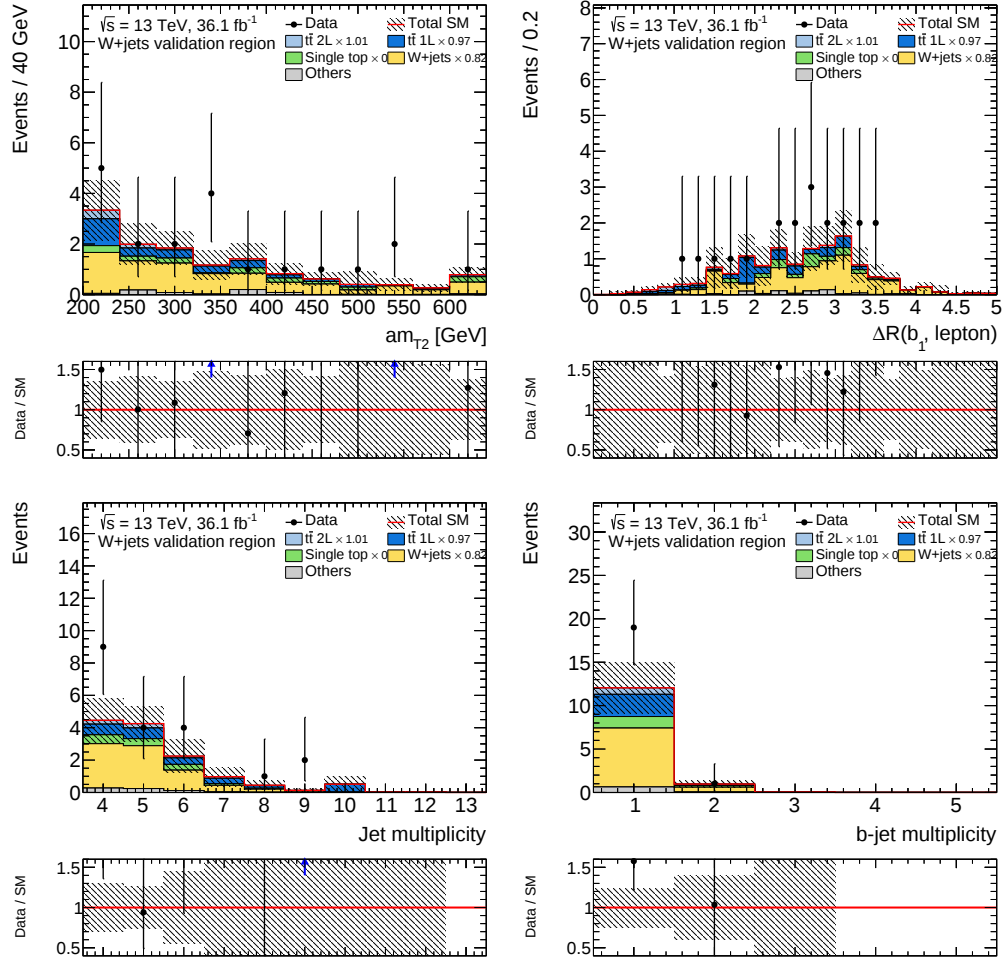
Figure C.19: Distribution of the am_{T2} and the \Delta R(b, \ell) (top) and the jet and the b -jet multiplicity (bottom) in the WVR. The background normalisation factors are applied as indicated in the legend. The lower panels show the ratio of the data to the prediction. The error bands include statistical and systematic uncertainties.
