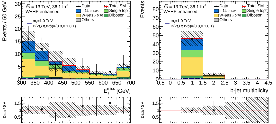
Figure 9.27: Distribution of the E_T^{\text{miss}} and the b -jet multiplicity in the W +HF enhanced region. The t\bar{t} and W +jets normalisation factors are applied as indicated in the legend and the last bin contains overflow events. The lower panels show the ratio of the data to the prediction. The error bands include statistical and systematic uncertainties.
