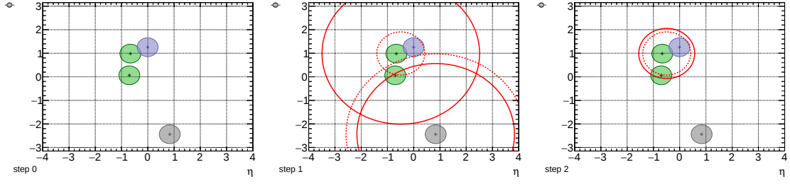
Figure 10.3: Illustrative display of the jets in the \eta \times \phi plane for one event in the different steps of the hadronic top reconstruction algorithm. The b -jet of the hadronic top decay is marked in blue, the light jets from the top decay in green and other jets in the event are shown in grey. The actual radius of the candidates is shown with red solid lines, the “optimal” radius according to the p_T with red dashed lines.
