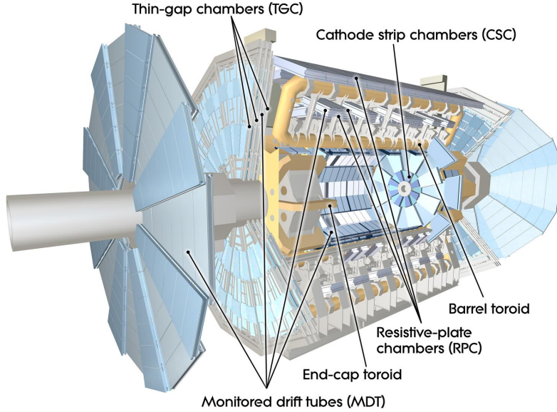
Figure 6.4: Schematic view of the ATLAS muon spectrometer [99].
