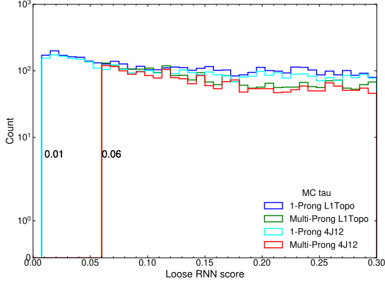
(g) RNN score of 1-prong ( \text{RNN}_{1p}^{\text{loose}} ) and multi-prong ( \text{RNN}_{mp}^{\text{loose}} ) \tau leptons matched to \text{HLT}_{\text{L1Topo}} and \text{HLT}_{4J12} chains with loose working point.
