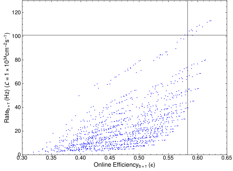
Figure C.4: Efficiencies and rates of the \text{HLT}_{b+\tau} chain generated by varying the thresholds of different trigger parameter. The intersection point corresponds to the rate and efficiency of the default trigger parameters of the \text{HLT}_{b+\tau} chain.
