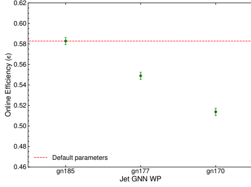
(k) Correlation between efficiency and GN1 WP requirement of the jet.
