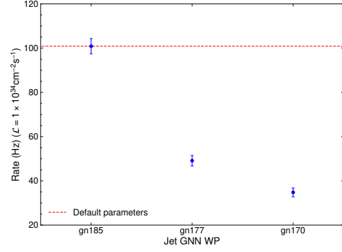
(l) Correlation between rate and GN1 WP requirement of the jet.
