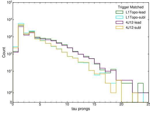
(i) \tau_{\text{prong}} distribution with objects matched to \text{HLT}_{\text{L1Topo}} and \text{HLT}_{4J12} chains in each event.
