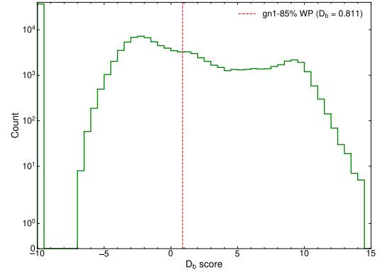
(j) D_b score of all HLT jets calculated using Eq. (4.1).
