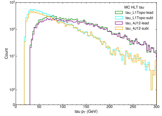
(d) \tau_{p_T} spectra with objects matched to \text{HLT}_{\text{L1Topo}} and \text{HLT}_{4\text{J12}} chains in each event.
