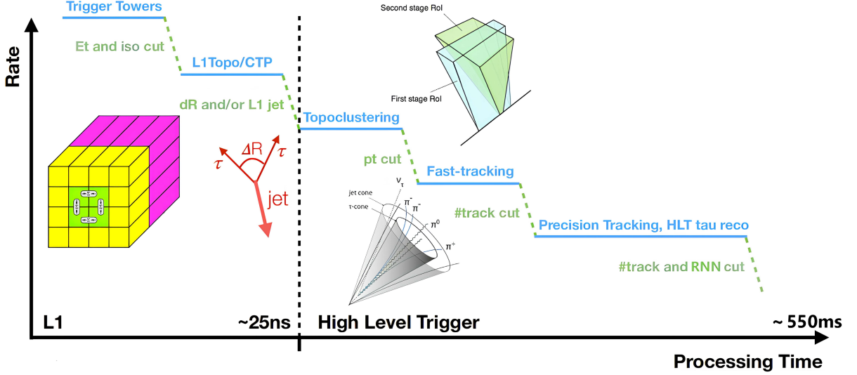
Figure 4.4: Different stages of reconstruction and selection, at different trigger levels for \tau_{\text{had}} objects. Adapted from graphic by © Serhat Örddek, CC BY 2.5, PhD thesis .
