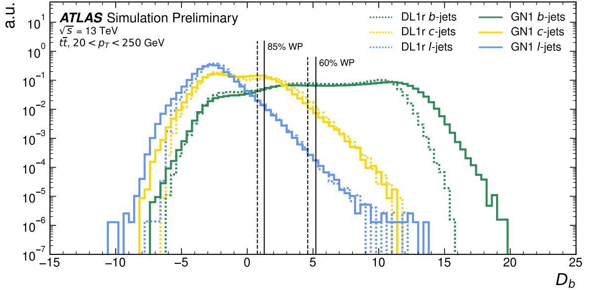
Figure 4.10: Comparison between the DL1r and GN1 bt tag discriminant D_b for jets in the t\bar{t} sample. The 85% WP and the 60% WP are marked by the solid (dashed) lines for GN1 (DL1r), representing the loosest and tightest WPs, respectively, used by analyses. A value of f_c = 0.018 is used in the calculation of D_b for DL1r and f_c = 0.05 is used for GN1. The distributions of the different jet flavours have been normalised to unity area [63].
