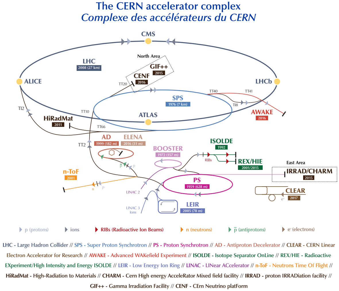
Figure 3.1: The CERN Accelerator Complex showing all experiments around the LHC (Image: CERN).
