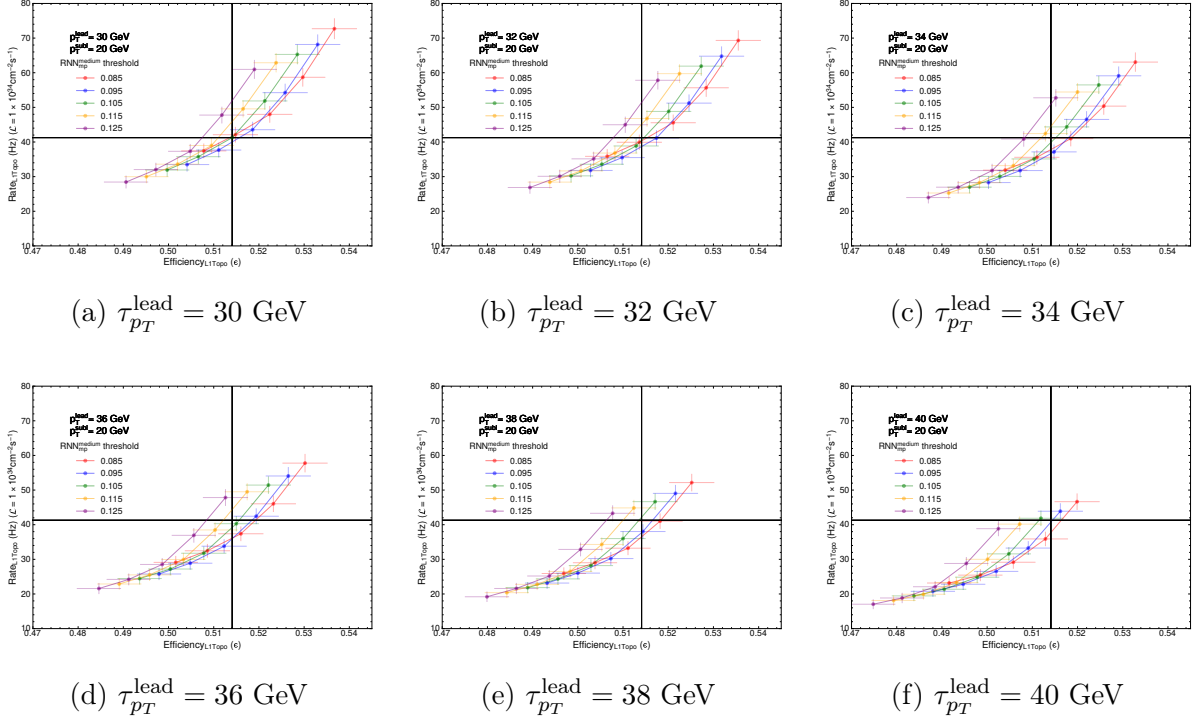
Figure 6.5: The plots show the efficiencies and rates of the \text{HLT}_{\text{L1Topo}} trigger when altering the thresholds for the leading p_T , \text{RNN}_{\text{lp}}^{\text{medium}} , and \text{RNN}_{\text{mp}}^{\text{medium}} associated with the tau objects. The p_T^{\text{subl}} is set at a constant 20 GeV. Each plot varies the \tau_{p_T}^{\text{lead}} threshold. The intersection point of the horizontal and vertical lines in each plot represents the rate and efficiency of the default variant of the \text{HLT}_{\text{L1Topo}} trigger. Different coloured contours on each plot indicate different multi-prong thresholds, while different points on the contour correspond to various 1-prong WPs. The y-axis range for the rates was constrained between 10 Hz and 80 Hz. Meanwhile, for efficiencies, the x-axis range was constrained between 0.470 and 0.545.
