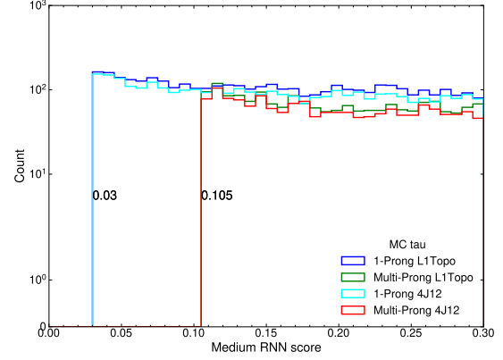
(h) RNN score of 1-prong ( \text{RNN}_{1p}^{\text{medium}} ) and multi-prong ( \text{RNN}_{mp}^{\text{medium}} ) \tau leptons matched to \text{HLT}_{\text{L1Topo}} and \text{HLT}_{4J12} chains with medium working point.
