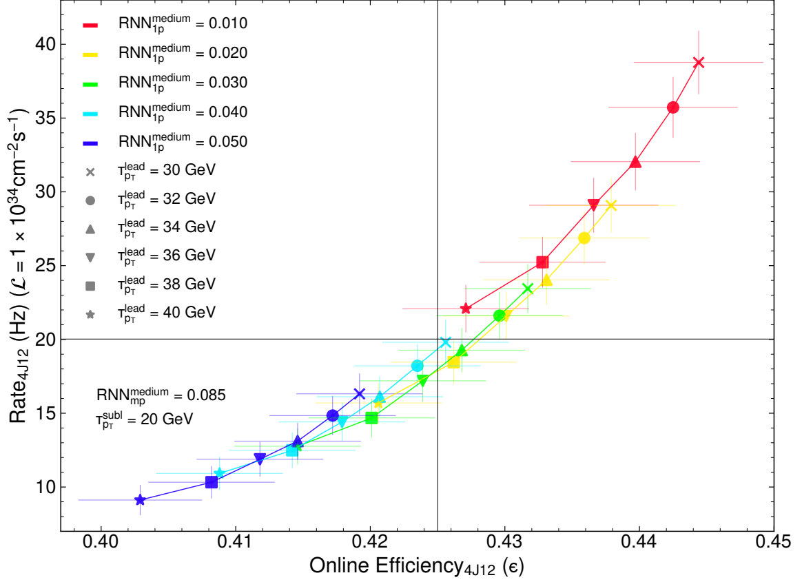
Figure 6.8: Plot displaying the variations in efficiencies and rates of the \text{HLT}_{4J12} trigger when altering the \tau_{pT}^{\text{lead}} and \text{RNN}_{1p}^{\text{medium}} thresholds associated with the tau objects. The \tau_{pT}^{\text{subl}} and \text{RNN}_{mp}^{\text{medium}} thresholds of the tau objects are set to a constant 20 GeV and 0.085 respectively. The intersection point of the horizontal and vertical lines represents the rate and efficiency of the default variant of the \text{HLT}_{4J12} trigger. Different colored contours on each plot indicate different \text{RNN}_{1p}^{\text{medium}} thresholds, while different markers correspond to various leading p_T thresholds.
