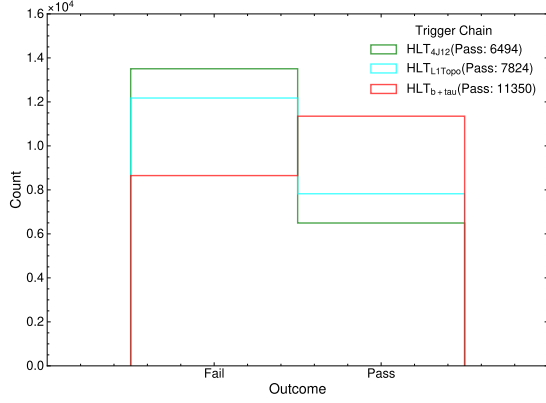
(a) Number of events that pass/fail \text{HLT}_{\text{L1Topo}} , \text{HLT}_{4\text{J12}} and \text{HLT}_{b+\tau} chains.
