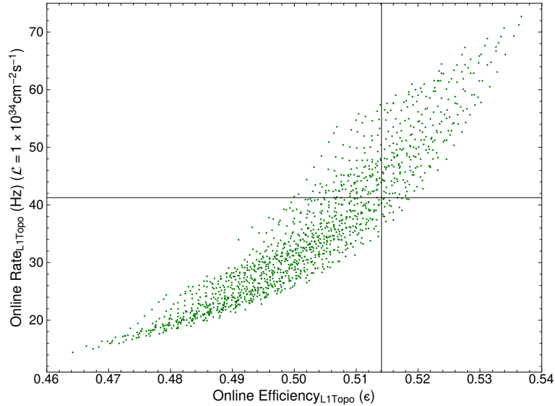
Figure C.3: Efficiencies and rates of the \text{HLT}_{L1Topo} chain generated by varying the thresholds of different trigger parameter. The intersection point corresponds to the rate and efficiency of the default trigger parameters of the \text{HLT}_{L1Topo} chain.
