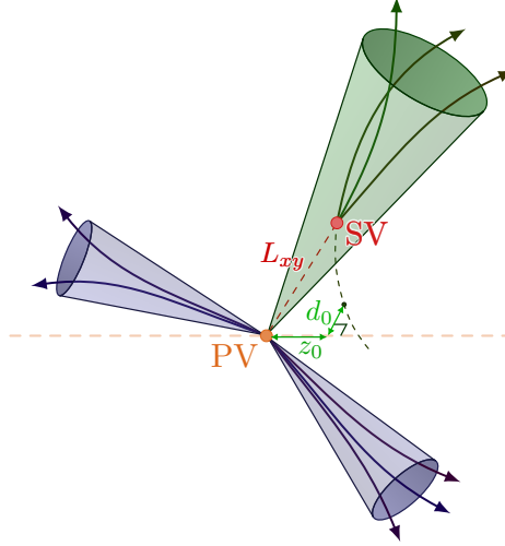
Figure 4.9: Characteristics of a jet initiated by a bottom quark with the secondary vertex, as well as a longitudinal ( z_0 ) and transverse impact parameter ( d_0 ) of individual tracks from their point of closest approach to the primary vertex. Adapted from graphic by © Izaak Neutelings, CC BY 2.5.
