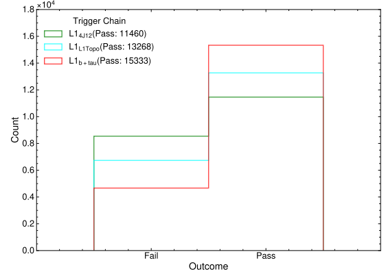
(b) Number of events that pass/fail the L1 seed of \text{HLT}_{\text{L1Topo}} , \text{HLT}_{4\text{J12}} and \text{HLT}_{b+\tau} chains.
