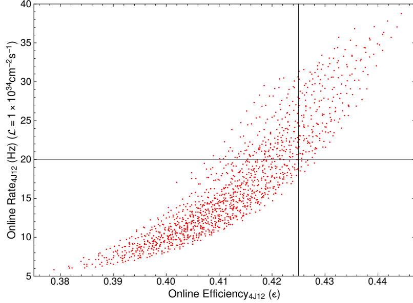
Figure C.2: Efficiencies and rates of the \text{HLT}_{4J12} chain generated by varying the thresholds of different trigger parameter. The intersection point corresponds to the rate and efficiency of the default trigger parameters of the \text{HLT}_{4J12} chain.
