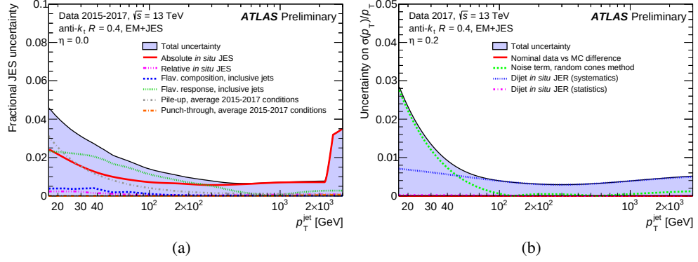
Figure 4.7: (a) Fractional jet energy scale systematic uncertainty components as a function of jet- p_T for small- R jets at \eta = 0.0 and, (b) jet energy resolution uncertainty as a function of jet- p_T for small- R jets at \eta = 0.2 . The total uncertainty (all components summed in quadrature) is shown as a filled region topped by a solid black line [76, 78].
