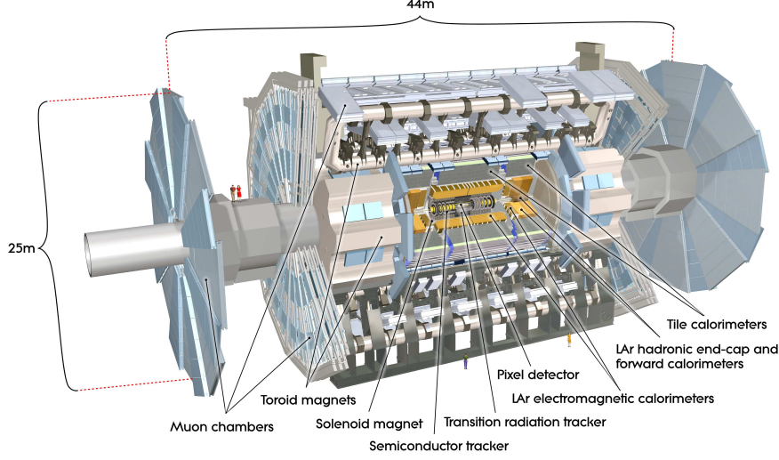
Figure 2.3: Cut-away view of the ATLAS detector [29].
