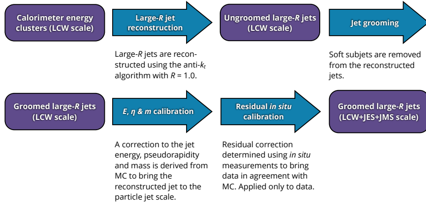
Figure 4.11: Overview of the large- R jet calibration procedure [85].
