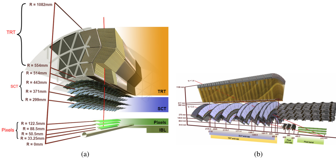
Figure 2.5: (a) Cut-away of the ATLAS ID barrel diagram made up by the IBL, the three pixel layers, the four layers of the SCT and the straw layers of the TRT [33]. (b) Cut-away of the ID end-cap made up by three pixel disks, nine disks of the SCT and TRT wheels [29].
