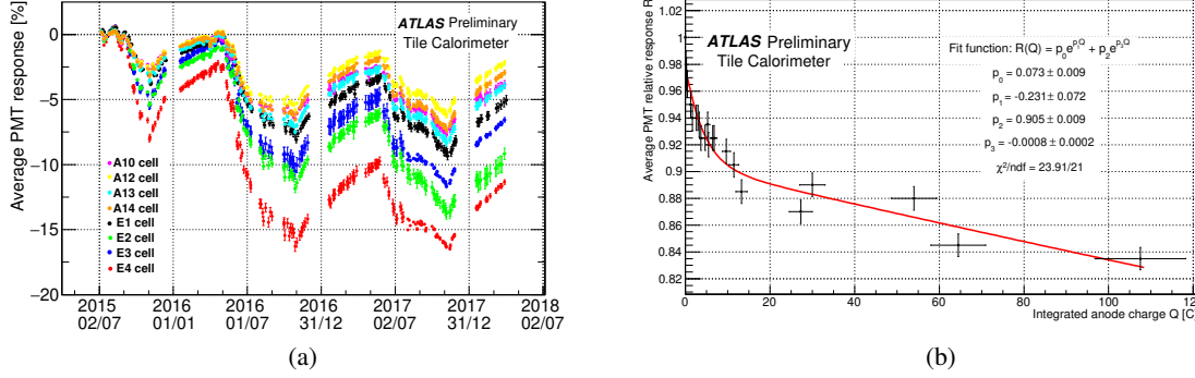
Figure B.5: Average PMT response variation of the most exposed TileCal cells as a function of time (a) and of the integrated anode charge (b) during the Run 2 [111].
