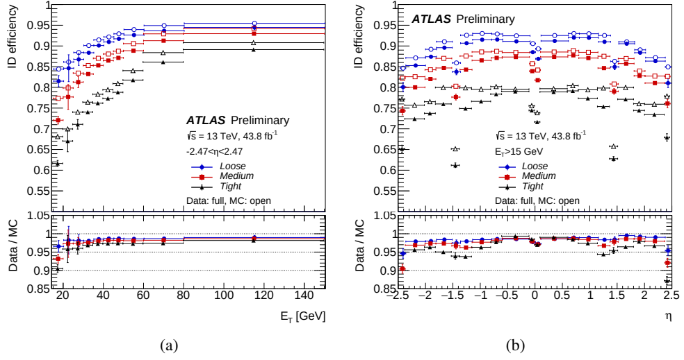
Figure 4.3: Electron identification efficiencies in Z \rightarrow ee events as a function of transverse energy E_T , integrated over the full pseudo-rapidity range (a), and as a function of pseudo-rapidity \eta for electrons with E_T > 15 GeV (b). The efficiencies are shown in data and MC for three operating points, Loose (blue points), Medium (red points) and Tight (black points). For both plots, the bottom panel shows the data-to-simulation ratios [68].
