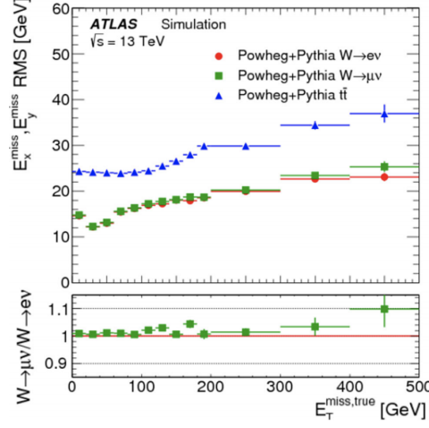
Figure 4.17: E_T^{\text{miss}} resolution measured by \text{RMS}_{x(y)}^{\text{miss}} as a function of the true missing transverse momentum E_T^{\text{miss,true}} for the W \rightarrow e\nu , W \rightarrow \mu\nu and t\bar{t} samples from the MC simulations [97].
