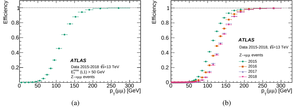
Figure 3.1: (a) The L1 E_T^{\text{miss}} trigger efficiency as a function of p_T(\mu\mu) . (b) Full chain E_T^{\text{miss}} trigger efficiencies for each year as a function of p_T(\mu\mu) . In both plots the error bands correspond only to the statistical uncertainty [36].
