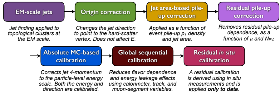
Figure 4.5: Steps of the JES calibration procedure applied to small- R jets. Each stage of the calibration is applied to the four-momentum of the jet [74].
