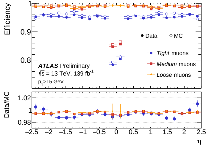
Figure 4.4: Muon reconstruction efficiency for the Loose, Medium and Tight identification algorithms measured in Z \rightarrow \mu\mu events as a function of the pseudorapidity of muon with p_T > 15 \text{ GeV} . The prediction by the MC simulation is depicted as open circles, while filled dots indicate the observation in collision data. The bottom panel shows the ratio between expected and observation efficiencies [70].
