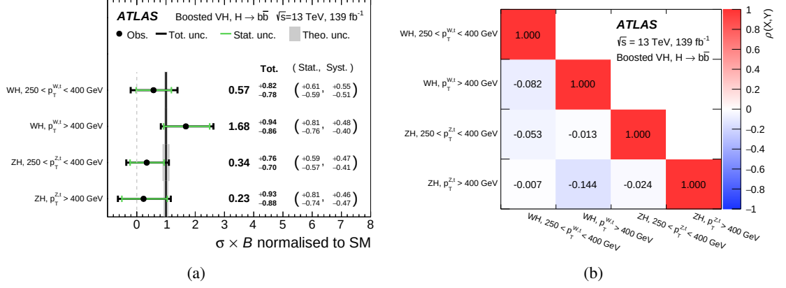
Figure 8.10: (a) Measured cross-section times BRs normalised to the SM predictions. The grey error bands correspond to the theoretical uncertainty on the normalised \sigma \times BR . (b) Observed correlations among the cross-sections in the STXS bins. The colour indicates the size of the correlation [21].
