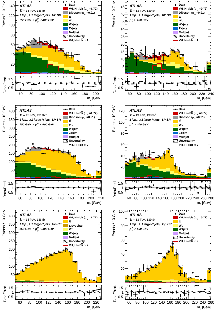
Figure 8.2: The large- R jet mass post-fit distribution in 1-lepton channel in the HP SRs (top row), LP SRs (middle row) and CRs (bottom row) for 250 \text{ GeV} \leq p_T^V < 400 \text{ GeV} (left) and p_T^V \geq 400 \text{ GeV} (right) regions. The data are shown as black dots. The background contributions are shown as filled histograms. The Higgs boson signal with m_H = 125 \text{ GeV} is shown as a filled histogram on the top of the fitted background multiplied by the signal strength \mu_{VH} , and unstacked as an unfilled histogram, multiplied by a factor 2. The size of the combined statistical and systematic uncertainty for the sum of the signal and background is indicated by the hatched band. The highest bin in the distributions contains the overflow. The ratio of the data to the sum of the fitted signal and background is shown in the lower panel [21].
