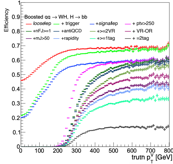
Figure 5.5: Efficiency breakdown in 1-lepton channel. The cuts have been applied in cascade so in each step there is an additional request. Each curve with different colors shows the effect of cut cascade as described in the text.
