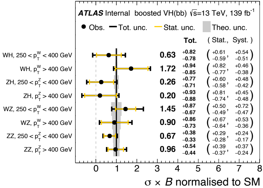
Figure 9.9: Measured VH and VZ cross-sections times branching ratios divided by the SM predictions. The grey area shows the theoretical uncertainty on the SM prediction.
