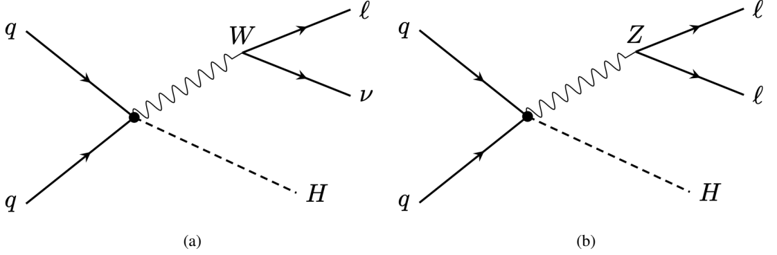
Figure 1.11: Feynman diagrams of the operator that multiplies the c_{Hq3} Wilson coefficient and that affects the WH (a) and ZH (b) production cross-sections. The black points show which vertices are impacted by the operator.
