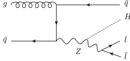
Figure 3.6: One of the leading order Feynman diagram of the qg -initiated process.
