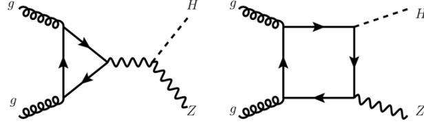
Figure 3.5: Two leading order Feynman diagrams of the gg \rightarrow ZH -process.
