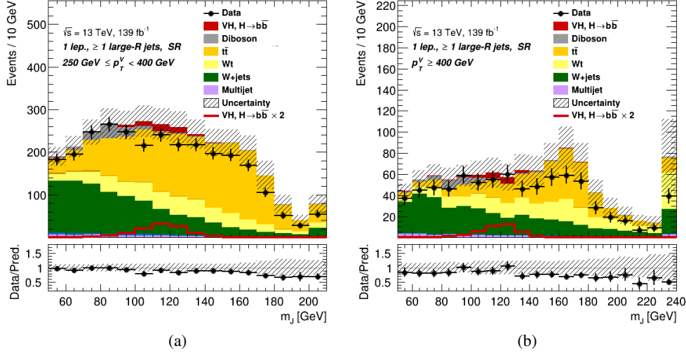
Figure 5.6: The invariant large- R jet mass m_J pre-fit distribution in the 1-lepton channel in the SR in the 250 \text{ GeV} \leq p_T^V < 400 \text{ GeV} (a) and p_T^V \geq 400 \text{ GeV} (b) momentum ranges. The data are shown as black dots. The background contributions are shown as filled histograms. The Higgs boson signal is shown as a filled histogram on the top of the background contribution, and unstacked as an unfilled histogram, multiplied by a factor 2. The size of the combined statistical and systematic uncertainty for the sum of the signal and background is indicated by the hatched band. The highest bin in the distributions contains the overflow. The ratio of the data to the sum of the signal and background is shown in the lower panel.
