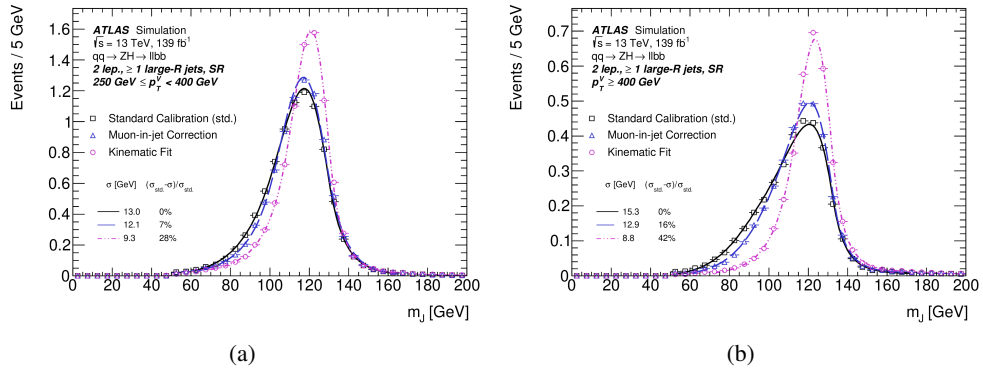
Figure 5.1: Comparison of the large- R mass distributions when additional corrections are applied to the jet energy scale for the signal in the 2-lepton channel, 250 \text{ GeV} \leq p_T^V < 400 \text{ GeV} (a) and p_T^V \geq 400 \text{ GeV} regions for the dominant qq \rightarrow ZH contribution. The distributions are fitted with a Bukin function [99] and the resolution values, \sigma , correspond to the width of the fitted function [21].
