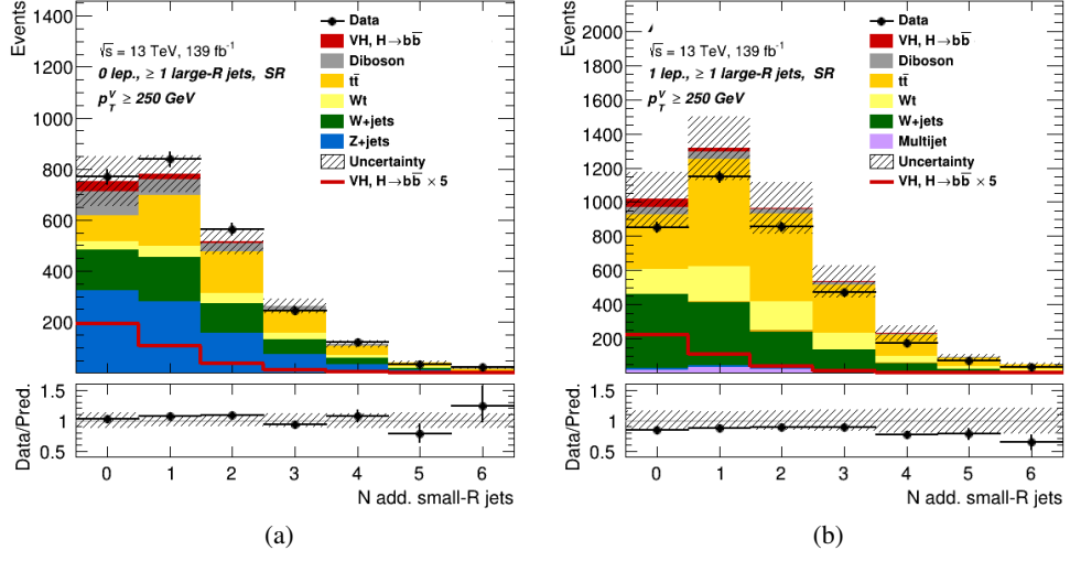
Figure 5.13: Number of small- R jets non-matched to the Higgs candidate jet distribution in 0-lepton (a) and 1-lepton (b) SRs for p_T^V \geq 250 GeV. The data are shown as black dots. The background contributions are shown as filled histograms. The Higgs boson signal is shown as a filled histograms on top of the background contribution, and unstacked as an unfilled histogram, multiplied by a factor 5. The size of the combined statistical and systematic uncertainty for the sum of the signal and background is indicated by the hatched band. The highest bin in the distributions contains the overflow. The ratio of the data to the sum of the signal and background is shown in the lower panel.
