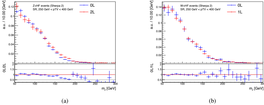
Figure 6.8: Normalised large- R jet mass m_J distribution of Z +HF (a) and W +HF (b) in the SR in the different lepton channels.
