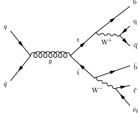
Figure 3.8: Lowest order Feynman diagram for the t\bar{t} process.
