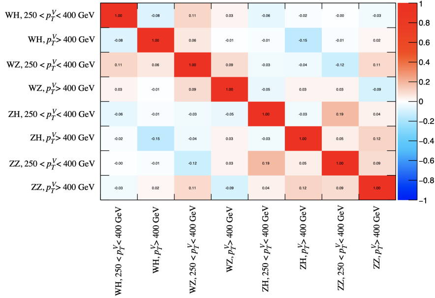
Figure 9.8: Observed correlations among the cross-sections in the different regions. The colour indicates the size of the correlation.
