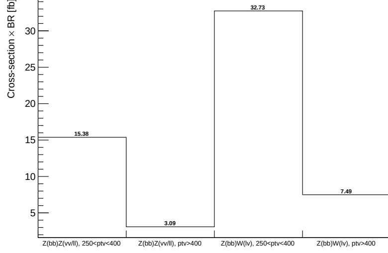
Figure 9.4: SM VZ(b\bar{b}) cross-sections times branching ratios in each bin of the main splitting scheme at \sqrt{s} = 13 TeV.
