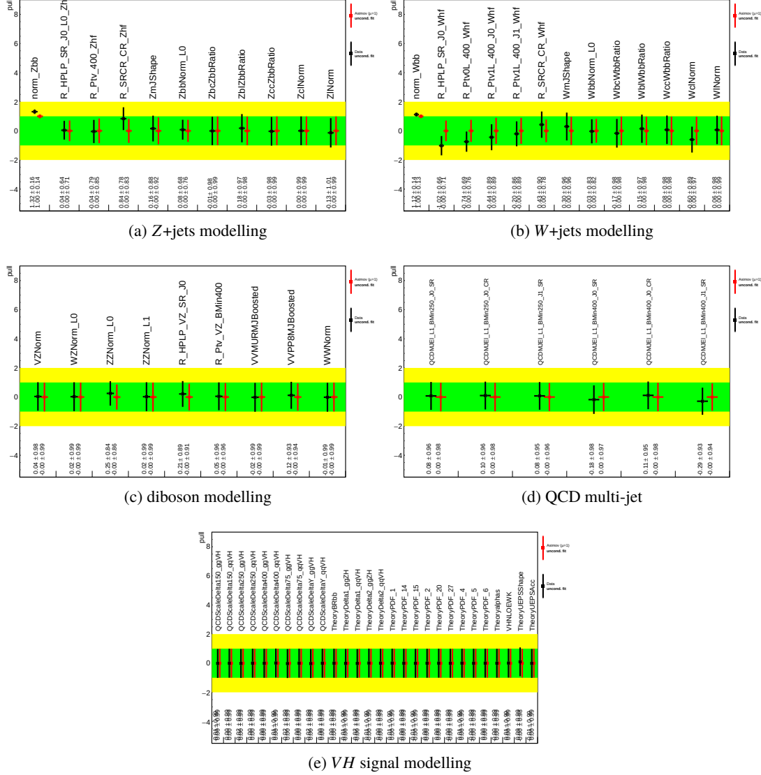
Figure D.1: Monte Carlo modelling-related and QCD multi-jet nuisance parameter pulls, constraints and post-fit normalisation scale factors for the freely floating parameters, obtained from the unconditional fit in all three lepton channels to the Asimov- (red) and the actual dataset (black).
