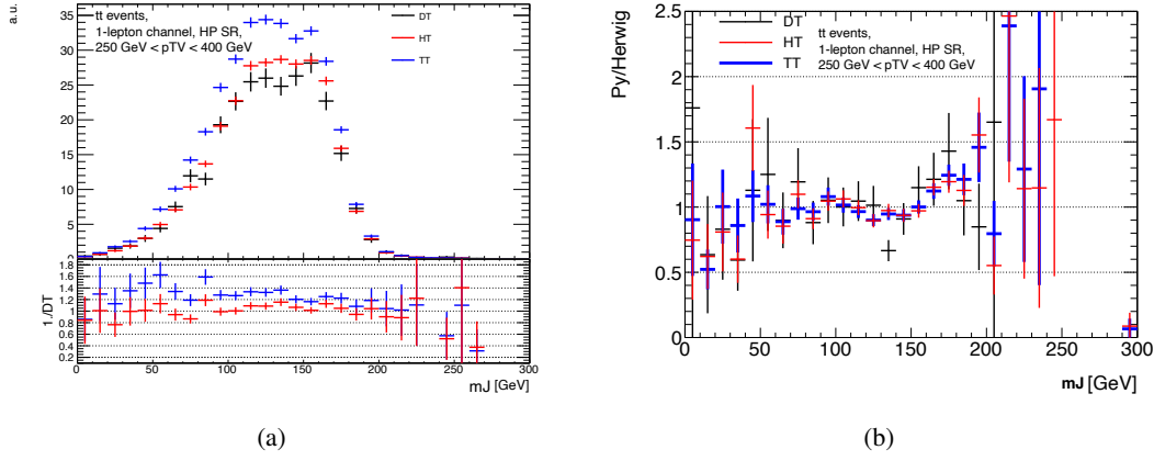
Figure 6.1: (a) m_J distributions obtained applying the direct (black line), hybrid (red line) and truth tagging (blue line) using t\bar{t} sample in the HP SR, medium p_T^V region in 1-lepton channel. (b) Comparison between t\bar{t} nominal (Poweg+Pythia) and alternative (Poweg+Herwig) samples applying the direct (black line), hybrid (red line) and truth tagging (blue line) in the HP SR, medium p_T^V region in 1-lepton channel.
