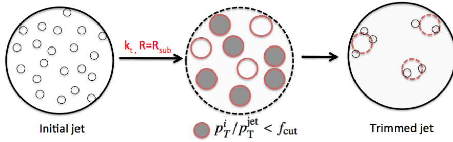
Figure 4.9: Diagram depicting the jet trimming procedure. The input of the trimming procedure is a topo-cluster jet reconstructed with the anti- k_t algorithm with R = 1.0 (left). The jet constituents of the original jet are reclustered using k_t algorithm into smaller subjets with R_{\text{sub}} = 0.2 (center). Any subjets that is carrying a transverse momentum fraction smaller than f_{\text{cut}} = 5\% of the parent jet is removed (right) [82].
