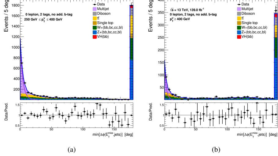
Figure 6.14: Post-fit \min[\Delta\phi(E_T^{\text{miss}}, \text{small-}R \text{ jets})] distributions in 250 \text{ GeV} \leq p_T^V < 400 \text{ GeV} (a) and p_T^V \geq 400 \text{ GeV} (b) regions in the SR excluding the selection cut on this variable. The MJ is modeled using an exponential shape.
