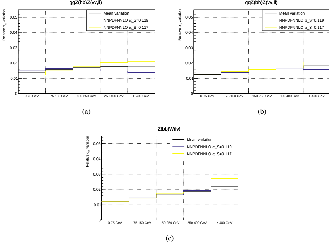
Figure 9.7: Absolute value of the relative \alpha_S variations in STXS bins for (a) gg \rightarrow ZZ , (b) qq \rightarrow ZZ and (c) qq \rightarrow WZ production modes. The black line represents the relative \alpha_S uncertainty.
