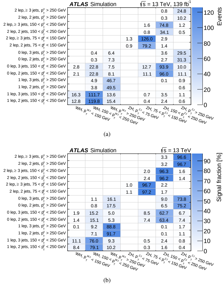
Figure 1.9: Expected signal yields (a) and signal fractions (b) in each reconstructed category as a function of the STXS region. Events with event yield below 0.1 or signal fractions below 0.1% are not shown [20].
