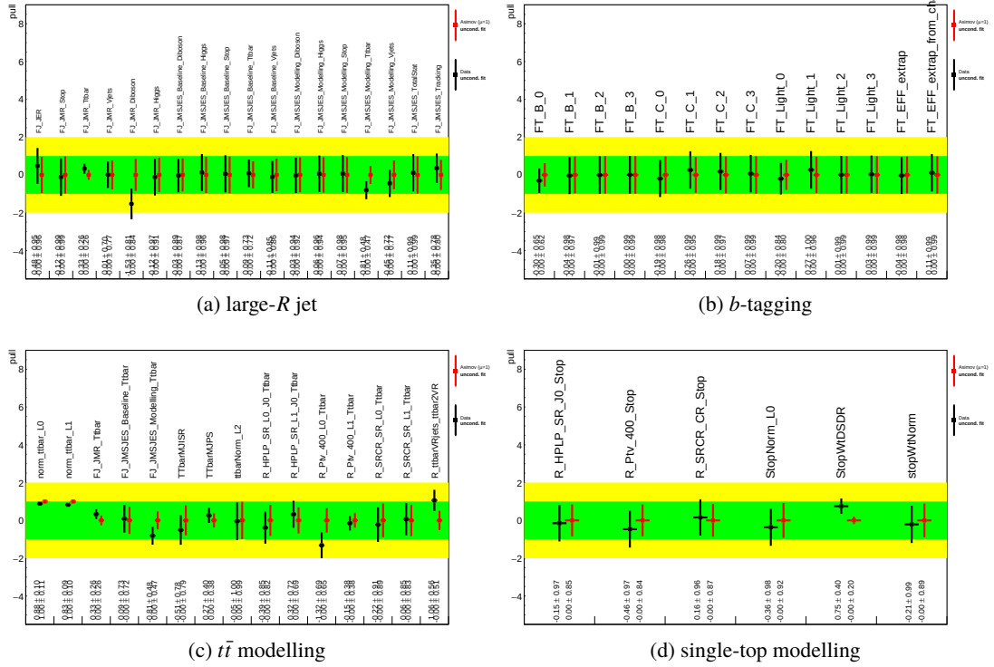
Figure 8.5: Detector-related (top row) and MC modelling-related (bottom row) nuisance parameter pulls, constraints and post-fit normalisation scale factors for the freely floating parameters. All the results are obtained from the unconditional fit in all three lepton channels to the Asimov- (red) and the actual dataset (black).
