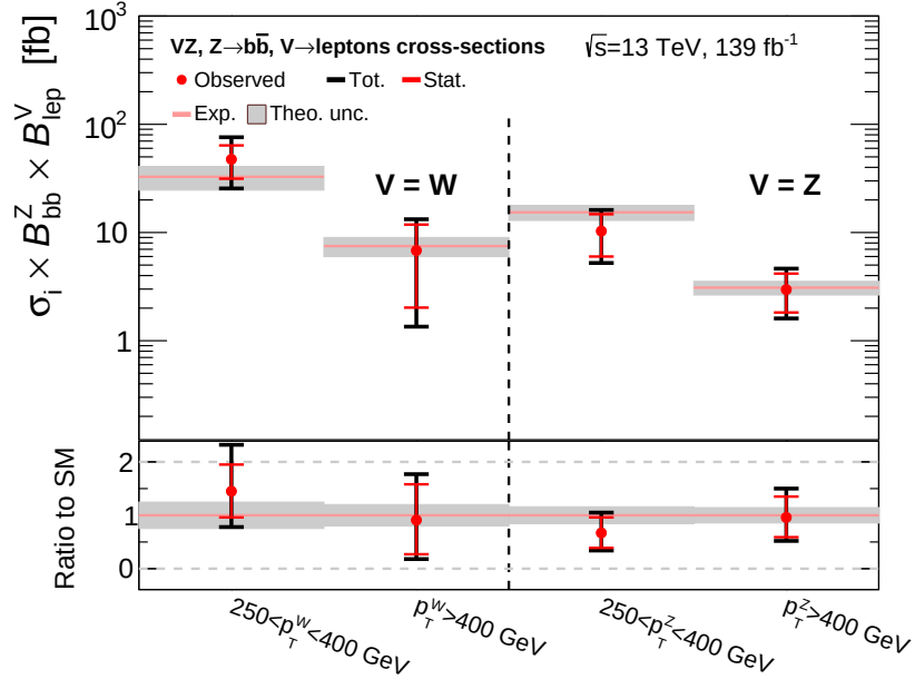
Figure 9.10: Measured VZ cross-sections times branching ratios in the four STXS bins at \sqrt{s} = 13 \text{ TeV} .
