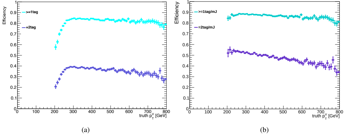
Figure 5.3: (a) b -tagging efficiency in the 1-tag (light blue dots) and 2-tag (violet dots) region as a function of the truth transverse momentum of the vector boson. (b) b -tagging efficiency in the 1-tag (light blue dots) and 2-tag (violet dots) region as a function of the truth transverse momentum of the vector boson requiring also the VR track-jets reconstruct correctly the b -hadron.
