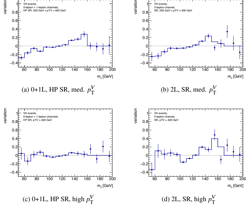
Figure 6.2: m_J variation due to the change of PS generator from Pythia 8 to Herwig 7. The contributions in the 0- and 1-lepton channels are summed. The variation Herwig 7 w.r.t. Pythia 8 is depicted using points whereas the final fit template is shown as a solid blue line.
