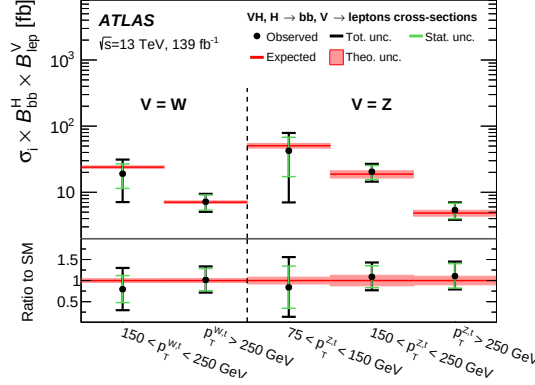
Figure 1.10: Observed values of the \sigma \times BR in the five STXS bins. The total observed uncertainty (black) is quoted together with the statistical component (green). The observation is compared to the SM prediction (red lines) and its uncertainty is represented by the red area [20].
