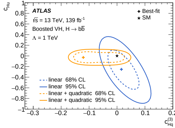
Figure 8.13: Observed confidence interval at 68% (dashed lines) and 95% (solid lines) CLs on the pair of c_{Hq3} and c_{Hu} Wilson coefficients. The limits are shown for the case where only linear (blue lines) and linear and quadratic (orange lines) terms are considered. The best-fit points are marked by a cross. The SM prediction is marked by a star [21].
