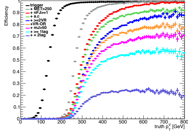
Figure 5.2: Efficiency breakdown in 0-lepton channel. The cuts have been applied in cascade so in each step there is an additional request. Each curve with different colors shows the effect of cut cascade as described in the text.
