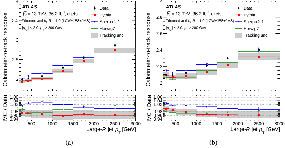
Figure 4.12: Measurement of r_{\text{trk}}^{\text{PT}} (a) and r_{\text{trk}}^m (b) as a function of the large- R jet p_T for large- R jets with m/p_T = 0.2 . Data are compared with three generators and with three tracking variations for the default generator PYTHIA 8. The double ratio of r_{\text{trk}}^{\text{PT}} and r_{\text{trk}}^m measured in simulations and data is shown in the lower panel [85].
