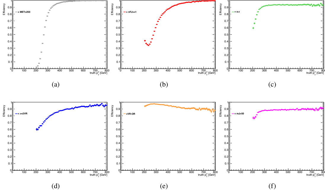
Figure C.1: Efficiency breakdown in 0-lepton channel. (a) Events that pass the E_T^{\text{miss}} cut ( E_T^{\text{miss}} > 250 GeV) divided by the events that pass the trigger cut. (b) Events have at least one large- R jet, that pass the E_T^{\text{miss}} and trigger cuts divided by the events that pass the trigger and E_T^{\text{miss}} cuts. (c) Events that pass the trigger, E_T^{\text{miss}} , large- R jet and anti- QCD cuts divided by the events that pass trigger, E_T^{\text{miss}} and large- R jet cuts. (d) Events that pass the trigger, E_T^{\text{miss}} , large- R jet, anti- QCD and VR track-jets cuts divided by the events that pass trigger, E_T^{\text{miss}} , large- R jet and anti- QCD cuts. (e) Events that pass the trigger, E_T^{\text{miss}} , large- R jet, anti- QCD , VR track-jets and VR overlap removal cuts divided by the events that pass the trigger, E_T^{\text{miss}} , large- R jet, anti- QCD and VR track-jets cuts. (f) Events that pass the trigger, E_T^{\text{miss}} , large- R jet, anti- QCD , VR track-jets, VR overlap removal and m_J cuts divided by events that pass the trigger, E_T^{\text{miss}} , large- R jet, anti- QCD , VR track-jets and VR overlap removal cuts.
