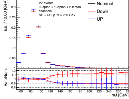
Figure 6.11: Normalised large- R jet mass distribution of the nominal sample and alternative sample with varied \mu_R for WZ and ZZ processes, including the contributions of all the analysis regions. The renormalisation scale \mu_R has been varied giving an up and down variation. The red line in the bottom panel shows the fitting results of the hyperbolic tangent function.
