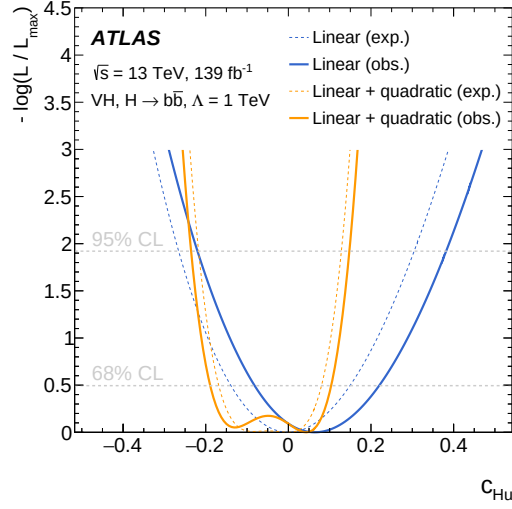
Figure 1.13: Observed (solid lines) and expected (dotted lines) profiled negative log-likelihood functions for one-dimensional fits to constrain a single coefficient of an effective Lagrangian when the other coefficients are assumed to vanish. The coefficients c_{Hu} is shown for the case where only linear (blue lines) or linear and quadratic (orange lines) terms are considered [20].
