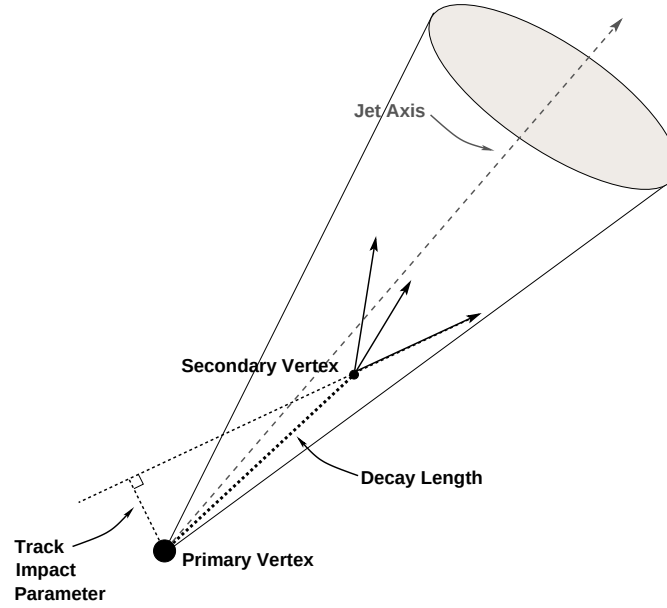
Figure 4.14: Illustration of a jet with a secondary vertex reconstructed from displaced tracks with a large impact parameter and with a significant decay length indicating the decay of a heavy long-lived particle, i.e. a b -hadron [91].
