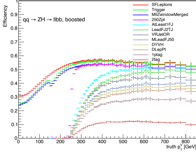
Figure 5.7: Efficiency breakdown in 2-lepton channel. The cuts have been applied in cascade so in each step there is an additional request. Each curve with different colors shows the effect of cut cascade as described in the text.
