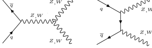
Figure 3.10: Lowest order Feynman diagrams for the diboson process.
