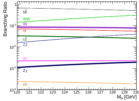
Figure 1.5: Predicted branching ratios of Higgs boson as a function of its mass [11].
