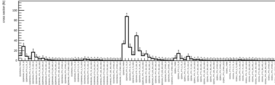
Figure 1.7: Standard Model cross-sections in each region of the maximum splitting scheme at the centre-of-mass energy \sqrt{s} = 13 TeV.
