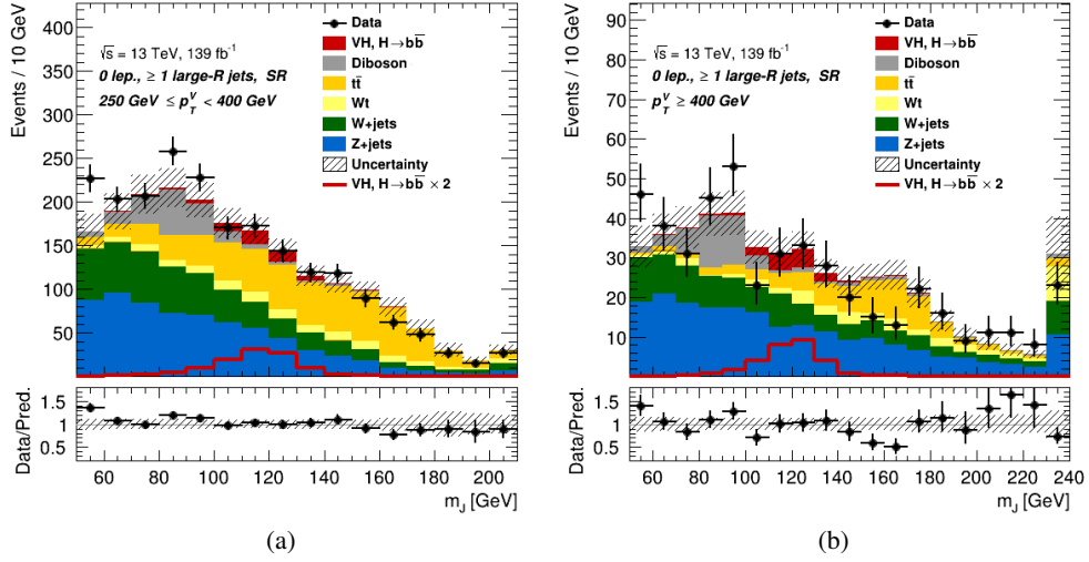
Figure 5.4: The invariant large- R jet mass m_J pre-fit distribution in the 0-lepton channel in the SR in the 250 \text{ GeV} \leq p_T^V < 400 \text{ GeV} (a) and p_T^V \geq 400 \text{ GeV} (b) momentum ranges. The data are shown as black dots. The background contributions are shown as filled histograms. The Higgs boson signal is shown as a filled histogram on the top of the background contribution, and unstacked as an unfilled histogram, multiplied by a factor 2. The size of the combined statistical and systematic uncertainty for the sum of the signal and background is indicated by the hatched band. The highest bin in the distributions contains the overflow. The ratio of the data to the sum of the signal and background is shown in the lower panel.
