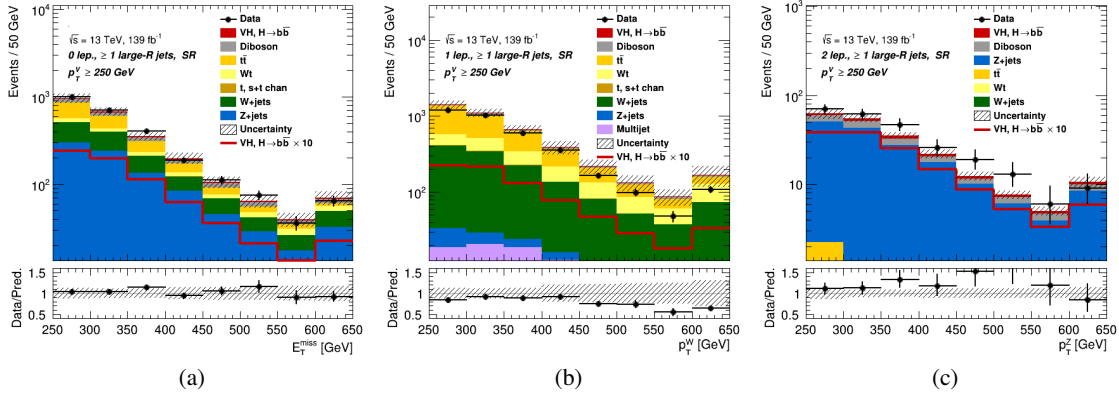
Figure 5.9: The p_T^V pre-fit distributions in 0-lepton (a), 1-lepton (b) and 2-lepton (c) SRs for p_T^V \geq 250 GeV. The data are shown as black dots. The background contributions are shown as filled histograms. The Higgs boson signal is shown as a filled histograms on top of the background contribution, and unstacked as an unfilled histogram, multiplied by a factor 10. The size of the combined statistical and systematic uncertainty for the sum of the signal and background is indicated by the hatched band. The highest bin in the distributions contains the overflow. The ratio of the data to the sum of the signal and background is shown in the lower panel.
