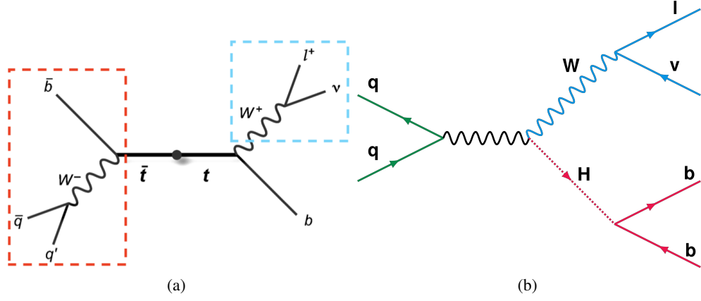
Figure 5.10: Leading order Feynman diagram for the t\bar{t} (a) and WH (b) processes. The red box in the Feynman diagram of the t\bar{t} process indicates the decay products of a hadronically decaying top quark which can be wrongly selected as Higgs candidate jet. The light blue box includes the decay products of a W boson which is correctly reconstructed as V boson candidate.
