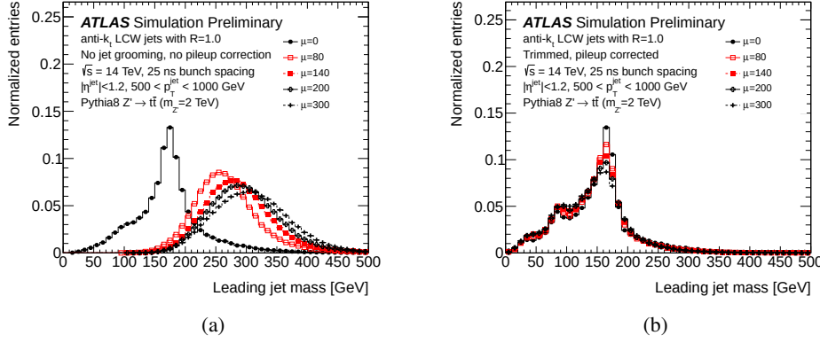
Figure 4.10: Mass distribution of anti- k_t large- R jet with (right) and without (left) applying the trimming technique [84].
