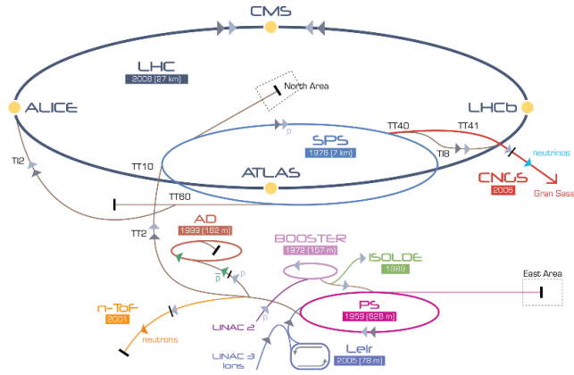
Figure 2.1: Schematic view of the accelerator system at CERN with the four collision points and other beams extracted at different accelerator level.
