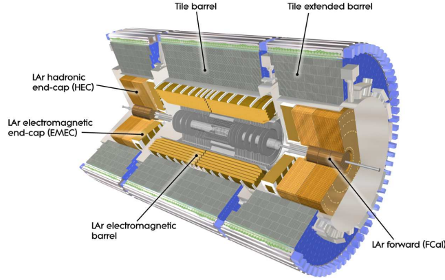
Figure 2.6: Cut-away view of ATLAS calorimetric system [29].
