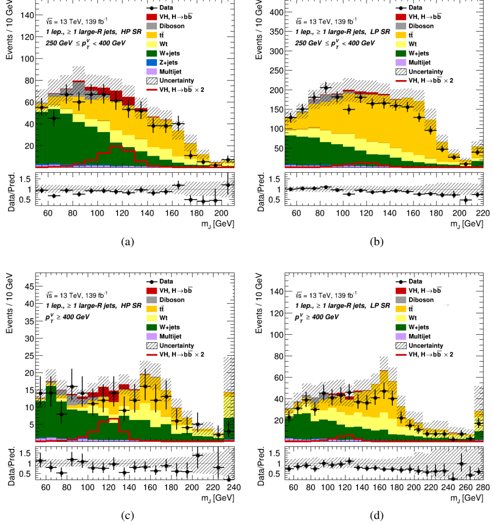
Figure 5.15: The invariant large- R jet mass m_J pre-fit distributions in the 1-lepton channel in the HP SR (left) and LP SR (right) in the 250 \text{ GeV} \leq p_T^V < 400 \text{ GeV} (top) and p_T^V \geq 400 \text{ GeV} (bottom) region. The data are shown as black dots. The background contributions are shown as filled histograms. The Higgs boson signal is shown as a filled histogram on the top of the background contribution, and unstacked as an unfilled histogram, multiplied by a factor 2. The size of the combined statistical and systematic uncertainty for the sum of the signal and background is indicated by the hatched band. The highest bin in the distributions contains the overflow. The ratio of the data to the sum of the signal and background is shown in the lower panel.
