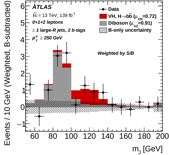
Figure 8.4: The large- R jet mass m_j distribution in data after subtraction of all the backgrounds except for the WZ and ZZ diboson processes. The contribution of all the three lepton channels and SRs are summed and weighted by their respective values of the ratio of fitted Higgs boson signal with m_H = 125 \text{ GeV} and background yields. The VH signal contribution is multiplied by the measured VH signal strength \mu_{VH} . The diboson contribution is normalised to its VZ signal strength \mu_{VZ} . The hatched band shows the size of the combined statistical and systematic uncertainties [21]
