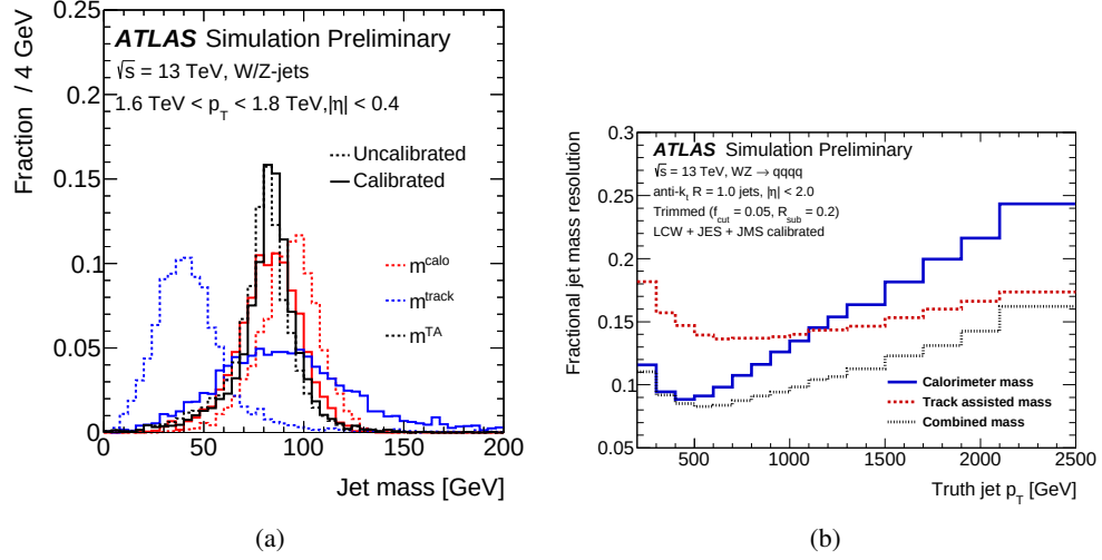
Figure 4.8: (a) Uncalibrated (dashed line) and calibrated (solid line) reconstructed jet mass distribution for the different large- R jet mass definition [80]. (b) Fractional jet mass resolution vs. the truth jet mass transverse momentum for the three large- R jet mass definition [81].
