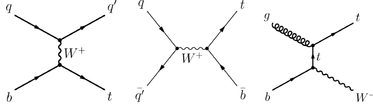
Figure 3.9: Lowest order Feynman diagrams for the three channels of the single top production: t-channel (left), s-channel (middle), Wt-channel (right).
