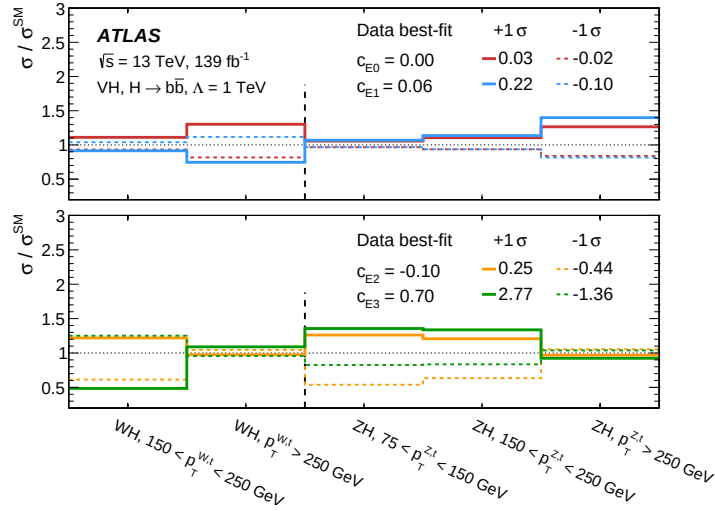
Figure A.1: Impact of the leading four eigenvectors on the STXS cross-section measurements. The change of the cross-section is indicated at +1\sigma (solid line) and -1\sigma (dashed line) limits of the corresponding coefficient. The value of the coefficients are extracted from a simultaneous fit of all five eigenvectors. [20]
