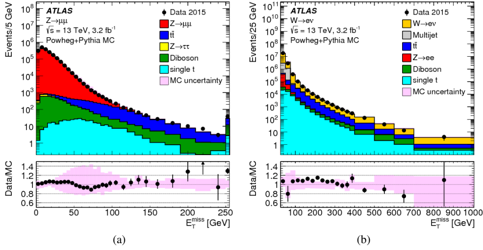
Figure 4.16: E_T^{\text{miss}} distribution for Z \rightarrow \mu\mu (a) and W \rightarrow e\nu (b) events in data. The expectation from MC simulation is superimposed and includes all relevant background final states passing the event selection. The shaded areas indicate the total uncertainty for MC simulations, including the overall statistical uncertainty combined with systematic uncertainties from the p_T scale and resolution which are contributed by muons, electrons, jets and soft term. The last bin of each distribution includes the overflow. The respective ratios between data and MC simulations are shown in the bottom pad, with the shaded areas showing the total uncertainties for MC simulations [97].
