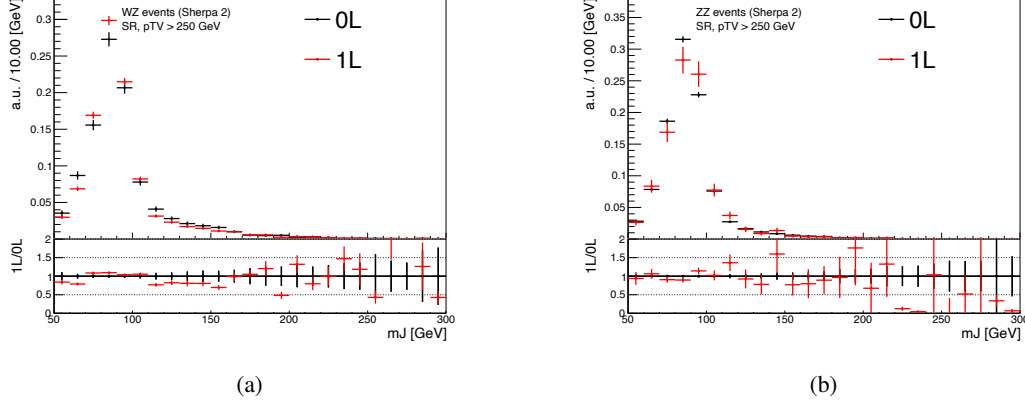
Figure 6.10: Normalised large- R jet mass distribution of WZ (a) and ZZ (b) events in the SR with p_T^V > 250 GeV in 0- and 1-lepton channels.
