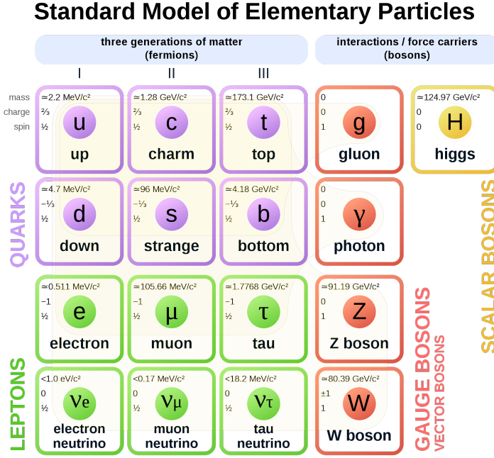
Figure 1.1: Summary of the Standard Model elementary particles and their properties. The twelve fermions and five fundamental bosons (the eight gluons and the two W bosons are shown in a single g and W box respectively) are shown.
