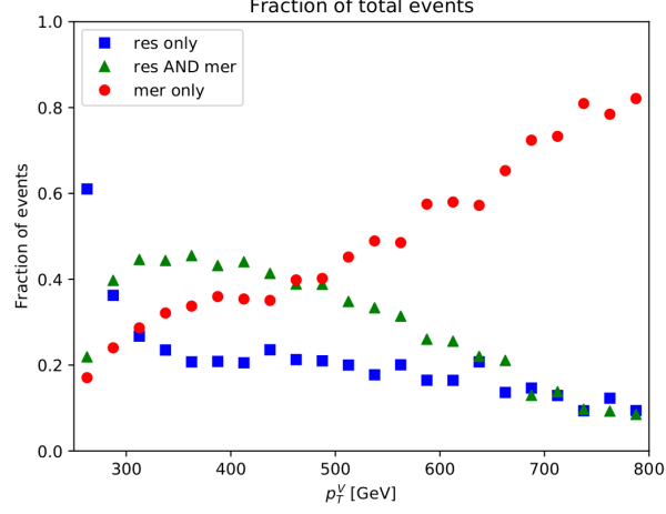
Figure 8.15: Fraction of the simulated signal VH events reconstructed only by the resolved (blue squares) and boosted (red dots) analysis, together with the fraction of overlap events (green triangles) as a function of the p_T^V in the 0-lepton channel.
