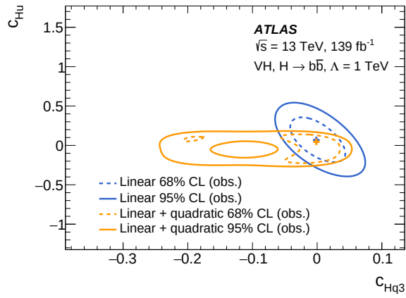
Figure 1.15: Observed confidence intervals on the simultaneous likelihood to the pair of c_{Hq3} and c_{Hu} Wilson coefficients, at 68% (dashed lines) and 95% CL (solid lines). Limits are shown for the case where only linear (blue lines) or linear and quadratic (orange lines) terms are considered. The best points are marked by a cross [20].
