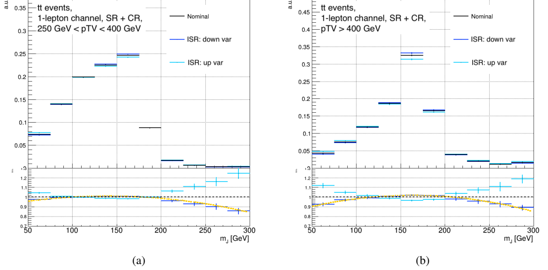
Figure 6.4: Normalized large- R jet mass m_J distributions for ISR uncertainties for t\bar{t} events in the 1-lepton channel in the 250 \text{ GeV} \leq p_T^V < 400 \text{ GeV} (a) and the p_T^V \geq 400 \text{ GeV} (b) regions. The distribution is obtained summing the contribution in the SR and in the CR. The second order polynomial used as fitting function is drawn as a dashed yellow line.
