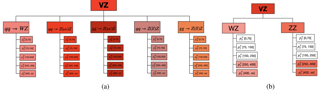
Figure 9.1: (a) Maximum splitting and (b) main splitting of the VZ events in STXS bins. The boundaries of the truth p_T^V regions are expressed in GeV. In the main splitting the measurements are performed only in the bin shown in red, the bins shown in white are fixed to their SM values.
