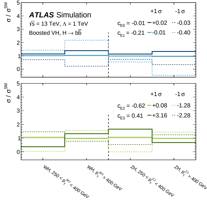
Figure 8.14: Impact of the four eigenvectors on the STXS cross-section measurements. The change of the cross-section is indicated at +1\sigma (solid line) and -1\sigma (dashed line) limits of the corresponding coefficient. The value of the coefficients are extracted from a simultaneous fit of all four eigenvectors. [21]
