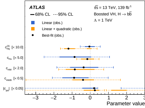
Figure 8.12: Summary of the observed best-fit values and one-dimensional confidence intervals for the Wilson coefficients to which the analysis has the greatest sensitivity and for the |c_{dH}| coefficient which directly affects the H \rightarrow b\bar{b} decay width. Limits are shown for the case where only linear (blue) and linear and quadratic (orange) terms are considered. Confidence intervals are shown at both 68% CL (solid line) and 95% CL (dashed line) [21].
