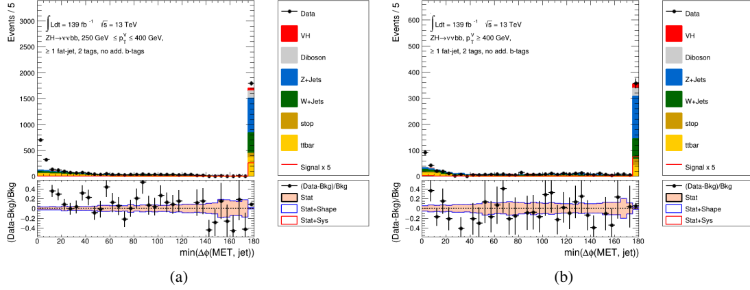
Figure 6.13: Pre-fit \min[\Delta\phi(E_T^{\text{miss}}, \text{small-}R \text{ jets})] distributions in 250 \text{ GeV} \leq p_T^V < 400 \text{ GeV} (a) and p_T^V \geq 400 \text{ GeV} (b) regions in the SR excluding the selection cut on this variable.
