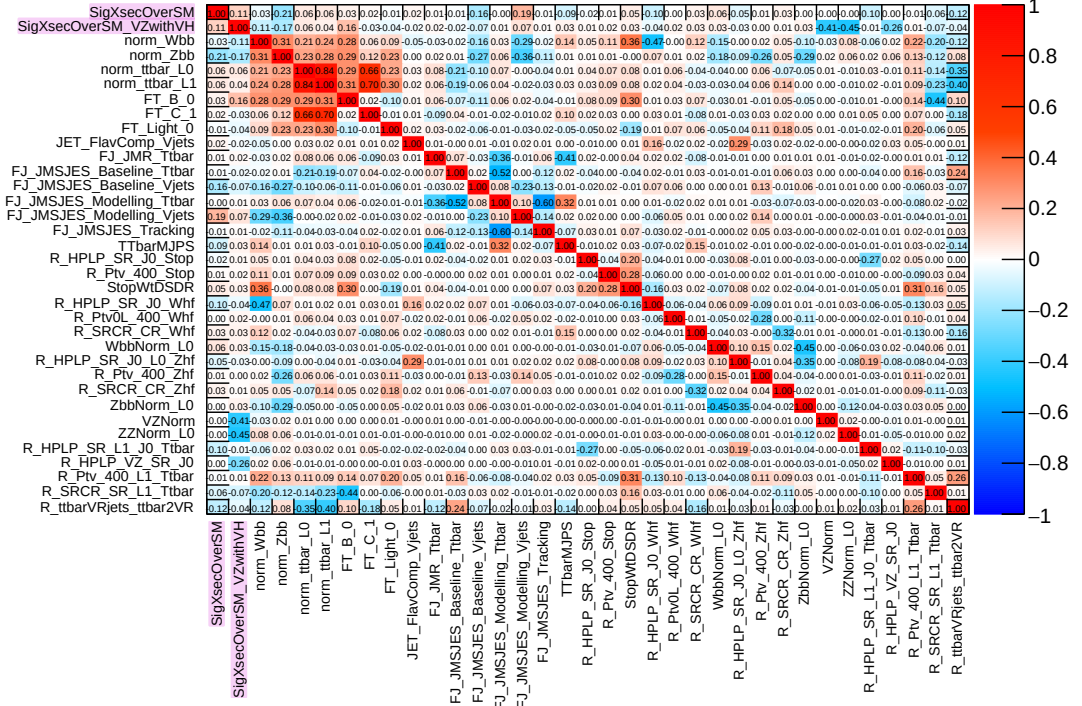
Figure 8.6: Correlation matrix obtained from the unconditional fit to the actual dataset.
