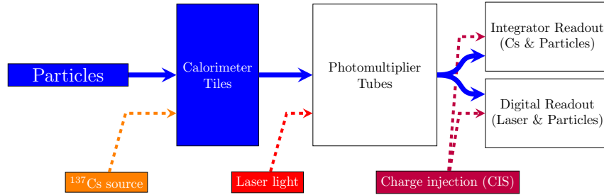
Figure B.3: The signal paths for each of the three calibration systems used by TileCal. The physics signal is denoted by the solid line, while the path taken by each calibration system is shown with dashed lines [111].
