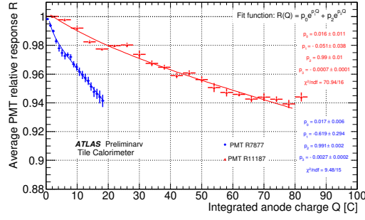
Figure B.6: Average PMT relative response of the old (blue) and new (red) PMT models at the test bench [111].
