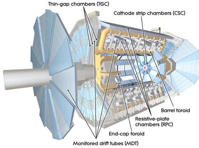
Figure 2.7: Cut-away view of ATLAS muon system [29].
