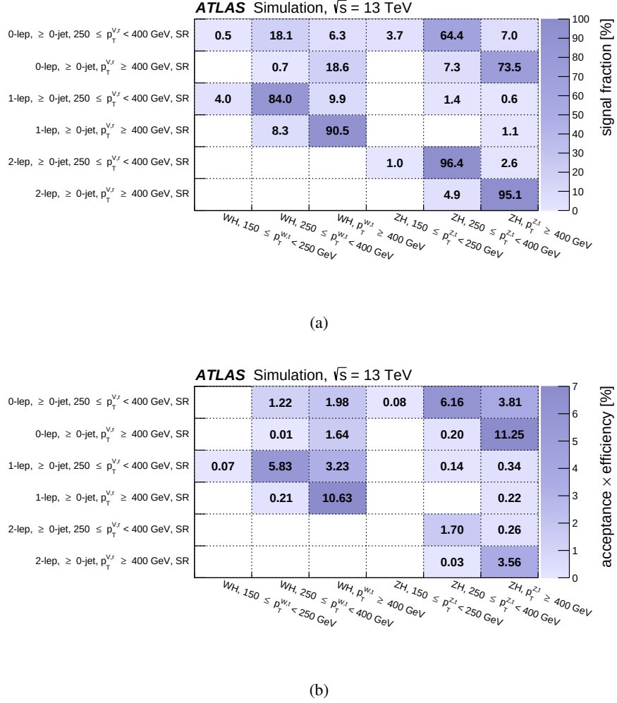
Figure 8.9: (a) Fraction of signal events and (b) acceptance times efficiency from each STXS bin ( x -axis) in every reconstructed event category ( y -axis). The values are in percent. The HP and LP SRs in 0- and 1-lepton channels have been merged. The signal contribution in the CRs is negligible and therefore not reported in the plots. Entries with acceptance times efficiency below 0.01% or signal fractions below 0.1% are not shown [21].
