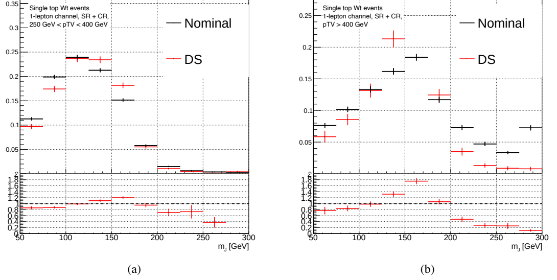
Figure 6.7: Normalised m_J distributions of the nominal sample and the alternative sample with the DS scheme for the single-top Wt events in the medium (a) and high (b) p_T^V regions in 1-lepton channel summing the contribution of the SRs and CRs.
