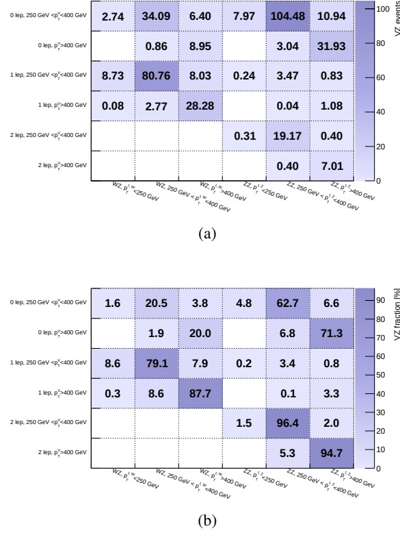
Figure 9.5: (a) VZ events and (b) VZ fraction from each STXS bin ( x -axis) in every reconstructed event category ( y -axis). The HP and LP SRs in 0- and 1-lepton channels have been merged and the contribution in the CRs is not shown because it is negligible.
