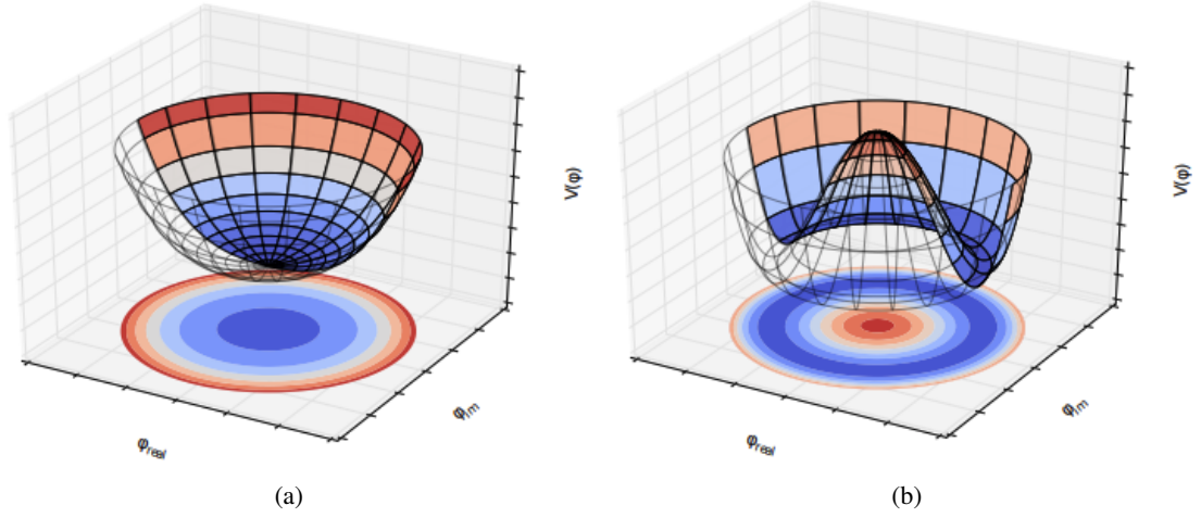
Figure 1.2: Higgs potential V(\phi) for a complex scalar field for \mu^2 > 0 (a) and \mu^2 < 0 (b).
