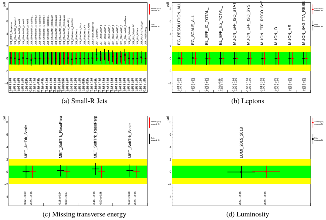
Figure D.2: Detector-related nuisance parameter pulls and constraints, obtained from the unconditional fit in all three lepton channels to the Asimov- (red) and the actual dataset (black).
