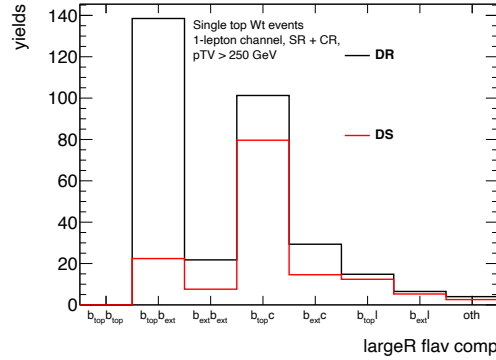
Figure 6.6: Flavour composition of the large- R jet in 1-lepton channel for nominal (DR scheme) and alternative (DS scheme) sample. The plot is done by summing the contribution of the SR and CR, and the two p_T^V regions. In the plot the b -quark from the top is indicated as b_{\text{top}} , while the spectator b as b_{\text{ext}} .
