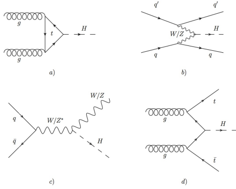
Figure 1.3: Feynman diagram for the Higgs production: (a) gluon-gluon fusion , (b) vector boson fusion , (c) associated production with a vector boson , (d) associated production with a pair of top quarks .
