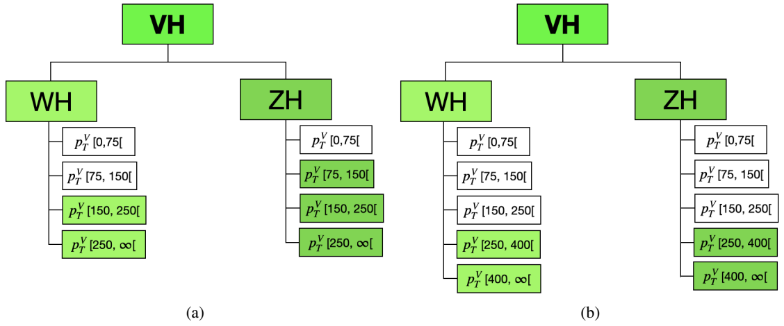
Figure 1.8: VH STXS regions in the main splitting scheme used by the resolved (a) and boosted (b) analyses, respectively. The measurements are performed only in the bins shown in green. The bins shown in white are fixed to their SM values
