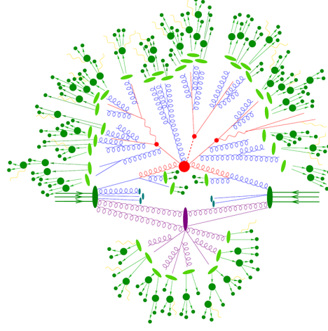
Figure 3.3: Schematic diagram of the steps of the event simulation. The simulation of the hard process is shown in red while the parton shower is represented with blue lines. The production of hadrons and their decay is represented by green lines and dots. The purple lines represent the simulation of the underlying events [40].
