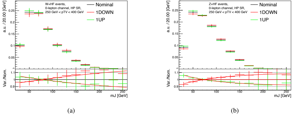
Figure 6.9: Normalised large- R jet mass distribution of nominal sample and alternative sample with varied \mu_R for W+HF (a) and Z + HF (b) processes in the HP SR, medium p_T^V region of the 0-lepton channel. The renormalisation scale \mu_R has been varied giving an up and down variation.
