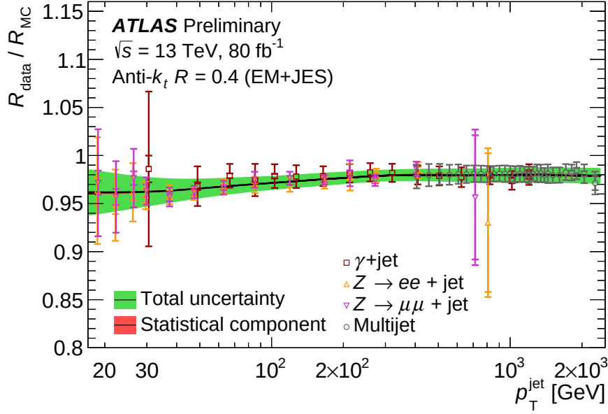
Figure 4.6: Data-to-simulation ratio of the average jet p_T response as a function of the jet p_T . The result is based on three in-situ techniques: Z +jets (triangles), \gamma + jets (squares) and multi-jet balance method (circles) [76].
