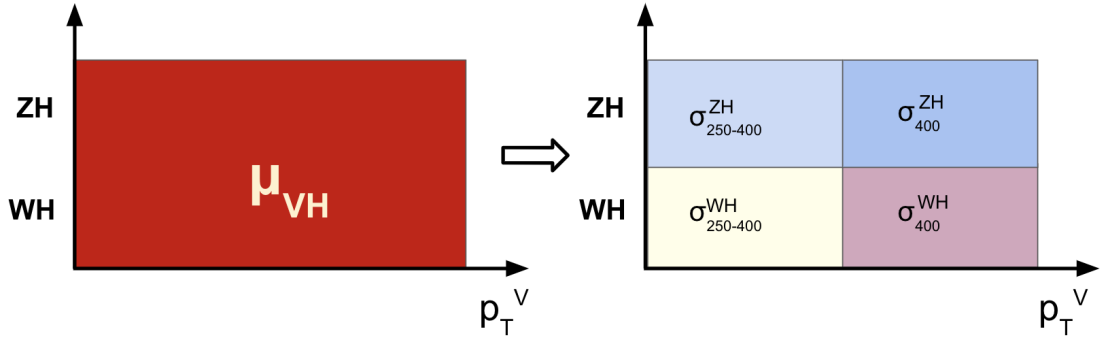
Figure 8.8: Signal strength measurement of the VH process (left) compared to the cross-section measurement (right). p_T^V is the transverse momentum of the V boson at generator level.
