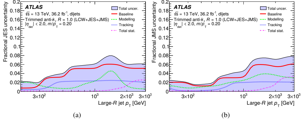
Figure 4.13: Total uncertainty in the relative JES (a) and JMS (b) in data and simulations as a function of the large- R transverse momentum [85].
