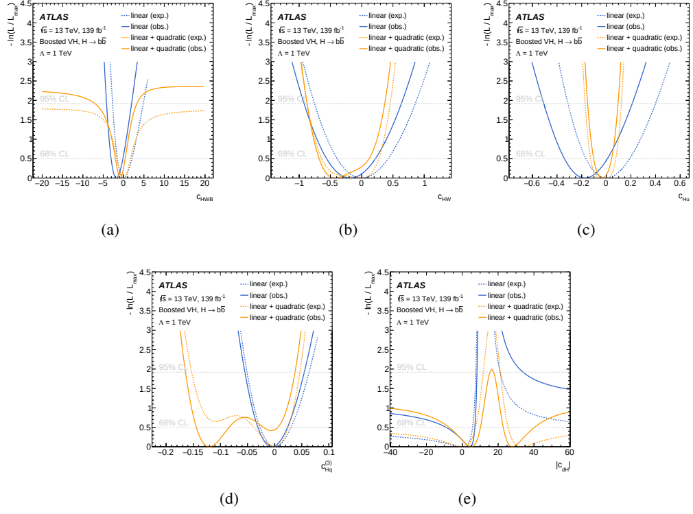
Figure 8.11: Observed (solid lines) and expected (dotted lines) profiled negative log-likelihood functions for one-dimensional fits to constrain a single coefficient of an effective Lagrangian when the other coefficients are assumed to vanish. The coefficients c_{HWB} , c_{HW} , c_{Hu} , c_{Hq3} and |c_{dH}| are shown for the case where only linear (blue lines) or linear and quadratic (orange lines) terms are considered [21].
