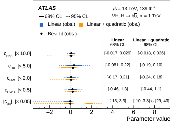
Figure 1.14: Observed best-fit values and 1D confidence intervals for the Wilson coefficients to which this analysis has the greatest sensitivity and the |c_{dH}| coefficient which directly affects the H \rightarrow b\bar{b} decay width. Limits are shown for the case where only linear (blue) and linear and quadratic (orange) terms are considered. Confidence intervals are shown at both 68% CL (solid line) and 95% CL (dashed line) [20]
