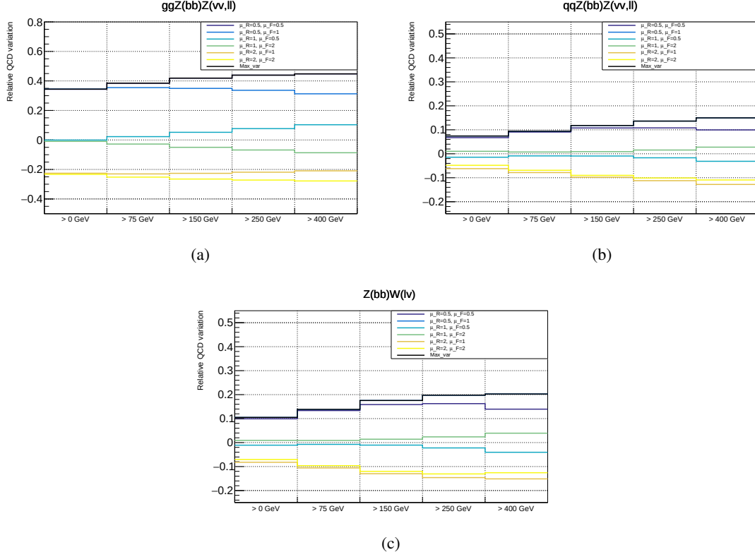
Figure 9.6: Relative QCD scale variations in inclusive p_T^V bins for (a) gg \rightarrow ZZ , (b) qq \rightarrow ZZ and (c) qq \rightarrow WZ production modes. The black line represents the absolute value of the maximum variation and it coincides with one of the six variations.
