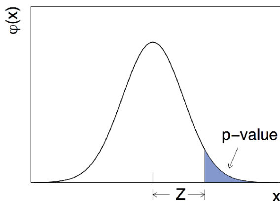
Figure 7.1: Relationship between a p-value and a significance of Z sigma [106].
