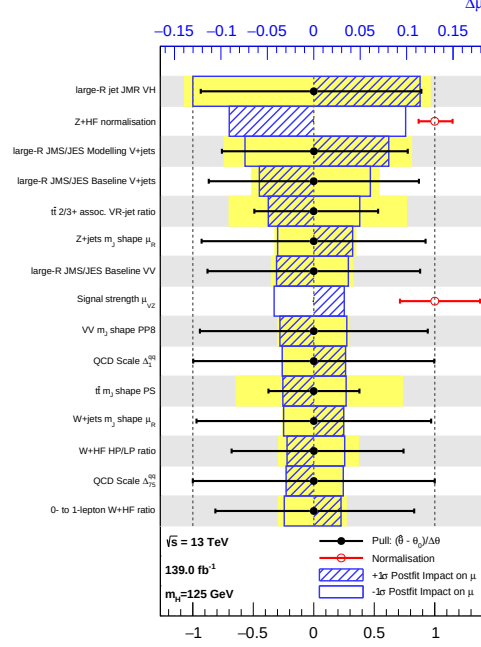
Figure 7.5: Impact of the uncertainties on the VH signal strength \mu_{VH} parameter obtained from a fit to the Asimov dataset. The uncertainties are sorted in a decreasing order. The boxes show the variation of \hat{\mu}_{VH} , referring to the top x -axis, when fixing the corresponding NP. The impact of the up- and down-variations can be distinguished via the dashed and plane box fillings. The yellow boxes show the pre-fit impact, referring to the top x -axis, by varying each NP by \pm 1\sigma . The filled black points with the corresponding error bars show the pull of each NP, referring to the bottom x -axis. The open red circles with the error bars show the fitted values and the uncertainties of the normalisation factors which are freely floating in the fit. The dotted vertical are placed at \pm 1 and are referred to the bottom x -axis.
