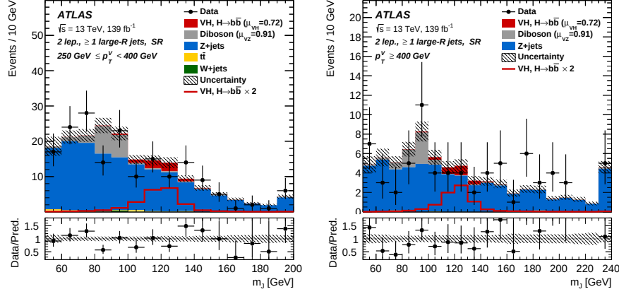
Figure 8.3: The large- R jet mass post-fit distribution in 2-lepton channel in the SR for 250 \text{ GeV} \leq p_T^V < 400 \text{ GeV} (a) and p_T^V \geq 400 \text{ GeV} (b) regions. The data are shown as black dots. The background contributions are shown as filled histograms. The Higgs boson signal with m_H = 125 \text{ GeV} is shown as a filled histogram on the top of the fitted background multiplied by the signal strength \mu_{VH} , and unstacked as an unfilled histogram, multiplied by a factor 2. The size of the combined statistical and systematic uncertainty for the sum of the signal and background is indicated by the hatched band. The highest bin in the distributions contains the overflow. The ratio of the data to the sum of the fitted signal and background is shown in the lower panel [21].
