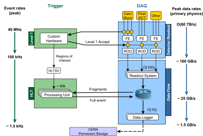
Figure 2.8: Block diagram of the ATLAS trigger (left) and data acquisition (right) system [35].
