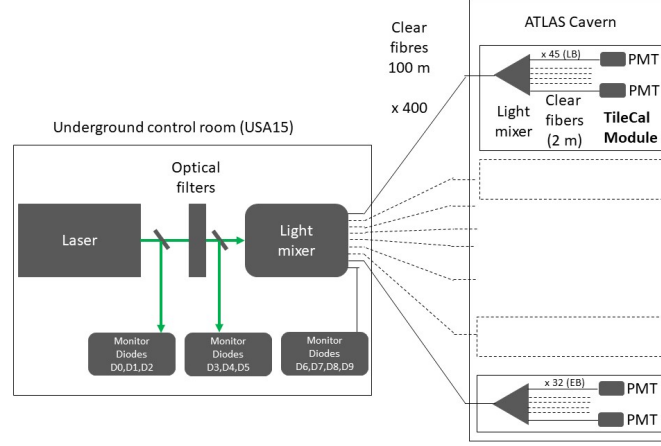
Figure B.4: Sketch of the Laser II system.
