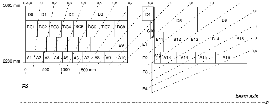
Figure B.2: The layout of the TileCal cells, denoted by a letter (A to E) plus an integer number. The A-layer is closest to the beam-line [111].
