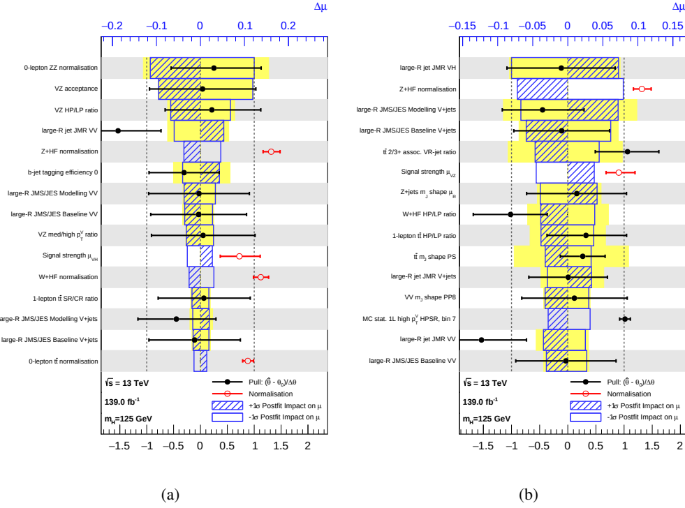
Figure 8.7: Impact of systematic uncertainties on the fitted VZ (a) and VH (b) signal-strength parameters \hat{\mu} sorted in decreasing order. The boxes show the variations of \hat{\mu} , referring to the top x -axis, when fixing the corresponding individual nuisance parameter to its post-fit value modified upwards or downwards by its post-fit uncertainty, i.e. \hat{\theta} \pm \sigma_{\hat{\theta}} , and repeating the fit. The impact of up- and down-variations can be distinguished via the dashed and plane box fillings. The yellow boxes show the pre-fit impact (top x -axis) by varying each nuisance parameter by \pm 1\sigma . The filled circles show the deviation of the fitted value for each nuisance parameter, \hat{\theta} , from their nominal input value \theta_0 expressed in standard deviations with respect to their nominal uncertainties \Delta\theta (bottom x -axis). The error bars show the post-fit uncertainties on \hat{\theta} with respect to their nominal uncertainties. The open circles show the fitted values and uncertainties of the normalization parameters that are freely floating in the fit.
