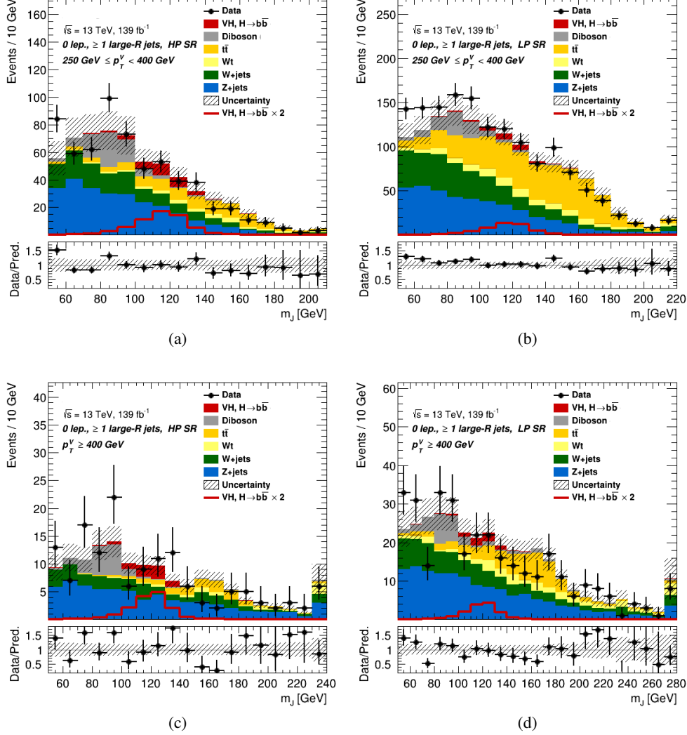
Figure 5.14: The invariant large- R jet mass m_J pre-fit distributions in the 0-lepton channel in the HP SR (left) and LP SR (right) in the 250 \text{ GeV} \leq p_T^V < 400 \text{ GeV} (top) and p_T^V \geq 400 \text{ GeV} (bottom) region. The data are shown as black dots. The background contributions are shown as filled histograms. The Higgs boson signal is shown as a filled histogram on the top of the background contribution, and unstacked as an unfilled histogram, multiplied by a factor 2. The size of the combined statistical and systematic uncertainty for the sum of the signal and background is indicated by the hatched band. The highest bin in the distributions contains the overflow. The ratio of the data to the sum of the signal and background is shown in the lower panel.
