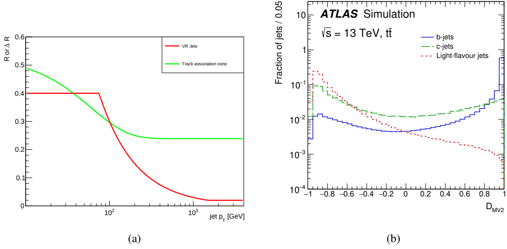
Figure 4.15: (a) Distribution of the VR track-jet radius parameter R (red line) and of the track association cone \Delta R as a function of the jet p_T [91]. (b) Distribution of the output discriminant of the MV2 b -tagging algorithm for b -jets, c -jets and light-flavour jets in the baseline t\bar{t} simulated events [92].
