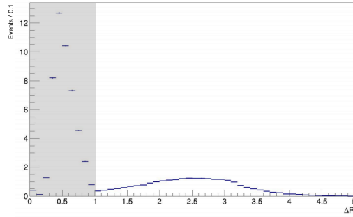
Figure 5.11: Distribution of the angular distance between the Higgs candidate and the leading small- R jet for VH signal events in 1-lepton SR, 250 \text{ GeV} \leq p_T^V < 400 \text{ GeV} . The gray area represents all the signal events in which the selected small- R jet is matched to the Higgs candidate.
