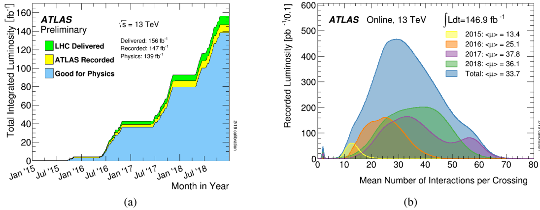
Figure 2.2: (a) Total integrated luminosity versus time delivered to ATLAS (green), recorded by ATLAS (yellow), and certified to be good quality data (blue) during stable beam proton-proton collisions at 13 TeV center-of-mass energy in 2015-2018. (b) Mean number of interactions per bunch crossing for the fill Run 2 period [27].
