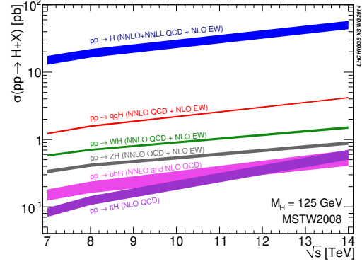
Figure 1.4: Cross-section production of Higgs boson with m_H = 125 GeV as a function of the center-of-mass energy \sqrt{s} [11].
