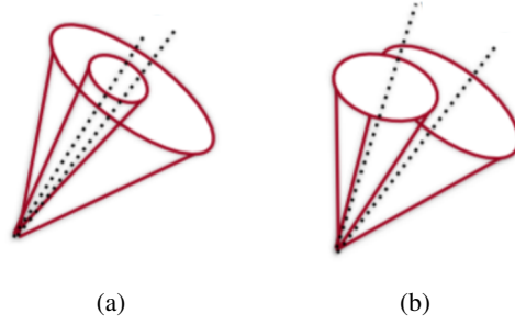
Figure 4.18: (a) Example of events discarded when the overlap removal is applied. (b) Example of events considered when the OR is applied.
