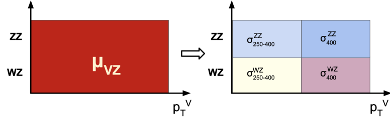
Figure 9.2: Pictorial representation of the PoIs for the signal strength measurement of the VZ process (left) compared to the cross-section measurements (right).
