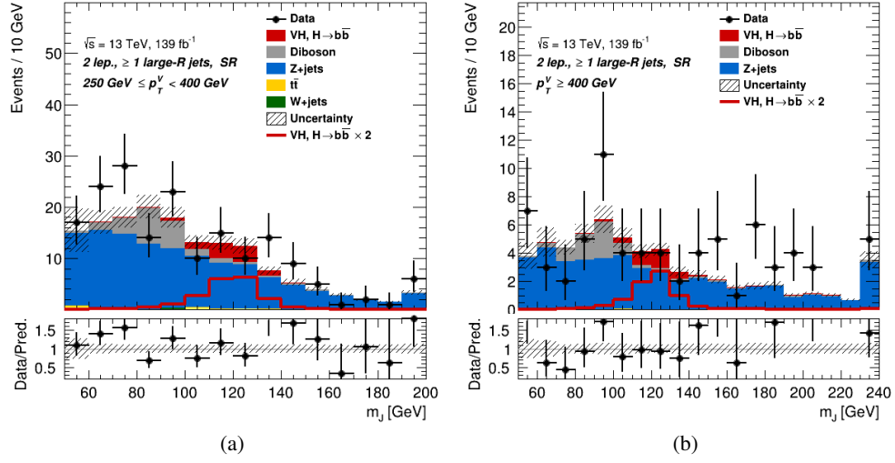
Figure 5.8: The invariant large- R jet mass m_J pre-fit distribution in the 2-lepton channel in the SR in the 250 \text{ GeV} \leq p_T^V < 400 \text{ GeV} (a) and p_T^V \geq 400 \text{ GeV} (b) momentum ranges. The data are shown as black dots. The background contributions are shown as filled histograms. The Higgs boson signal is shown as a filled histogram on the top of the background contribution, and unstacked as an unfilled histogram, multiplied by a factor 2. The size of the combined statistical and systematic uncertainty for the sum of the signal and background is indicated by the hatched band. The highest bin in the distributions contains the overflow. The ratio of the data to the sum of the signal and background is shown in the lower panel.
