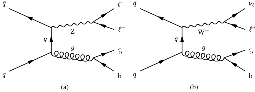
Figure 3.7: Lowest order Feynman diagrams for the quark induced Z +jets (a) and W +jets (b) processes.
