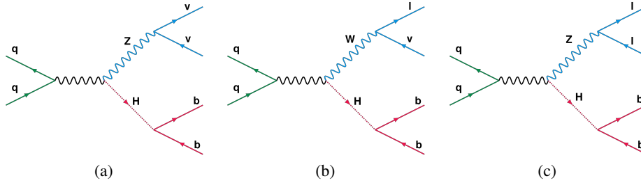
Figure 3.4: Leading order Feynman diagram for ZH \rightarrow \nu\nu b\bar{b} , WH \rightarrow l\nu b\bar{b} and ZH \rightarrow ll b\bar{b} processes with l = e, \mu, \tau . These diagrams represent the 0-, 1-, and 2-lepton channels.
