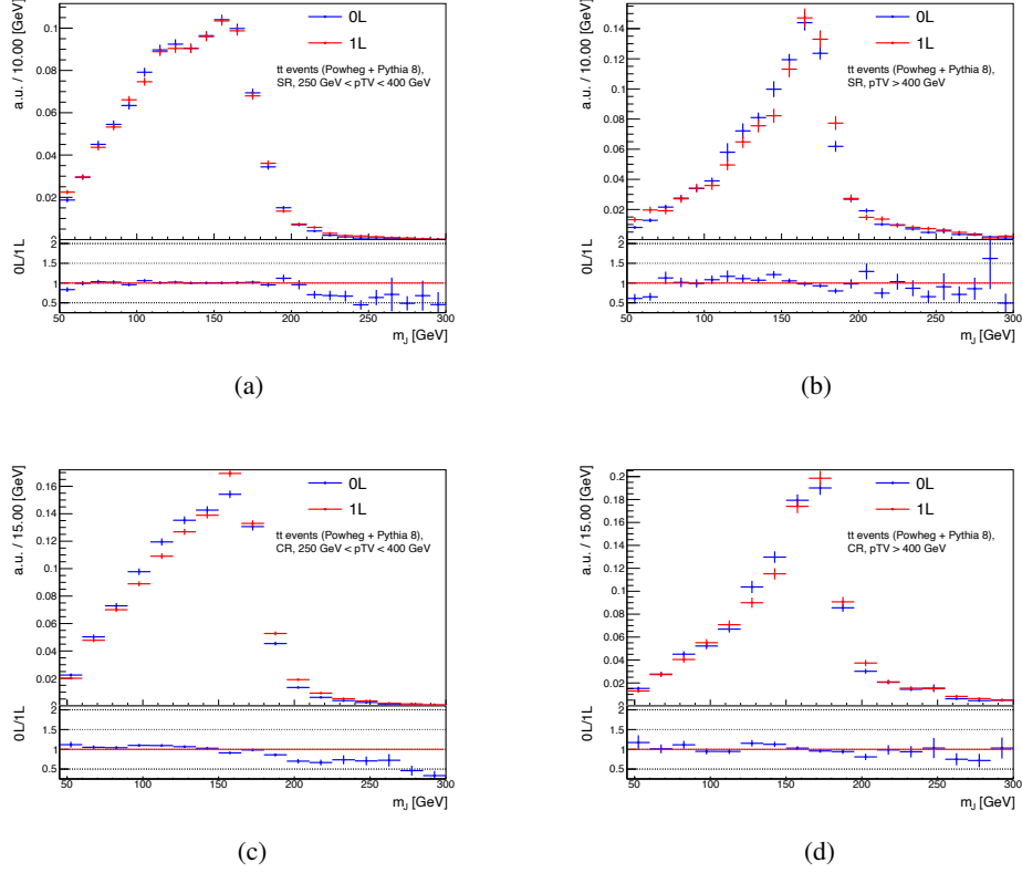
Figure 6.3: Normalised large- R jet mass m_J distribution from t\bar{t} process in the SR (top row) and CR (bottom row) in medium p_T^V (left side) and high p_T^V (right side) region in 0-lepton (blue line) and 1-lepton (red line) channels.
