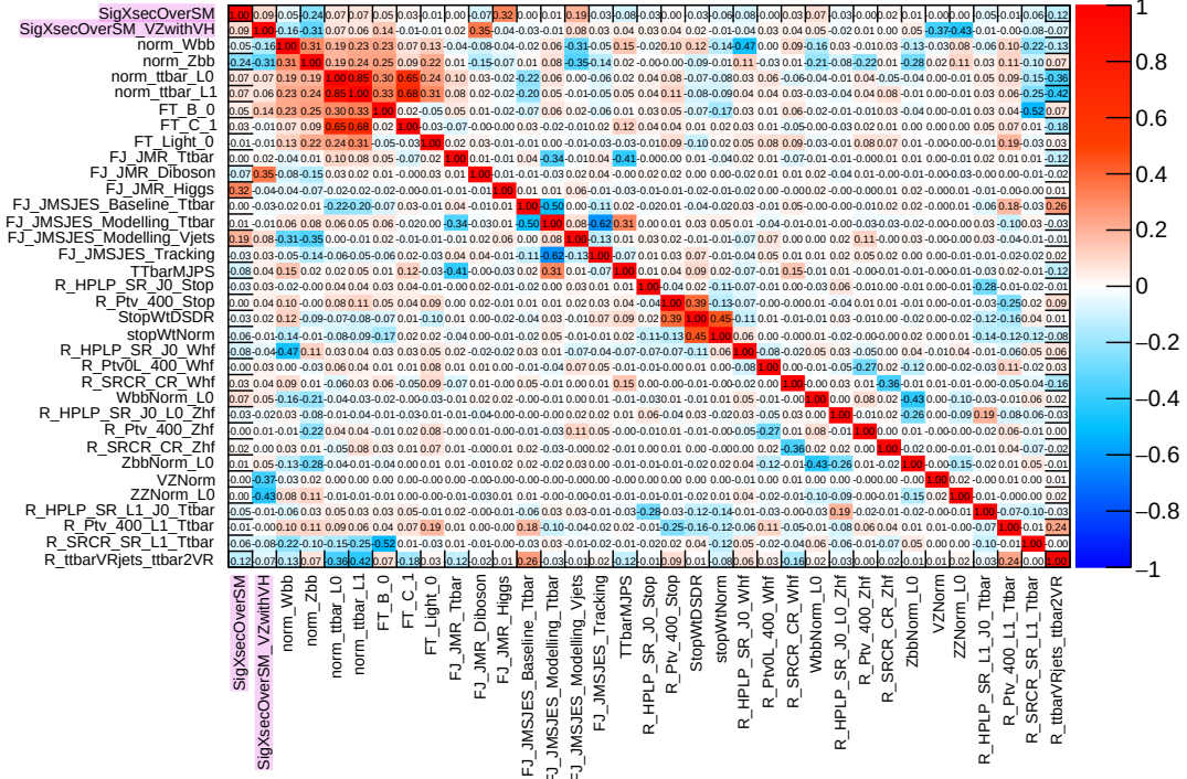
Figure 7.4: Correlation matrix obtained from a fit to the Asimov dataset.
