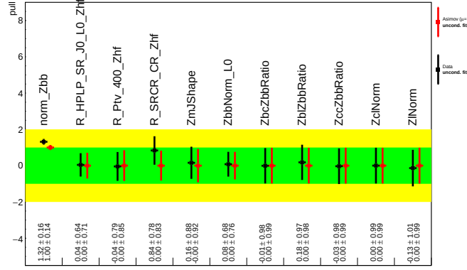
Figure 7.3: Example of pull plot obtained from an unconditional fit to Asimov (red dots) and real dataset (black dots).
