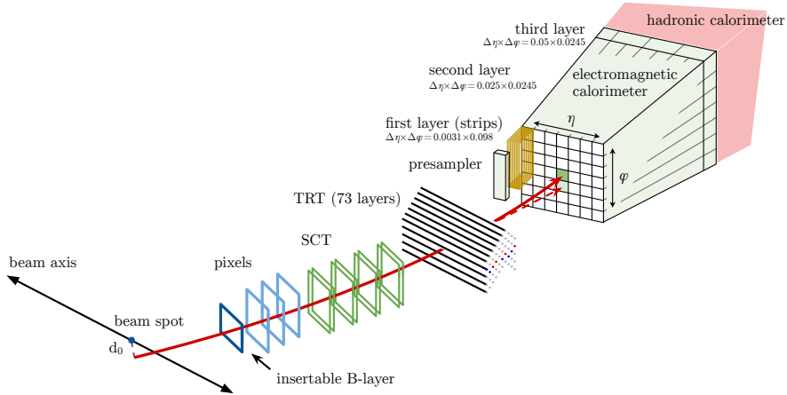
Figure 4.2: Schematic illustration of the path of an electron through the detector. The red trajectory shows the path of an electron while the dashed red trajectory indicates the path of a photon produced by the interaction of the electron with the material of the tracking system [65].
