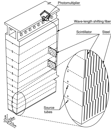
Figure B.1: Illustration of the mechanical assembly and optical read-out of a single TileCal modules [111].
