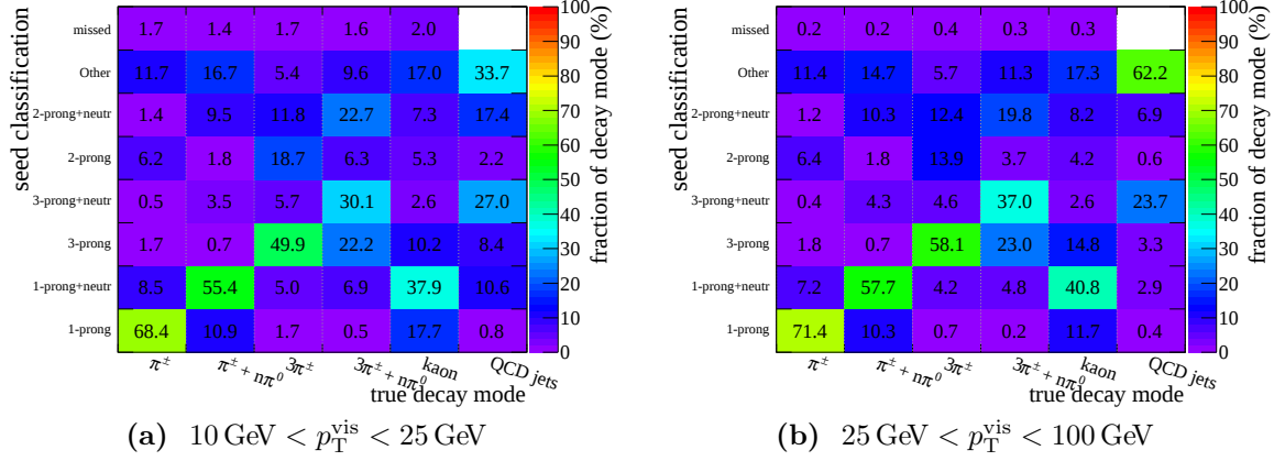
Figure 4.14: Performance of the seed classification in PanTau. Tau candidates in W \rightarrow \tau\nu and Z \rightarrow \tau\tau events are matched to true hadronic tau decays. Distributions are shown for Pythia (DW tune) Monte Carlo samples with tau candidates seeded from cone jets with R = 0.4 in the pseudo-rapidity range |\eta^{\text{vis}}| < 2.0 . Candidates in QCD di-jet events are given for comparison, where the reconstructed E_T and \eta are used instead. The numbers give the percentage of candidates for a given true decay mode, i.e. they are normalised column-wise.
