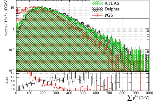
Figure 3.8: \sum_{\text{lep}} p_T in BC 1 signal in different detector simulations. No event selection cuts, despite the cleaning cuts explained in the text, were applied.
