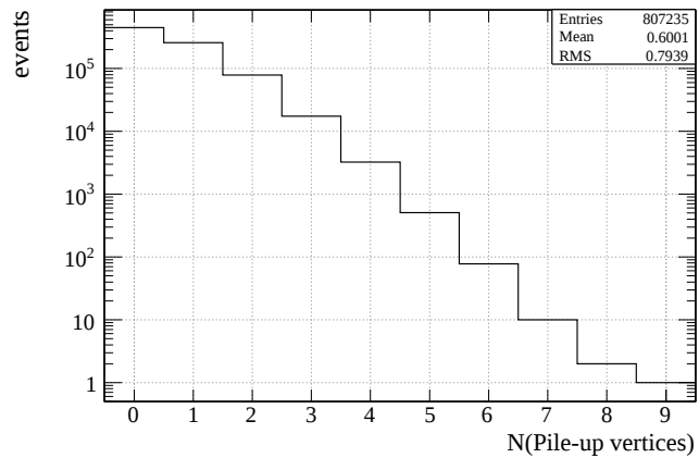
Figure 4.32: Number of reconstructed pile-up vertices in the data events used for the Monte Carlo to data comparisons in this Section. Only events passing the selection cuts given in Table 4.5 are included here.
