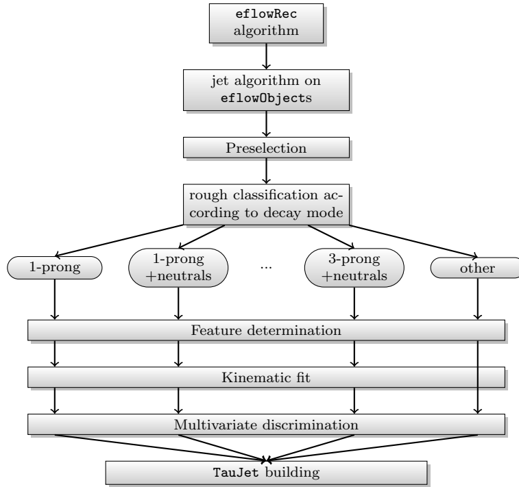
Figure 4.13: Workflow of the PanTau algorithm.
