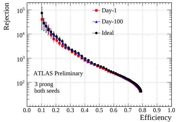
Figure 4.9: Tau efficiency versus jet rejection in the momentum range 10 \text{ GeV} < p_{T_{\text{vis}}}^{\text{MCtruth}} < 30 \text{ GeV} for Z \rightarrow \tau\tau 3-prong candidates (efficiency) and QCD di-jet (rejection). The jet rejection is the inverse of the fake rate, for more details see Section 4.5.3. The performance curves are given for the standard Tau-Rec algorithm with different levels of misalignment of the Inner Detector.
