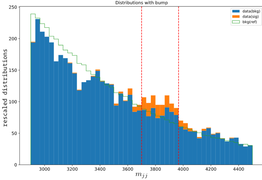
Figure 7.17.: Results of bump hunting after comparing the Black Box 1 data, depicted as a green line, with the subsample of 99 th percentile anomalous events, depicted as coloured bars: blue for background events and orange for signal events. Signal and background labels were added after the fact, the unblinding being used to confirm the presence of real BSM signal.
