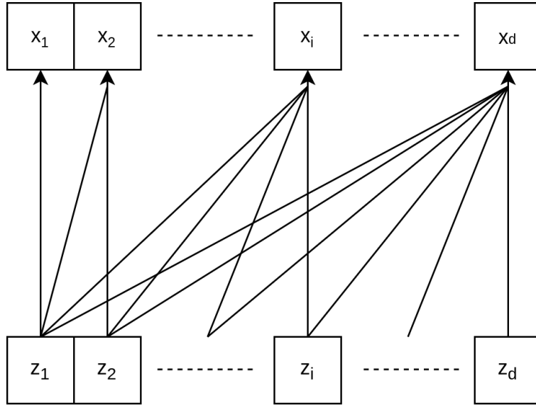
Figure 7.5.: Schematic representation between the input z and output x of an autoregressive transformation T , where x = T(z) .
