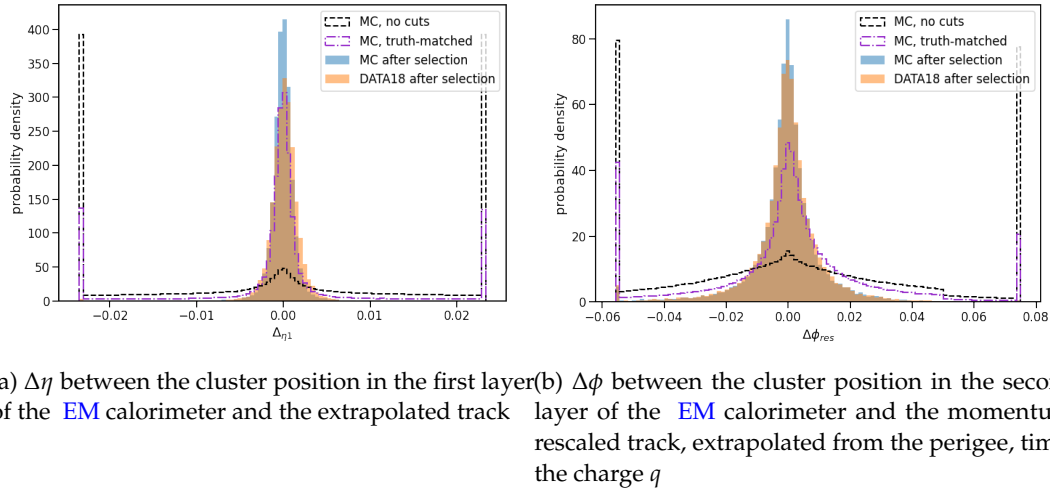
Figure 4.7.: Normalized distributions of \Delta\eta_1 (a) and \Delta\phi_{\text{res}} (b), shower shape electron identification variables related track-cluster matching. Electron samples have been obtained by applying the selection model to EGAM1 derivations of MC (blue) and DATA18 (orange). The reference distributions are presented for all probes before the selection (black) and probes truth-matched to b -quarks (Purple) for MC events only.
