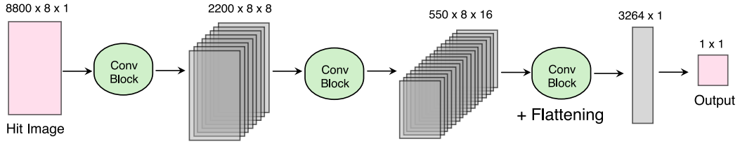
Figure 6.12.: Neural Network architecture deployed in \Delta\Theta regression
