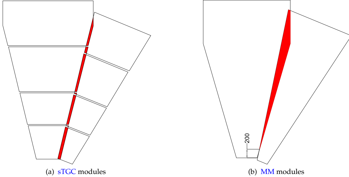
Figure 2.11.: Representation of active area overlap between small and large sectors [42].
