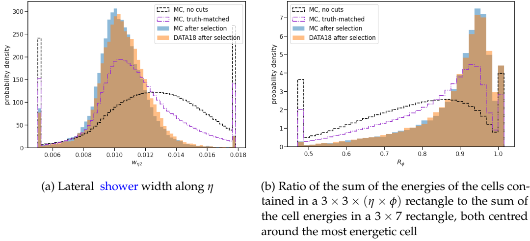
Figure 4.5.: Normalized distributions of w_{\eta 2} (a) and R_{\phi} (b), electron identification variables related to the second layer of the Electromagnetic (EM) calorimeter. Electron samples have been obtained by applying the selection model to EGAM1 derivations of Monte Carlo (blue) and DATA18 (orange). The reference distributions are presented for all probes before the selection (black) and probes truth-matched to b -quarks (Purple) for MC events only.
