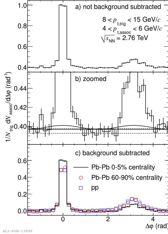
Figure 1.6: Jet quenching at ALICE [36]. Corrected per-trigger pair yield for 4 < p_{T,\text{assoc}} < 6 \text{ GeV}/c for central Pb-Pb events (histogram), peripheral Pb-Pb (red circles) and pp collisions (blue squares).
