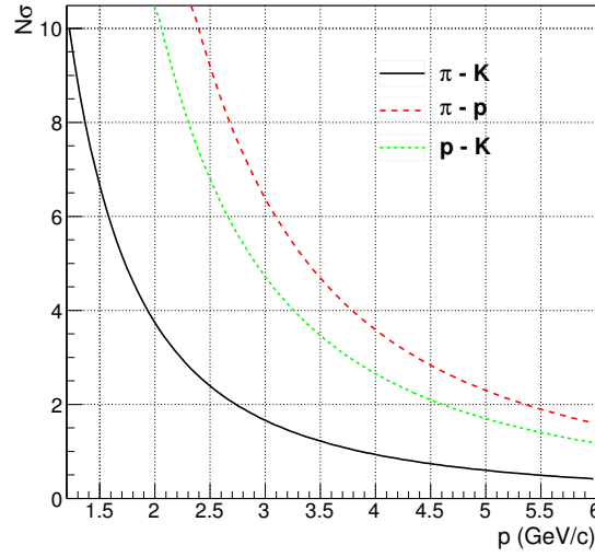
Figure 5.8: Expected separation between the times-of-flight of the \pi , K and p hadrons measured in n\sigma_{PID} units (Equation 5.13).
