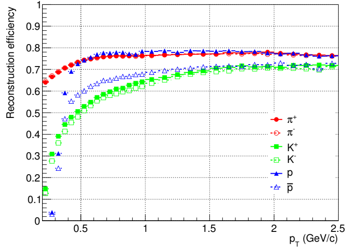
Figure 5.21: Track reconstruction efficiency for pion (red), kaon (green) and proton (blue) tracks.
