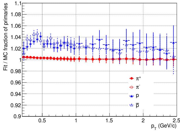
Figure 6.24: Ratio between the fraction of primary tracks measured in the data and generated by Monte Carlo (tracks passing the standard track cuts).
