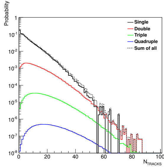
Figure A-1: Multiplicity distributions of single-event (black), and double (red), triple (green) and quadruple (blue) pile-up, generated using Poisson probabilities with a \mu = 0.07 . The single-event distribution is normalised to 1 (normalisation is explained in the text). Even though the overall amount of pile-up in the data is about 3.0%, it becomes dominant at high multiplicities. The sum of all the contributions is shown with a dashed black line.
