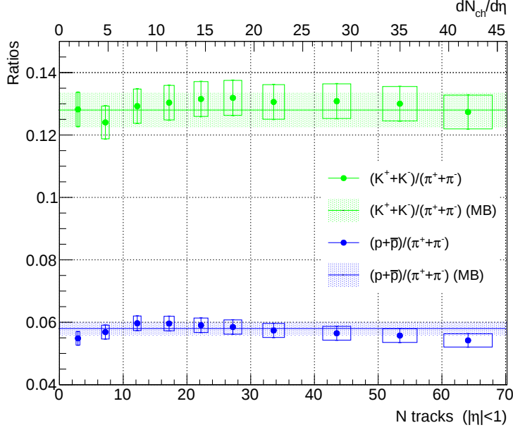
Figure 7.17: The measured (K^+ + K^-)/(\pi^+ + \pi^-) and (p + \bar{p})/(\pi^+ + \pi^-) ratios as a function of multiplicity. The green and blue lines represent the values for MB events.
