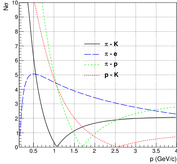
Figure 5.6: Momentum dependence of the TPC \langle dE/dx \rangle separation for the most important particle combinations in units of \sigma_{dE/dx} .
