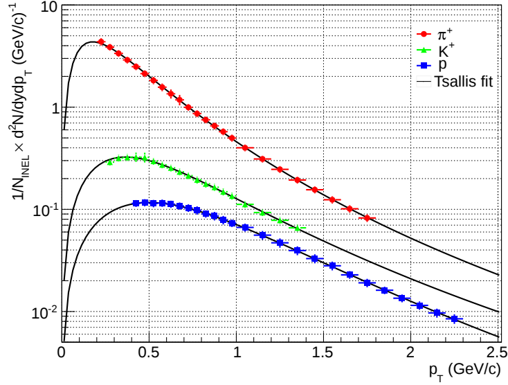
Figure 7.1: Measured p_T spectra of positive pions, kaons and protons in MB p-p events at \sqrt{s} = 7 TeV. The yields are normalised to the number of inelastic collisions, N_{\text{INEL}} . The black lines correspond to the Tsallis distribution used to extract the mean transverse momenta and integrated yields.
