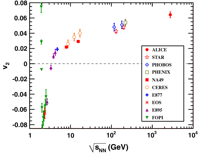
Figure 1.7: Elliptic flow in Pb-Pb collisions at \sqrt{s_{NN}} = 2.76 TeV and collision centrality of 20-30% as measured by ALICE [47], shown with results from lower energies and similar centralities.
