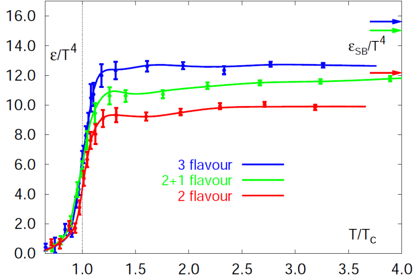
Figure 1.2: The energy density of hadronic matter from Lattice QCD calculations [17] in units of T^4 . The curves labelled ‘2 flavour’ and ‘3 flavour’ present calculations done with two and three light (massless) quark flavours. The ‘2+1 flavour’ indicates a calculation for two light flavours and a heavier strange quark. Including all quarks in the lattice QCD calculations is computationally demanding. However, at a temperature of 200 MeV, the thermal production of charm, top and bottom will have negligible influence on the equation of state. The arrows represent the predicted Stefan-Boltzmann values (discussed in the text).
