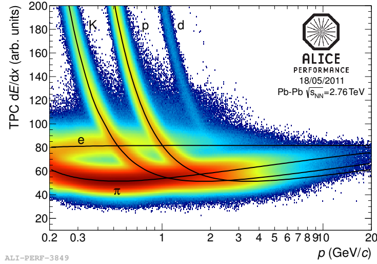
Figure 5.4: TPC dE/dx of charged particles as a function of their momentum p . The black lines correspond to the Bethe-Bloch parametrisation of the detector response.
