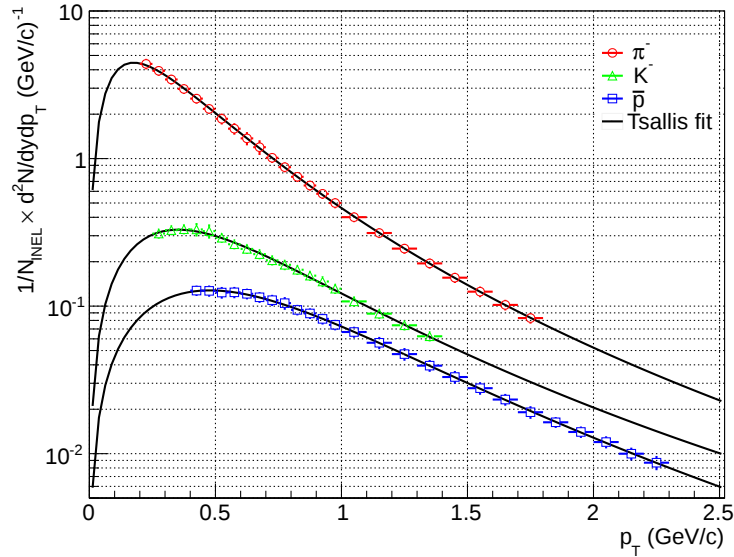
Figure 7.2: Measured p_T spectra of negative pions, kaons and protons in MB p-p events at \sqrt{s} = 7 TeV. The yields are normalised to the number of inelastic collisions, N_{\text{INEL}} . The black lines correspond to the Tsallis distribution used to extract the mean transverse momenta and integrated yields.
