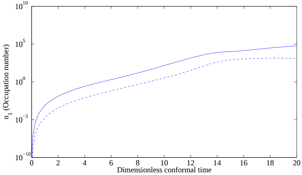
Figure 4.2: Occupation number for one of the excited fields as a function of dimensionless conformal time, obtained using eq. (4.25) after numerically integrating the background field equations and Bogolyubov matrices; k = \mu_1/3 \times 10^5 , other parameters as explained in the text. The solid lines represents preheated fields with \varphi_{20}/\varphi_{10} = 1 while the dashed lines indicate the preheated fields with \varphi_{20}/\varphi_{10} = 0.1
