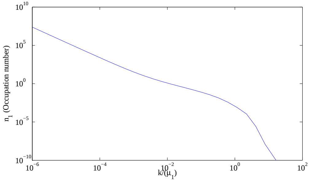
Figure 4.3: Occupation number as a function of comoving momentum obtained as for FIG. 4.2, with \varphi_{20}/\varphi_{10} = 0.5 at time t = 20 .
