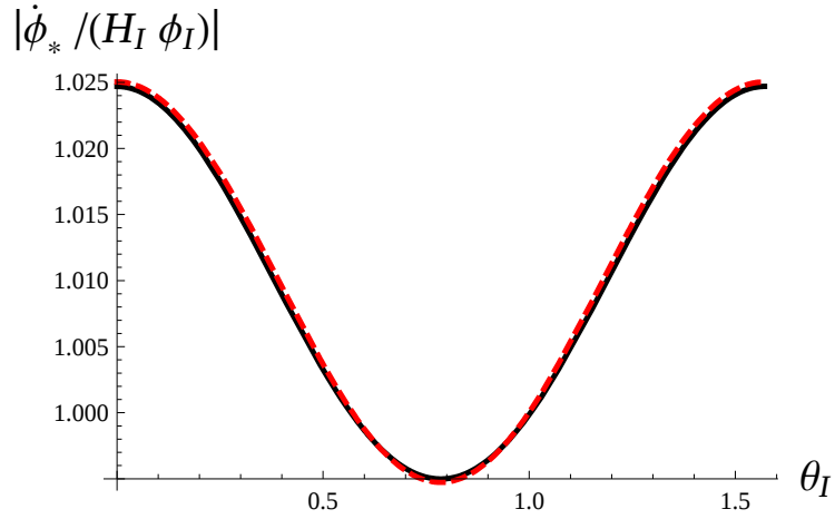
Figure 3.2: The angular dependence of the flat direction velocity |\dot{\phi}_*| at \phi_* (the minimum distance from the origin) plotted for a_{\text{osc}} = 0.003 and n = 4 in units of H_I |\phi_I| (see Appendix A). The numerical evaluation (with \beta = 0.1 and \lambda = 0.01 ) is represented by the continuous line, while the analytical estimate of Eq. (3.13) is dashed.
