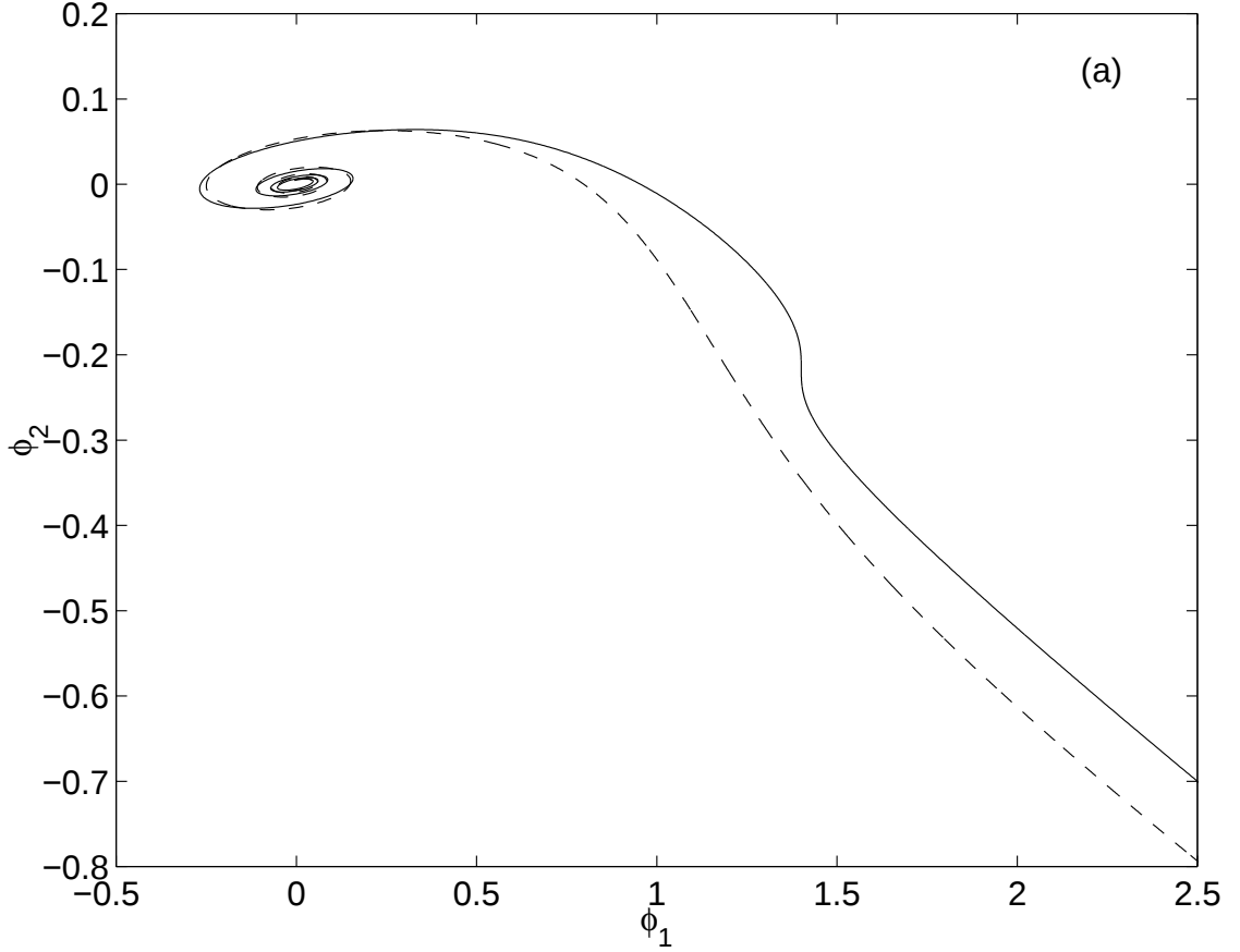
Figure 4.1: Motion of the flat direction VEV in the complex plane for n = 4 (solid) and n = 6 (dashed) with initial condition \theta = -\pi/10 . Taken from [74].
