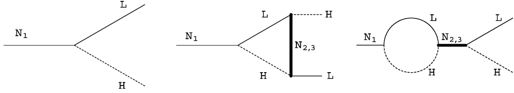
Figure 2.1: The Feynman diagrams describing the tree-level and one loop contributions to the decay of the lightest RH neutrino N_1 .
