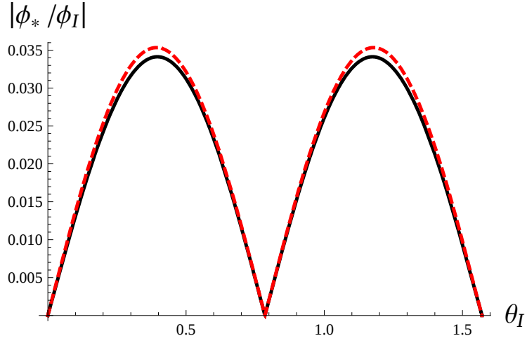
Figure 3.1: The angular dependence of |\phi_*| , the minimum distance from the origin plotted in units of its initial value |\phi_I| for a_{\text{osc}} = 0.003 and n = 4 (see Appendix A). The numerical evaluation (with \beta = 0.1 and \lambda = 0.01 ) is represented by the continuous line, while the analytical estimate of Eq. (3.12) is dashed.
