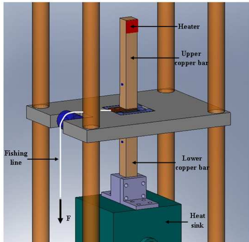
Figure 6.2: Solid Works model of the sandwich placed inside the wooden base
