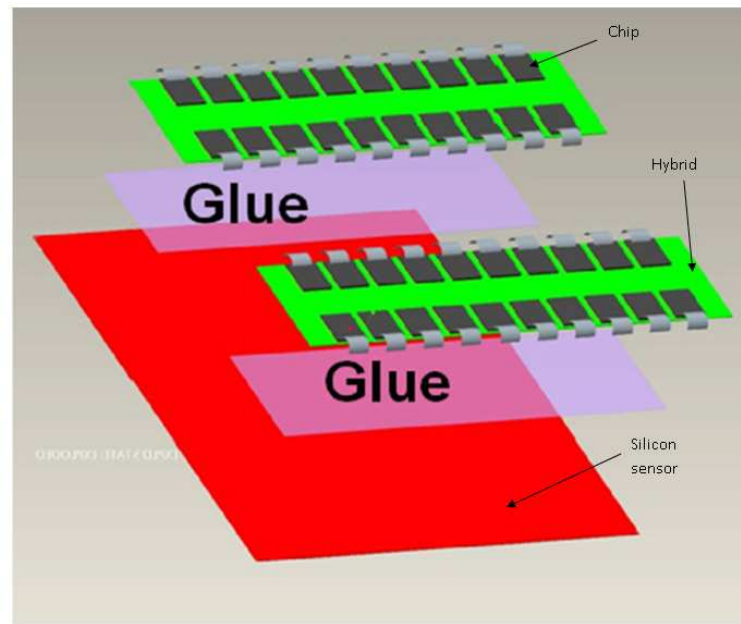
Figure 1.5: Overview of a single sided-module [22]. The red component is the silicon and the green component is the hybrid.
