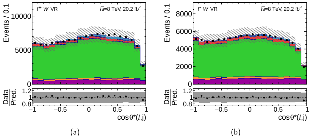
Figure 7.11.: Distributions normalised to the number of expected events of the discriminating variable \cos\theta^*(\ell, j) for the \ell^+ channel (left) and \ell^- channel (right) in the W + \text{jets} VR. The hatched uncertainty band represents the uncertainty in the pre-fit process cross-sections and the bin-by-bin MC statistical uncertainty, added in quadrature. The ratio of observed to predicted (Pred.) number of events in each bin is shown in the lower panel.
