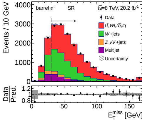
(a) Barrel electron channel in the SR.
