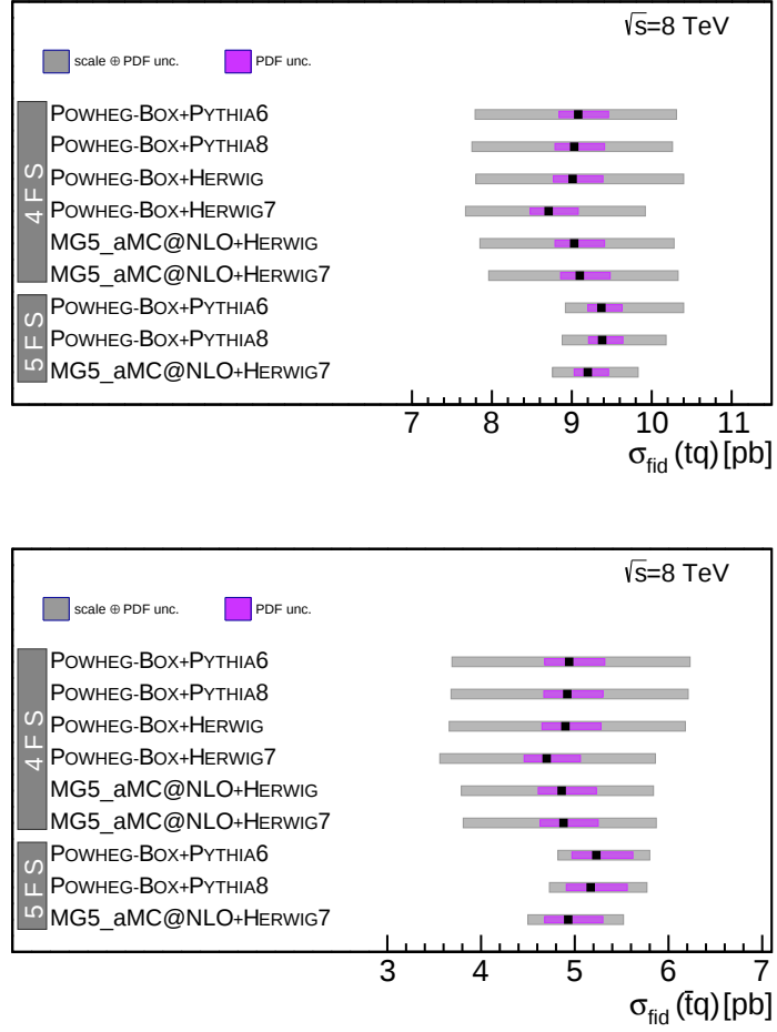
Figure 6.3.: Predicted t -channel single top-quark and top-antiquark fiducial cross-sections for different NLO MC generators. The uncertainty on the predictions consists of the scale uncertainty and the uncertainty on the PDFs.
