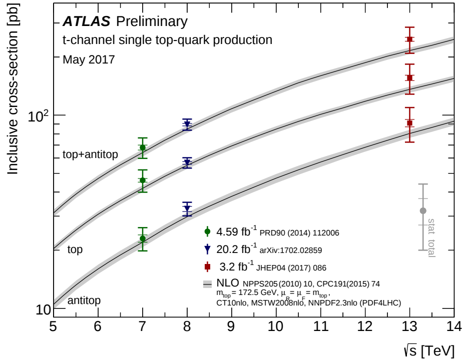
Figure 9.1.: Summary of the t -channel single top-quark measurements performed at \sqrt{s} = 8 TeV with the ATLAS and CMS experiments in (a) and ATLAS measurements for 7, 8 and 13 TeV center-of-mass energies [165] in (b).
