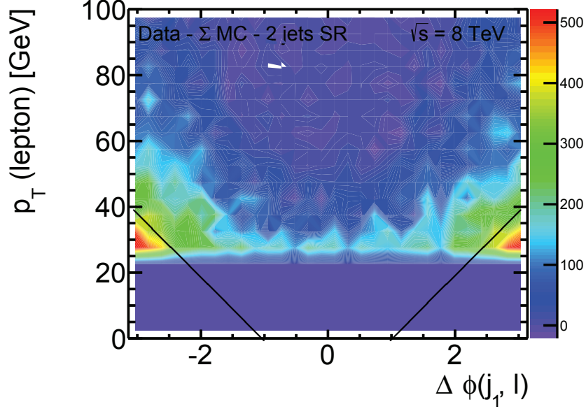
Figure 5.3.: The event rate dependence on the lepton p_T and the \Delta\phi(j_1, \ell) for data after subtracting the MC predictions for all background processes.
