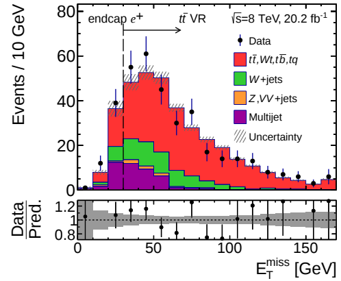
(f) Endcap electron channel in the t\bar{t} VR.
