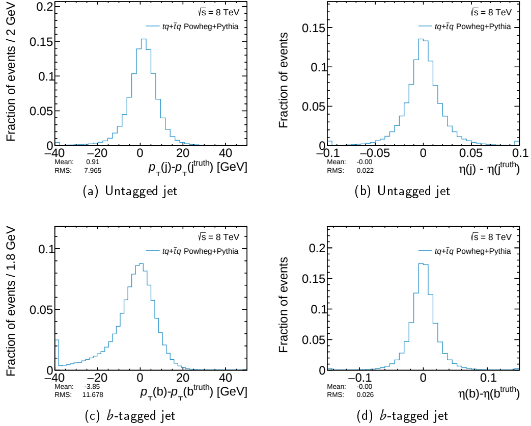
Figure 4.5.: The residual distribution of reconstructed jets for selected leptons of t -channel single top-quark events. Figures (a) and (b) show the p_T and \eta distributions for the untagged jet, and Figures (c) and (d), show the same quantities for the tagged jet. Values beyond the axis range are contained in the first and last bin.
