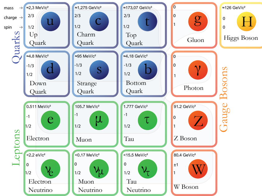
Figure 1.1.: Summary of the Standard Model of particle physics. On the left-hand side all fermions are specified, subdivided into quarks and leptons. The right-hand side shows the bosons of the SM, which mediate the weak, strong and electromagnetic interactions as well as the Higgs boson. The mass, charge and spin of all particles is given in the respective box. The generations of fermions are grouped vertically.[12, 13]
