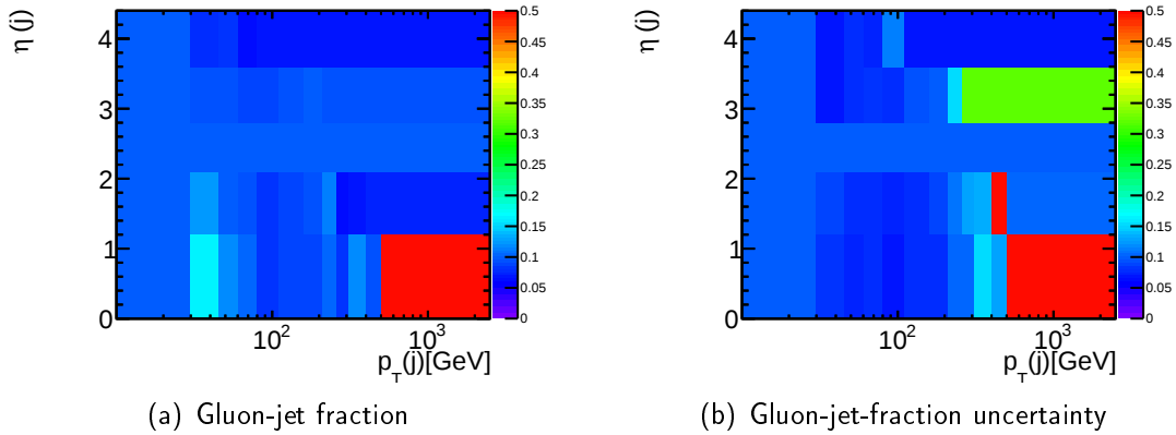
Figure 8.9.: Gluon fraction of non b -jets (a) and the corresponding uncertainty (b).
