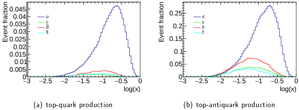
Figure 3.4.: Distribution of the momentum fraction x of the partons in t -channel single top-quark events in (a), for all involved initial quarks ( u, c, \bar{d}, \bar{s} ), and for the top-antiquark production in (b) for the involved initial quarks ( d, s, \bar{u}, \bar{c} ).
