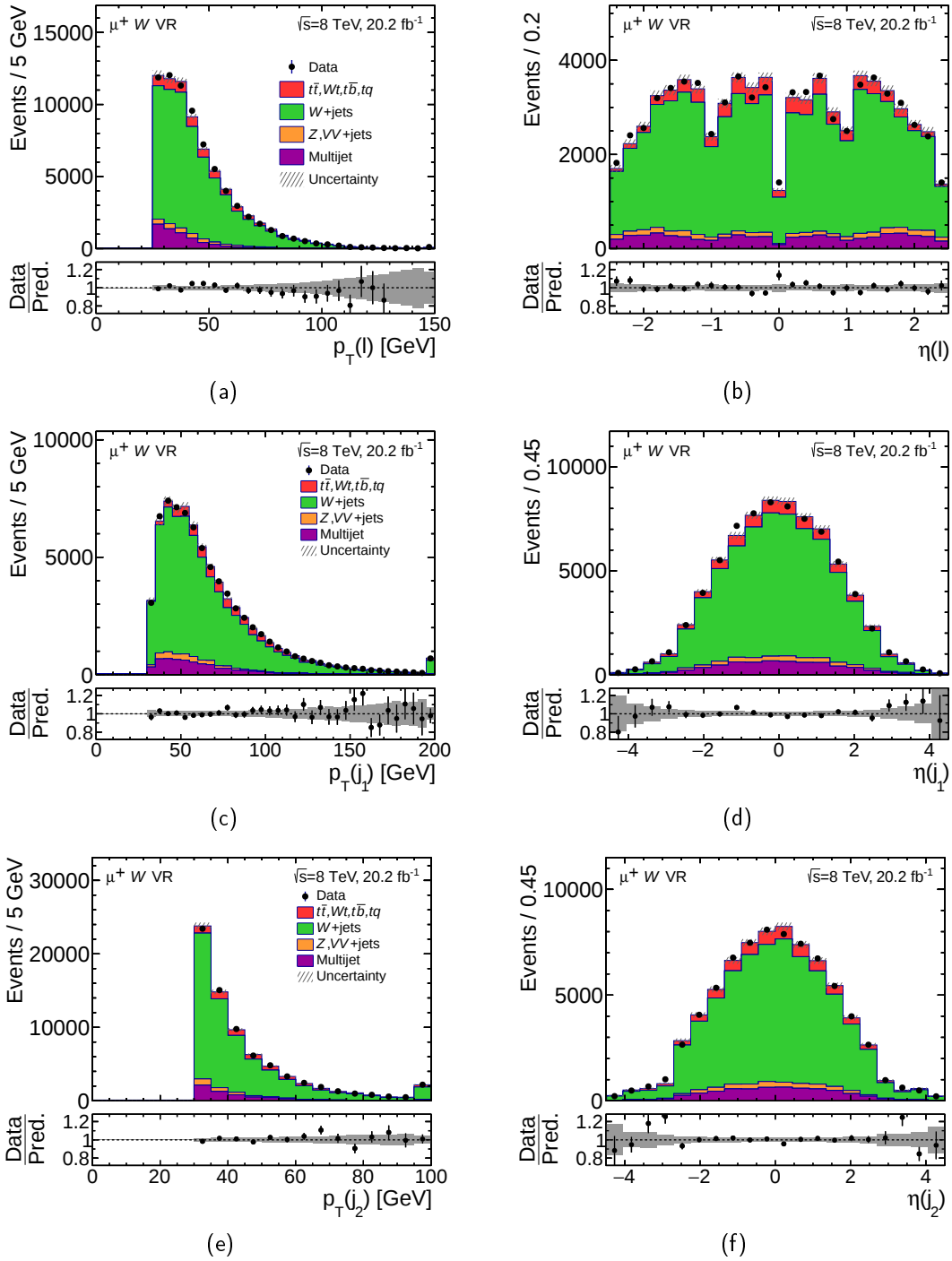
Figure 5.11.: Kinematic distributions in the W + \text{jets} VR for the \mu^+ channel. (a) p_T and (b) \eta of the muon, (c) p_T and (d) \eta of the leading jet and, (e) p_T and (f) \eta of the sub-leading jet. The hatched error band represents the uncertainty on the multijet rate as well as the MC statistical uncertainty. The ratio of observed to predicted (Pred.) number of events in each bin is shown in the lower panel. Events beyond the axis range are included in the last bin.
