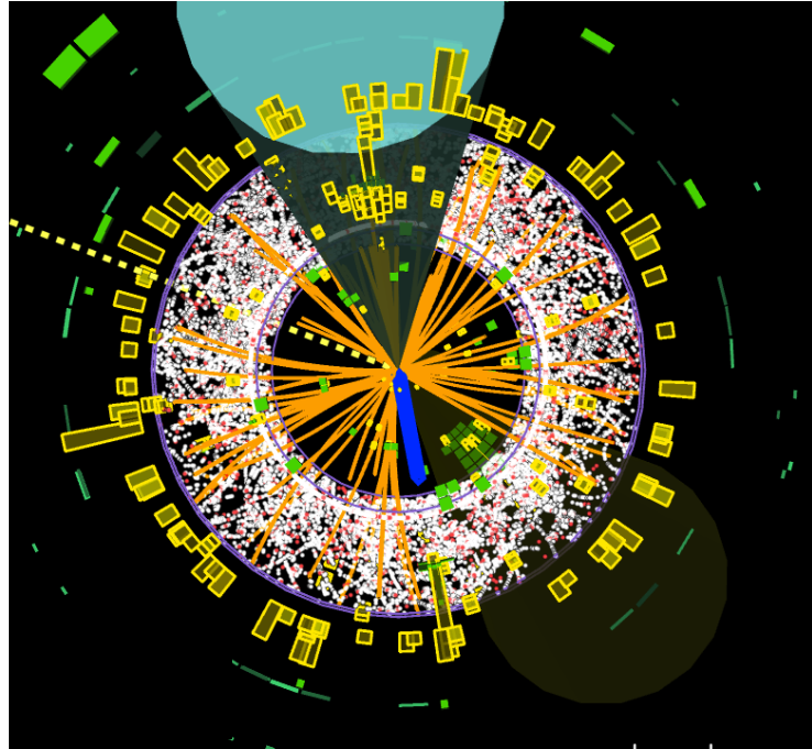
Figure 4.1.: Exemplary event display of a t -channel single top-quark event candidate in the electron channel [112]. The x - y projection at z = 0 is shown. The collision takes place in the center and the hits of the detectable particles in the TRT are seen as white dots. The orange lines show the reconstructed tracks and the yellow towers show the combined energy deposition in the calorimeter system. The blue line indicates the direction of the selected electron. The yellow and blue cones illustrate the reconstructed jets in the event.
