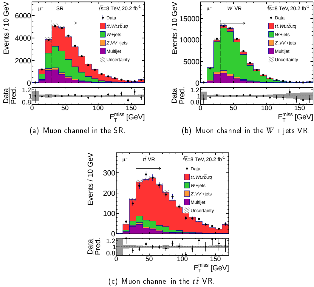
Figure 5.8.: Result of the binned maximum-likelihood fit to the E_T^{\text{miss}} distributions for the signal region (a), the W + jets VR (b), and t\bar{t} VR (c) for the muon channel with negative charge. The dashed vertical line indicates the threshold of the respective selection region. The ratio of observed to predicted (Pred.) number of events in each bin is shown in the lower panel.
