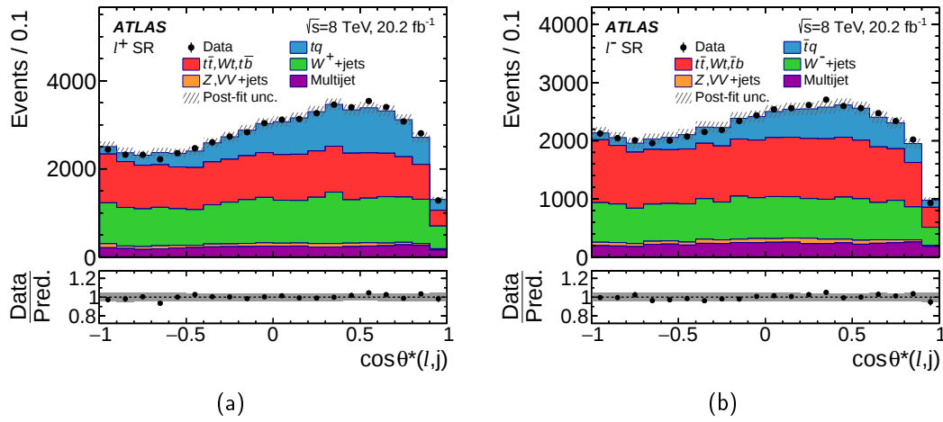
Figure 8.6.: The observed distribution of the \cos\theta^*(\ell, j) input variable in the signal region of (a) the \ell^+ channel channel and (b) the \ell^- channel channel is compared to the distribution of simulated signal and background events normalised to the number of fitted events. The uncertainty band represents the post-fit normalisation uncertainty and the uncertainty due to limited sample size. The ratio between the observed and expected number of events in each bin is shown in the lower panel.
