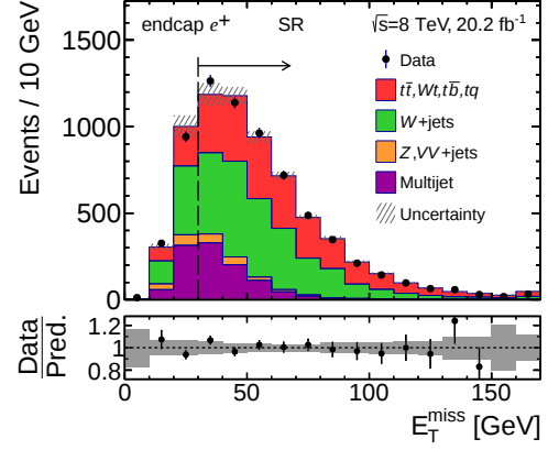
(b) Endcap electron channel in the SR.
