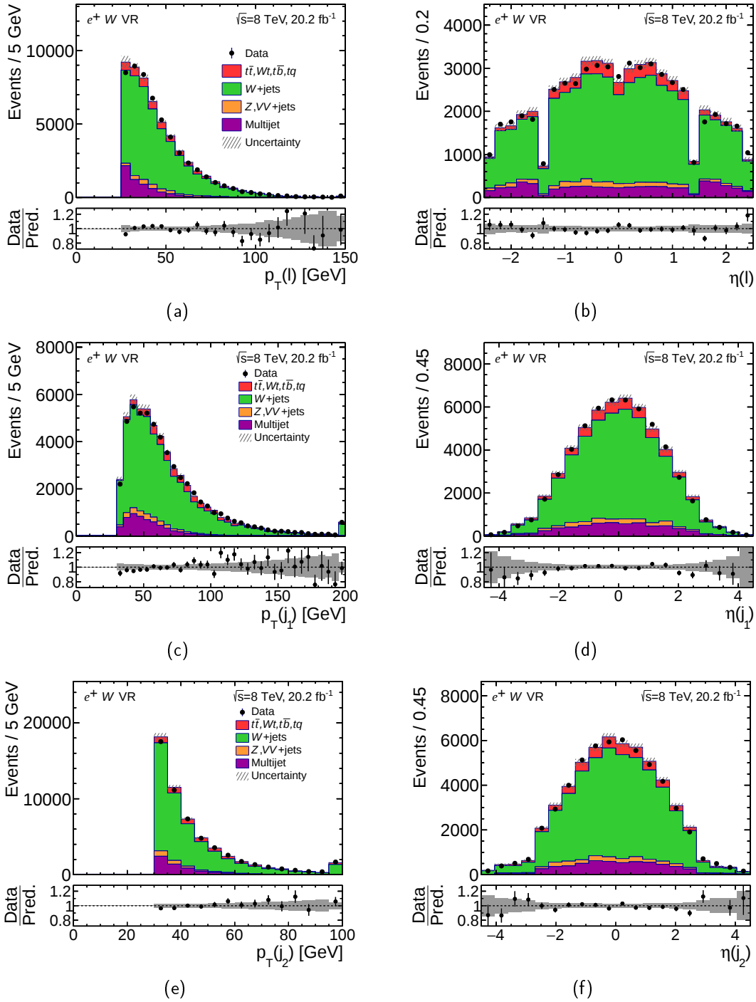
Figure 5.9.: Kinematic distributions in the W + jets VR for the e^+ channel. (a) p_T and (b) \eta of the electron, (c) p_T and (d) \eta of the leading jet and, (e) p_T and (f) \eta of the sub-leading jet. The hatched error band represents the uncertainty on the multijet rate as well as the MC statistical uncertainty. The ratio of observed to predicted (Pred.) number of events in each bin is shown in the lower panel. Events beyond the axis range are included in the last bin.
