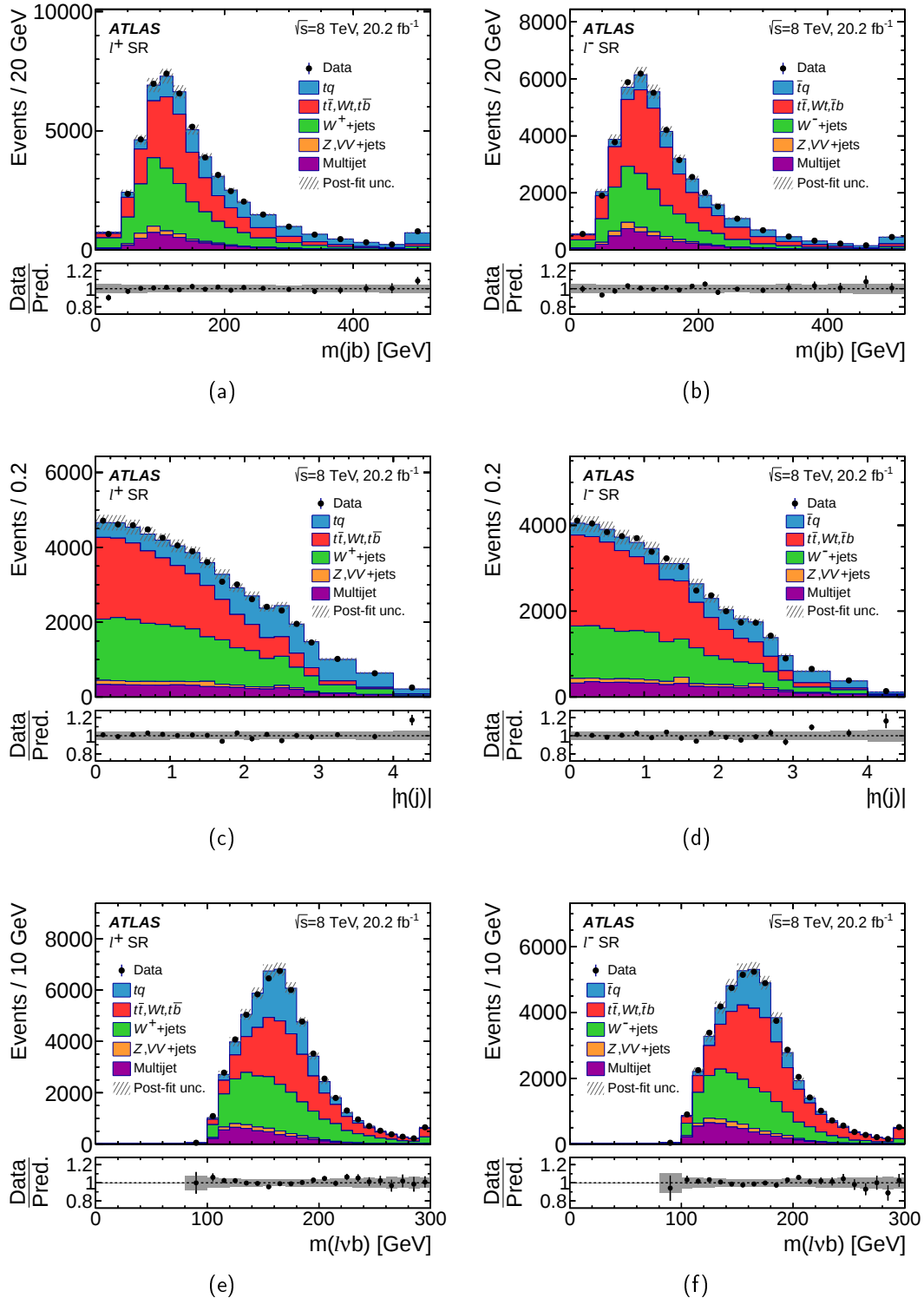
Figure 8.4.: The observed distribution of the three most discriminating input variables in the signal region of (left) the \ell^+ channel and (right) the \ell^- channel is compared to the distribution of simulated signal and background events normalised to the number of fitted events. The uncertainty band represents the post-fit normalisation uncertainty and the uncertainty due to limited sample size. The ratio between the observed and expected number of events in each bin is shown in the lower panel.
