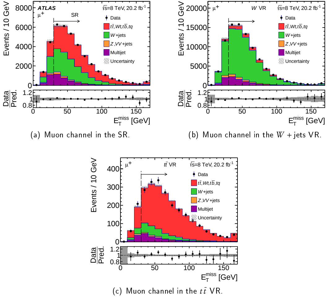
Figure 5.7.: Result of the binned maximum-likelihood fit to the E_T^{\text{miss}} distributions for the SR (a), the W + jets VR (b), and the t\bar{t} VR (c) for the muon channel with positive charge. The dashed vertical line indicates the threshold of the respective selection region. The ratio of observed to predicted (Pred.) number of events in each bin is shown in the lower panel.
