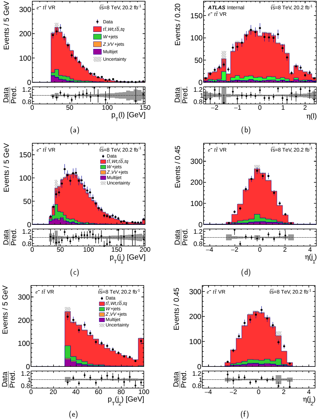
Figure 5.14.: Kinematic distributions in the t\bar{t} VR for the e^- channel. (a) p_T and (b) \eta of the electron, (c) p_T and (d) \eta of the leading jet and, (e) p_T and (f) \eta of the sub-leading jet. The hatched error band represents the uncertainty on the multijet rate as well as the MC statistical uncertainty. The ratio of observed to predicted (Pred.) number of events in each bin is shown in the lower panel. Events beyond the axis range are included in the last bin.
