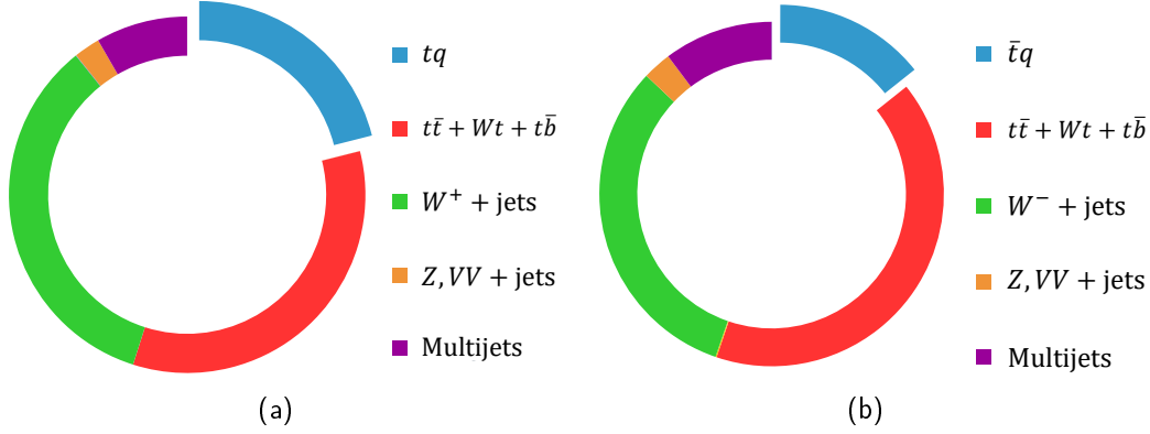
Figure 5.2.: Relative event yield of the \ell^+ channel in (a) and the \ell^- channel in (b) after the full selection is applied.
