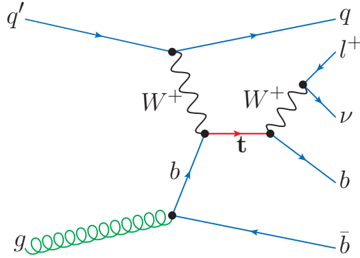
Figure 5.1.: Example Feynman diagram of the t -channel single top-quark production and semi-leptonic decay in the 4FS at LO QCD
