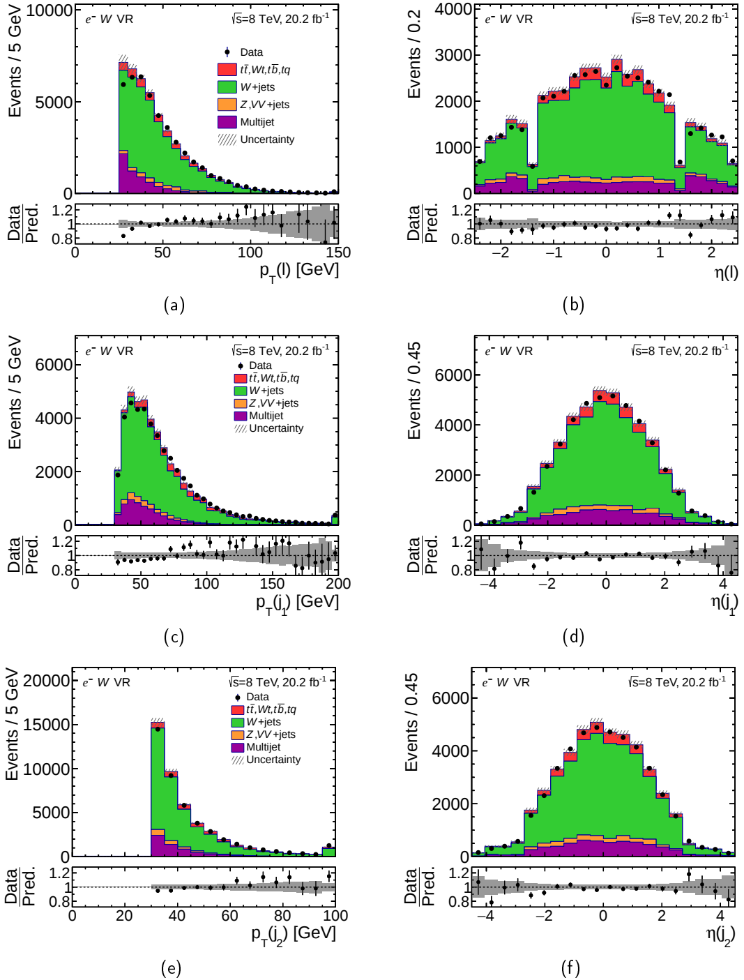
Figure 5.10.: Kinematic distributions in the W + jets VR for the e^- channel. (a) p_T and (b) \eta of the electron, (c) p_T and (d) \eta of the leading jet and, (e) p_T and (f) \eta of the sub-leading jet. The hatched error band represents the uncertainty on the multijet rate as well as the MC statistical uncertainty. The ratio of observed to predicted (Pred.) number of events in each bin is shown in the lower panel. Events beyond the axis range are included in the last bin.
