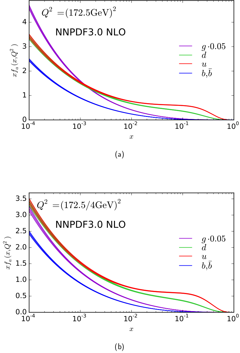
Figure 1.3.: Parton distribution functions of NNPDF 3.0 at NLO and \alpha_s(m_Z) = 0.118 . The distributions of the valence quarks u and d are shown with the b, \bar{b} sea-quarks and the gluon. The gluon PDF is scaled by 0.05. The Q^2 = m_t^2 = (172.5 \text{ GeV})^2 is chosen for (a) and Q^2 = (m_t/4 \text{ GeV})^2 in (b).
