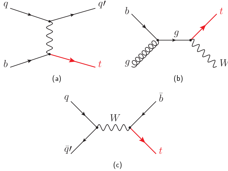
Figure 1.5.: Feynman diagrams of the dominant single top-quark production modes. The t -channel production is shown in (a) at the LO representation in the 5 FS. The Wt -channel and s -channel LO representations are shown in (b) and (c), respectively.
