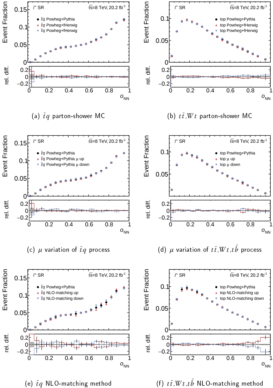
Figure 8.13.: The template shape components of the signal-modeling (left) and top-background modeling (right) uncertainties in the \ell^- channel.
