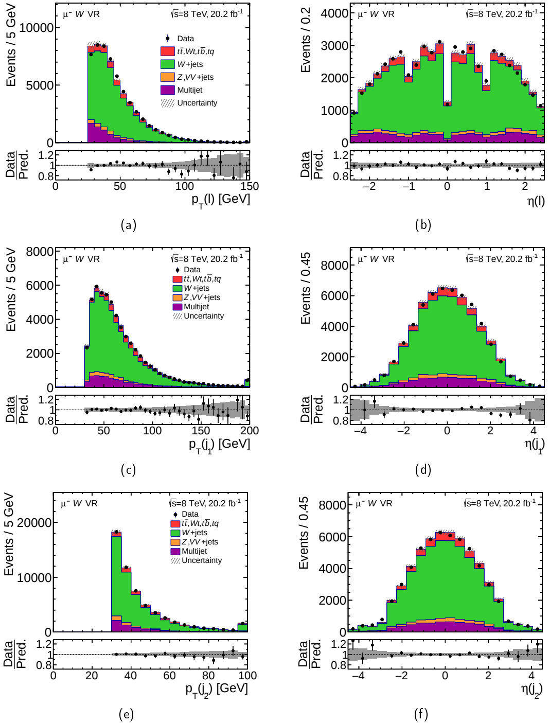
Figure 5.12.: Kinematic distributions in the W + jets VR for the \mu^- channel. (a) p_T and (b) \eta of the muon, (c) p_T and (d) \eta of the leading jet and, (e) p_T and (f) \eta of the sub-leading jet. The hatched error band represents the uncertainty on the multijet rate as well as the MC statistical uncertainty. The ratio of observed to predicted (Pred.) number of events in each bin is shown in the lower panel. Events beyond the axis range are included in the last bin.
