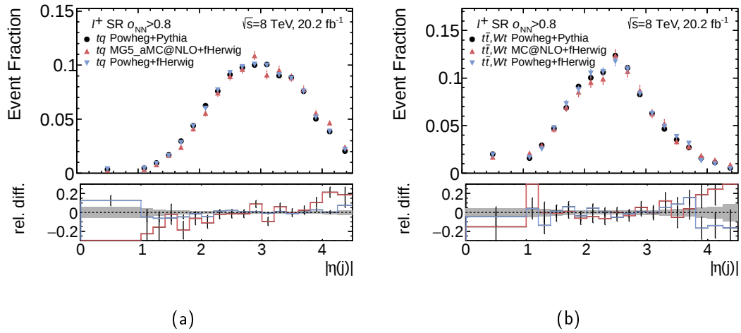
Figure 8.14.: Distribution of |\eta(j)| in the SR + O_{NN} > 0.8 region, for the signal process in (a) and for the t\bar{t} + Wt processes in (b). The nominal POWHEG-BOX + PYTHIA 6 MC generator is compared to POWHEG-BOX + HERWIG and MADGRAPH 5_aMC@NLO + HERWIG.
