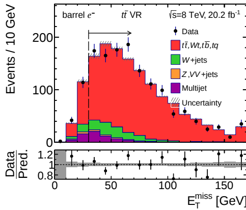
(e) Barrel electron channel in the t\bar{t} VR.
