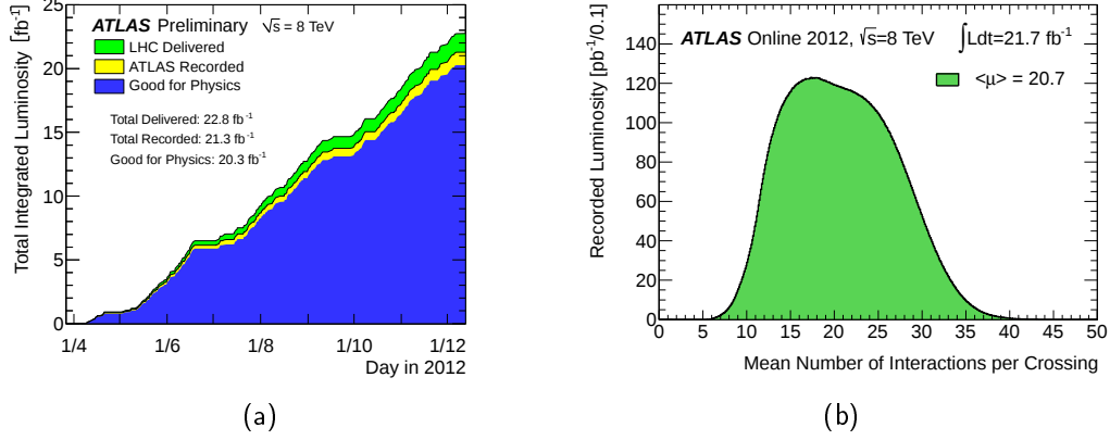
Figure 3.1.: Delivered LHC luminosity and ATLAS recorded in 2012 shown in (a) and average interactions per bunch-crossing for the 2012 dataset in (b). [81]
