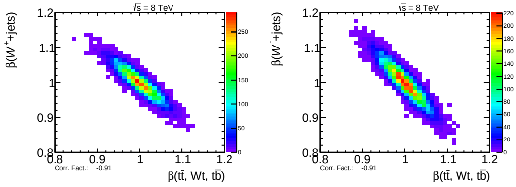
Figure 8.2.: Correlation of the W + \text{jets} and t\bar{t} + Wt + t\bar{b} background processes in the \ell^+ channel in (a) and the \ell^- channel in (b).
