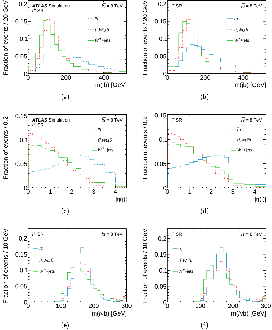
Figure 7.5.: Distributions normalised to unit area of the discriminating variables m(jb) , |\eta(j)| and m(\ell\nu b) for the \ell^+ channel (left) and \ell^- channel (right) in the SR.
