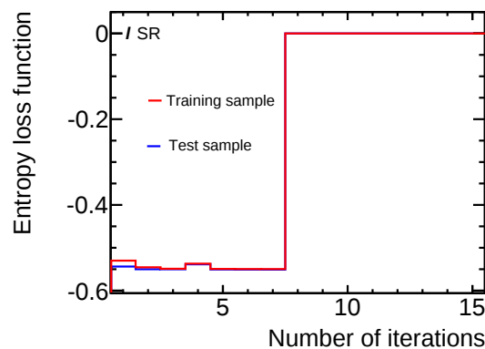
Figure 7.1.: Entropy loss function as a function of the number of training iterations. The training sample is shown in red, the test sample shown in blue.
