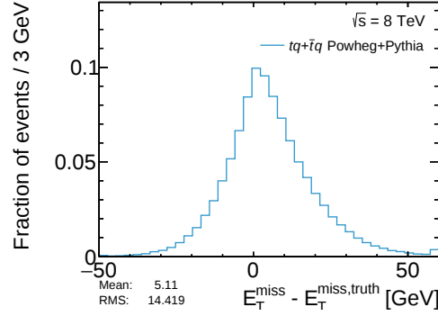
Figure 4.4.: The residual distribution of the reconstructed E_T^{\text{miss}} for selected events. The mean value of the distribution corresponds to a systematic bias in the reconstruction process. Values beyond the axis range are contained in the first and last bin.
