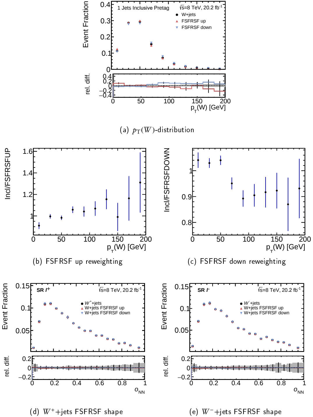
Figure 8.16.: Figure (a) shows the p_T(W) -distribution for all three MC samples. A reweighting is derived by scaling the inclusive W +jets MC sample to the FSFRSF up and down variation. Figures (b) and (c) show the weights assigned to each bin in the p_T(W) -distribution. The reweighting is applied on the nominal Sherpa W +jets MC samples, yielding the shape uncertainty templates for the O_{NN} distribution, see Figures (d) and (e).
