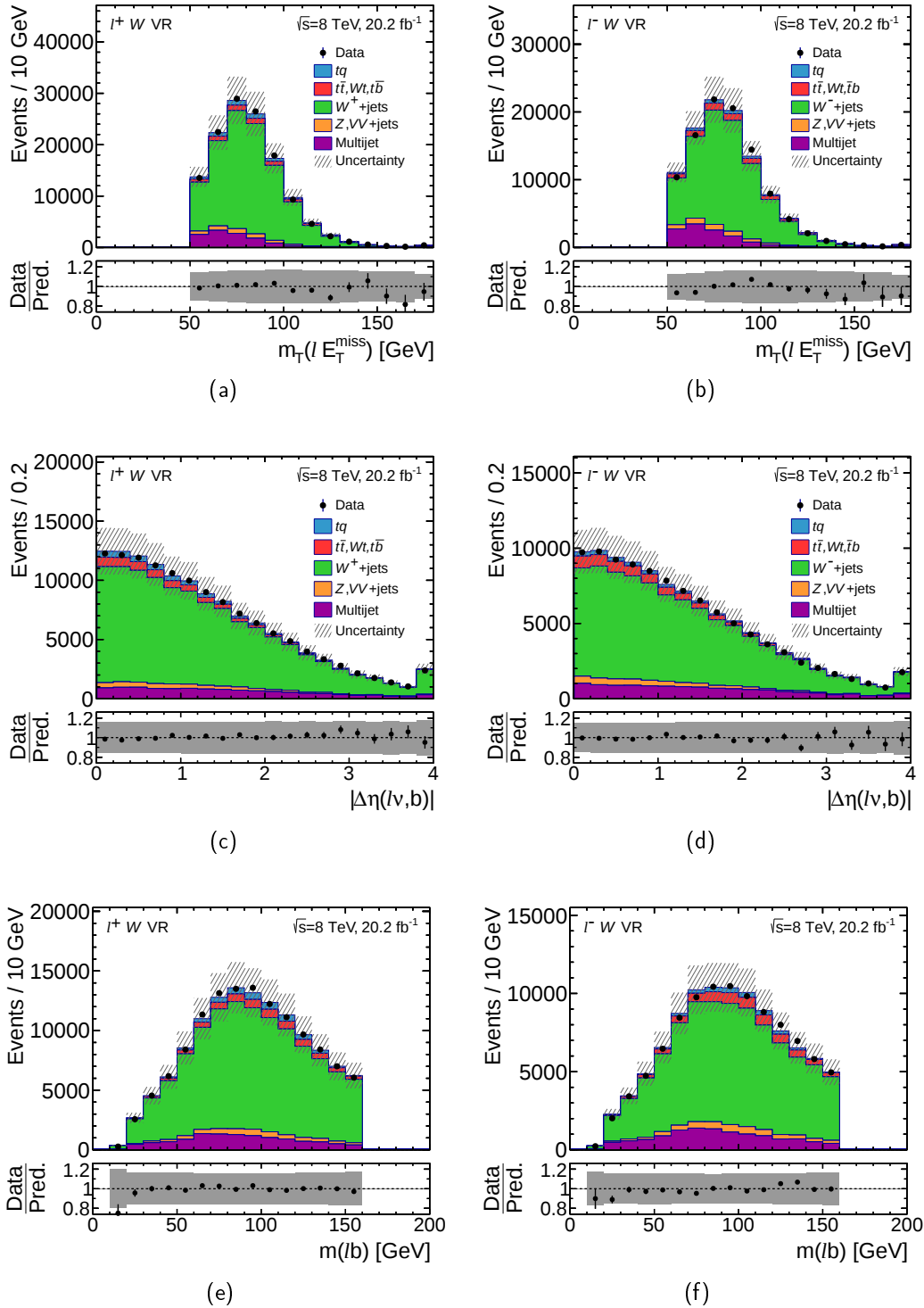
Figure 7.10.: Distributions normalised to the number of expected events of the discriminating variables m_T(\ell E_T^{\text{miss}}) , |\Delta\eta(\ell\nu, b)| and m(\ell b) for the \ell^+ channel (left) and \ell^- channel (right) in the W + \text{jets} VR. The hatched uncertainty band represents the uncertainty in the pre-fit process cross-sections and the bin-by-bin MC statistical uncertainty, added in quadrature. The ratio of observed to predicted (Pred.) number of events in each bin is shown in the lower panel. Events beyond the axis range are included in the last bin.
