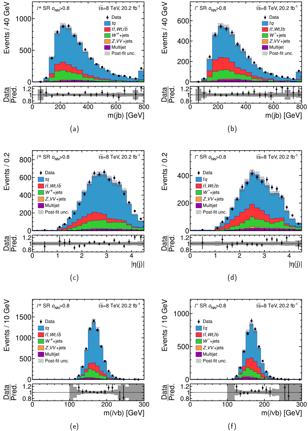
Figure 8.7.: The observed distribution of the three most discriminating input variables in the signal region +O_{NN} > 0.8 of (left) the \ell^+ channel and (right) the \ell^- channel is compared to the distribution of simulated signal and background events normalised to the number of fitted events. The uncertainty band represents the post-fit normalisation uncertainty and the uncertainty due to limited sample size. The ratio between the observed and expected number of events in each bin is shown in the lower panel.
