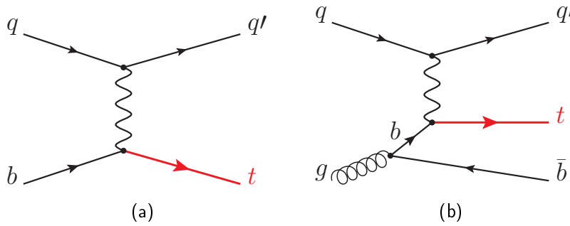
Figure 1.6.: Feynman diagrams of the t -channel single top-quark production modes in the 5 FS (a) and the 4 FS (b).
