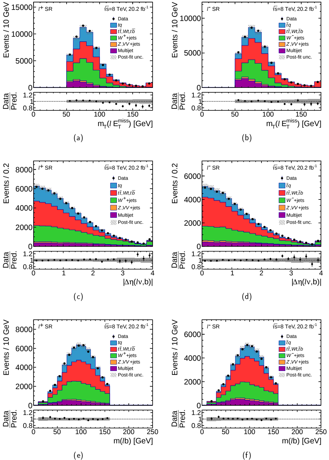
Figure 8.5.: The observed distribution of three input variables in the signal region of (left) the \ell^+ channel channel and (right) the \ell^- channel channel is compared to the distribution of simulated signal and background events normalised to the number of fitted events. The uncertainty band represents the post-fit normalisation uncertainty and the uncertainty due to limited sample size. The ratio between the observed and expected number of events in each bin is shown in the lower panel.
