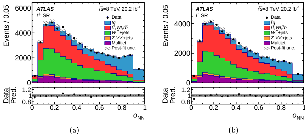
Figure 8.3.: Distributions of the neural network output: The observed distribution in the signal region of (a) the \ell^+ channel channel and (b) the \ell^- channel channel is compared to the distribution of simulated signal and background events normalised to the number of fitted events. The ratio of observed and expected number of events in each bin is shown in the lower panel. The uncertainty band contains the post-fit rate uncertainties for all processes and the MC statistical uncertainty.
