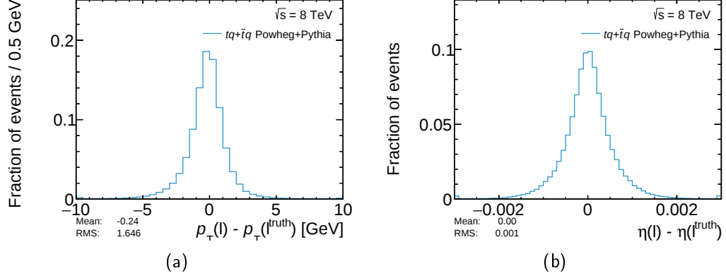
Figure 4.3.: Residual distributions of the lepton ( \ell ) transverse momentum (a) and pseudorapidity (b) for selected leptons of t -channel single top-quark events. The mean values of the distributions correspond to a systematic bias in the reconstruction process. Values beyond the axis range are contained in the first and last bin.
