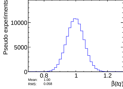
Figure 8.1.: Distribution of \hat{\beta}_{tq}^s for 100000 pseudo experiments considering all sources of systematic uncertainties. The RMS of the distribution corresponds to the relative total systematic uncertainty of the \sigma_{\text{fid}}(tq) measurement.
