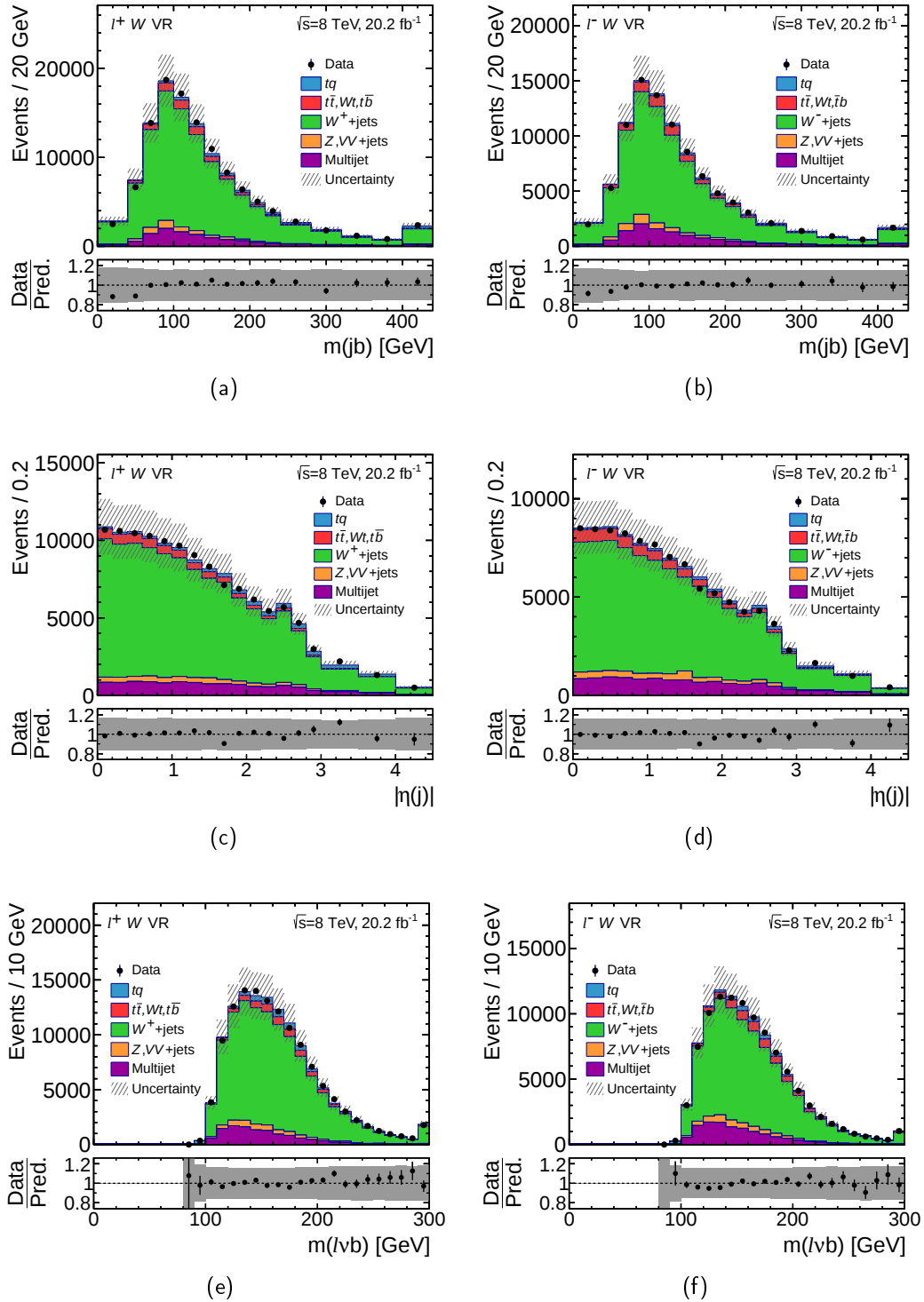
Figure 7.9.: Distributions normalised to the number of expected events of the discriminating variables m(jb) , |\eta(j)| and m(\ell vb) for the \ell^+ channel (left) and \ell^- channel (right) in the W + jets VR. The hatched uncertainty band represents the uncertainty in the pre-fit process cross-sections and the bin-by-bin MC statistical uncertainty, added in quadrature. The ratio of observed to predicted (Pred.) number of events in each bin is shown in the lower panel. Events beyond the axis range are included in the last bin.
