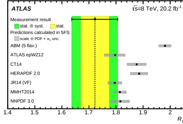
Figure 8.19.: Predicted values of R_t = \sigma_{\text{tot}}(tq)/\sigma_{\text{tot}}(\bar{t}q) calculated with HATHOR [141] at NLO precision in QCD [57] in the 5 FS using different NLO PDF sets [33, 163, 31, 39, 32, 35, 37] compared to the measured value. The error bars on the predictions include the uncertainty on the renormalisation and factorisation scales and the combined internal PDF and \alpha_s uncertainty. The dashed black line indicates the central value of the measured R_t value. The combined statistical and systematic uncertainty of the measurement is shown in green, while the statistical uncertainty is represented by the yellow error band. The uncertainty on the measured R_t value does not include the PDF components for this comparison.
