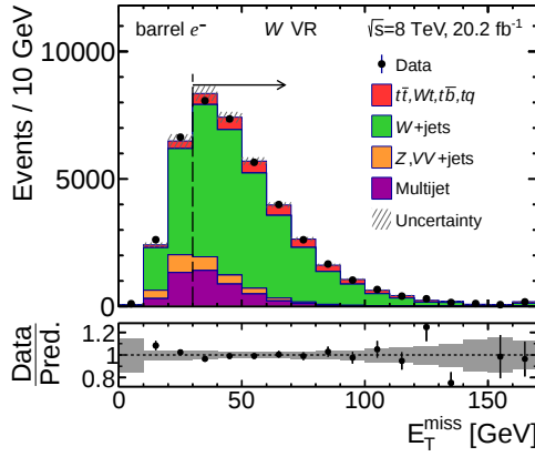
(c) Barrel electron channel in the W + jets VR.
