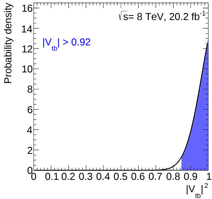
Figure 8.21.: Probability density function of the squared CKM matrix-element |V_{tb}| , assuming |V_{tb}| < 1 . A lower limit on the value of |V_{tb}|^2 is extracted at 95% confidence level (blue area) to be |V_{tb}|^2 > 0.85 , which corresponds to a lower limit of |V_{tb}| > 0.92 .
