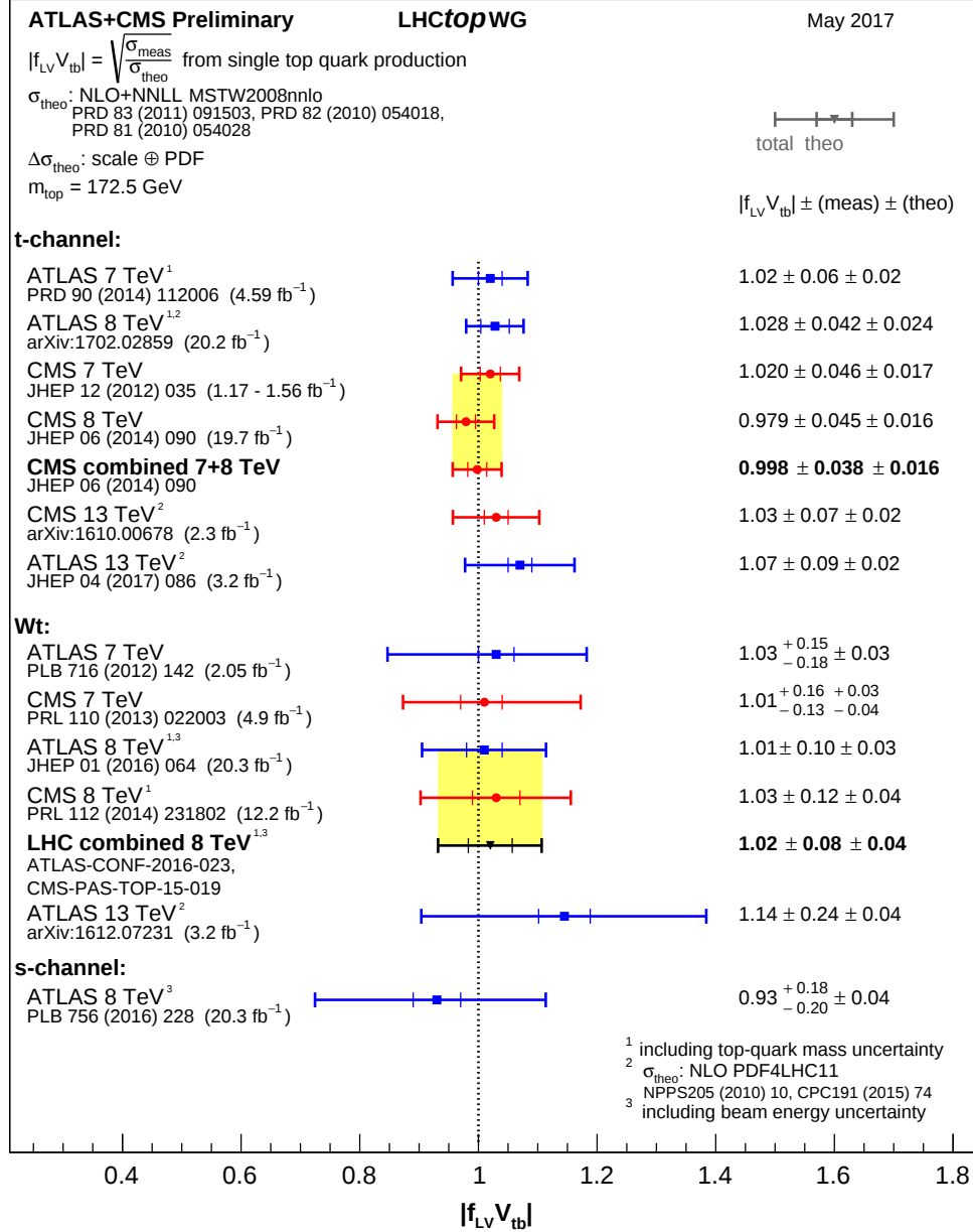
Figure 9.3.: Summary of measurements of the CKM matrix-element f_{LV} \cdot |V_{tb}| performed by ATLAS and CMS for all three single top-quark production modes and for 7,8 and 13 TeV center-of-mass energies [165].
