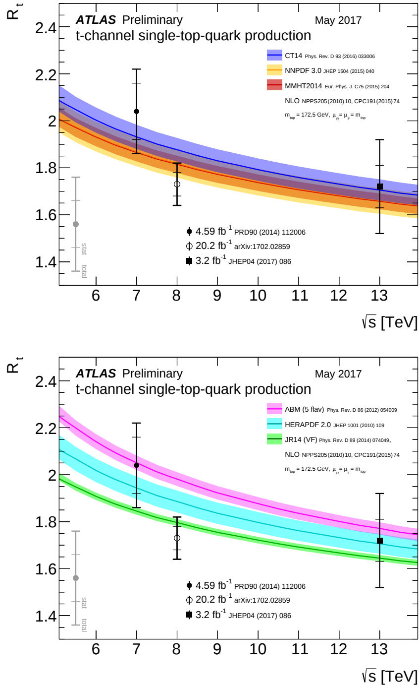
Figure 9.2.: The measured cross-section ratios at 7 and 13 TeV [165] are compared to this result. In (a) the measurements are compared to the main PDF-sets and to additional PDF sets in (b).
