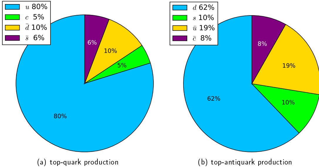
Figure 3.3.: Flavour fractions of initial light quarks in t -channel single top-quark production as determined by MC events generated with ACERMC + PYTHIA 6. (a) shows the flavour fractions in top-quark production, which is dominated by 80% of u quarks. (b) shows the corresponding fractions of the top-antiquark production. In case of the fractions of initial light quarks in top-antiquark production initial d -quarks are only dominating by 62%.
