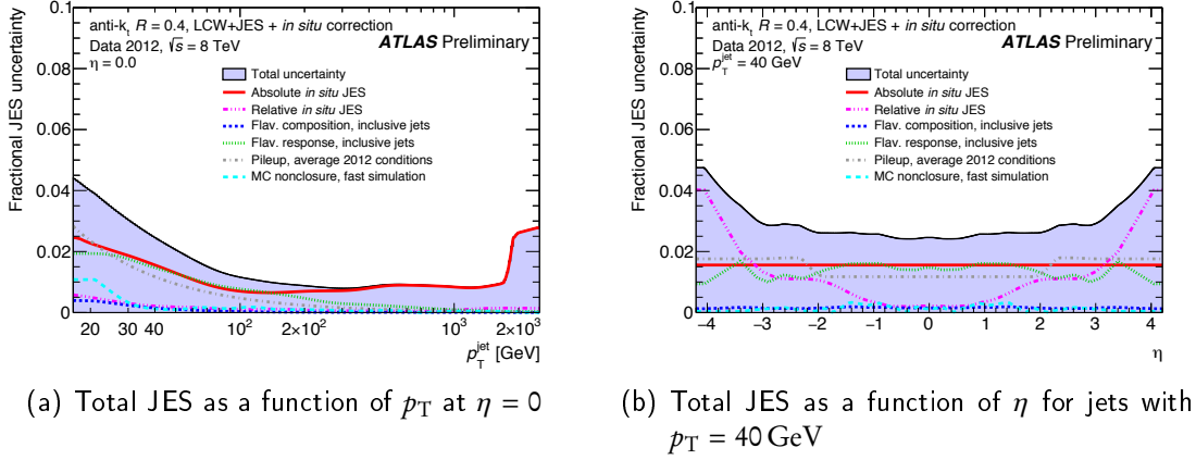
Figure 8.8.: Total JES as a function of p_T in (a) and \eta in (b). The individual contributions are added in quadrature. The contribution of the jet-flavour uncertainty corresponds to a gluon-jet fraction of 50 % and an uncertainty in this fraction of 50 % [155].
