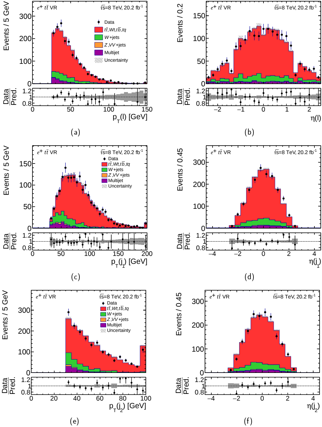
Figure 5.13.: Kinematic distributions in the t\bar{t} VR for the e^+ channel. (a) p_T and (b) \eta of the electron, (c) p_T and (d) \eta of the leading jet and, (e) p_T and (f) \eta of the sub-leading jet. The hatched error band represents the uncertainty on the multijet rate as well as the MC statistical uncertainty. The ratio of observed to predicted (Pred.) number of events in each bin is shown in the lower panel. Events beyond the axis range are included in the last bin.
