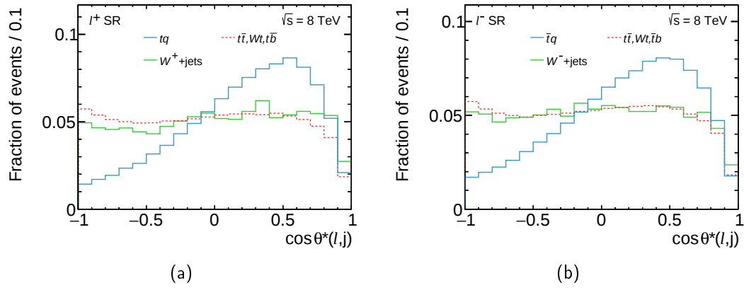
Figure 7.7.: Distributions normalised to unit area of the discriminating variable \cos\theta^*(\ell, j) for the \ell^+ channel (left) and \ell^- channel (right) in the SR.
