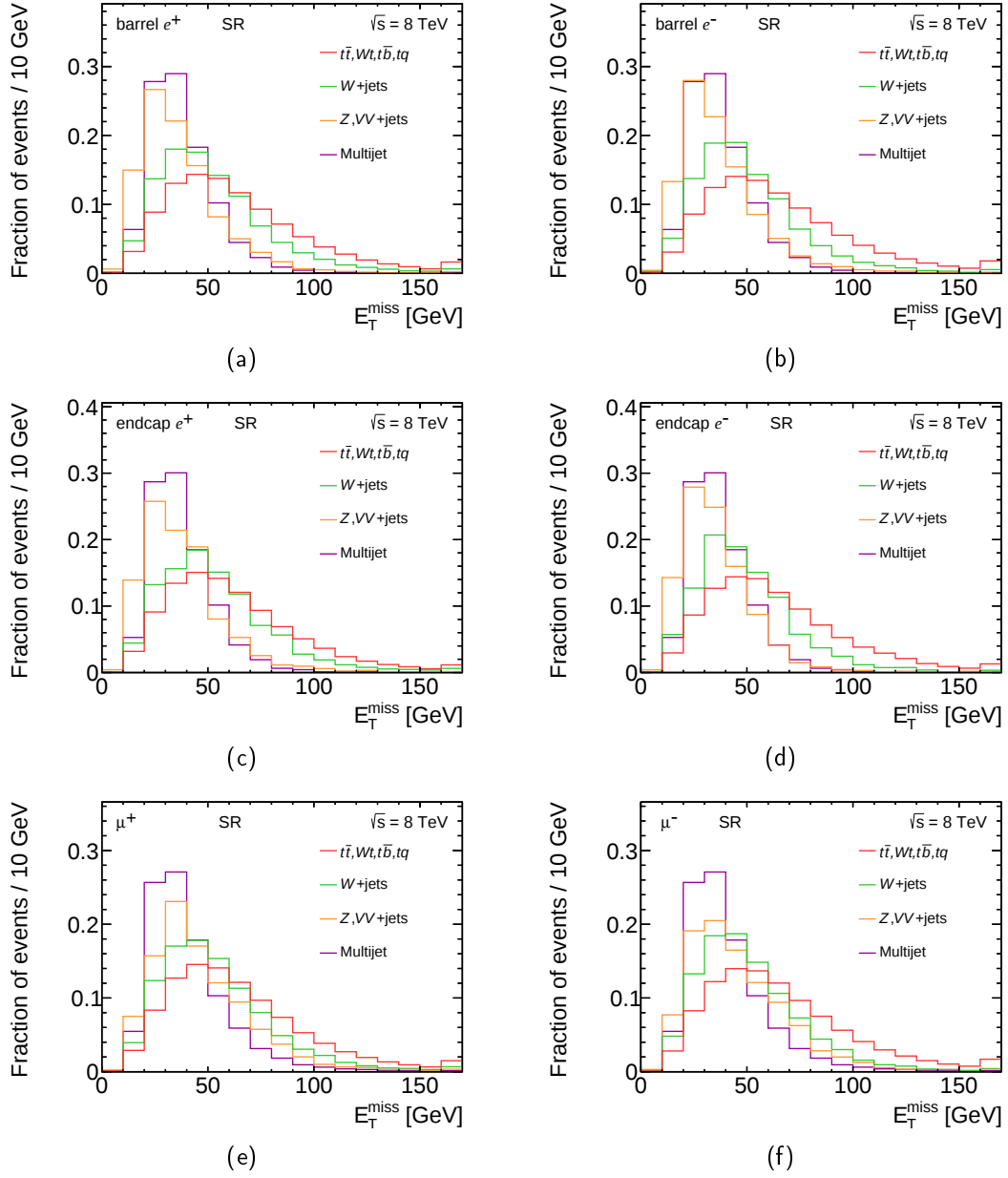
Figure 5.4.: Template E_T^{\text{miss}} distributions in the signal region. All distributions are normalised to unit area.
