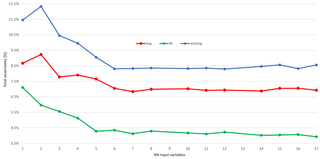
Figure 7.3.: Total systematic uncertainties as a function of the number of NN input variables. The total systematic uncertainty on the fiducial cross-section of top-quark production, top-antiquark production and the cross-section ratio R_t is shown.
