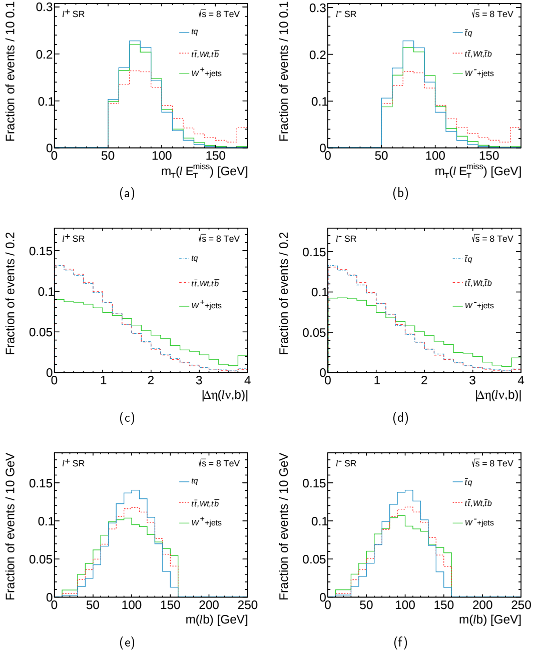
Figure 7.6.: Distributions normalised to unit area of the discriminating variables m_T(\ell E_T^{\text{miss}}) , |\Delta\eta(\ell\nu, b)| and m(\ell b) for the \ell^+ channel (left) and \ell^- channel (right) in the SR.
