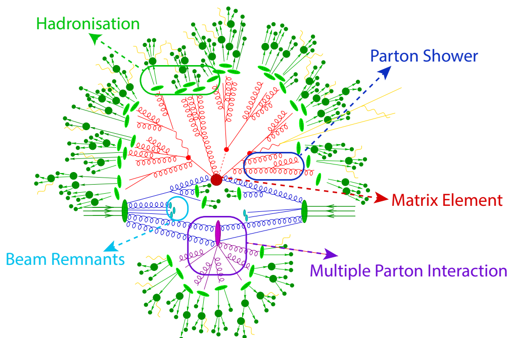
Figure 3.2.: Sketch of a hadron-hadron collision as simulated by a Monte-Carlo event generator. The generation of a Higgs boson in association with a t\bar{t} pair ( t\bar{t}h ) and the subsequent decay is illustrated. The red big circle indicates the hard process simulated by the ME part of the simulation, including initial/final state gluon radiation, indicated in red. The parton shower (PS) generator part of the simulation is indicated by the blue box, followed by the hadronisation exemplary shown in the green box. Parton-to-hadron transitions are indicated in light green, while soft photon radiation is represented in yellow. In addition, the beam remnants are indicated with the cyan box, and the purple box shows an example of multi parton interaction (MPI). [83]
