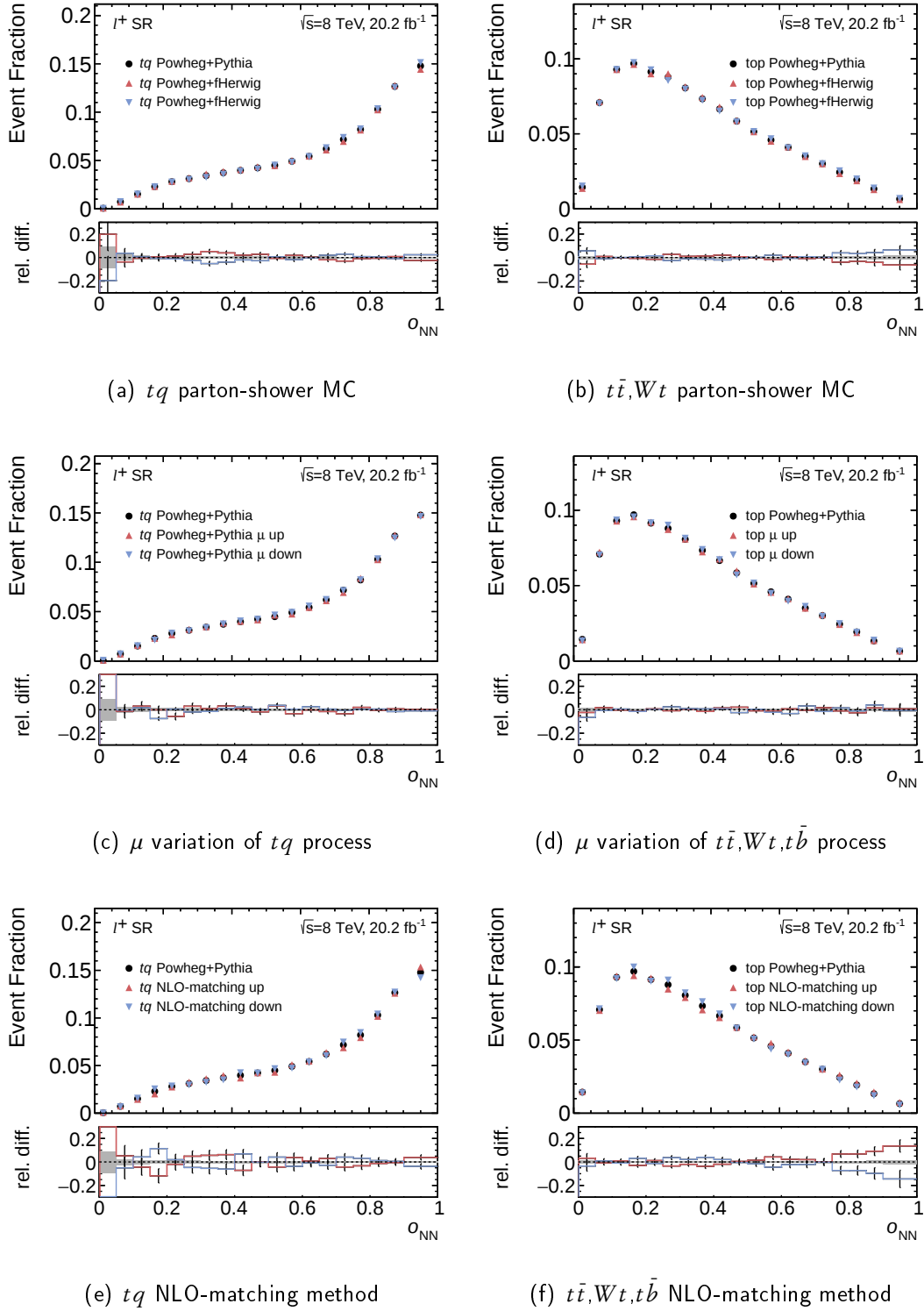
Figure 8.12.: The template shape components of the signal-modeling (left) and top-background modeling (right) uncertainties in the \ell^+ channel.
