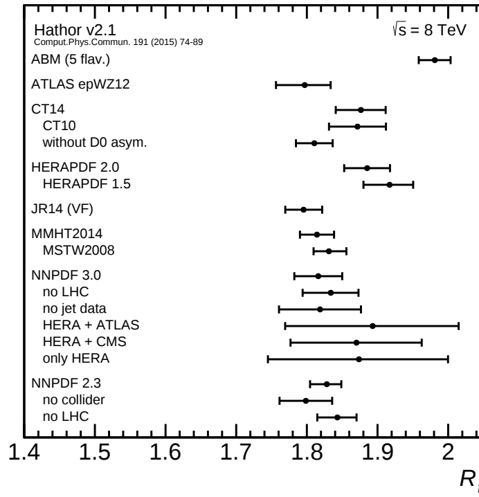
Figure 6.2.: Values of R_t calculated for different NLO PDF sets. The errors contain the uncertainty on the renormalisation and factorisation scale, the internal PDF uncertainty, and the uncertainty on \alpha_s .
