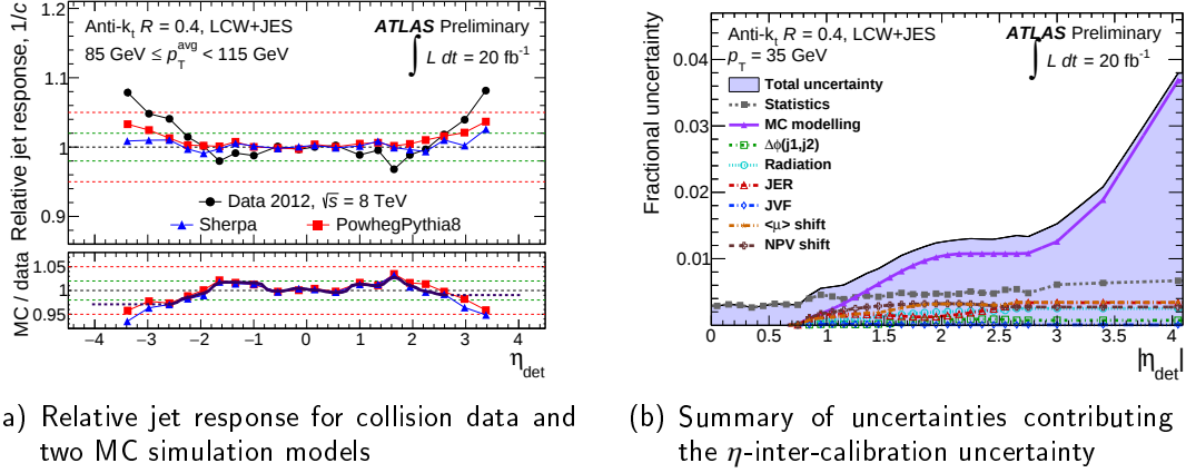
Figure 8.10.: Relative jet response for the SHERPA and POWHEG-BOX + PYTHIA 8 MC generators compared to data in (a) and the summary of contributions to the \eta -inter-calibration uncertainty (b). The individual contributions are added in quadrature. [156].
