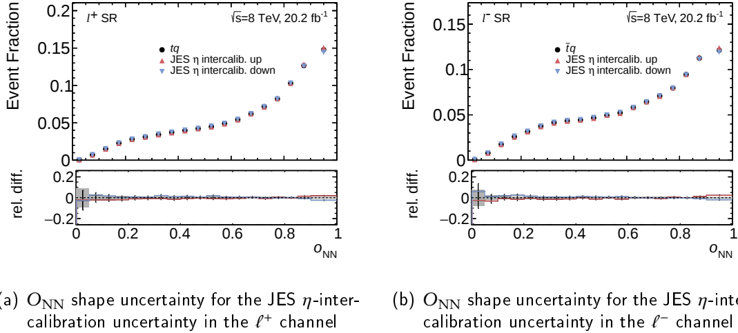
Figure 8.11.: Template shape uncertainty of the JES \eta -inter-calibration uncertainty in the \ell^+ channel (a) and the \ell^- channel (b).
