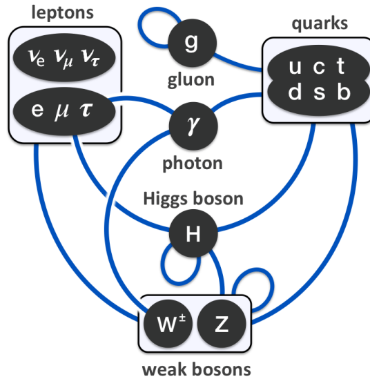
Figure 1.2.: Summary of the Standard Model interactions [18].
