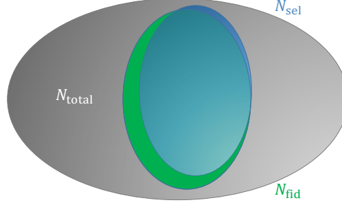
Figure 6.1.: Illustration of the relation of the total phase space (grey), the fiducial volume (green) and the reconstructed phase space (blue). The quantity N_{\text{total}} refers to the total number of expected events and N_{\text{sel}} refers to the number of expected events selected in the reconstructed phase space, as well as N_{\text{fid}} which refers to the number of expected events in the fiducial volume.
