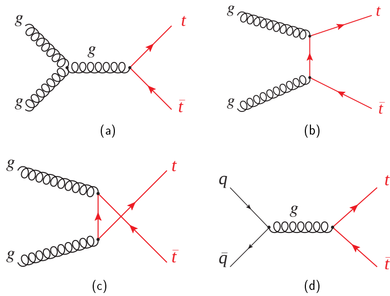
Figure 1.4.: Feynman diagrams of the dominant t\bar{t} production modes. (a)-(c) are gluon fusion induced processes, while (d) shows the production via q\bar{q} annihilation.
