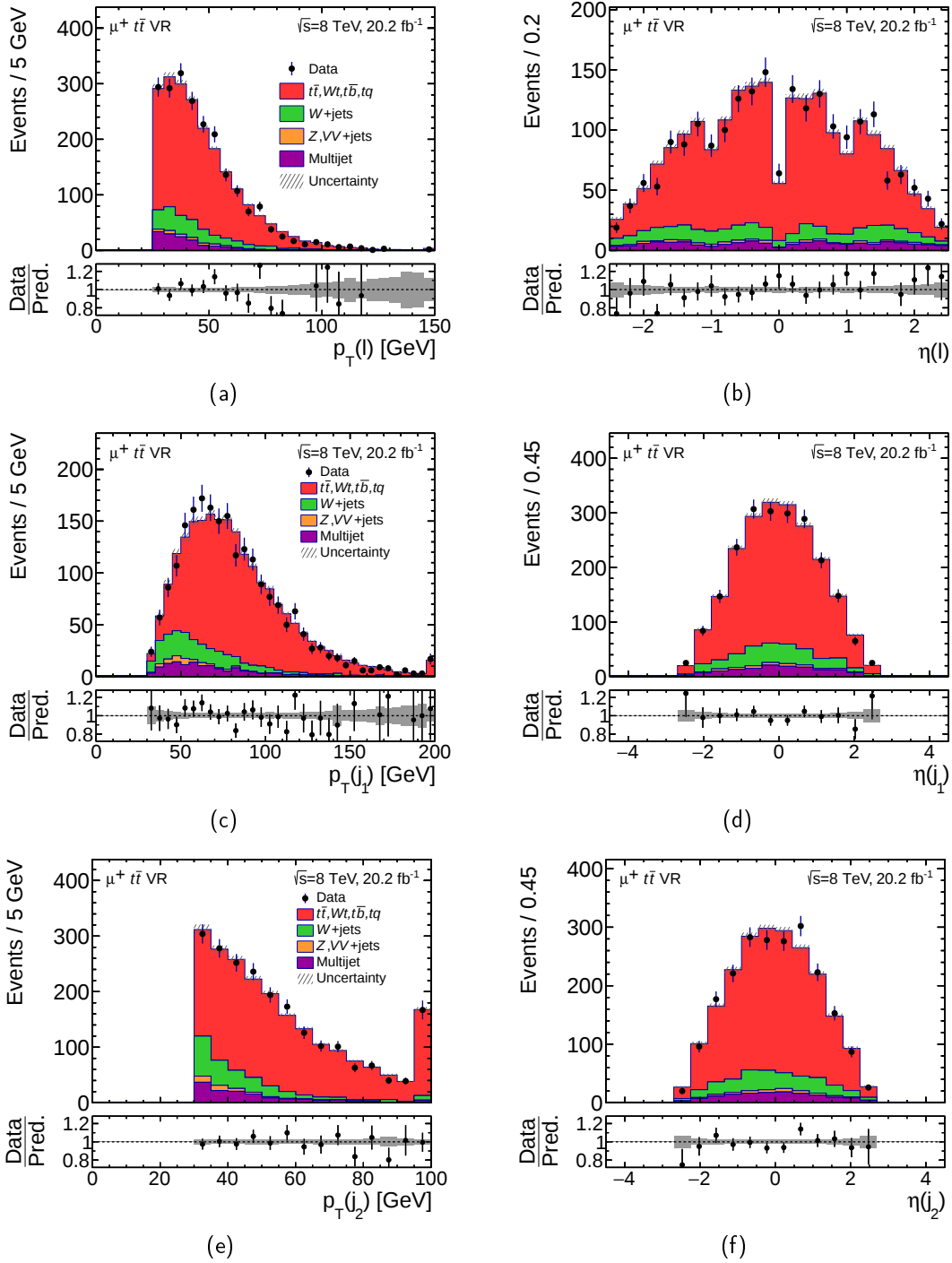
Figure 5.15.: Kinematic distributions in the t\bar{t} VR for the \mu^+ channel. (a) p_T and (b) \eta of the muon, (c) p_T and (d) \eta of the leading jet and, (e) p_T and (f) \eta of the sub-leading jet. The hatched error band represents the uncertainty on the multijet rate as well as the MC statistical uncertainty. The ratio of observed to predicted (Pred.) number of events in each bin is shown in the lower panel. Events beyond the axis range are included in the last bin.
