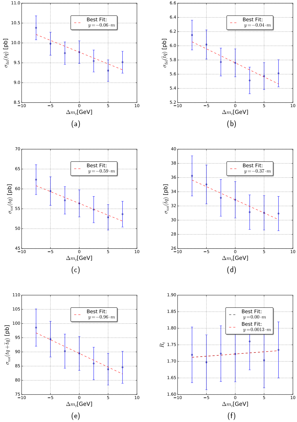
Figure 8.20.: Single top-quark t -channel cross-section dependence of the top-quark mass.
