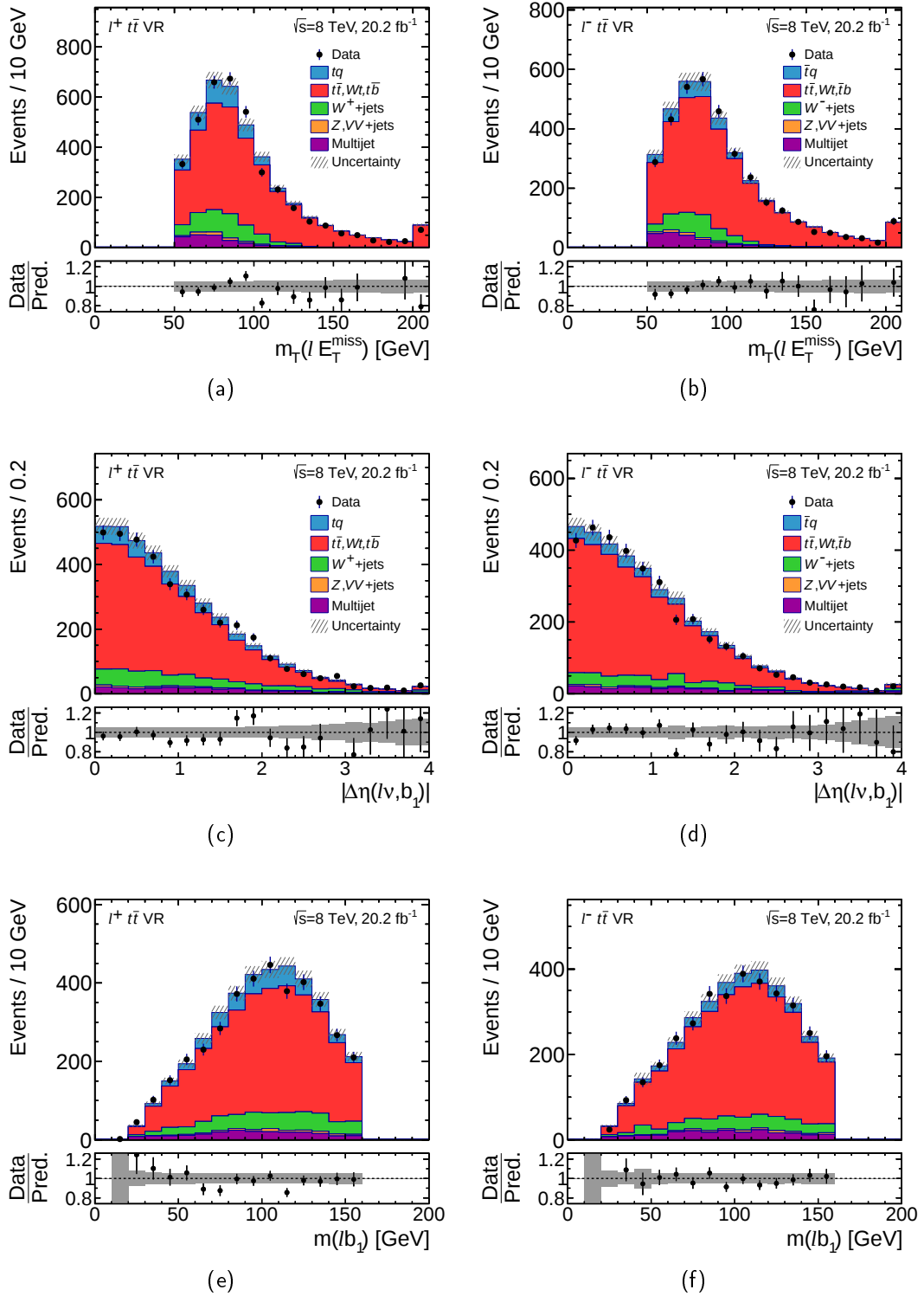
Figure 7.13.: Distributions normalised to the number of expected events of the discriminating variables m_T(\ell E_T^{\text{miss}}) , |\Delta\eta(\ell\nu, b)| and m(\ell b) for the \ell^+ channel (left) and \ell^- channel (right) in the t\bar{t} VR. The hatched uncertainty band represents the uncertainty in the pre-fit process cross-sections and the bin-by-bin MC statistical uncertainty, added in quadrature. The ratio of observed to predicted (Pred.) number of events in each bin is shown in the lower panel. Events beyond the axis range are included in the last bin.
