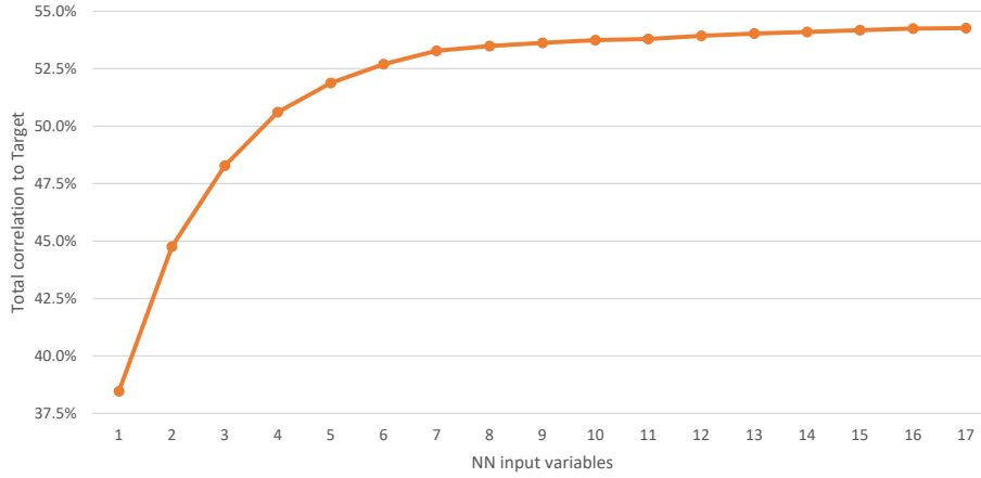
Figure 7.2.: The total correlation-to-target quantity as a function of the number of NN input variables.
