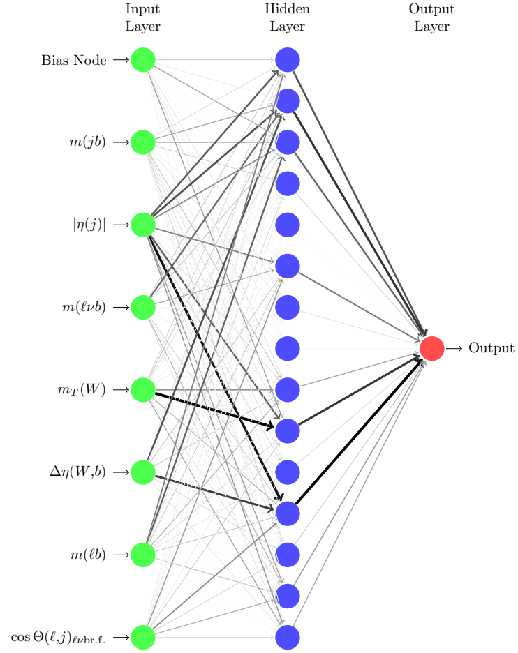
Figure 7.4.: Final network configuration. The width of the lines correspond to the weights between the nodes.
