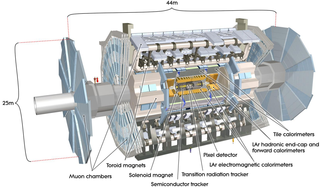
Figure 2.2.: Cut-away view of the ATLAS detector. The dimensions of the detector are 25 m in height and 44 m in length [2].
