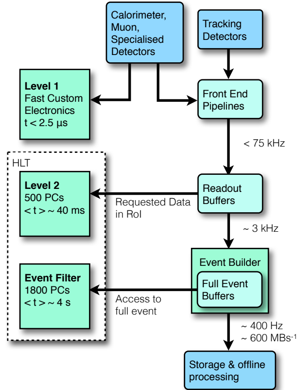
Figure 2.4.: Illustration of the ATLAS trigger system [79]. The individual trigger stages and the technical infrastructure are indicated with the approximate event rate demands. The displayed rates correspond to the 2011 data-taking period.
