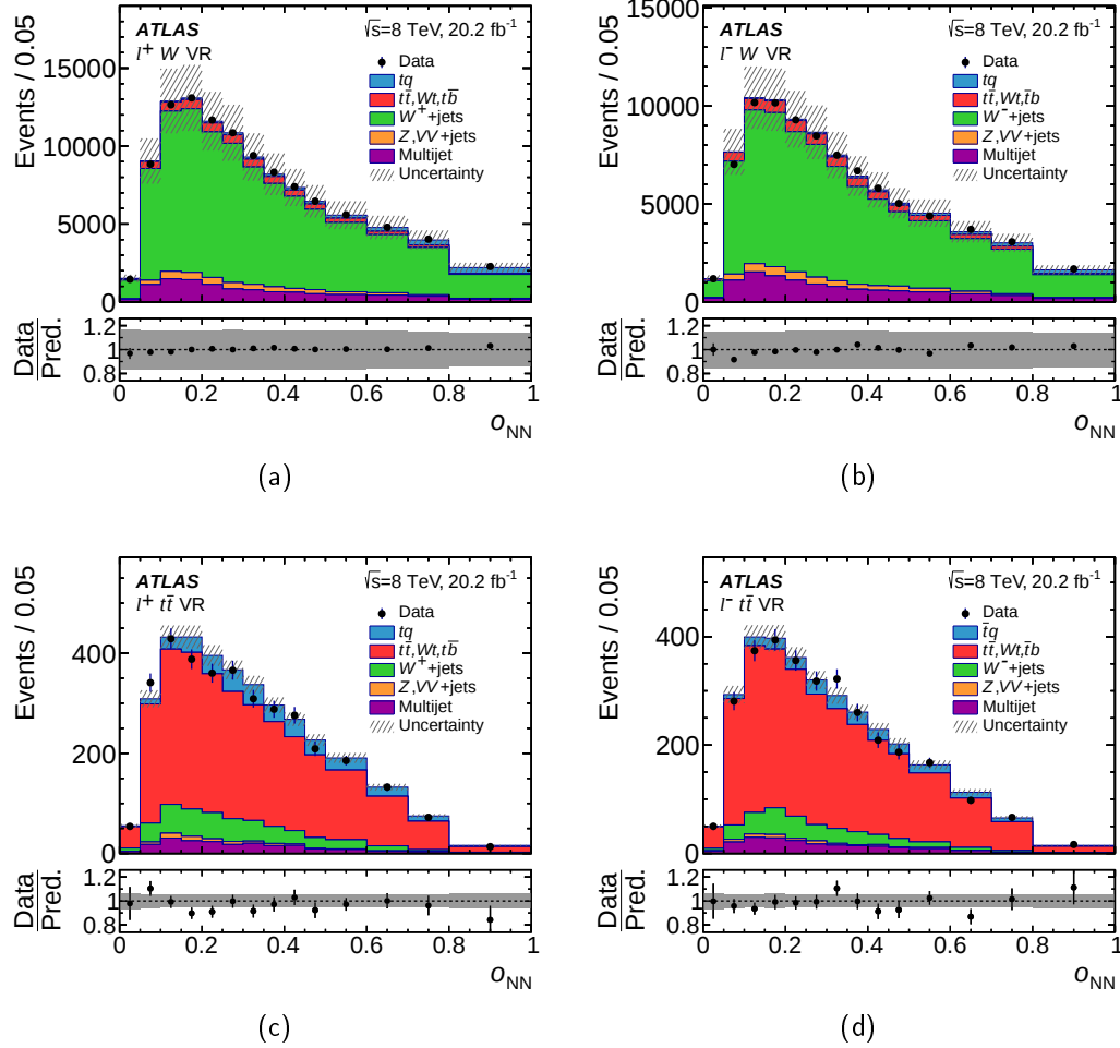
Figure 7.15.: Distributions of the neural network output: Distributions normalised to the number of expected events of the discriminating variables for the \ell^+ channel (left) and \ell^- channel (right) in the W +jets VR (top) and the t\bar{t} VR (bottom). The hatched uncertainty band represents the uncertainty in the pre-fit process cross-sections and the bin-by-bin MC statistical uncertainty, added in quadrature. The ratio of observed to predicted (Pred.) number of events in each bin is shown in the lower panel.
