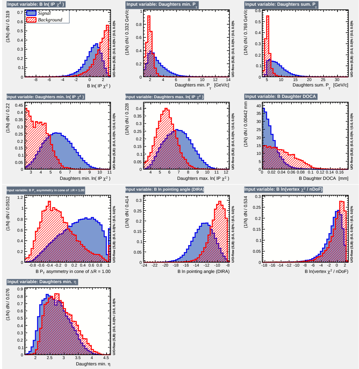
Figure 4.6: Distributions of the TMVA input discriminating variables for 2012 B^0 \rightarrow p\bar{p} MC signal and even numbered event sideband data samples.
