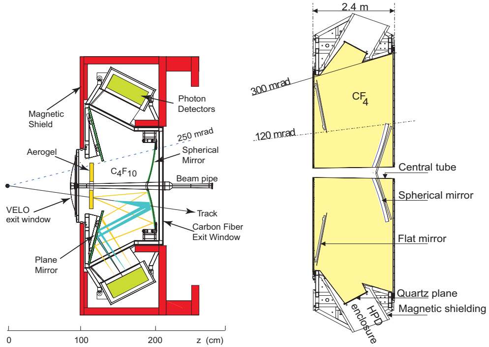
Figure 2.10: Schematic view of the LHCb RICH 1 (left) and RICH 2 (right) detectors. reproduced from [44].
