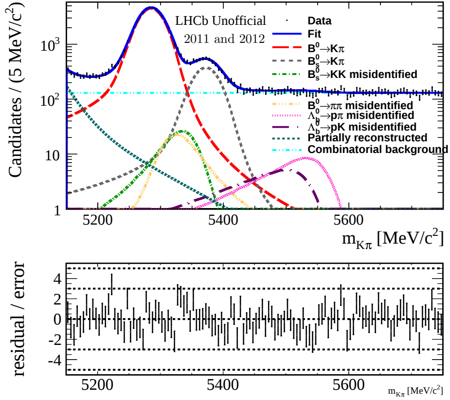
Figure 5.5: Mass fit to the B^0 \rightarrow K^+ \pi^- normalisation channel. The lower plot shows the binned residuals of the fit divided by the fit error. The parameters are extracted from an unbinned maximum likelihood fit, the binning of the data is only for illustration.
