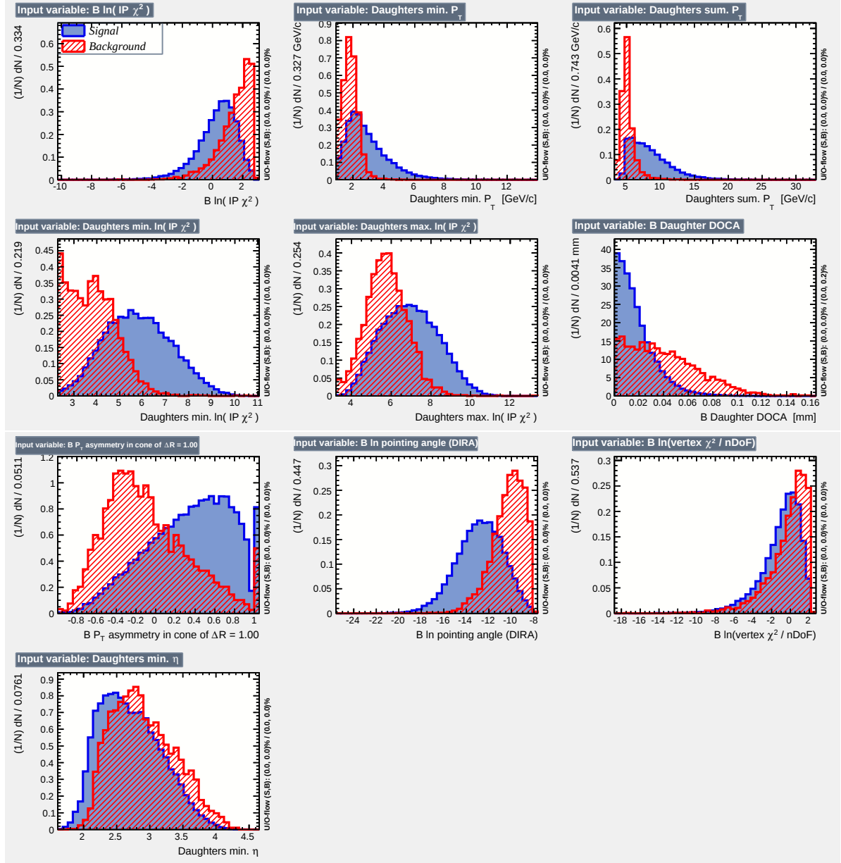
Figure 4.5: Distributions of the TMVA input discriminating variables for 2011 MC signal and even numbered event sideband data samples.
