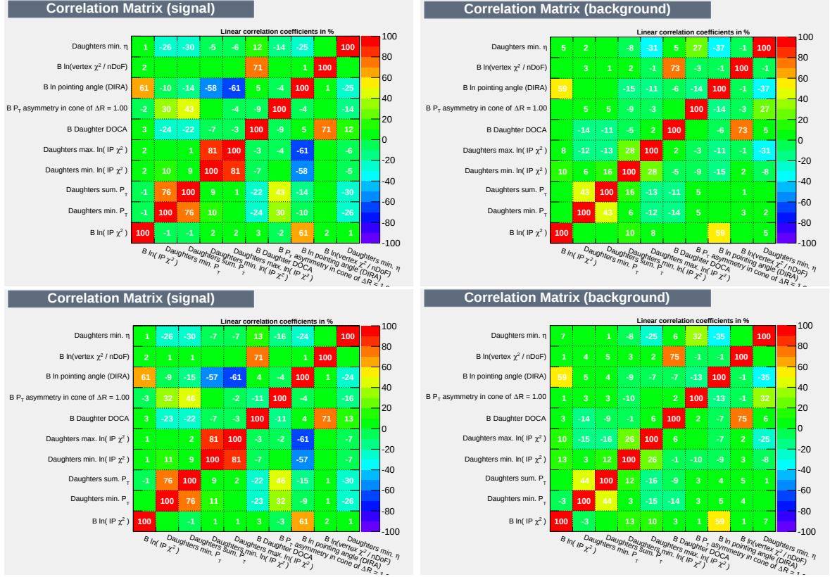
Figure 4.9: Correlation matrices of MVA input variables for B^0 \rightarrow p\bar{p} signal MC (left column) and even numbered event sideband data (right column) samples for 2011 (top row) and 2012 (bottom row).
