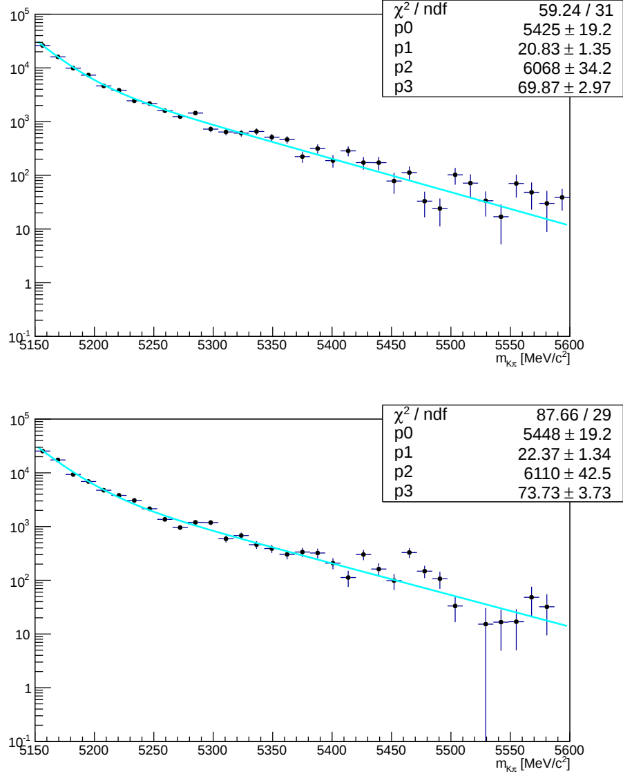
Figure 5.4: The reconstructed K\pi mass distributions of the weighted sum of all contributing partially reconstructed background decays for the K^+\pi^- (top) and \pi^+K^- (bottom) mass hypotheses. The list of decay modes is given in Table 4.2. The fitted linear combination of two exponential distributions is also shown. The listed parameters p1 and p3 give the gradients of the two exponential functions, \nabla_{part}^1 and \nabla_{part}^2 .
