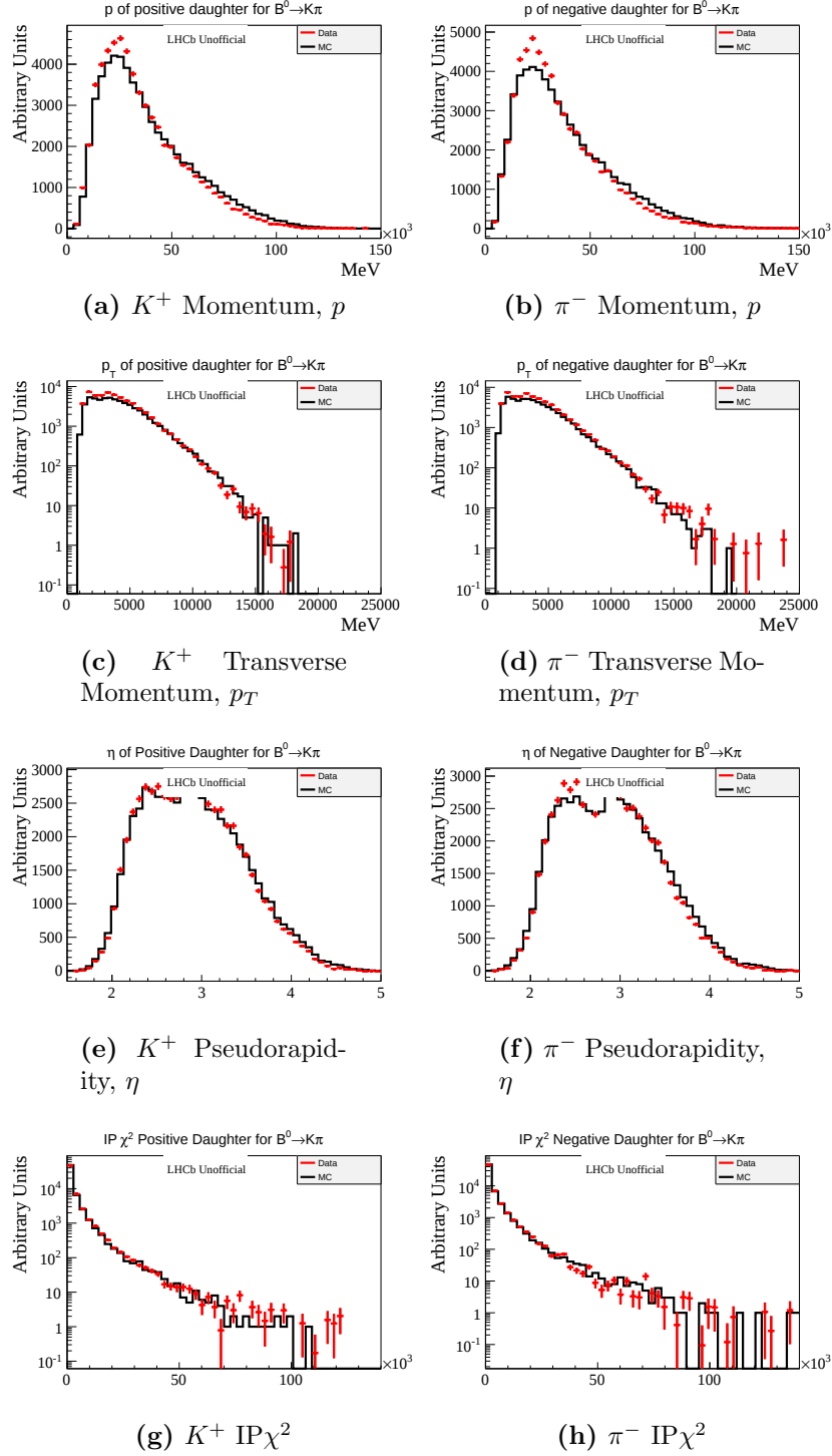
Figure B.3: Distributions of key daughter particle variables for B^0 \rightarrow K^+ \pi^- events. The distributions of data events are shown in red while MC simulation events are shown in black. The data histograms come from sPlots of the B^0 \rightarrow K^\pm \pi^\mp signal peak and the corresponding MC distributions come from the triggered, stripped and PID selected combined 2011 and 2012 MC samples.
