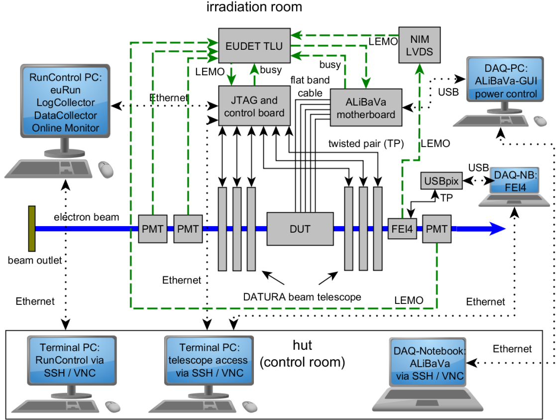
Figure 3.14.: Simplified sketch of DAQ and triggering at DESY. Dashed green lines are trigger signals over coaxial cables and dotted black lines are signal and digital data connections.
