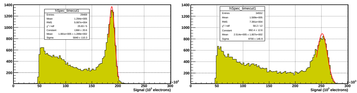
Figure 3.11.: Signal histogram of laser tests. Left: low intensity, right: high intensity Sensor: IFX Irrad, U_{\text{bias}} = -150 \text{ V}
