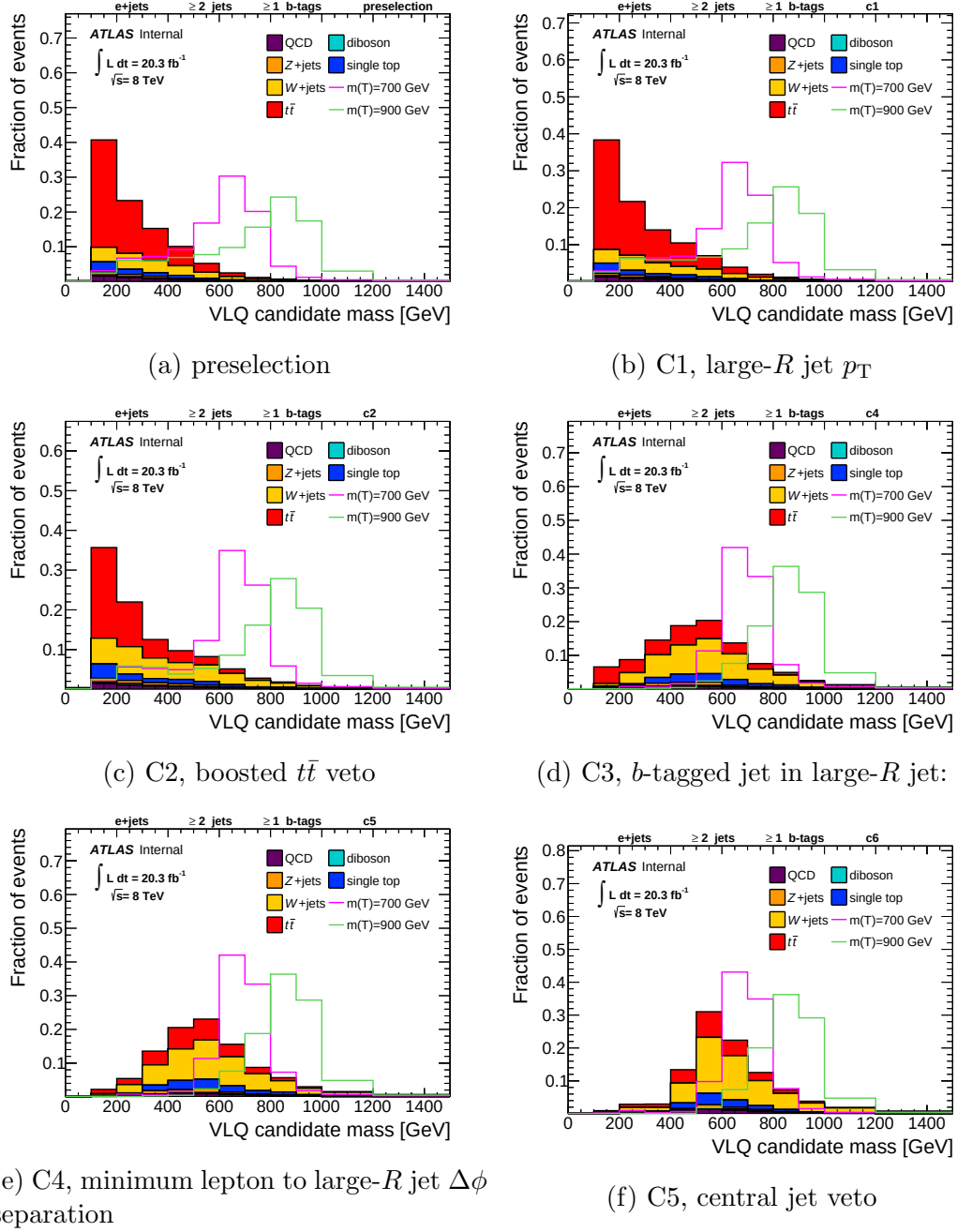
Figure 5.12: Signal to SM background shape-only comparison of the mass of the reconstructed VLQ candidate for the electron channel, after applying in sequence each one of the event selection criteria up to the central jet veto.
