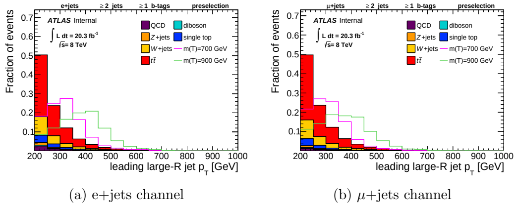
Figure 5.2: Signal to SM background shape-only comparison of the leading large- R jet p_T , both for the electron (left) and muon (right) channels. This is shown for events passing the event preselection.
