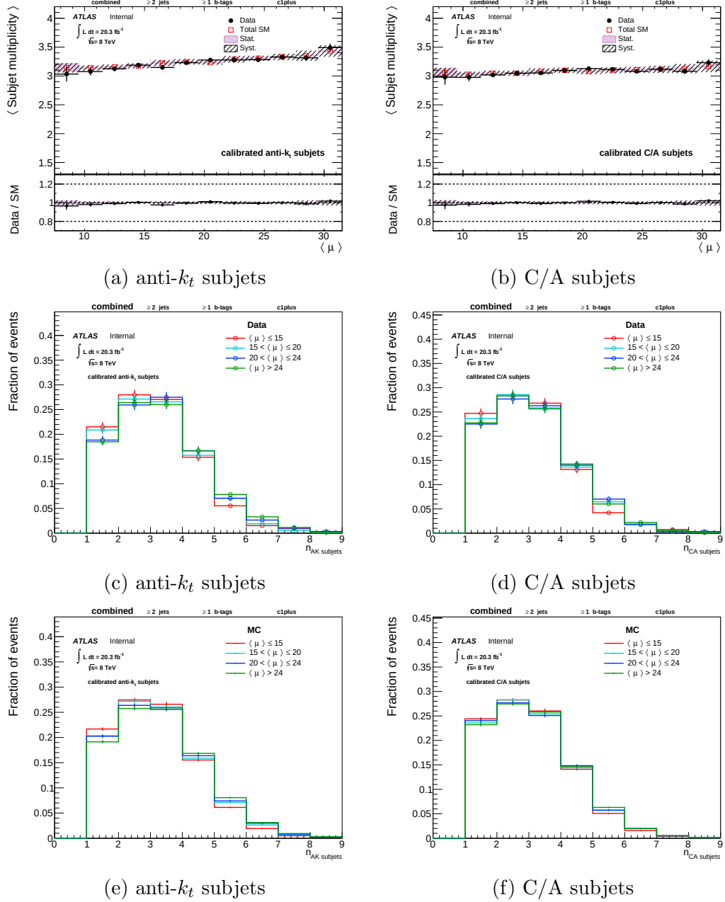
Figure 4.4: Mean subjet multiplicity versus mean number of collisions per bunch crossing \langle\mu\rangle (top). Subjet multiplicity in various \mu bins for data (middle) and MC (bottom). This is shown for calibrated anti- k_t (left) and C/A (right) subjects.
