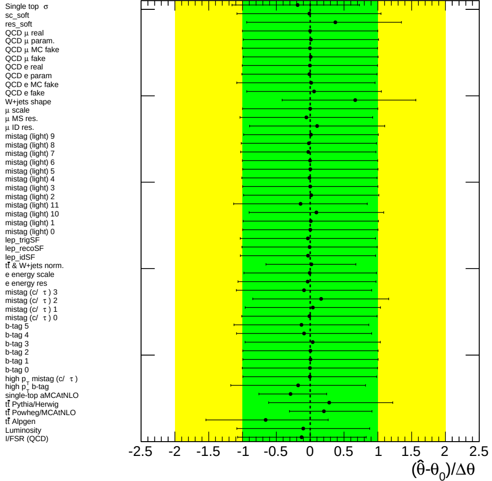
Figure 5.37: Fitted nuisance parameters in the background-only hypothesis. The constraint is given as the difference to the pre-fit \pm 1 values.
