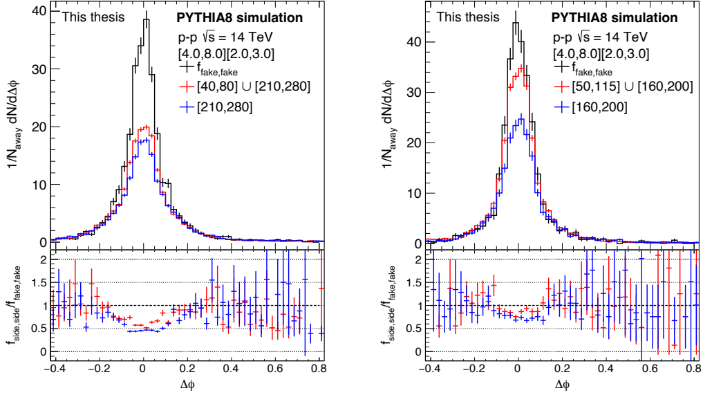
FIGURE 70 Comparison between the sideband correlation f_{\text{side,side}} and the true background correlation from the measured function ( f_{\text{fake,fake}} ). The ratios on the lower panel correspond to the colors on the upper panel.
