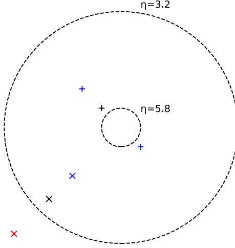
FIGURE 59 Pseudorapidity range visualized in x-y plane. Black markers represent two \pi^0 with same p_T hitting the opposite edges of the acceptance and the colored markers in their vicinity are their decay photons. In both cases, the opening angle is the same but only the inner particle marked with + can be reconstructed since both photons are inside the acceptance.
