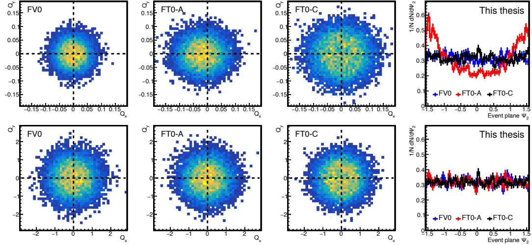
FIGURE 30 Q -vectors and \Psi_2 distributions from the O^2 simulations in centrality 20 – 30% for the three FIT detectors. The raw distributions are shown on the top row while the distributions after the corrections are on the bottom row.
