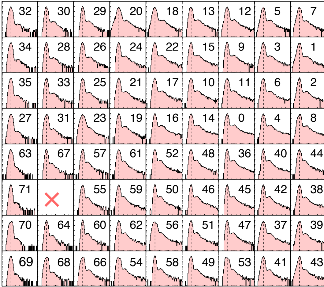
FIGURE 42 ADC distributions after pedestal and common noise subtractions, with isolation cut applied. For each channel, the channel number is presented in the corresponding panel. Channel 65 was not working and is thus marked with a red cross.
