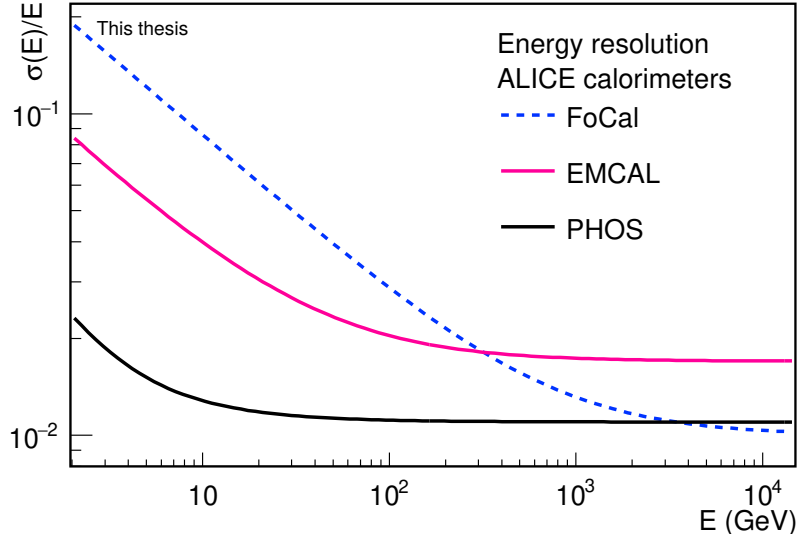
FIGURE 37 The energy resolutions of ALICE calorimeters.
