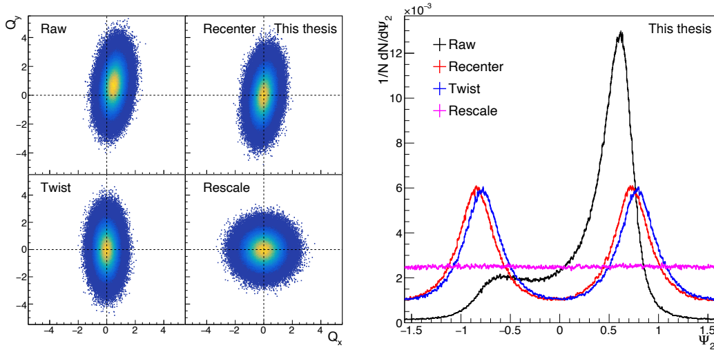
FIGURE 27 Validation of the Q -vector corrections using a toy model. The left side figure shows distributions of Q -vector x and y components after each correction, the top left panel showing the raw distribution. In the right side figure the event plane distribution calculated from the Q -vectors in the four different cases on the left is shown.
