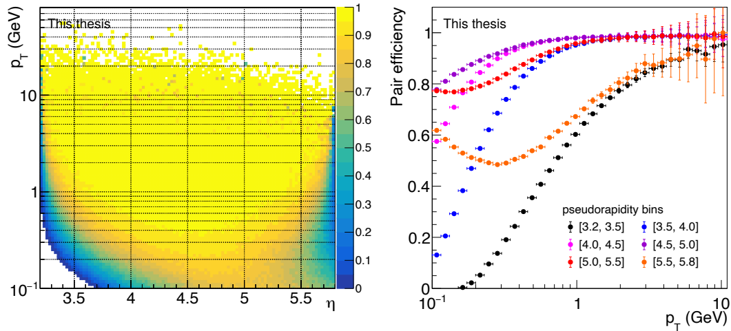
(a) The probability as a function of \pi^0 pseudorapidity (b) The same probability as a function of transverse momentum, divided into several pseudorapidity bins.
