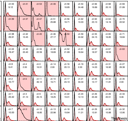
Position scan, 2022 PS testbeam, FoCal-E pad layers, ASIC 17
