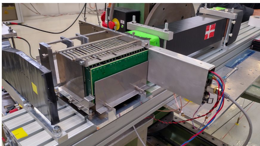
FIGURE 46 The setup of 18 pad layers in the 2022 PS test beam, accompanied by FoCal-H prototype behind it.
