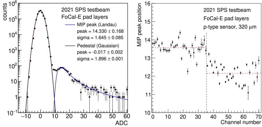
FIGURE 43 Results from the MIP analysis, ADC distribution from CALIB1 (left) and the MIP peak position values from the Landau fit in each channel (right).
