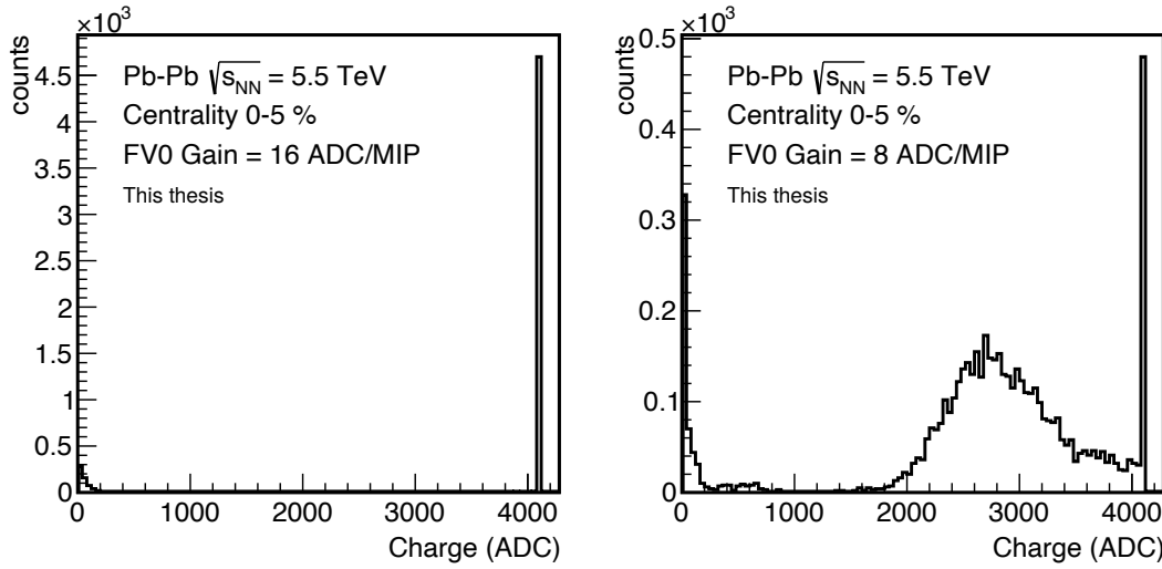
FIGURE 28 Simulated charge from all the FV0 channels with two different gain settings, one MIP corresponding to 16 ADC counts (left) and 8 ADC counts (right).
