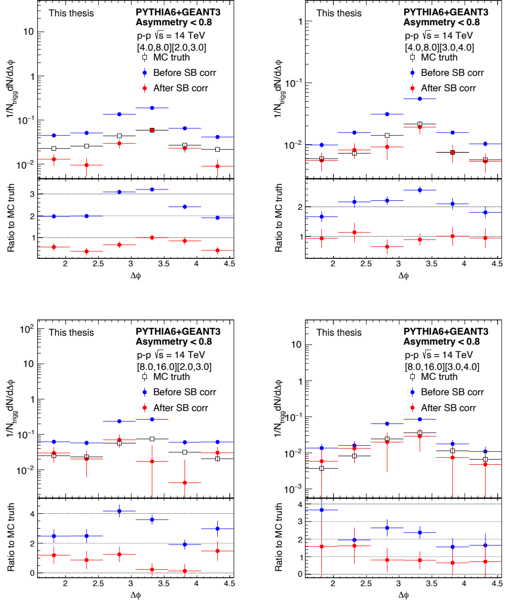
FIGURE 79 The away side of \pi^0 - \pi^0 correlation in four different p_T bins, calculated from clusters reconstructed in FoCal-E.
