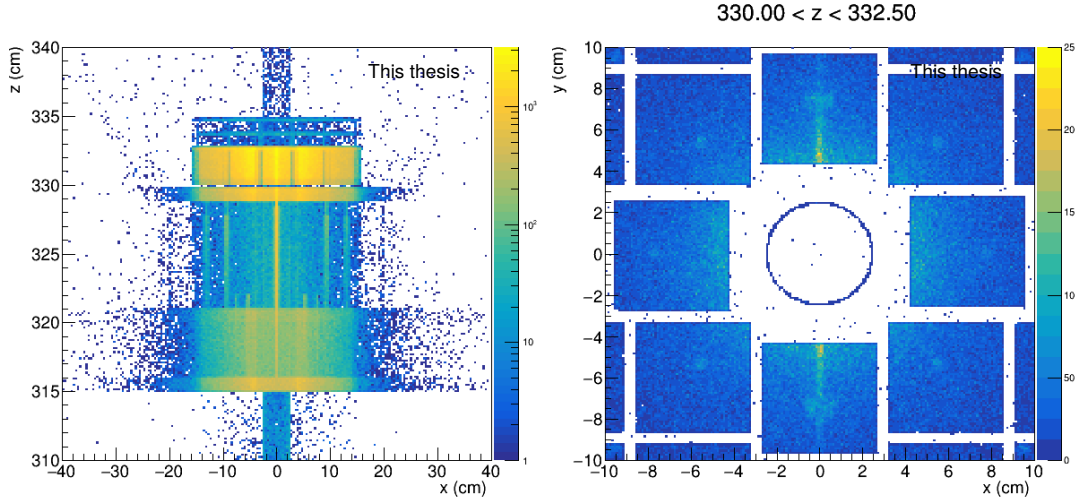
FIGURE 26 Secondary particle production vertices on the A-side (left figure) in which especially the middle part of FV0 case is visible. This can also be seen in the right figure which is a cross section of FT0-A.
